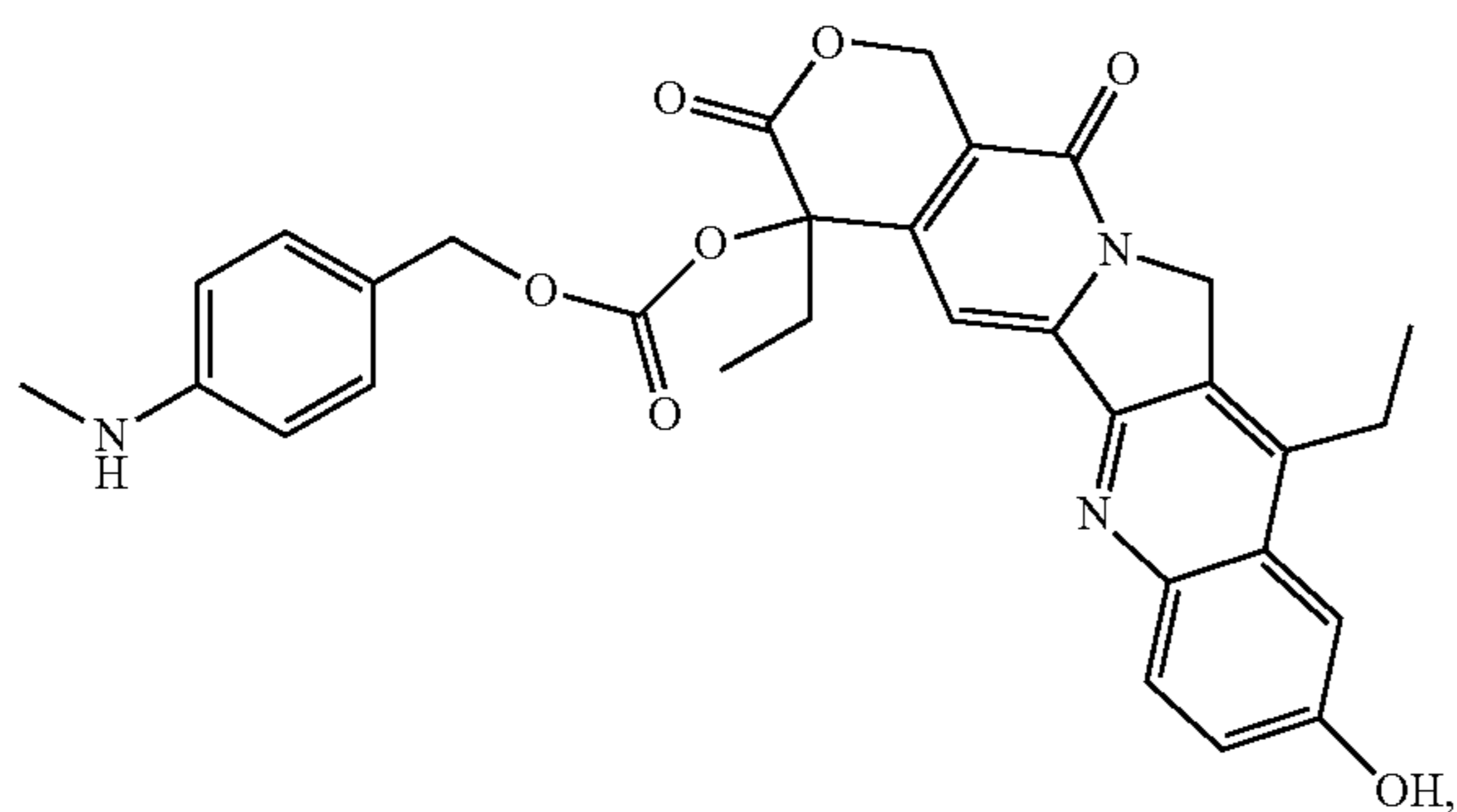
MAb-CL2A-SN-38
