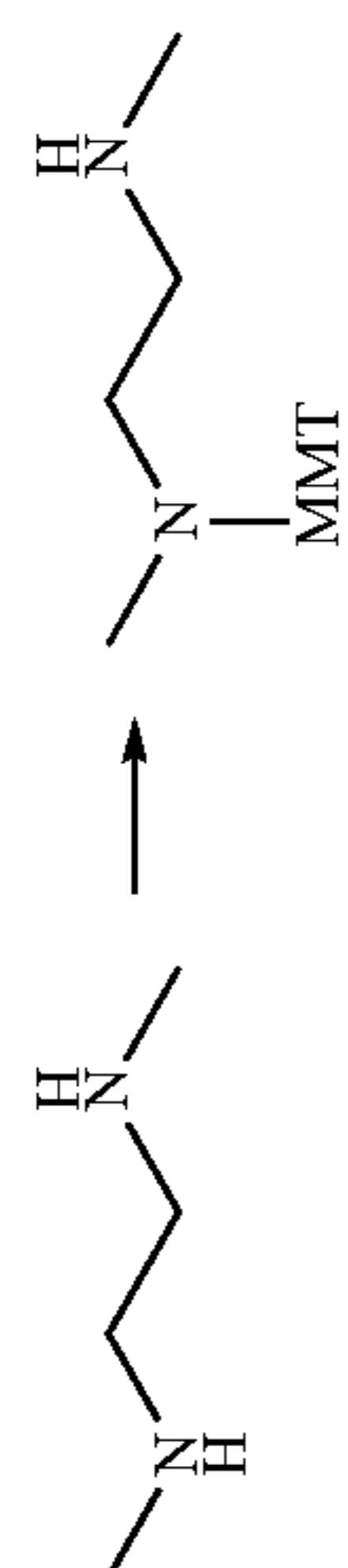
Scheme-4: Preparation of CL2E-SN-38
