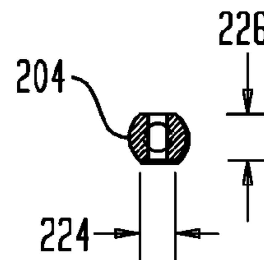
FIG. 30 (SECTION C-C OF FIG. 29)
