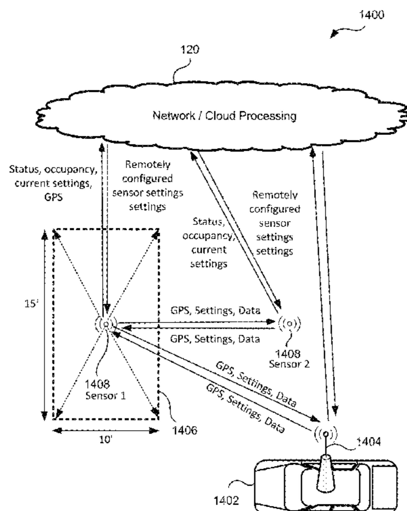
Sensor (on -- boundary set to 10x15 feet virtual parking spot boundary deployed)
