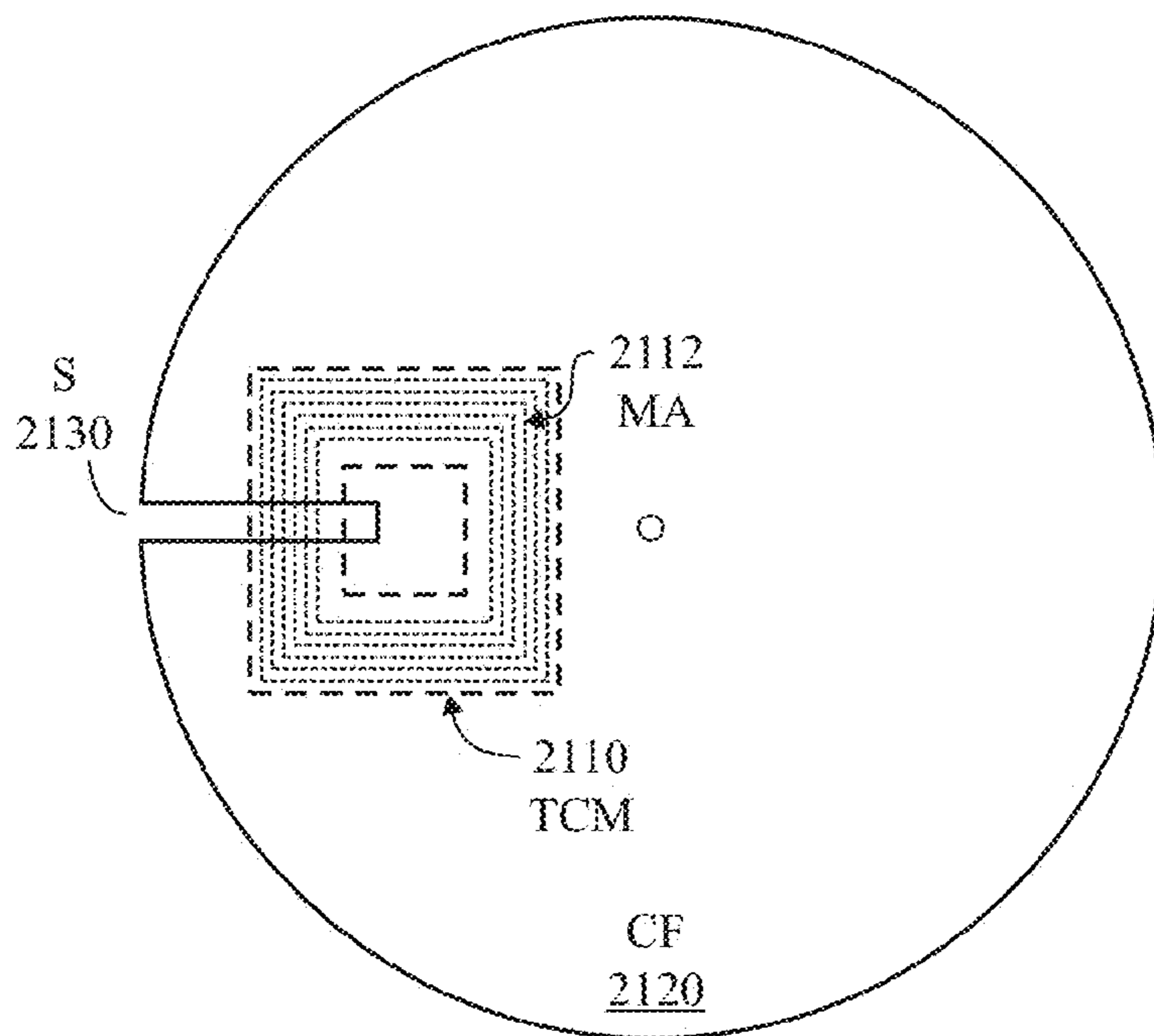
FIG. 21A one CF, one TCM, enabled
