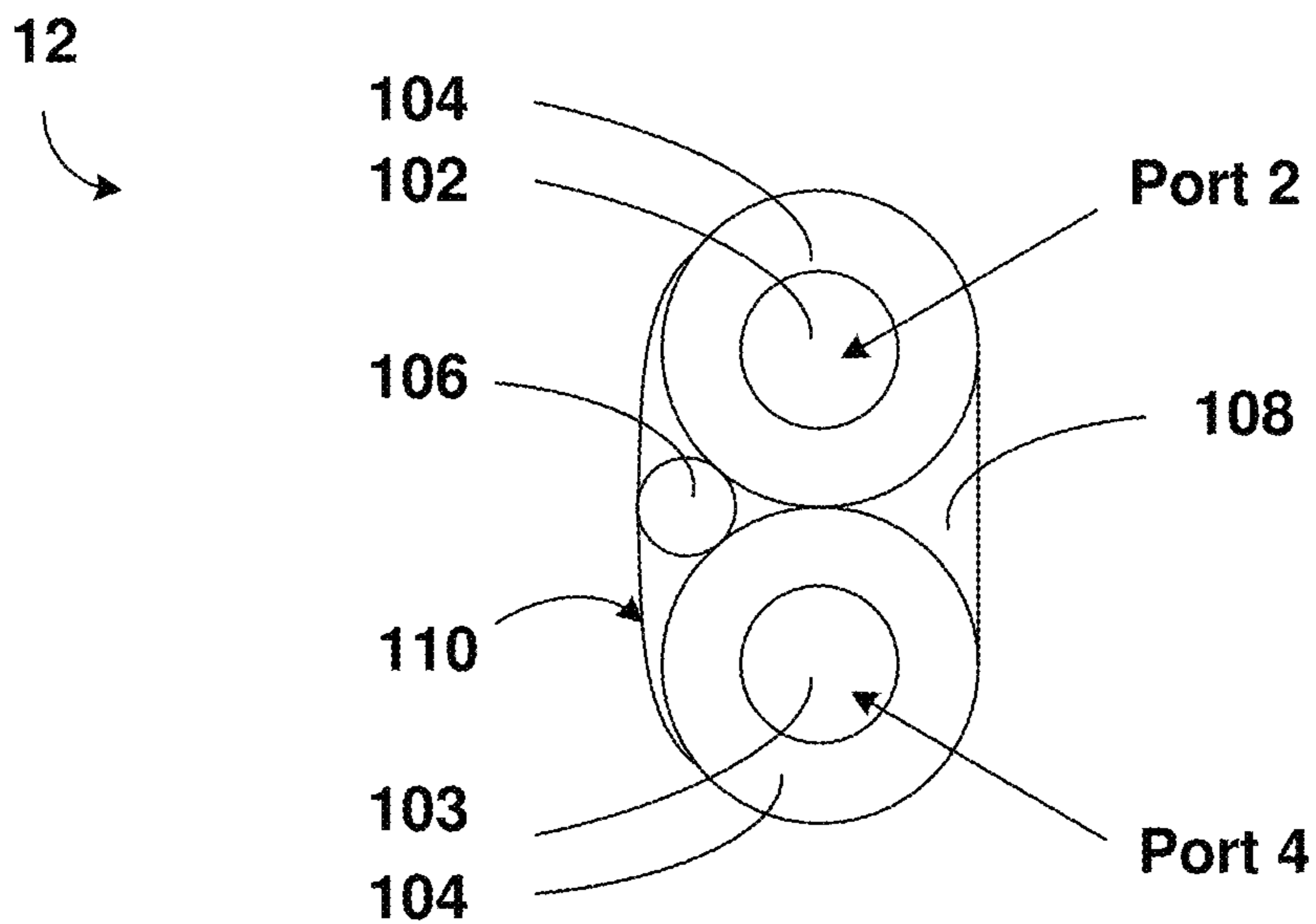
Figure 3 Section B-B
