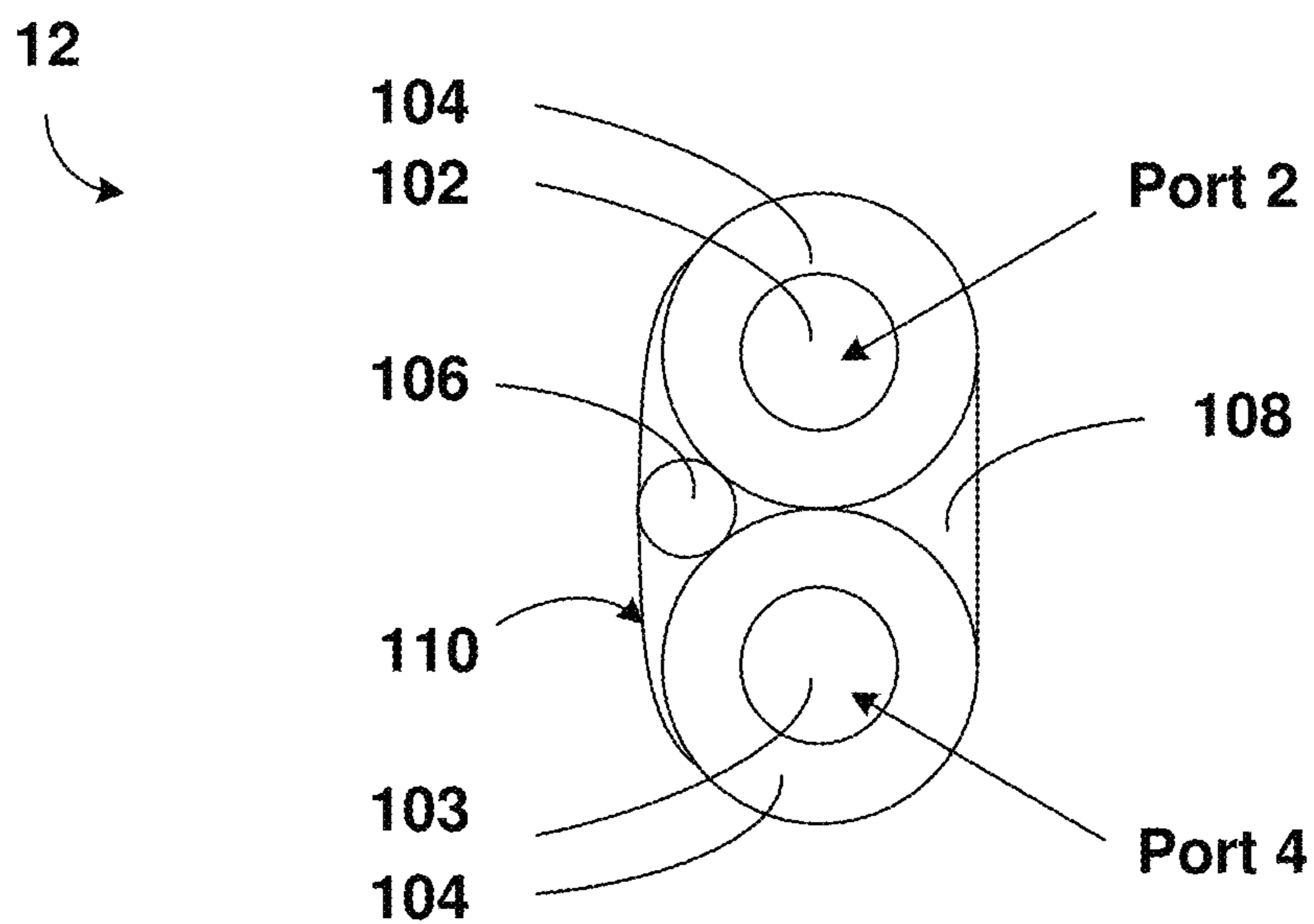
Figure 3 Section B-B
