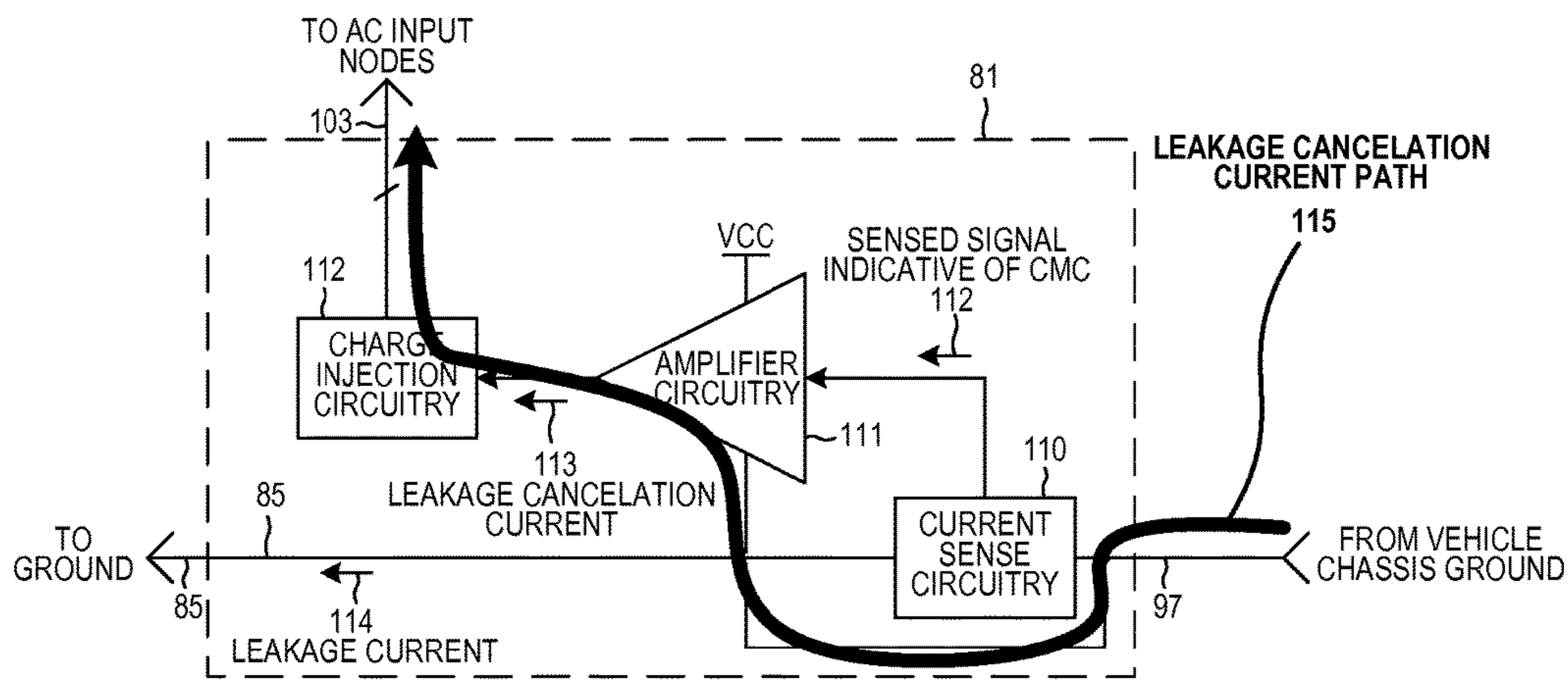
LEAKAGE CURRENT CANCELATION CIRCUIT FIG. 8
