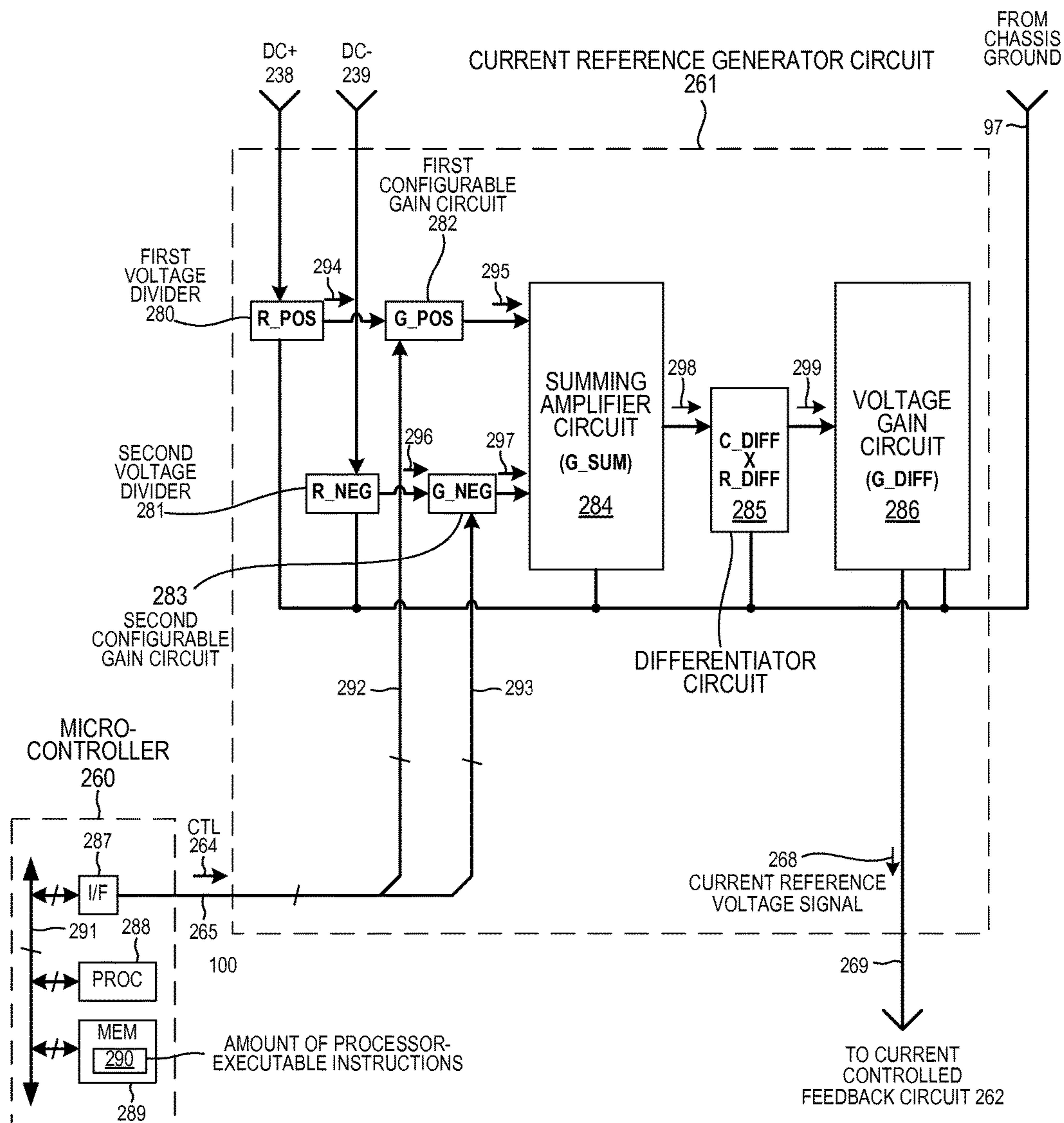
MICROCONTROLLER AND CURRENT REFERENCE GENERATOR CIRCUIT
