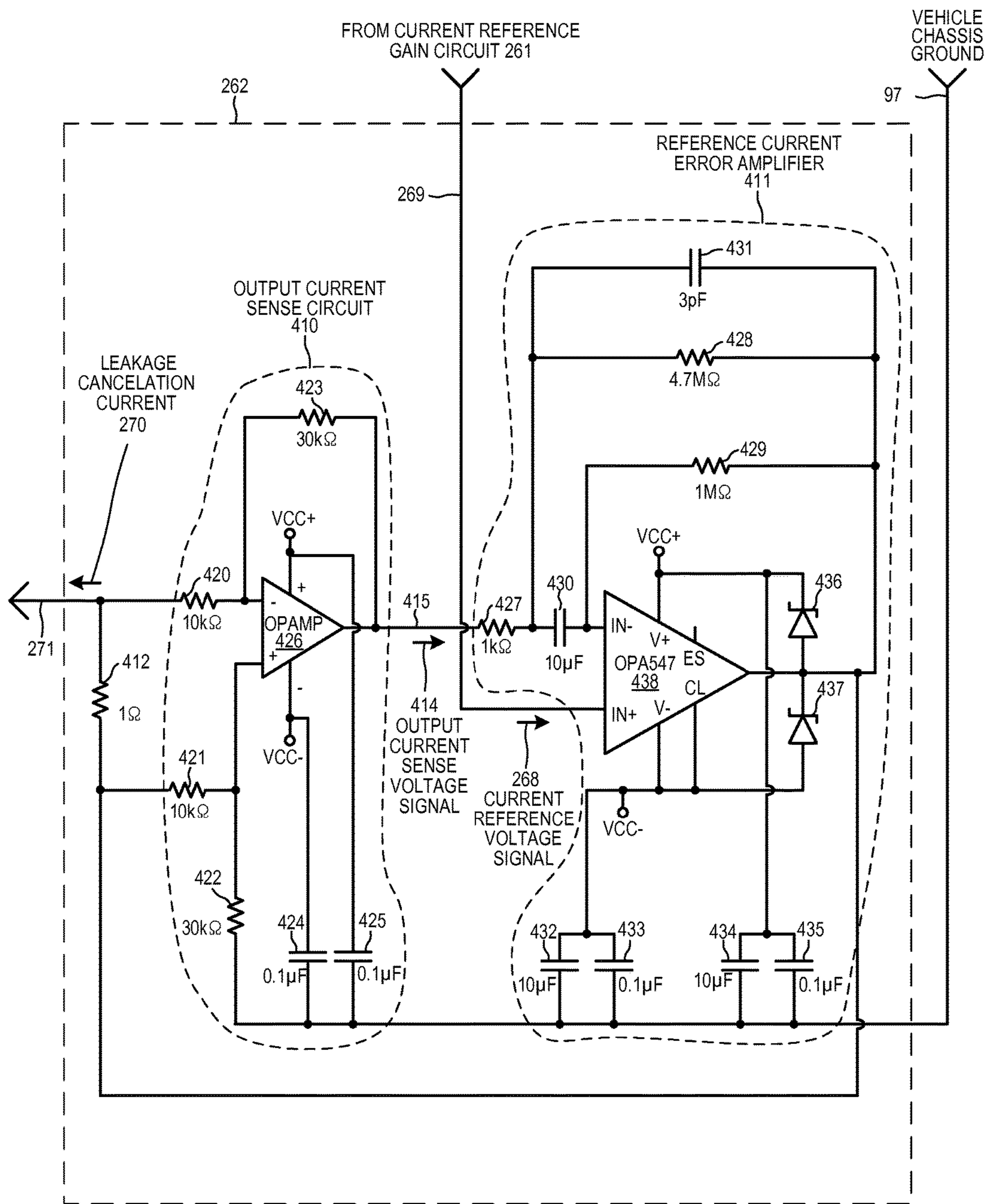
CURRENT CONTROLLED FEEDBACK CIRCUIT
