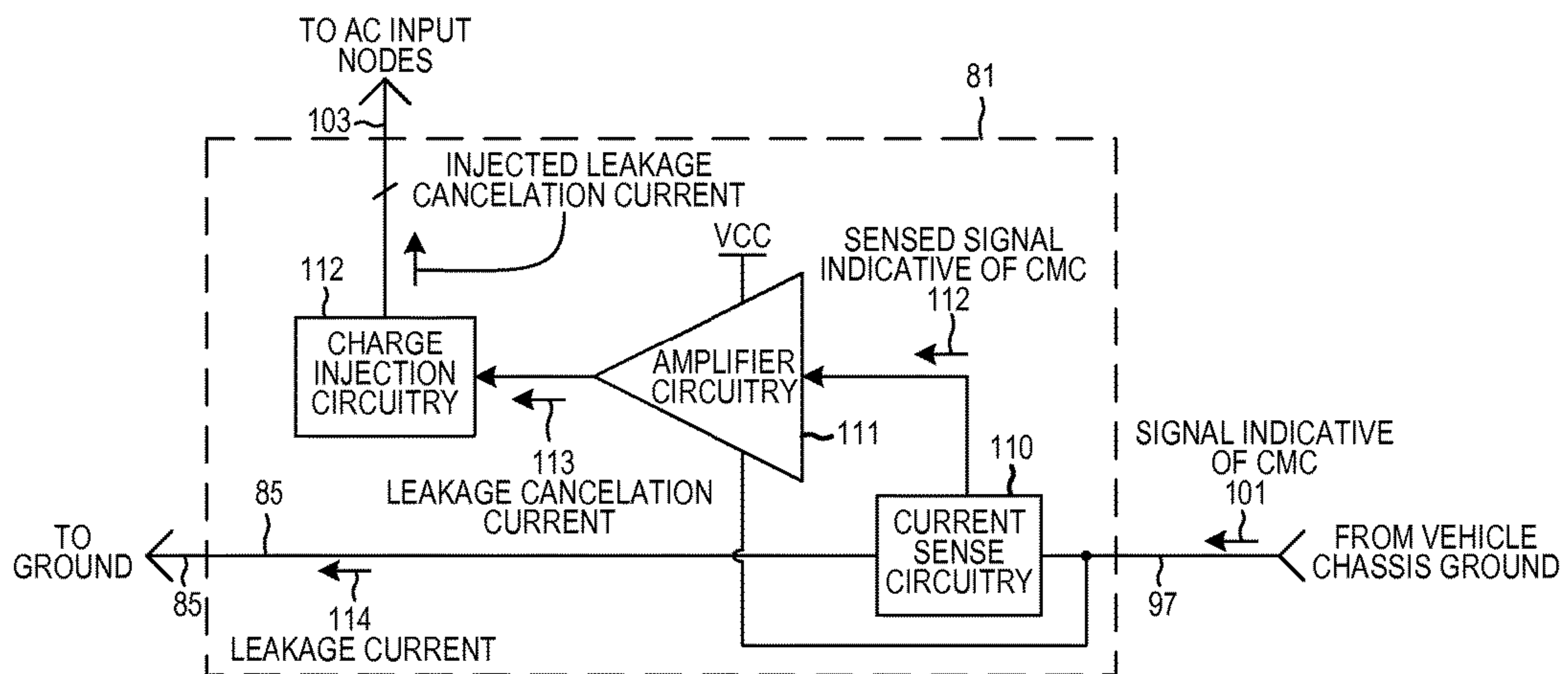
LEAKAGE CURRENT CANCELATION CIRCUIT
