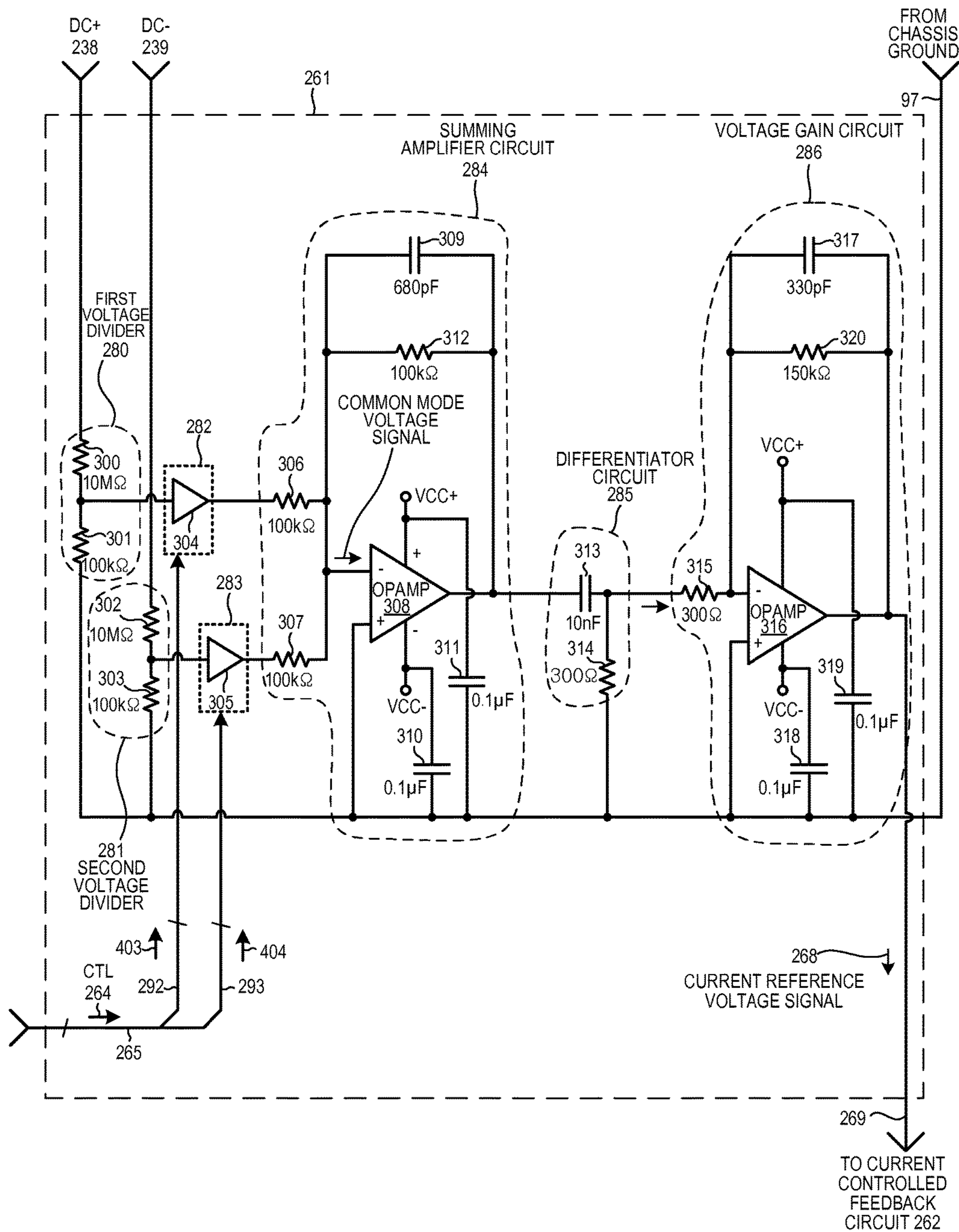
CURRENT REFERENCE GENERATOR CIRCUIT FIG. 22
