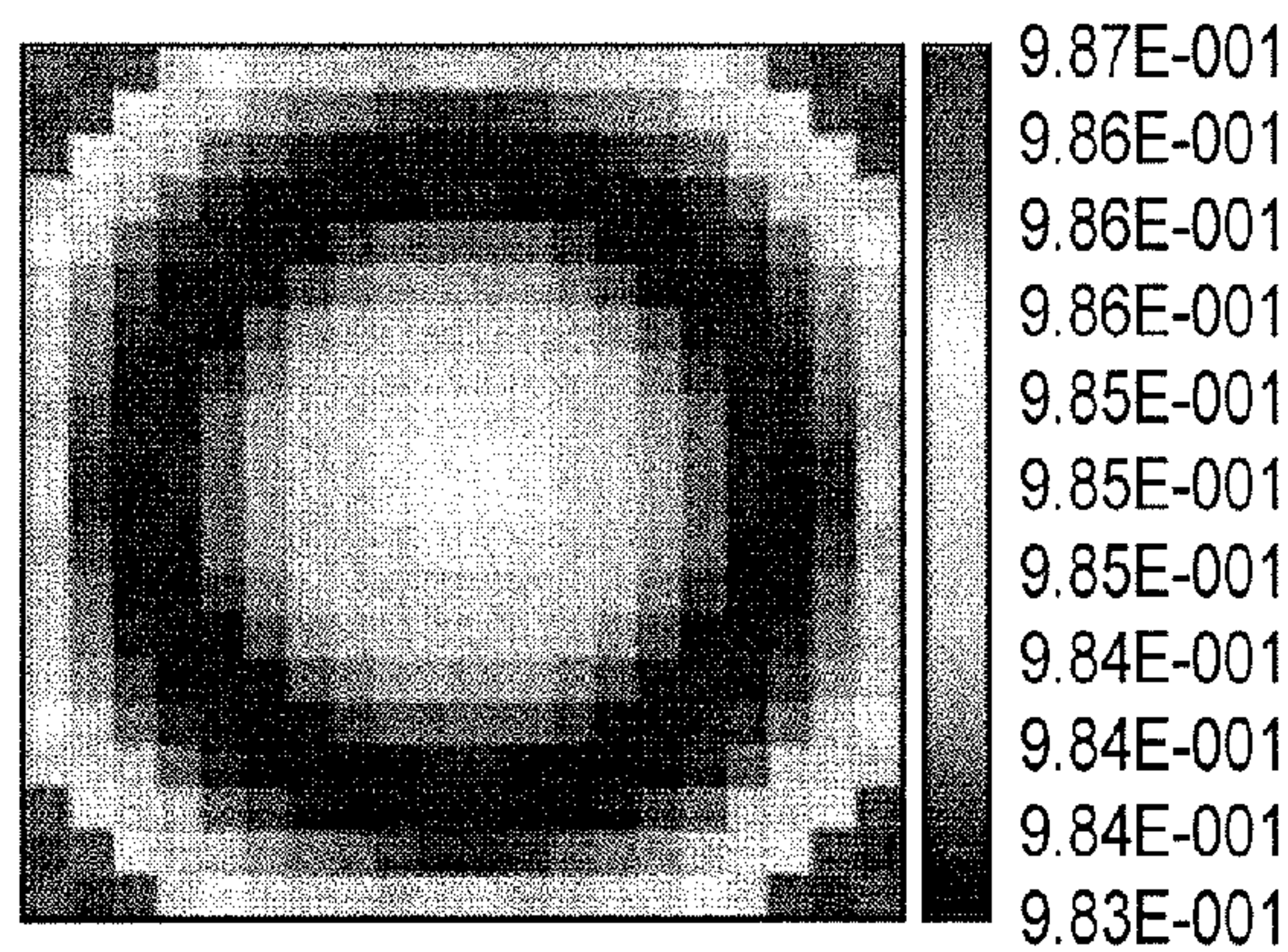
Strehl Ratio field Map
