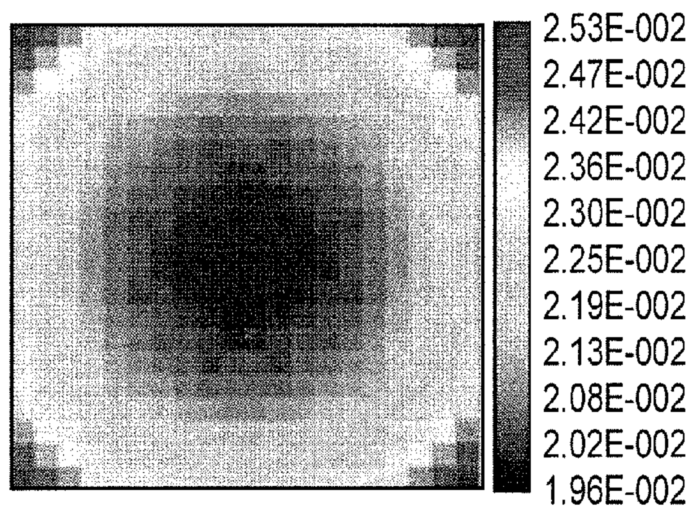
RMS Spot Radius Field Map
