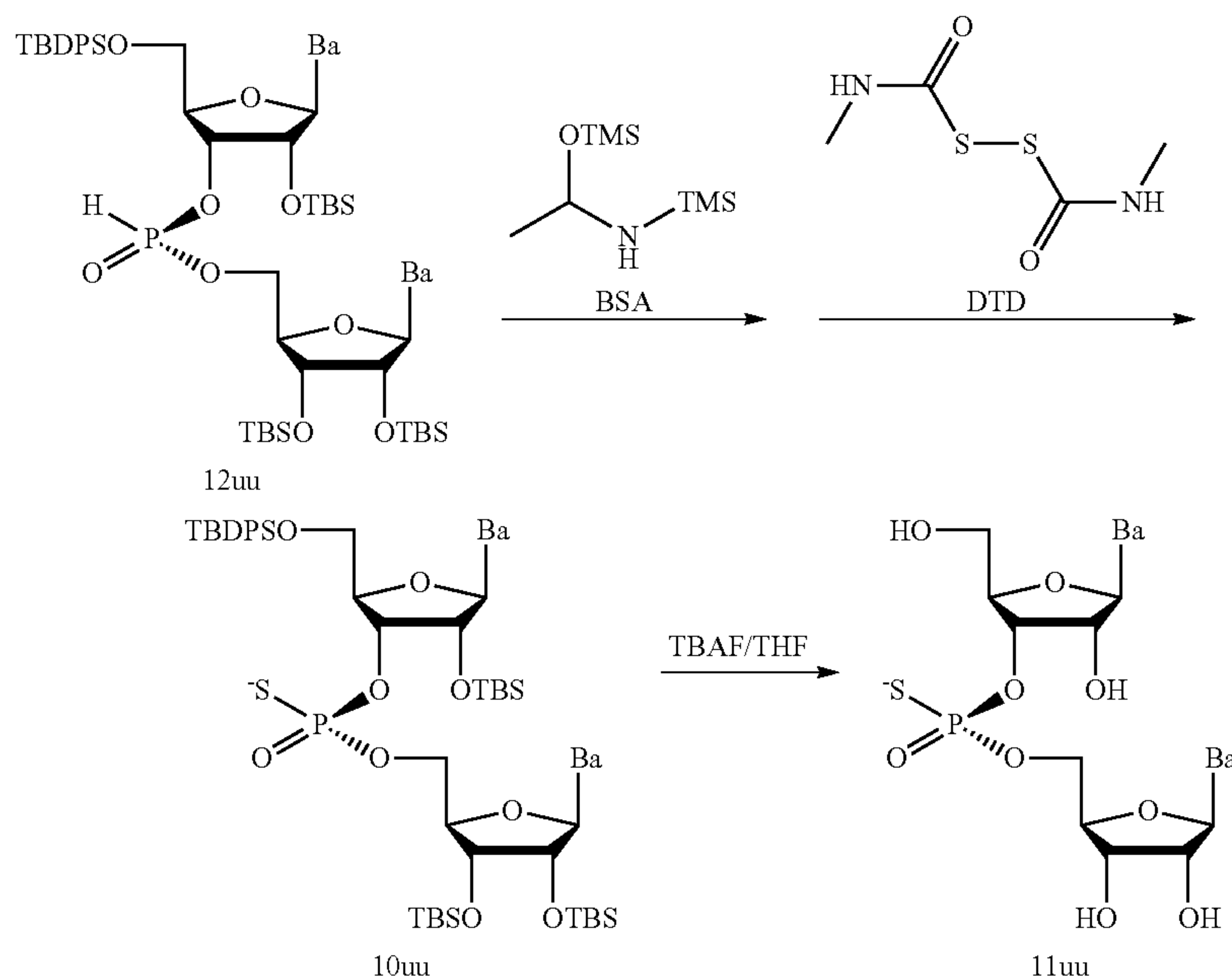
Scheme 17. Synthesis of chiral phosphorothioate.
