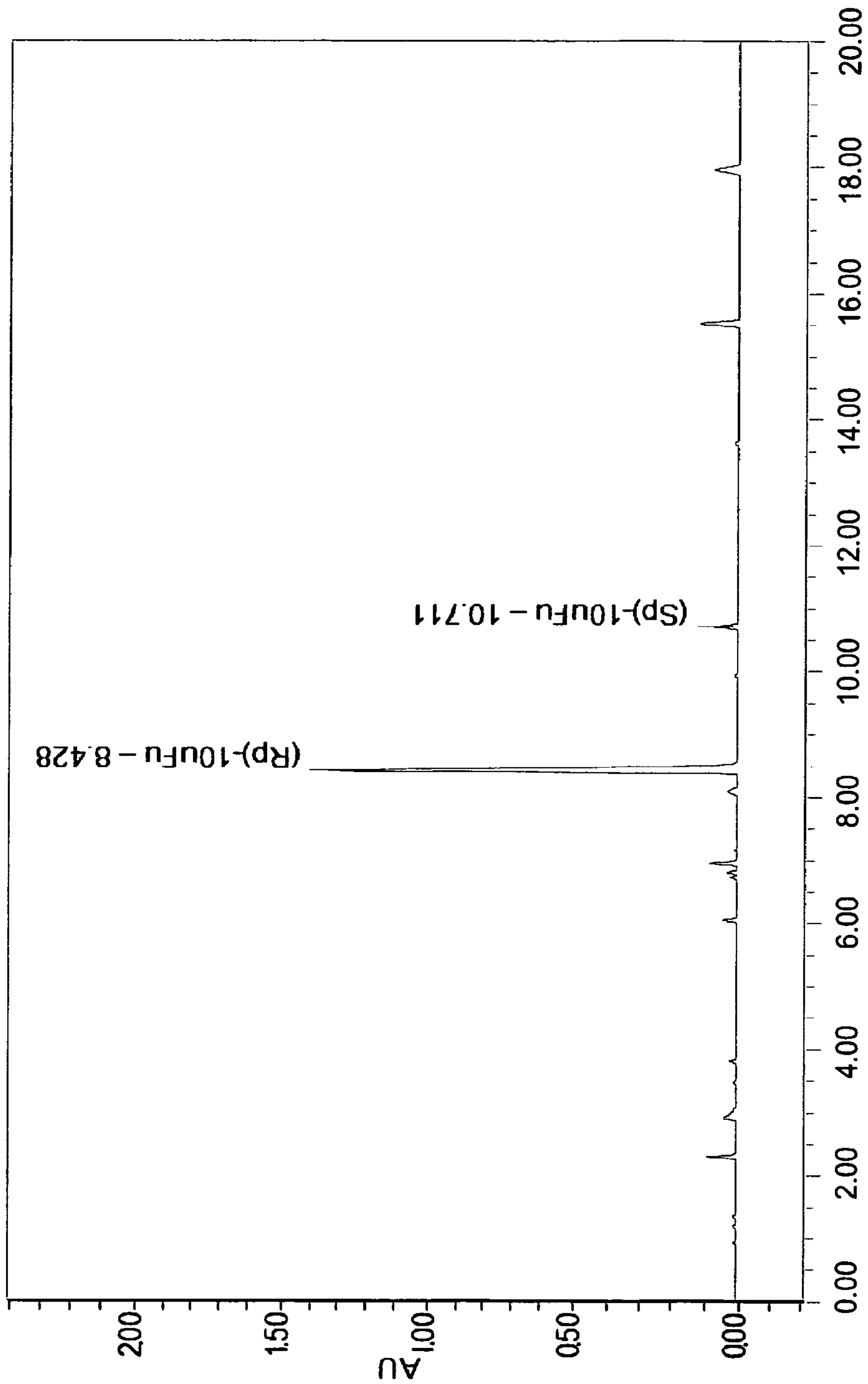
FIGURE 36A Crude UPLC ® profile of (R P )-10u Fu
