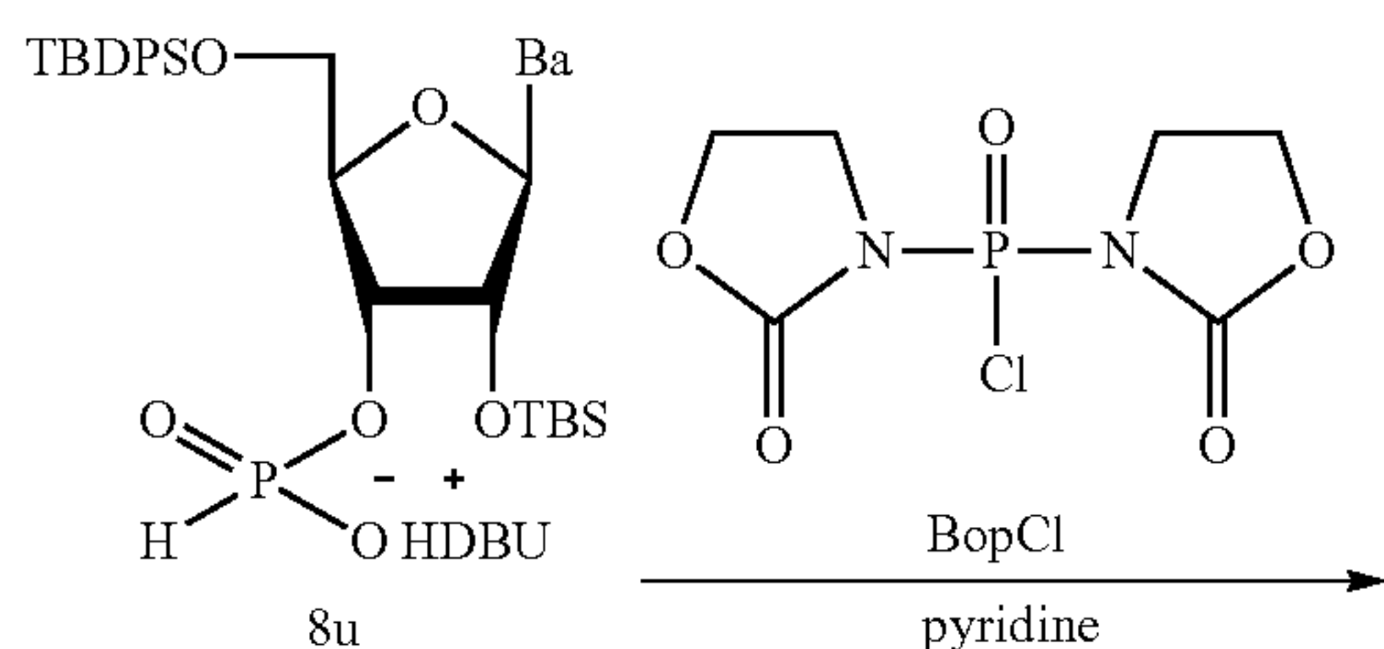
Scheme 16. Synthesis of RNA analogs via Scheme 6 (Route B).
