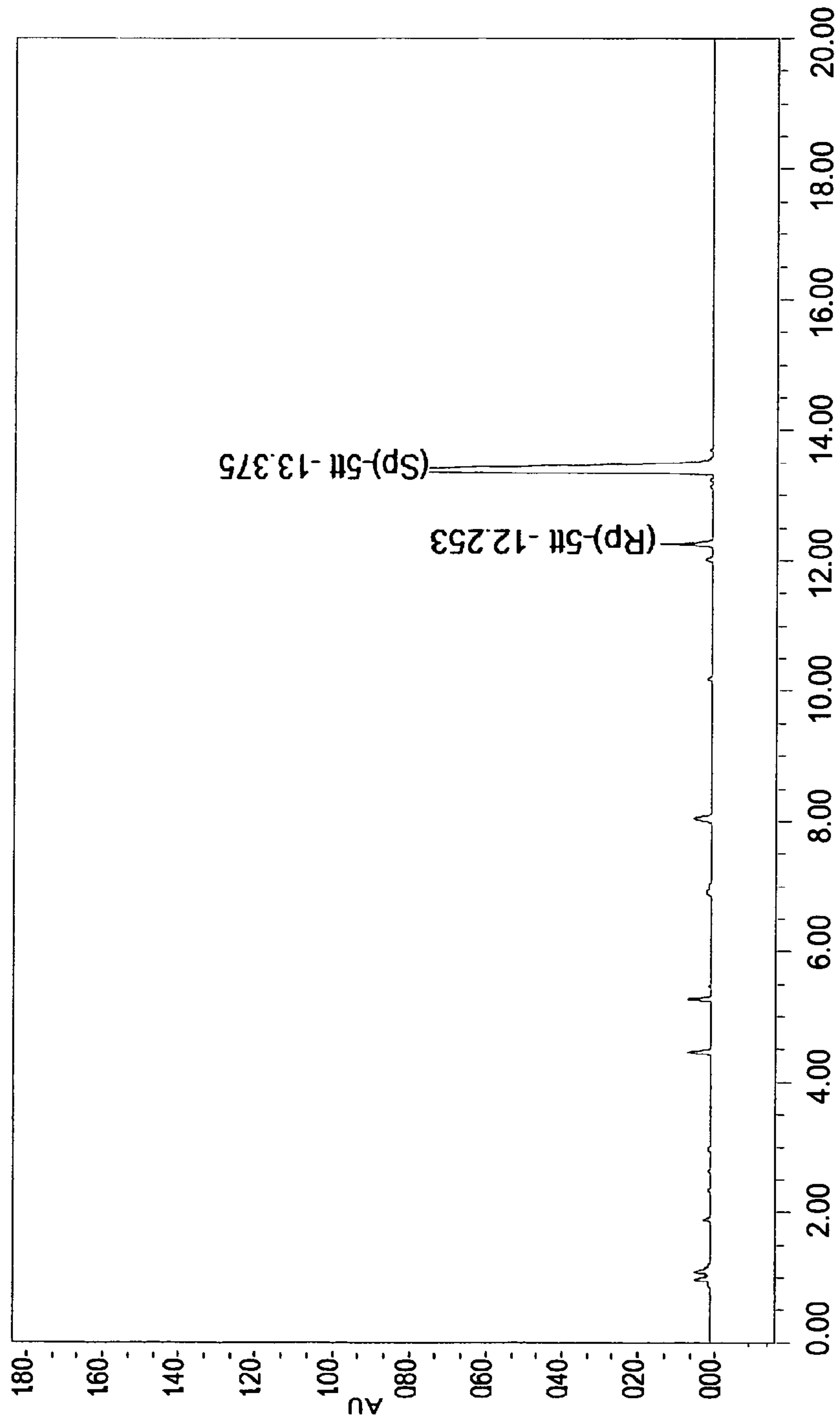
FIGURE 15B Crude UPLC ® profile of (S P )-5tt
