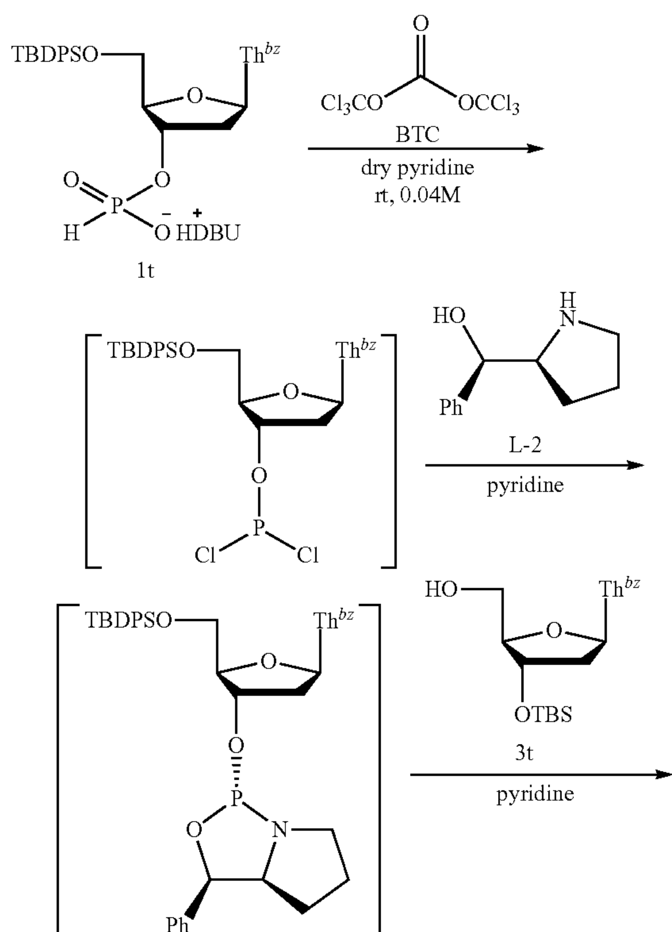
Scheme 10. Solution Synthesis of a DNA dimer as in Scheme 5 (Route A).
