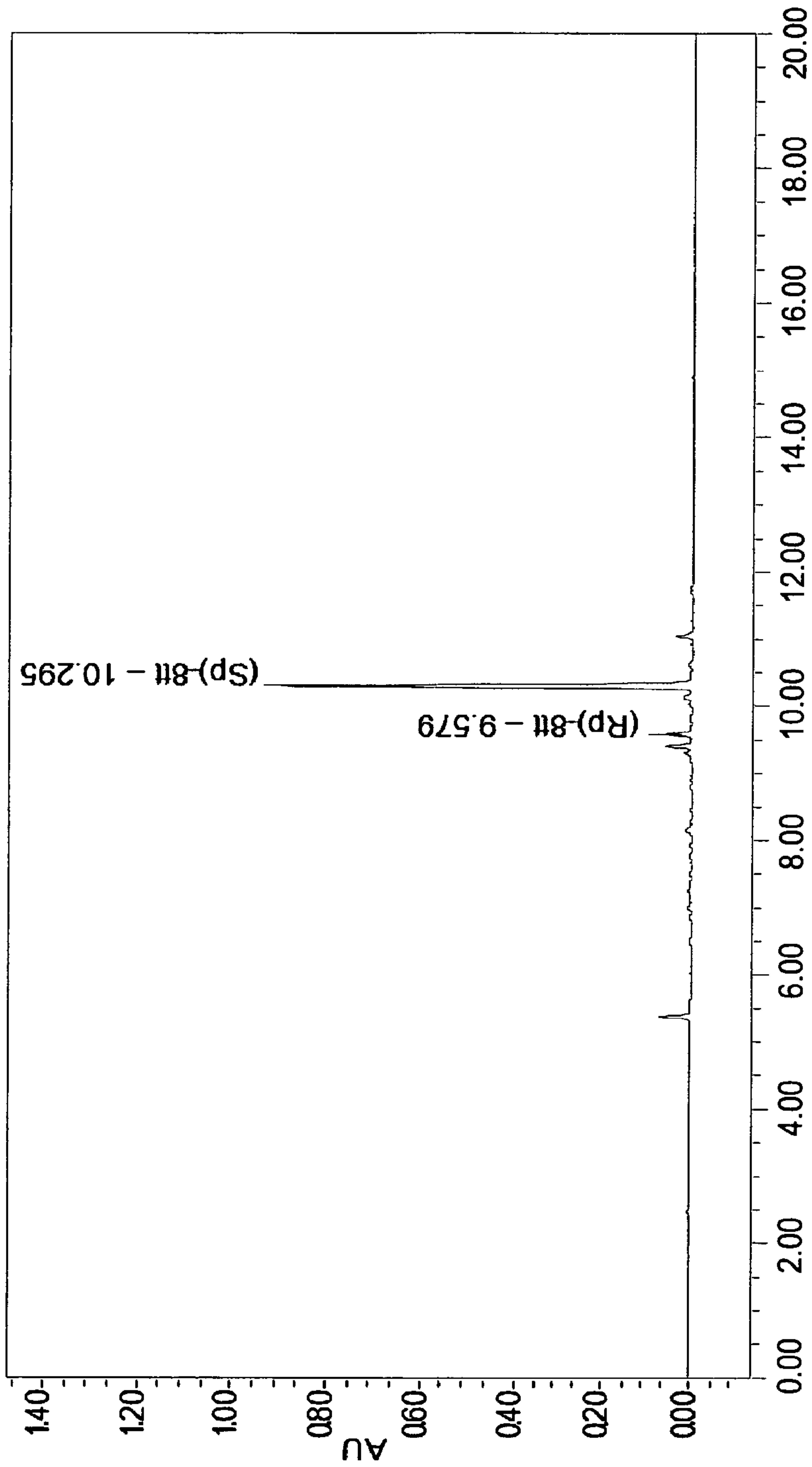
FIGURE 27 Crude UPLC ® profile of (S P )-8tt
