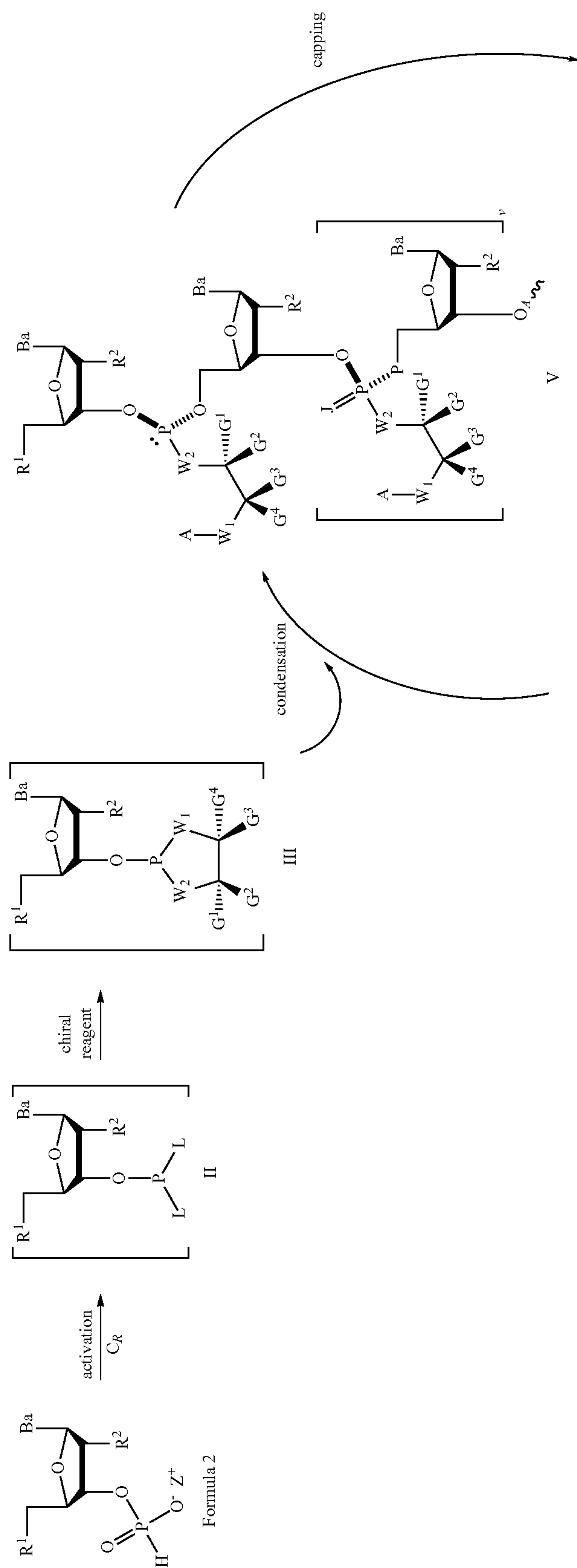
Scheme 5. Synthesis of a nucleic acid comprising a chiral X-phosphonate moiety of Formula 1 via Route A.
