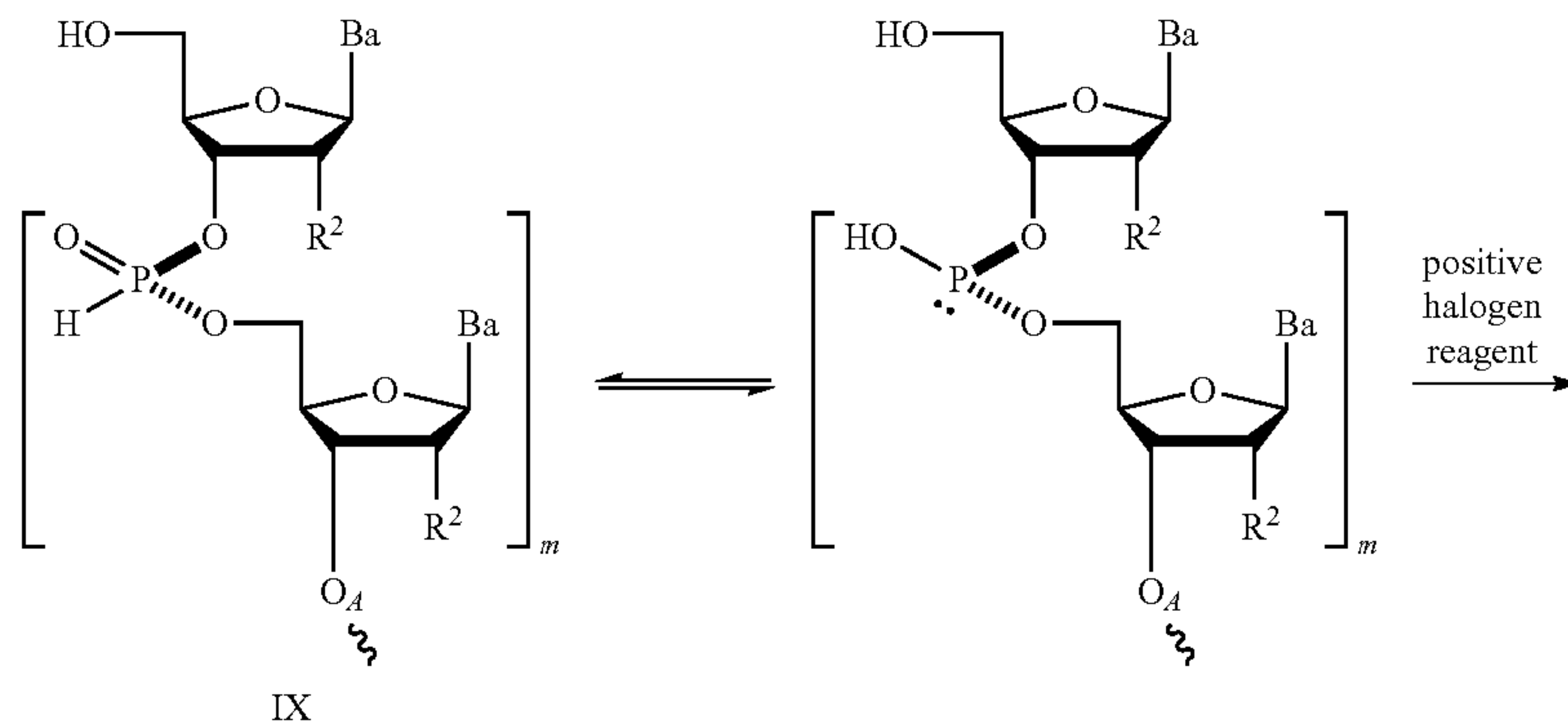
Reaction Scheme 9a. Modification of phosphorus in intermediates synthesized via Route B, using an initial halogenation at phosphorus.
