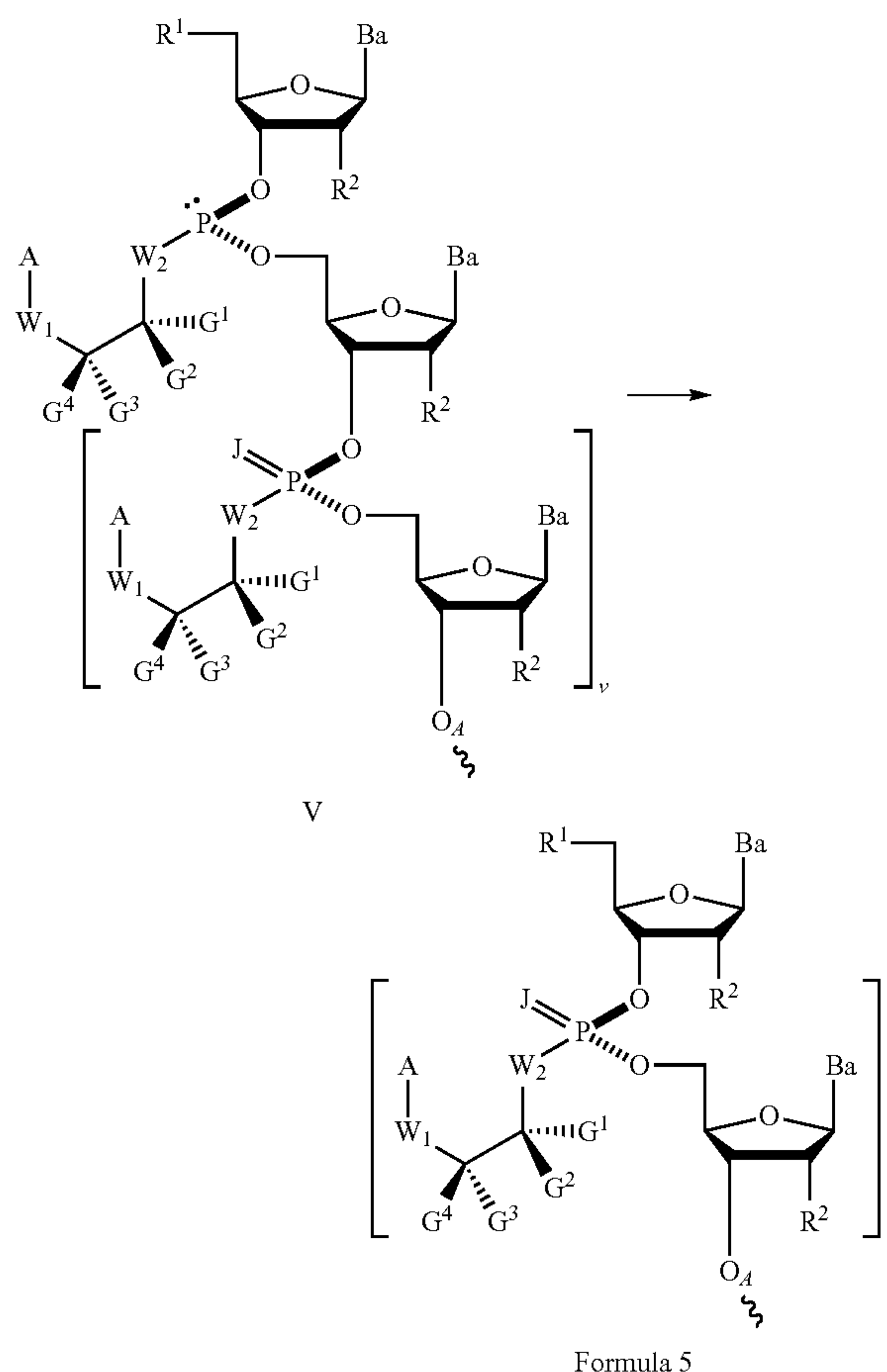
Scheme 8. Modification of the condensed intermediate obtained via Route A.
