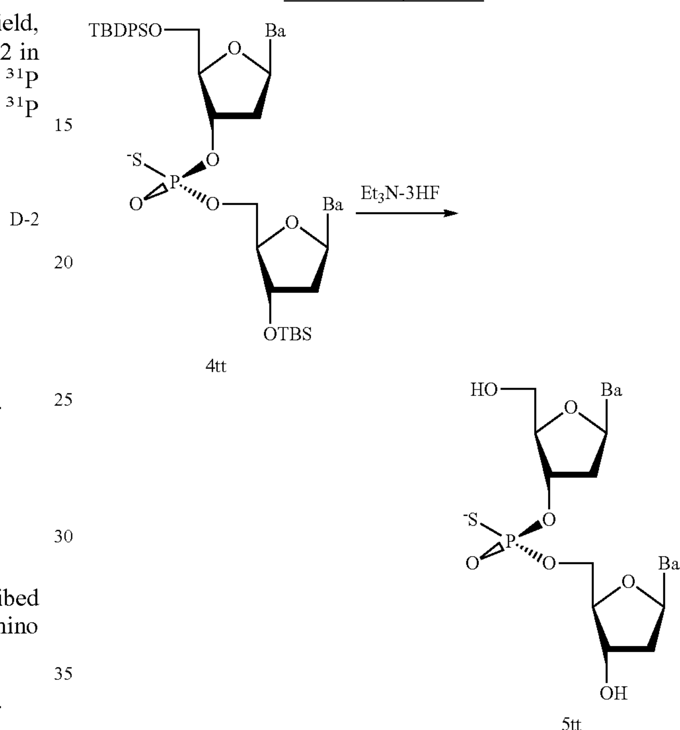
Scheme 11. Deprotection.
