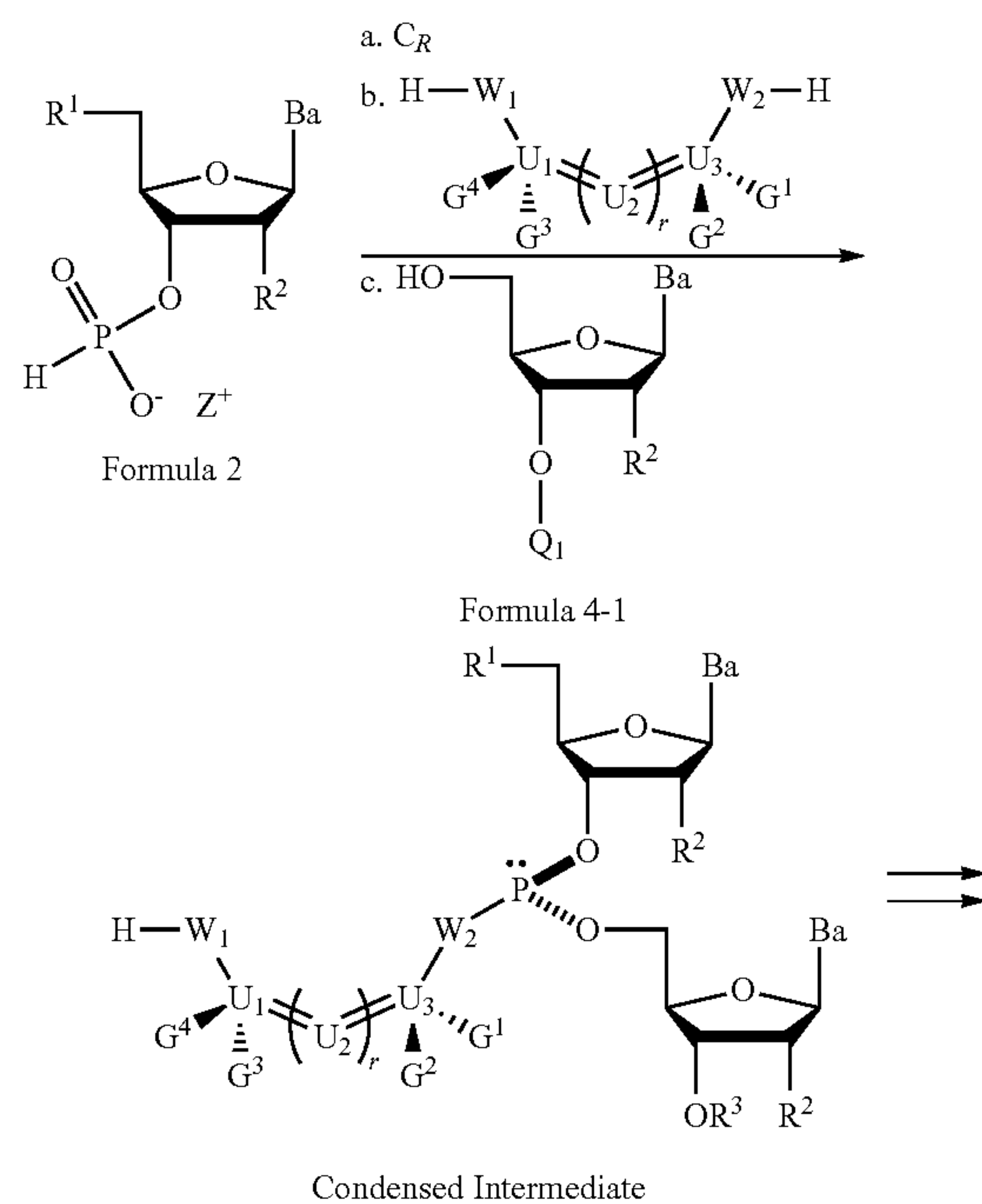
Scheme 2. Reaction steps leading to the formation of a condensed intermediate.
