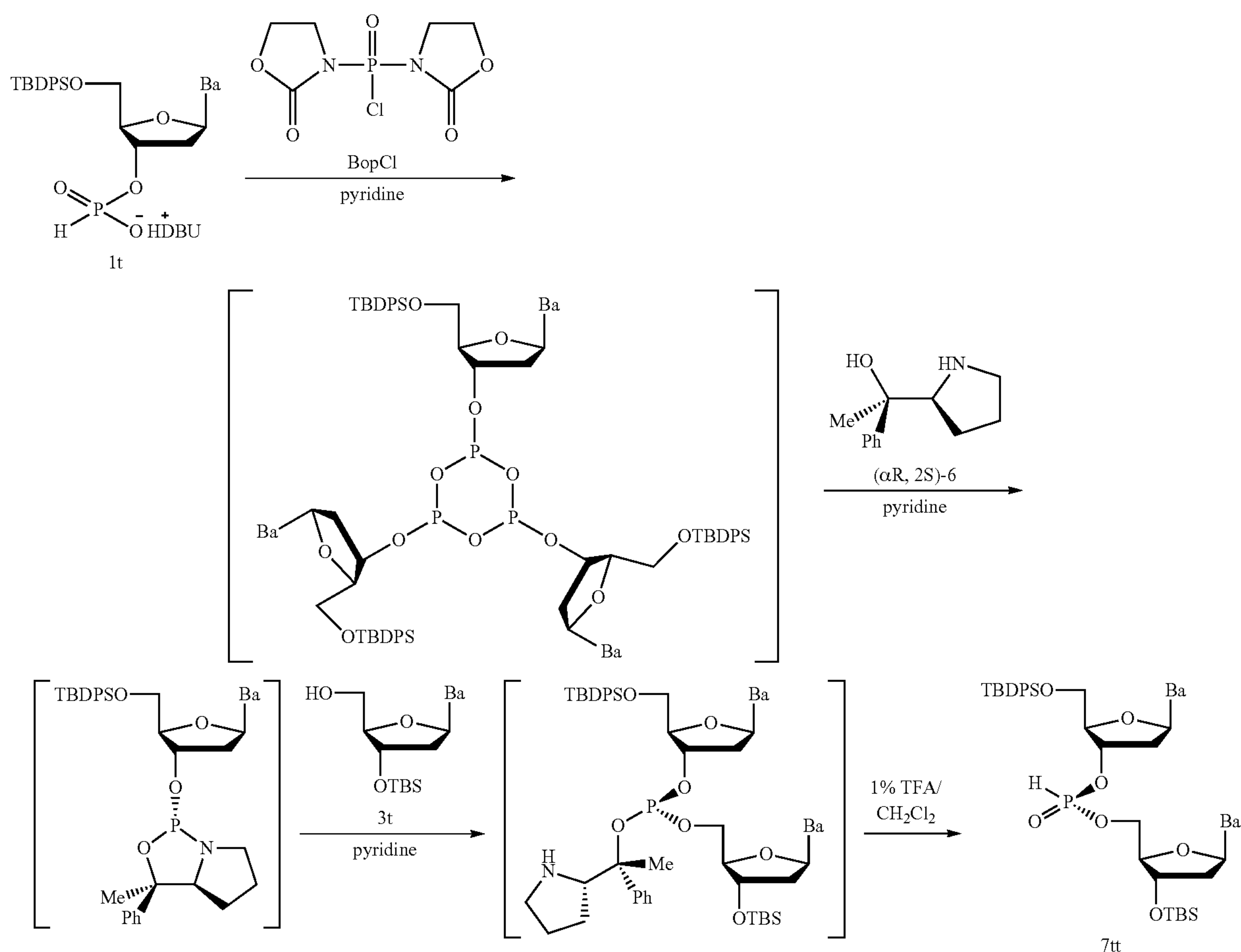
Scheme 12. Synthesis of a DNA analogs as in Scheme 6 (Route B).
