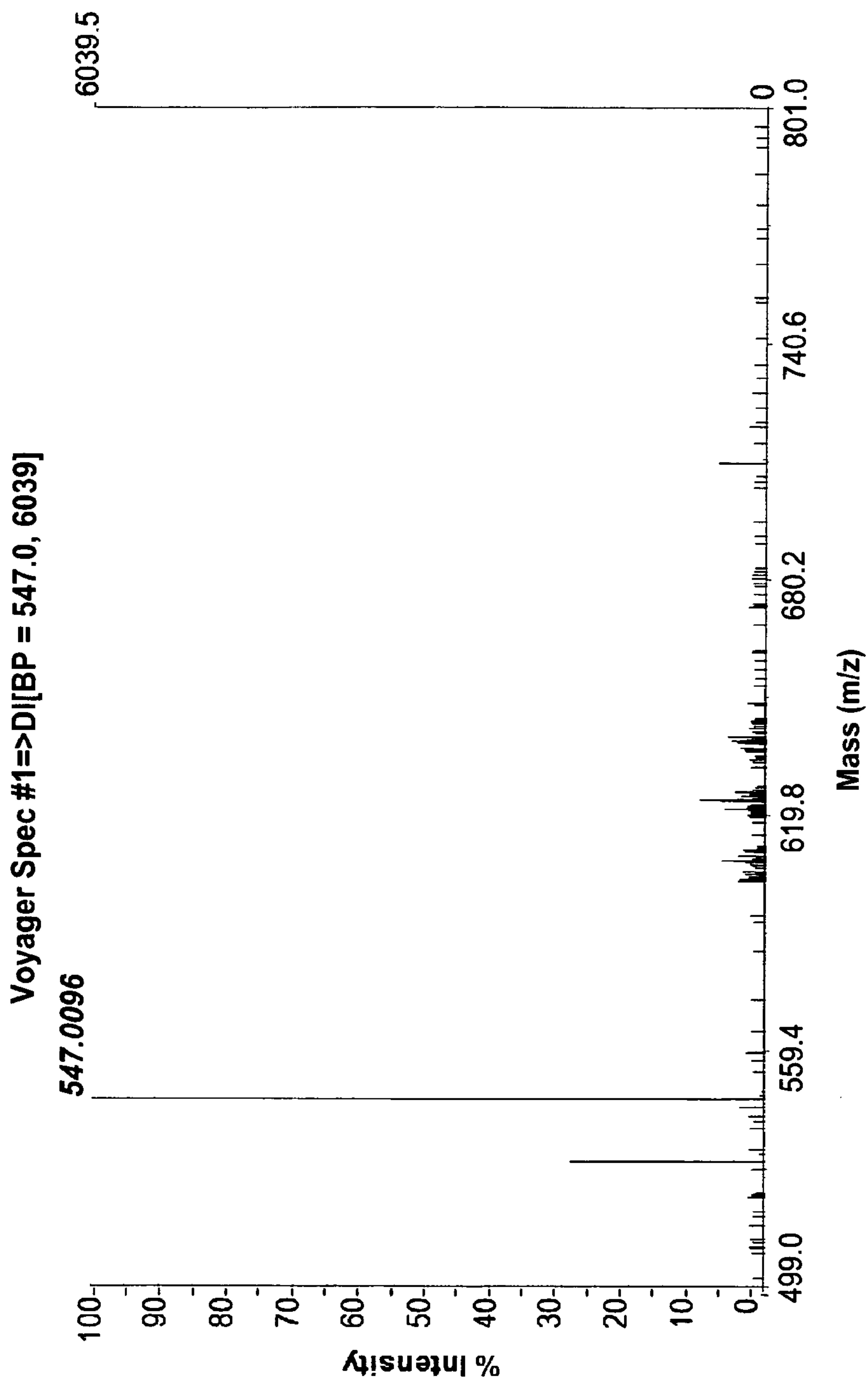
FIGURE 38B MALDI TOF-MS spectrum of (R p )-11nt
