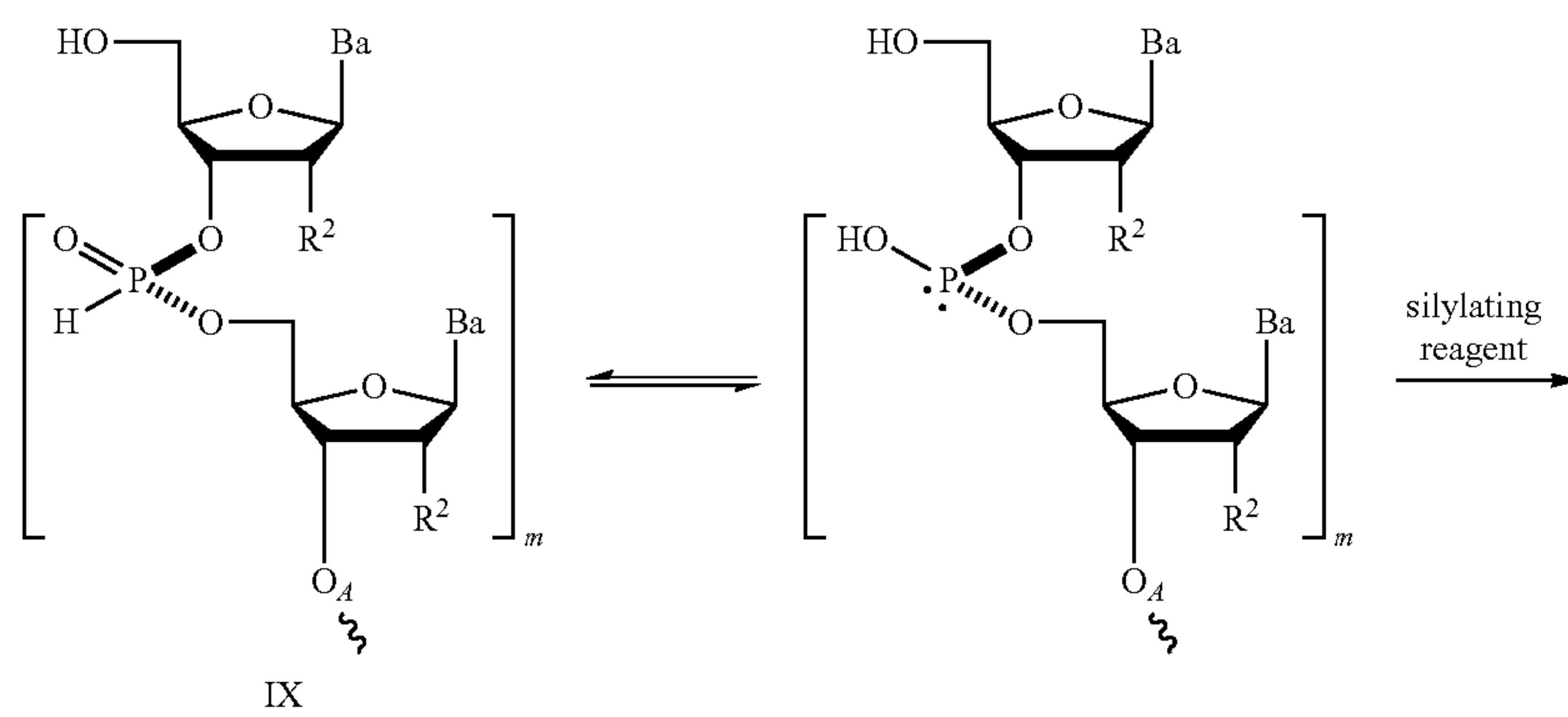
Reaction Scheme 9b. Modification of phosphorus in intermediates synthesized via Route B, using an initial silylation.
