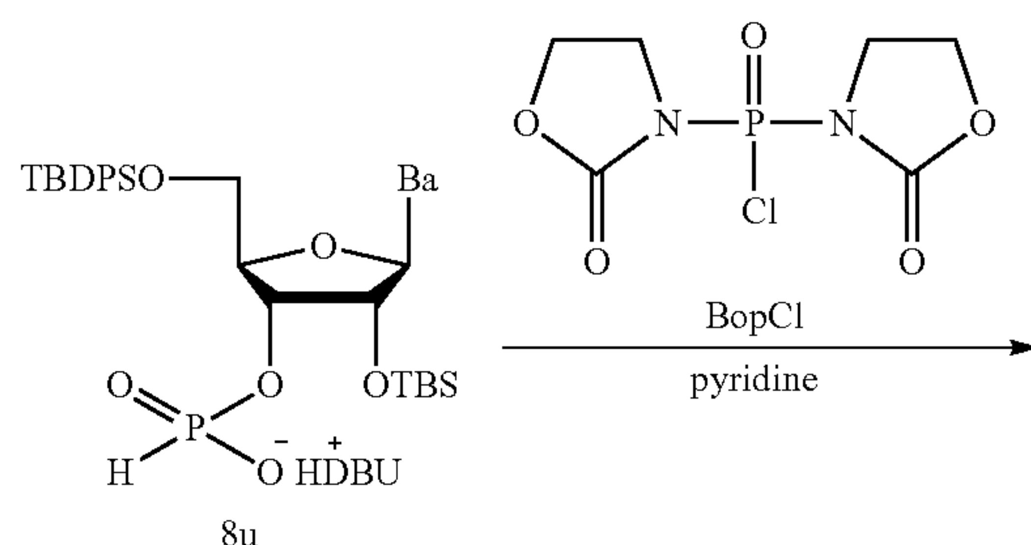
Scheme 14. Synthesis of RNA Analogs as in Scheme 5 (Route A).
