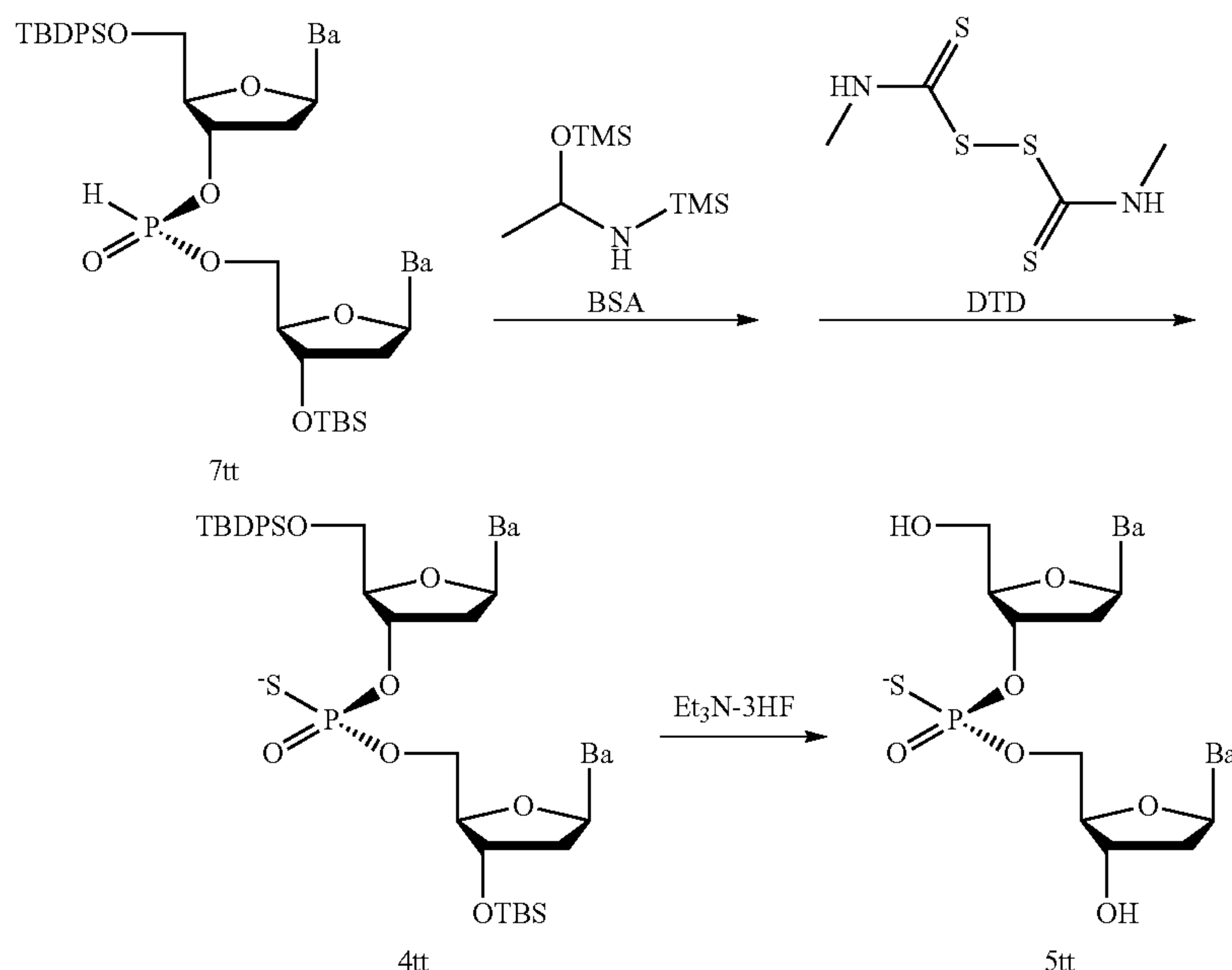
Scheme 13. Modification at Phosphorus to introduce Sulfur.
