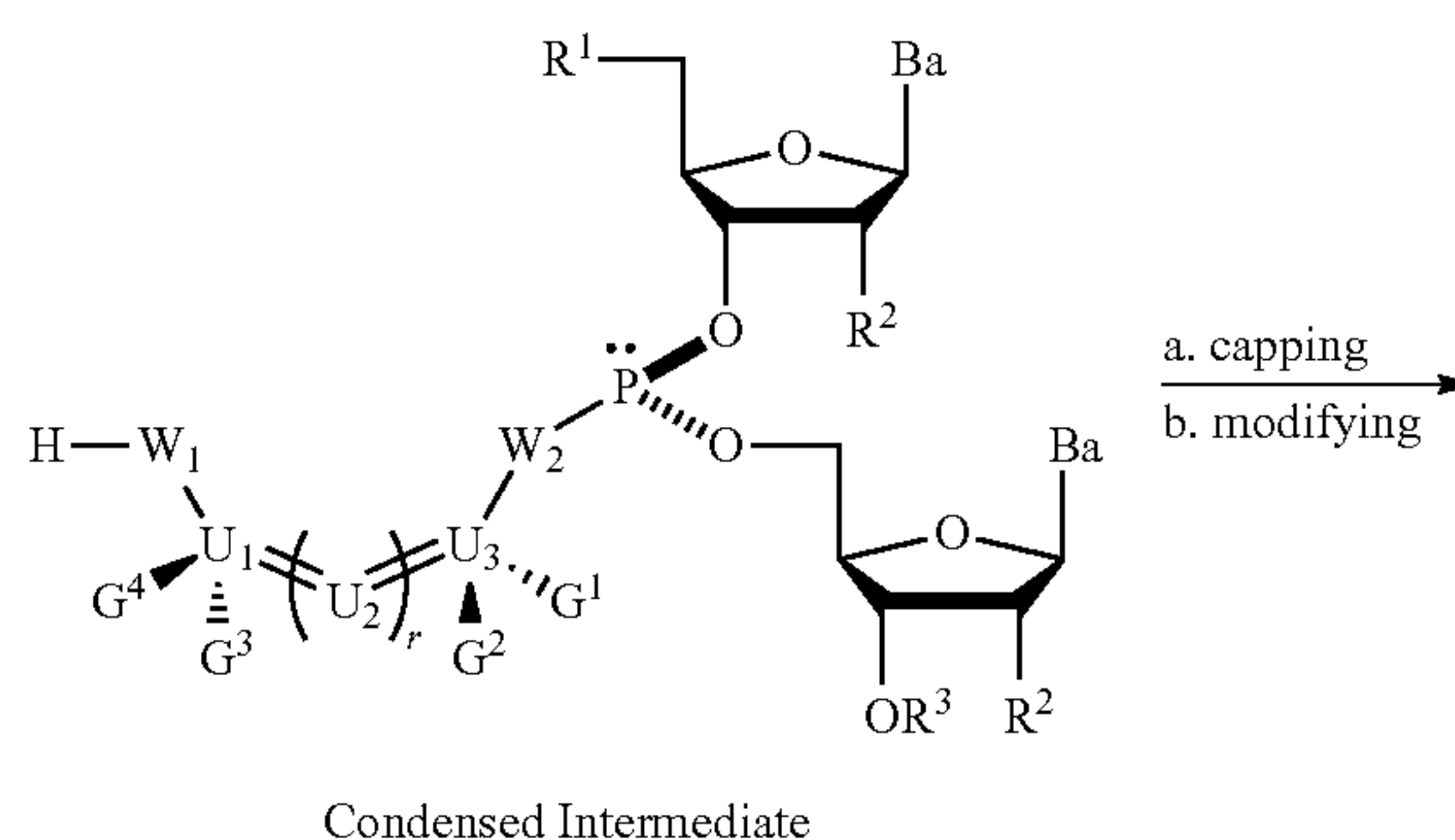
Scheme 3. Converting the condensed intermediate to the compound of Formula 1 via Route A.
