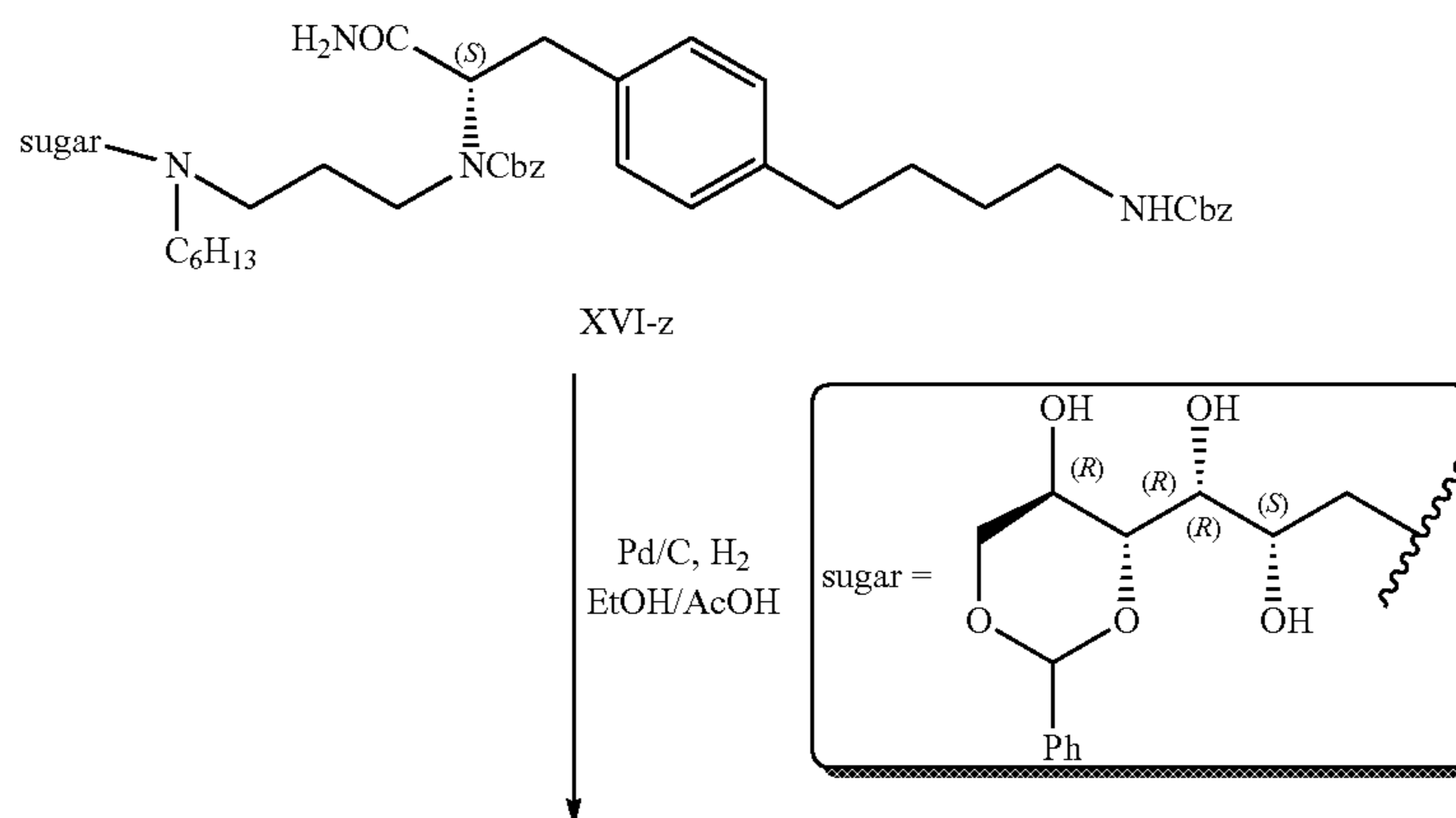
Scheme XVII. The Synthesis of the Hydrochloride Salt of 3,5-diamino-N-(N-(4-(4-((S)-3-amino-2-(3-(hexyl((2S,3R,4R,5R)-2,3,4,5,6-pentahydroxyhexyl)amino)propylamino)-3-oxopropyl)phenyl)butyl)carbamimidoyl)-6-chloropyrazine-2-carboxamide (XVII-d):
