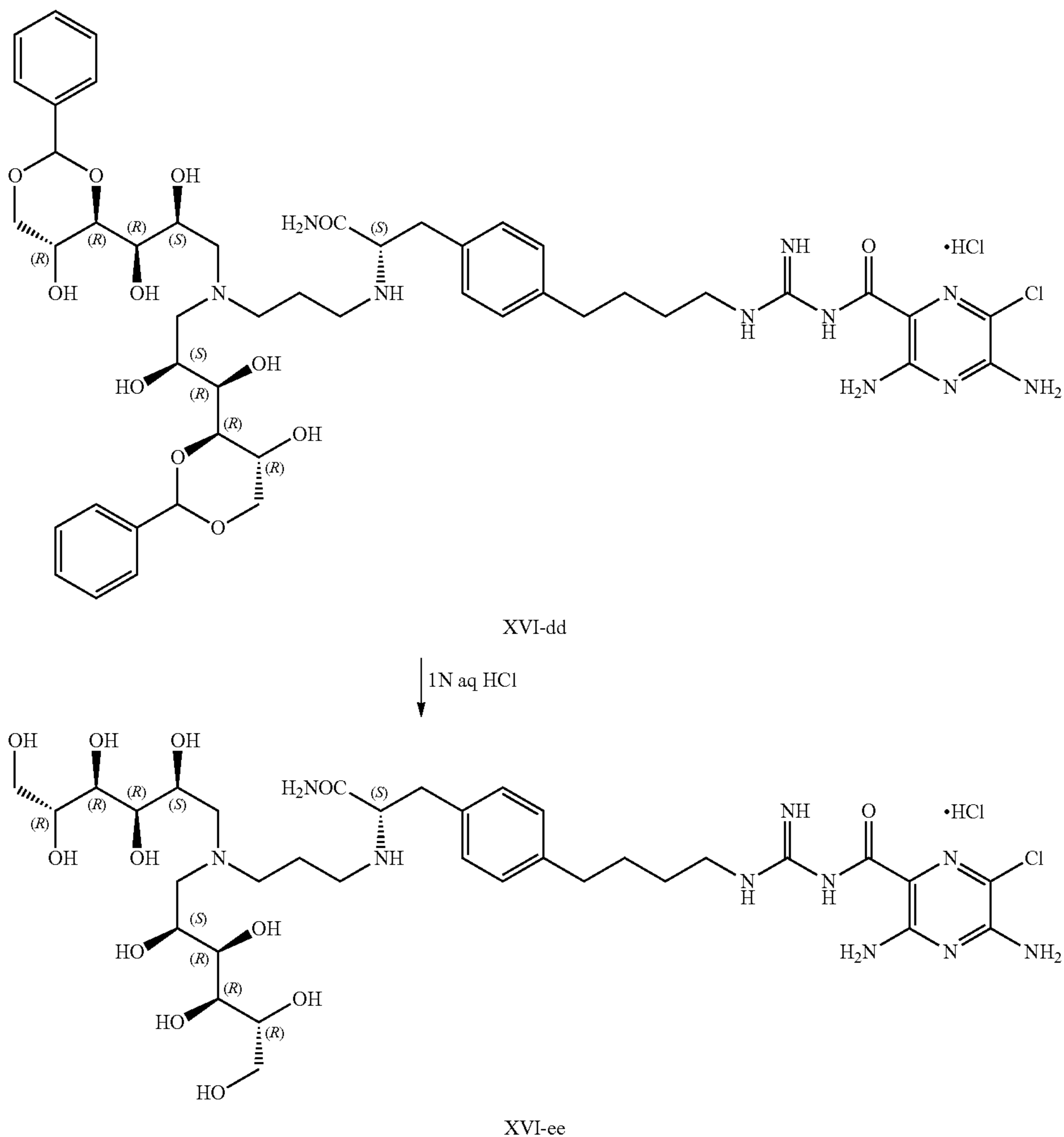
Scheme XVI. The Synthesis of the Hydrochloride Salt 3,5-diamino-N-(N-(4-(4-((S)-3-amino-2-(3-(bis((2S,3R,4R,5R)-2,3,4,5,6-pentahydroxyhexyl)amino)propylamino)-3-oxopropyl)phenyl)butyl)carbamimidoyl)-6-chloropyrazine-2-carboxamide (XVI-ee)
