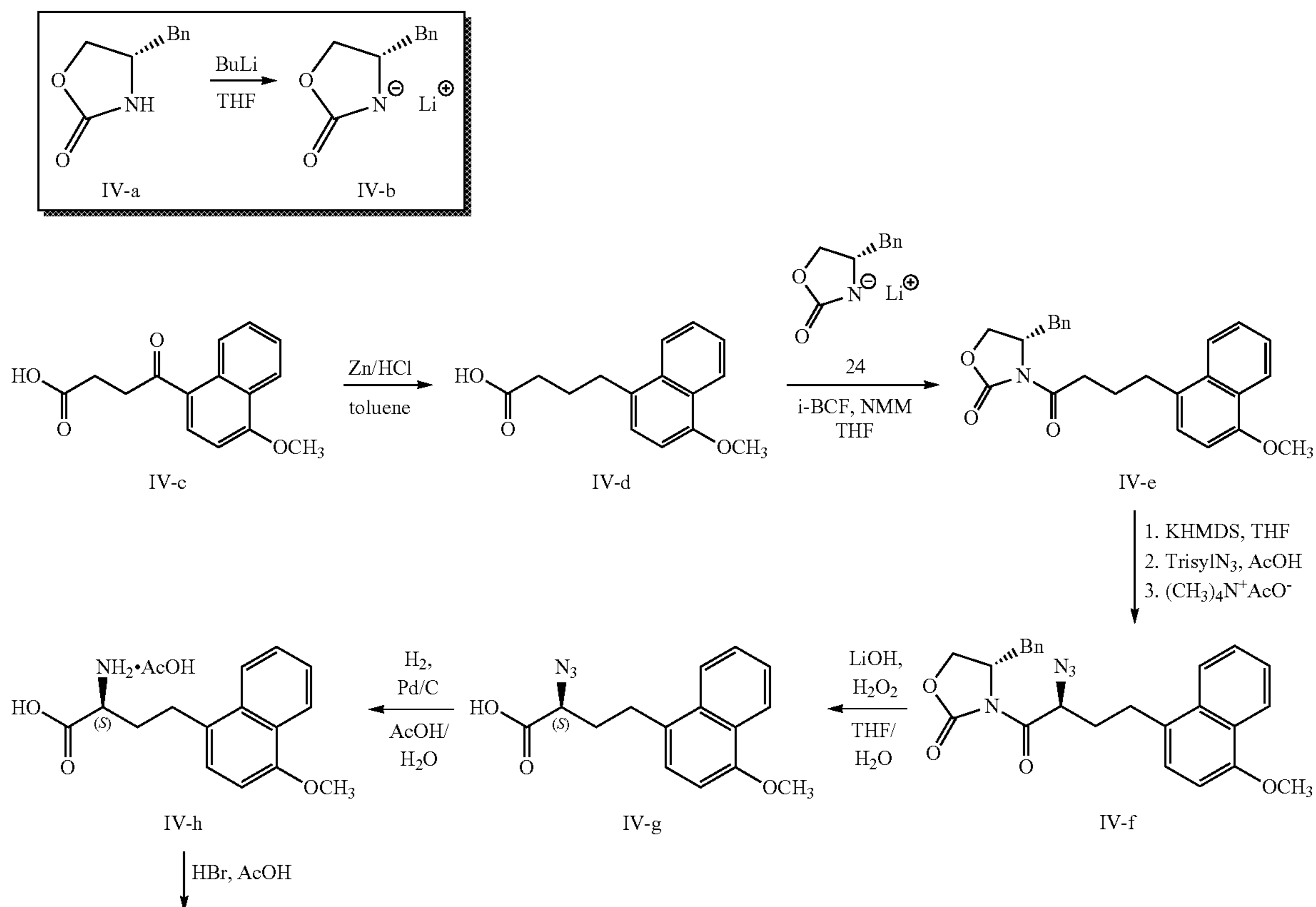
Scheme IV. Preparation of Intermediates IV-x and IV-y.
