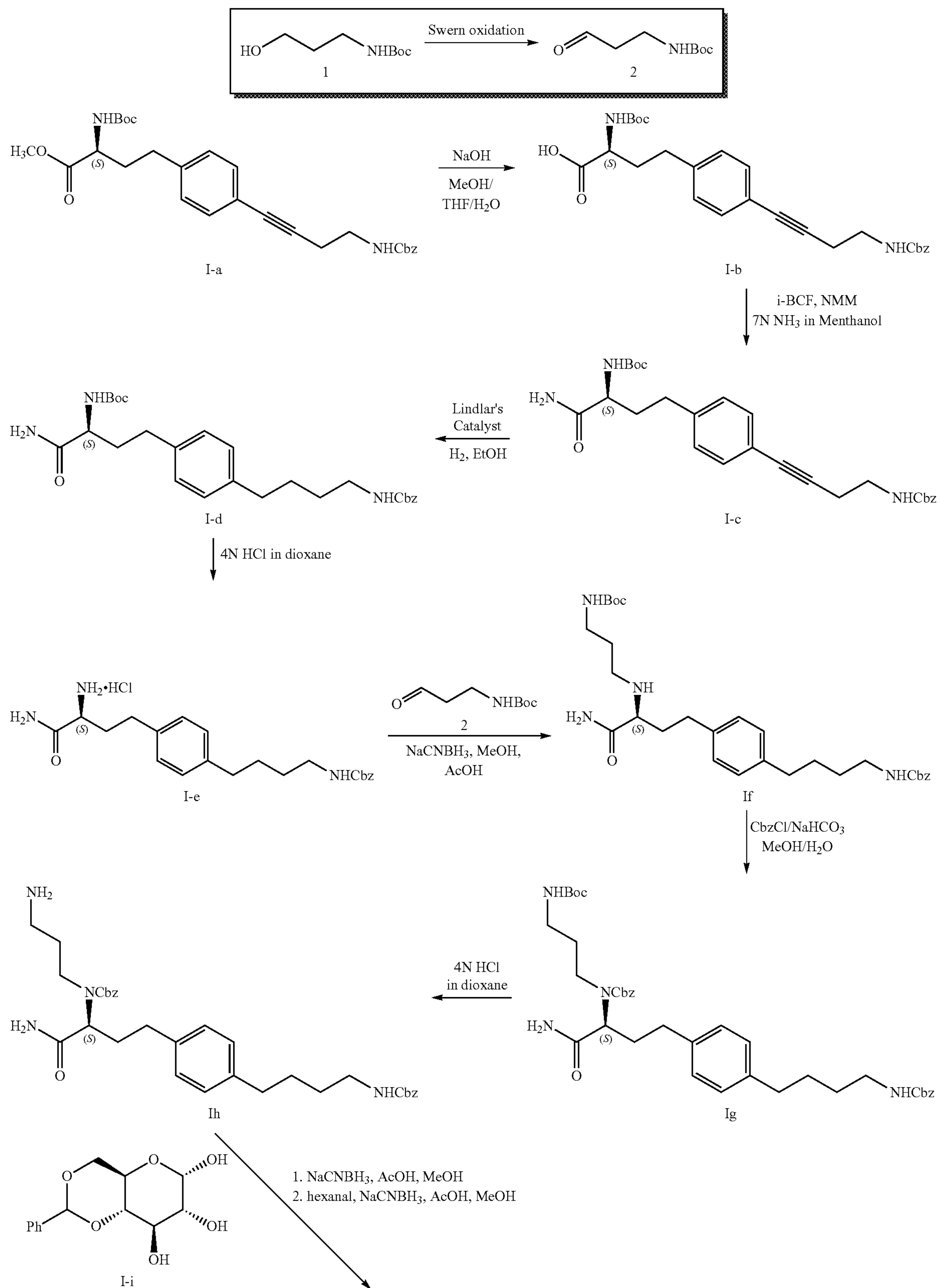
Scheme I. Preparation of intermediates 11-j and 1-k.
