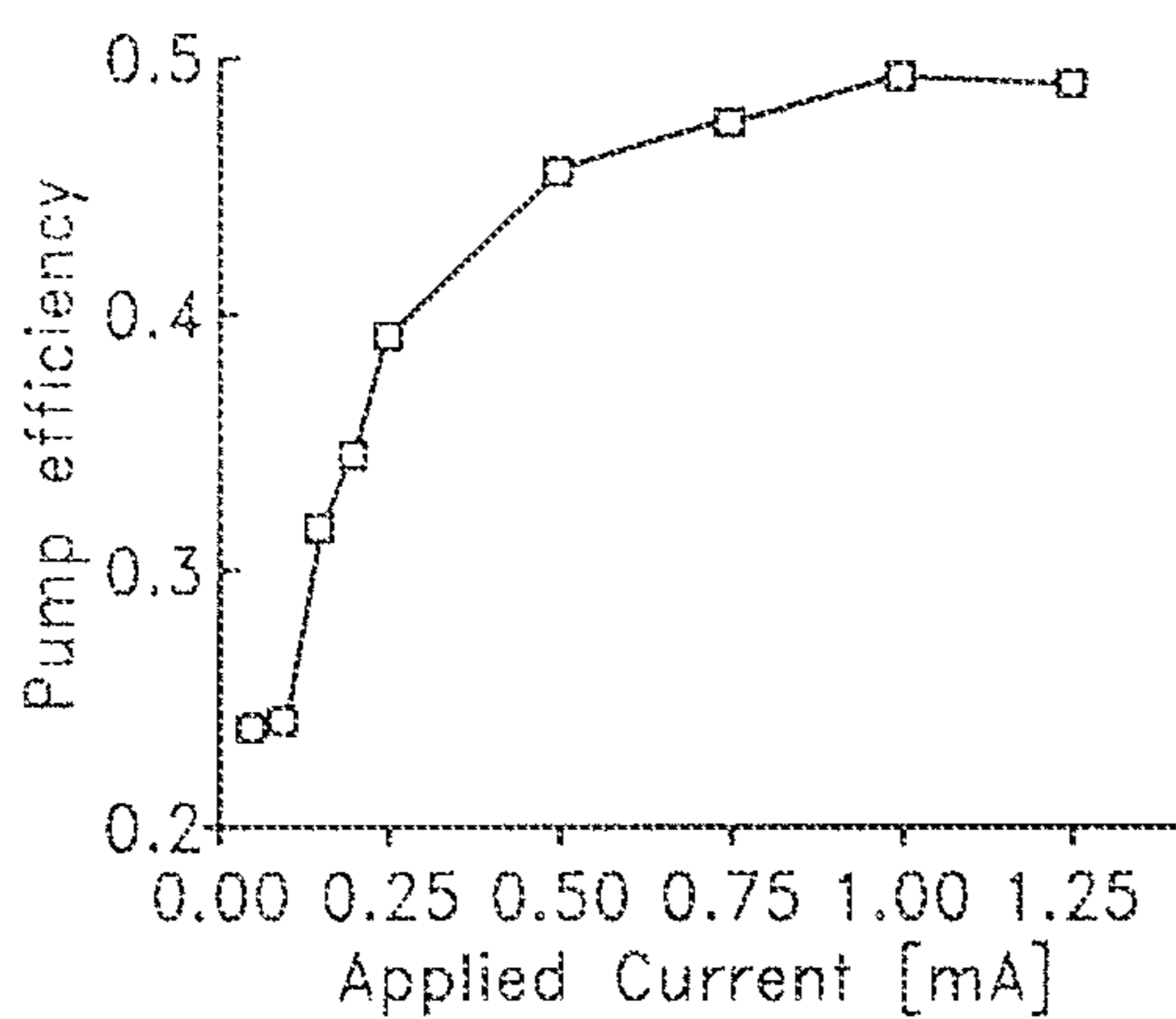
Pump efficiency
