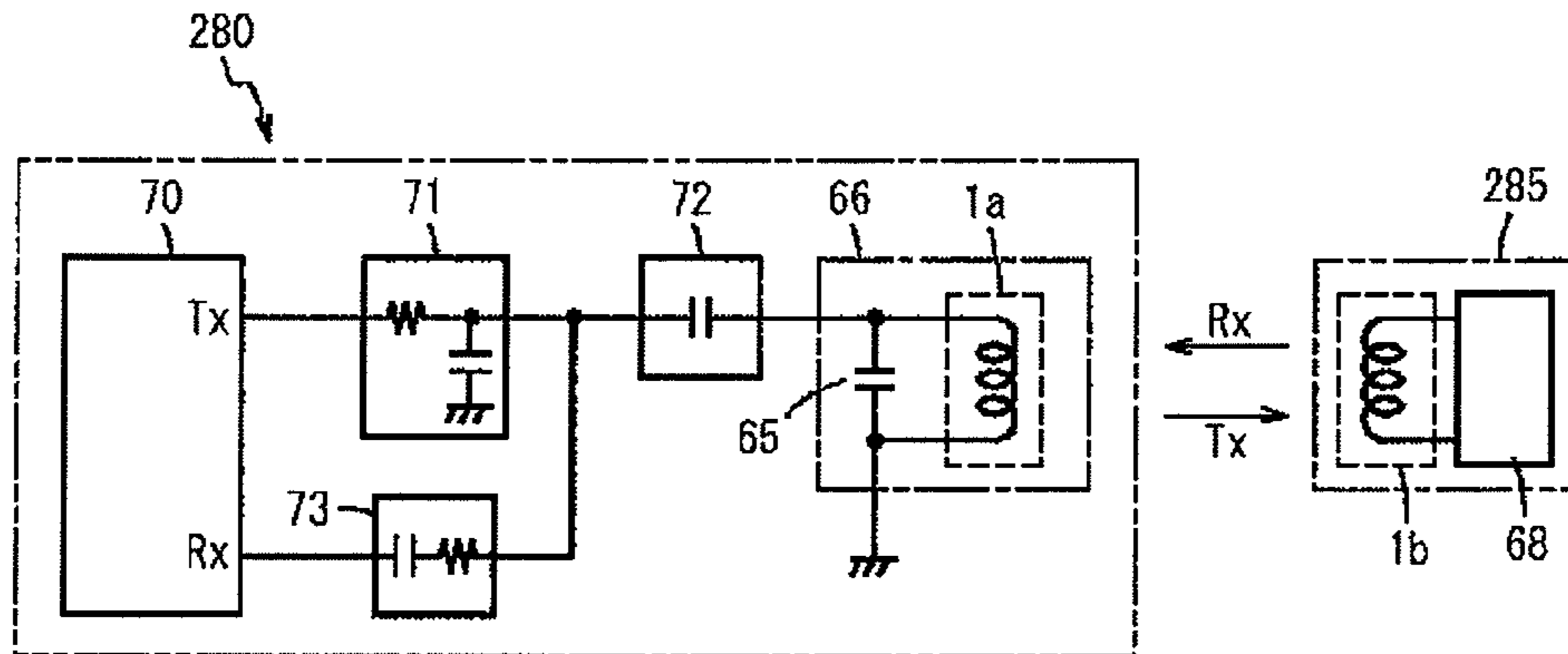
Fig. 24 CONVENTIONAL ART
