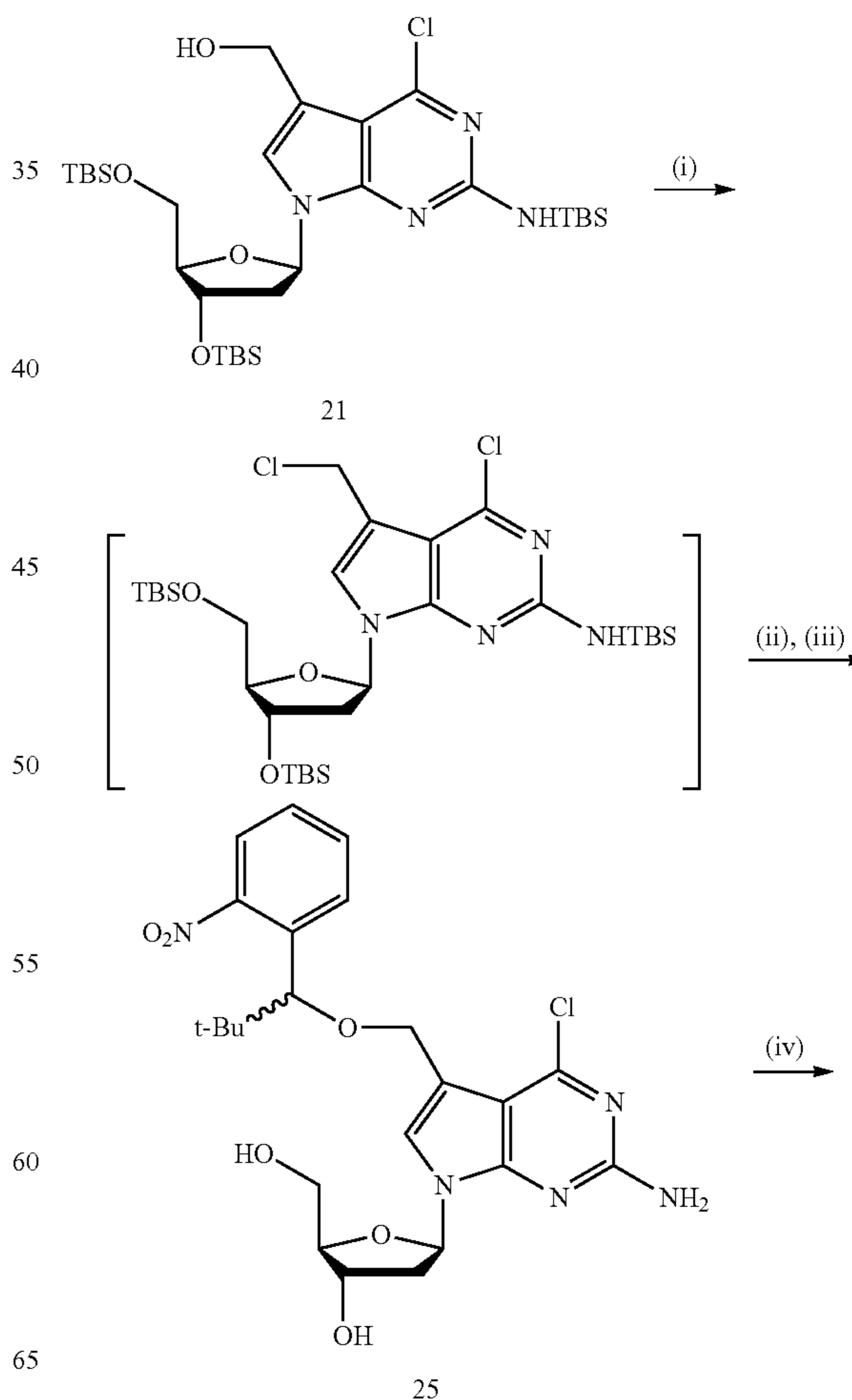
Scheme S13. Synthesis of 7-[1-(2-nitrophenyl)-2,2-dimethyl-propyloxy]methyl-7-deaza-2'-deoxy-guanosine-5'-triphosphate.
