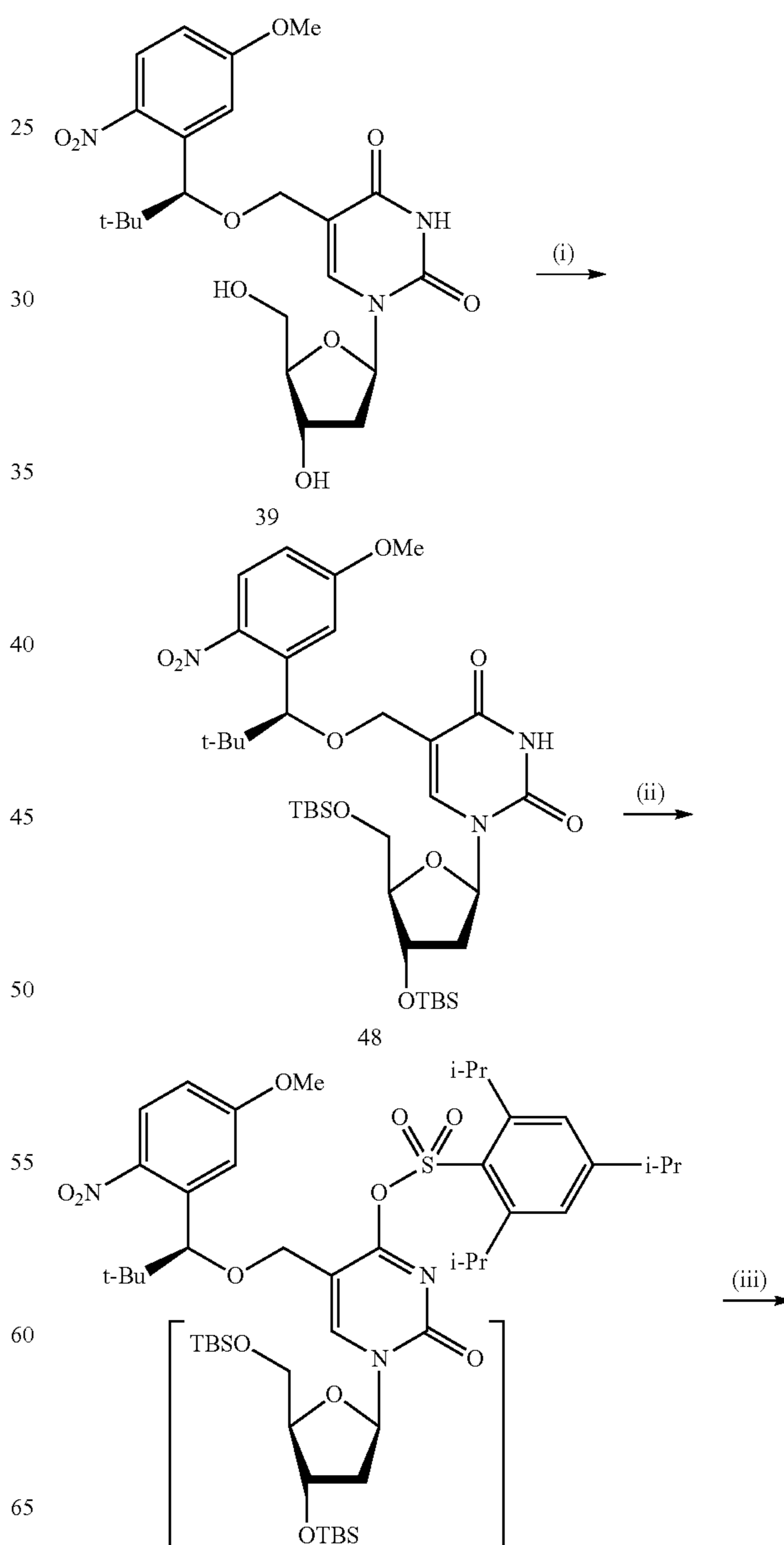
Scheme S22. Synthesis of 5-[(S)-1-(5-methoxy-2-nitrophenyl)-2,2-dimethyl-propyloxy]methyl-2'-deoxycytidine-5'-triphosphate.
