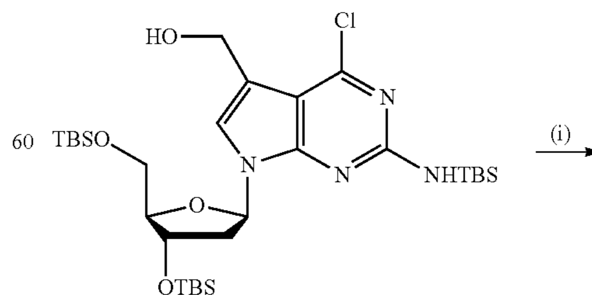
Scheme S14. Synthesis of 7-[(S)-1-(2-nitrophenyl)-2,2-dimethyl-propyloxy]methyl-7-deaza-2'-deoxy-guanosine-5'-triphosphate.
