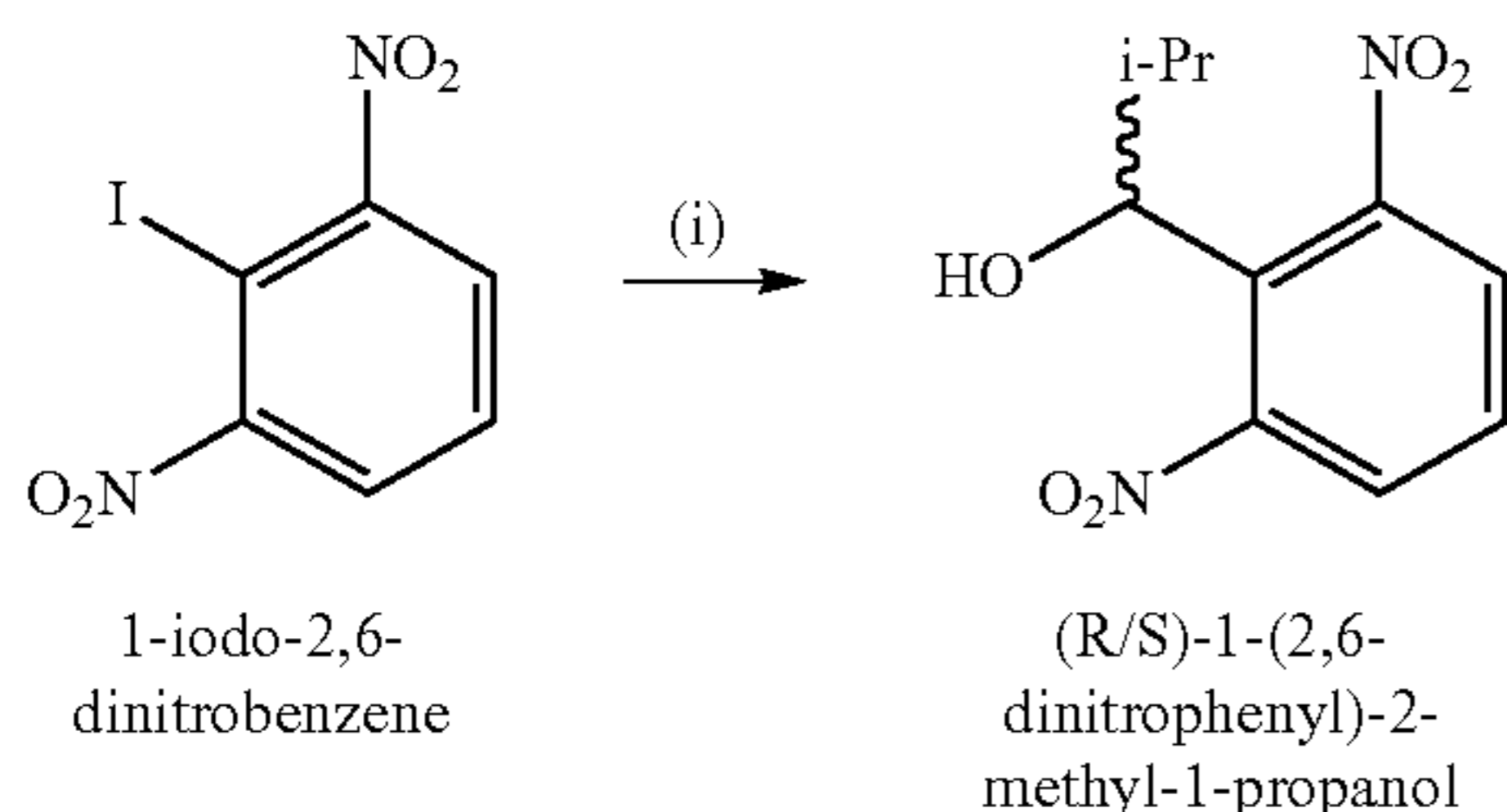
Scheme S1. Synthesis of (R/S)-1-(2,6-dinitrophenyl)-2-methyl-1-propanol.
