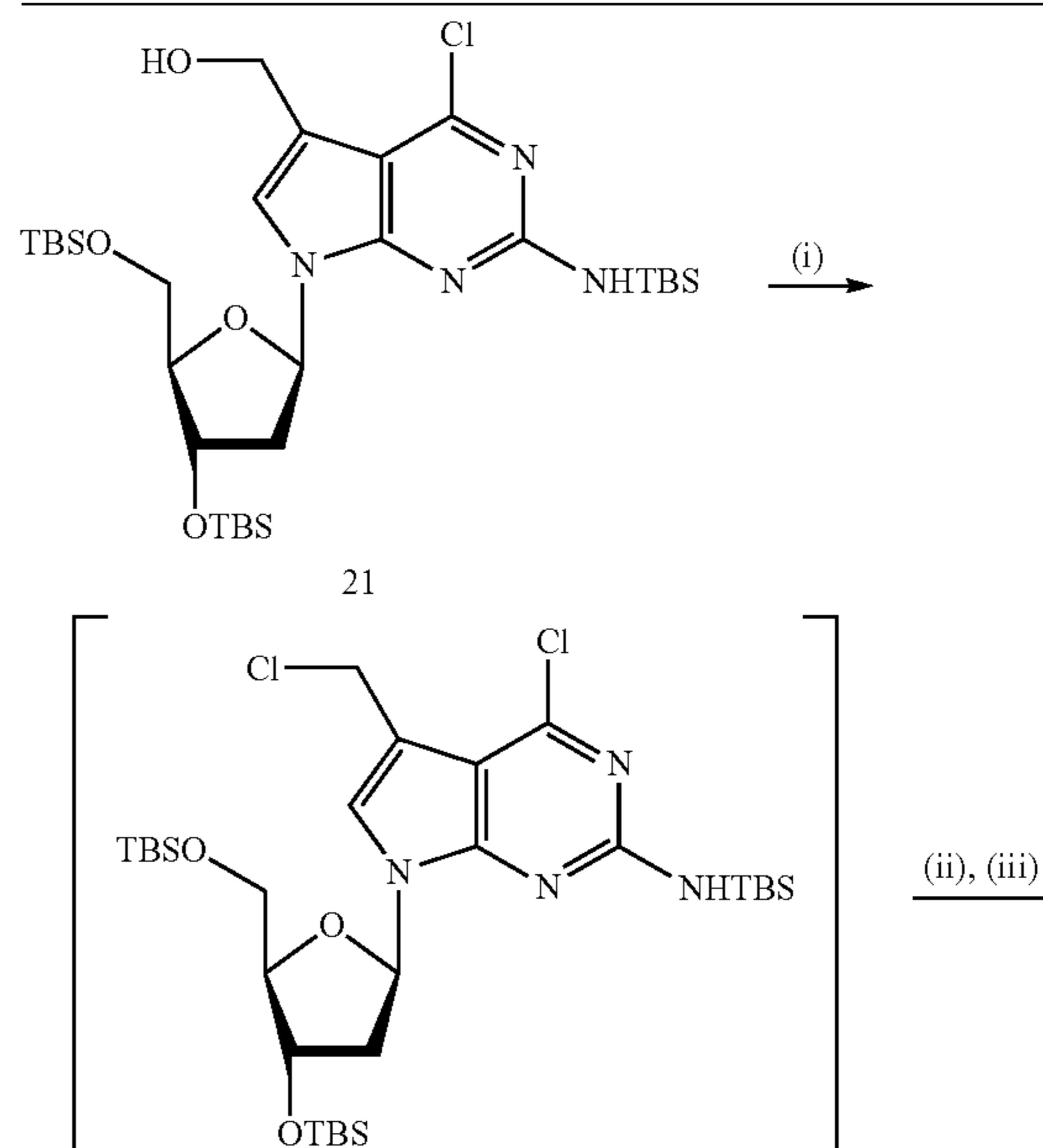
Scheme S16. Synthesis of 7-[1-(5-methoxy-2-nitrophenyl)-2,2-dimethyl-propyloxy]methyl-7-deaza-2'-deoxyguanosine-5'-triphosphate.
