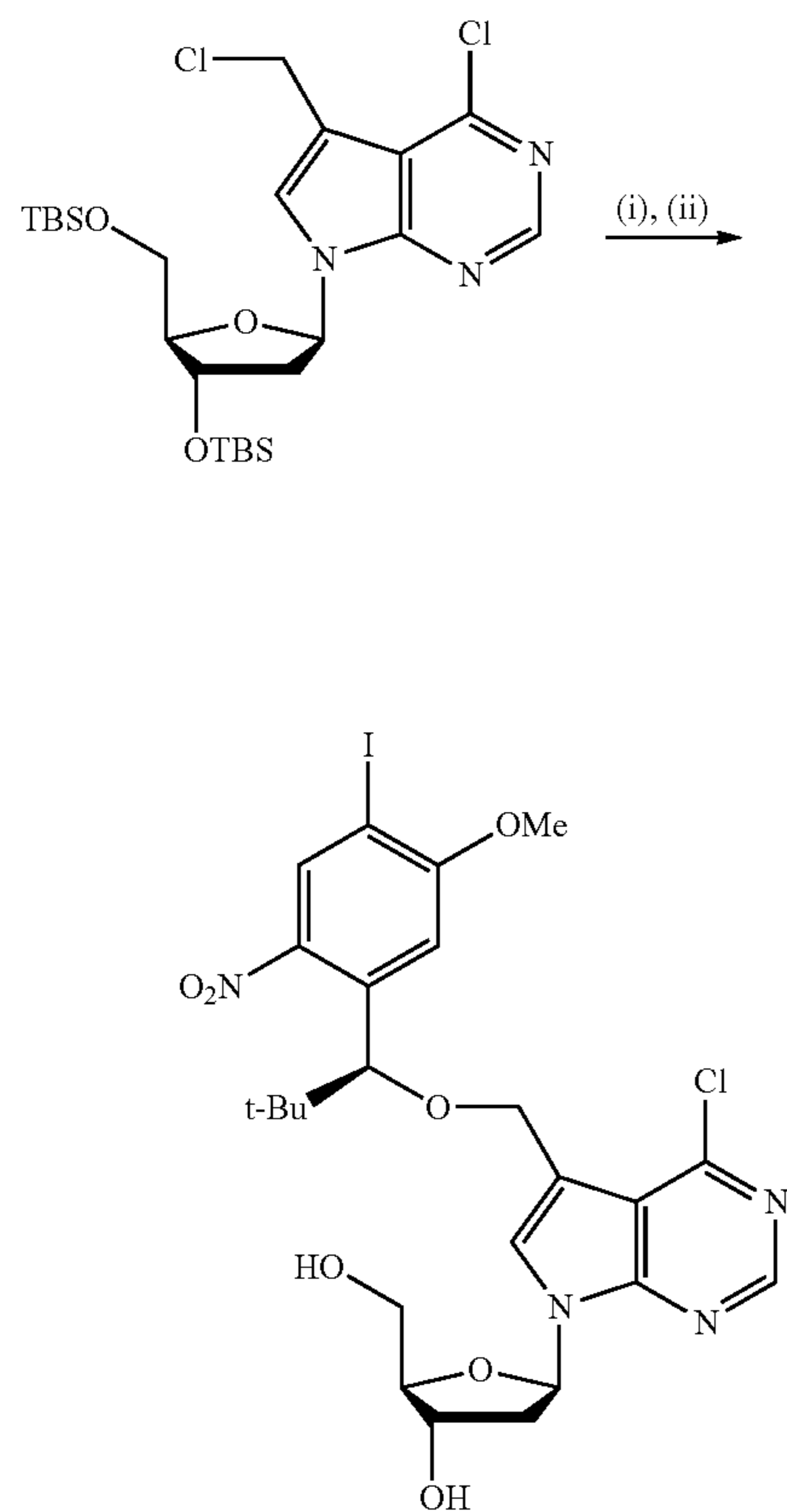
Scheme 2a. Synthesis of dye labeled 7-[(S)-1-(5-methoxy-2-nitrophenyl)- 2,2-dimethyl-propyloxy]methyl-7-deaza-2'- deoxyadenosine-5'-triphosphate.
