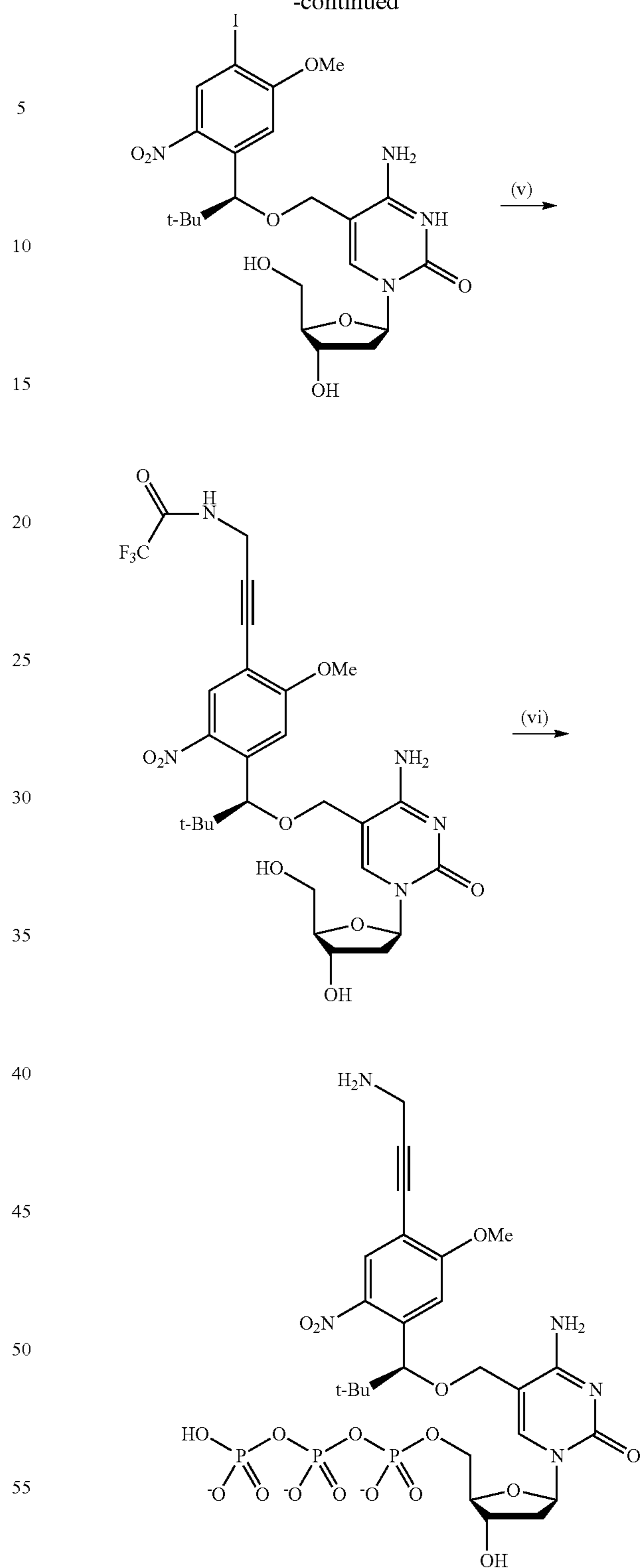
Scheme 5a. Synthesis of dye labeled 5-[(S)-1-(5-methoxy-2-nitrophenyl)-2,2-dimethyl-propyloxy]methyl-2'-deoxycytidine-5'-triphosphate.
