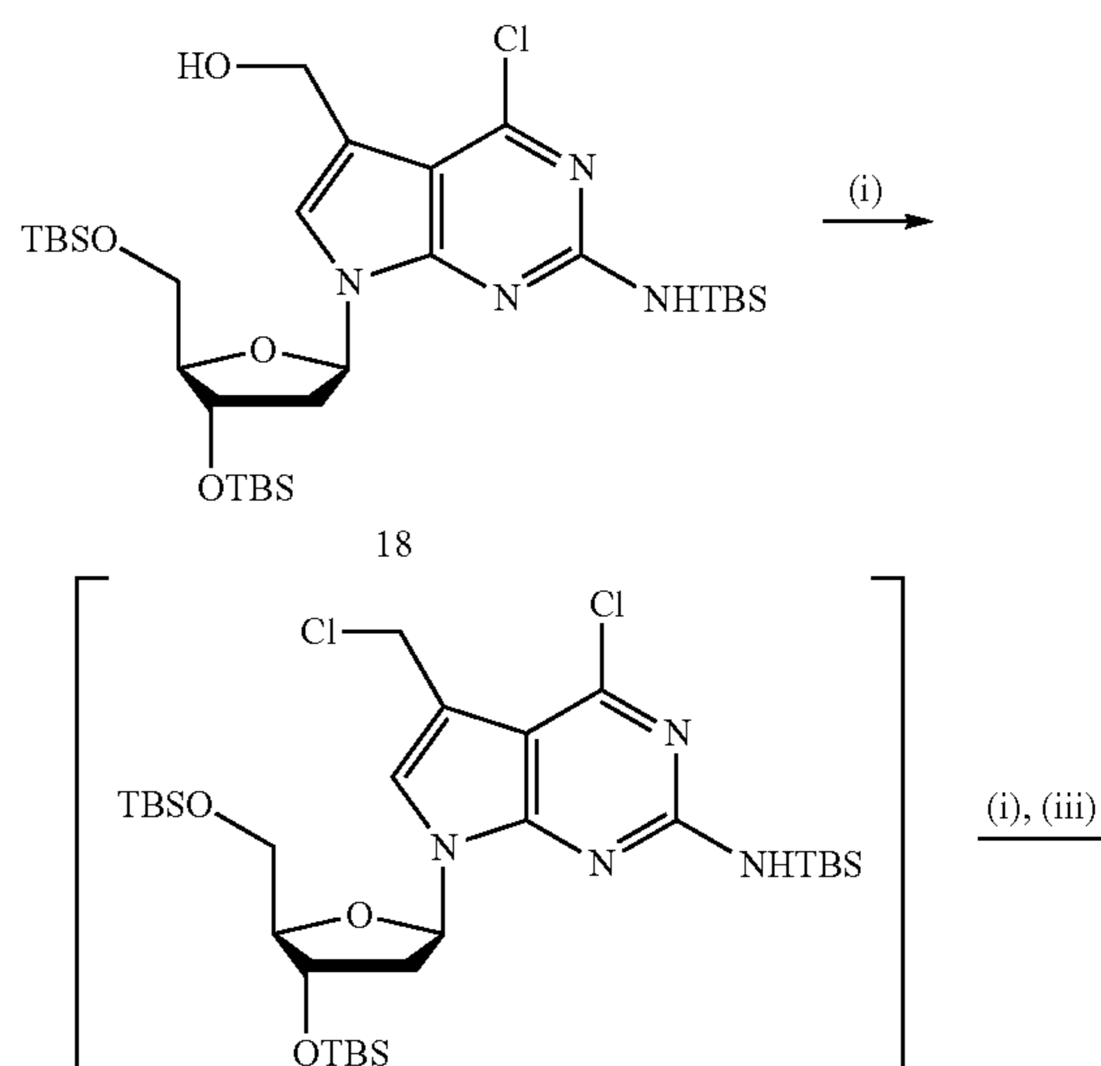
Scheme S26a. Synthesis of dye labeled 7-[(S)-1-[4-(3-amino-1-propynyl)-5-methoxy-2-nitrophenyl]-2,2-dimethyl-propyloxy}methyl-7-deaza-2'-deoxyguanosine-5'-triphosphate and 5'-α-thiotriphosphate.
