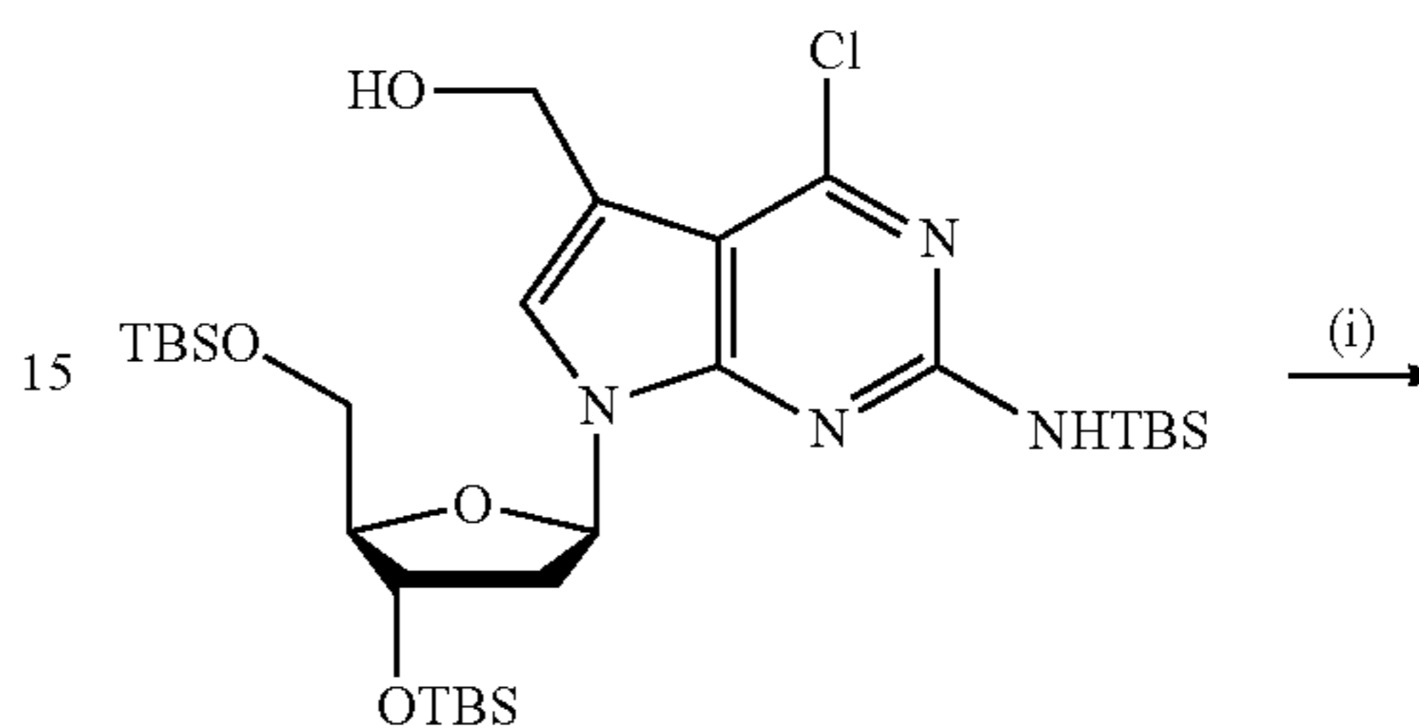
Scheme 4a. Synthesis of dye labeled 7-[(S)-1-(5-methoxy-2-nitrophenyl)-2,2-dimethyl-propyloxy]methyl-7-deaza-2'-deoxyguanosine-5'-triphosphate.
