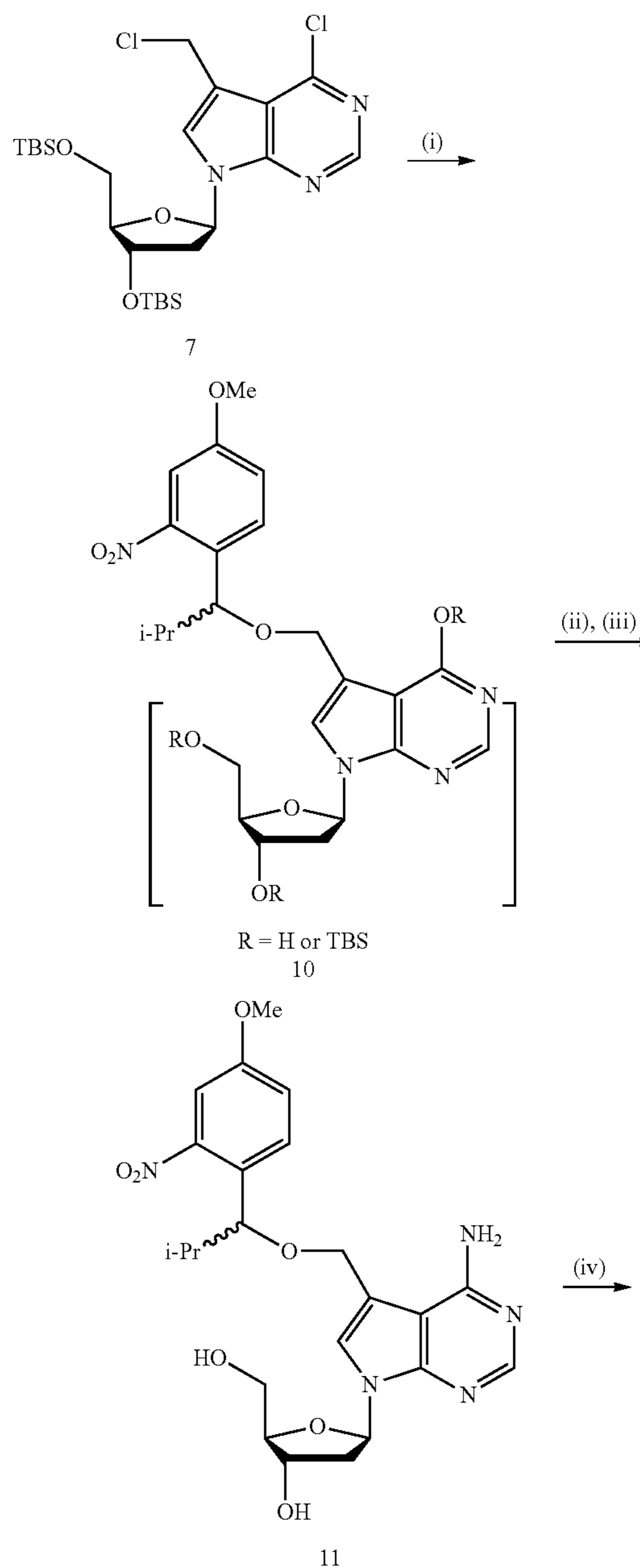
Scheme S8. Synthesis of 7-[1-(4-methoxy-2-nitrophenyl)-2-methyl-propyloxy]methyl-7-deaza-2'-deoxyadenosine-5'-triphosphate.
