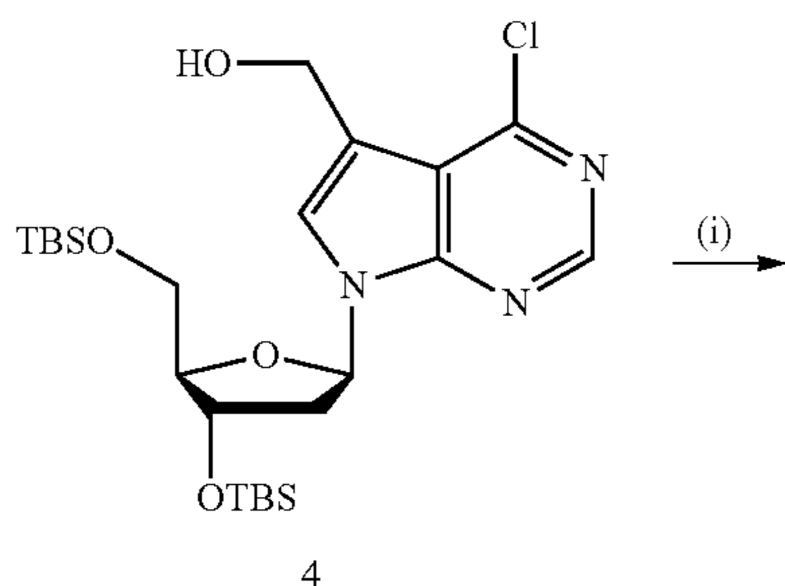
Scheme S7. Synthesis of 7-[1-(2-nitrophenyl)-2-methyl-propyloxy]methyl-7-deaza-2'-deoxyadenosine-5'-triphosphate.
