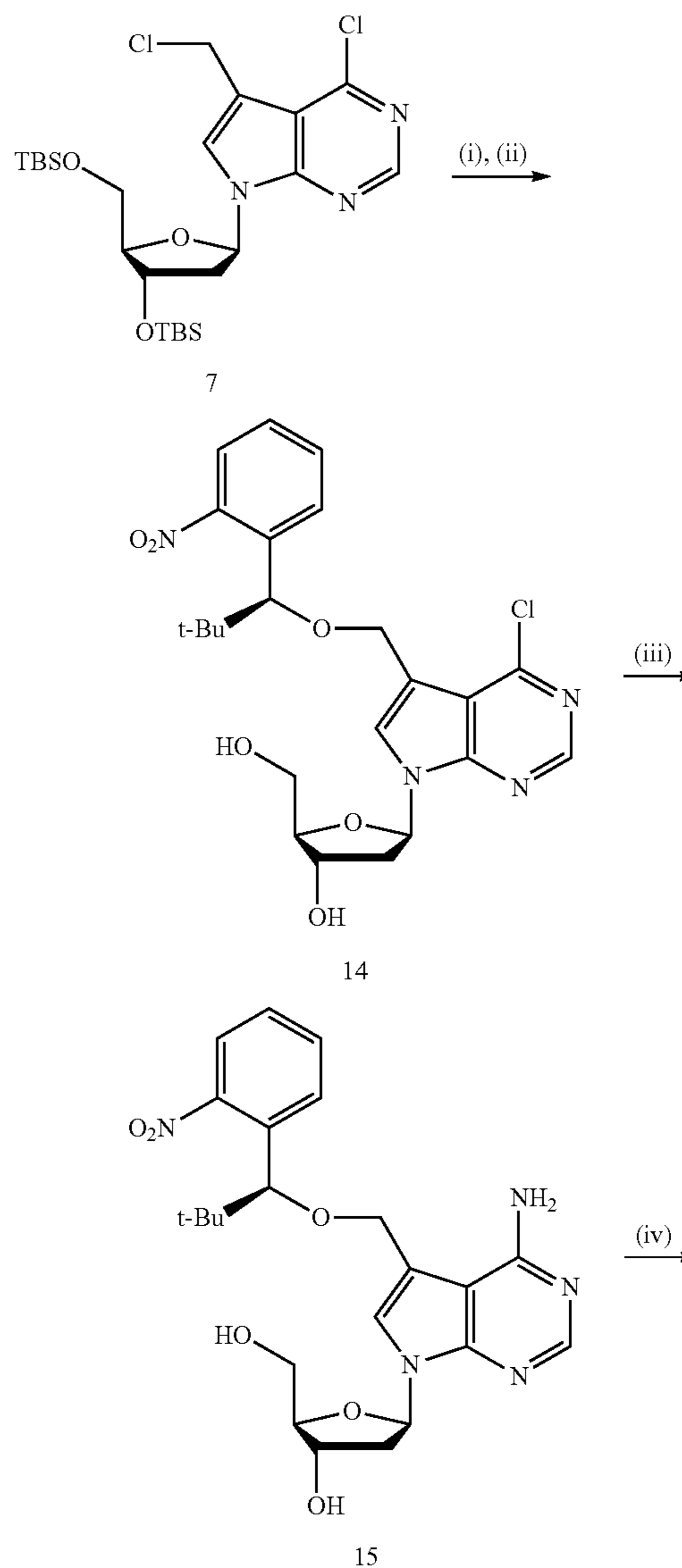
Scheme S10. Synthesis of 7-[(S)-1-(2-nitrophenyl)-2,2-dimethyl-propyloxy]methyl-7-deaza-2'-deoxyadenosine-5'-triphosphate.
