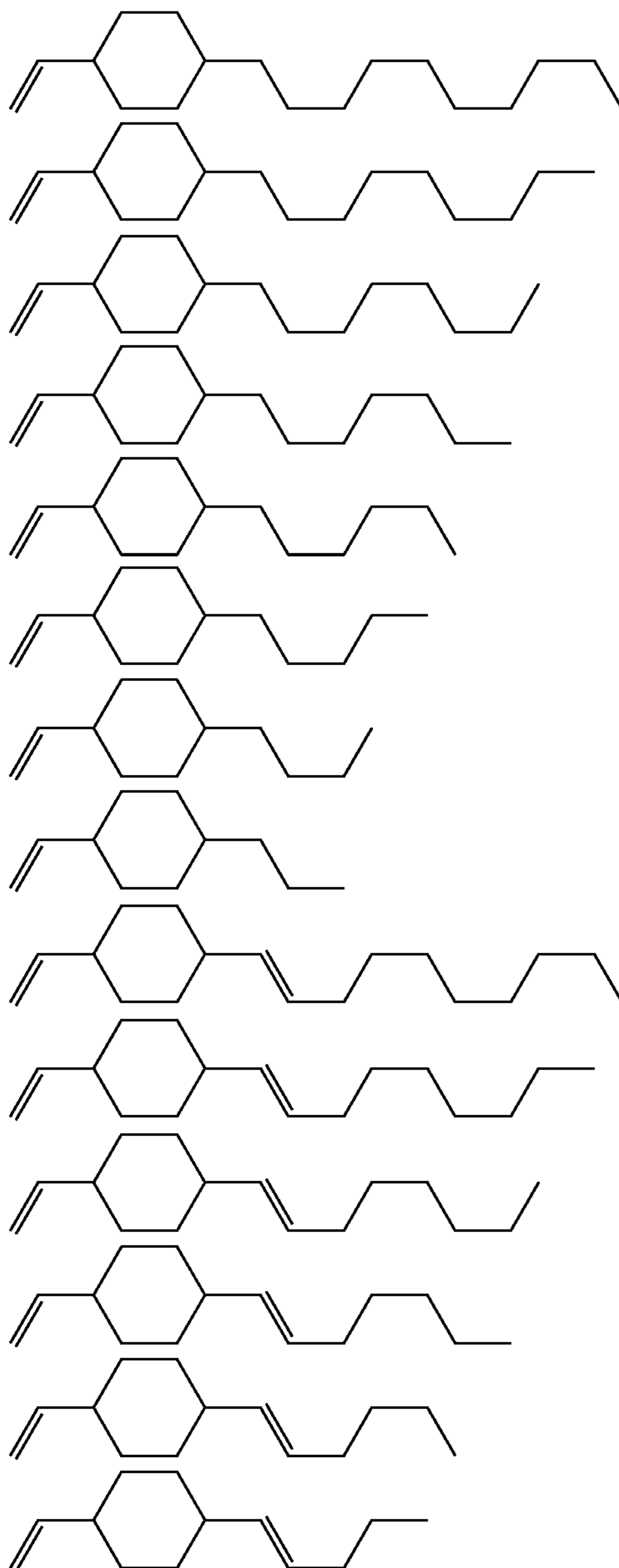
[Chem. 74]
