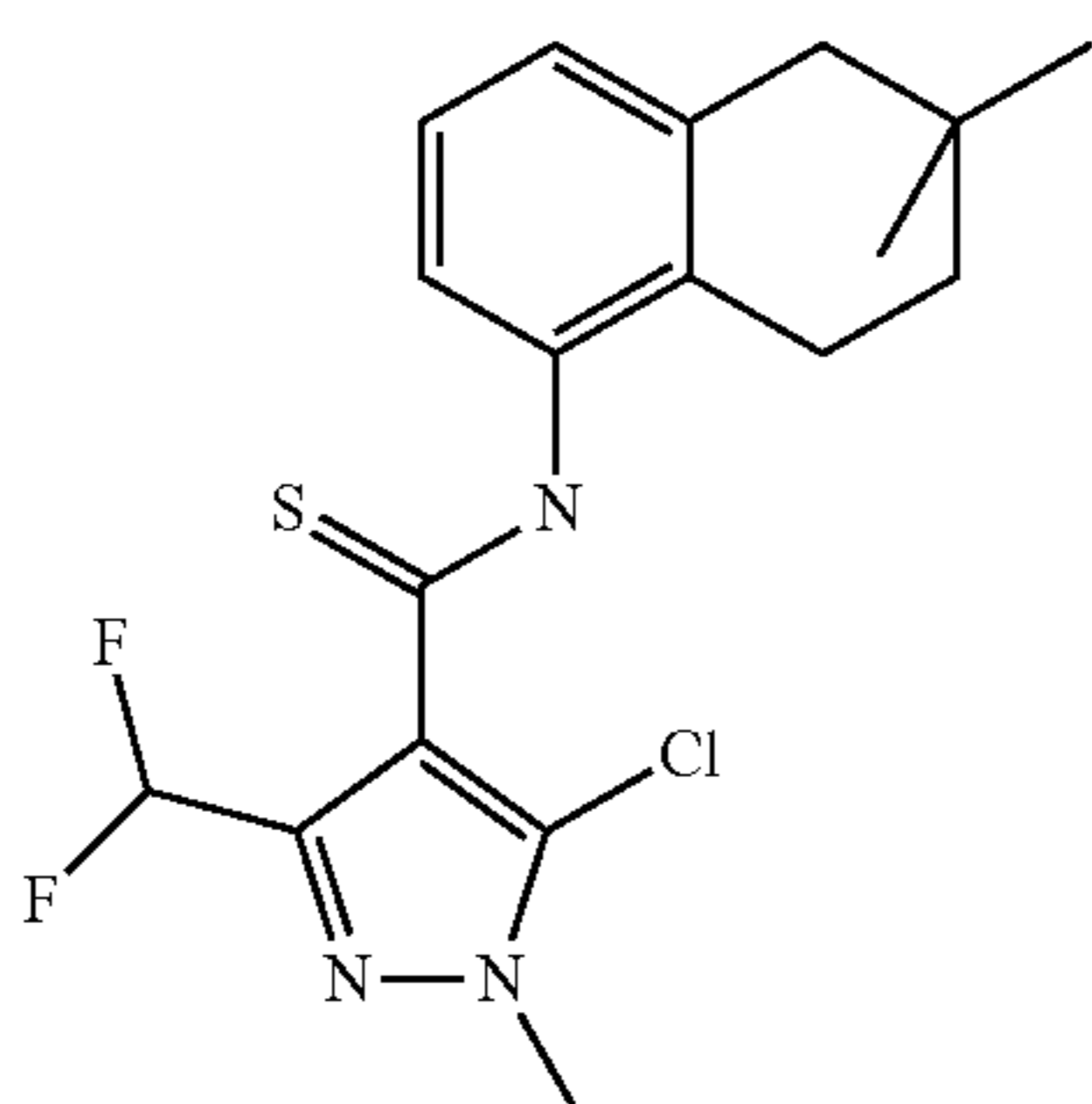
5-chloro-3-(difluoromethyl)-N-(6,6-dimethyl-5,6,7,8-tetrahydronaphthalen-1-yl)-1-methyl-1H-pyrazole-4-carbothioamide (example 33)
