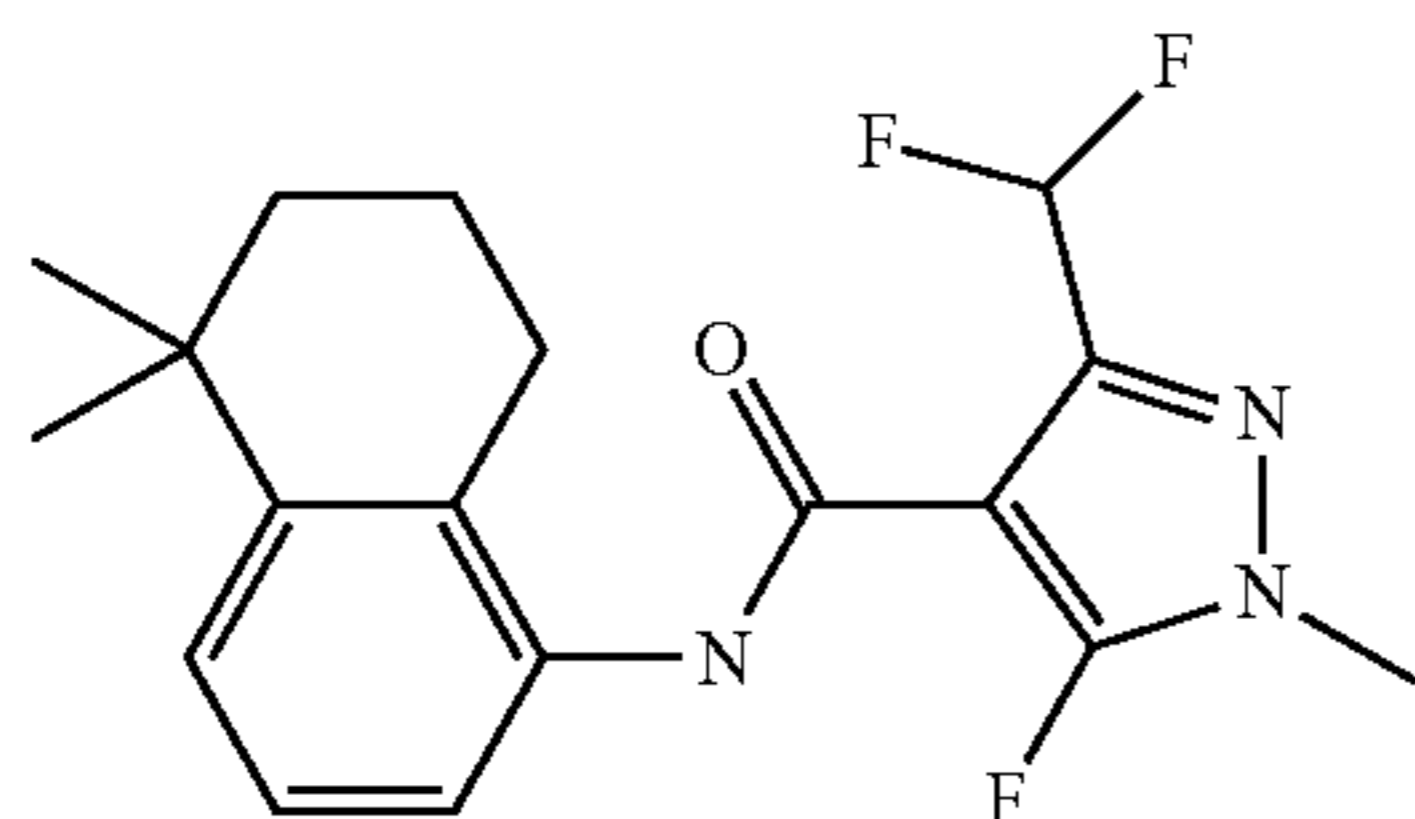
5-fluoro-3-(difluoromethyl)-N-(5,5-dimethyl-5,6,7,8-tetrahydronaphthalen-1-yl)-1-methyl-1H-pyrazole-4-carboxamide
