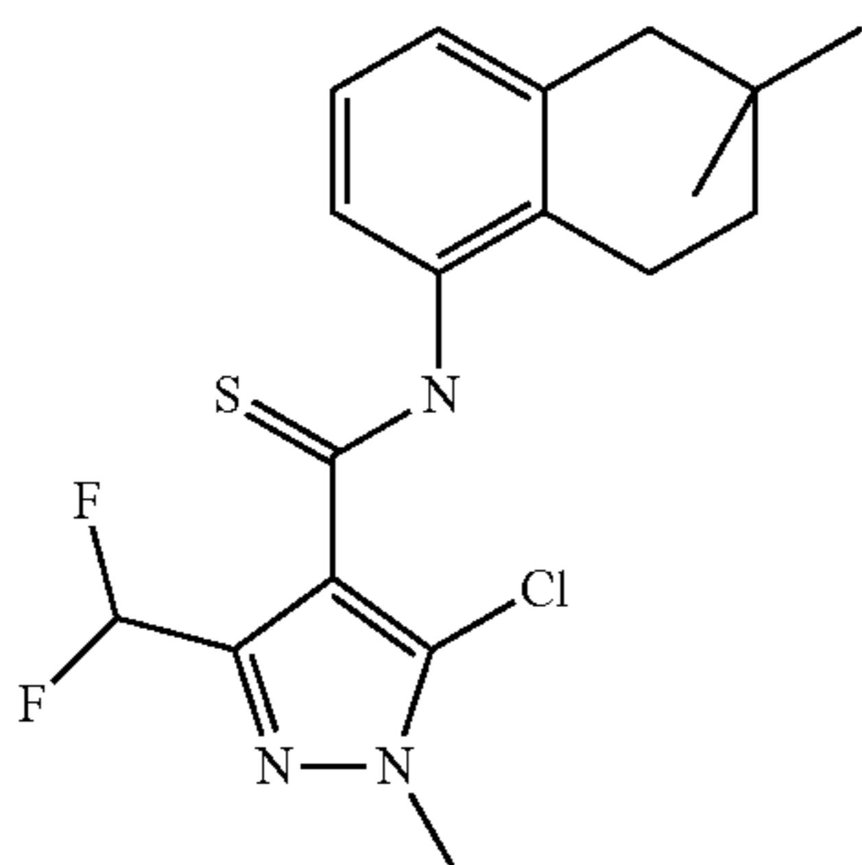
5-chloro-3-(difluoromethyl)-N-(6,6-dimethyl-5,6,7,8-tetrahydronaphthalen-1-yl)-1-methyl-1H-pyrazole-4-carbothioamide (example 33)
