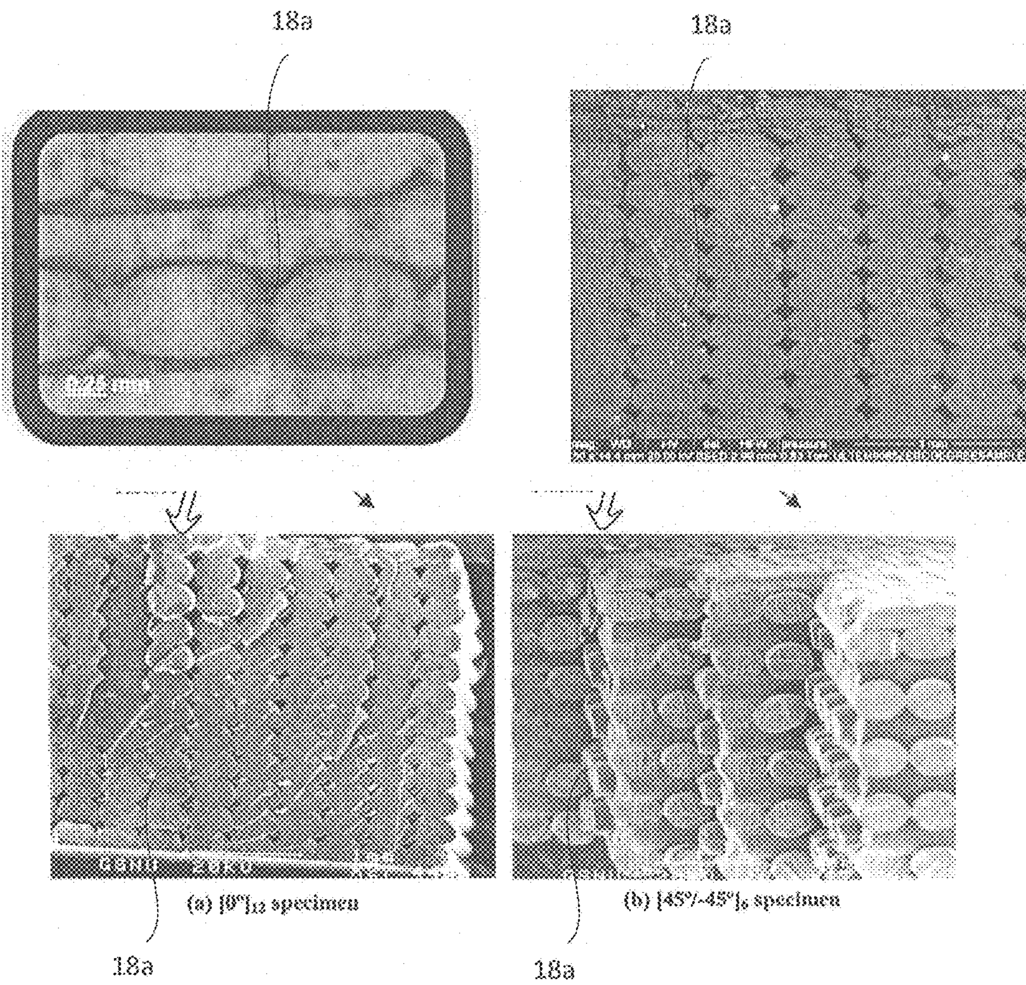
FIG. 1D FFF CROSS SECTIONS
