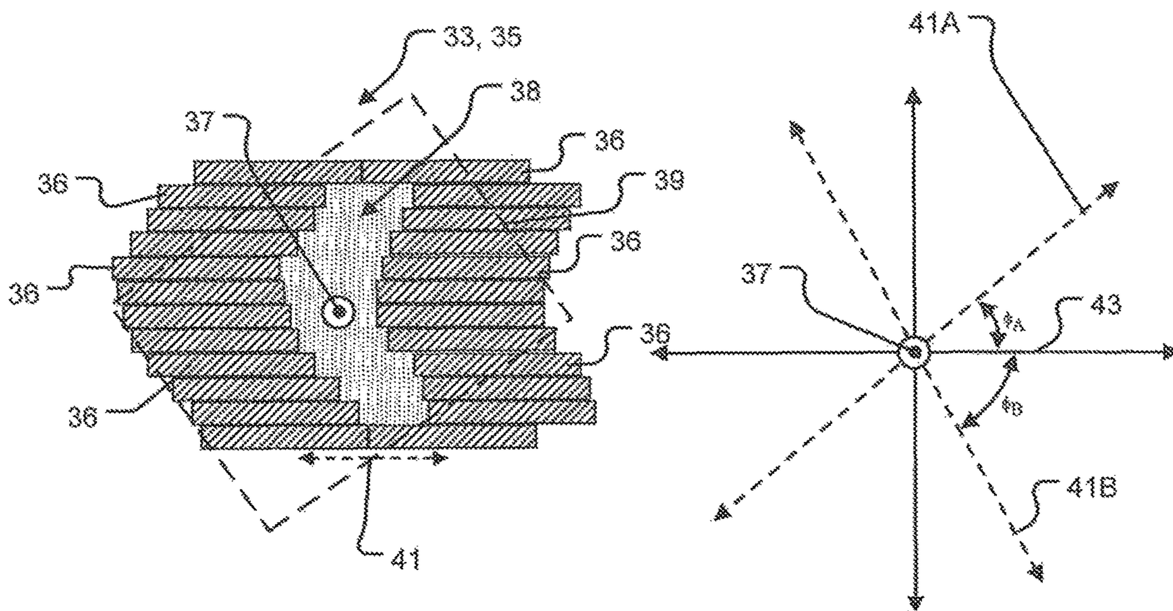
FIGURE 3B
