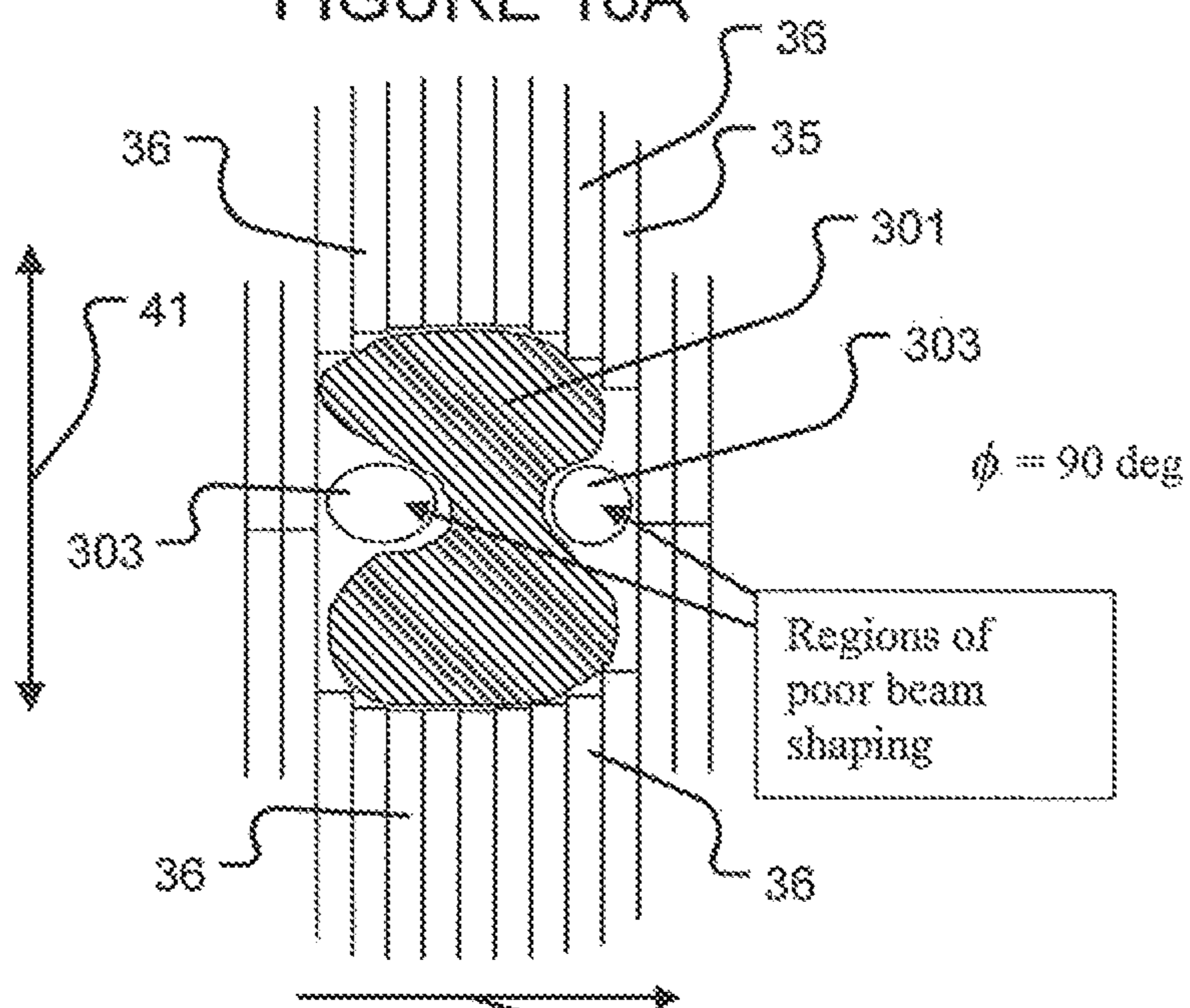
FIGURE 16A
