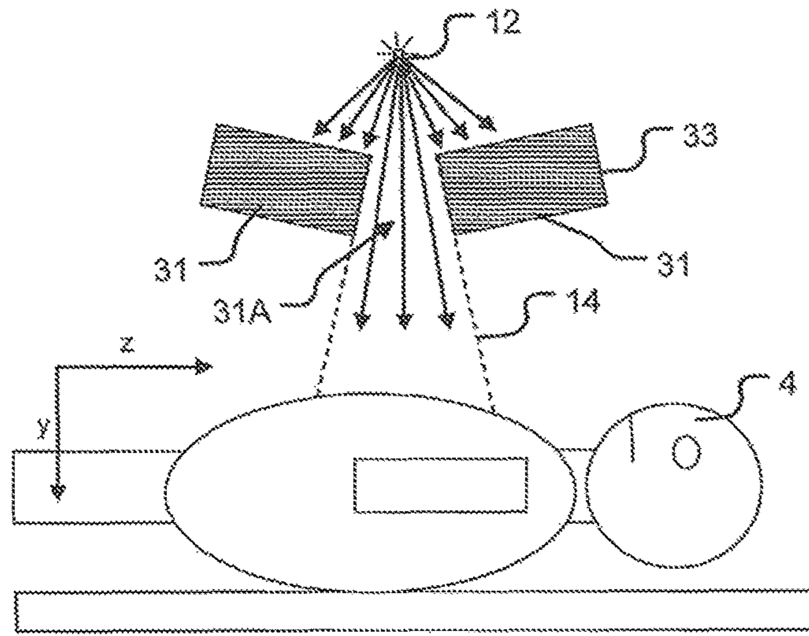
FIGURE 3A
