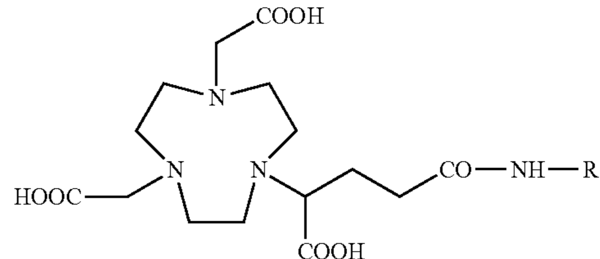
NODAGA-R
