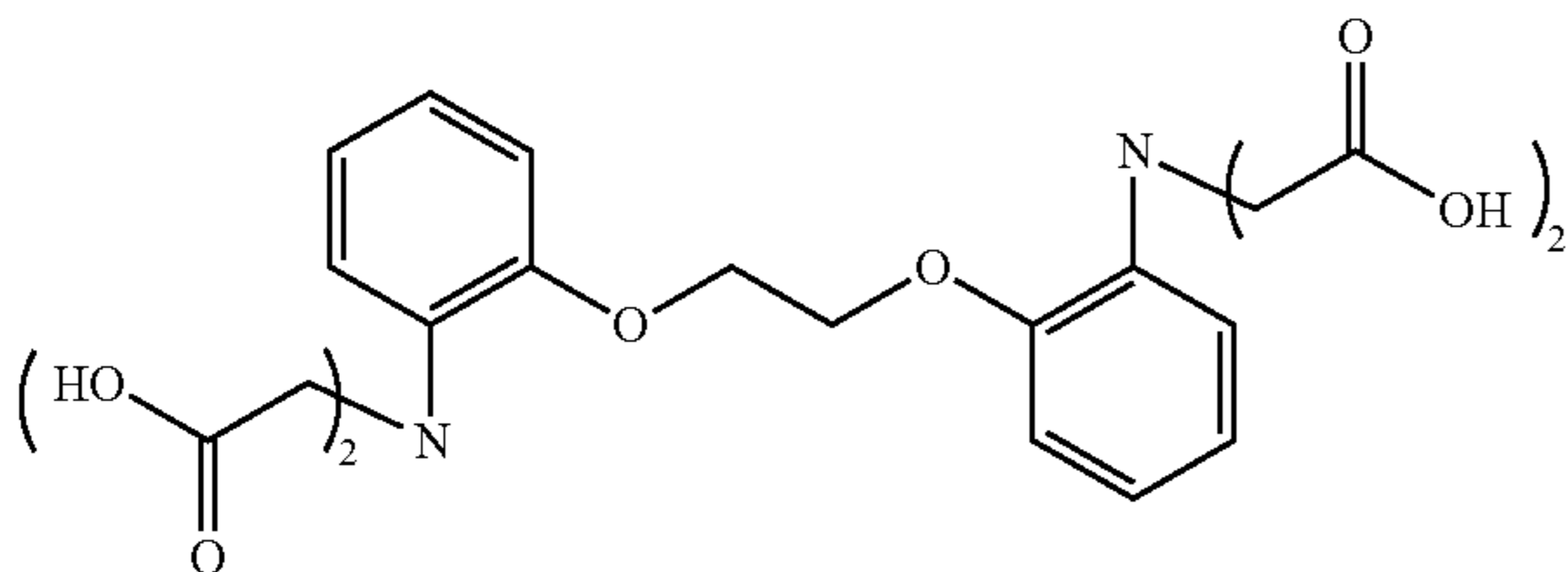
BAPTA
