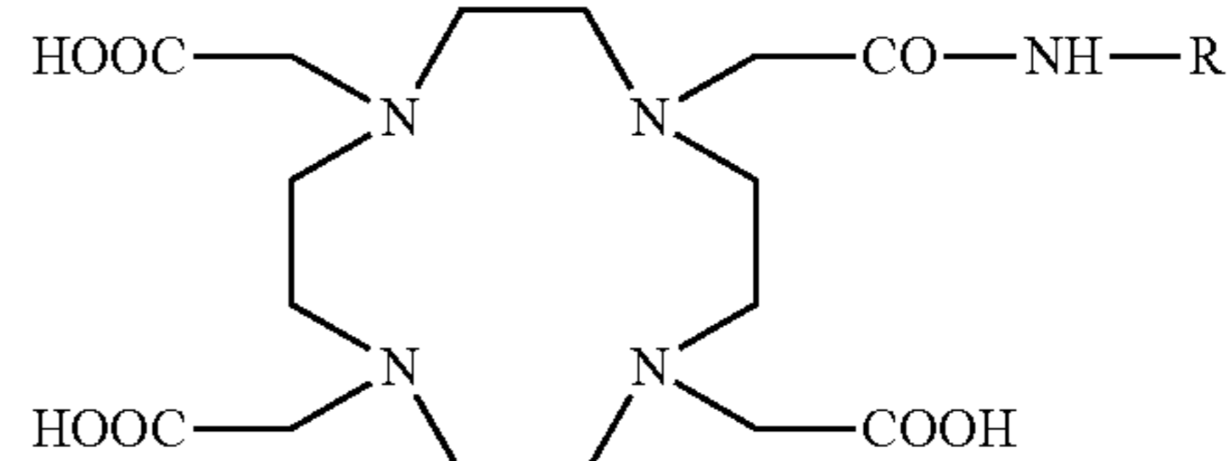
DOTA-R
