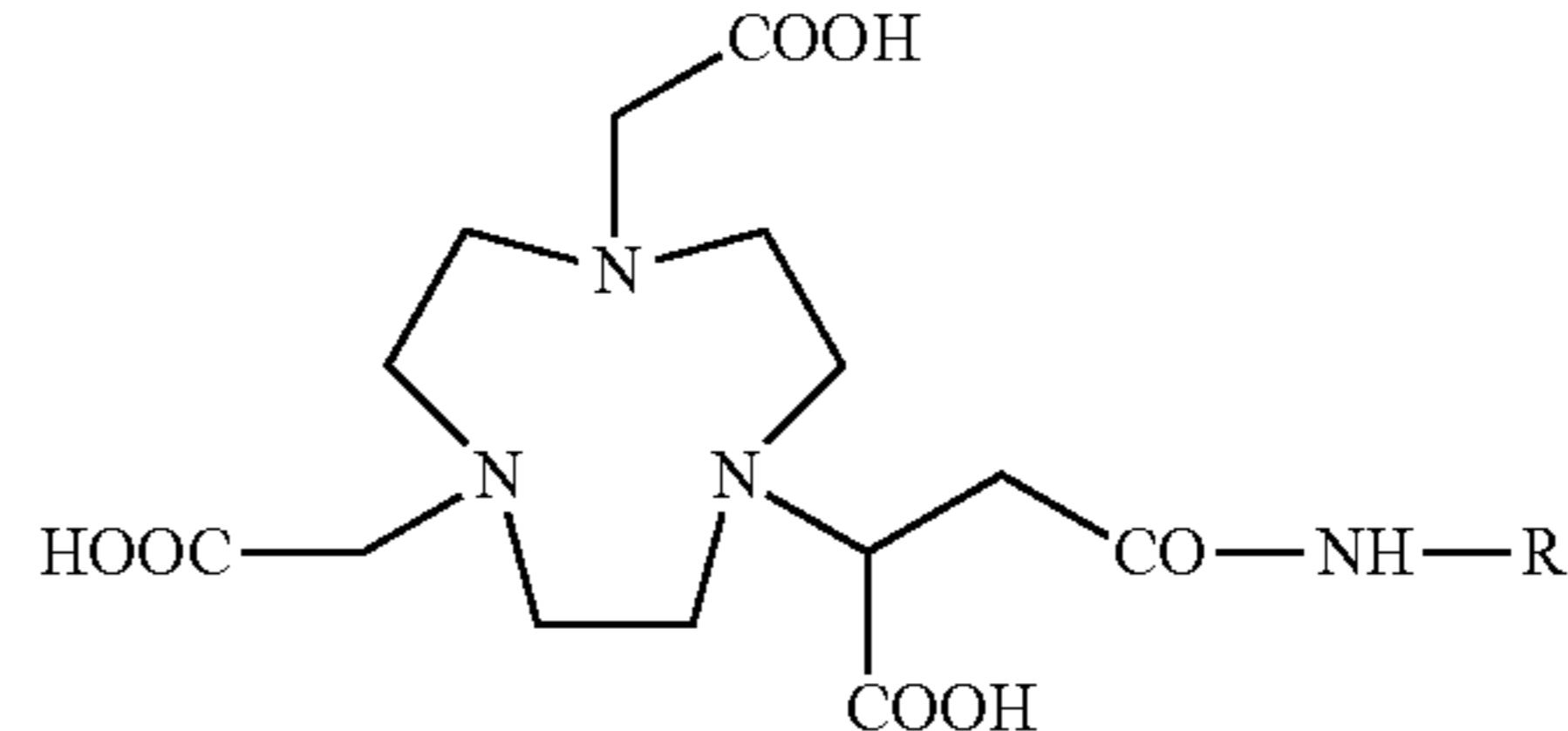
NODASA-R
