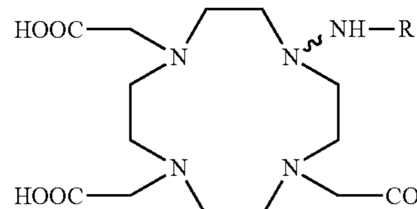
DO3A-R
