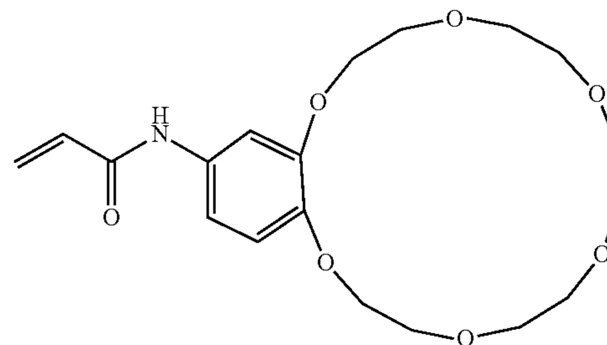
Compound B
