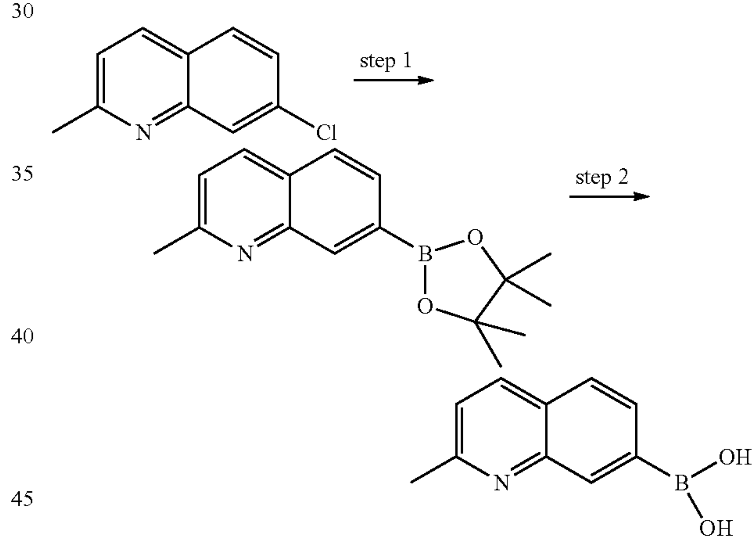
Scheme 29:
