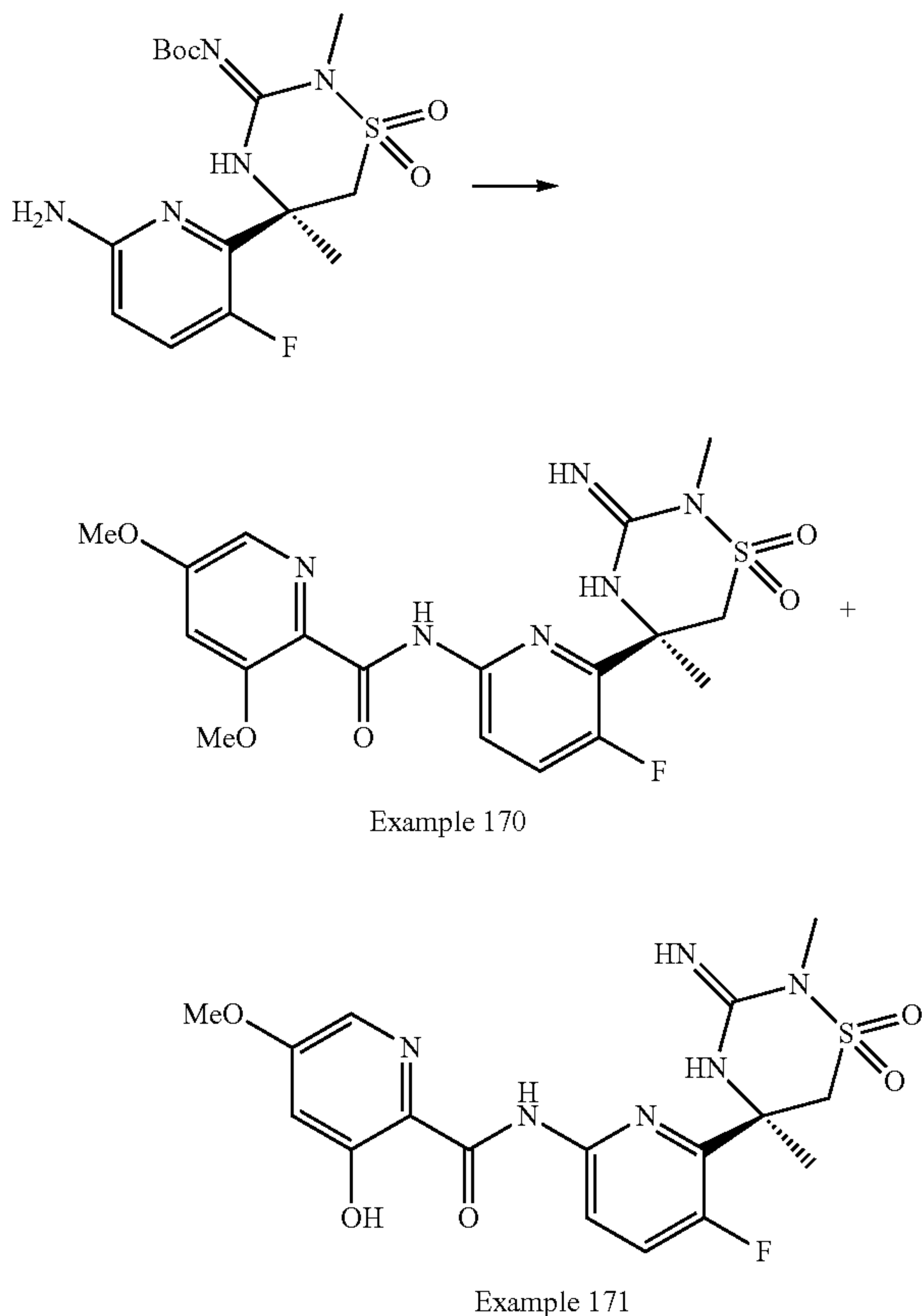
Scheme 42:
