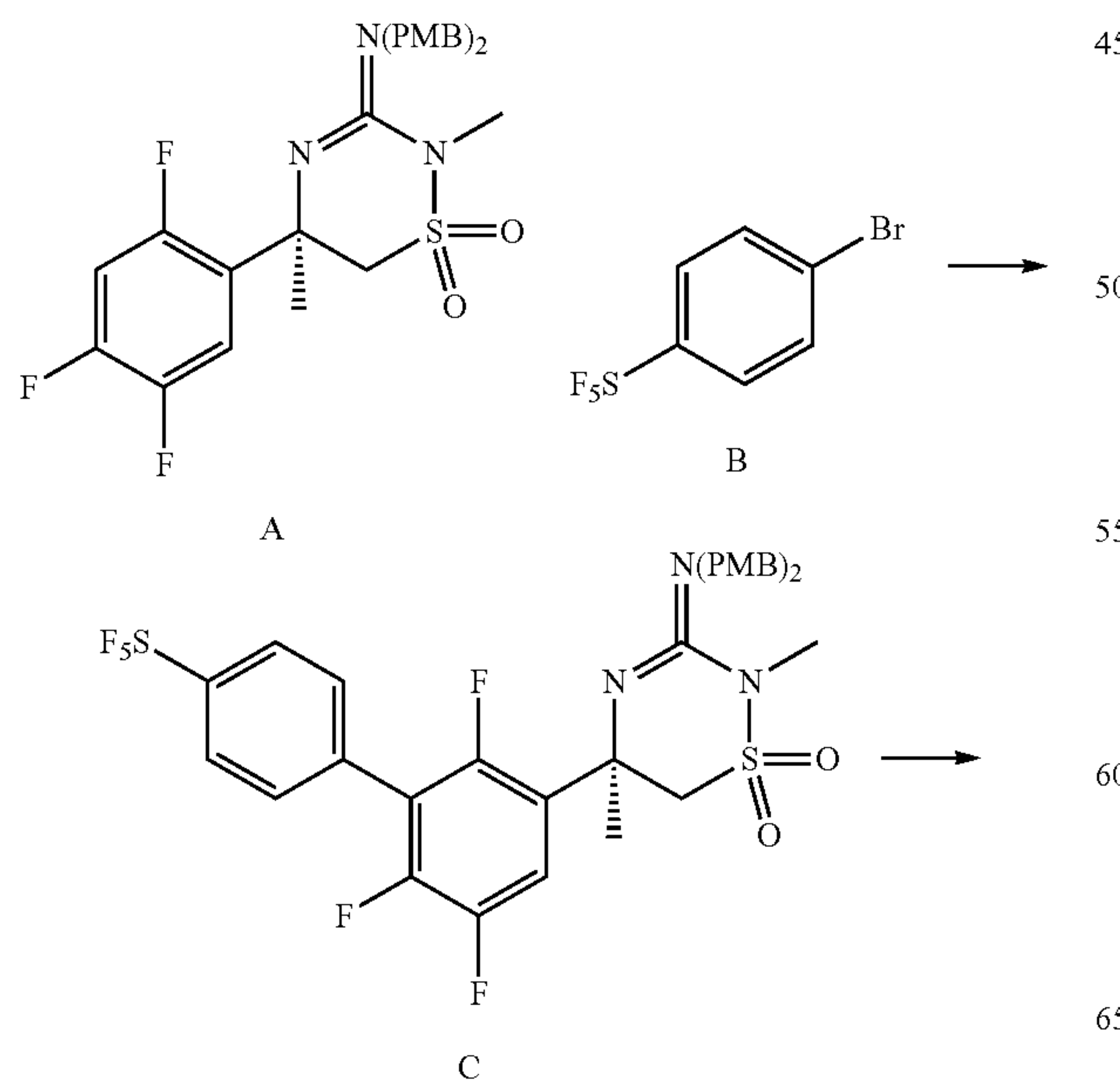
Scheme 5:
