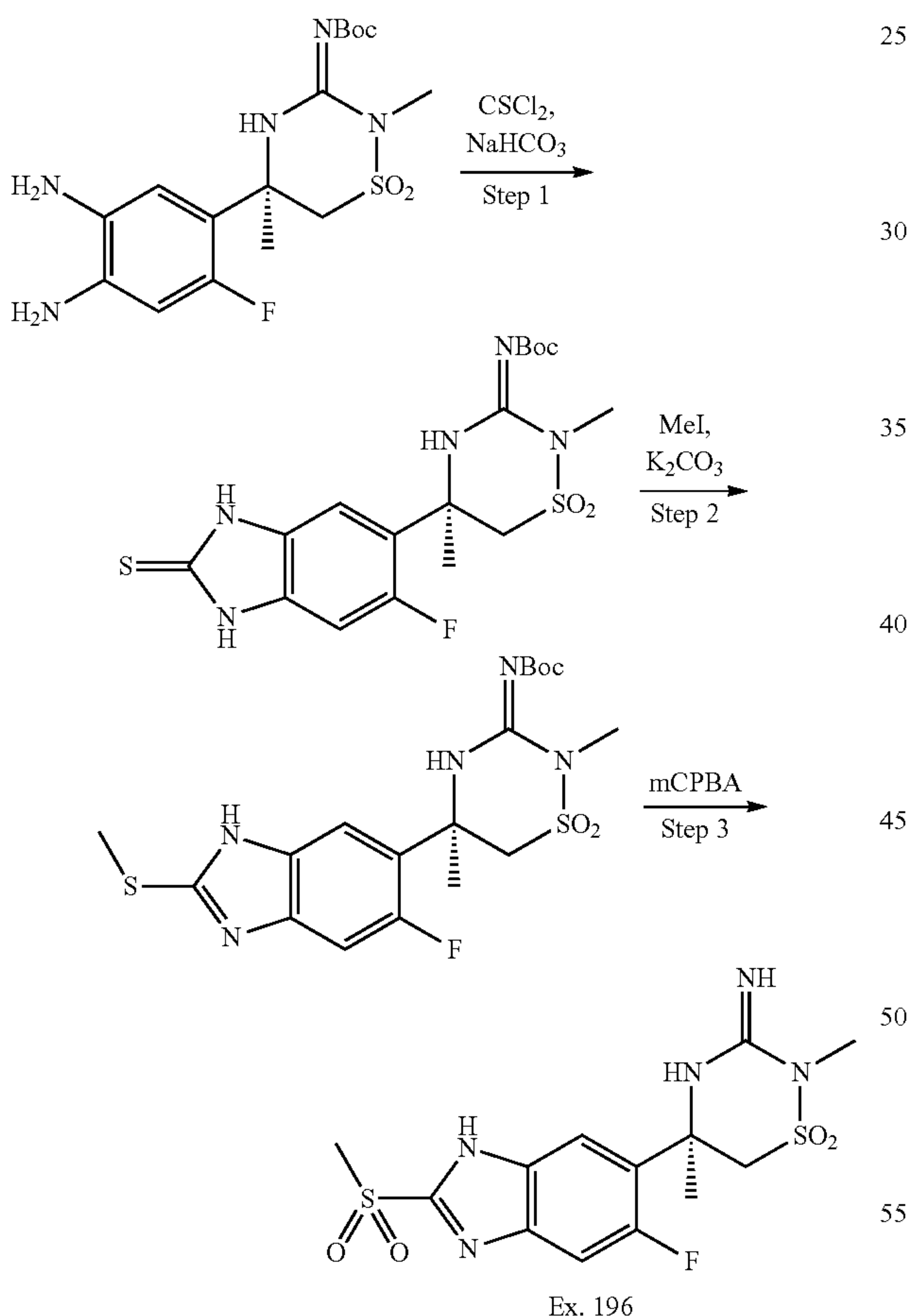
Scheme 50:
