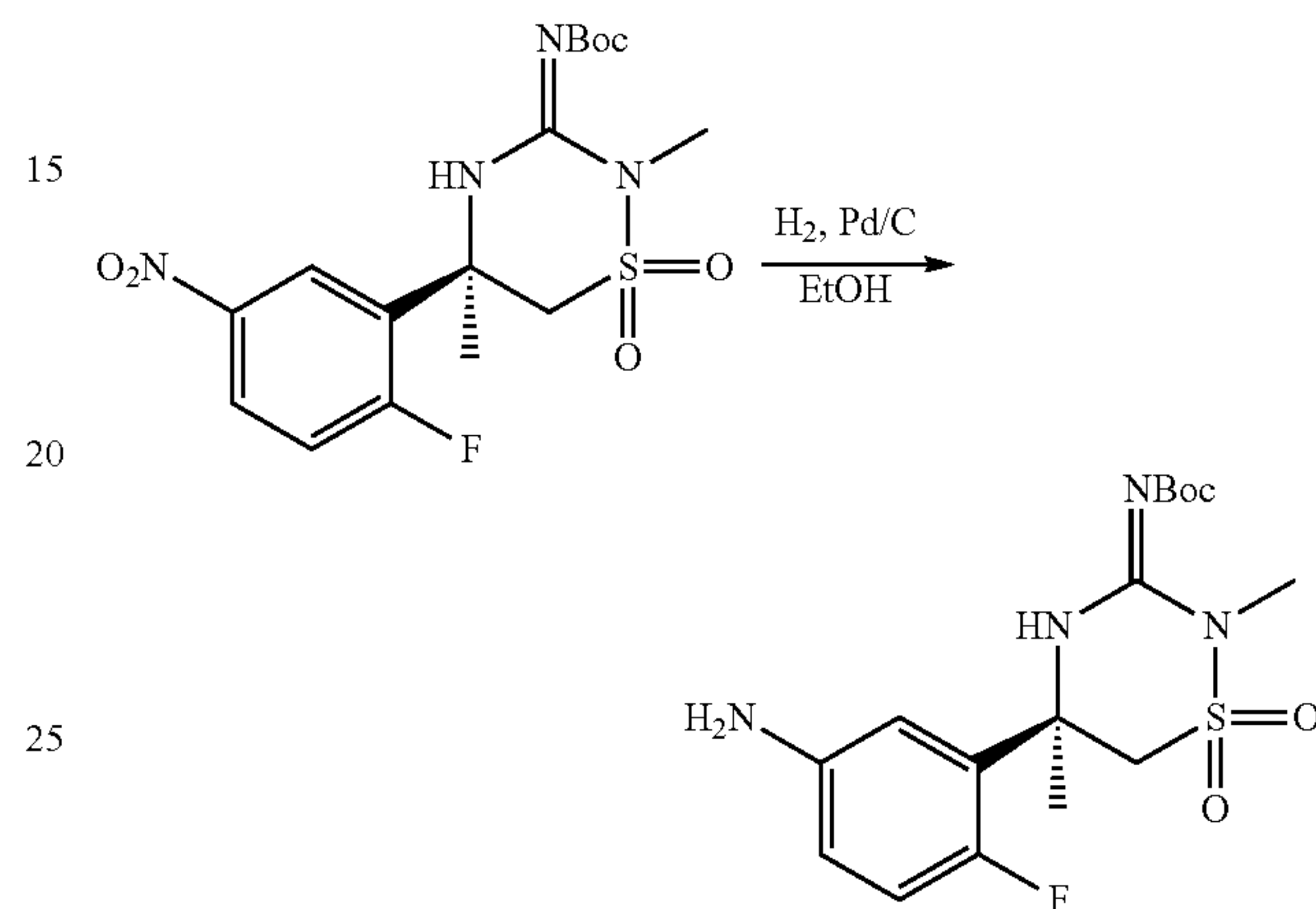
Scheme 10:
