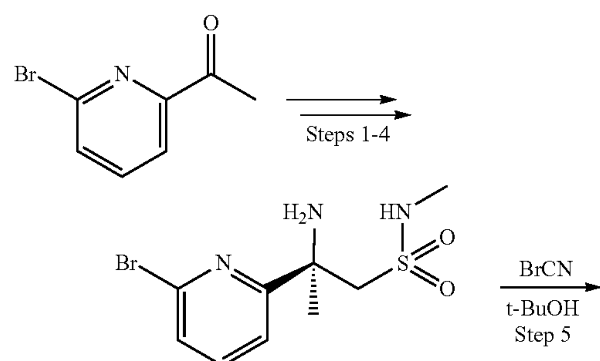
Scheme 7a:
