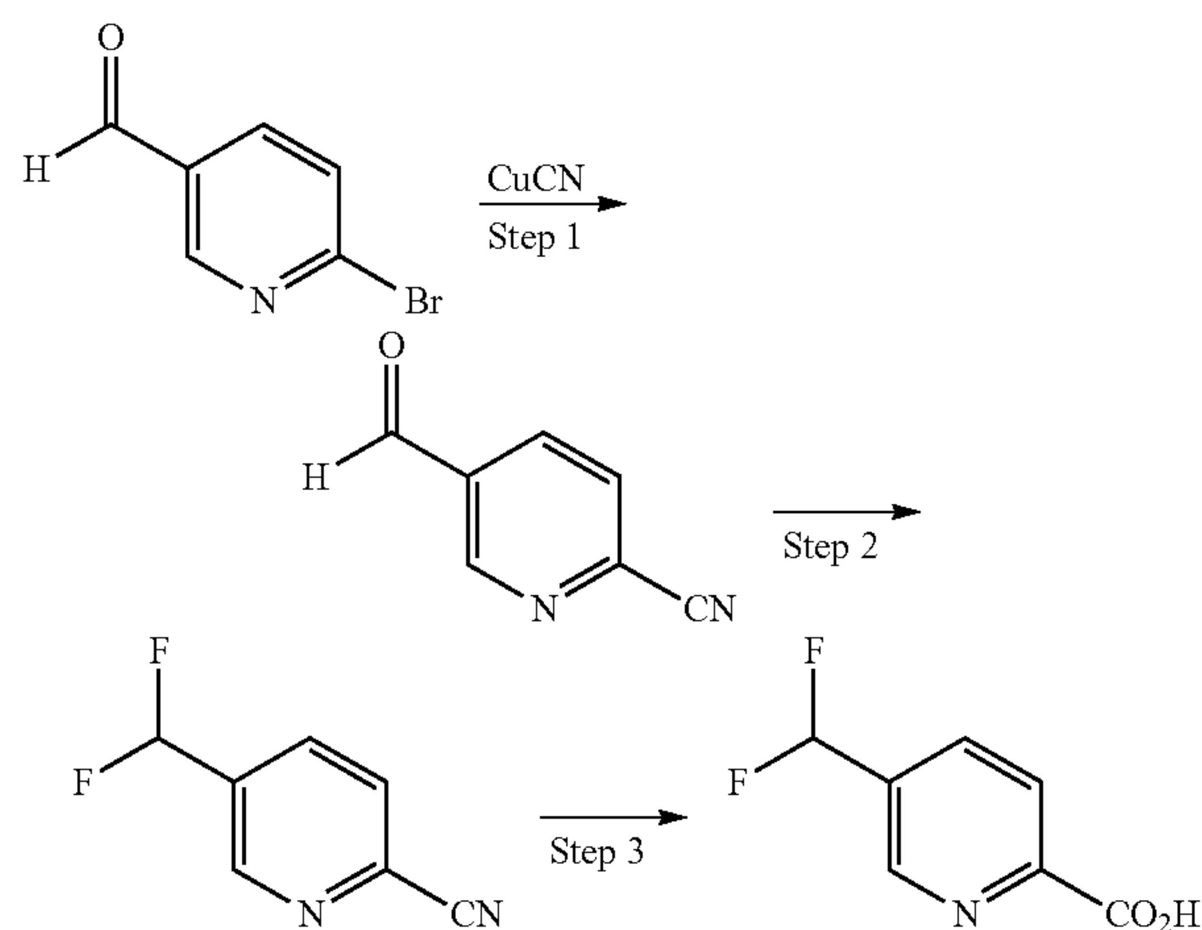
Scheme 11aa:
