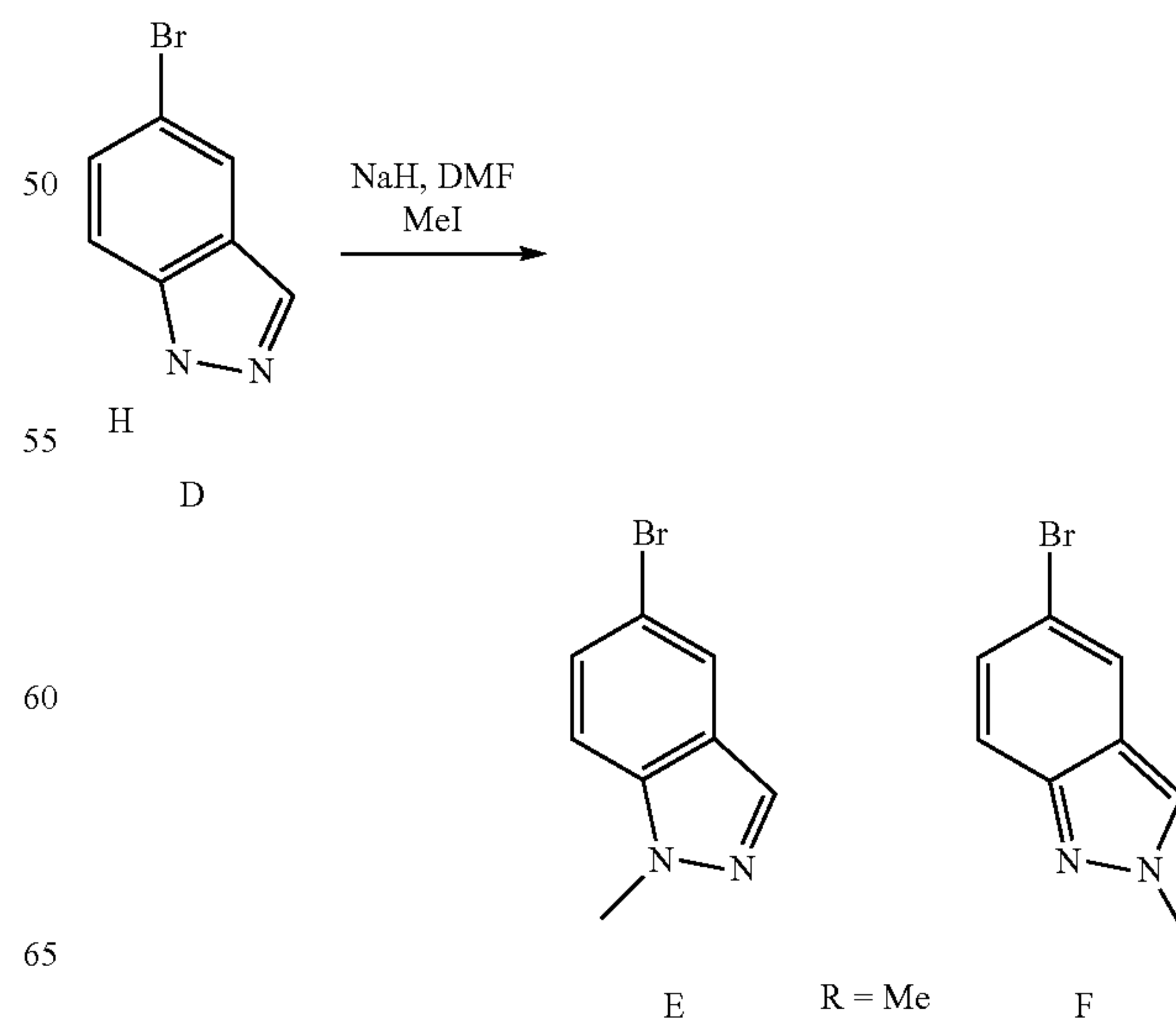
Scheme 6a:
