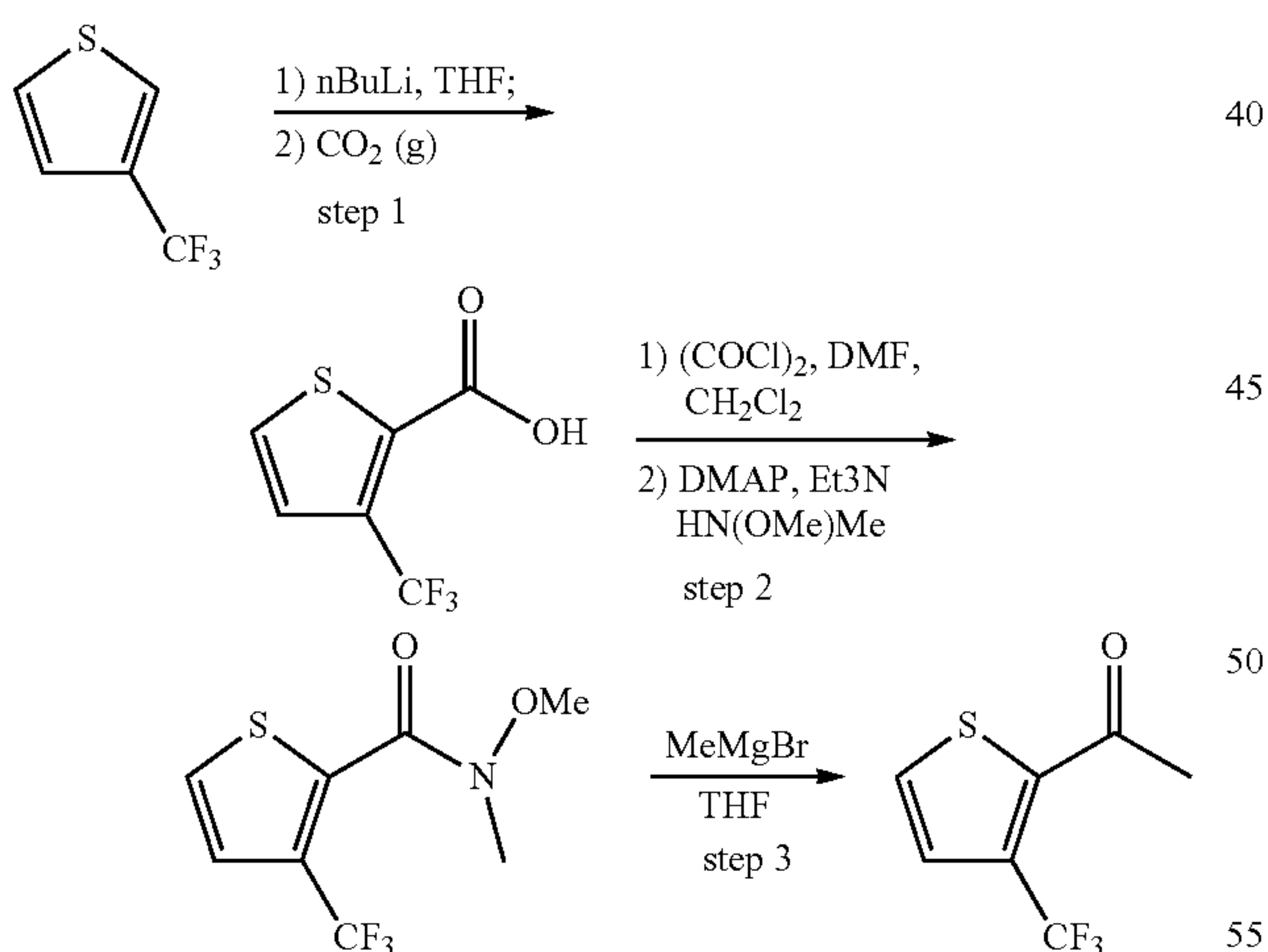
Scheme 2:
