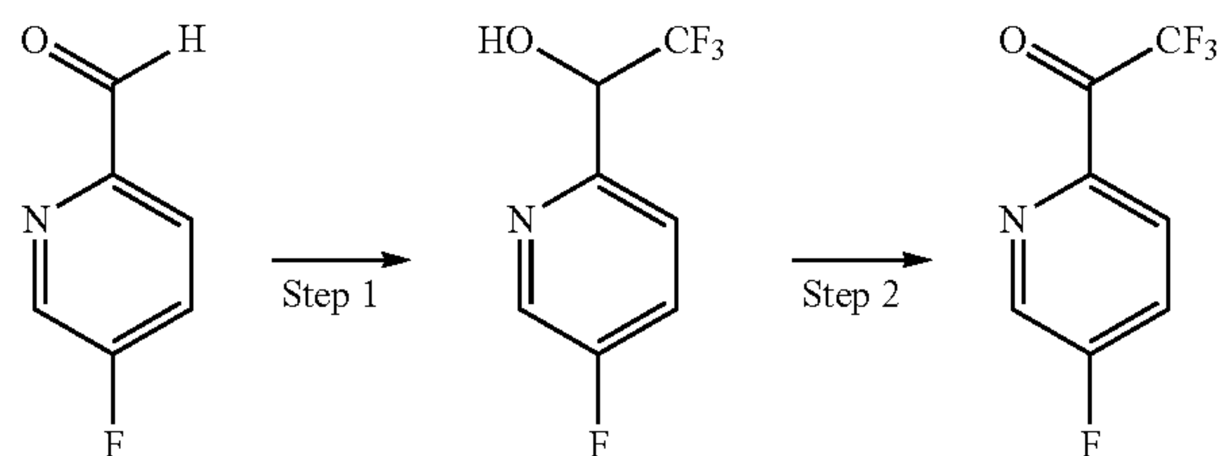
Scheme 11r:
