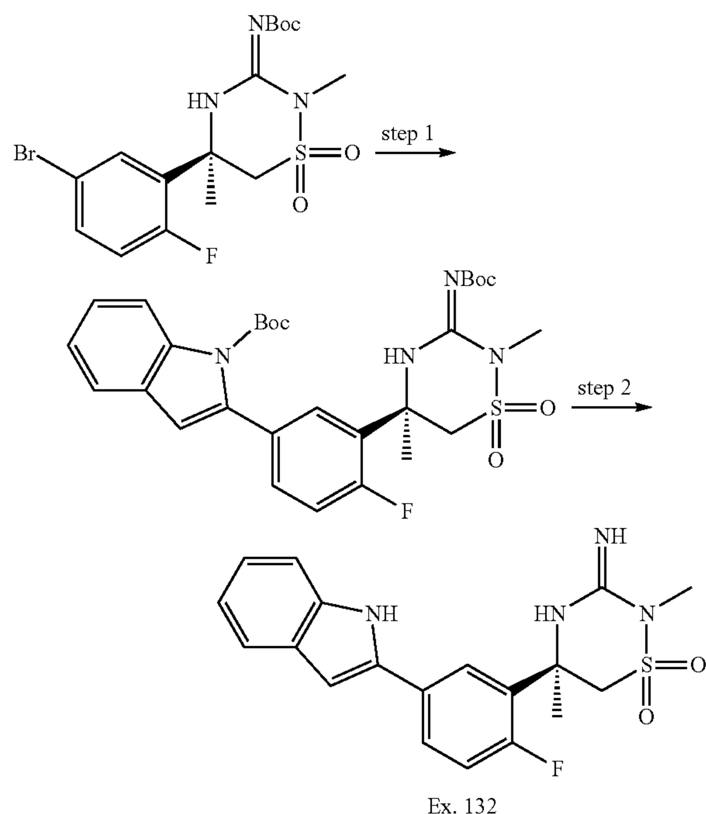
Scheme 30:
