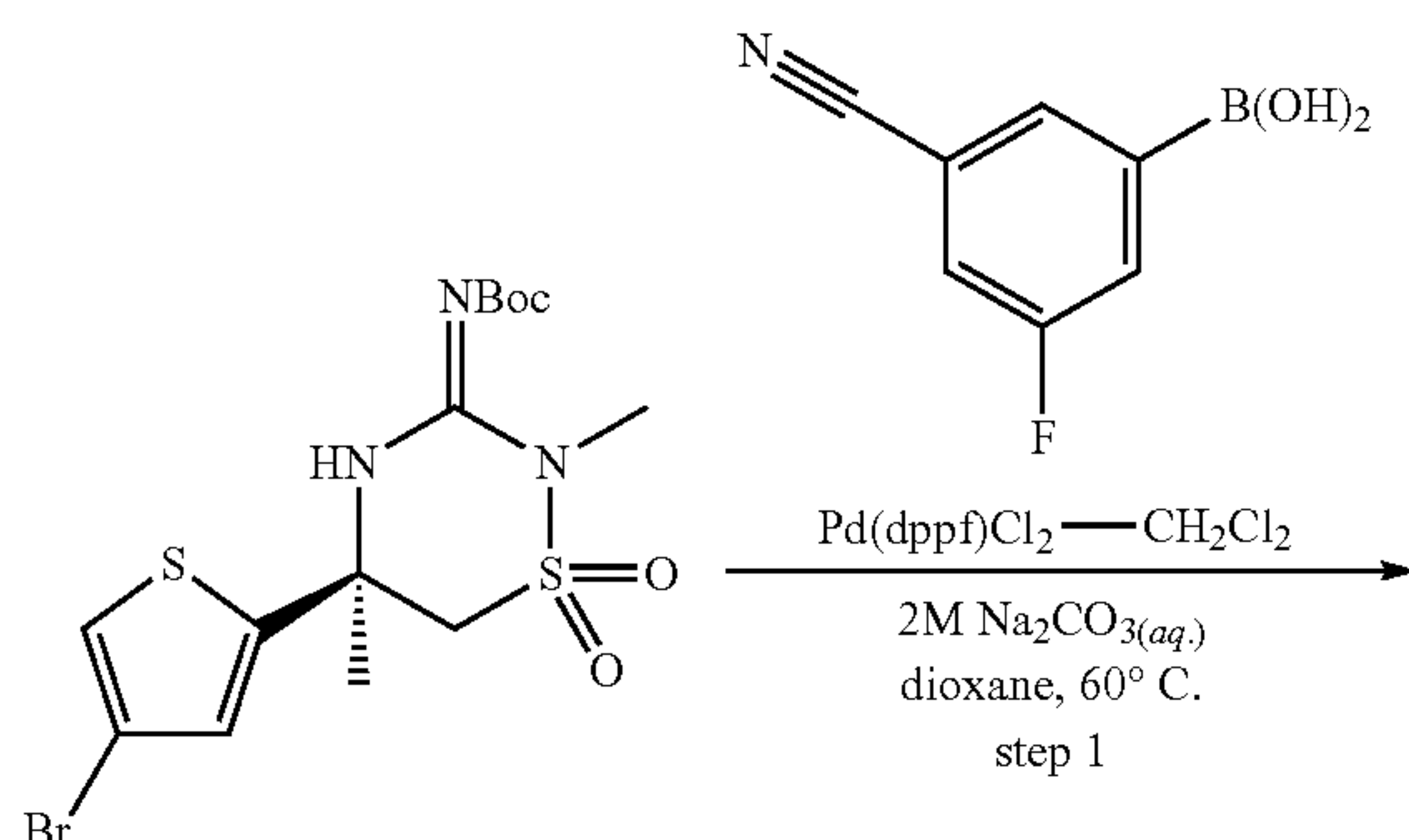
Scheme 15:
