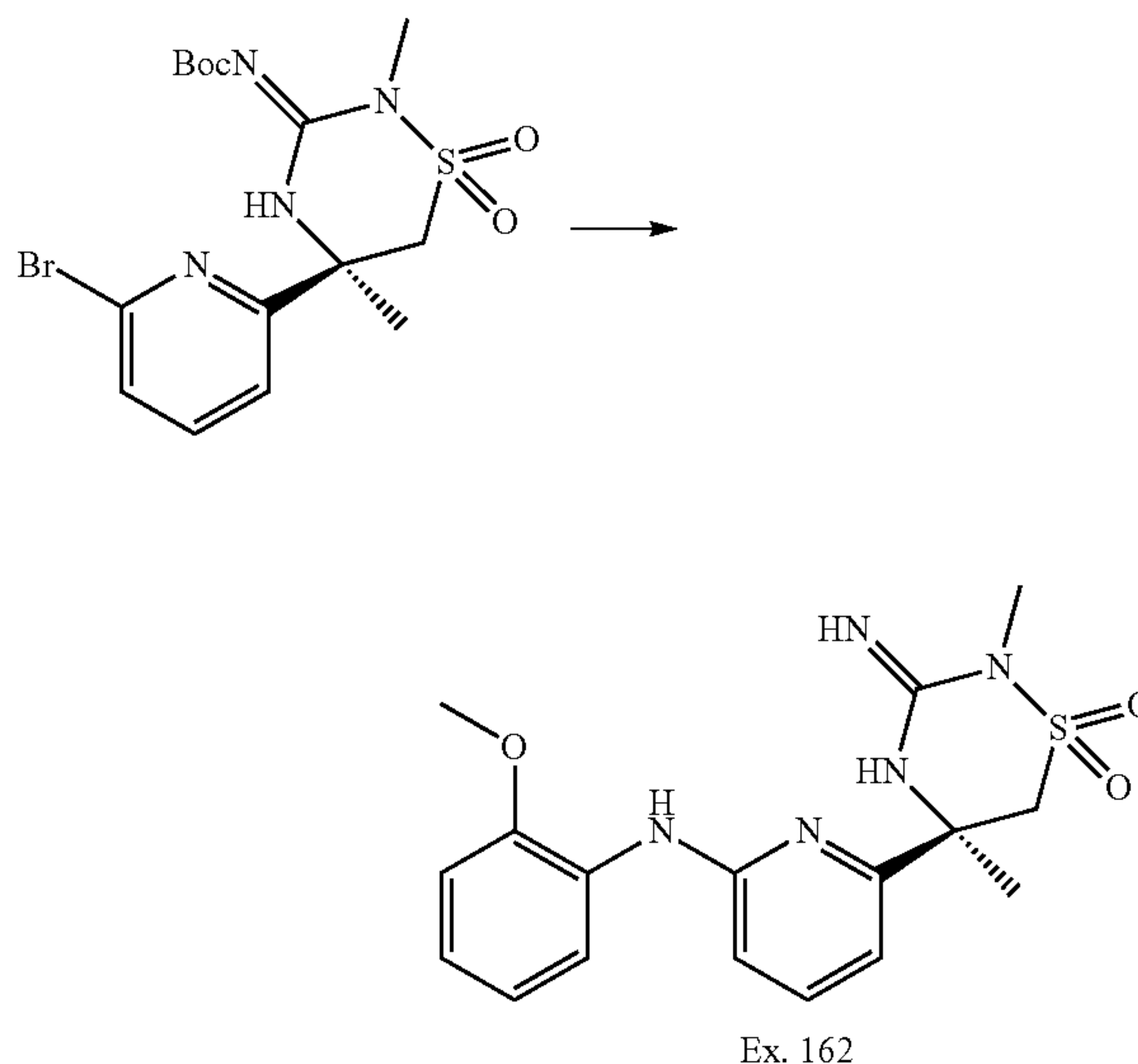
Scheme 40:
