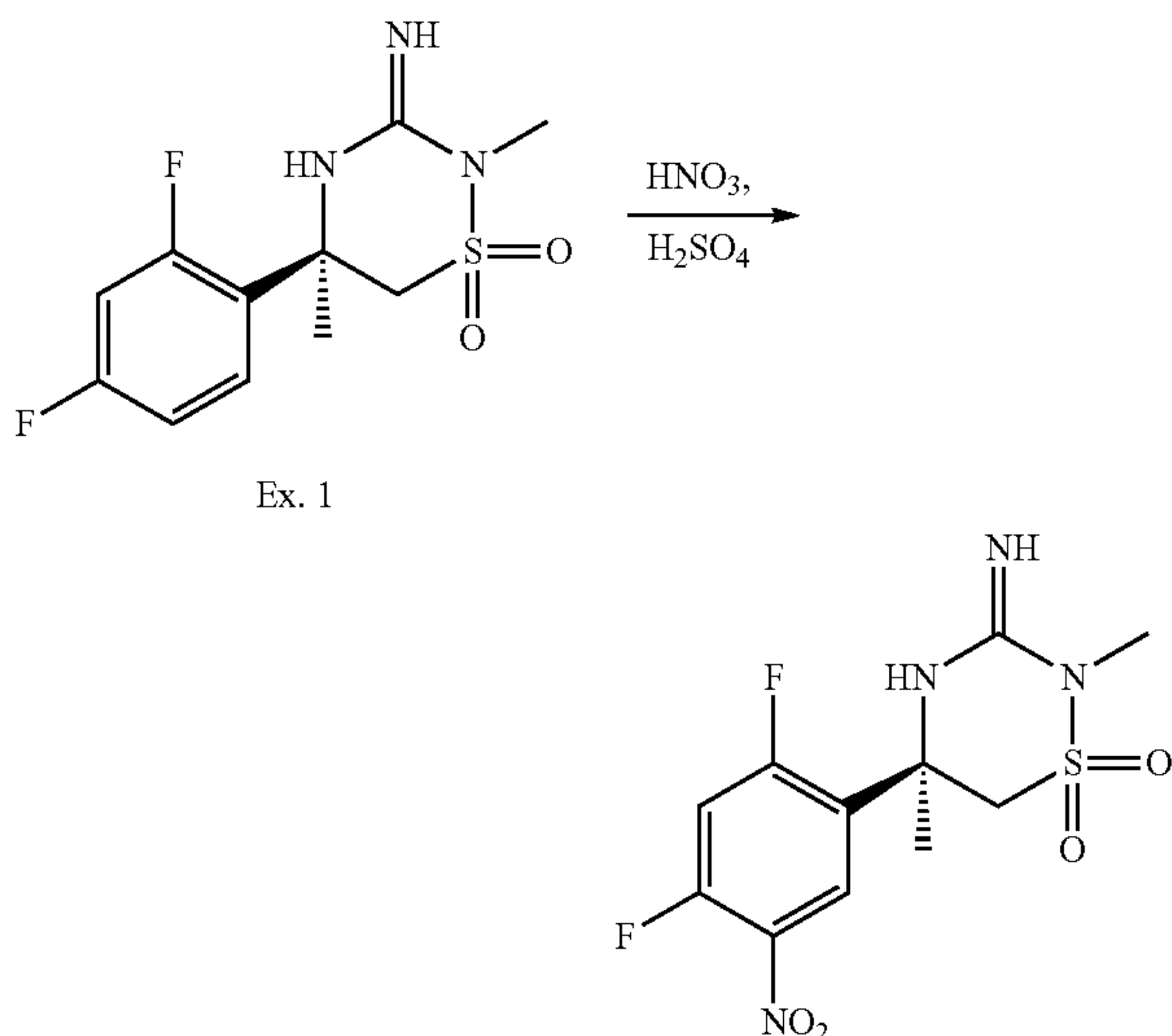
Scheme 1b:
