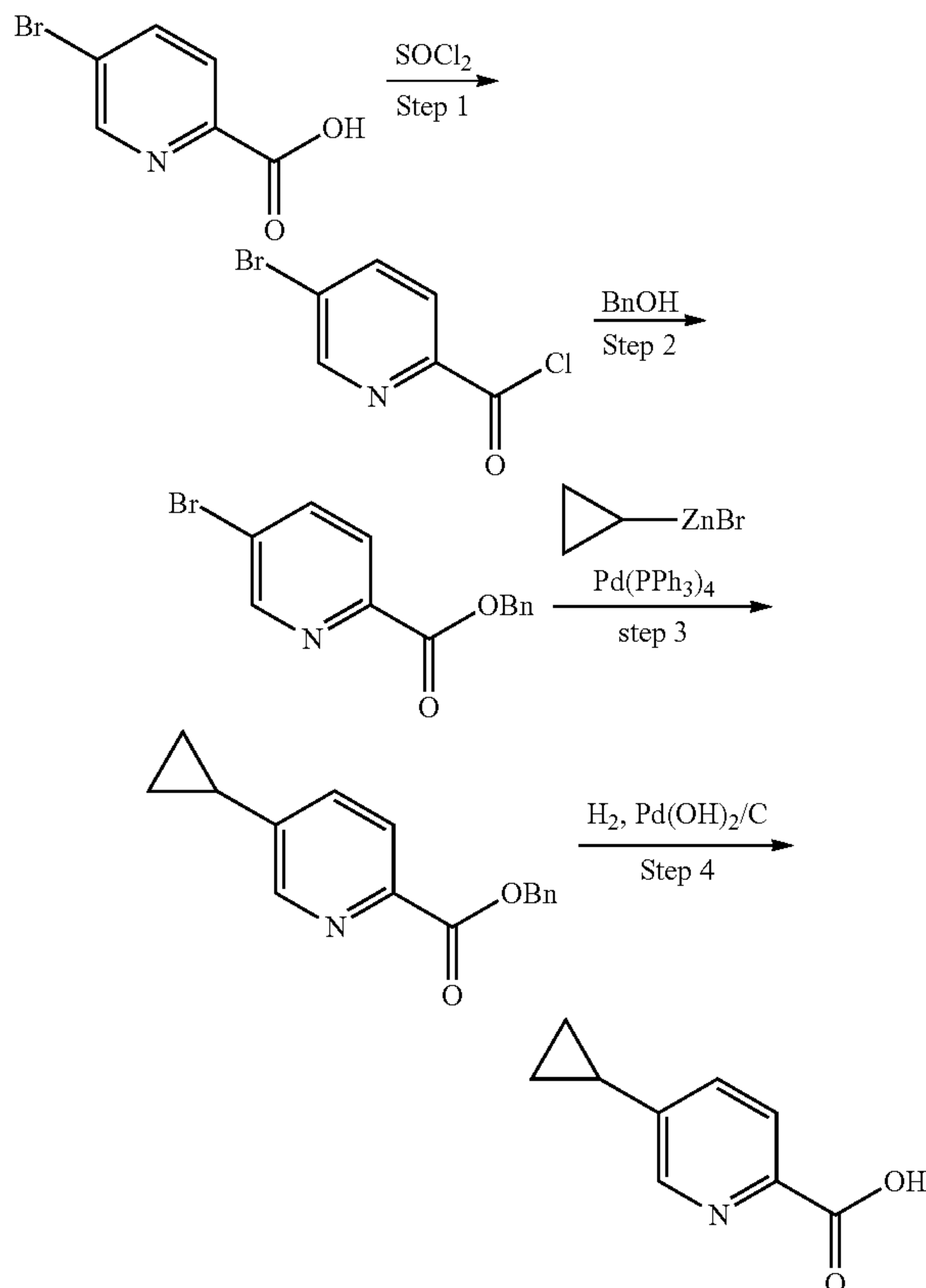
Scheme 11u:
