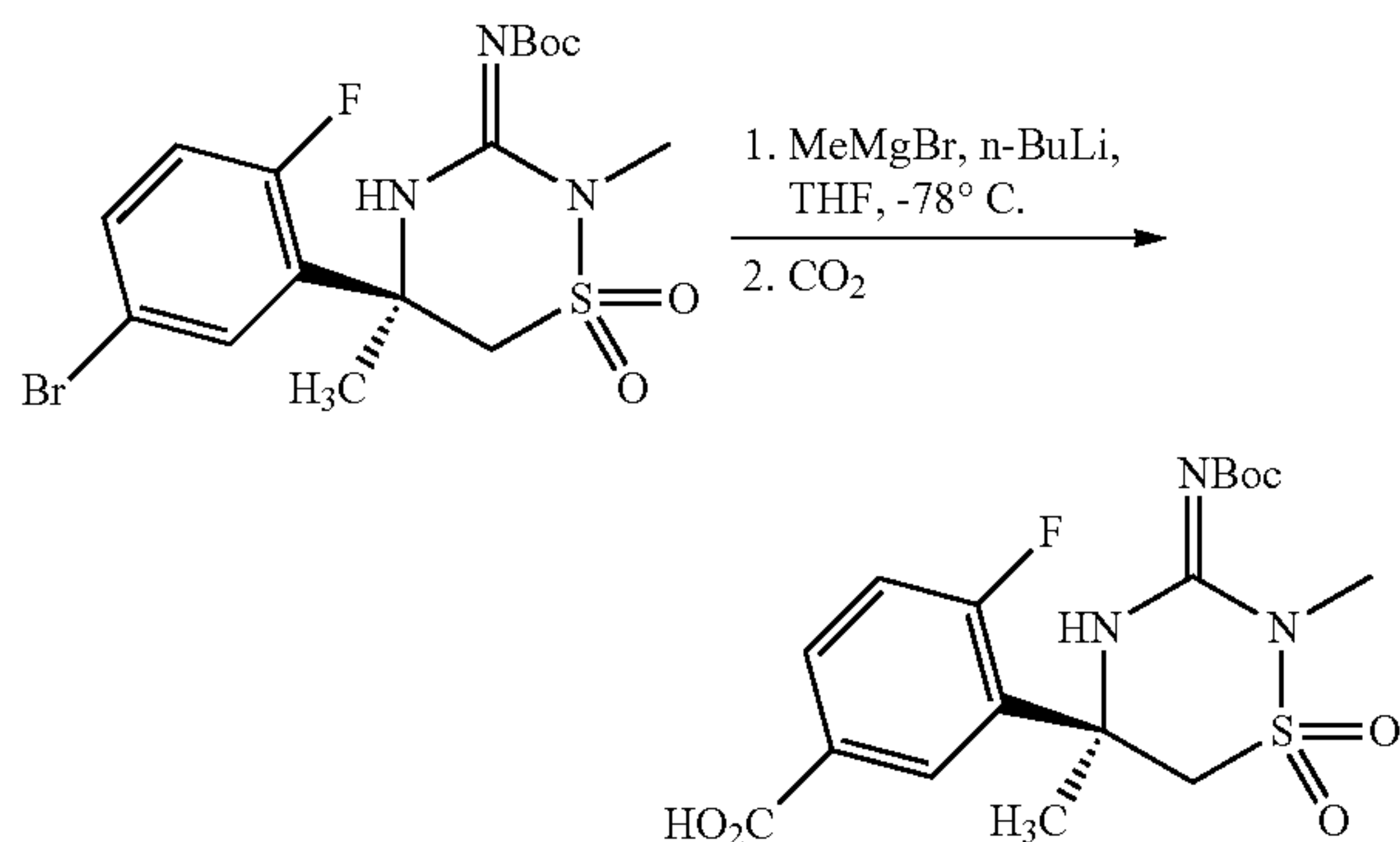
Scheme 22:
