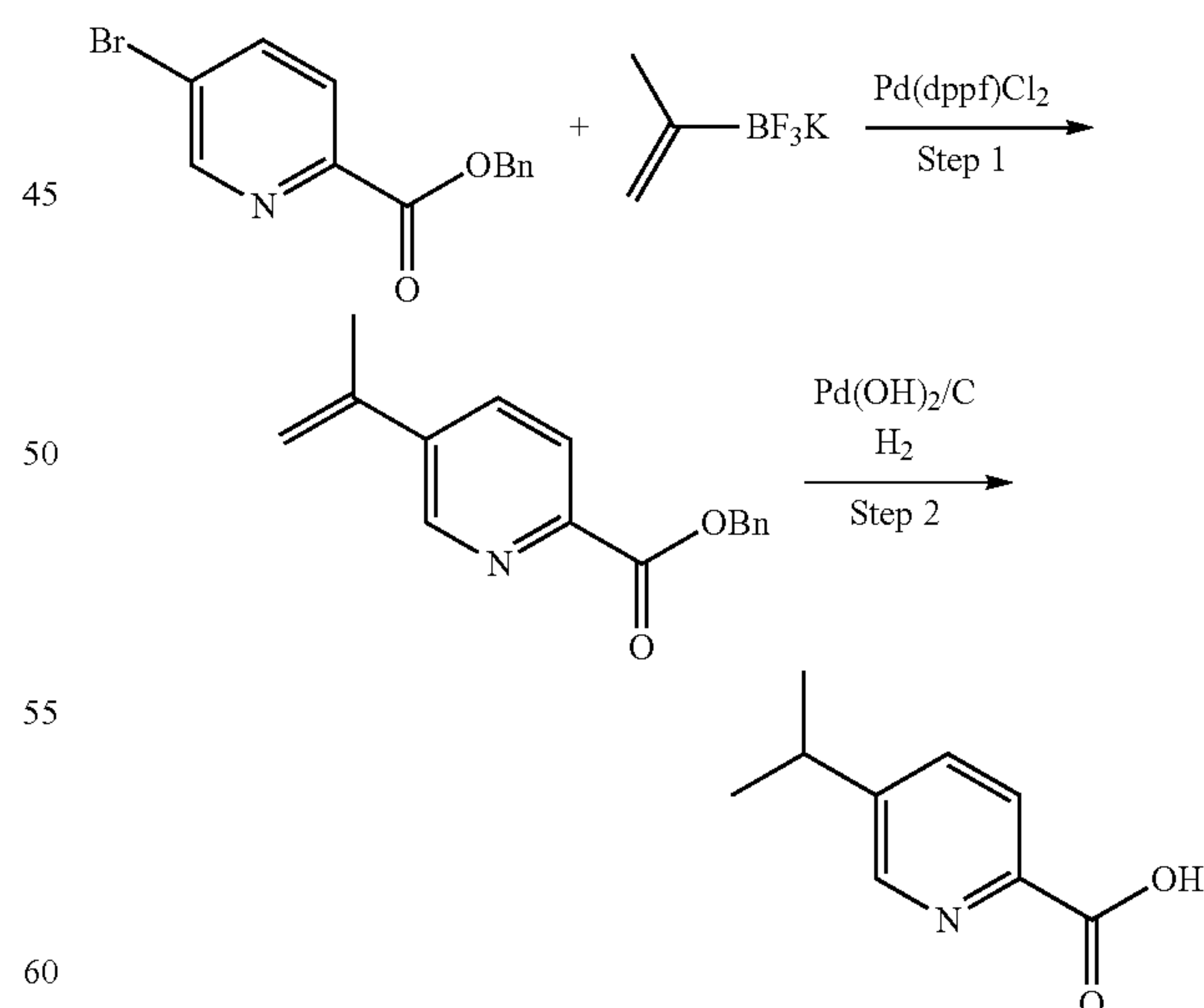
Scheme 11v:
