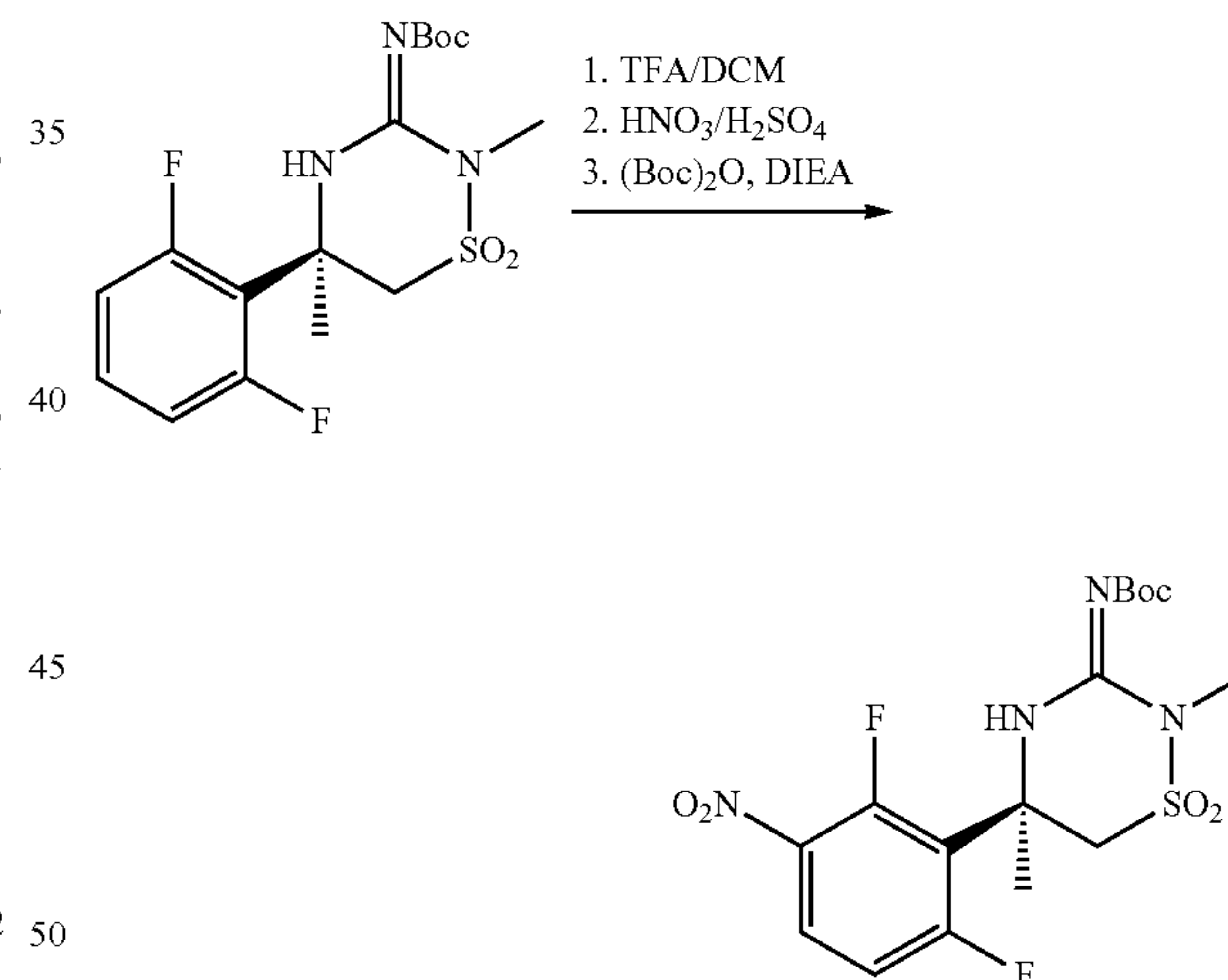
Scheme 7c:
