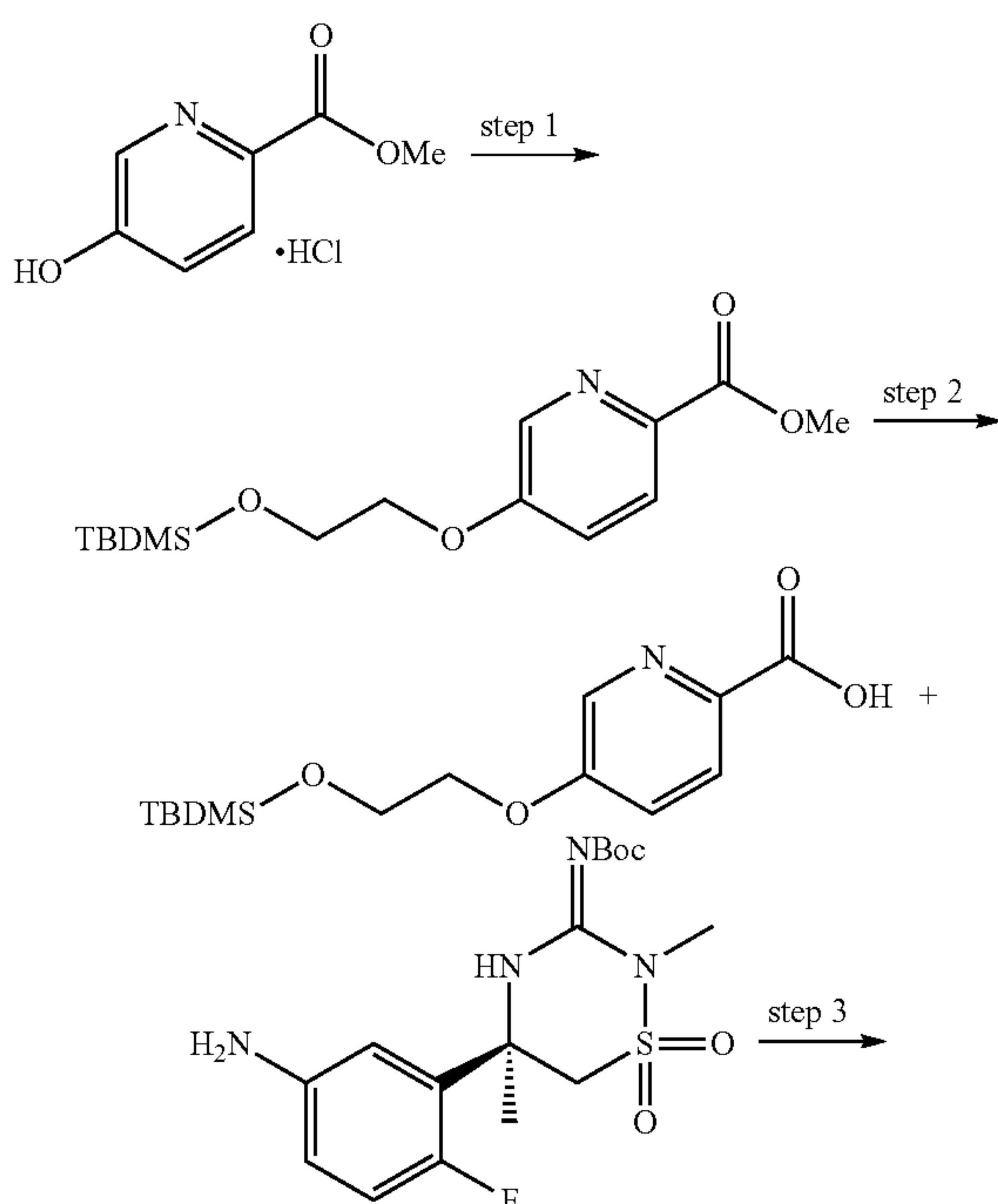
Scheme 24:
