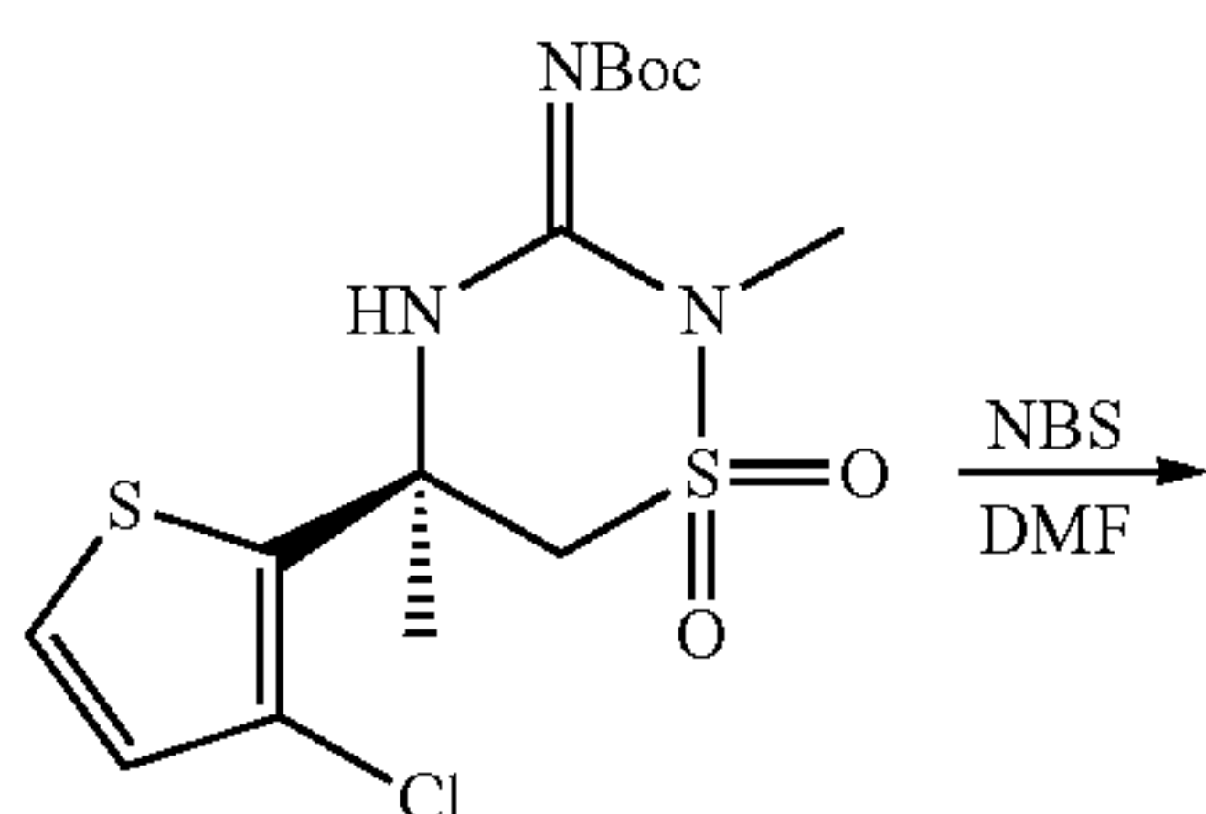
Scheme 13:
