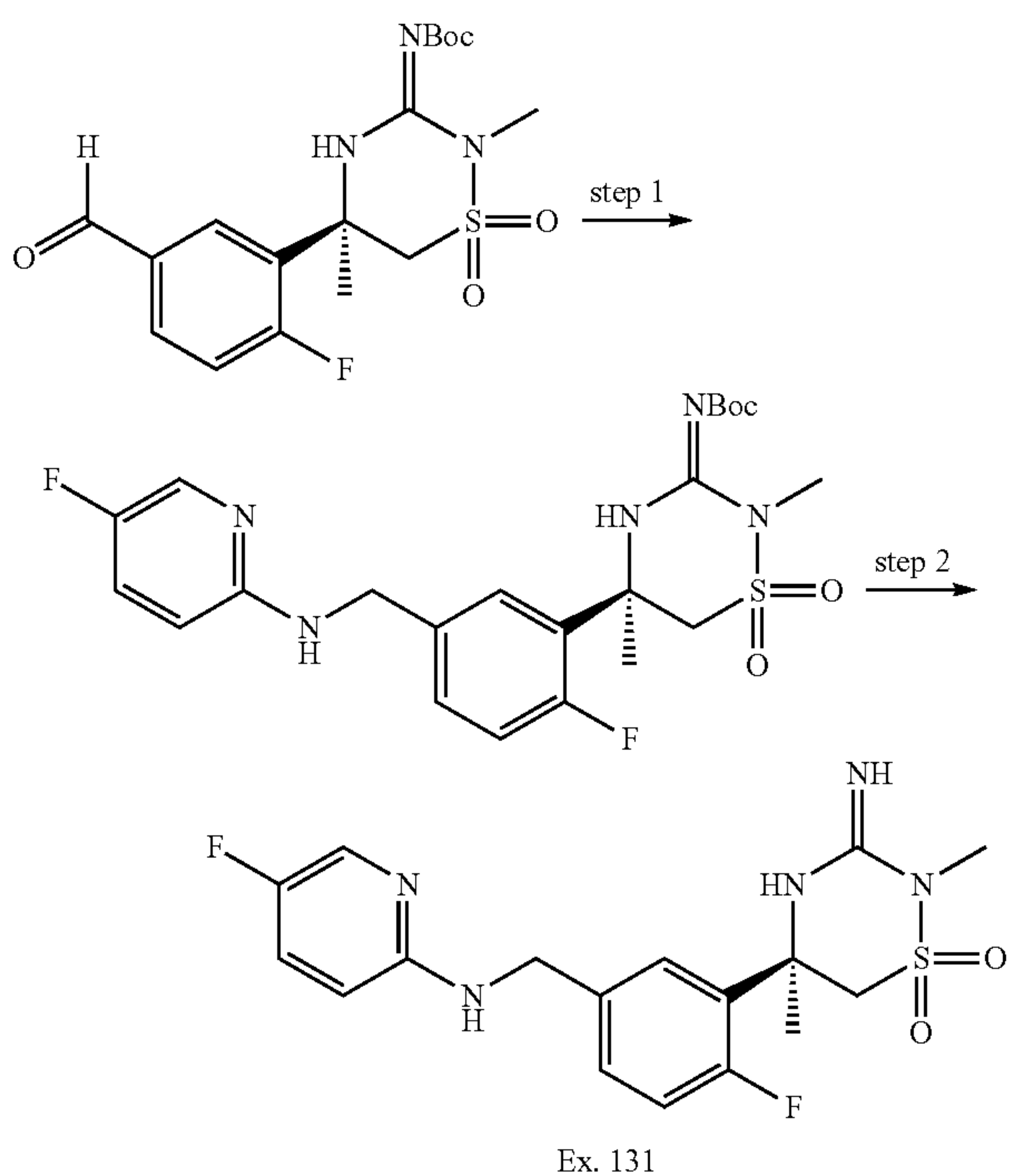
Scheme 28
