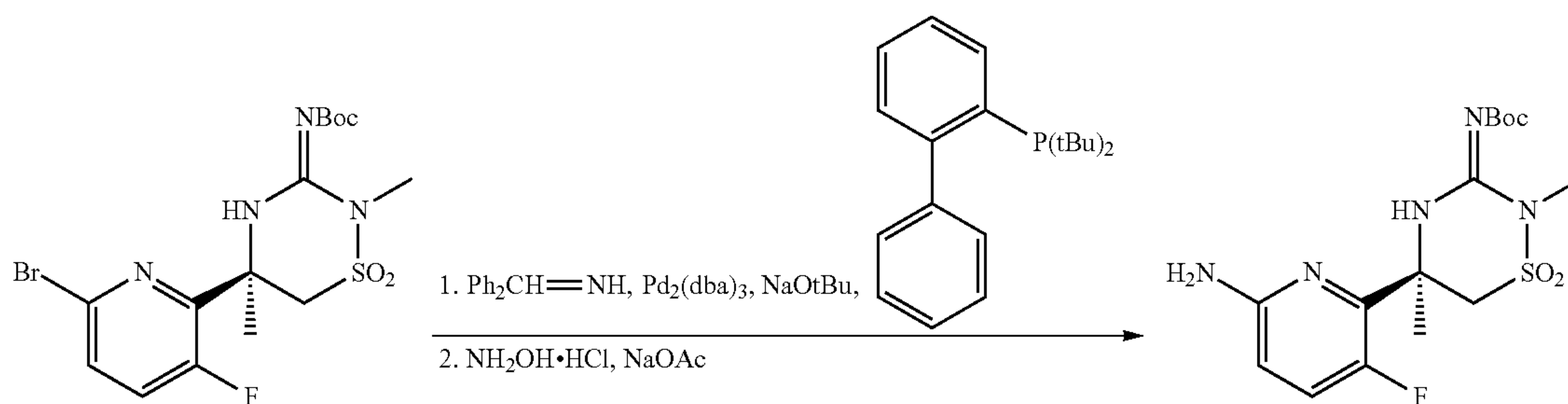
Scheme 7b:
