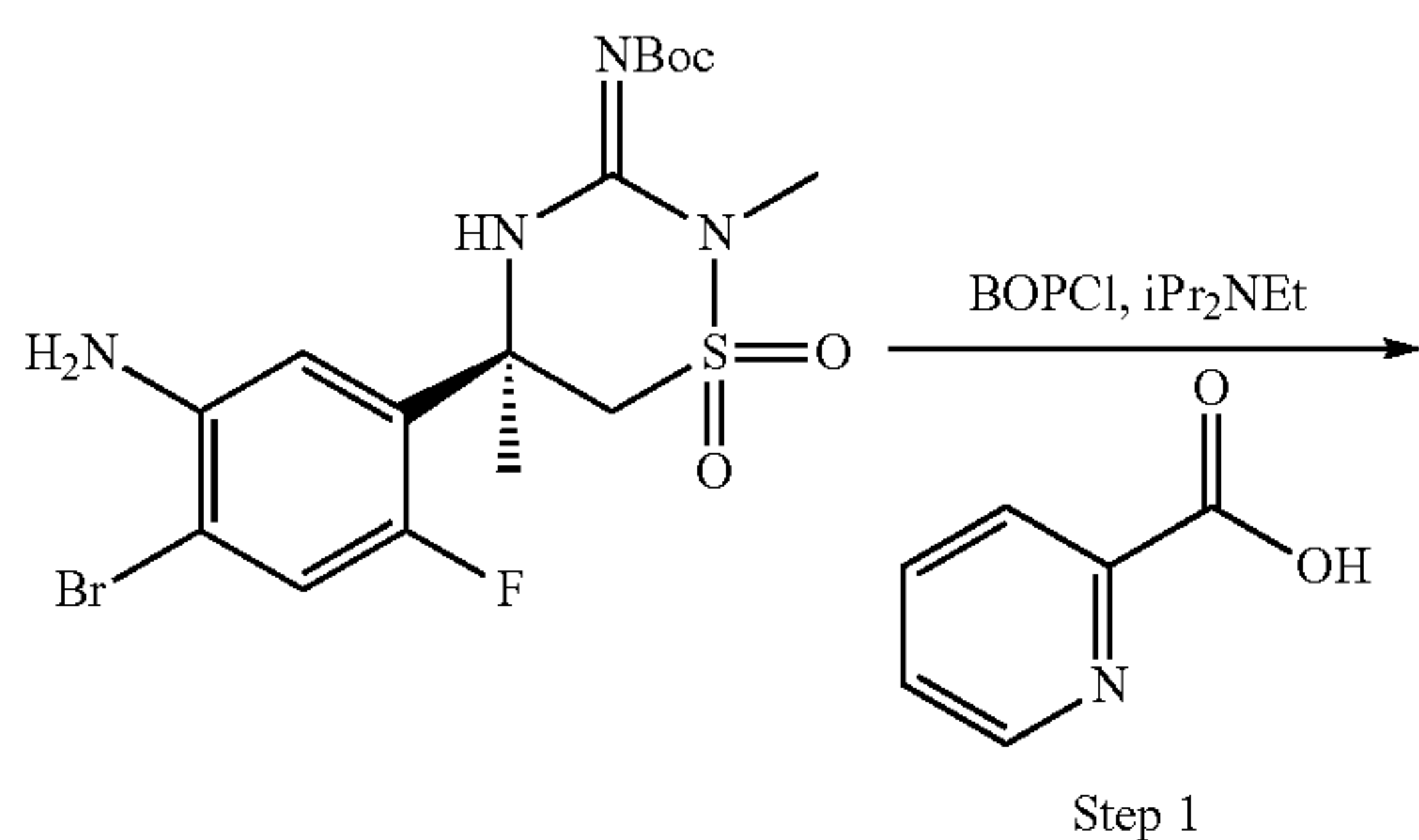
Scheme 34:
