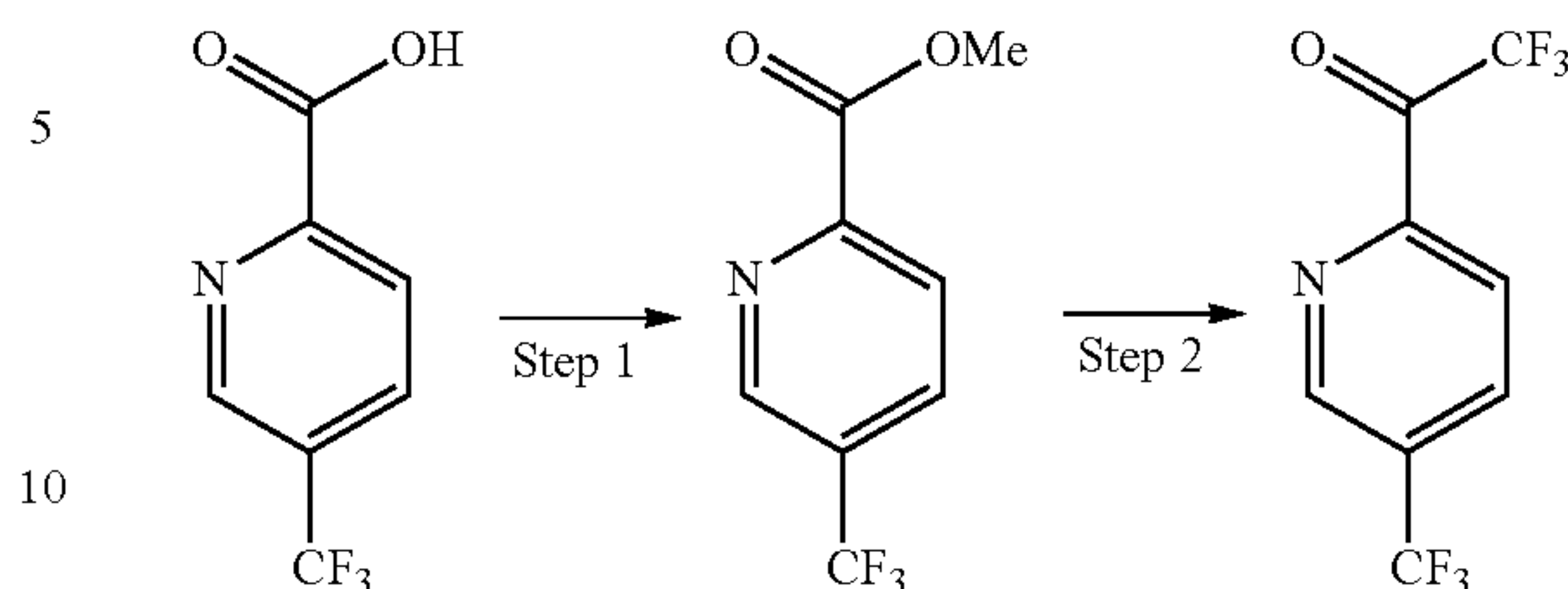
Scheme 11s:
