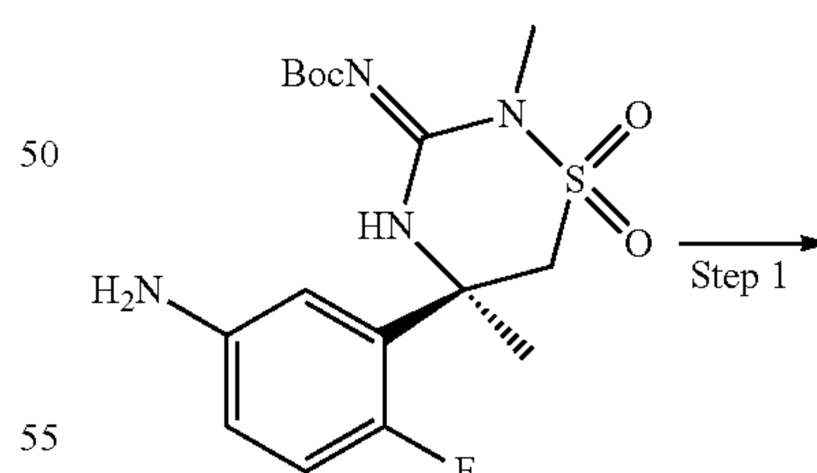
Scheme 35:
