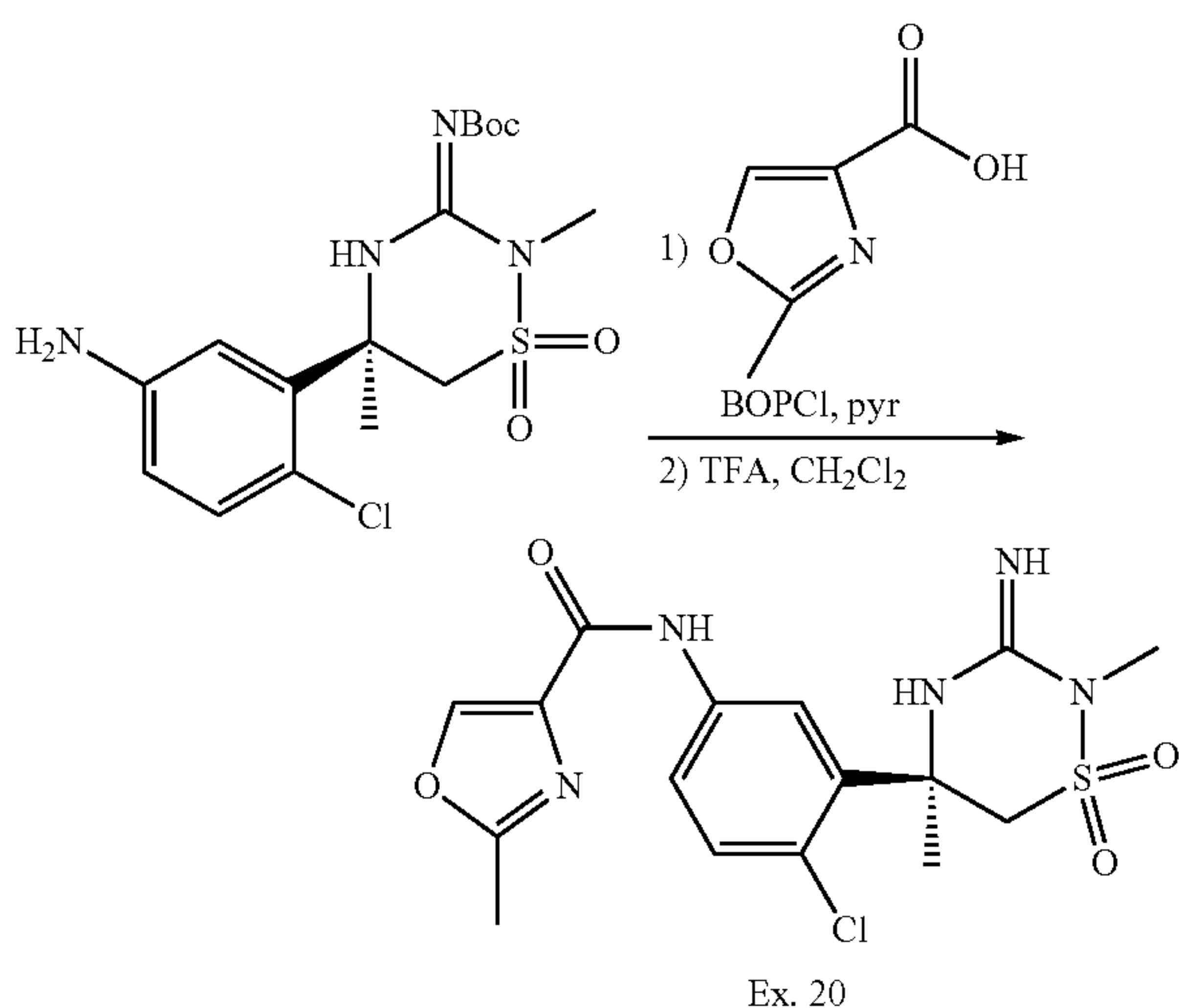
Scheme 11b:
