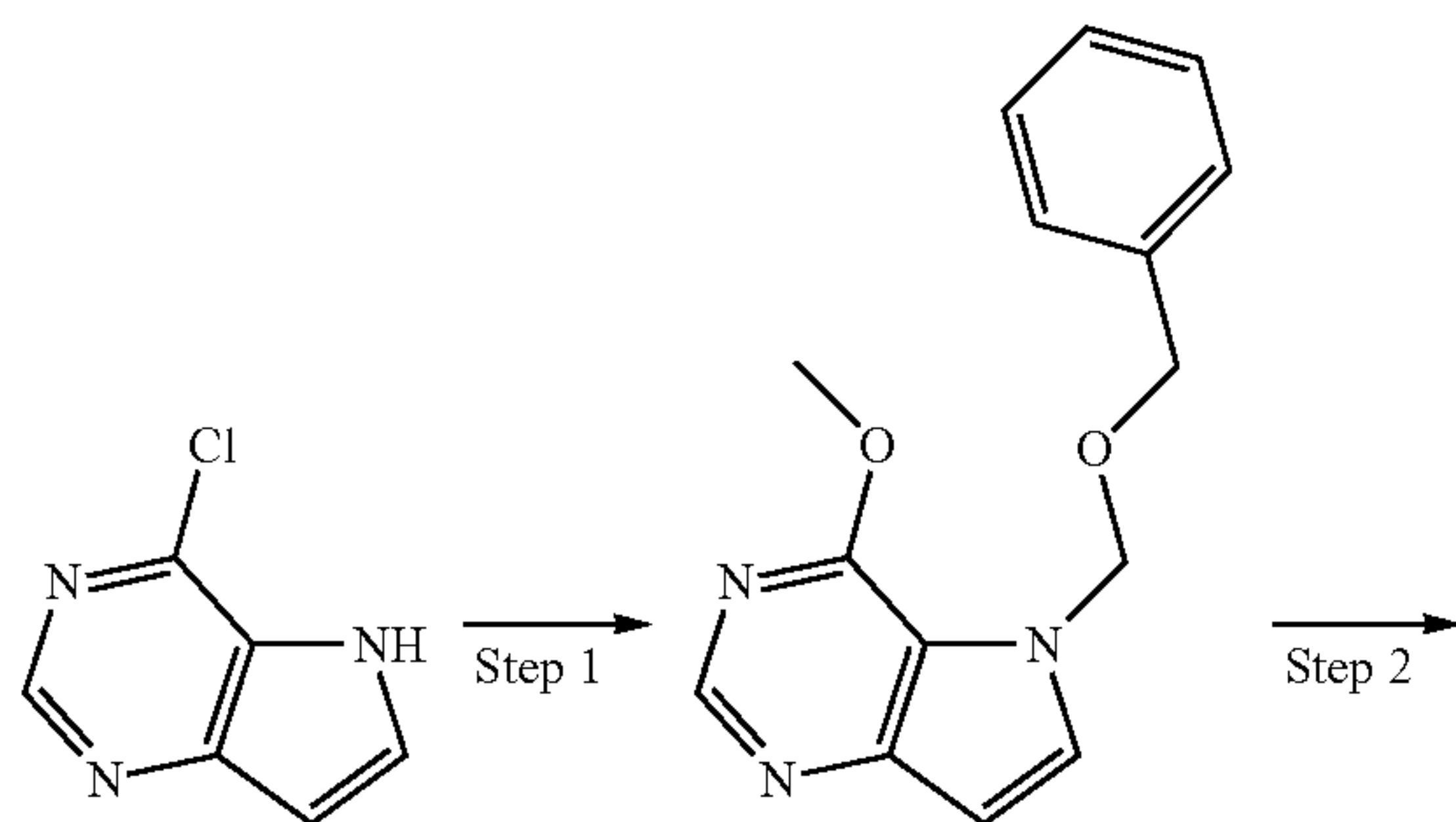
Scheme 52:
