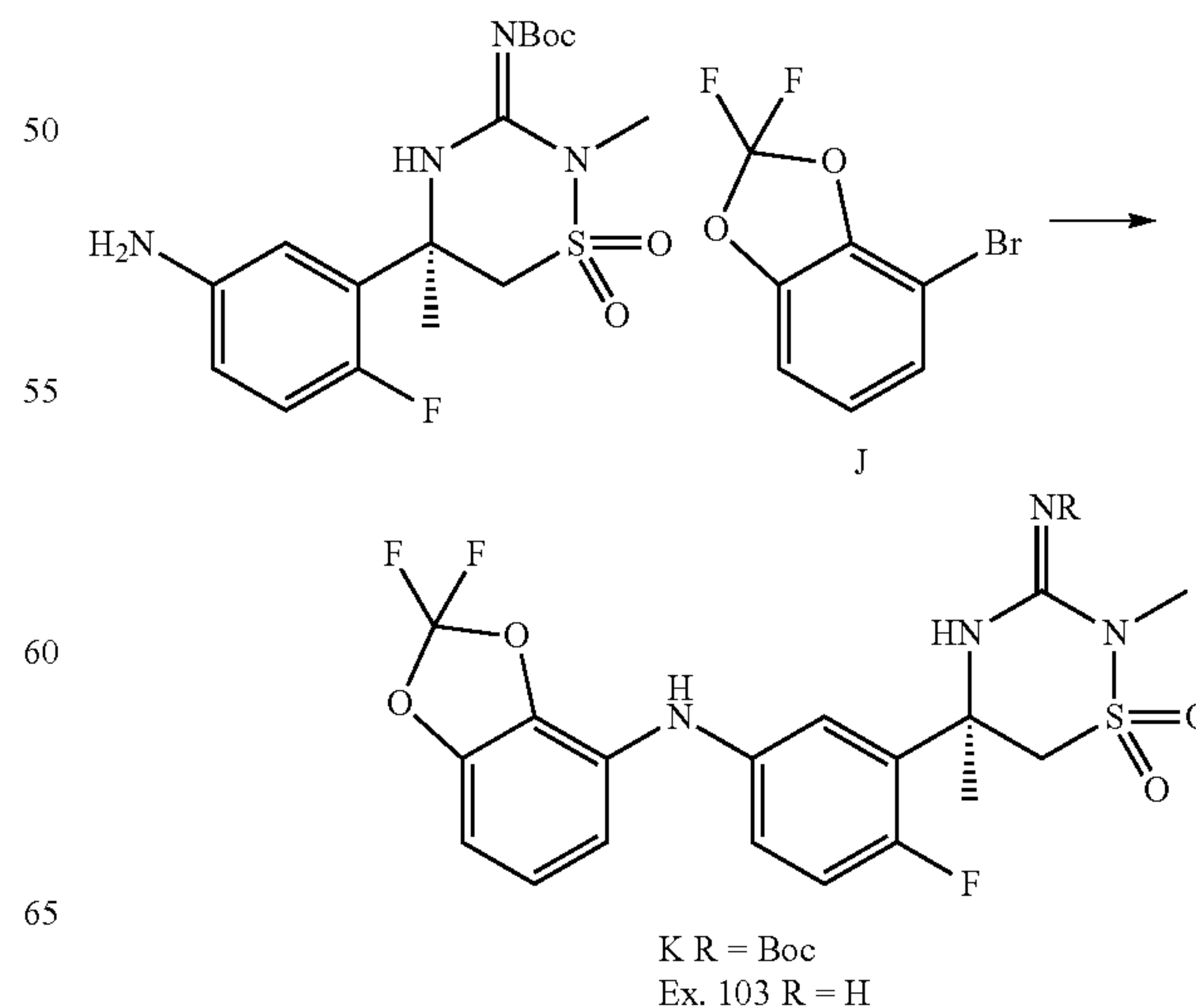
Scheme 18:
