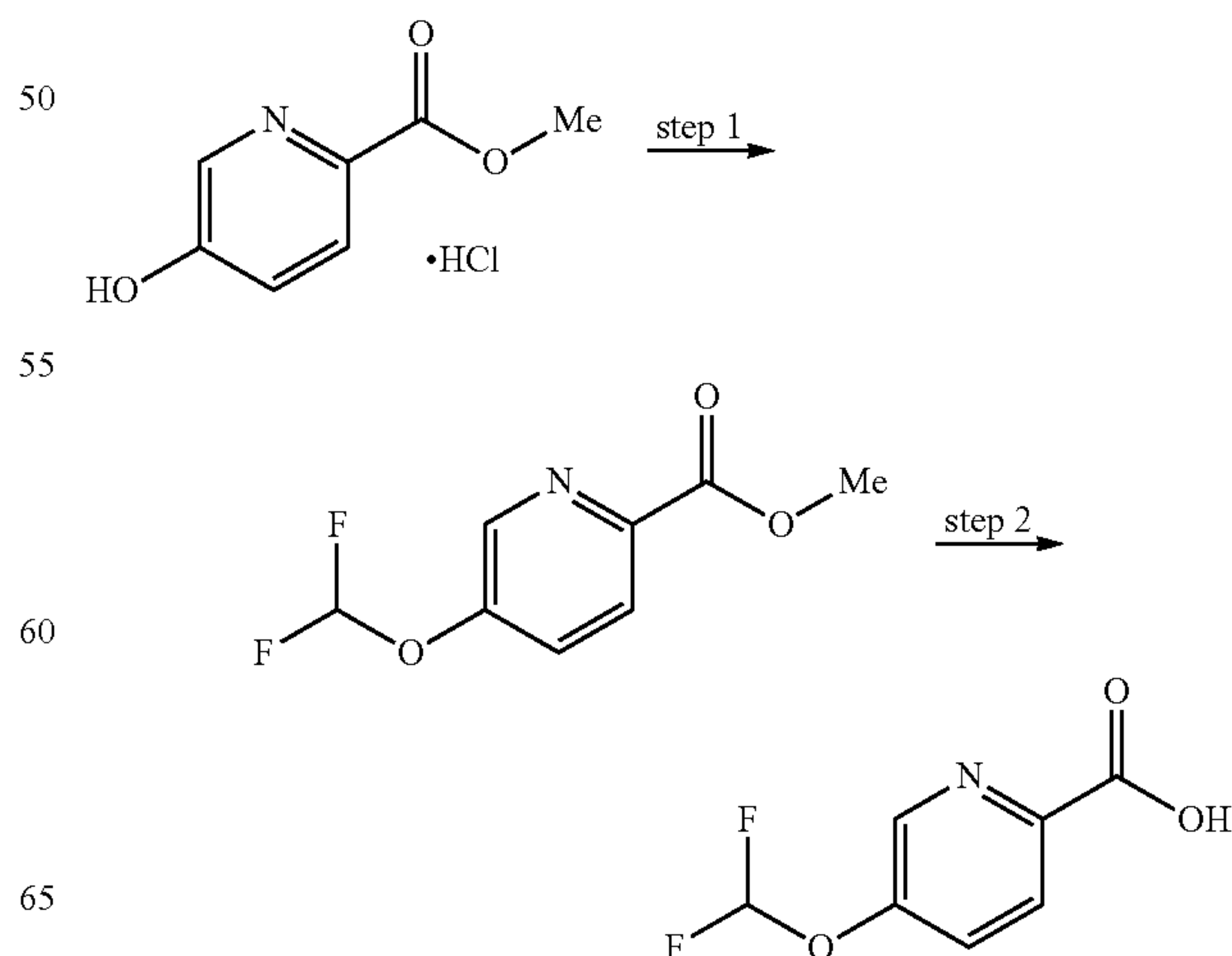
Scheme 11i:
