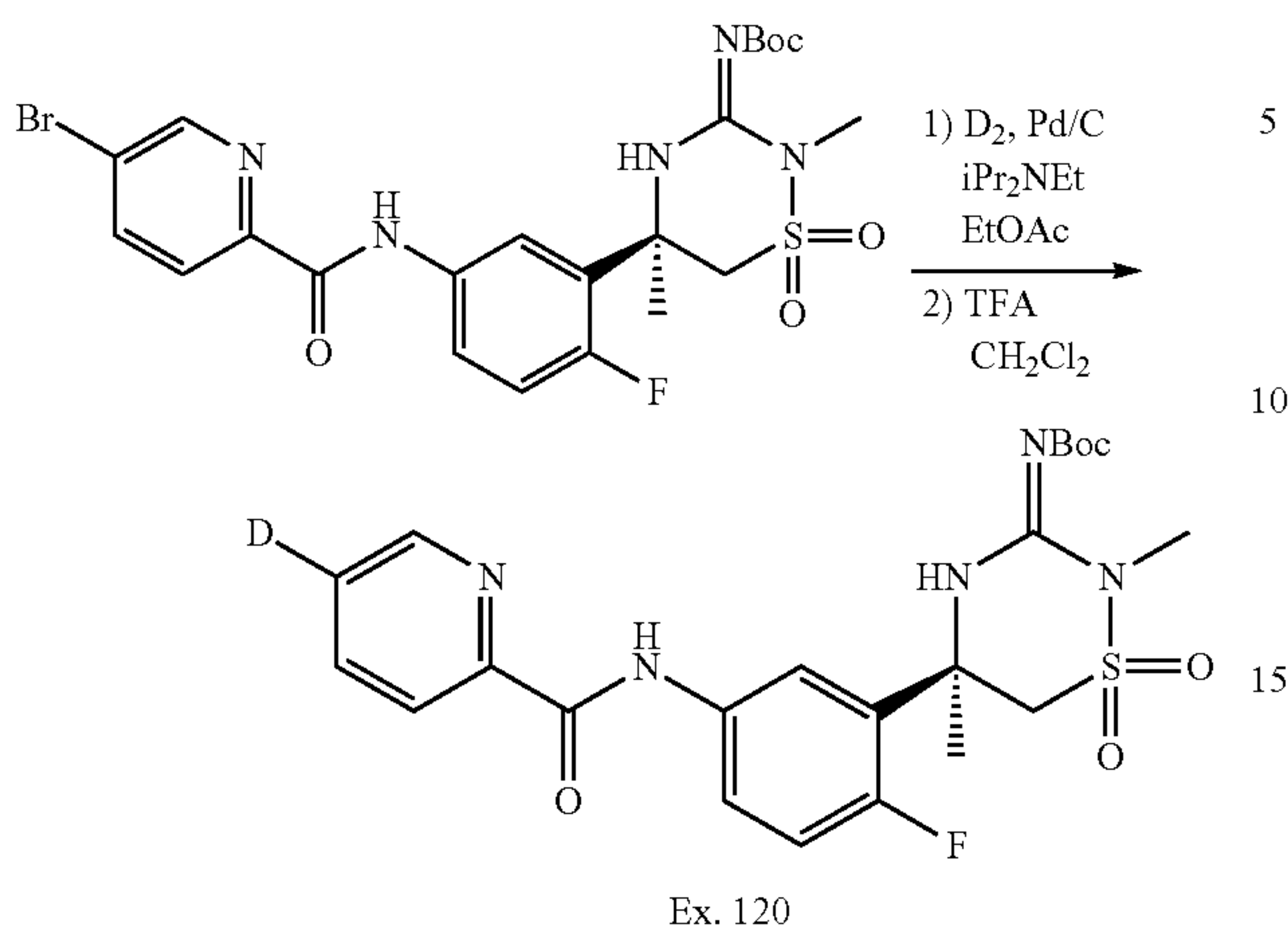
Scheme 23:
