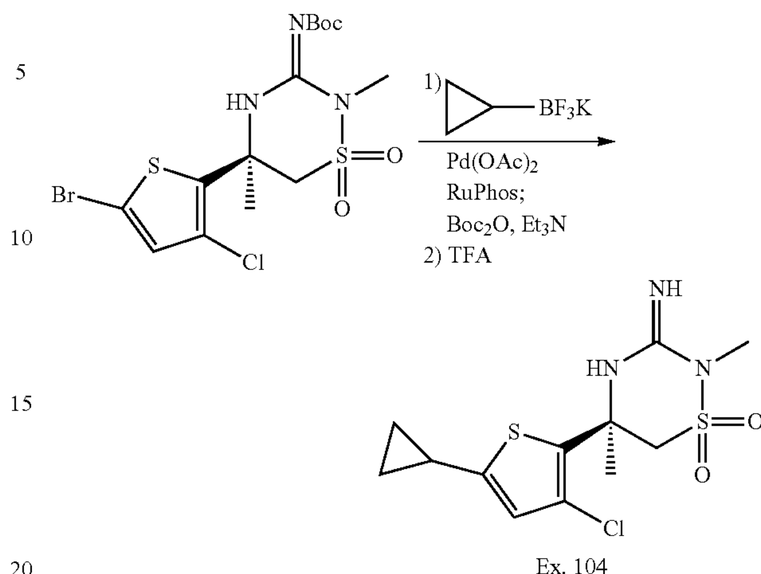
Scheme 19:
