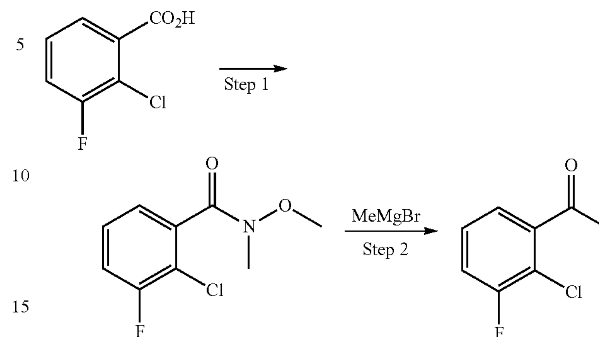
Scheme 2c:
