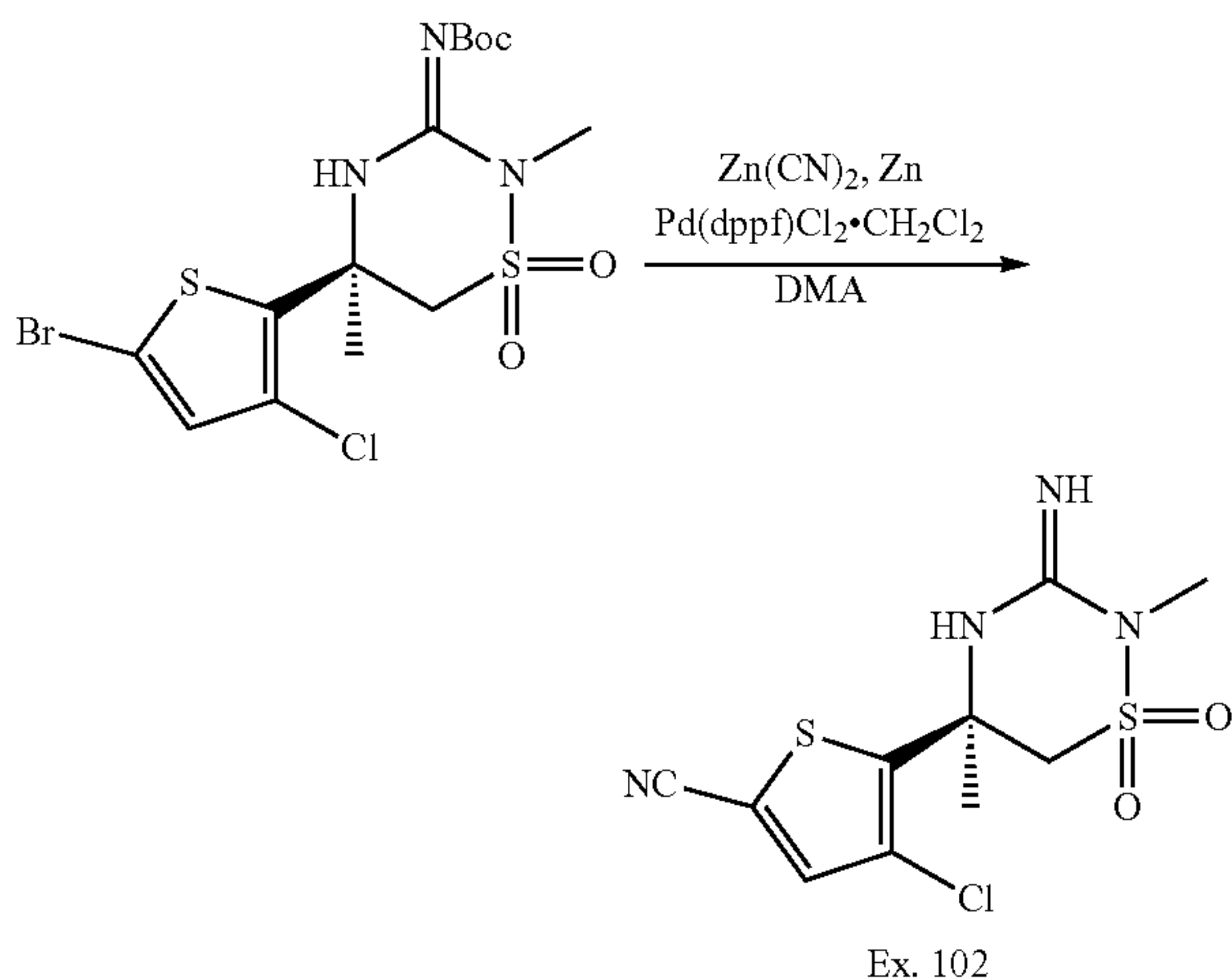
Scheme 17:
