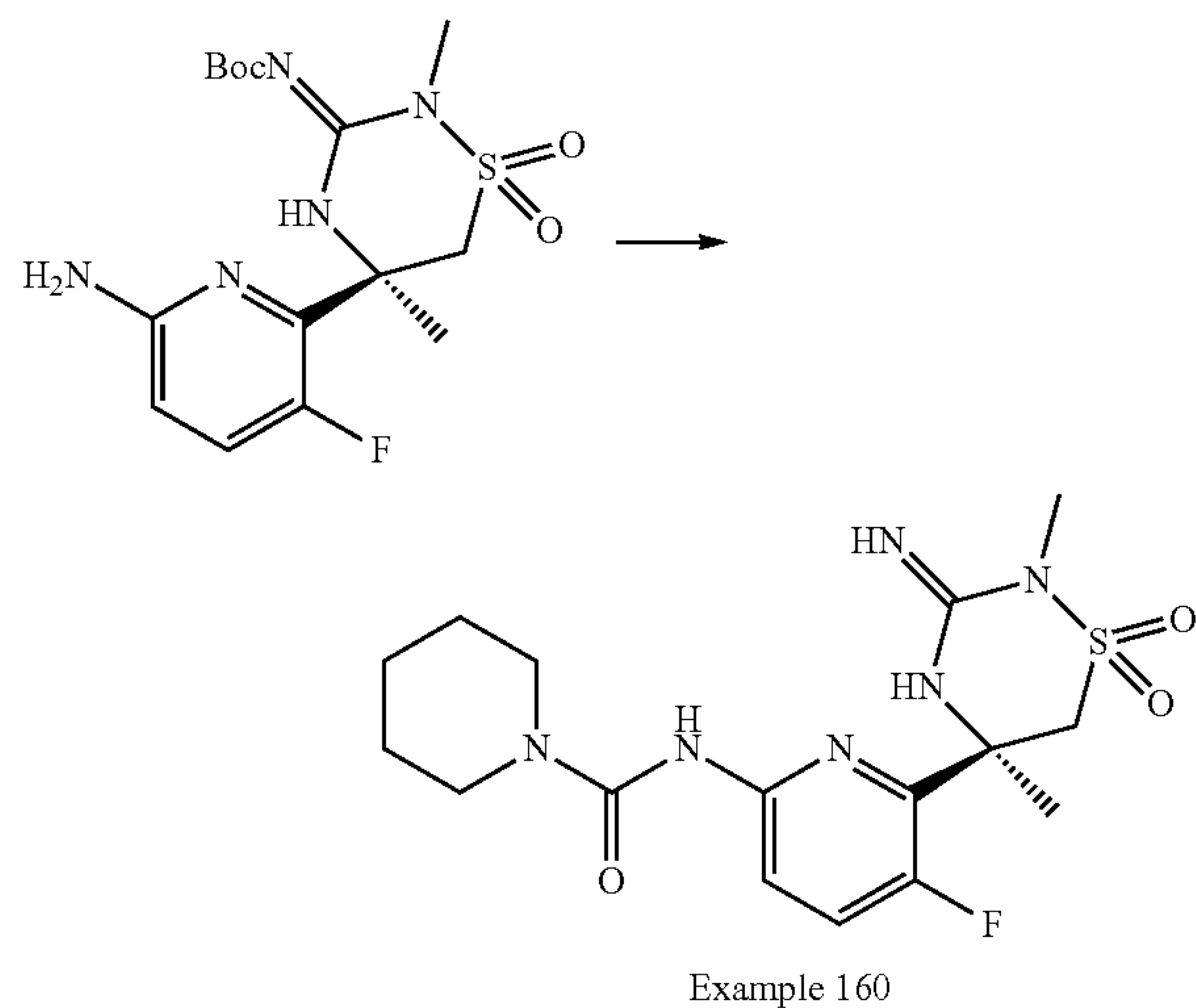
Scheme 39:
