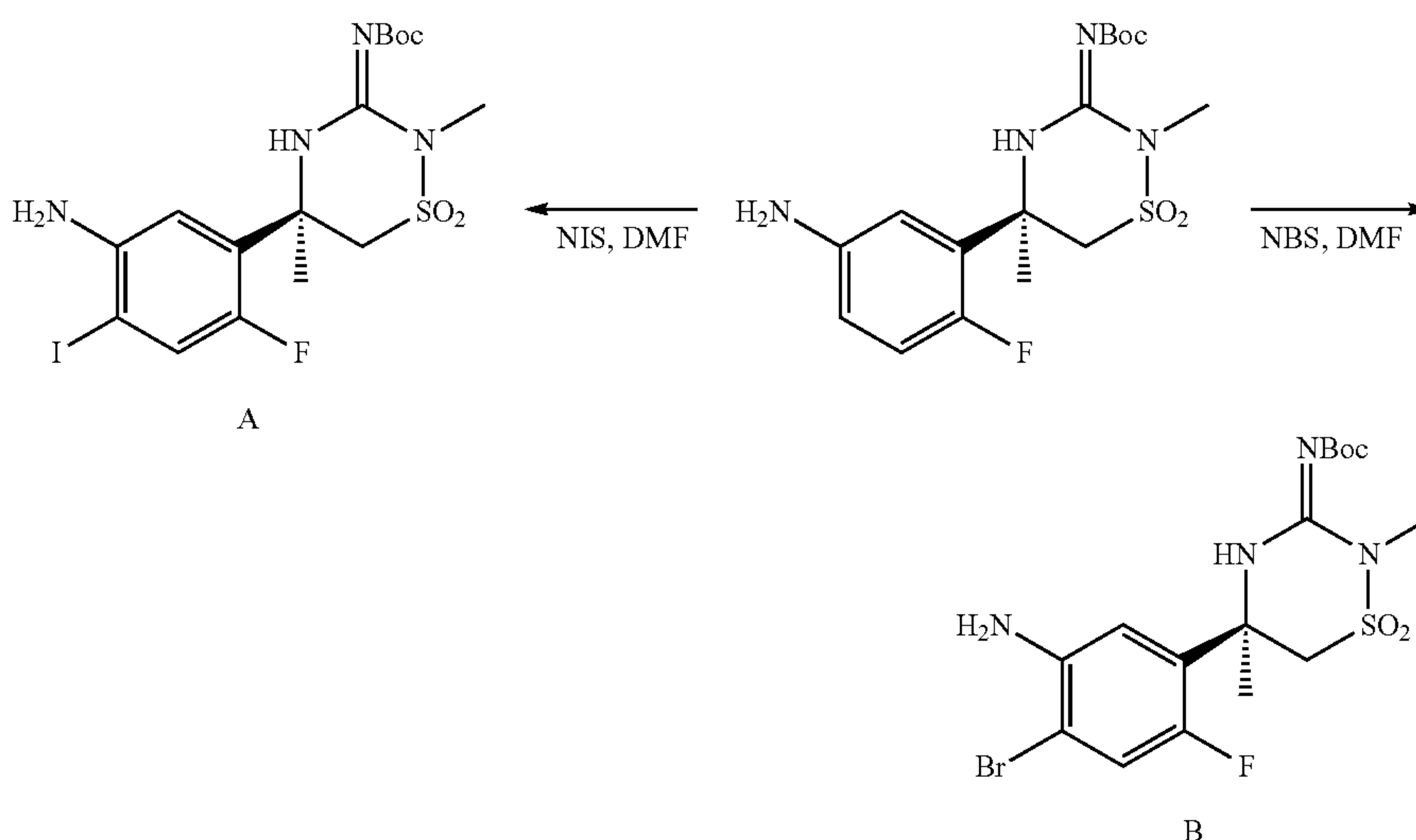
Scheme 10a:
