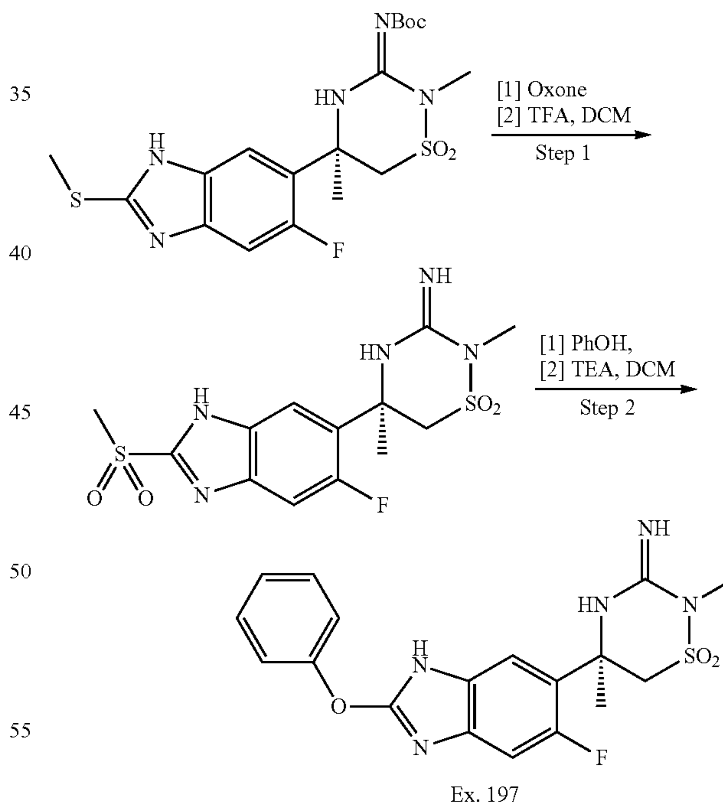
Scheme 51:
