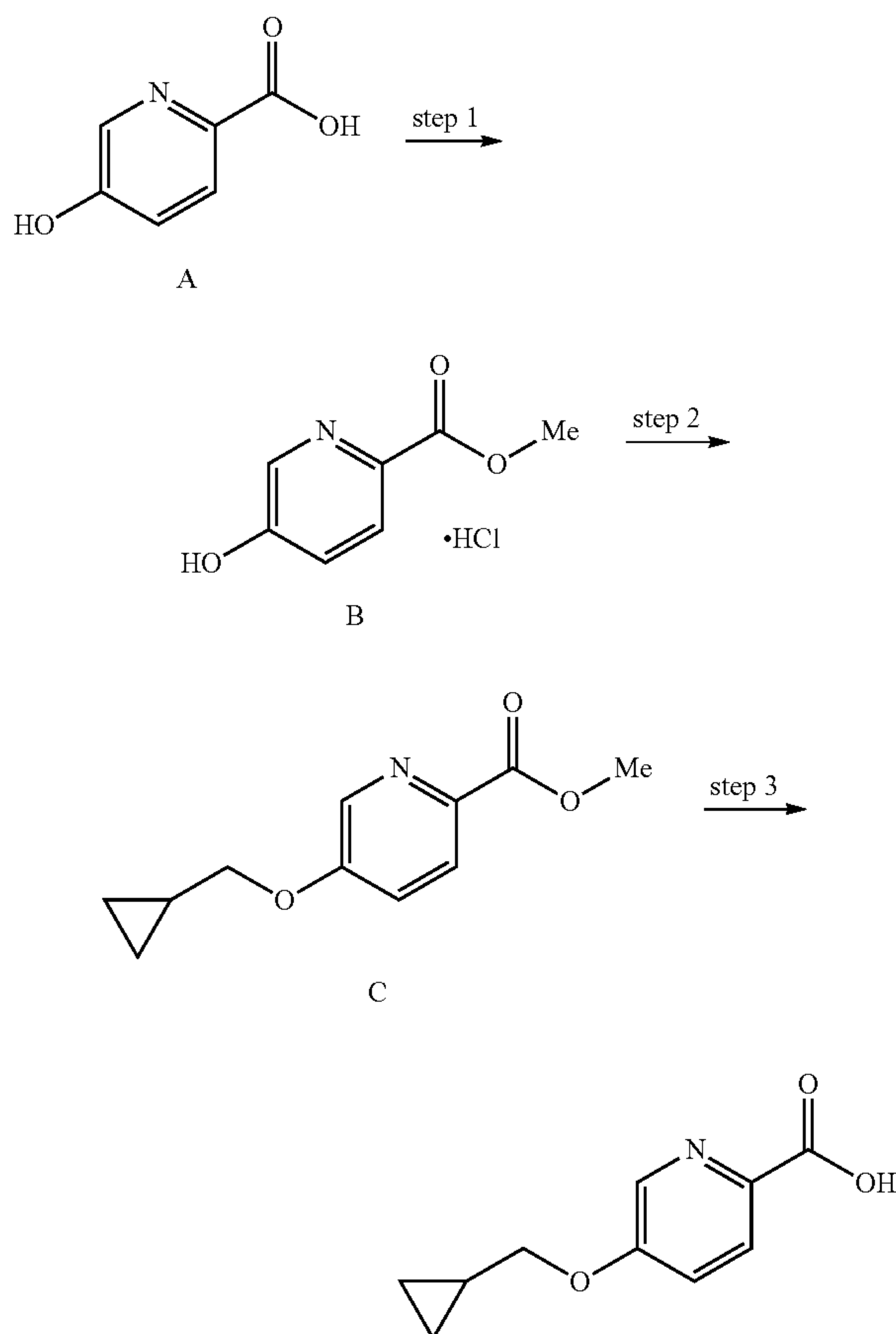
Scheme 11g:
