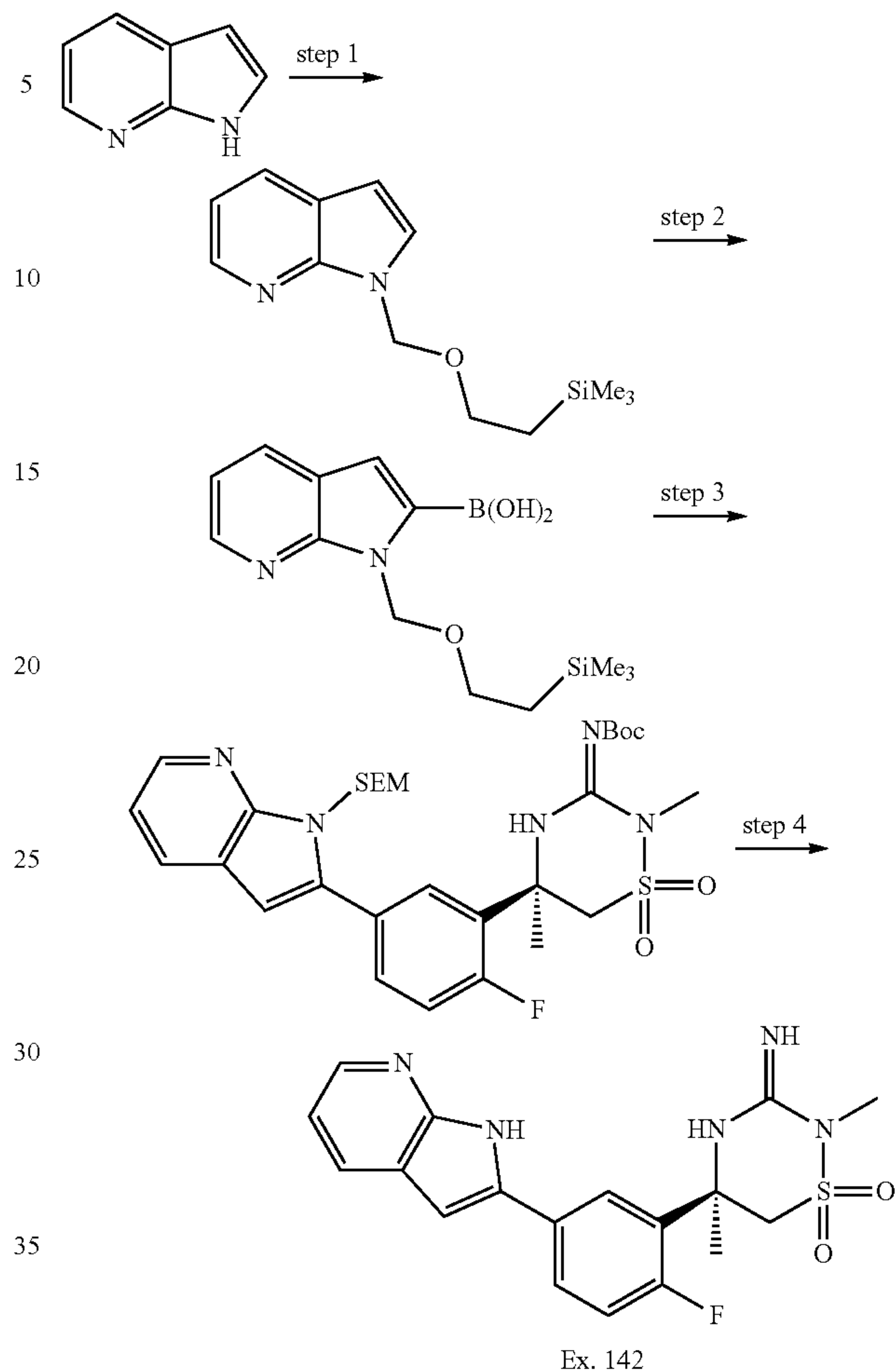
Scheme 31:
