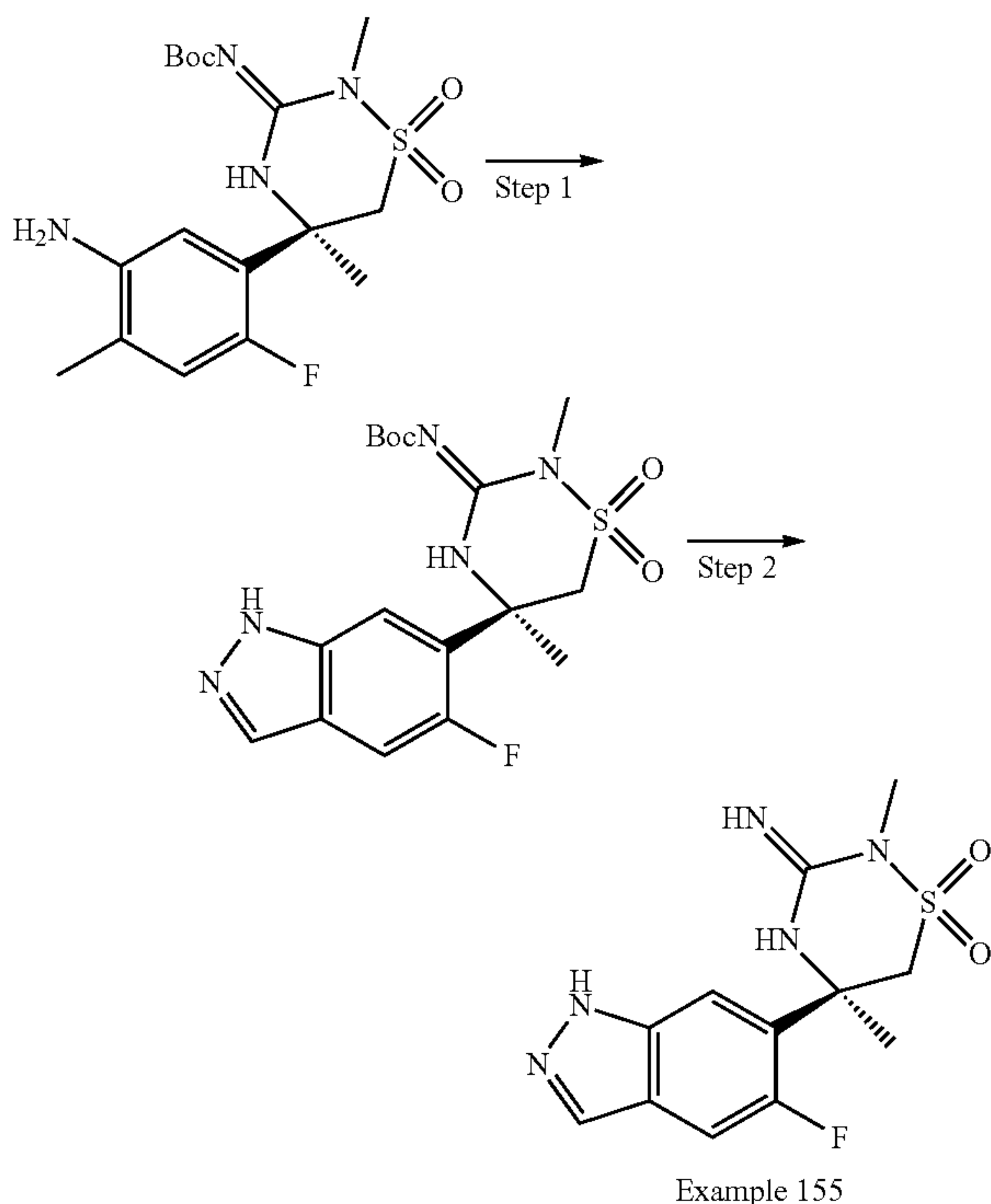
Scheme 36:
