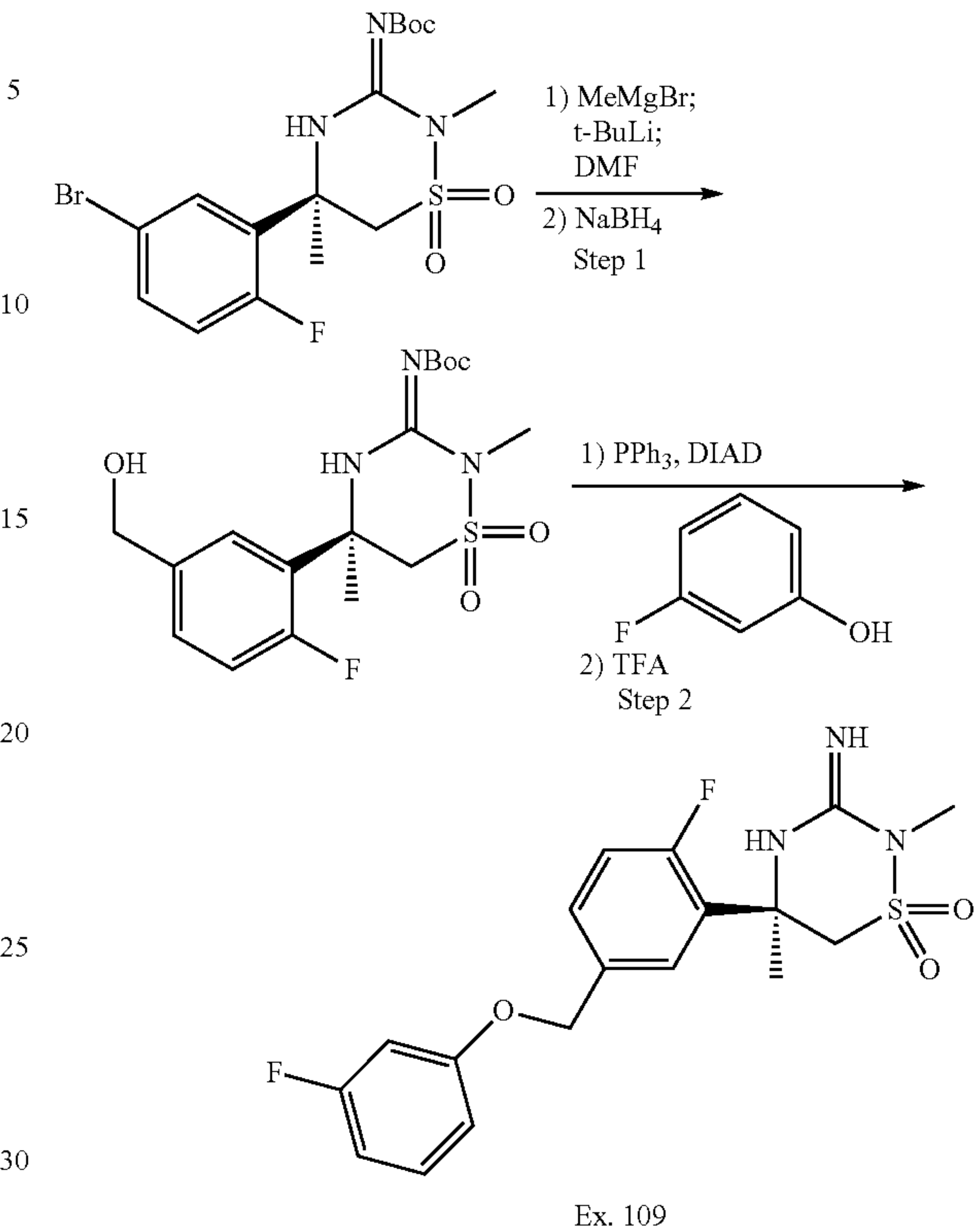
Scheme 21:
