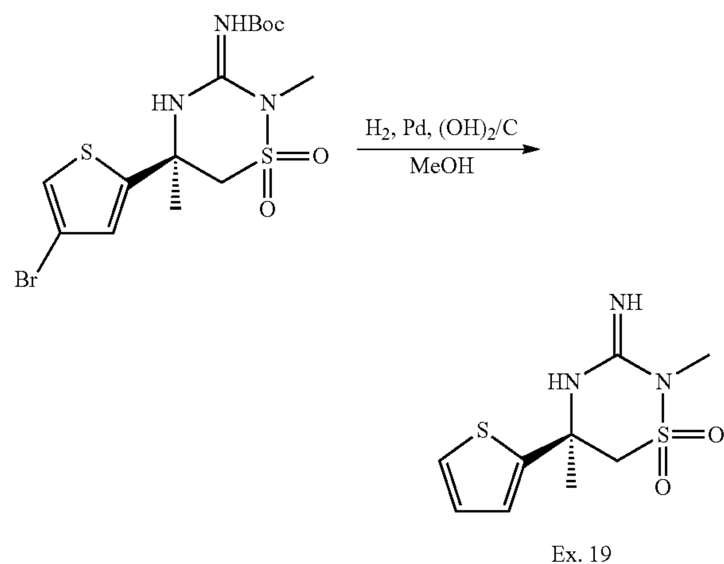
Scheme 9:
