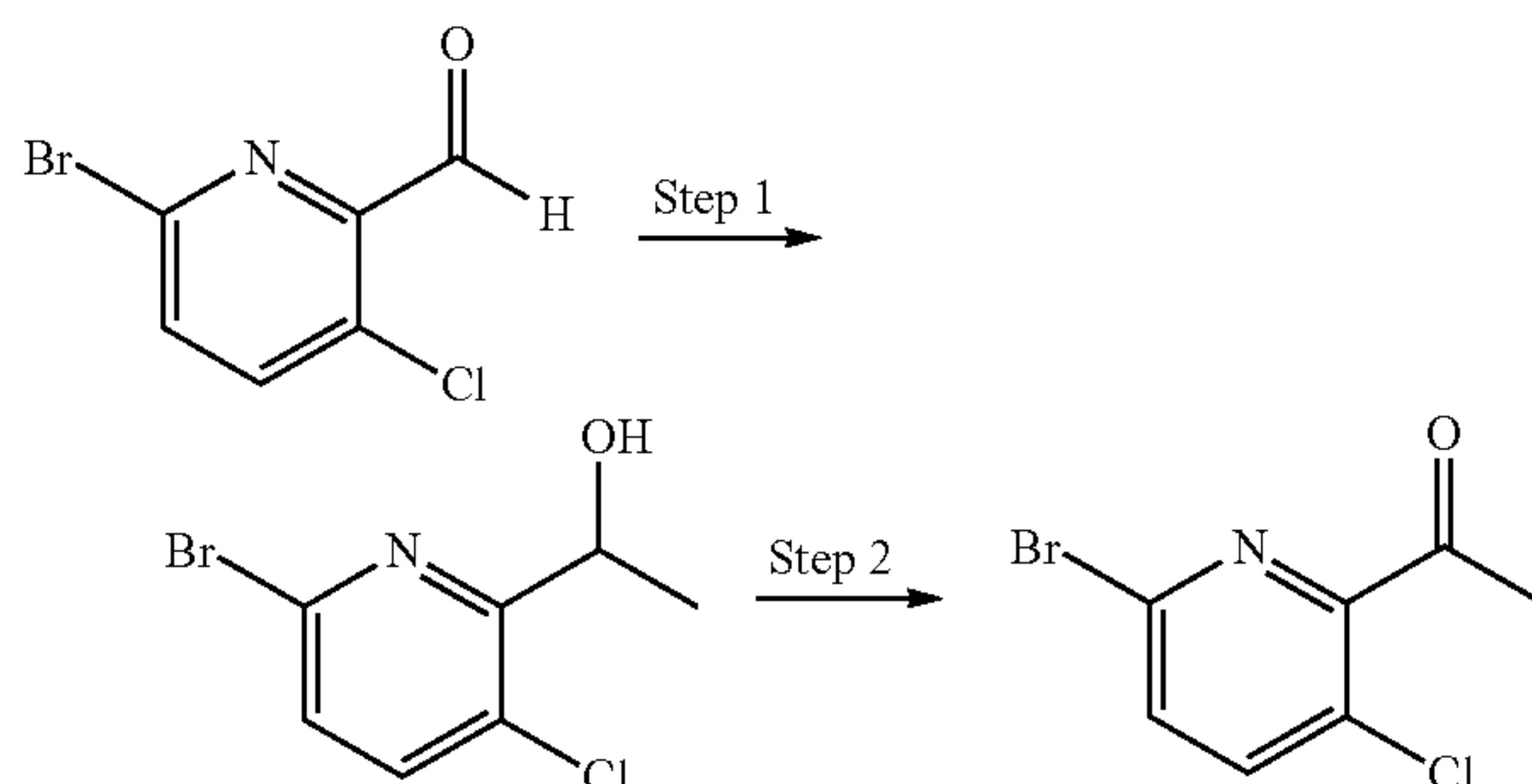
Scheme 2b:
