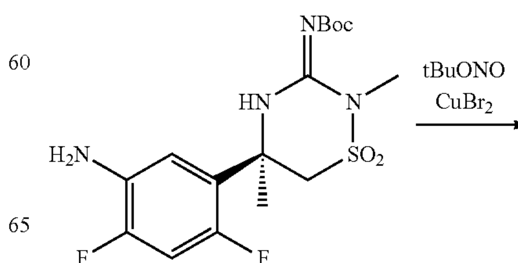
Scheme 11t:
