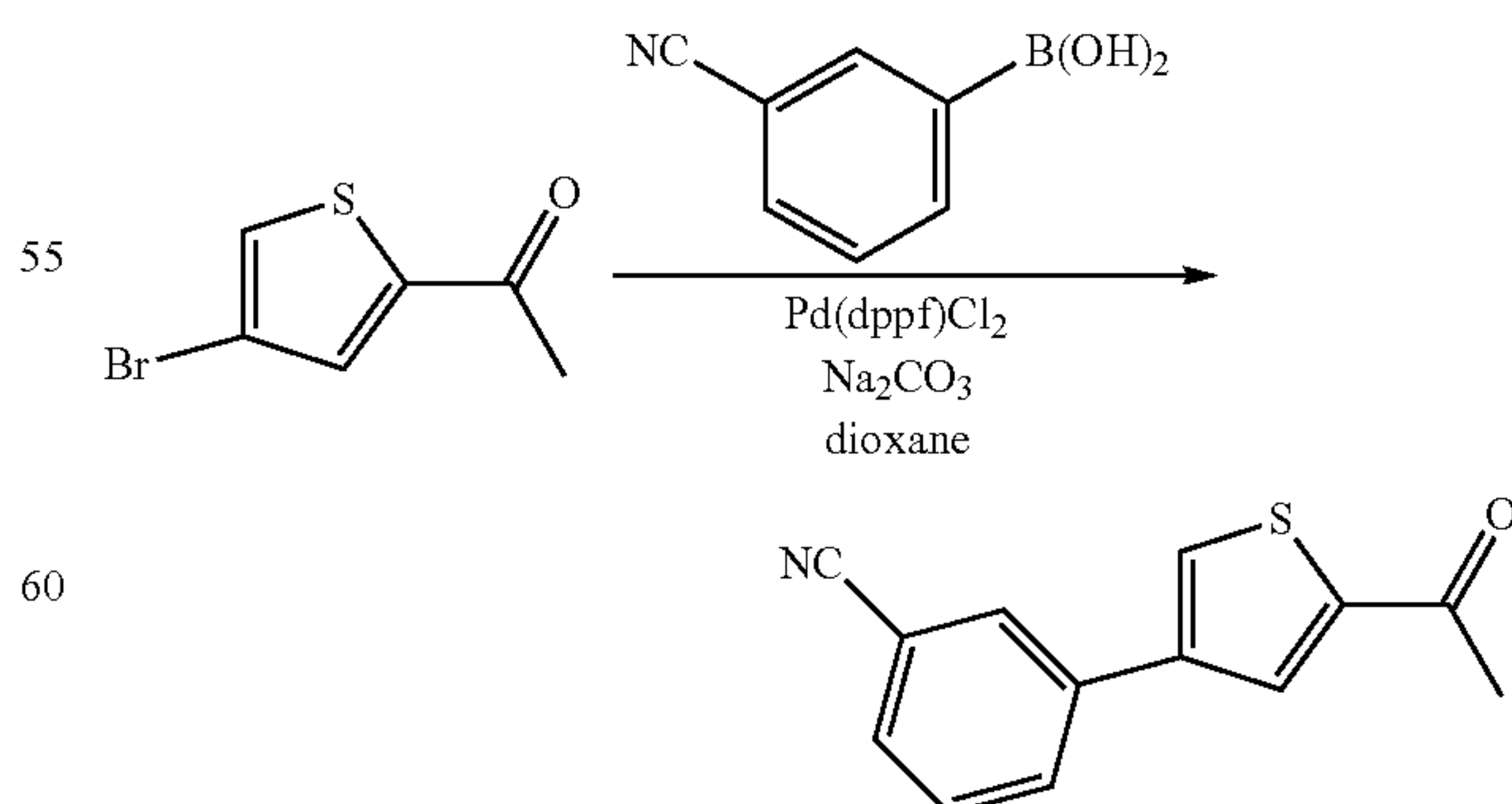
Scheme 20:
