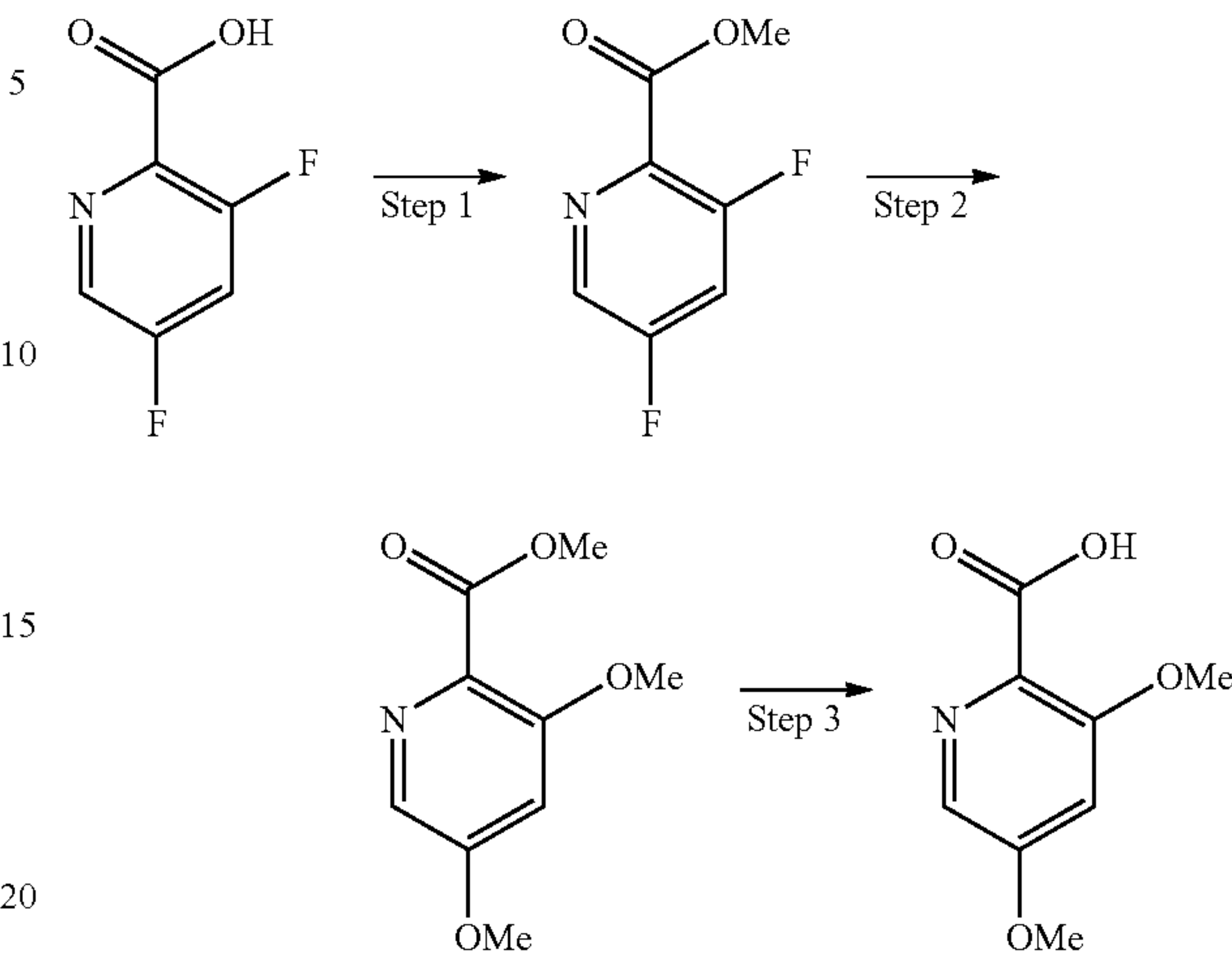
Scheme 11q:
