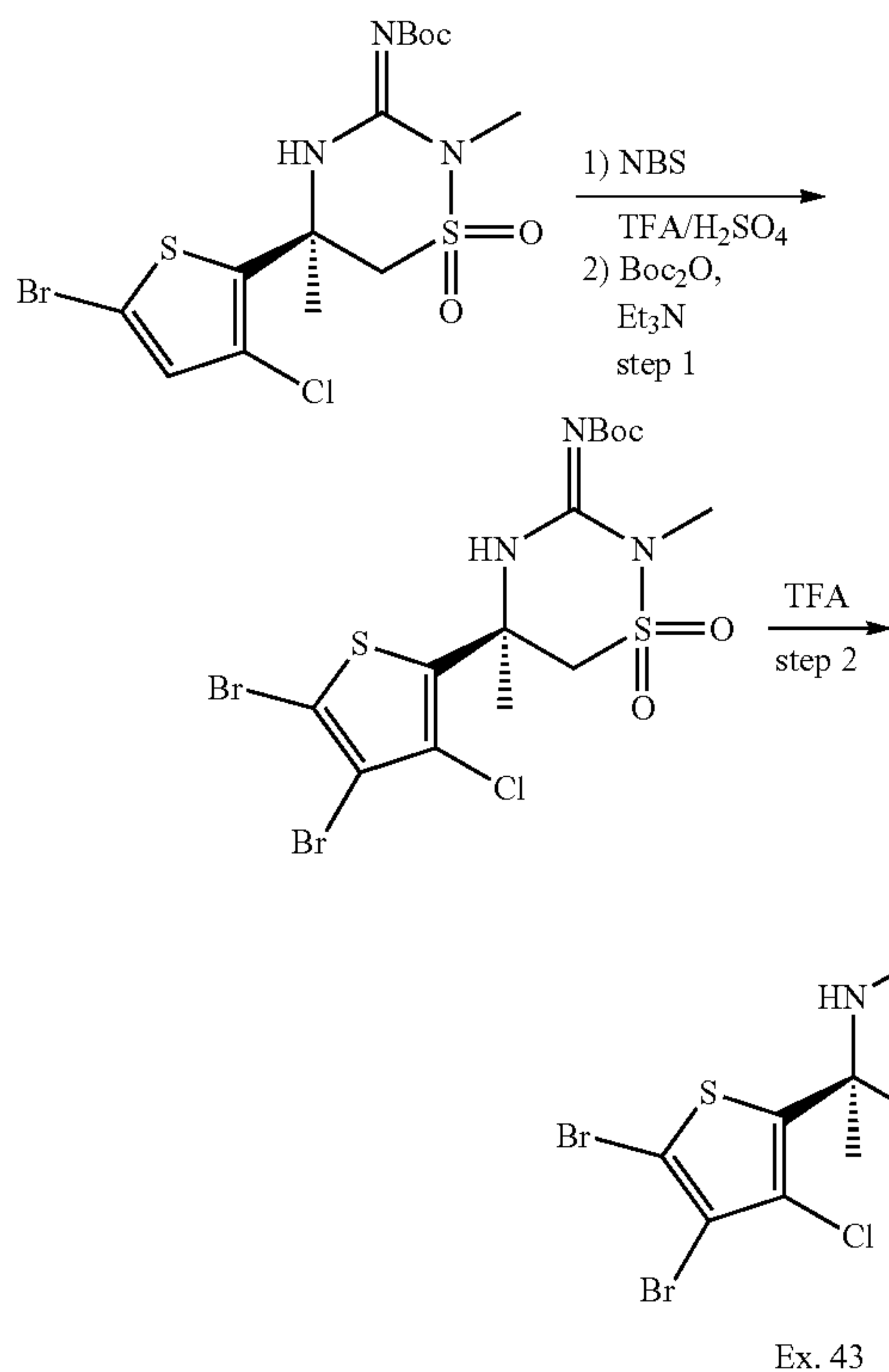
Scheme 14:
