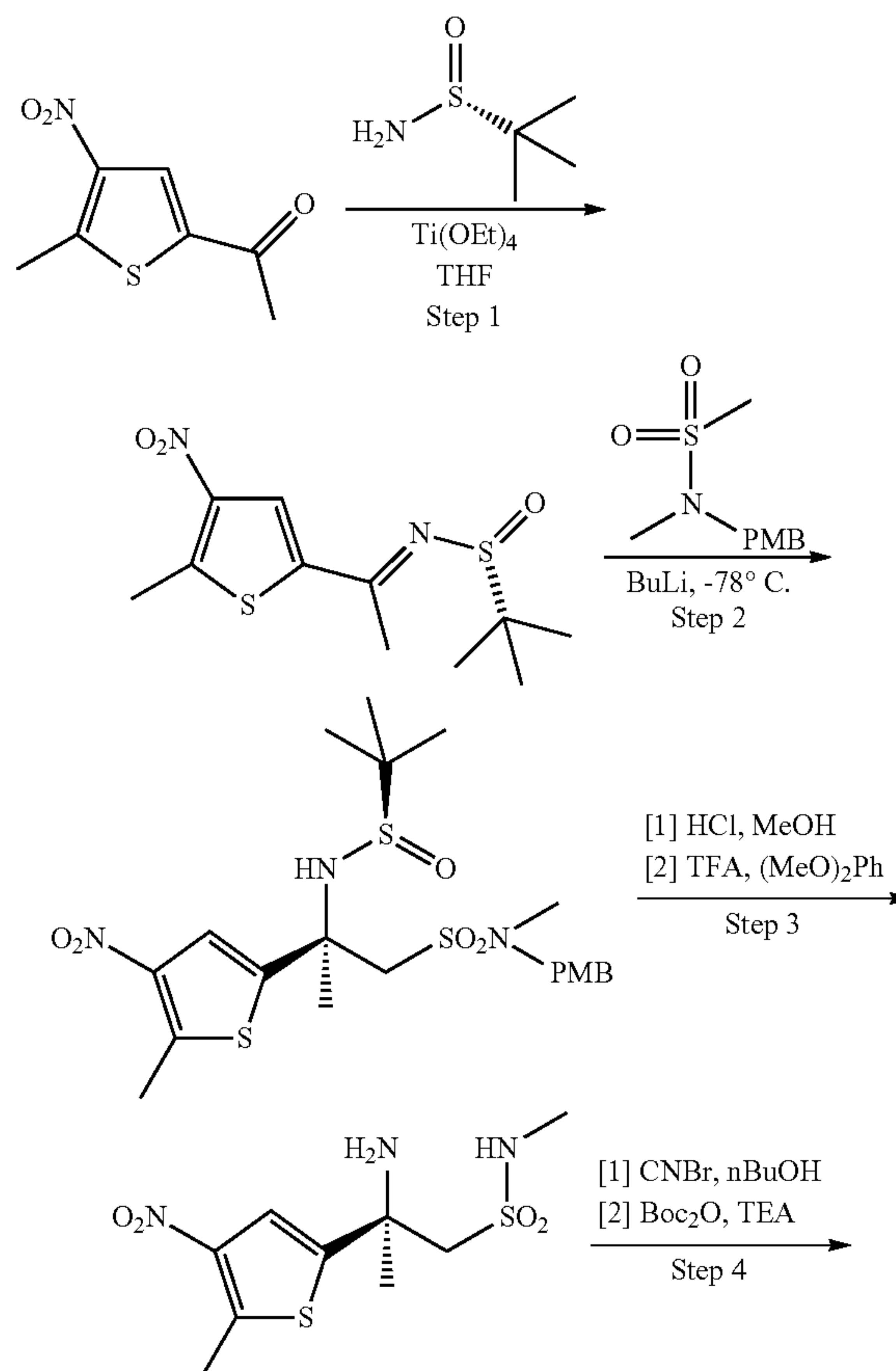
Scheme 44:
