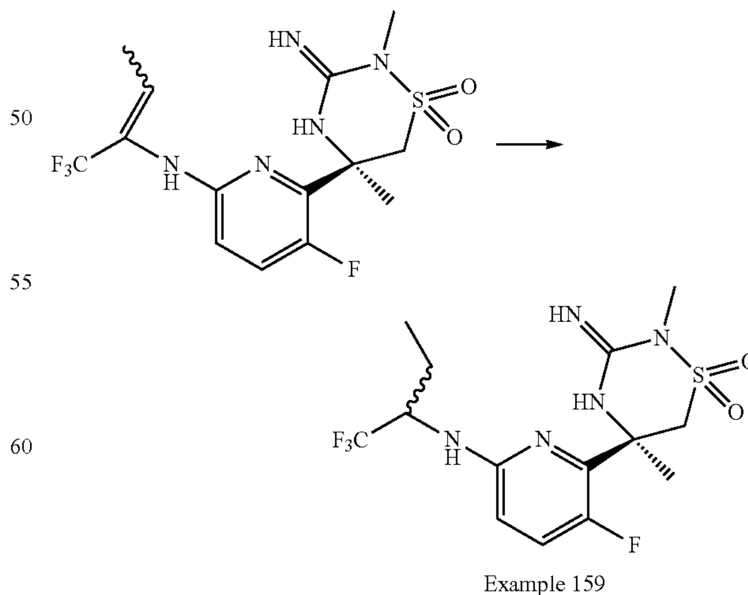
Scheme 38:
