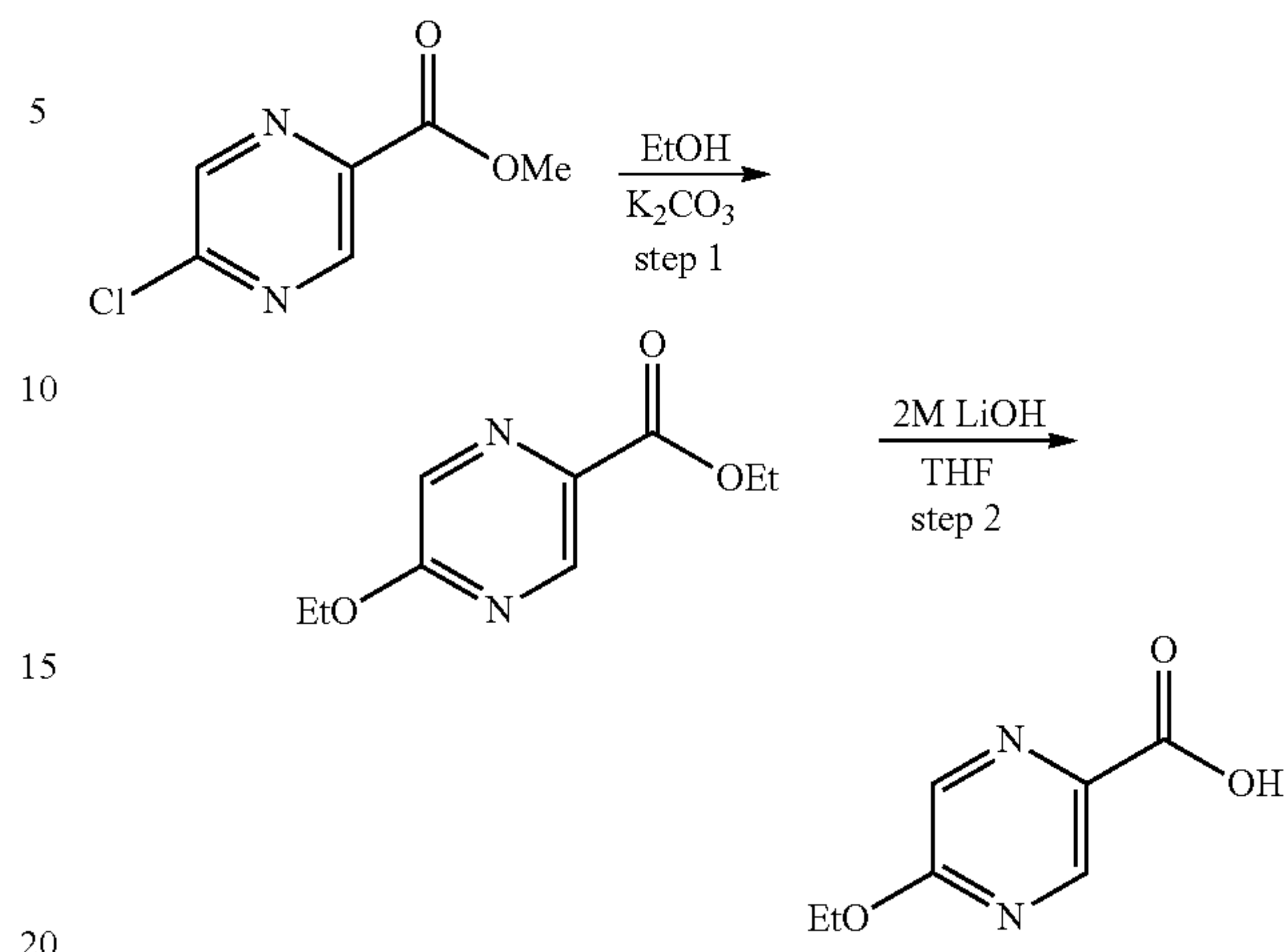
Scheme 11c:
