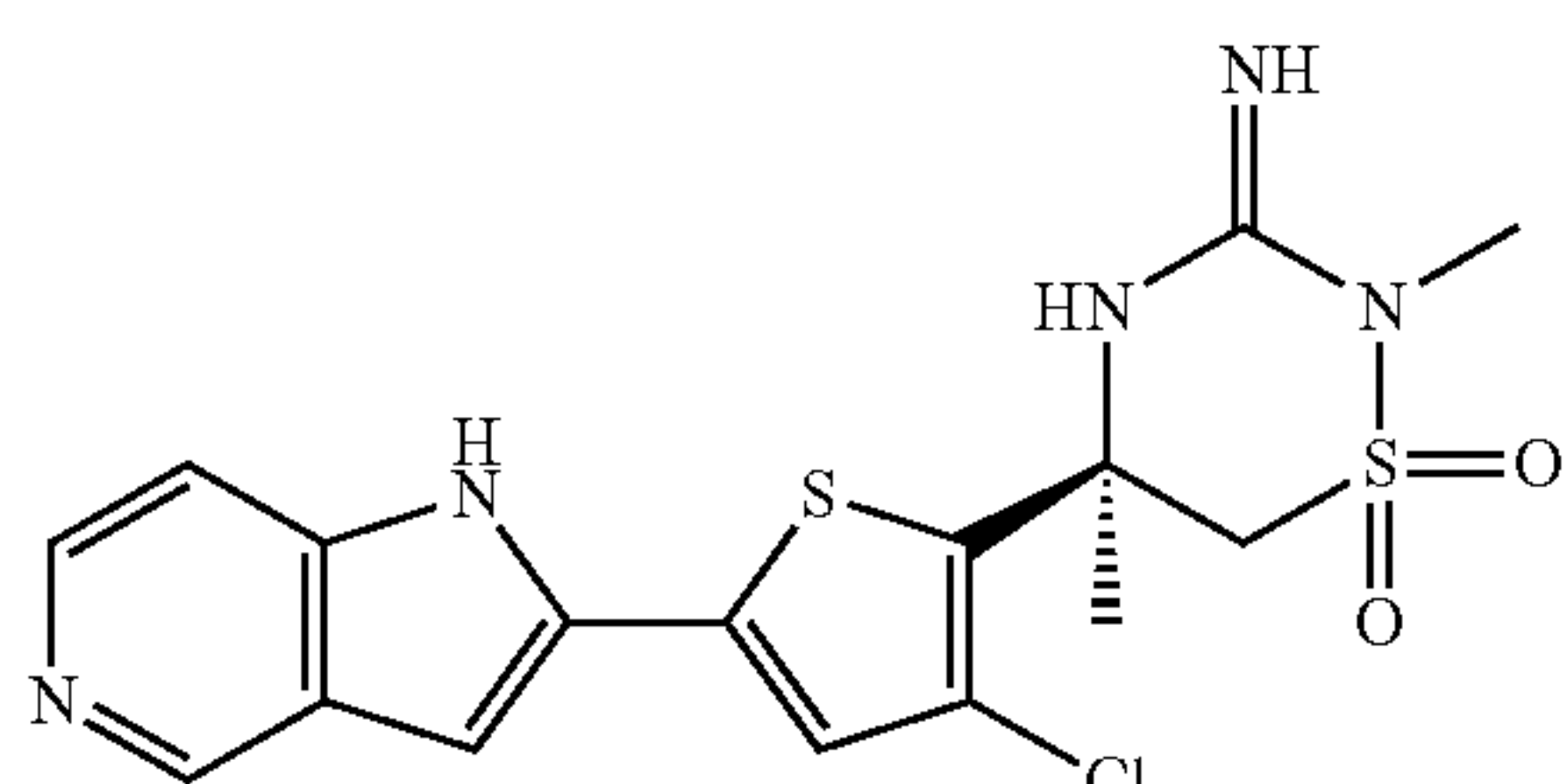
Scheme 35:
