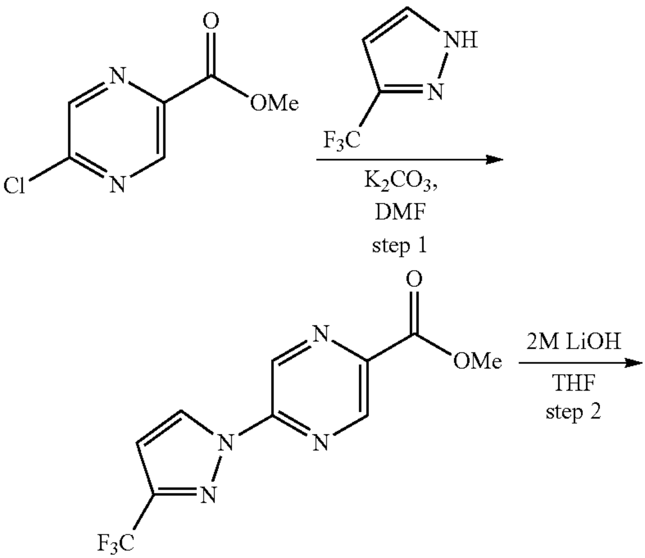
Scheme 11d:
