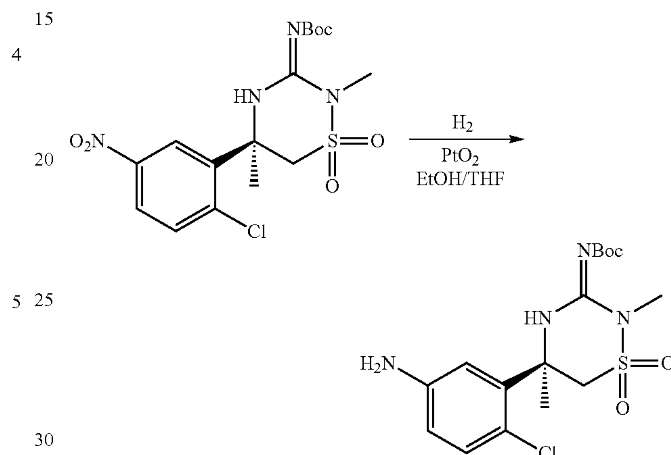
Scheme 11a:
