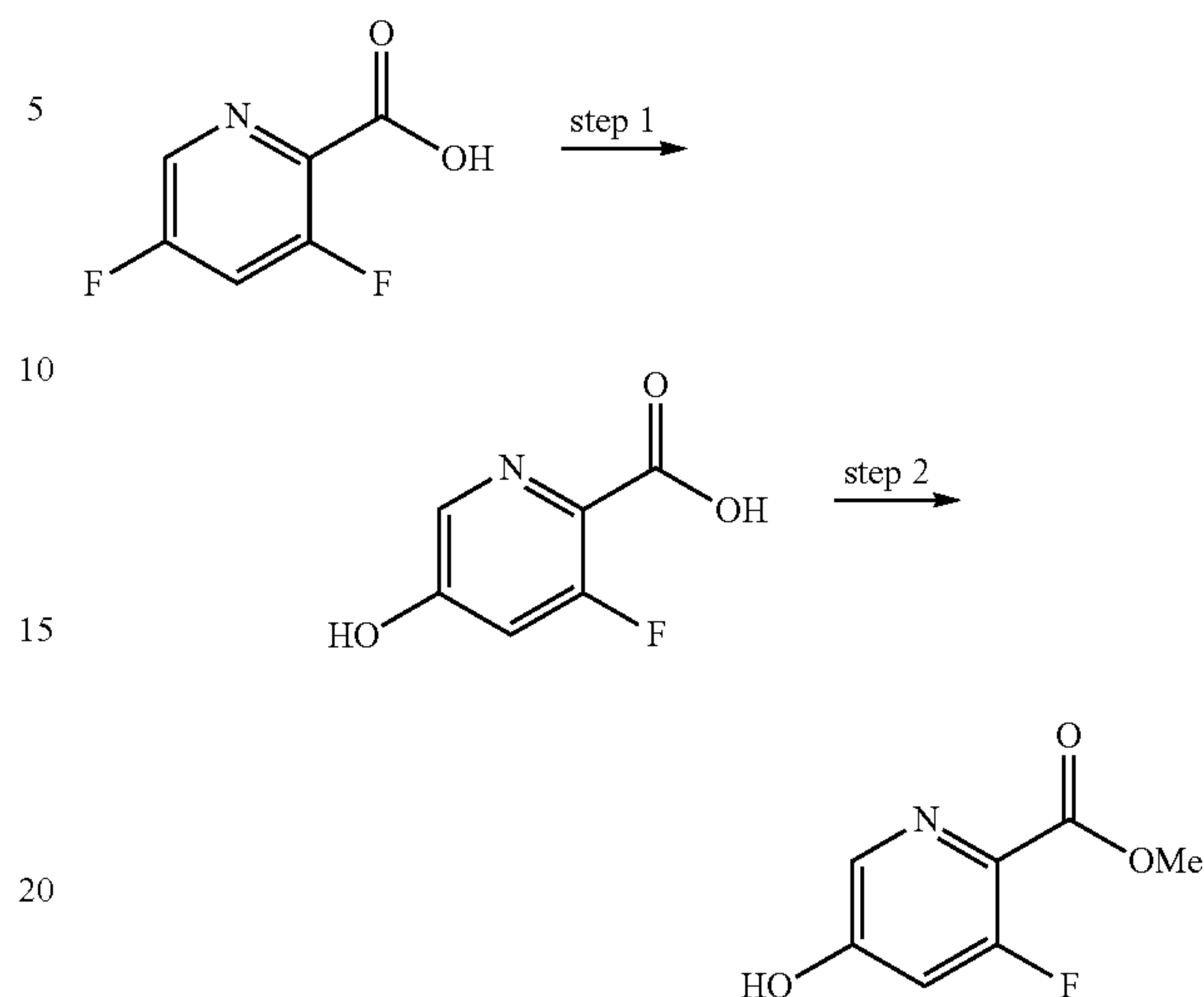
Scheme 11h:
