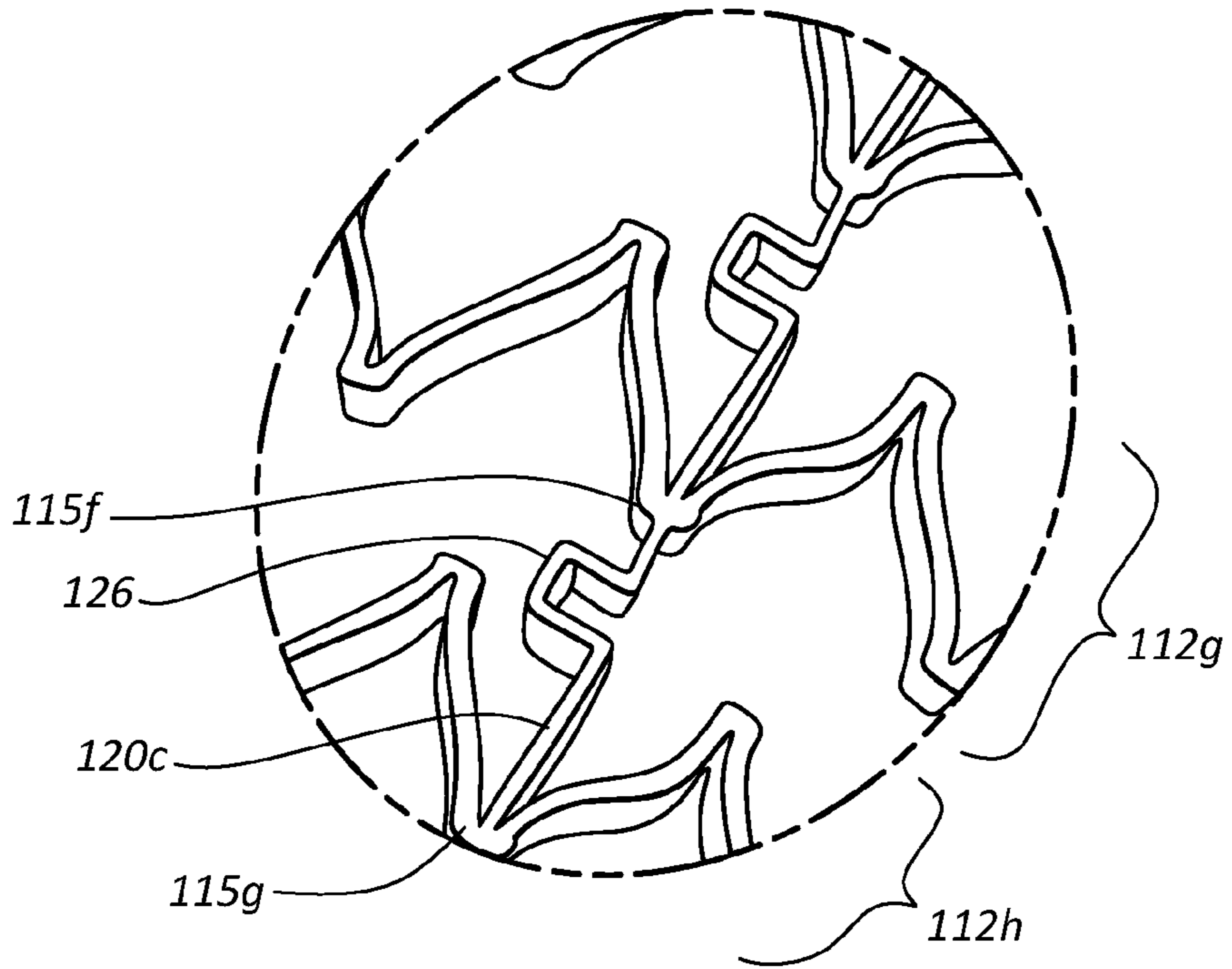
FIG. 1D
