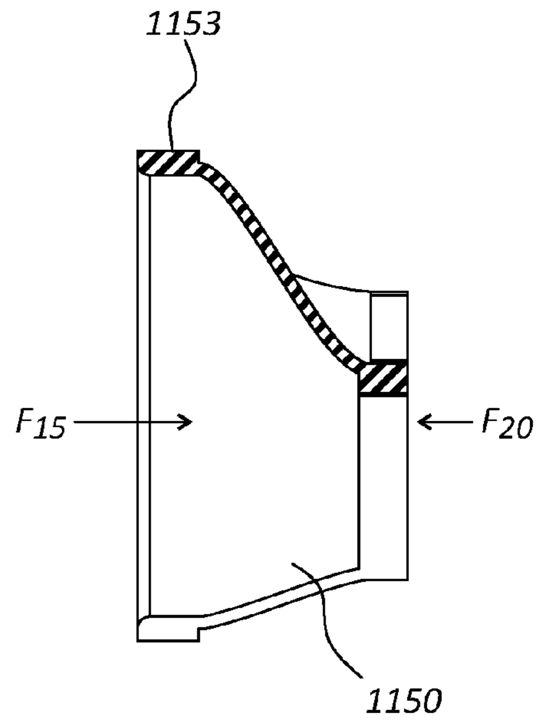
FIG. 11D
