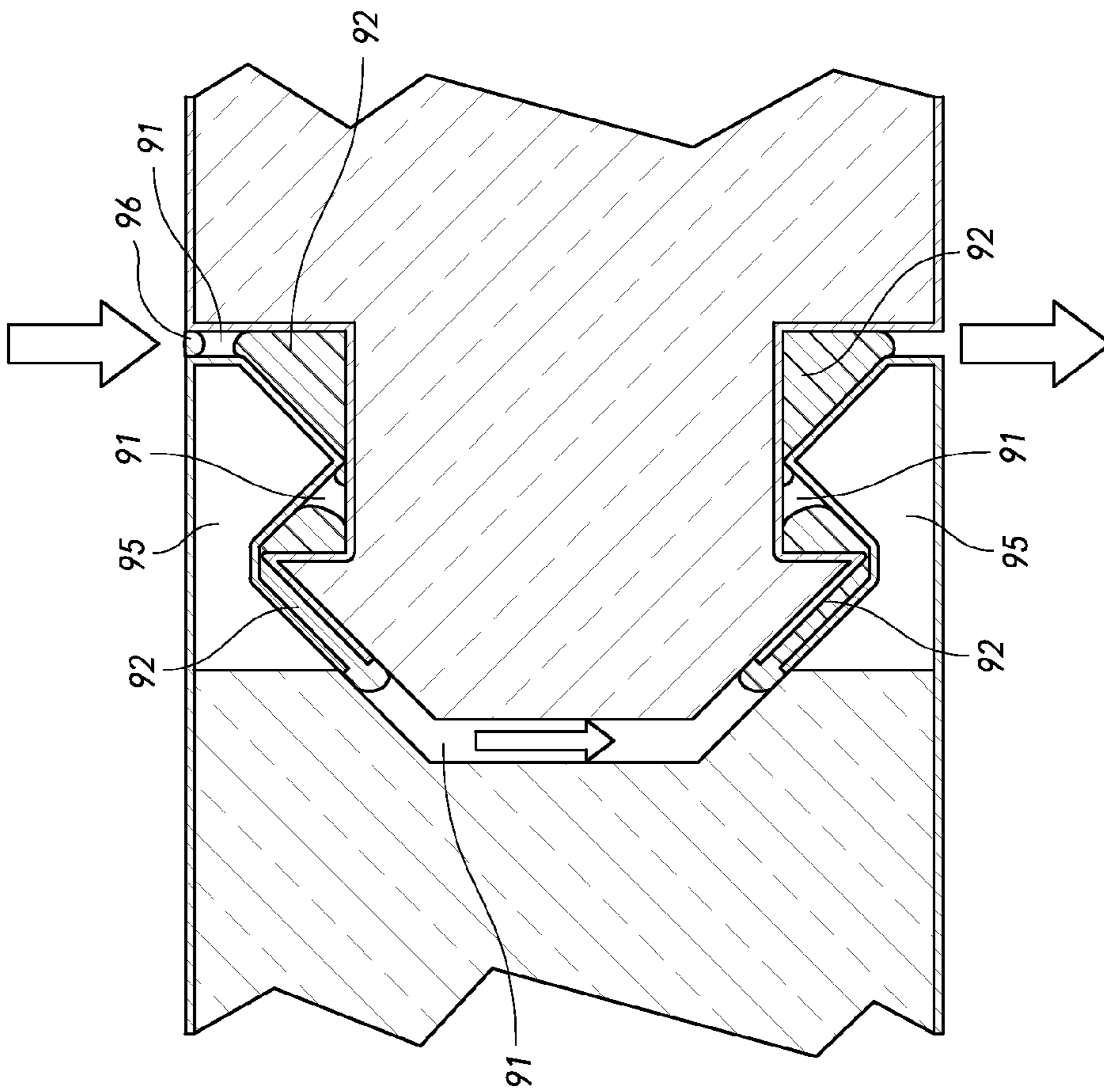
FIG. 9 (PRIOR ART)
