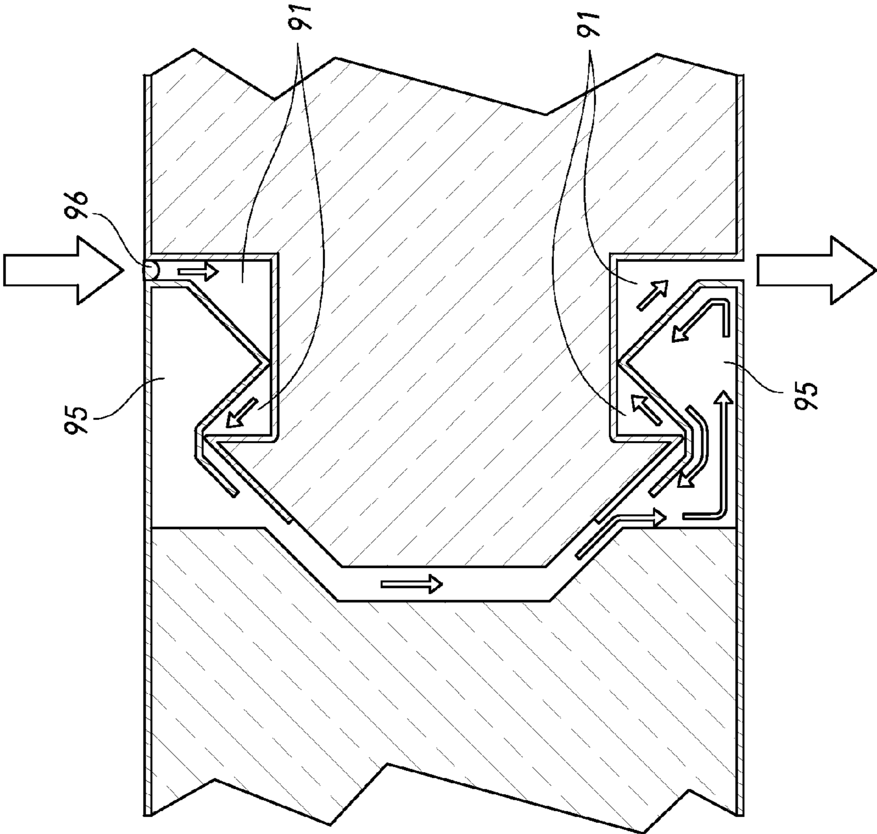
FIG. 10 (PRIOR ART)
