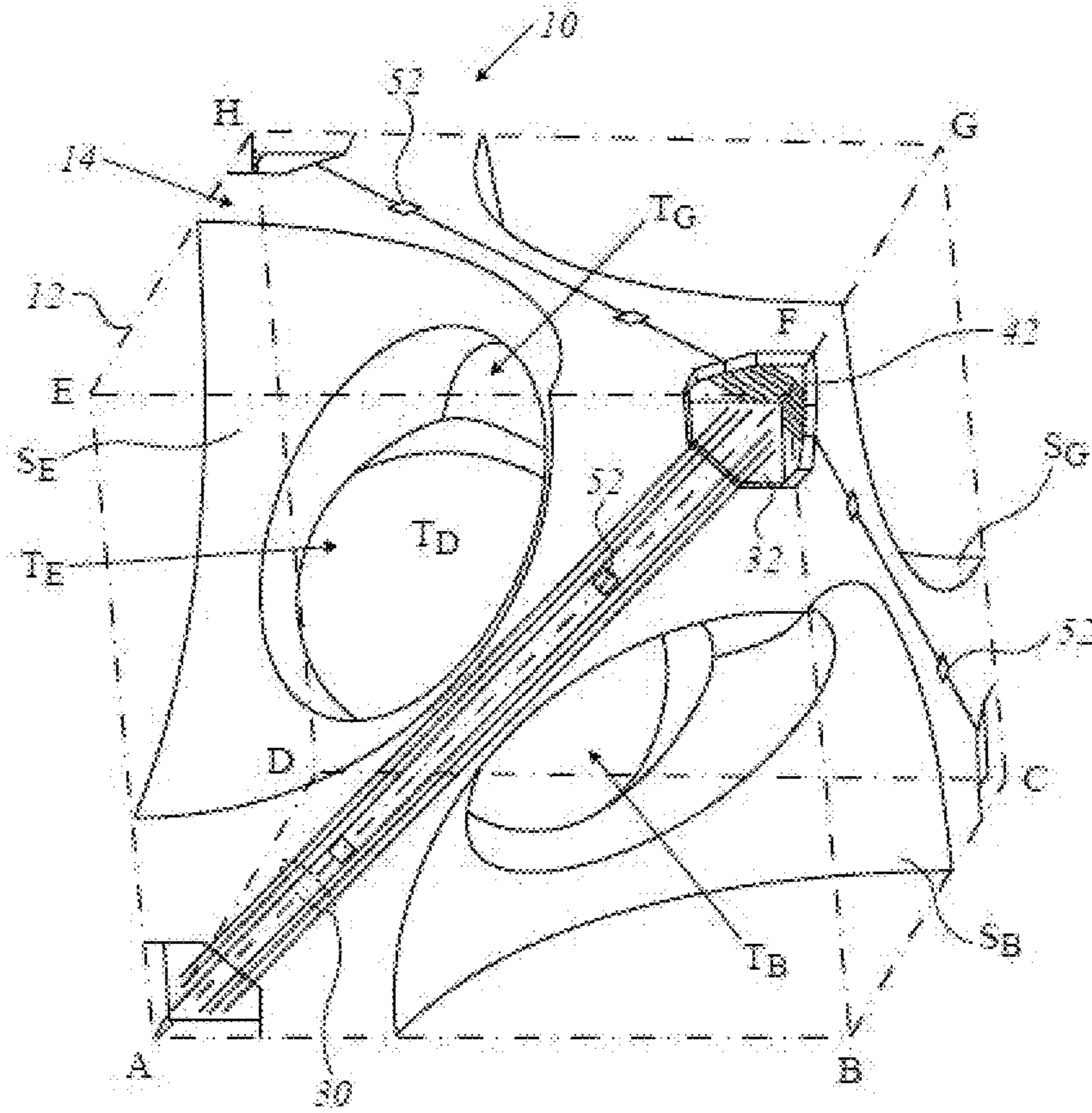
FIG. 1 Prior art
