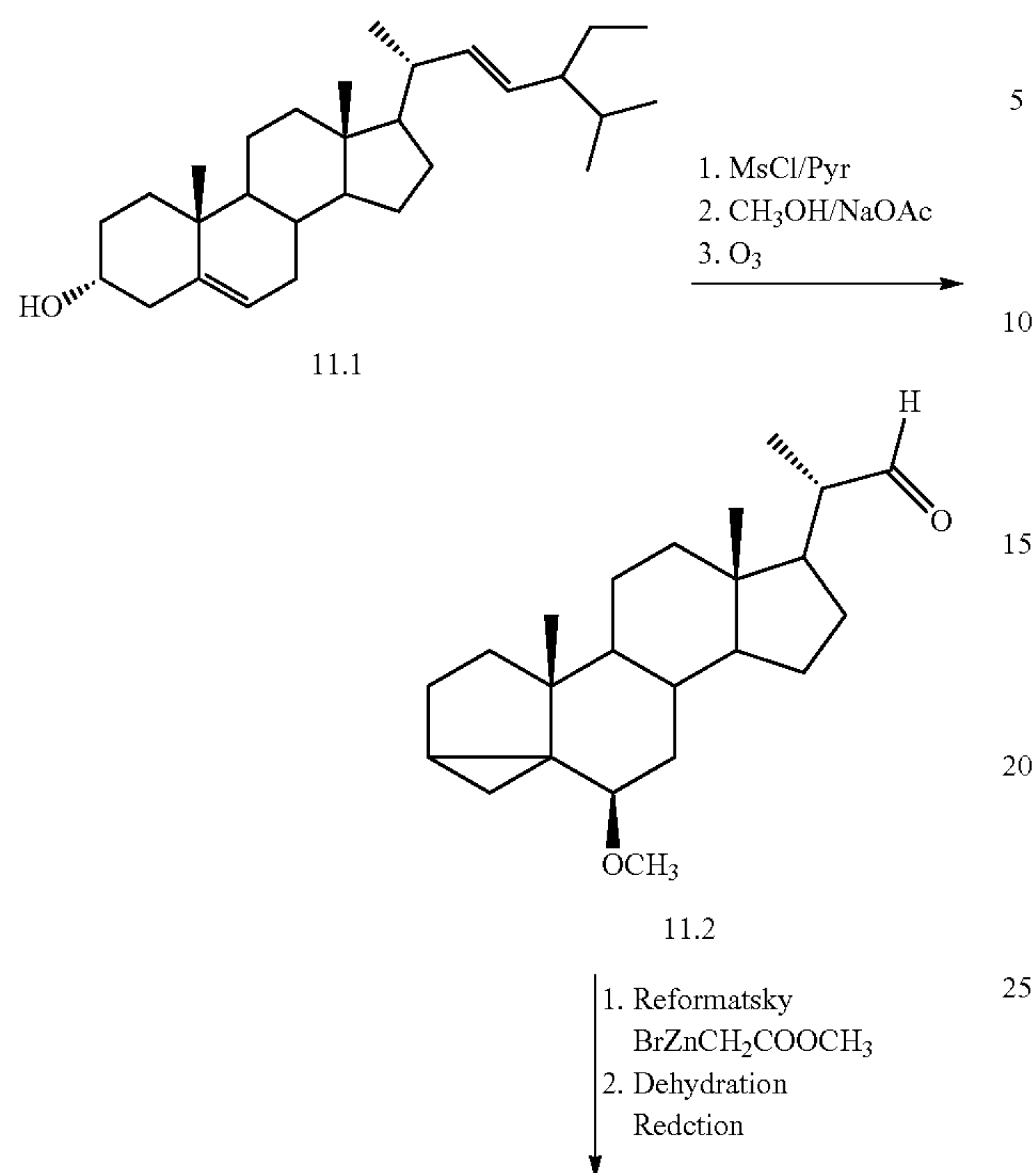
Scheme 11. Ozonolysis of i-seroid and side chain reduction
