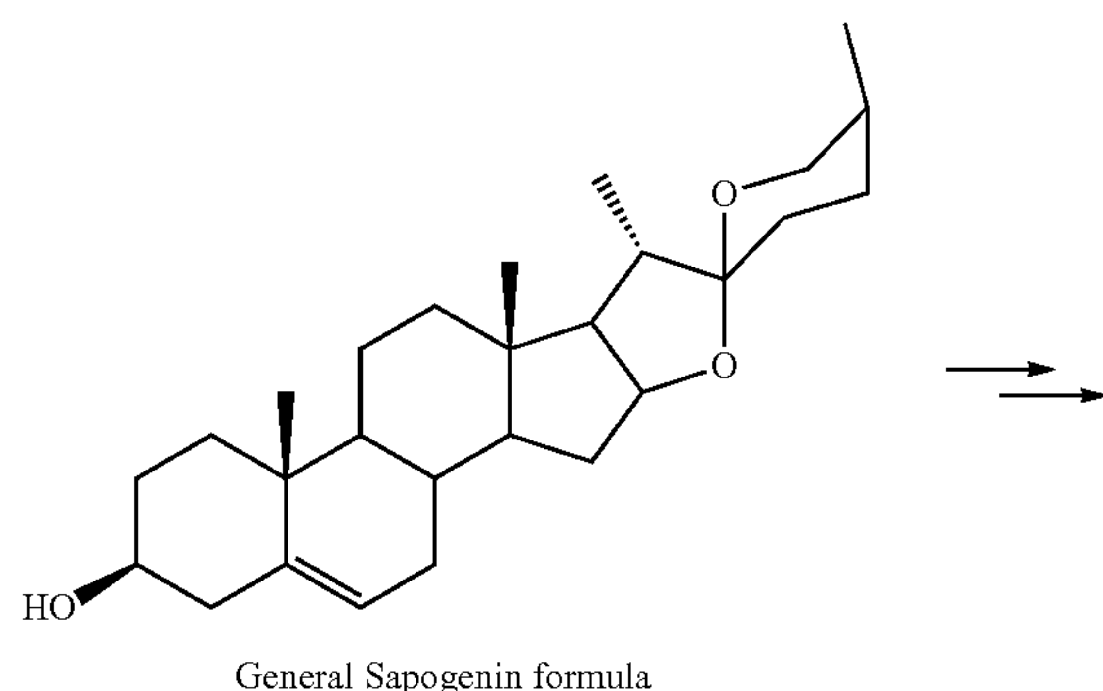
Scheme 10B. Synthetic route from saponin.
