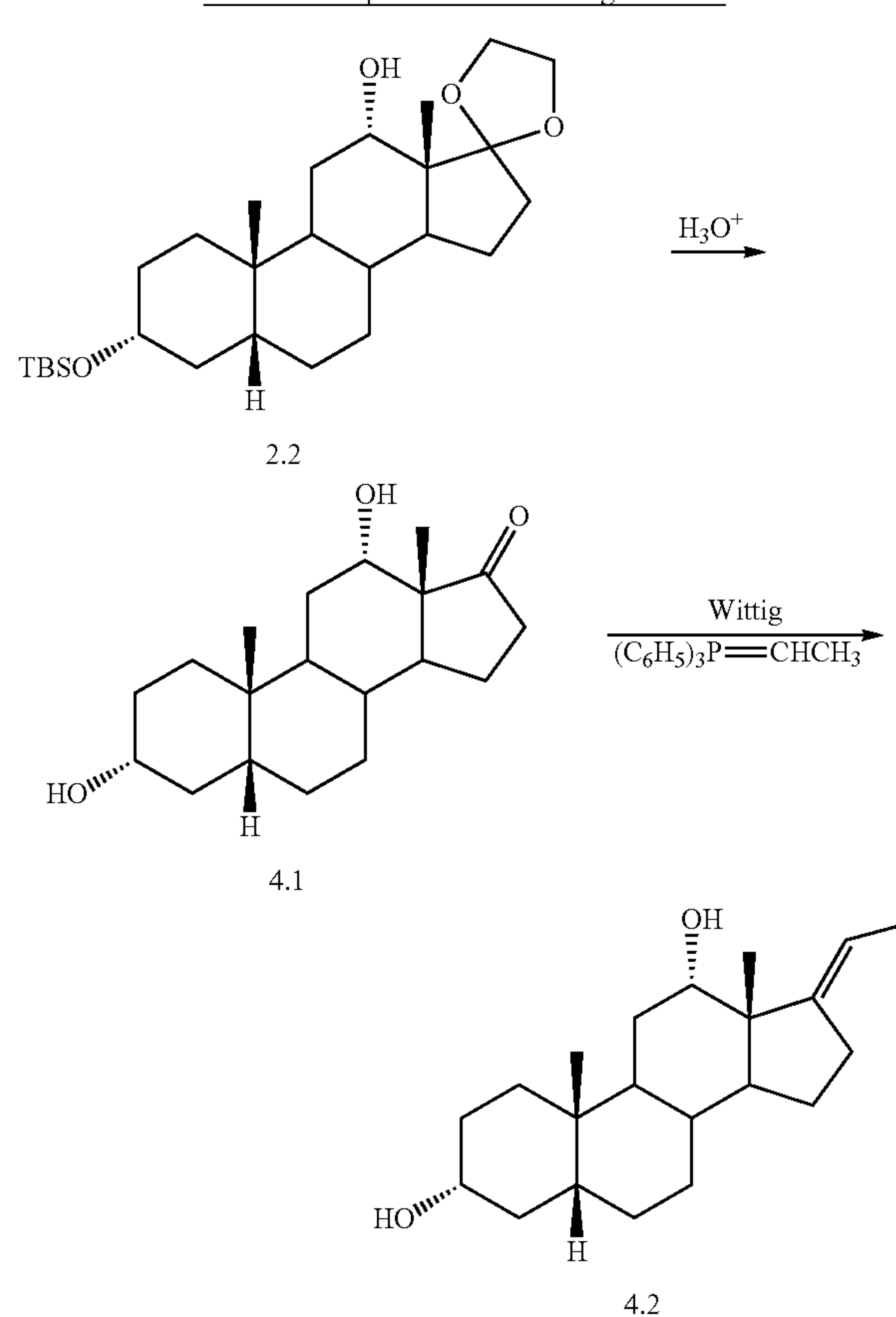
Scheme 4. Deprotection and Wittig Reaction
