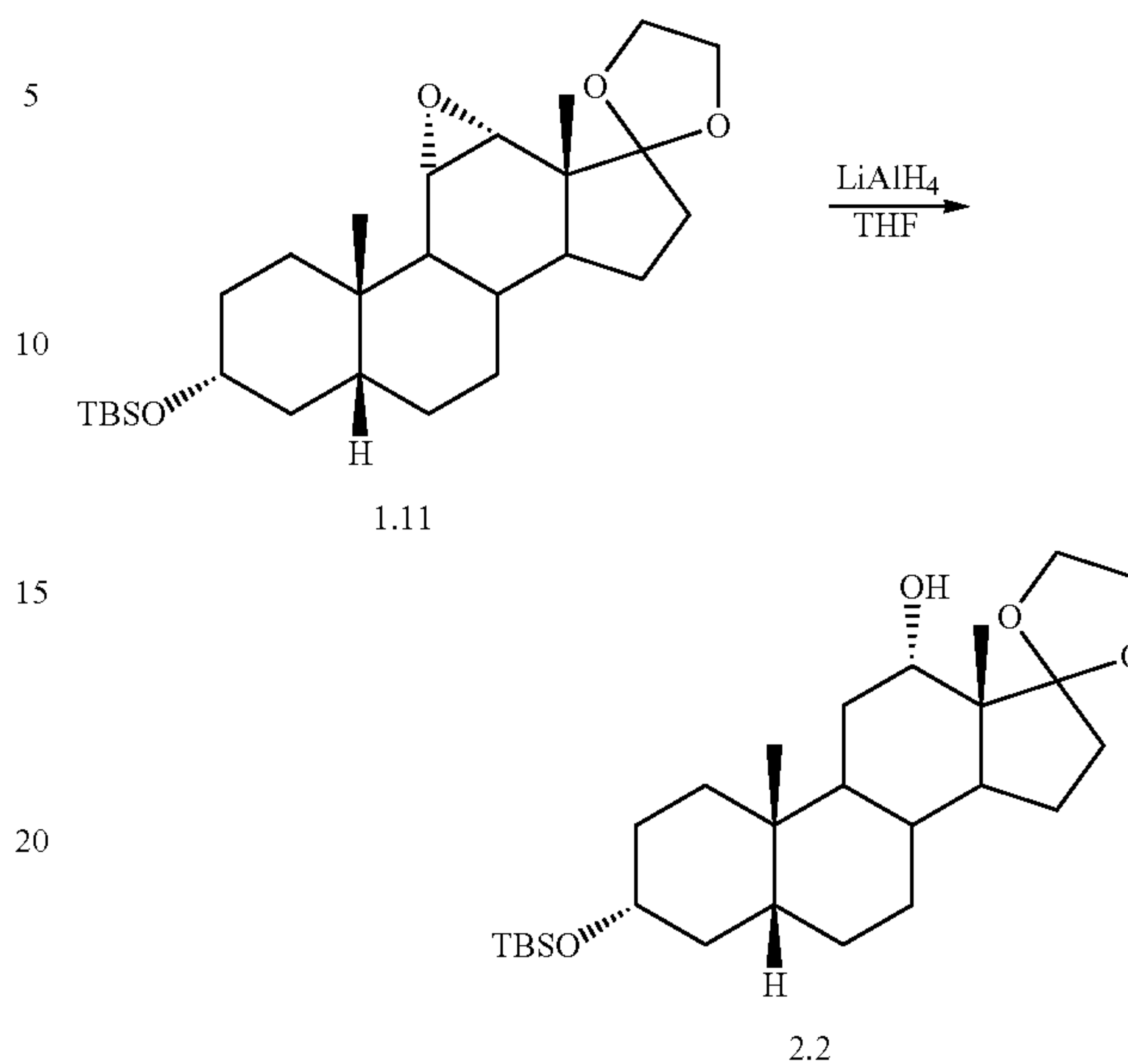
Scheme 3. Stereoselective Reduction of C 11 —C 12 epoxide.
