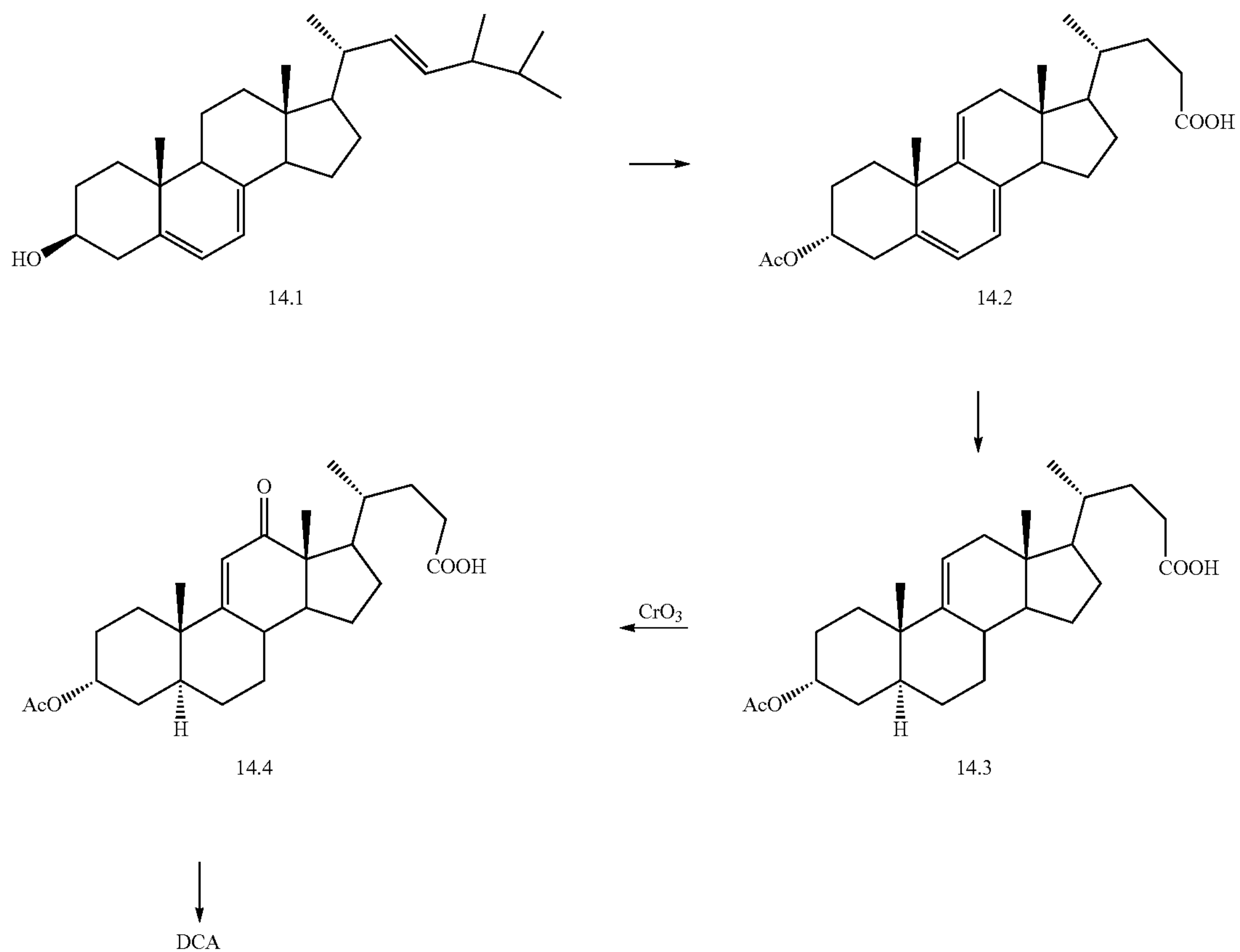
Scheme 14. Triene formation from Ergosterol
