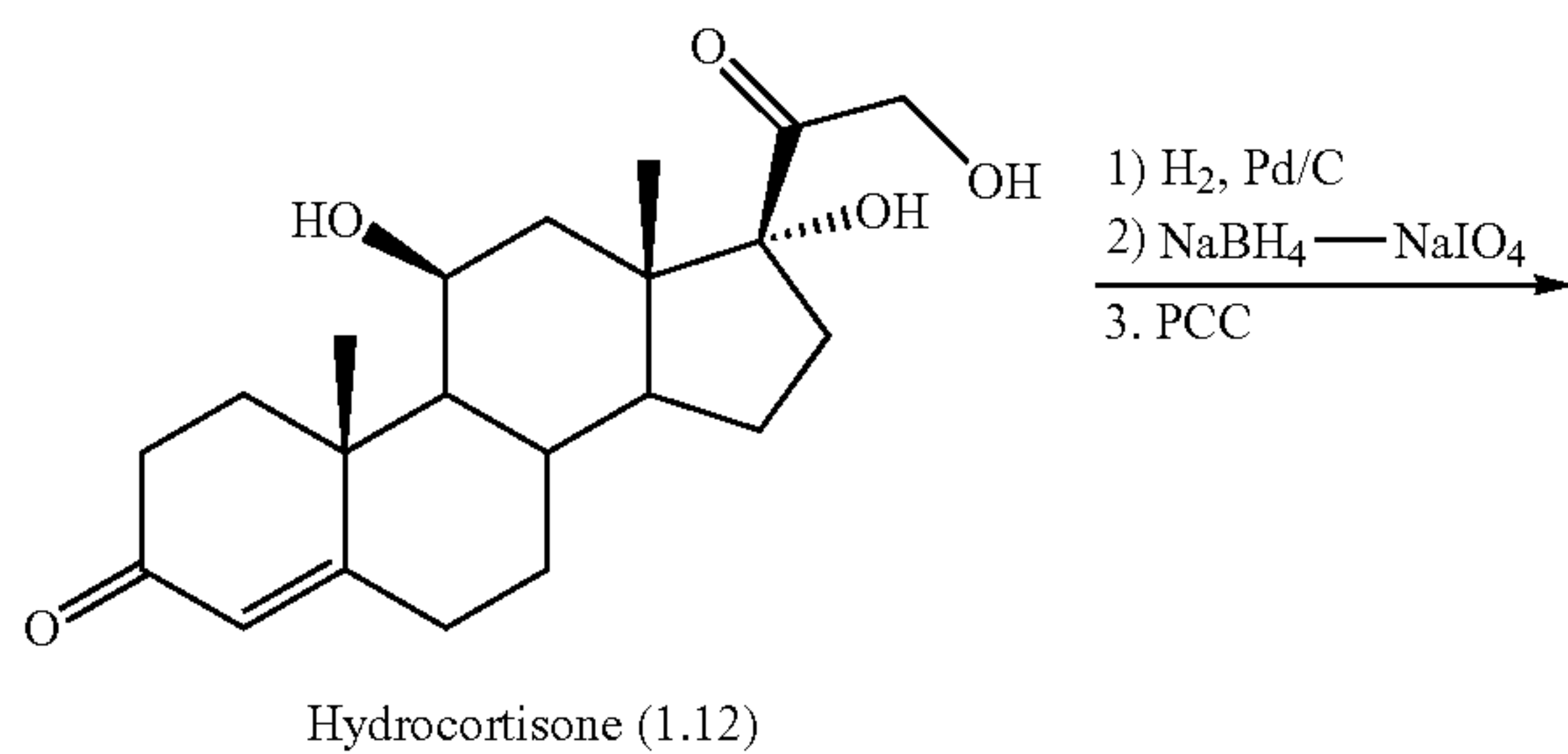
Scheme 1B. Synthesis of DCA from Hydrocortisone
