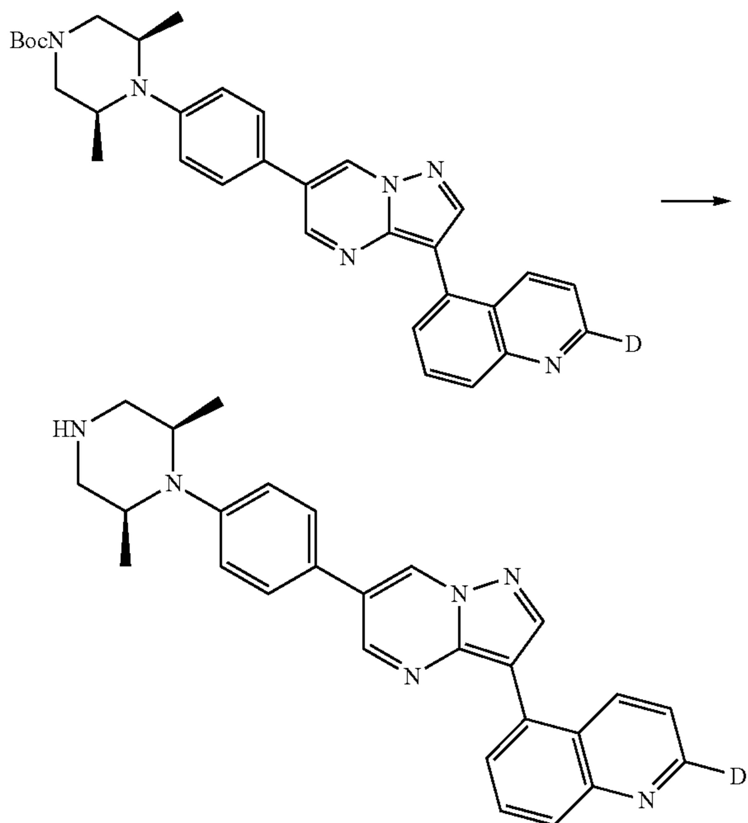
Scheme 183
