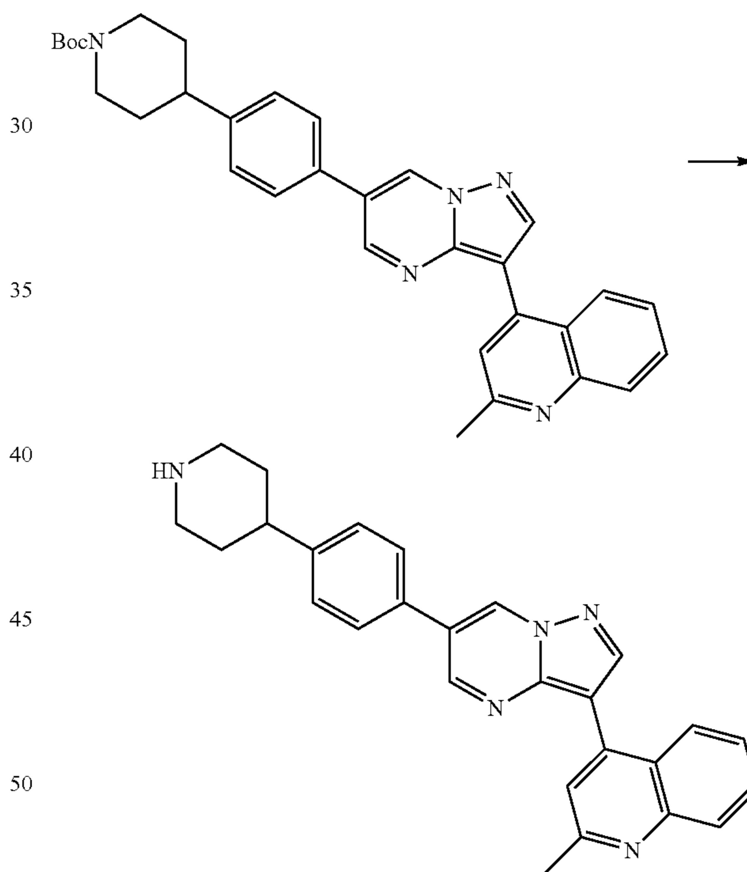
Scheme 45
