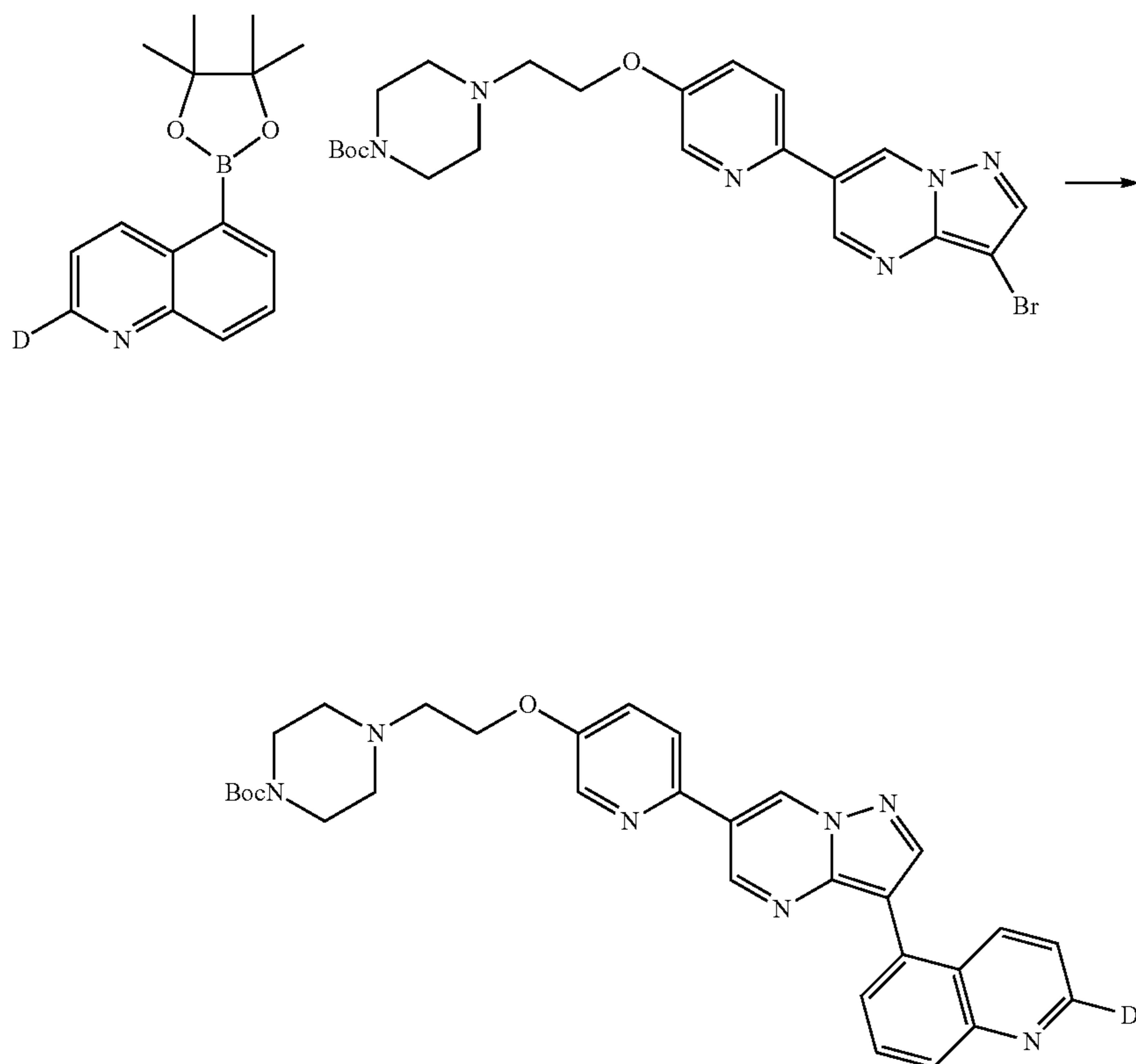
Scheme 175
