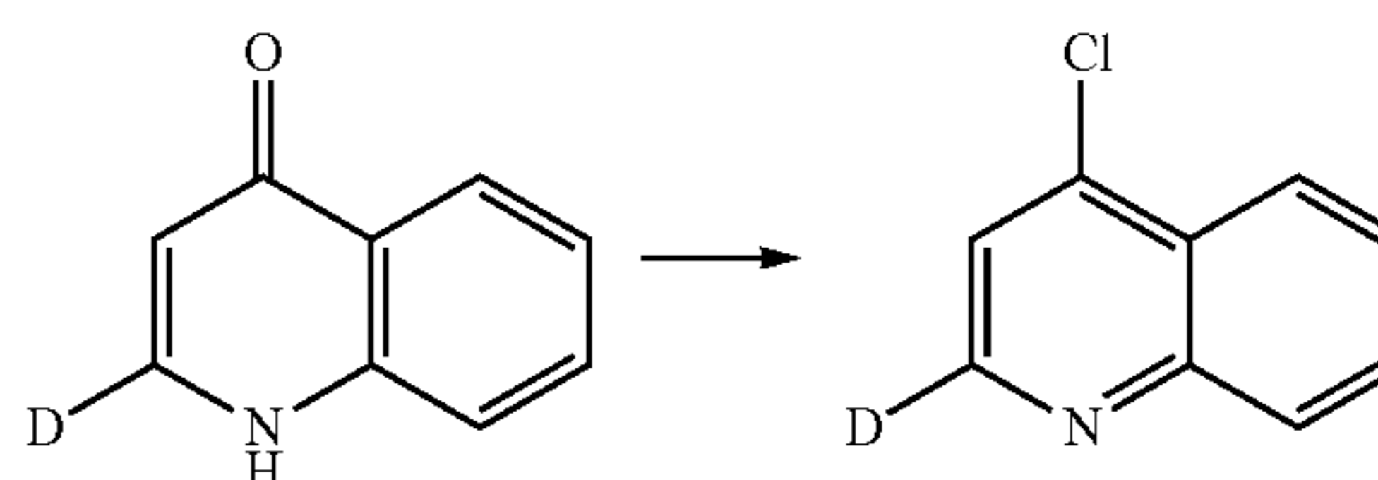
Scheme 48
