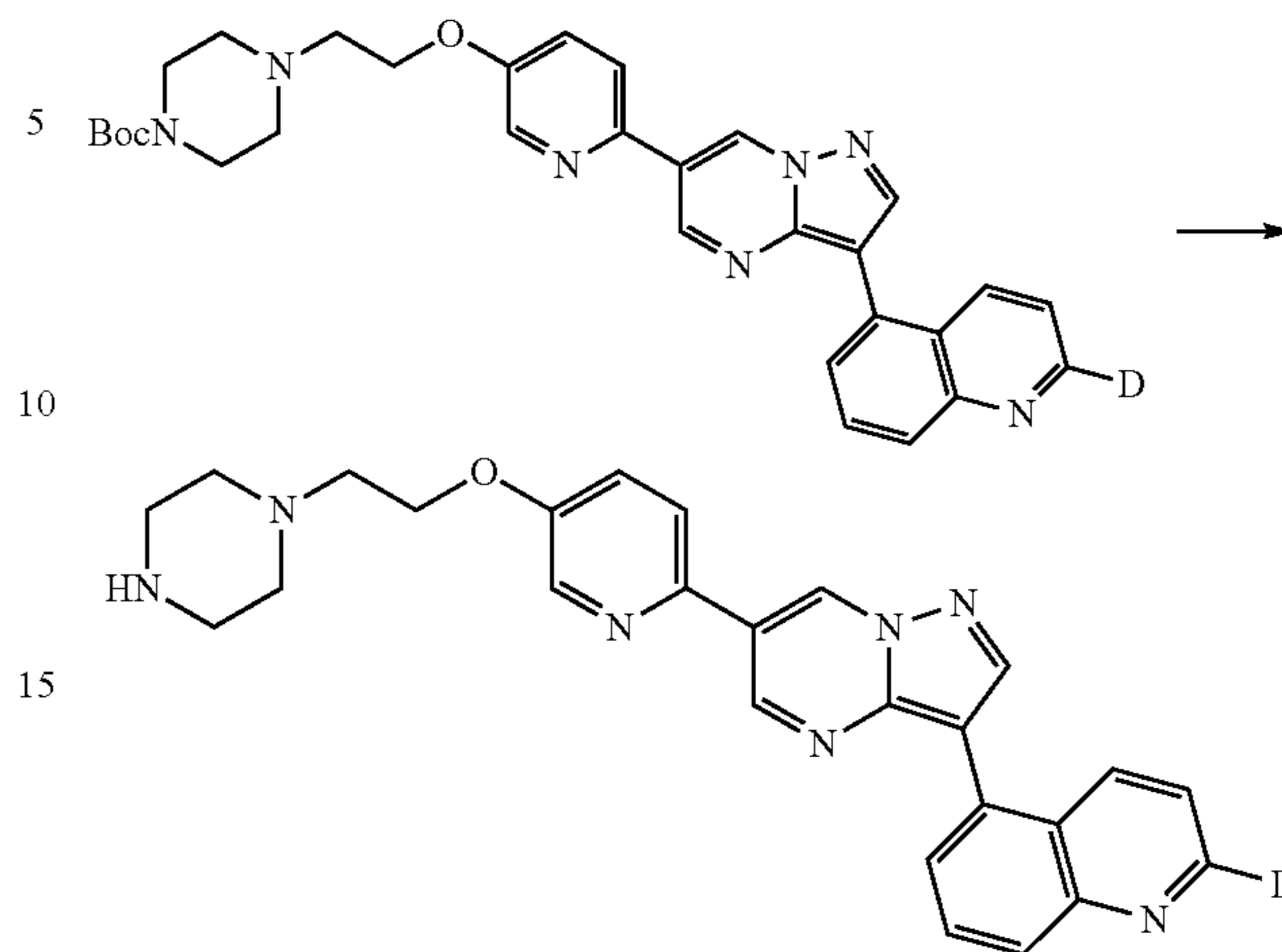
Scheme 176
