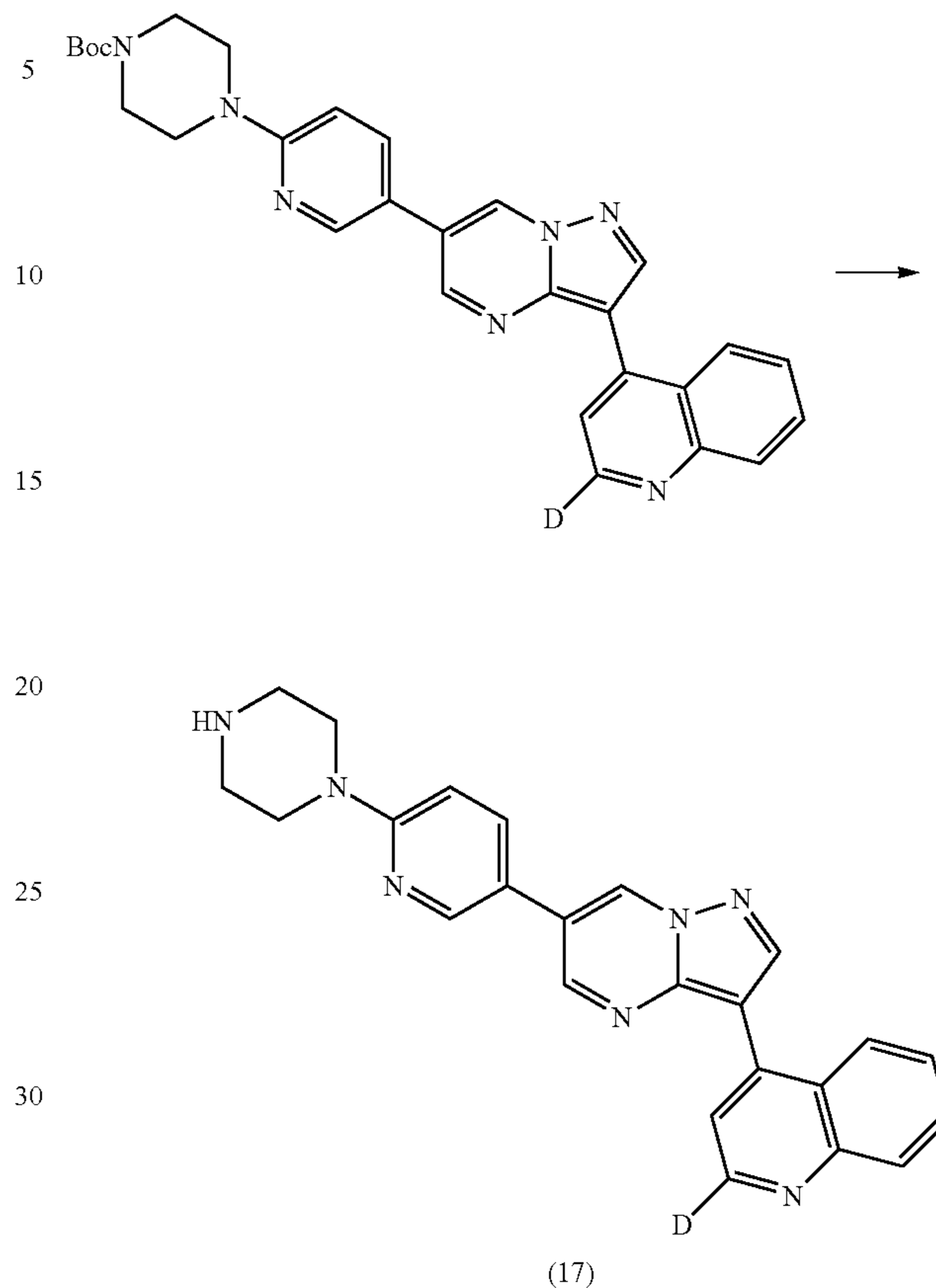
Scheme 51
