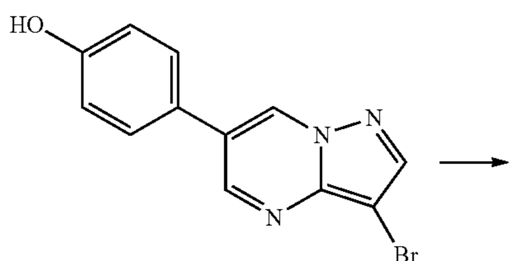
Scheme 103
