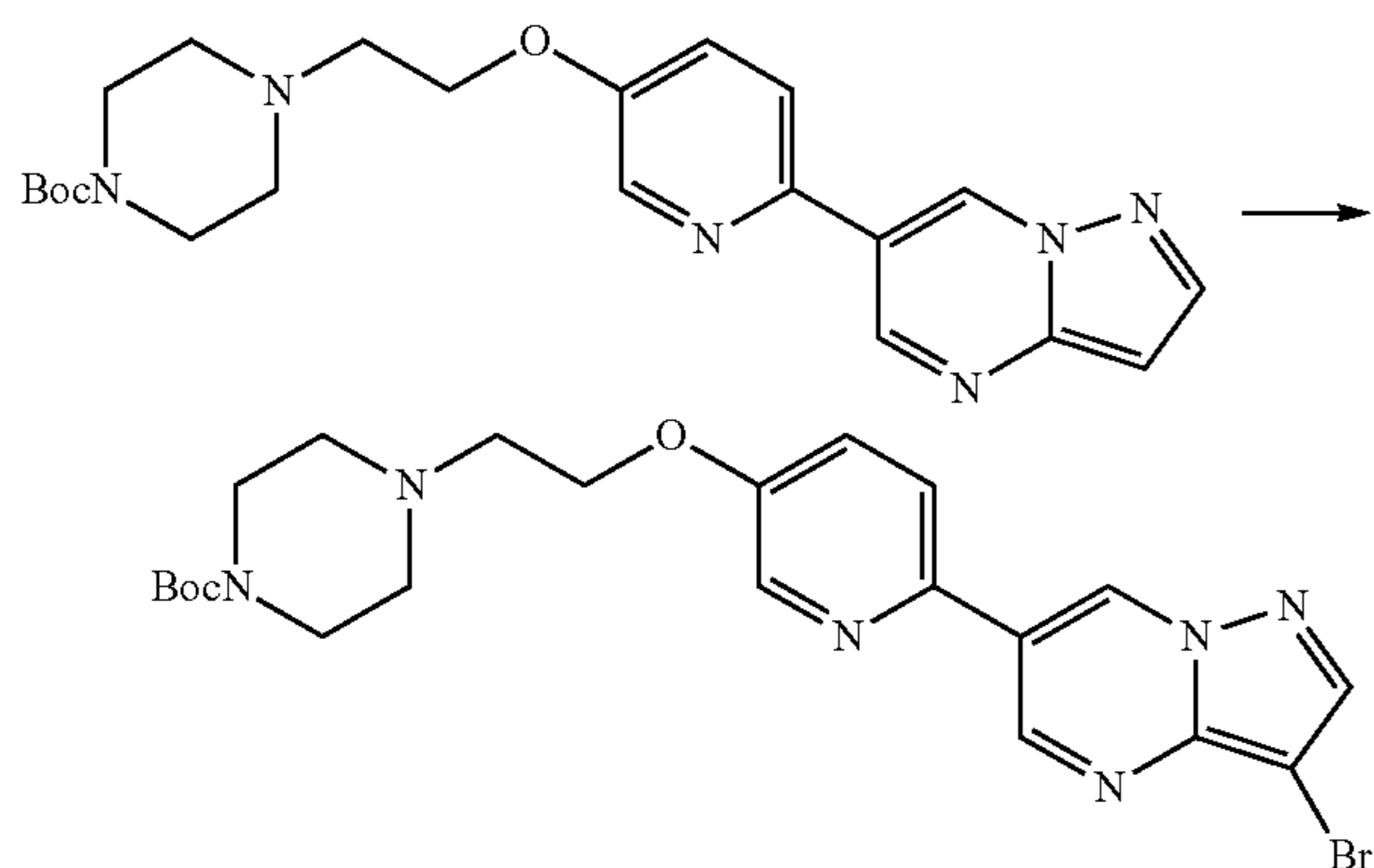
Scheme 174
