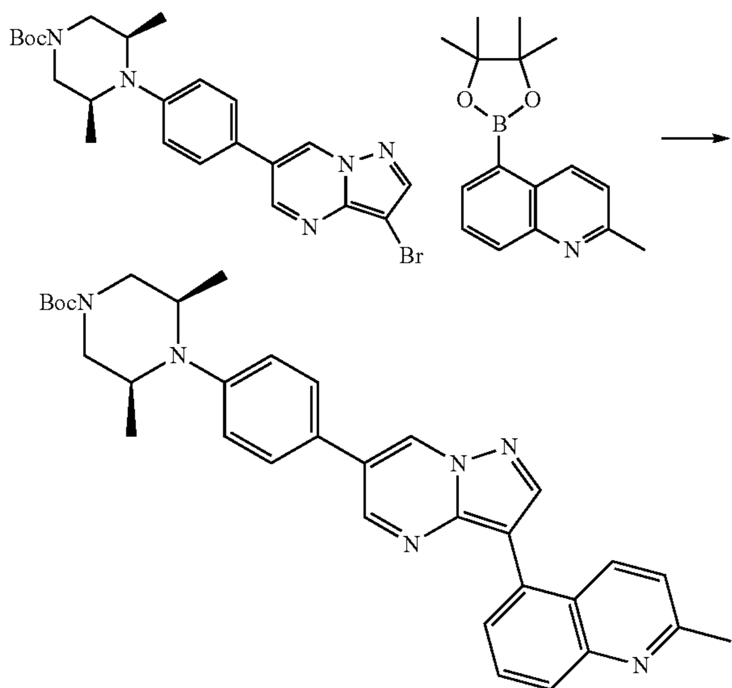
Scheme 184
