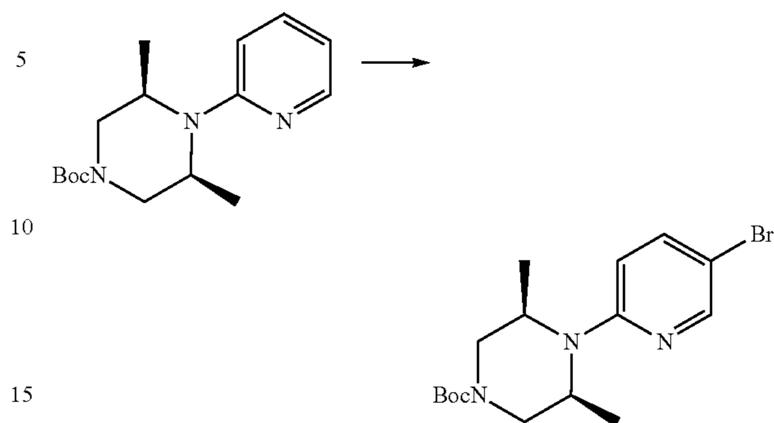
Scheme 114
