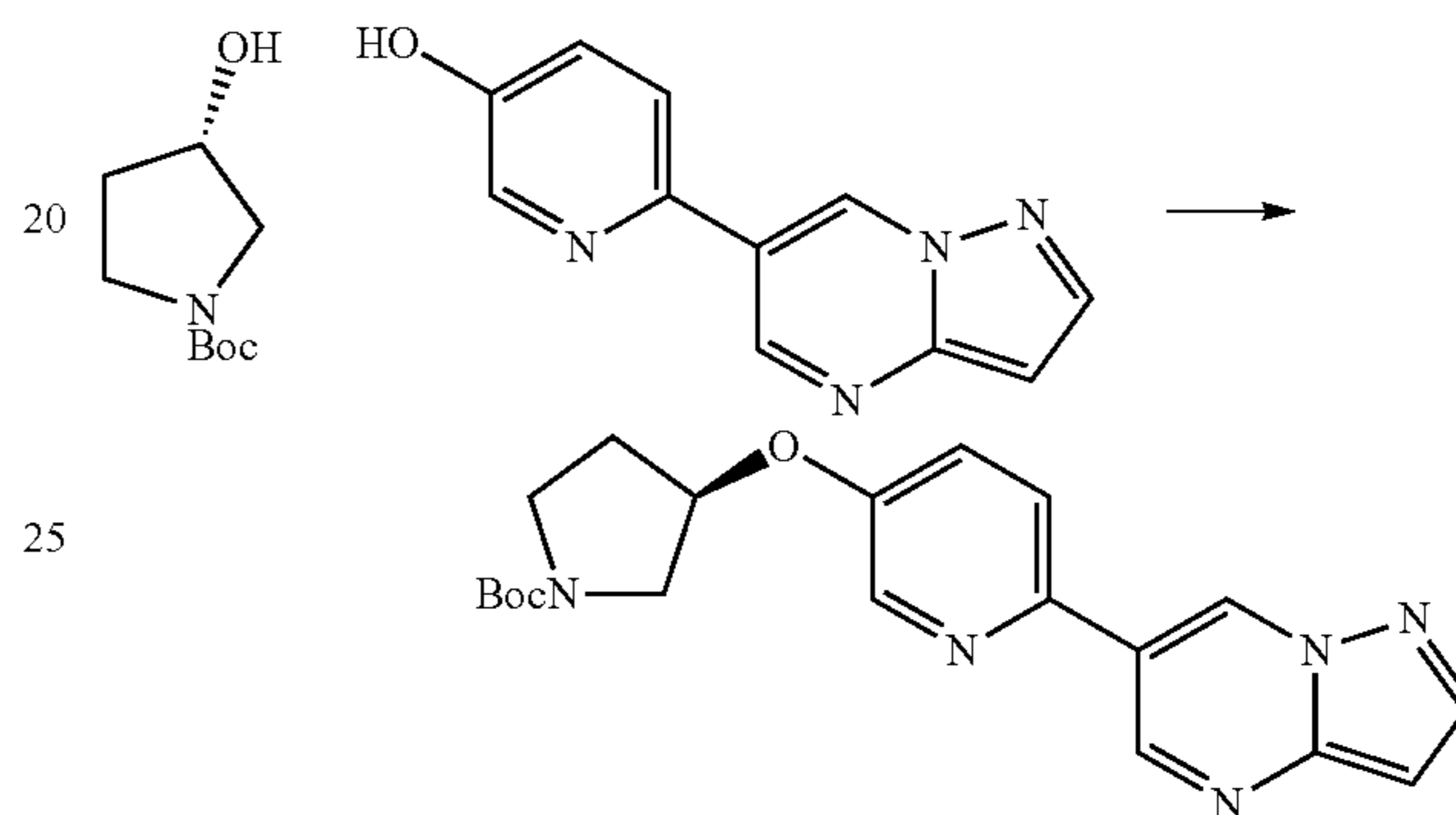
Scheme 204
