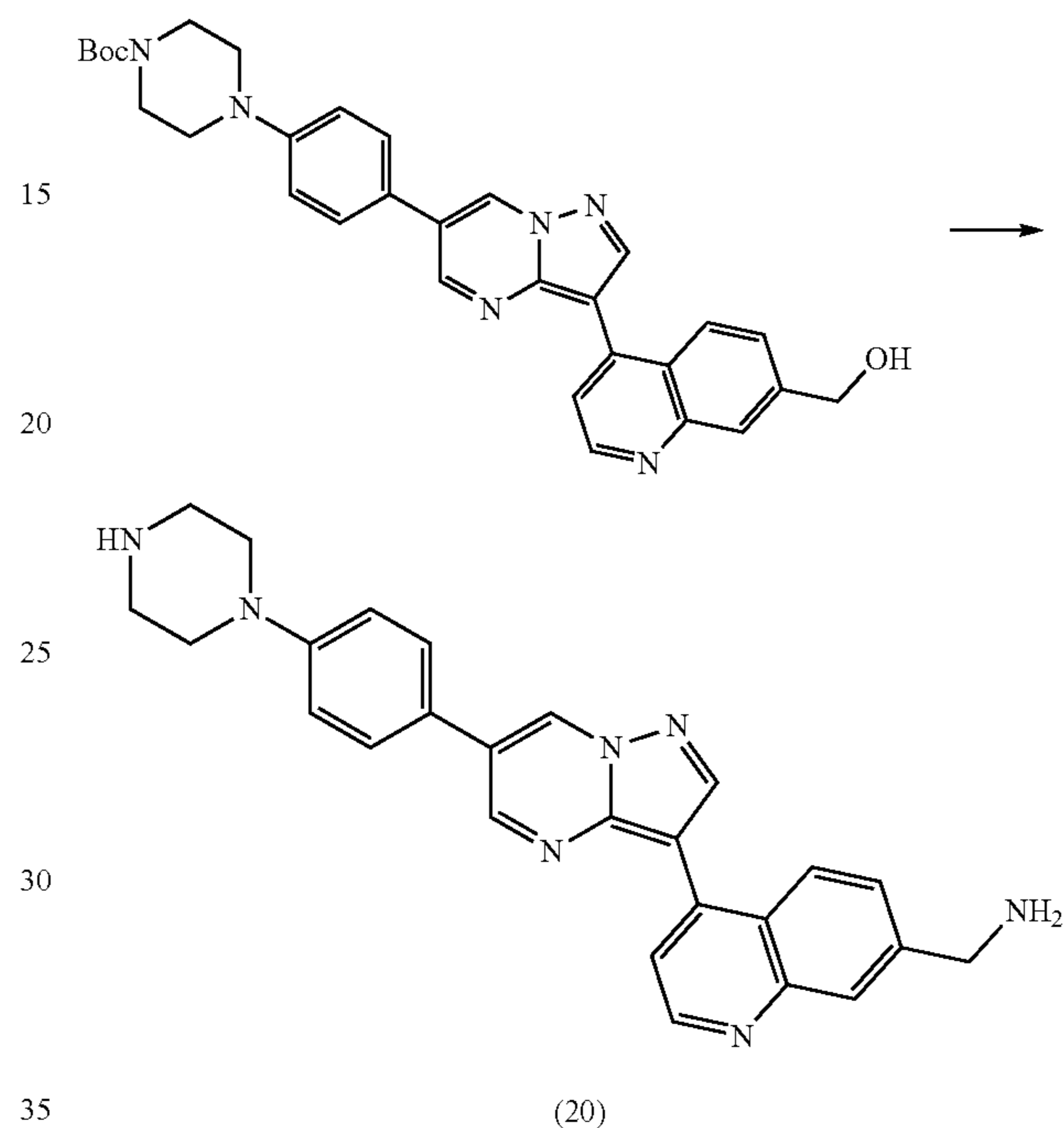
Scheme 66
