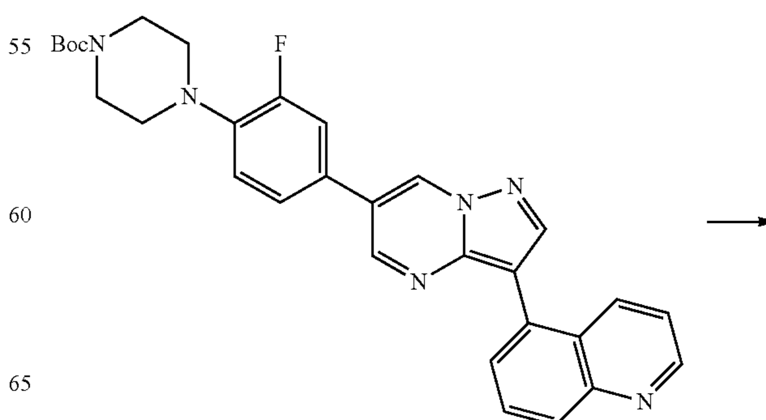
Scheme 148
