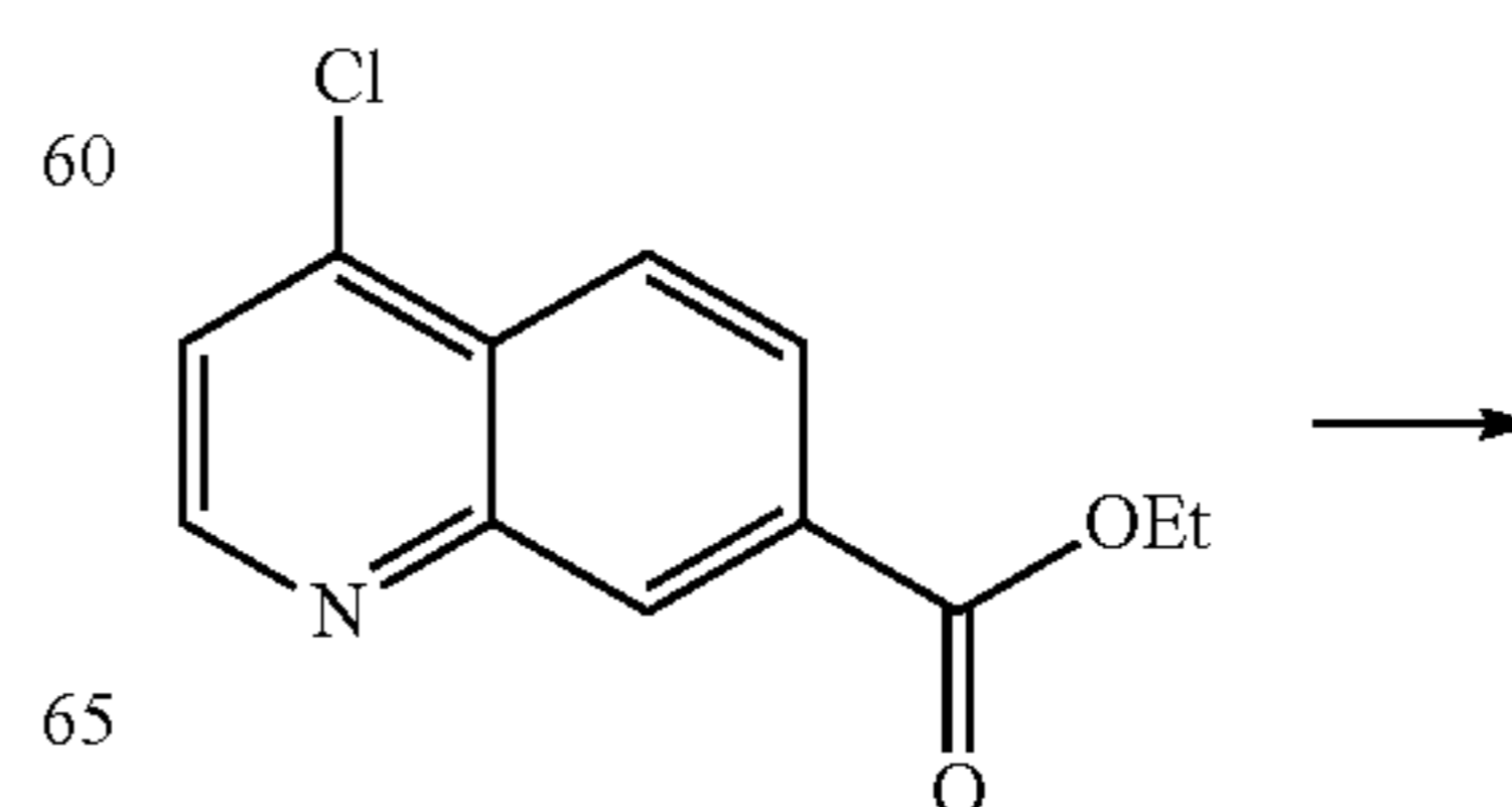
Scheme 55
