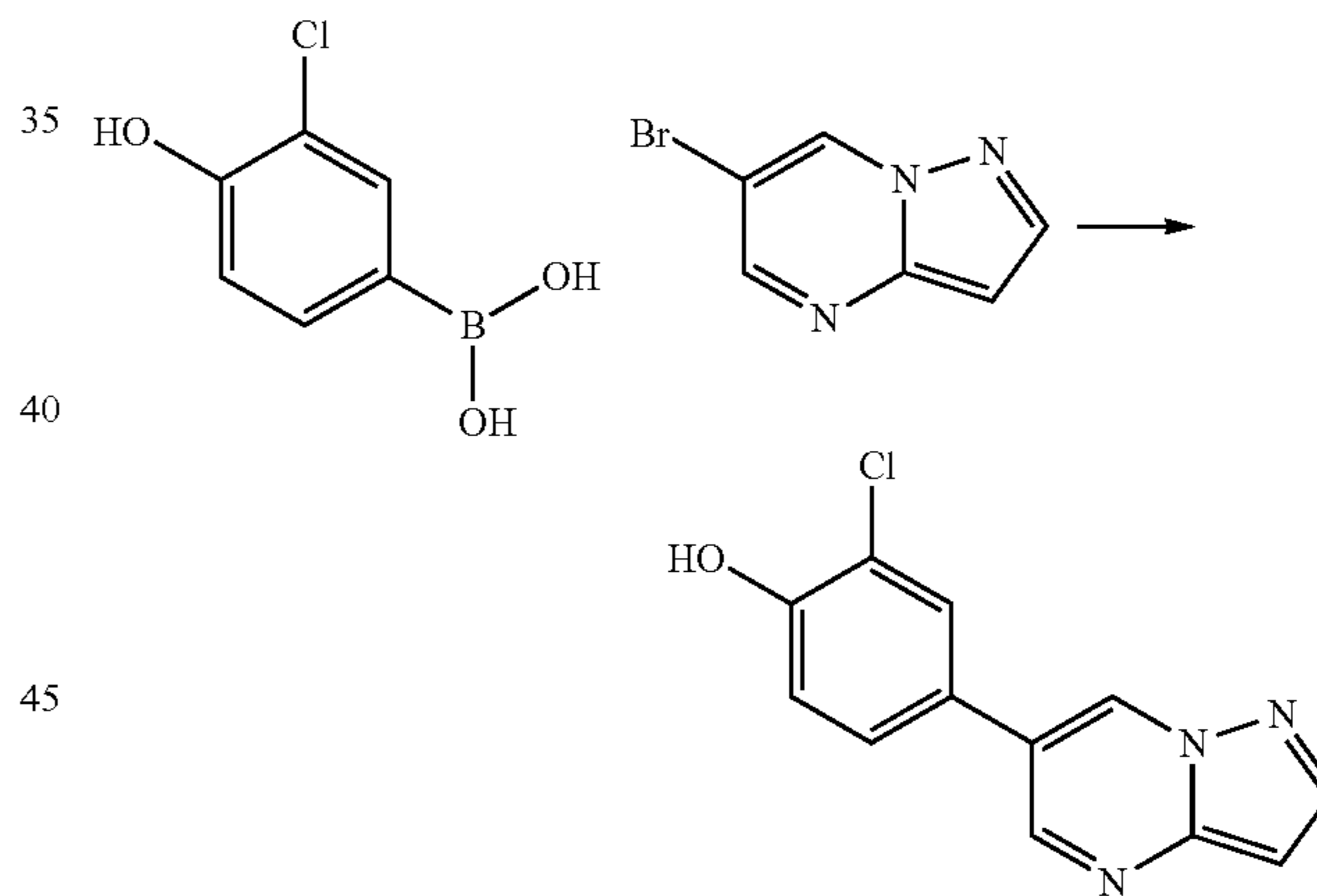
Scheme 159
