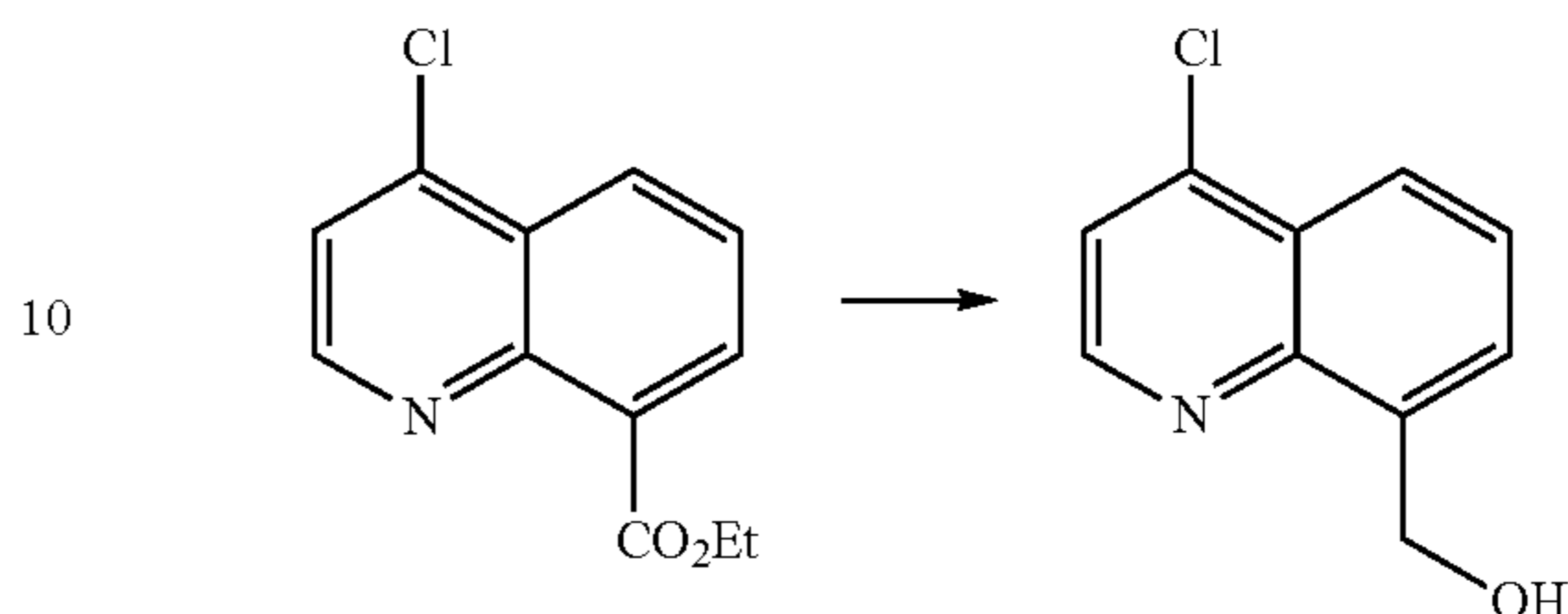
Scheme 77
