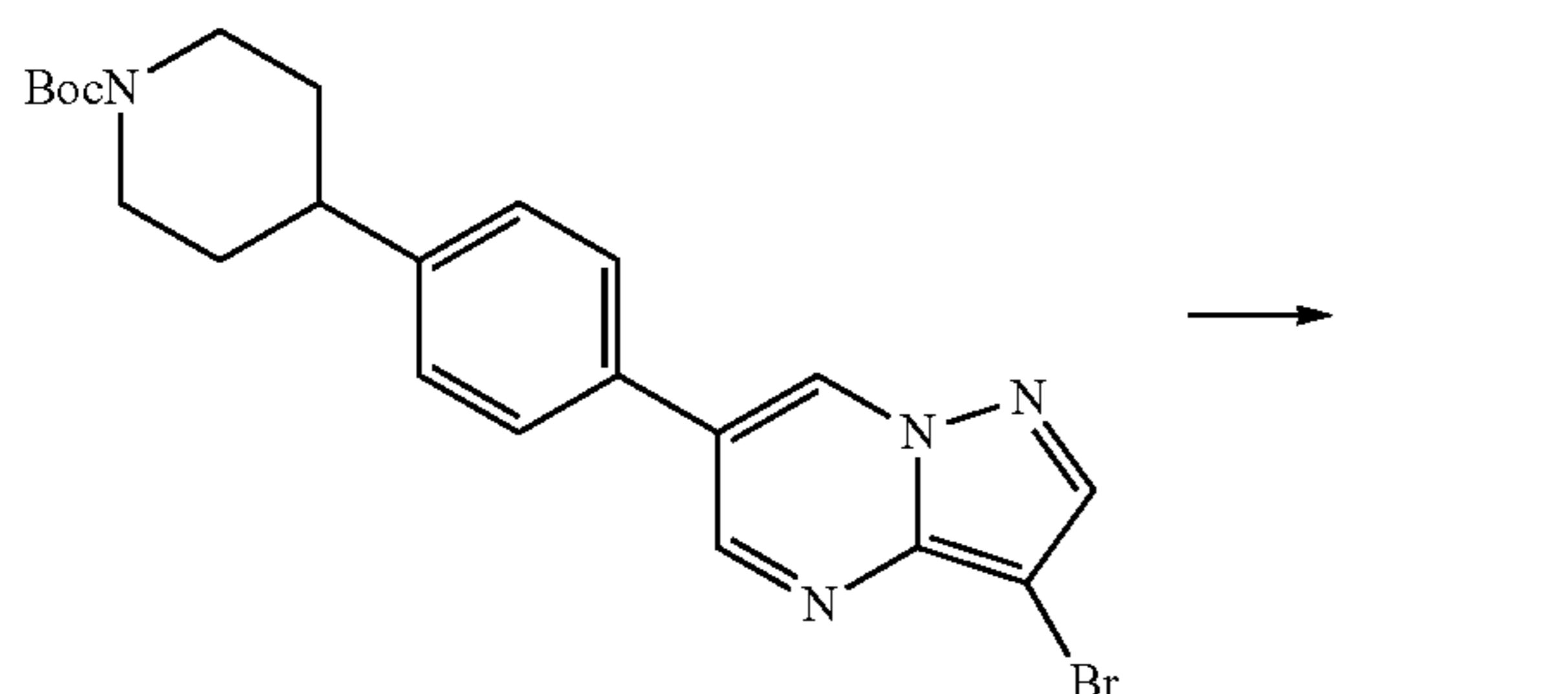
Scheme 44
