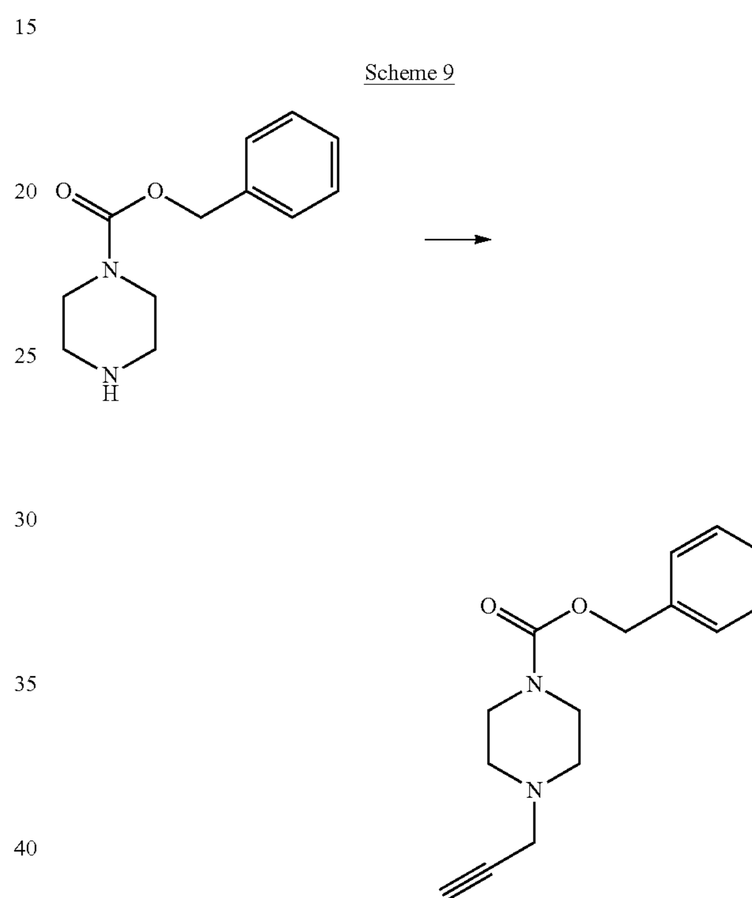
Compound 4
