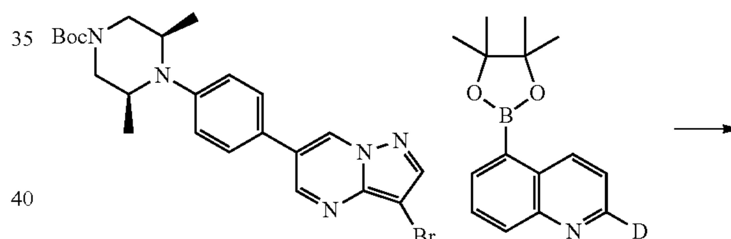
Scheme 182
