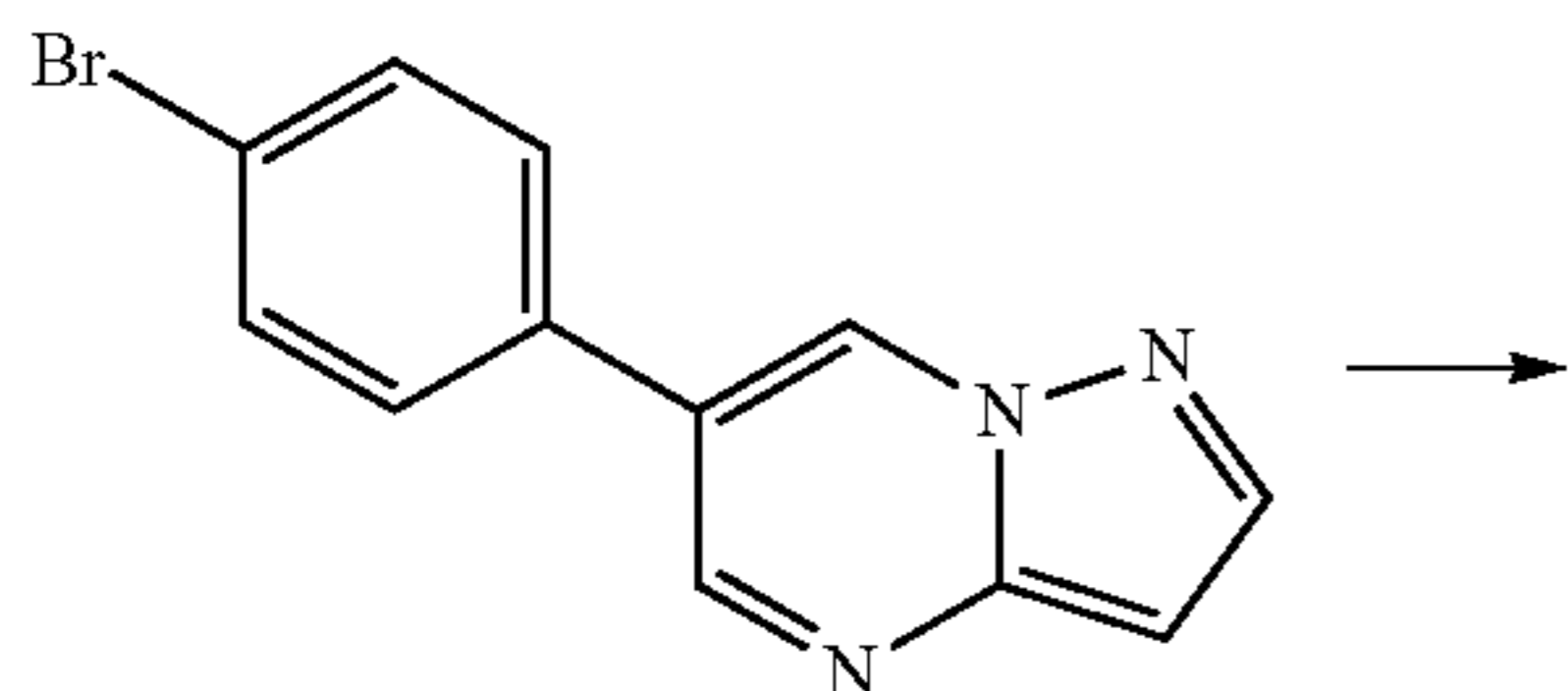
Scheme 3
