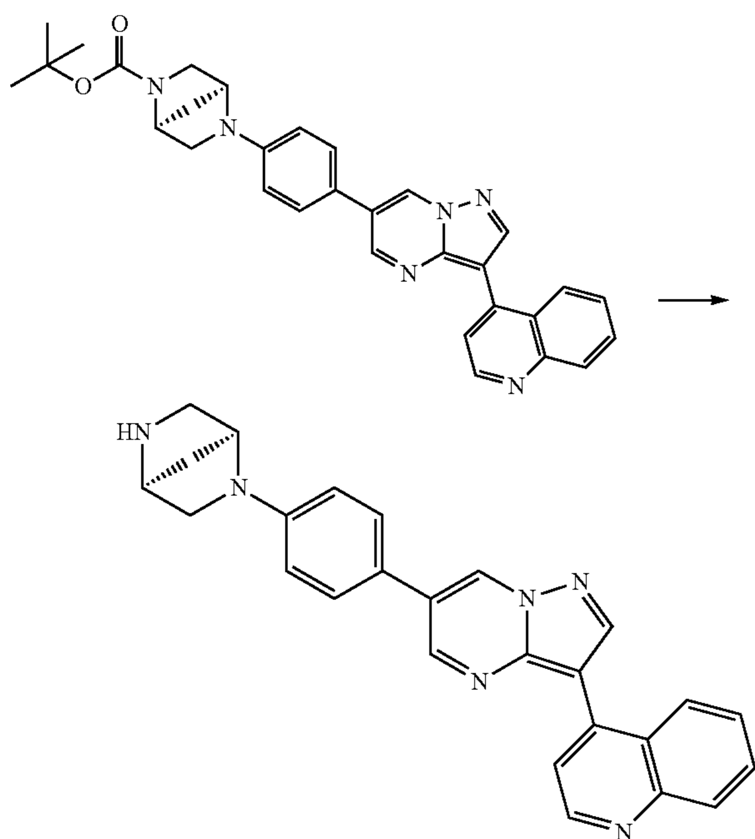
Scheme 17
