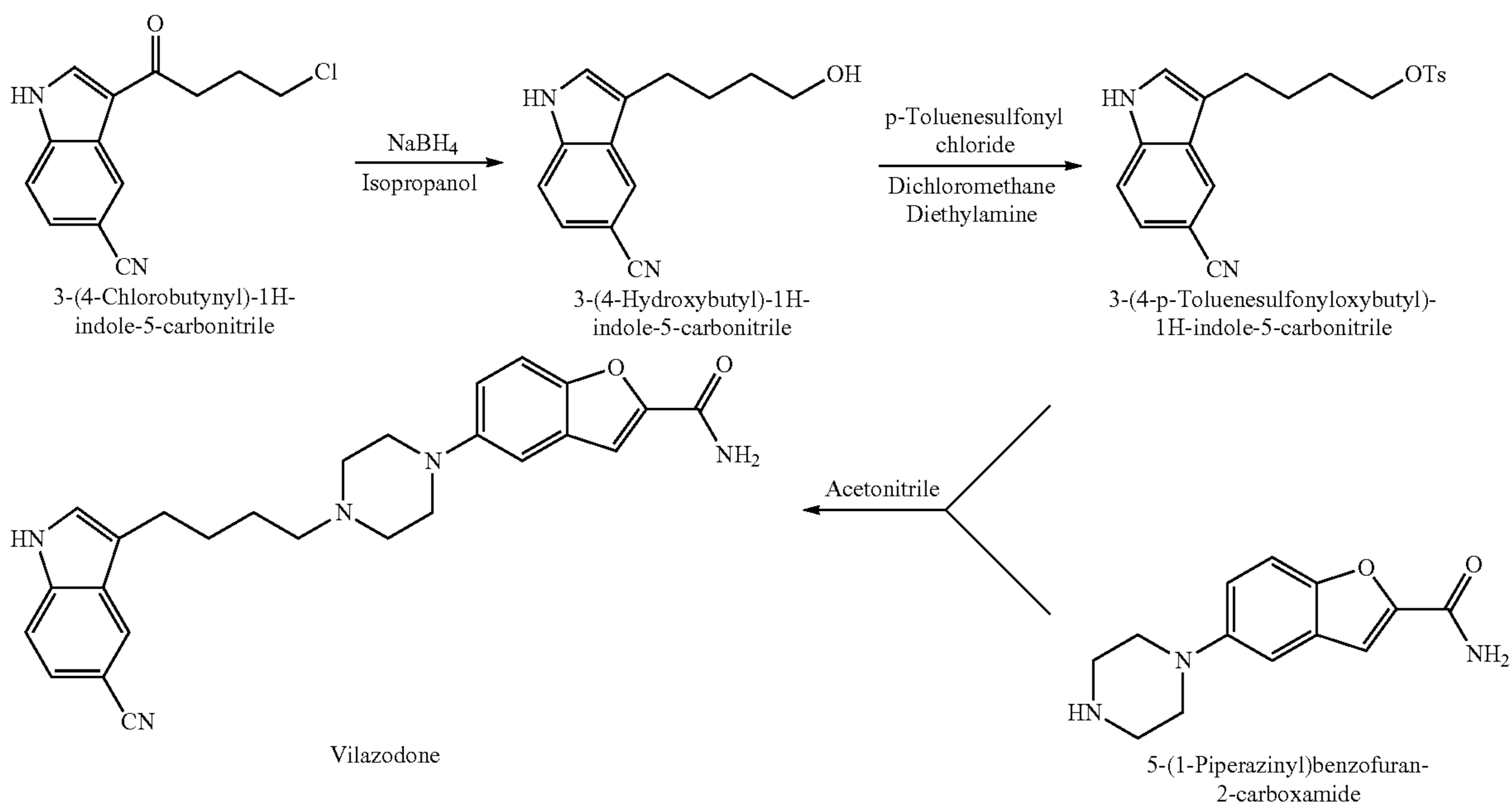
Scheme 4:
