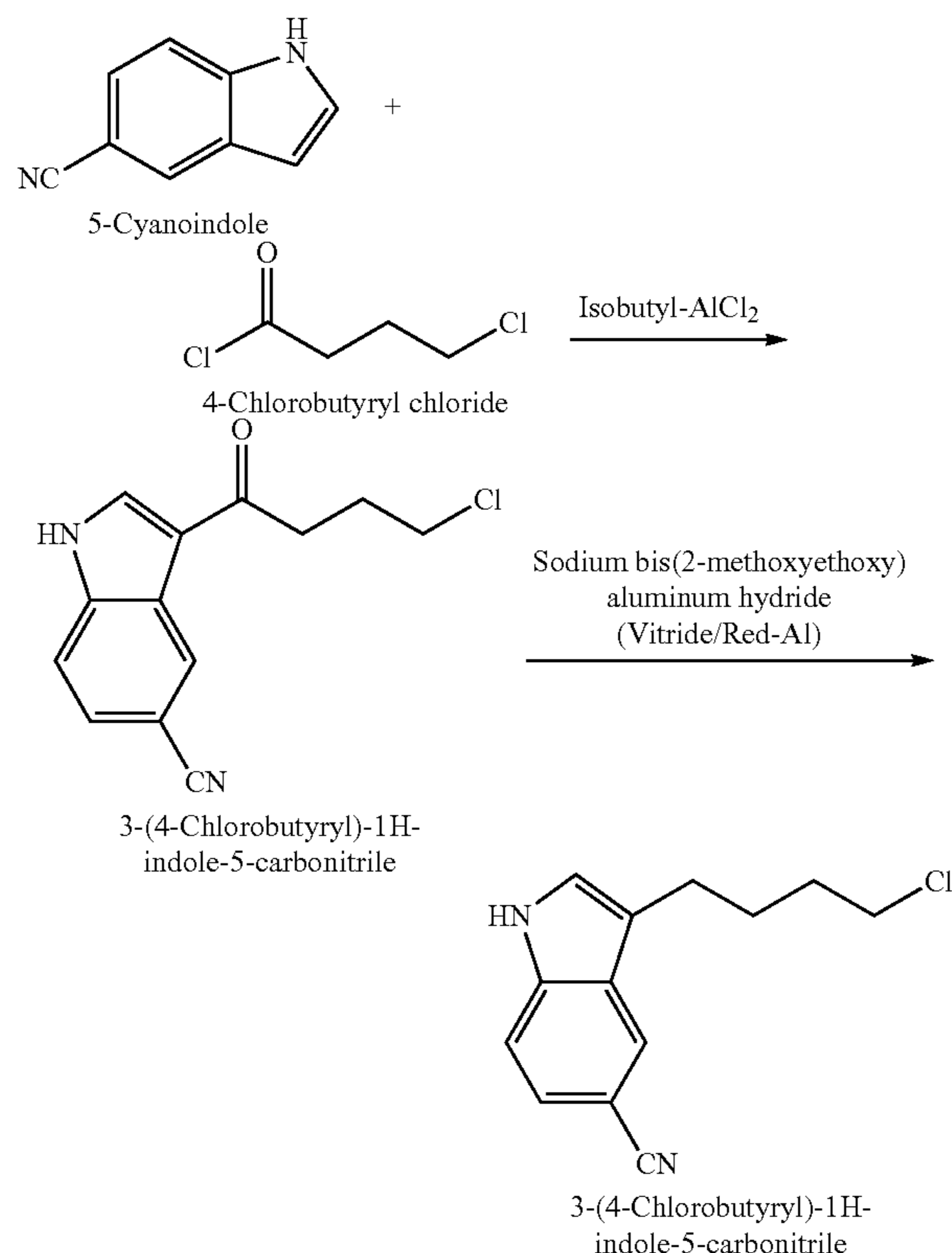
Scheme 2:
