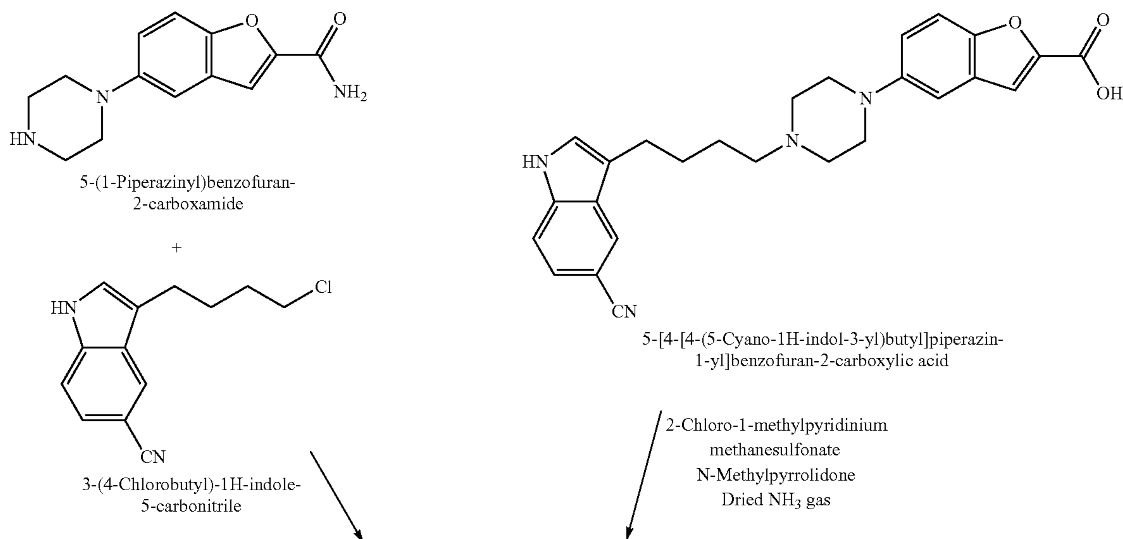
Scheme 1:
