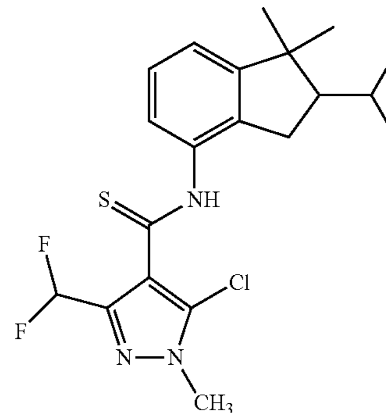
5-chloro-3-(difluoromethyl)-N-(2-isopropyl-1,1-dimethyl-2,3-dihydro-1H-inden-4-yl)-1-methyl-1H-pyrazole-4-carbothioamide (example 94)
