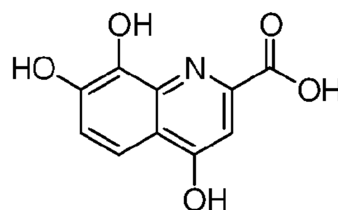
7,8-dihydroxykynurenic acid
