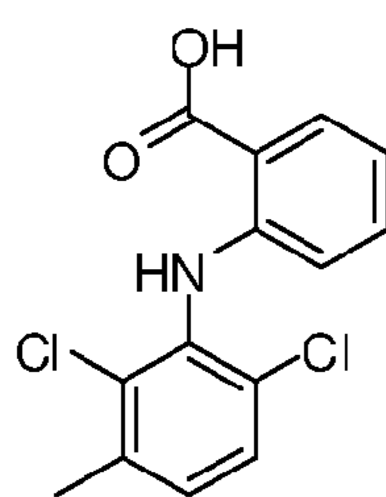
Meclofenamic acid
