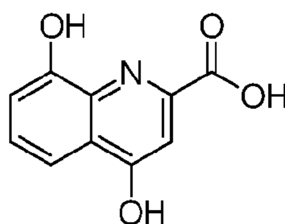
xanthurenic acid
