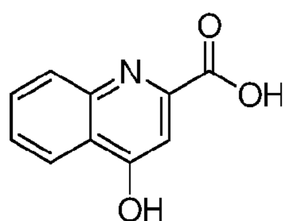
kynurenic acid
