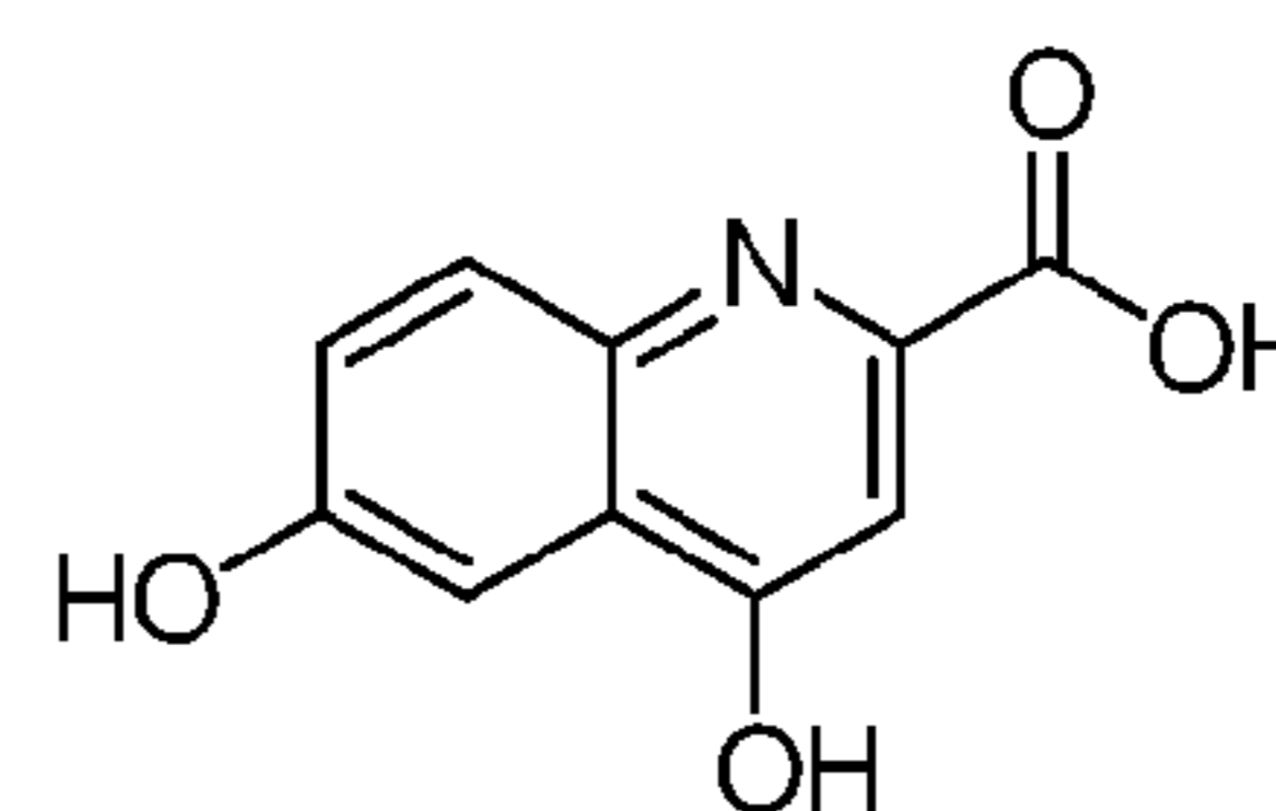
6-hydroxykynurenic acid
