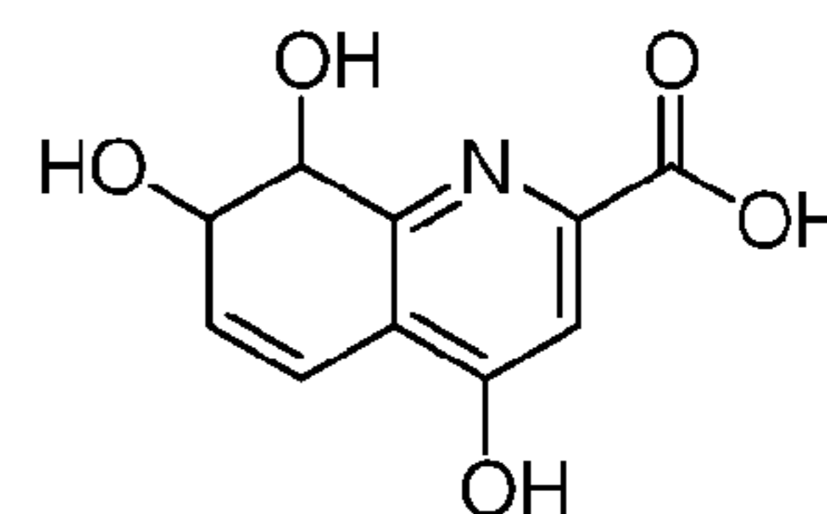
7,8-dihydro-7,8-dihydroxykynurenic acid
