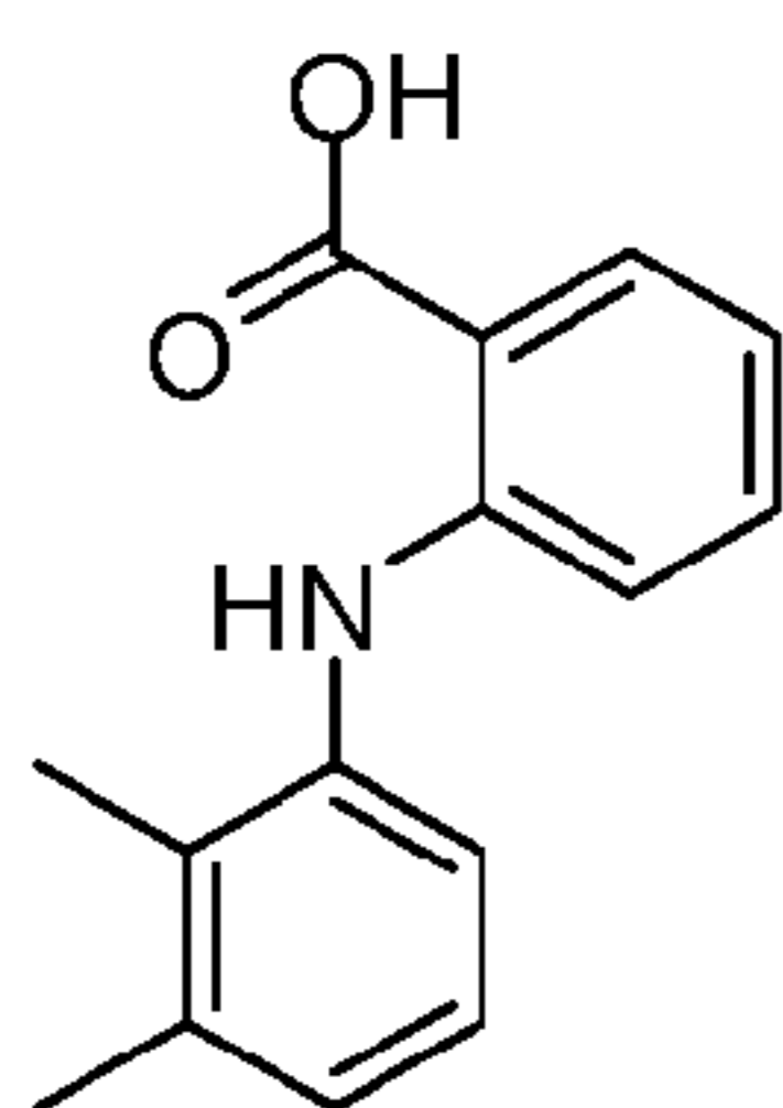
Mefenamic acid
