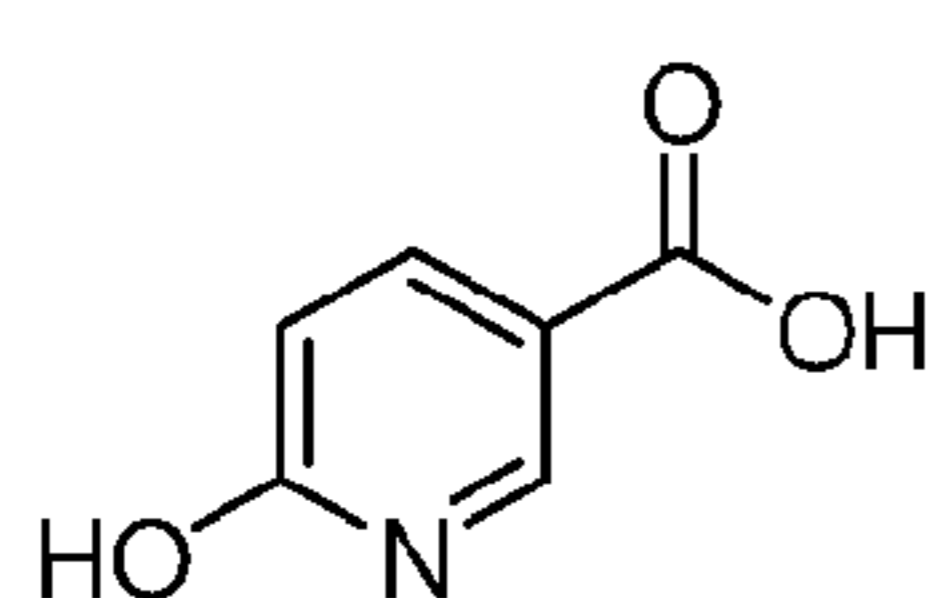
6-hydroxynicotinic acid
