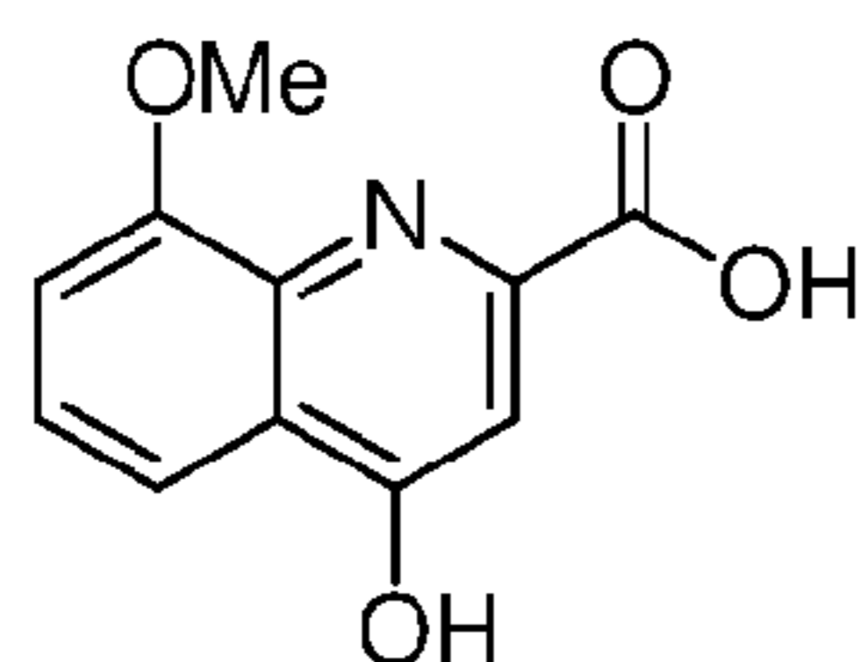
8-methoxykynurenic acid
