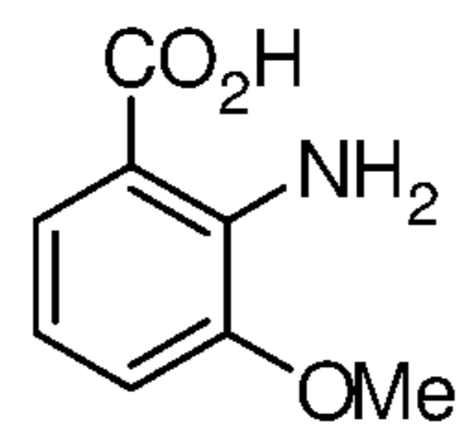
3-methoxyanthranilic acid
