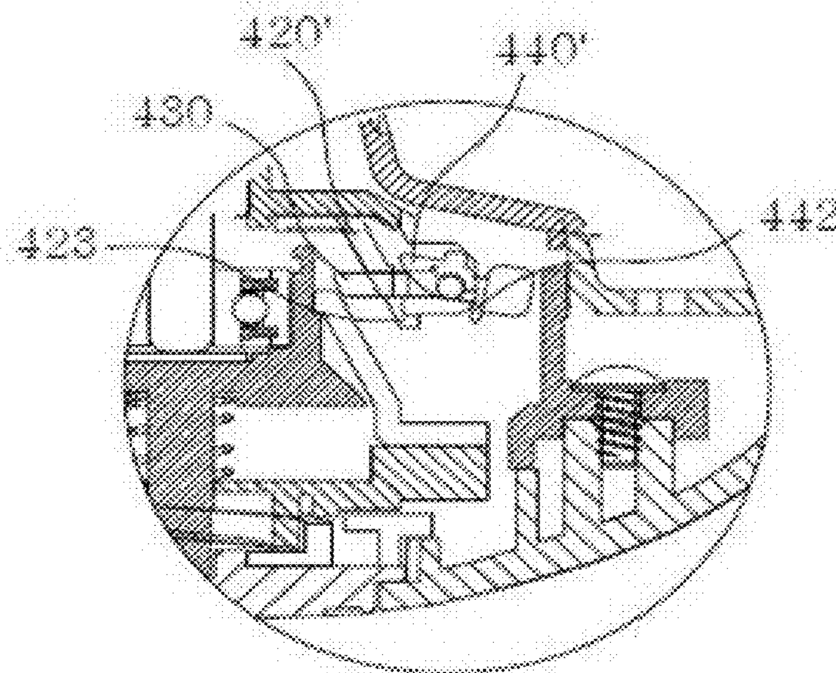
BRAKE SHOE OPERATING (ON) STATE
