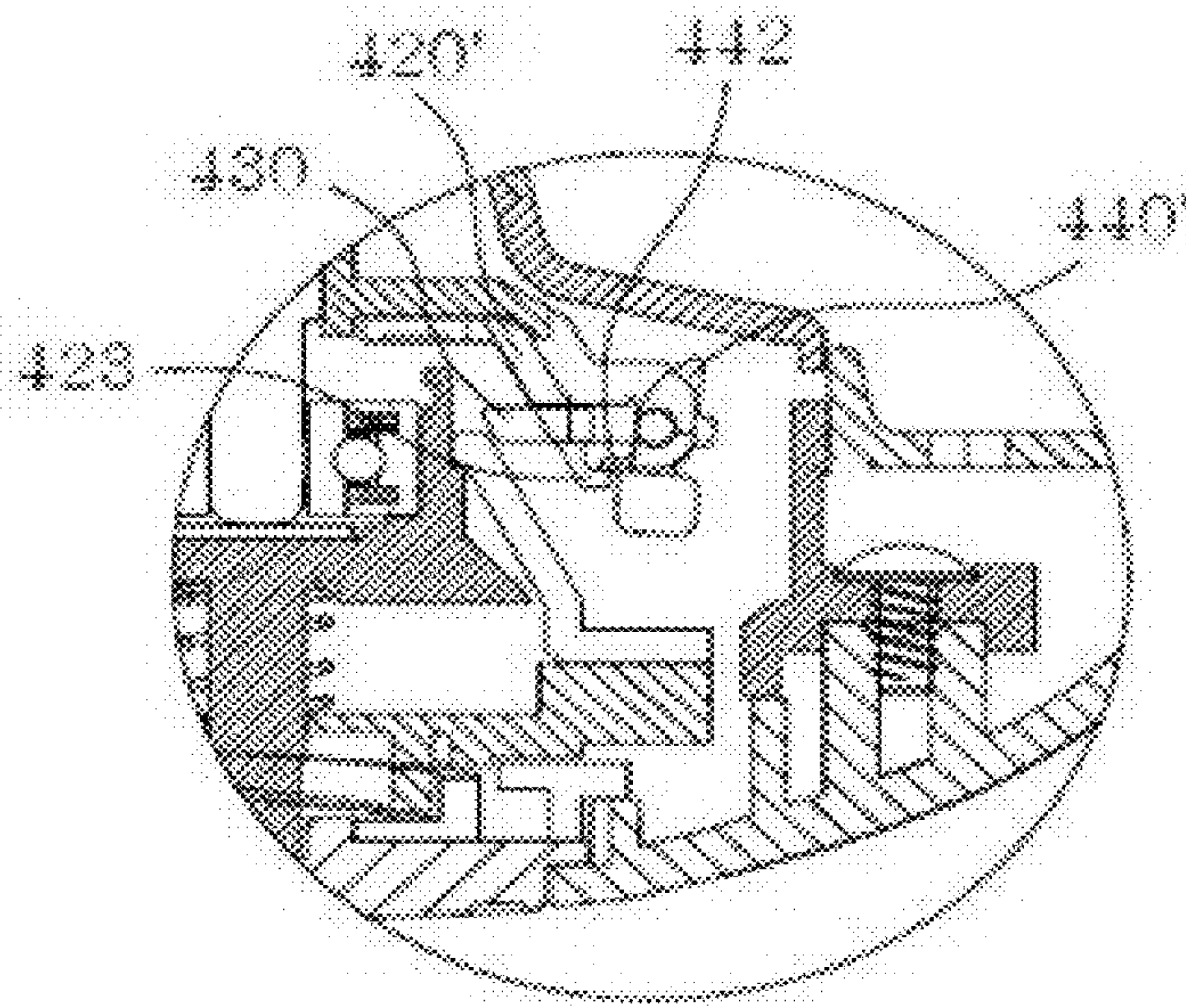
BRAKE SHOE NON-OPERATING (OFF) STATE
