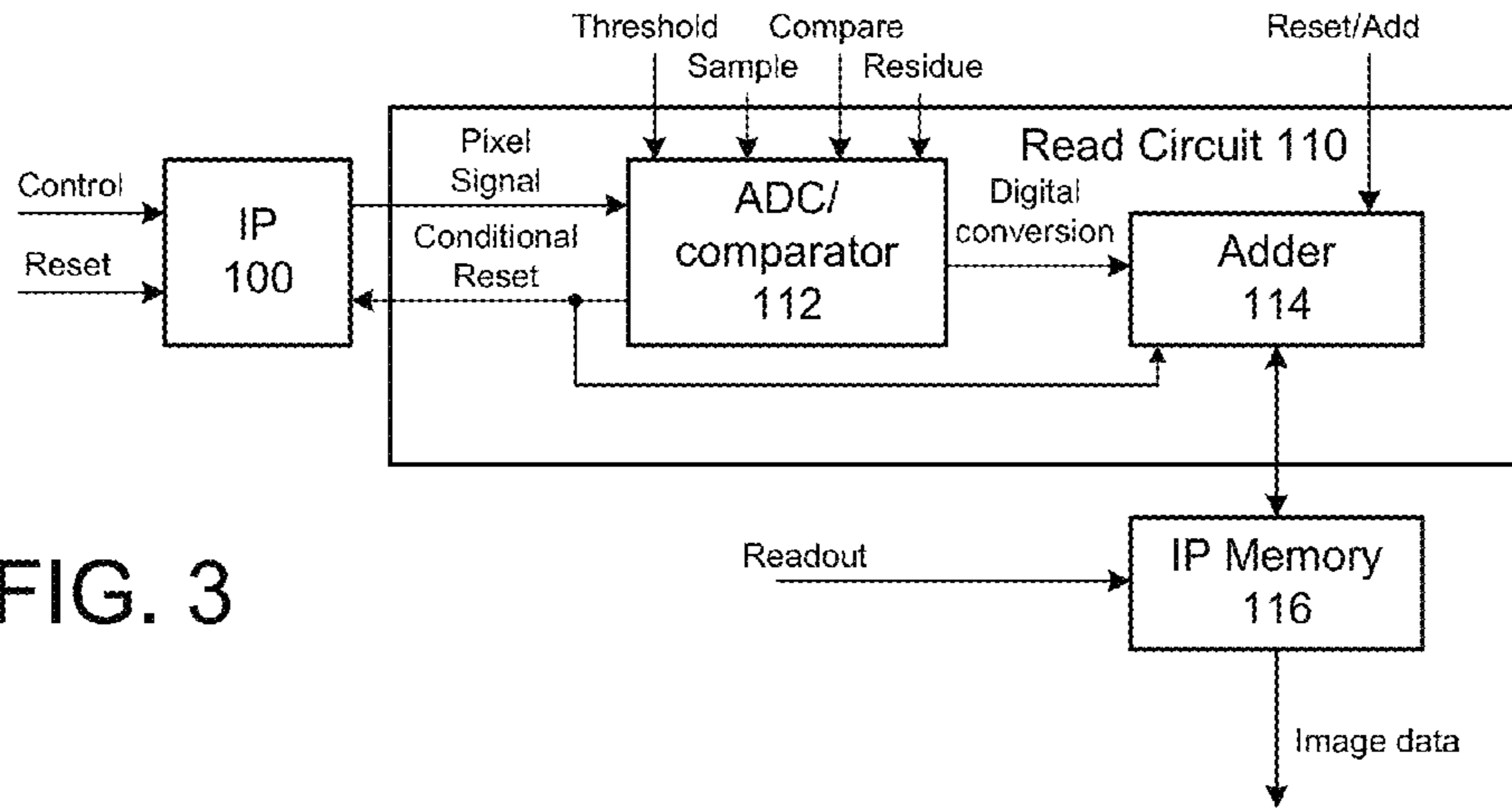
Image Sensor System 120
