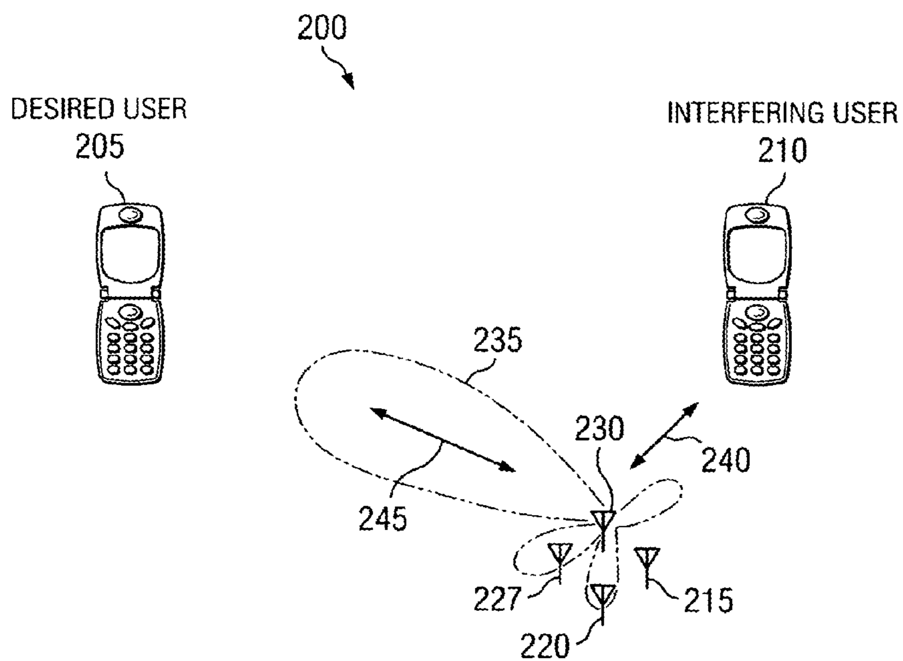
FIG. 2 (PRIOR ART)
