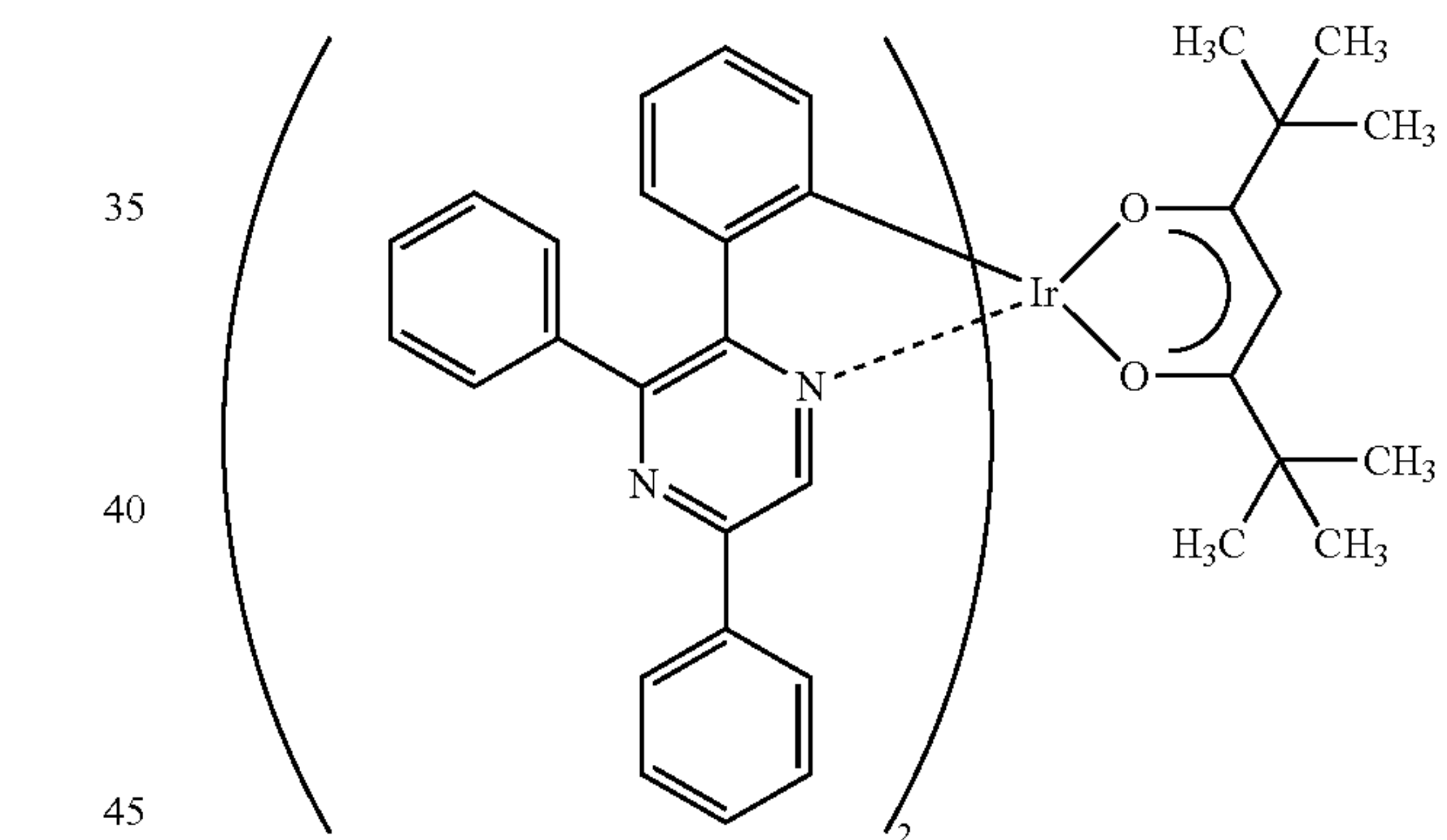
Ir(tppr) 2 (dpm)
