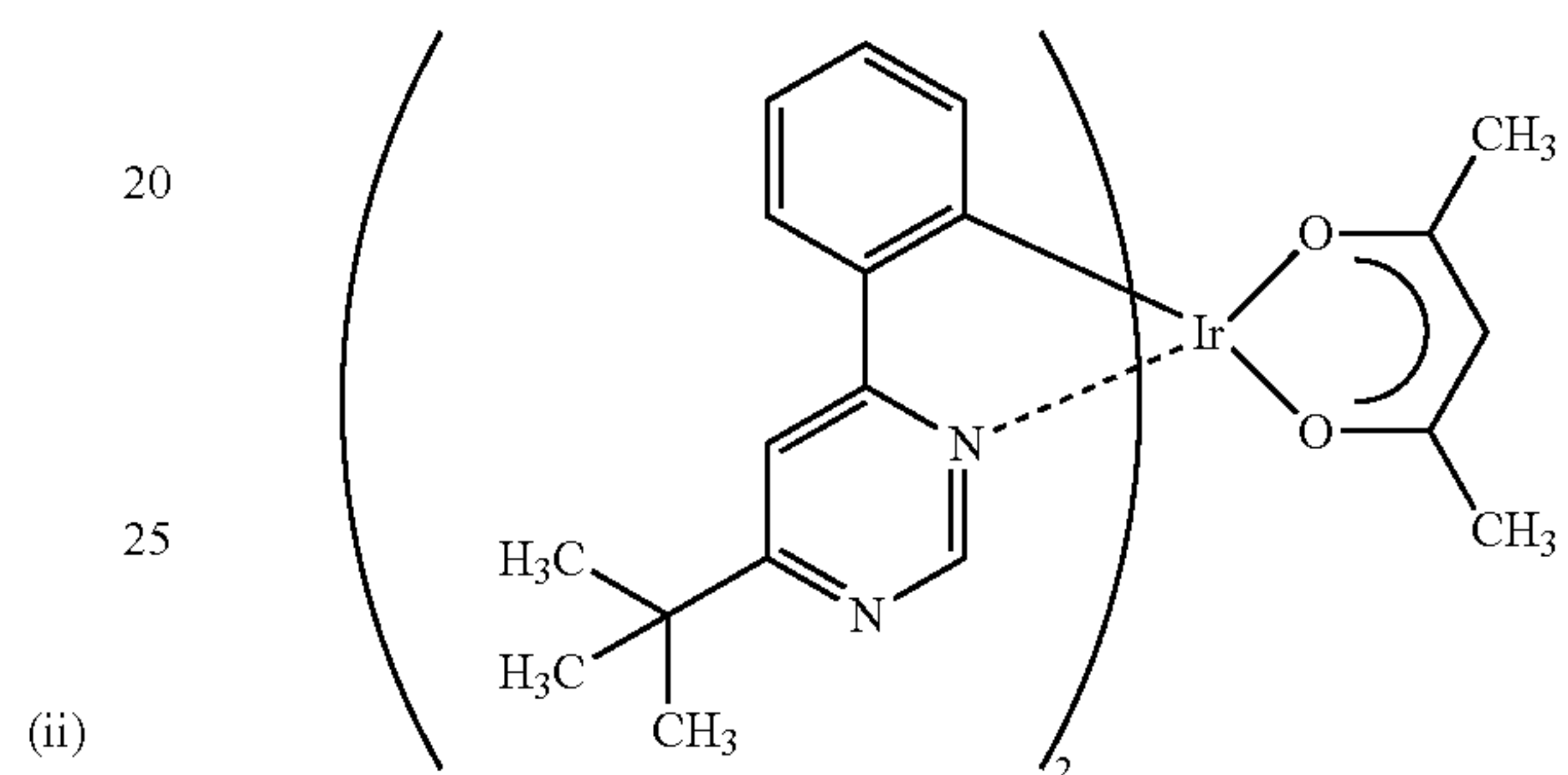
Ir(tBuppm) 2 (acac)
