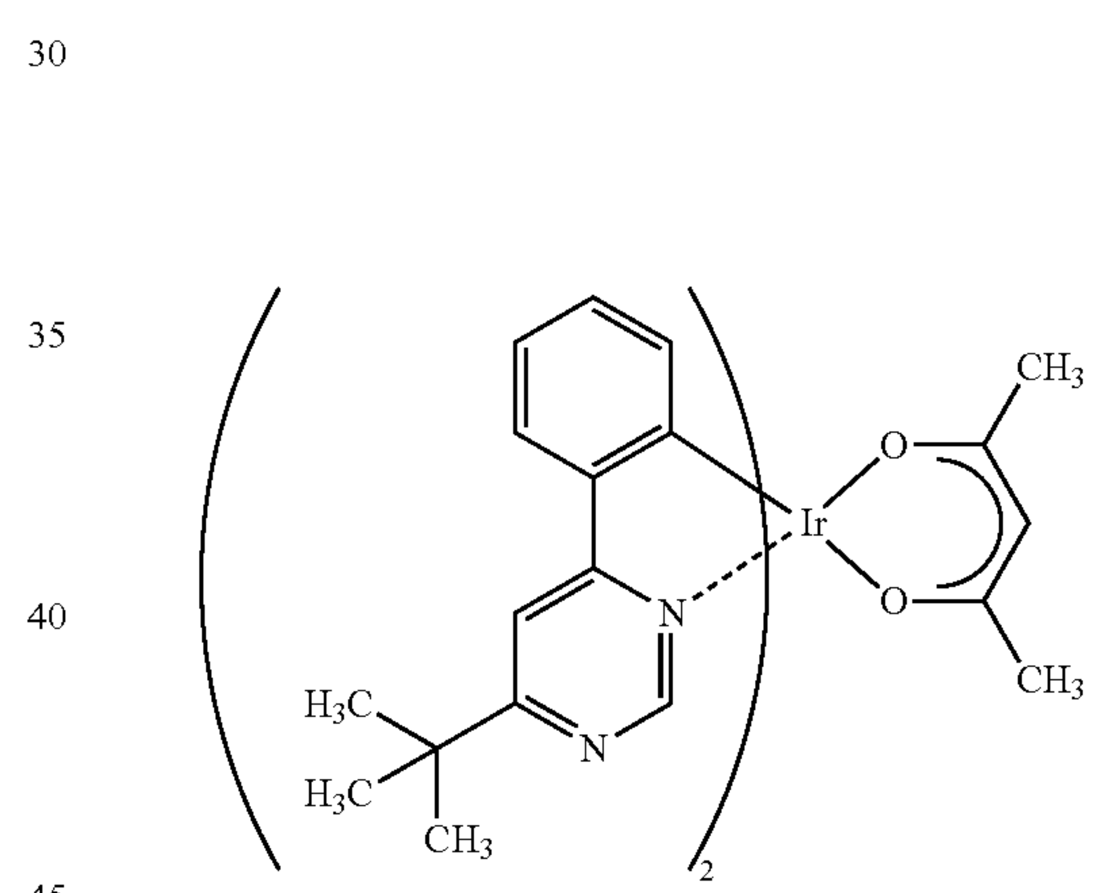
Ir(tBuppm) 2 (acac)
