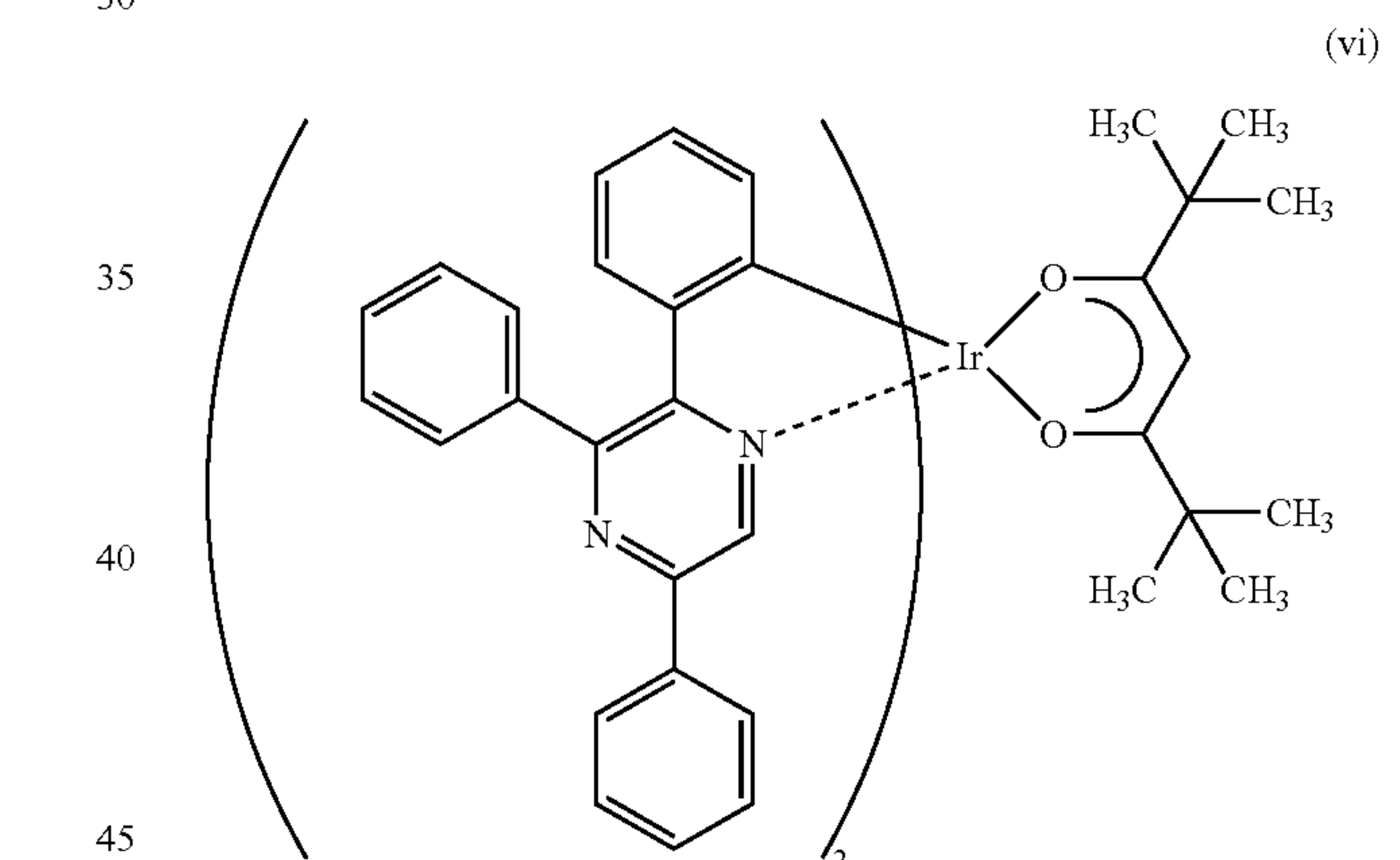
Ir(tppr) 2 (dpm)
