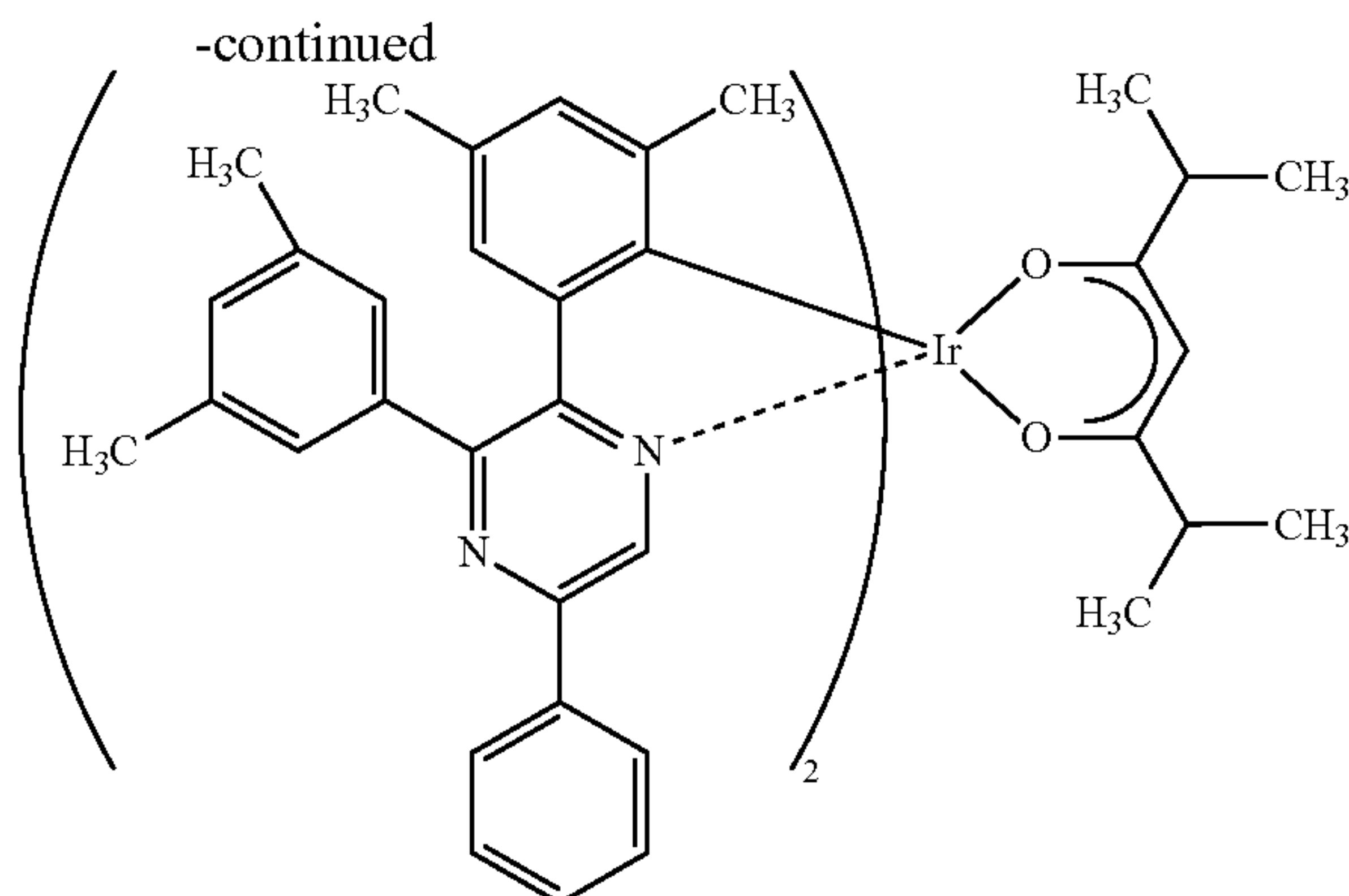
[Ir(dmdppr-P) 2 (dibm)]
