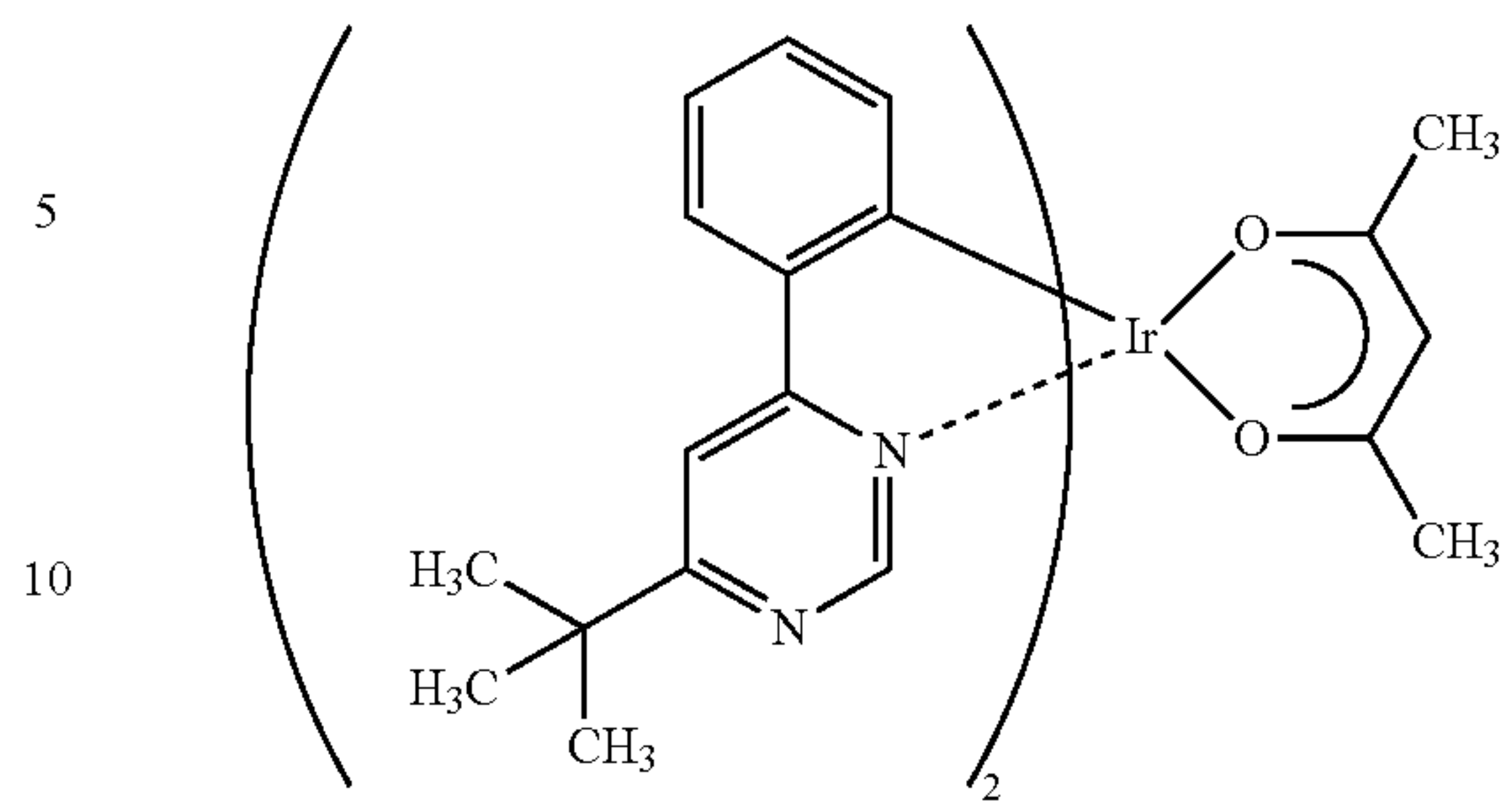
Ir(tBuppm) 2 (acac)
