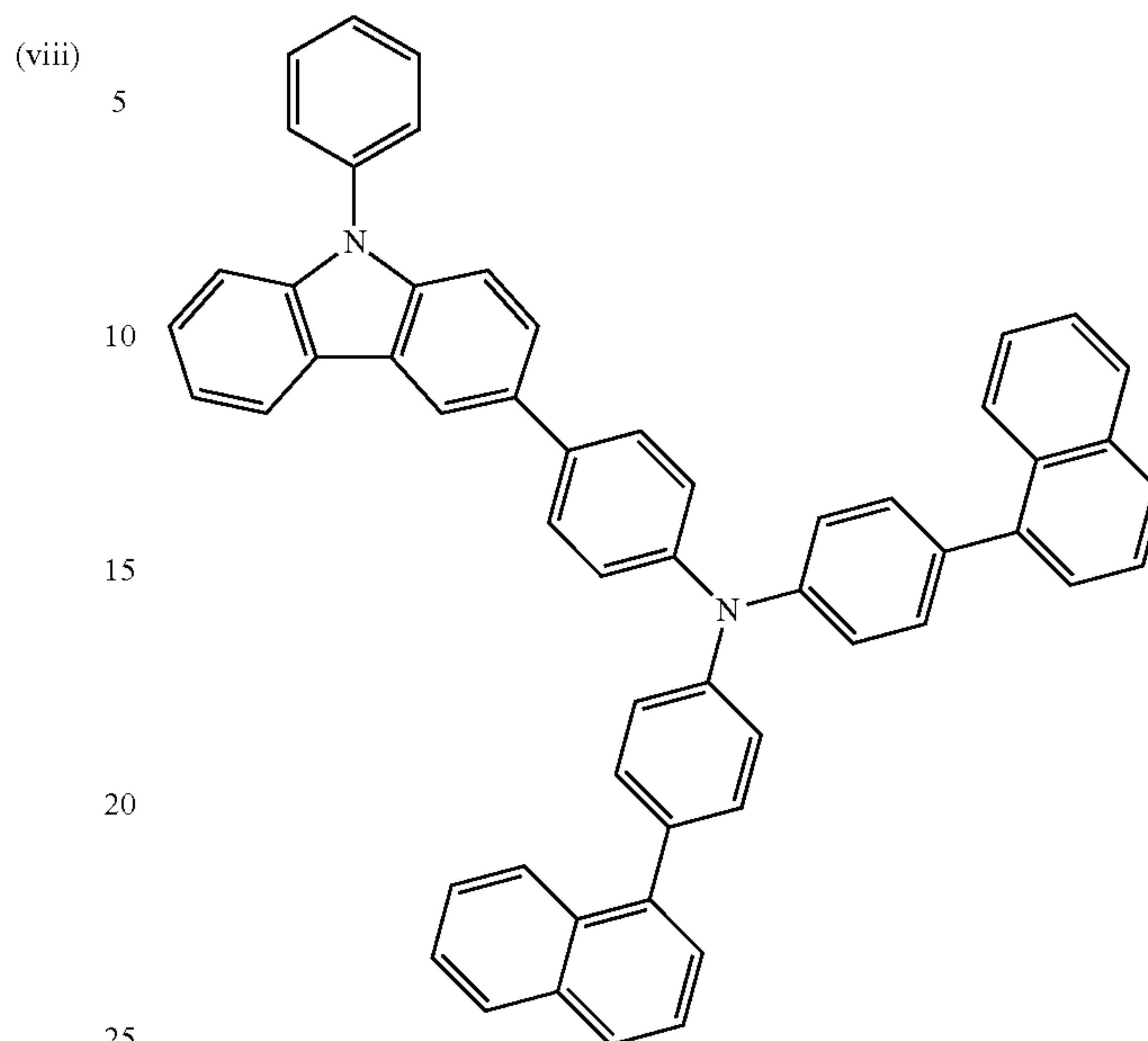
PCBNBB
