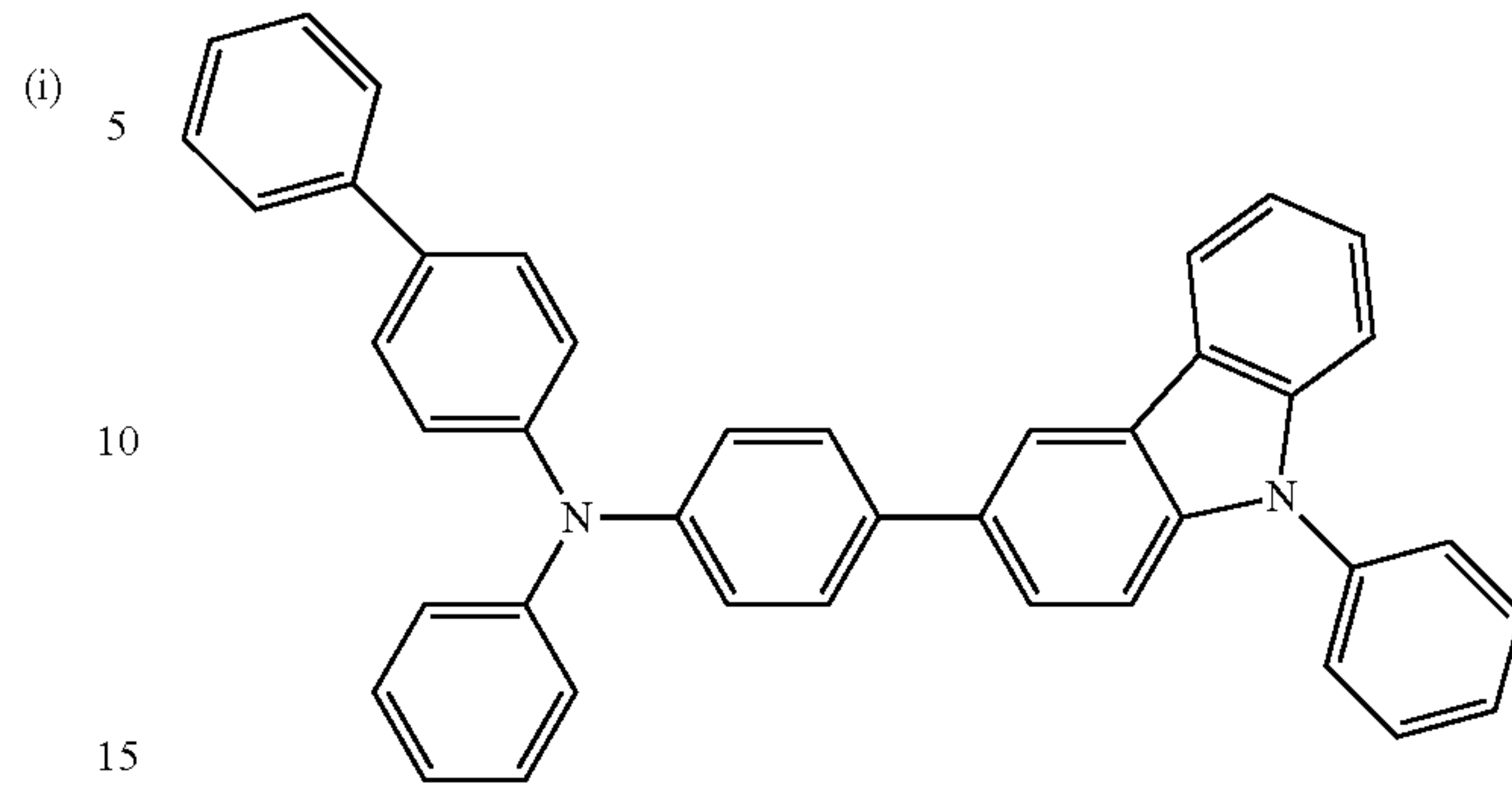
PCBA1BP
