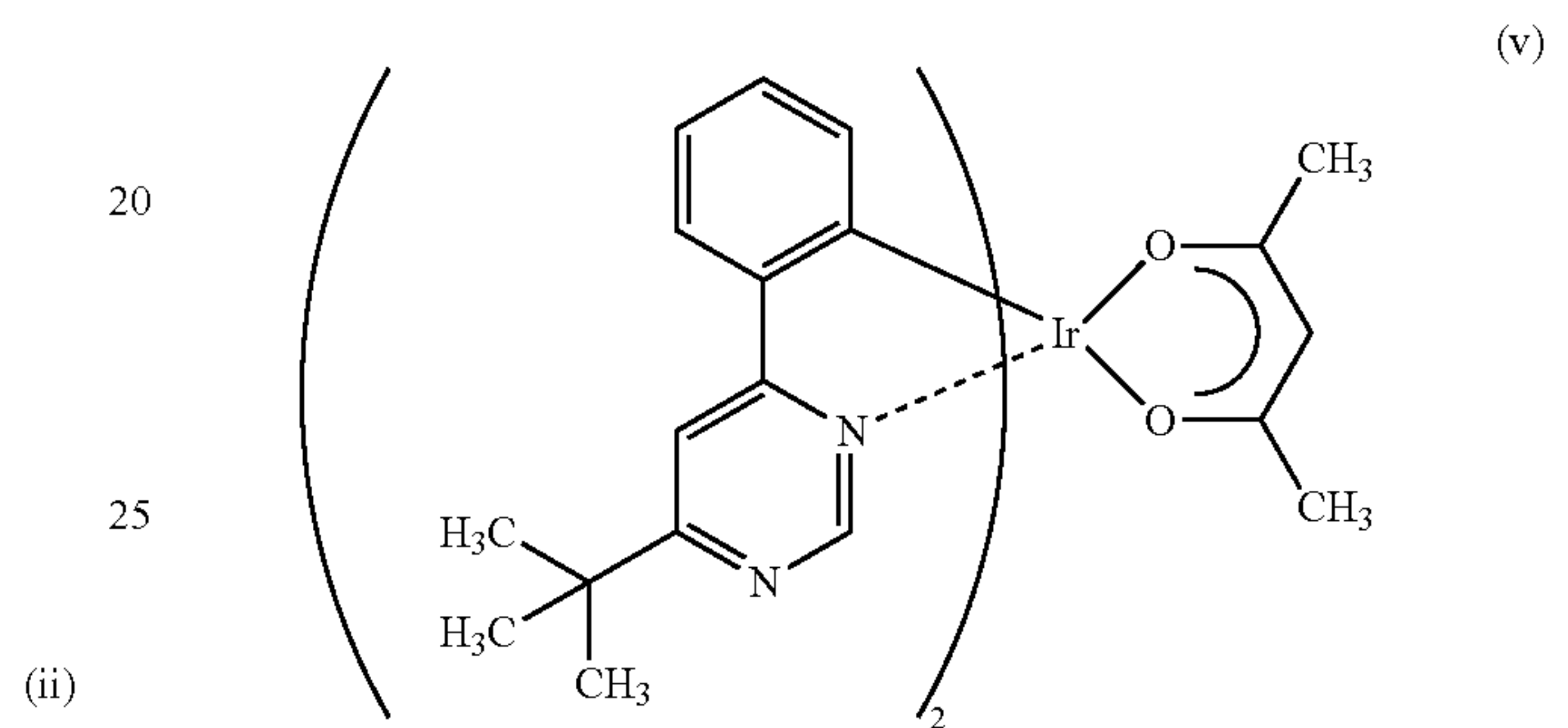
Ir(tBuppm) 2 (acac)
