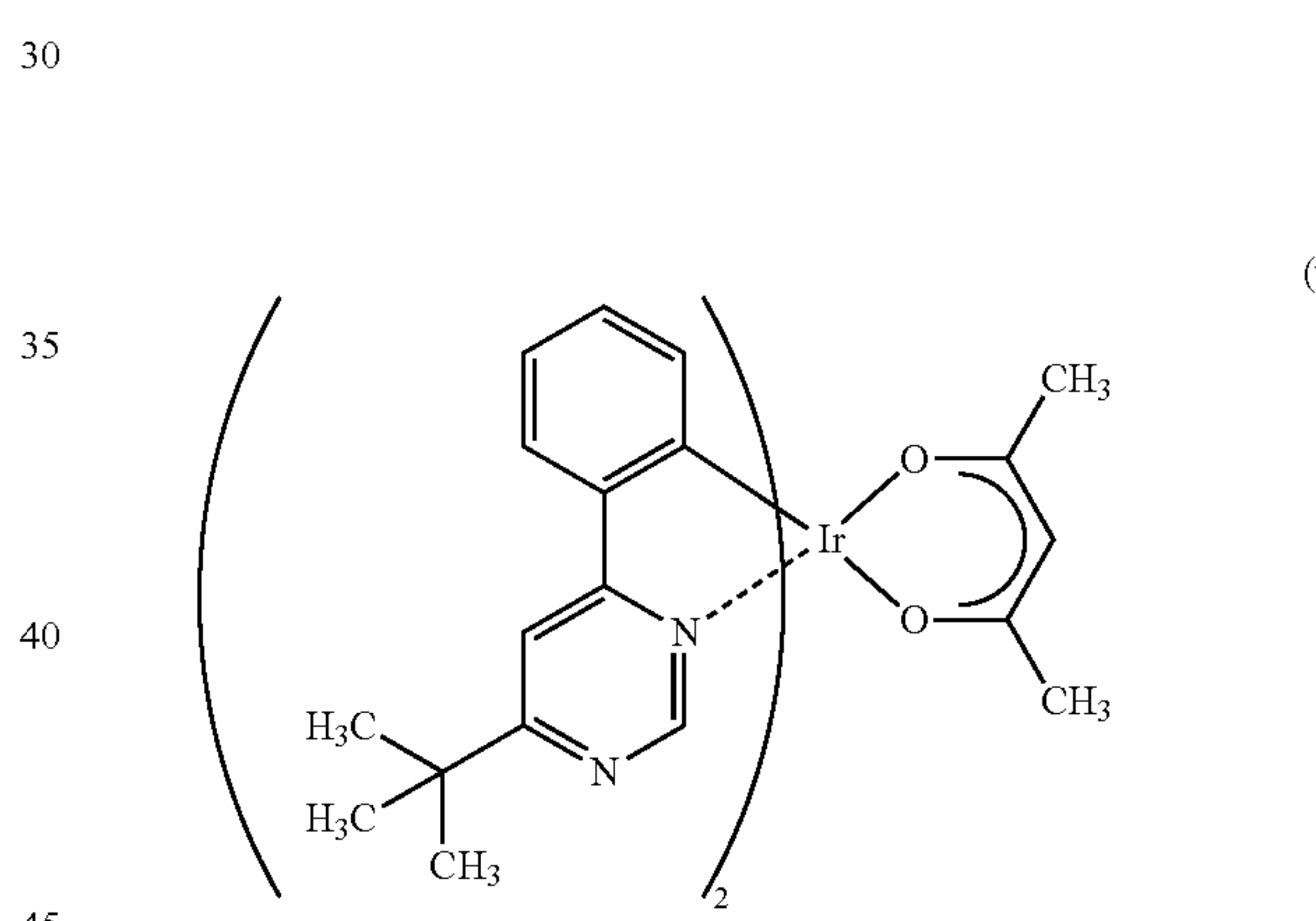
Ir(tBuppm) 2 (acac)
