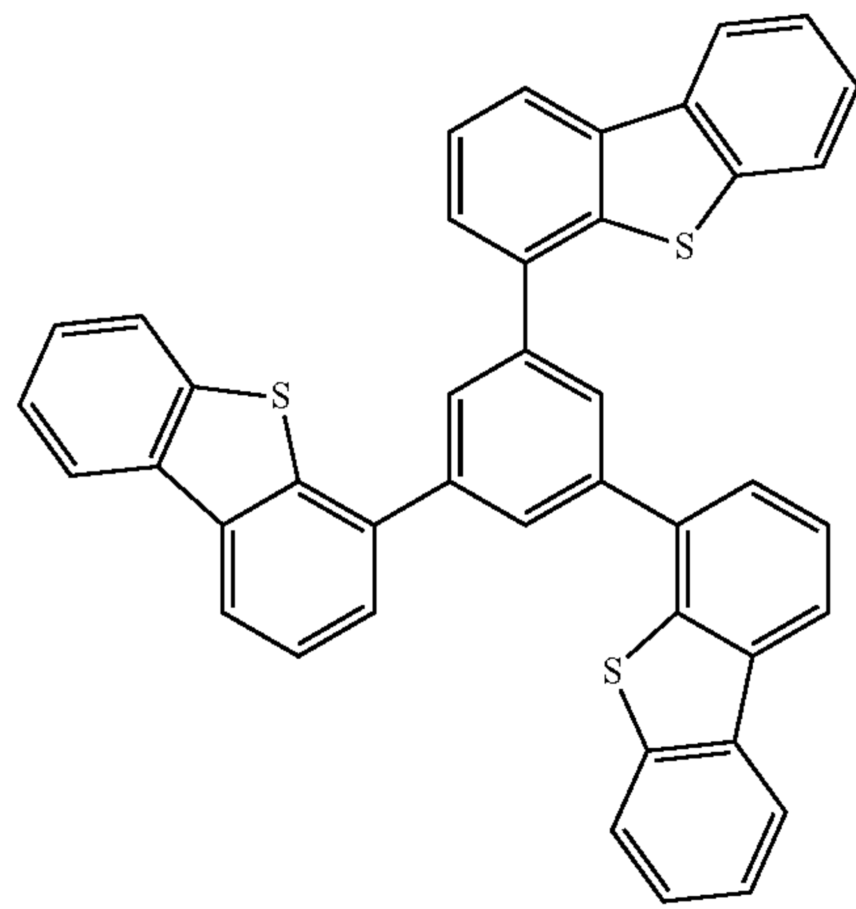
DBT3P-II
