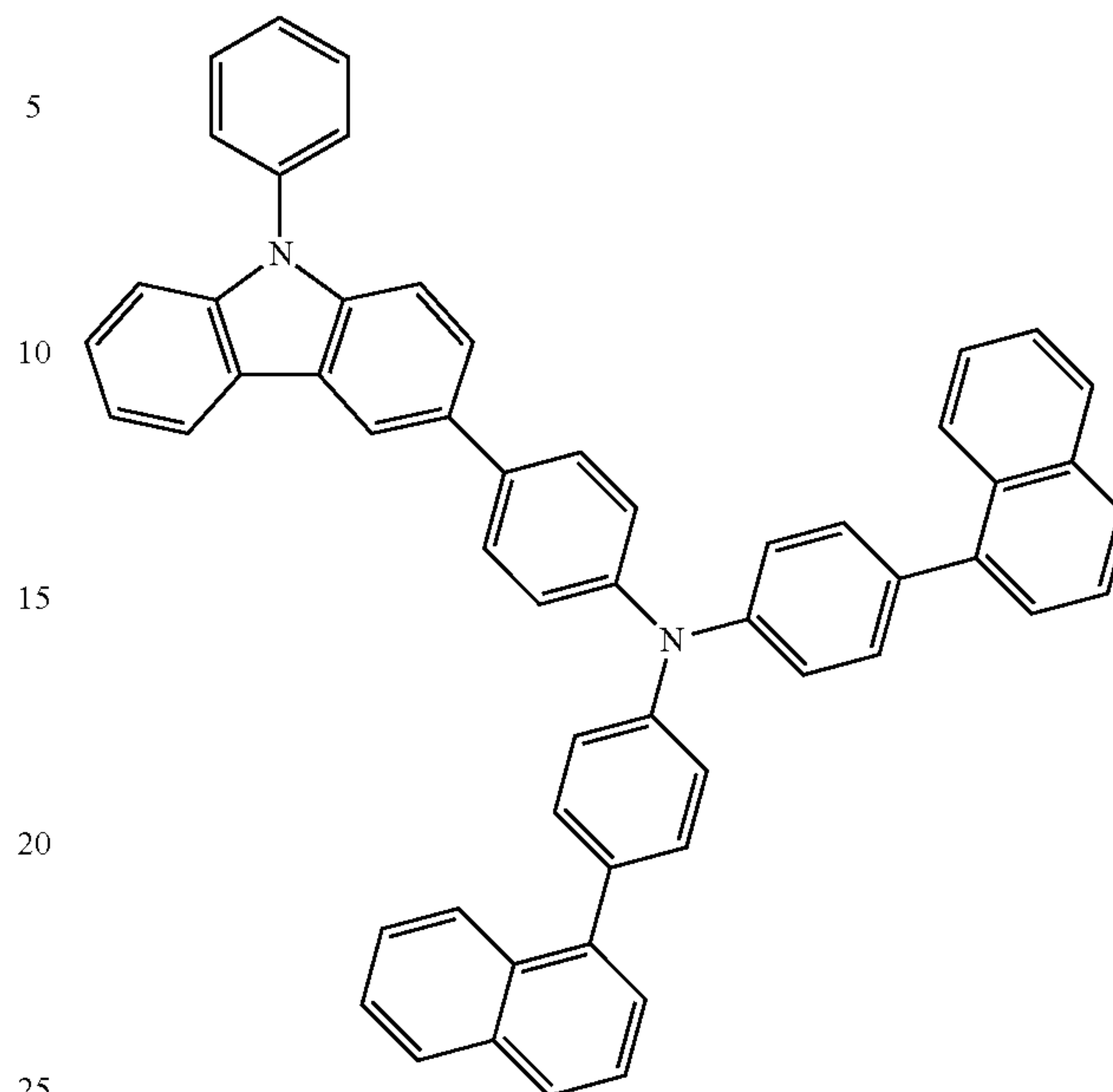
PCBNBB
