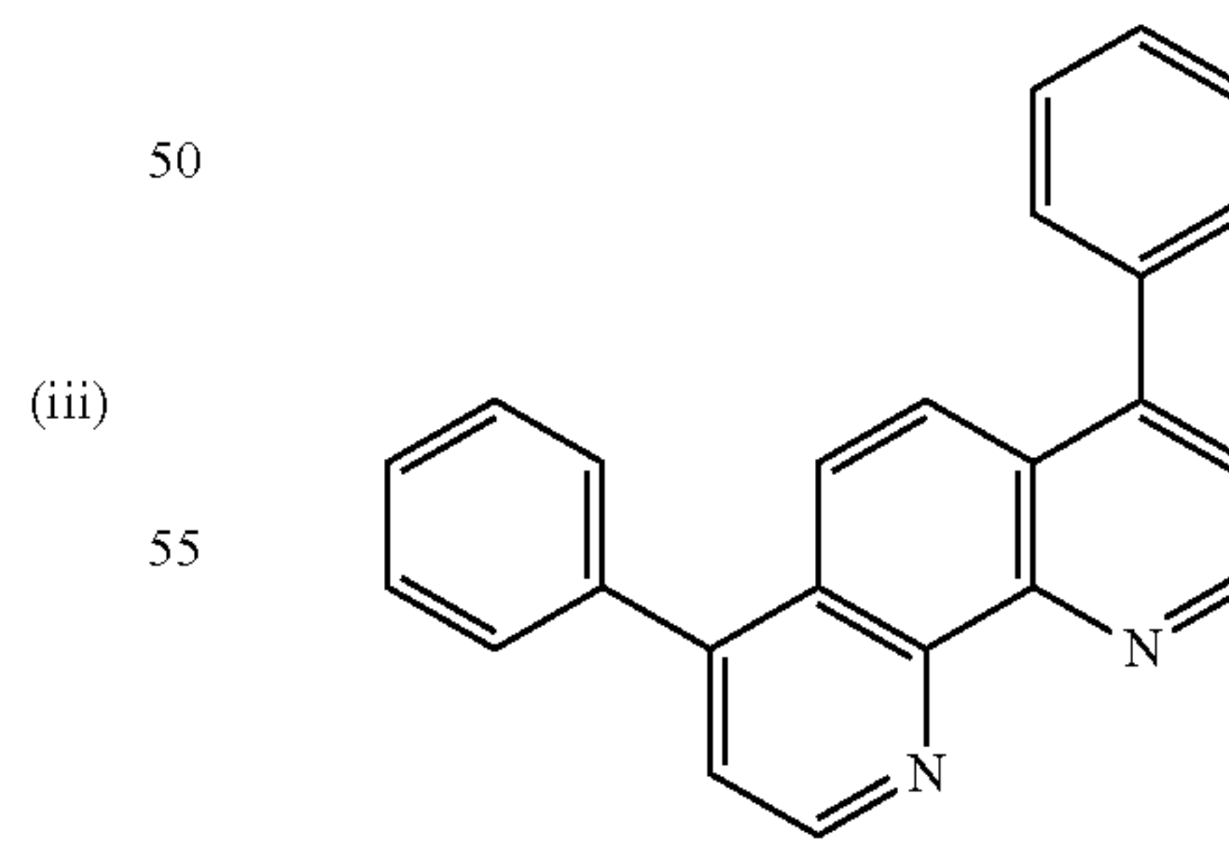
BPhen
