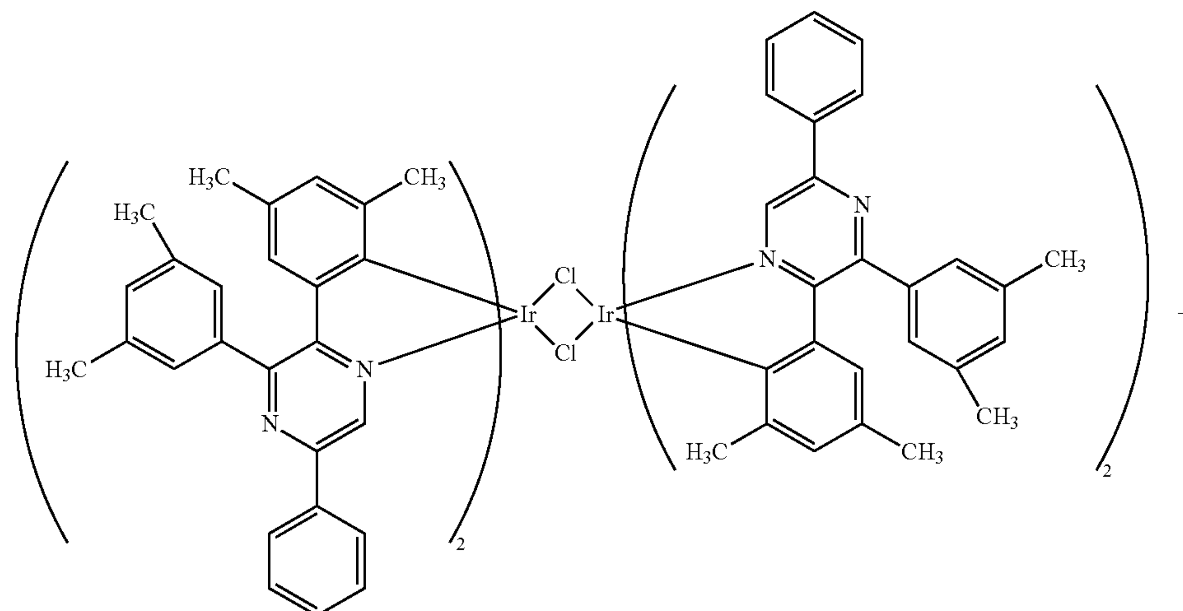
[Ir(dmdppr-P) 2 Cl] 2
