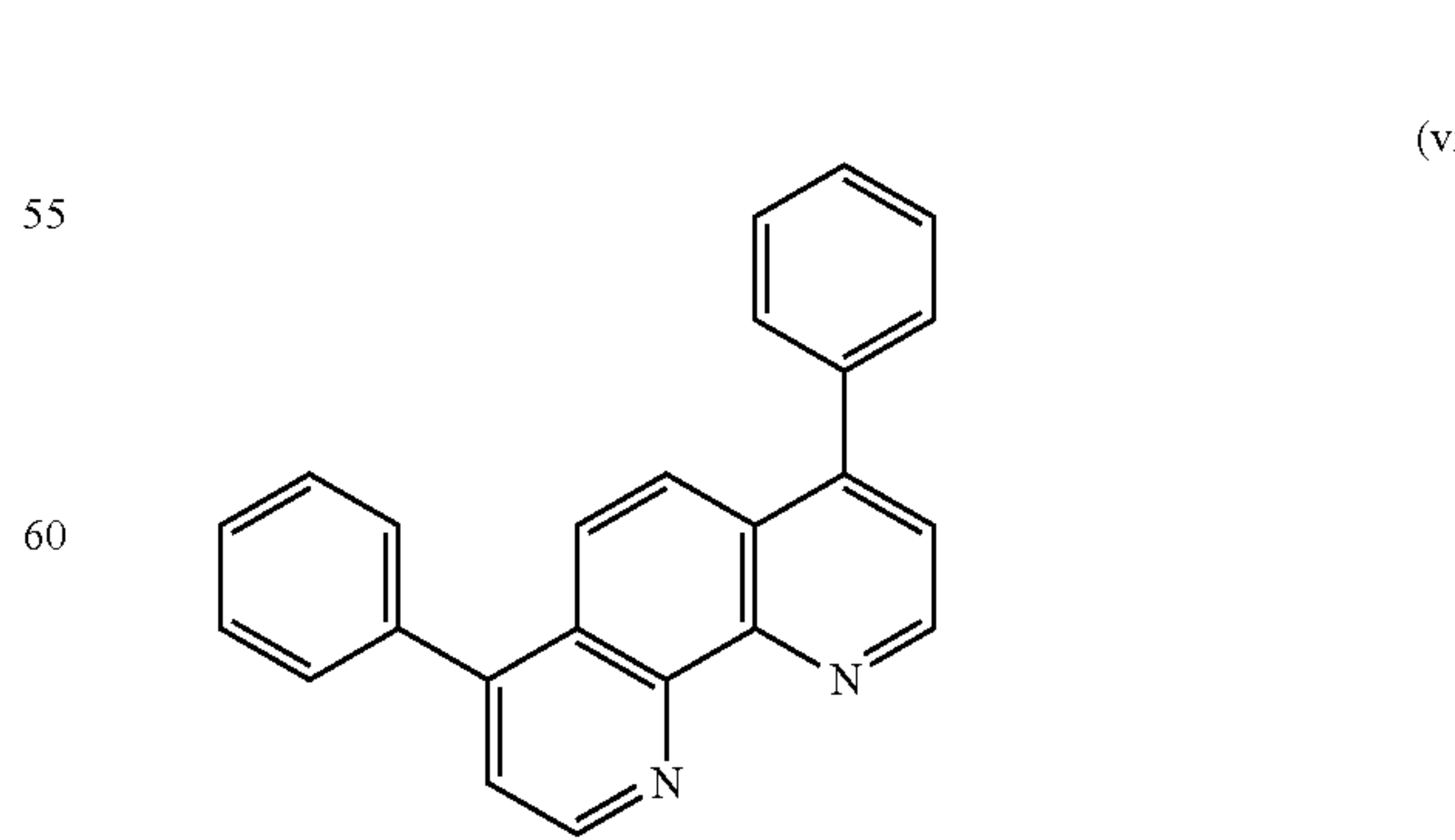
BPhen
