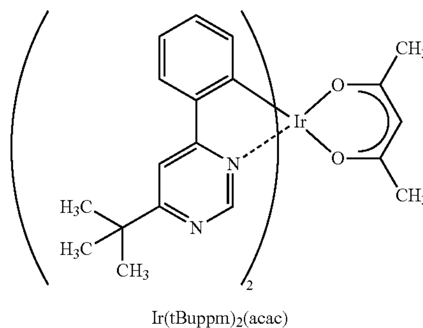
[Chemical formula 6]
