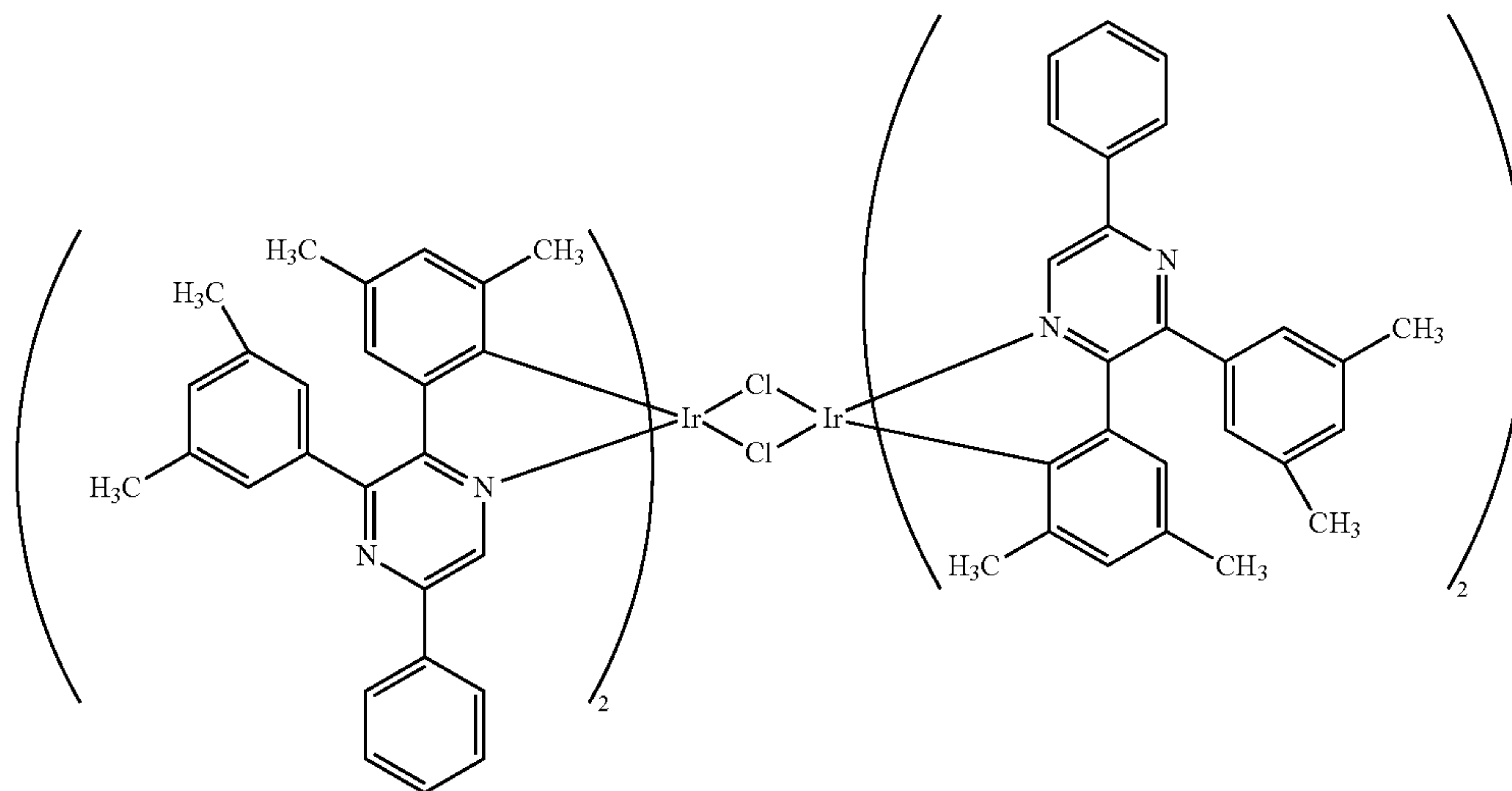
[Ir(dmdppr-P) 2 Cl] 2
