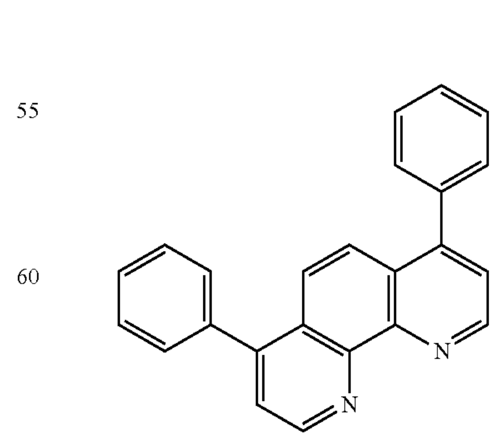
BPhen
