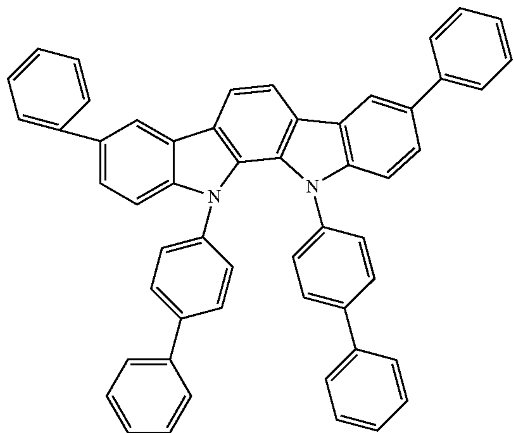
Compound H8
