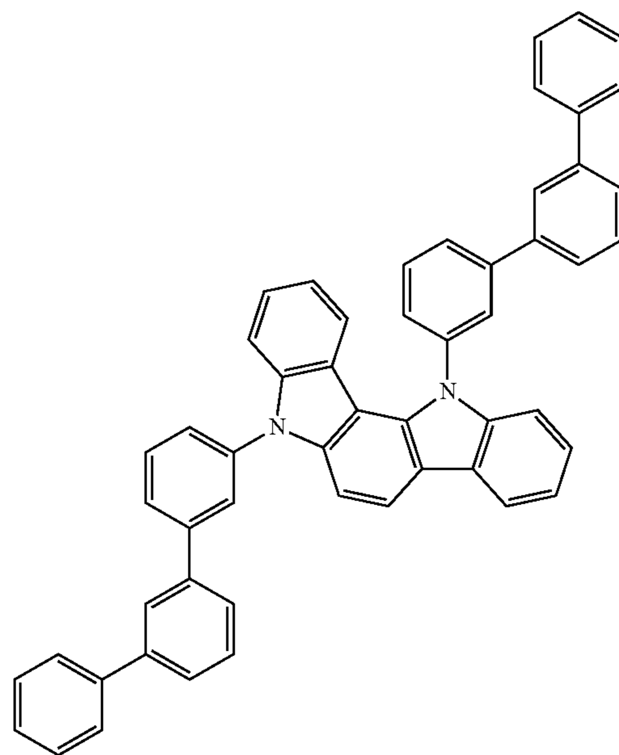
Compound H12
