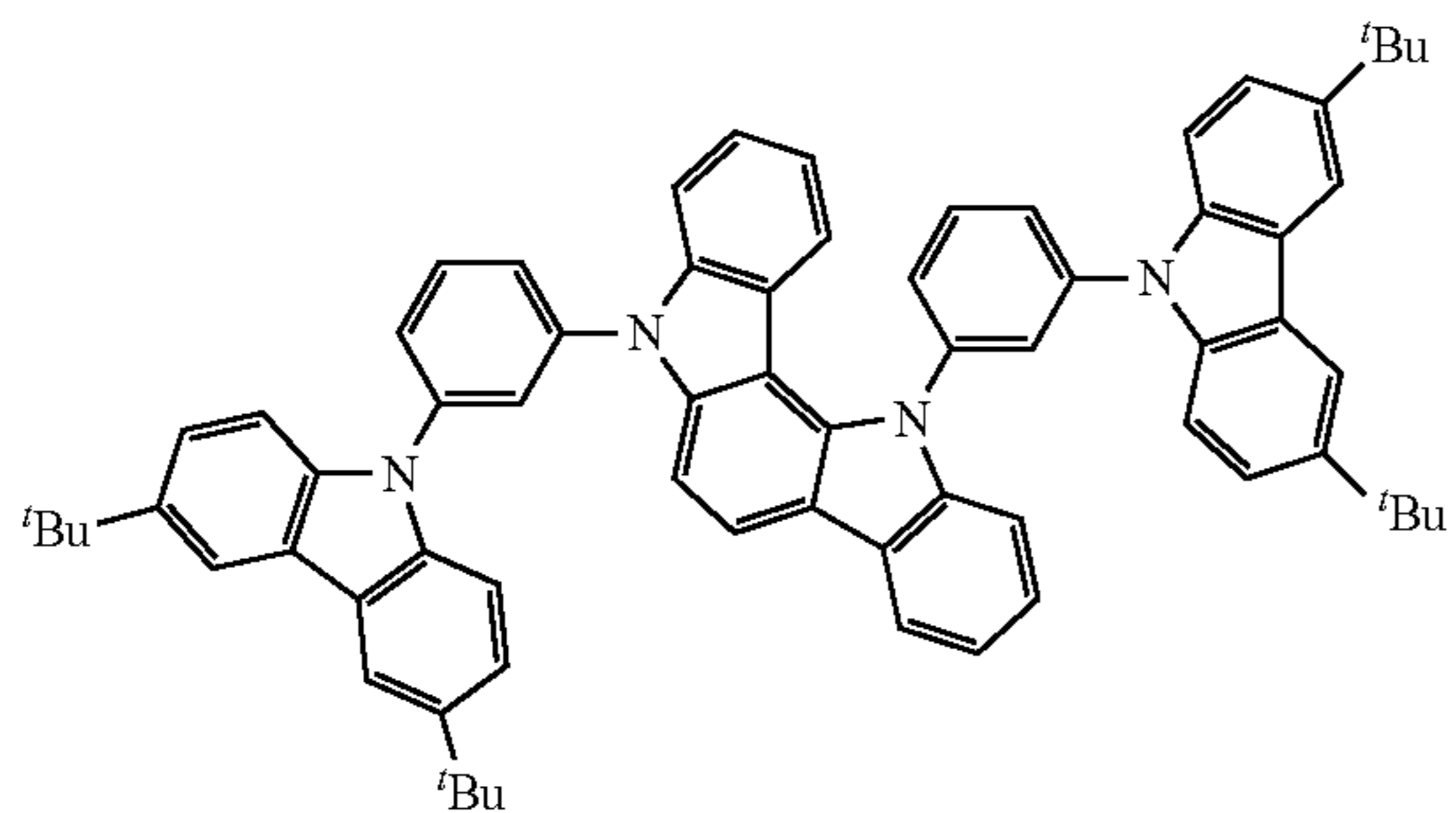
Compound H15
