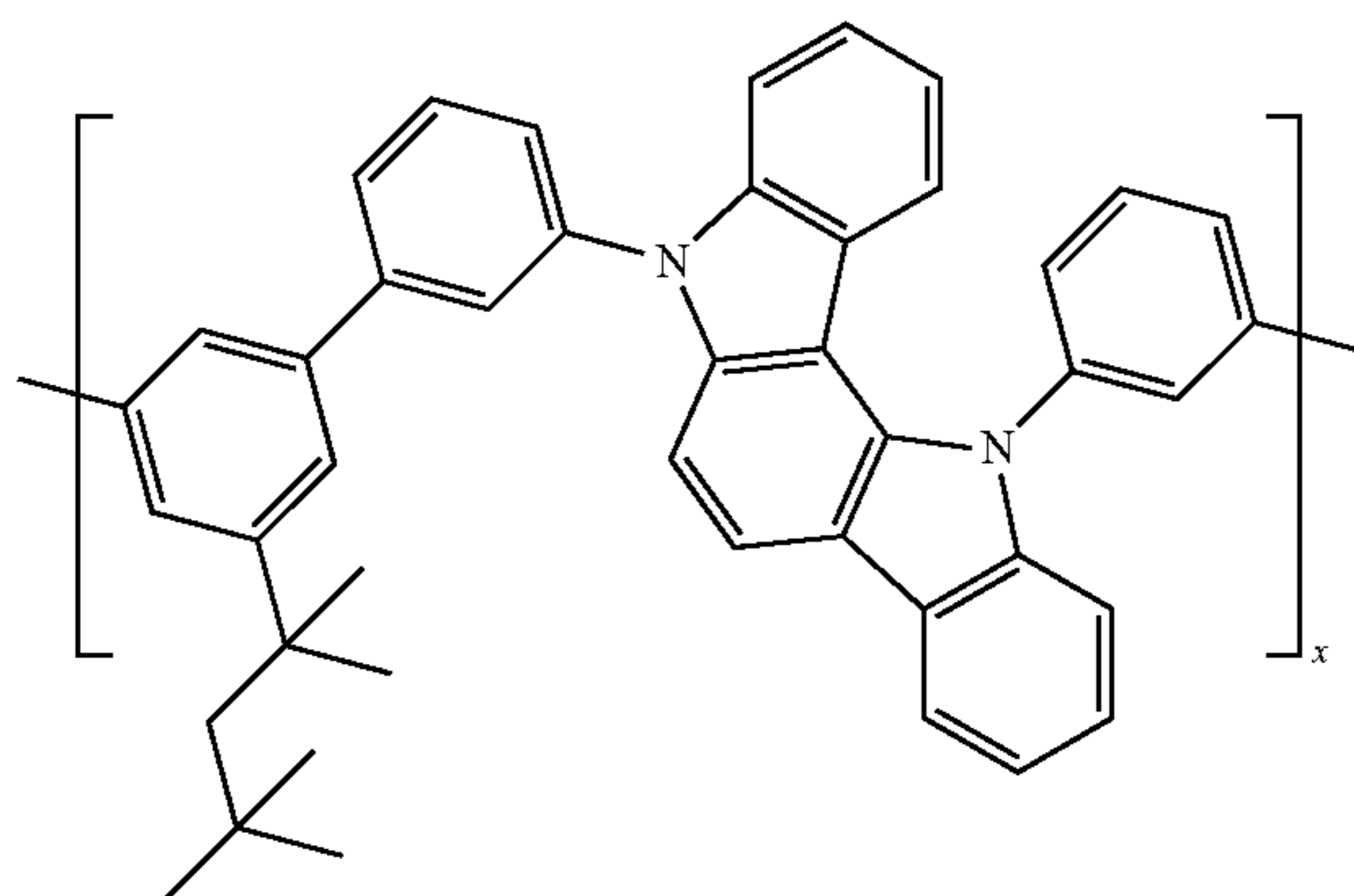
Compound H25
