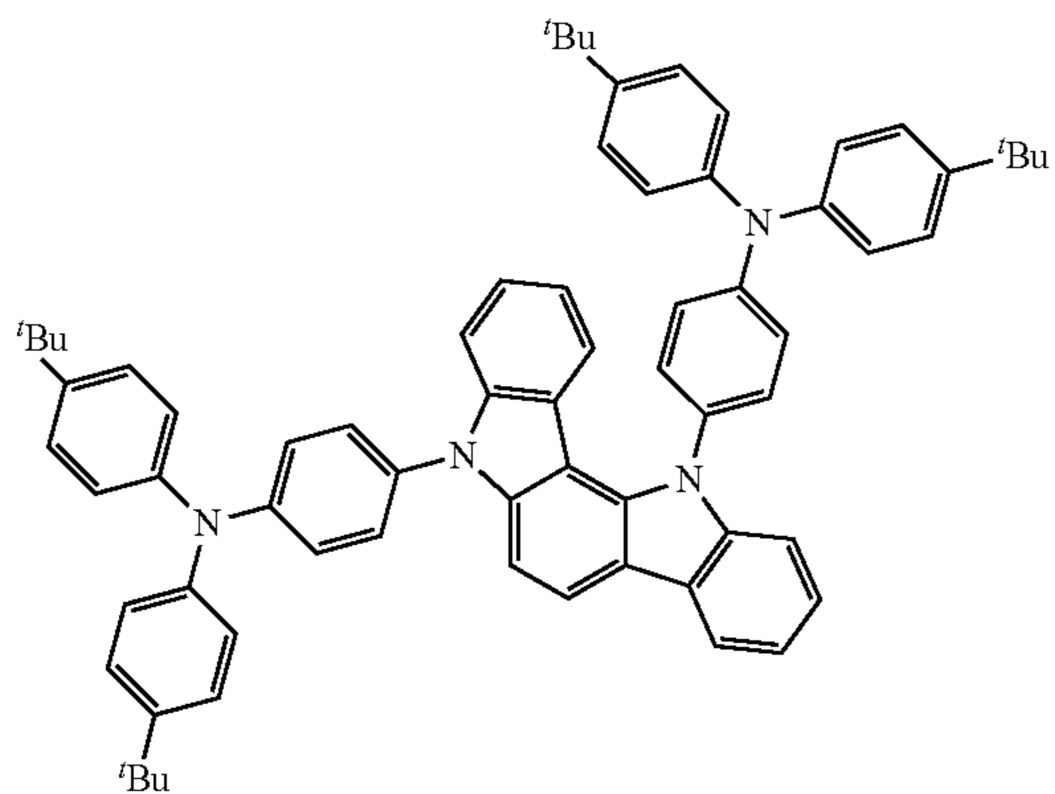
Compound H16
