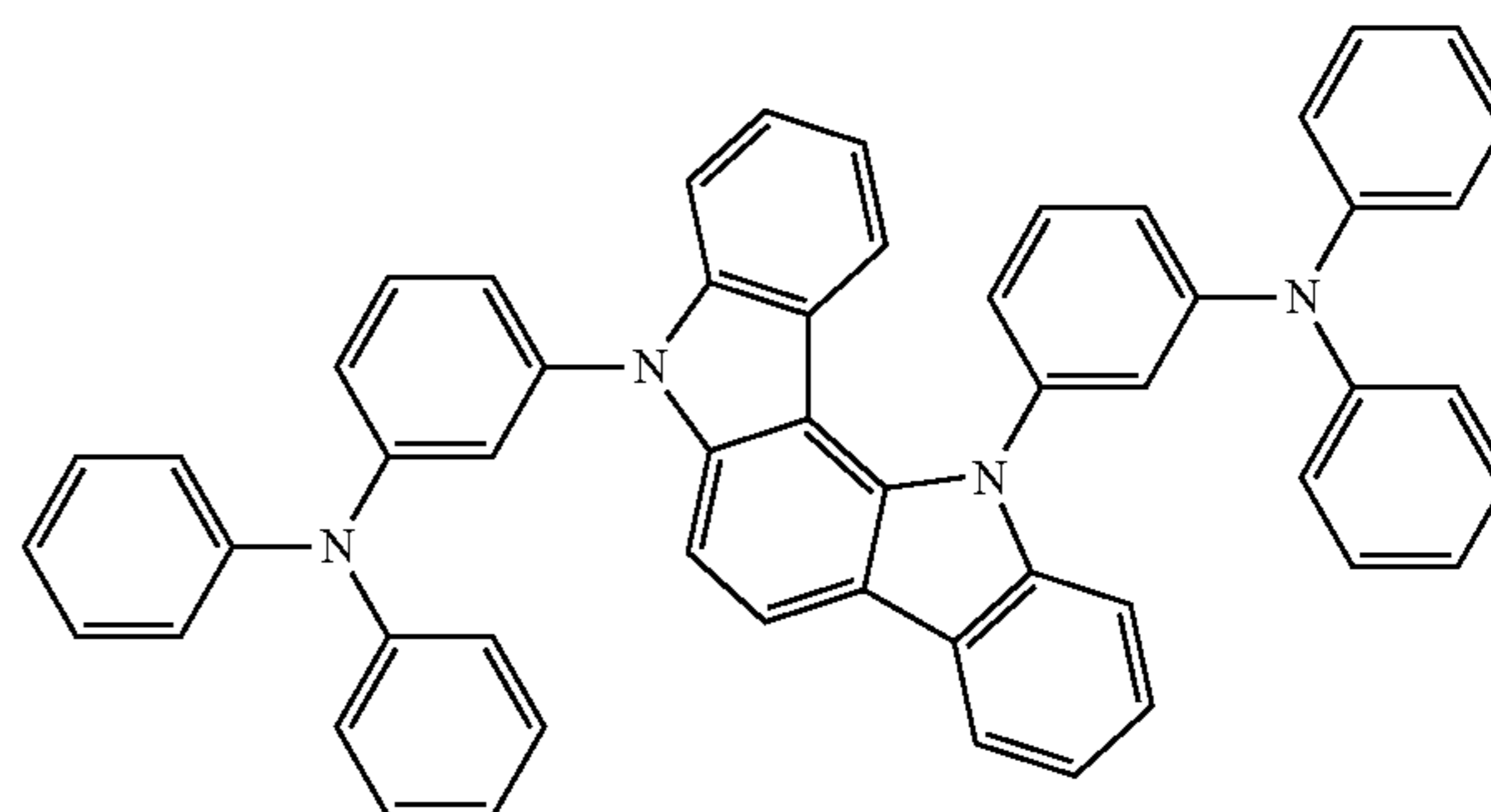
Compound H14
