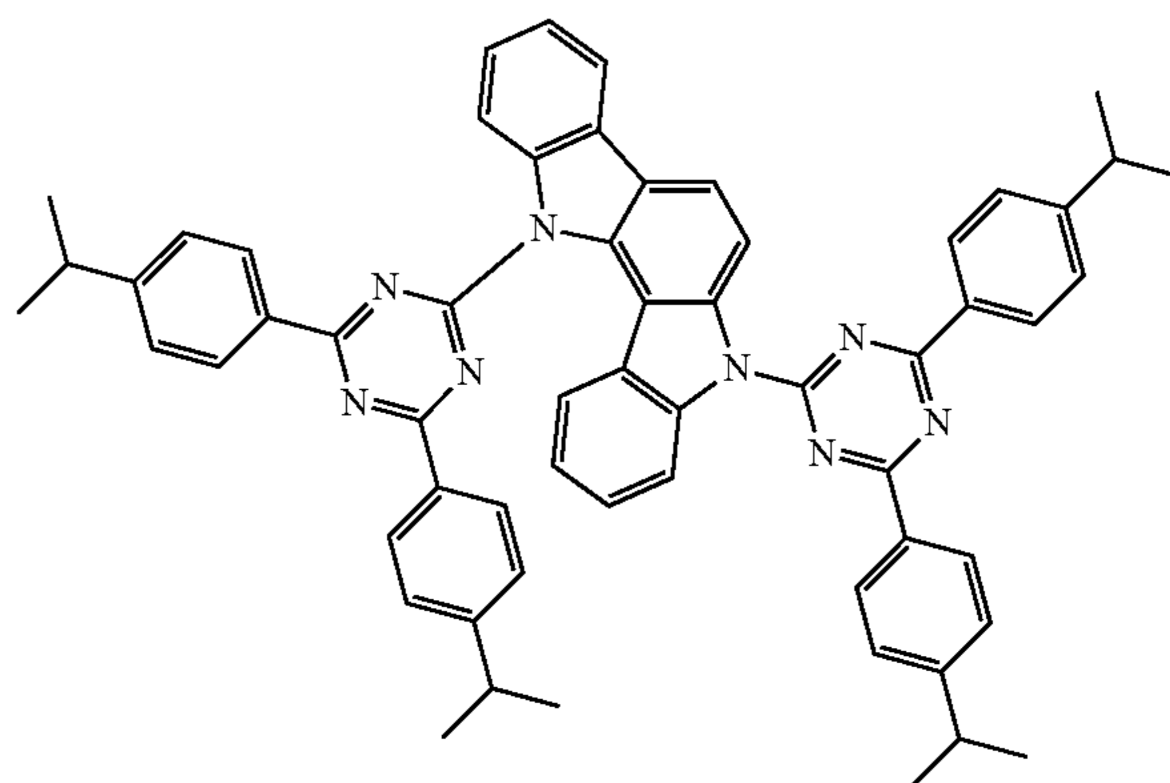
Compound H18
