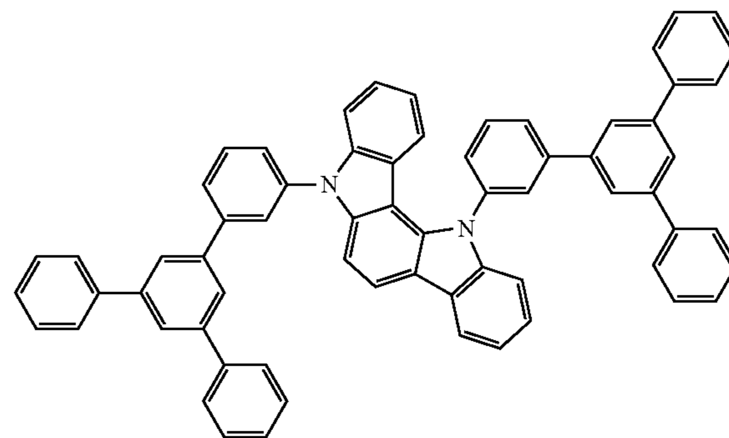
Compound H14
