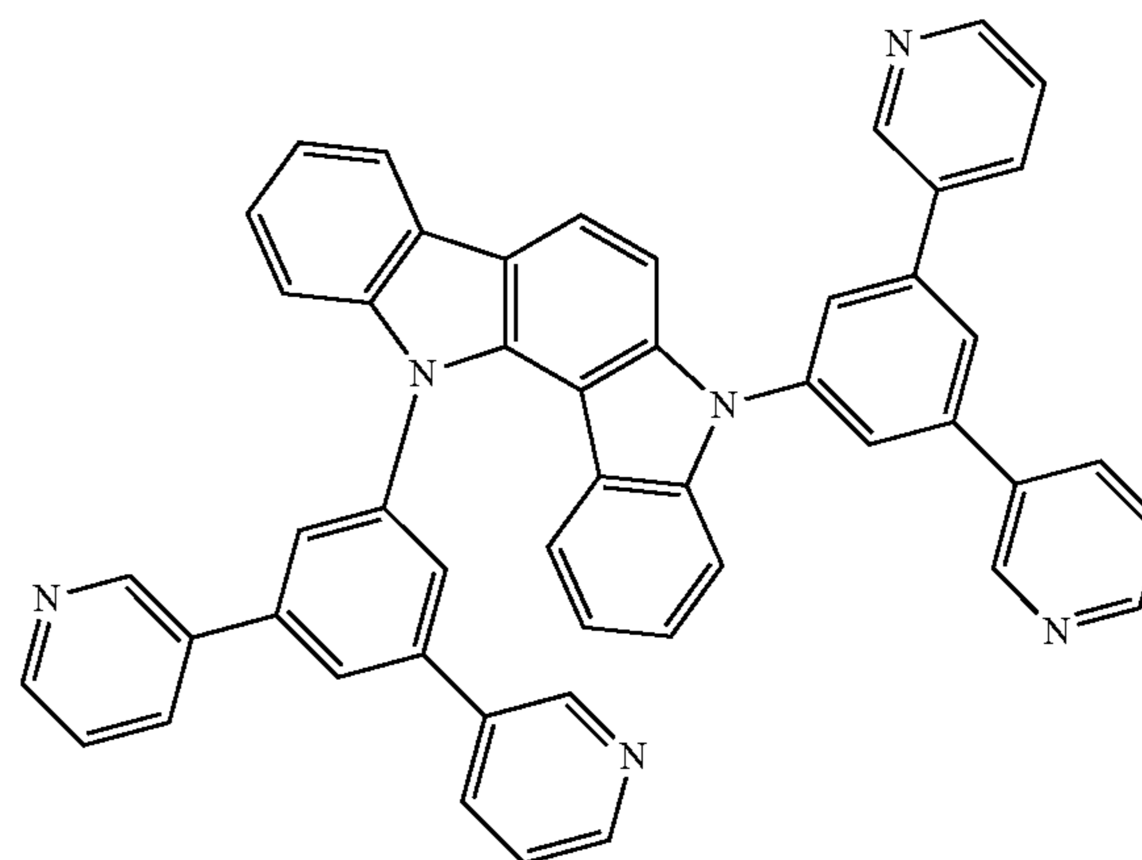
Compound H21
