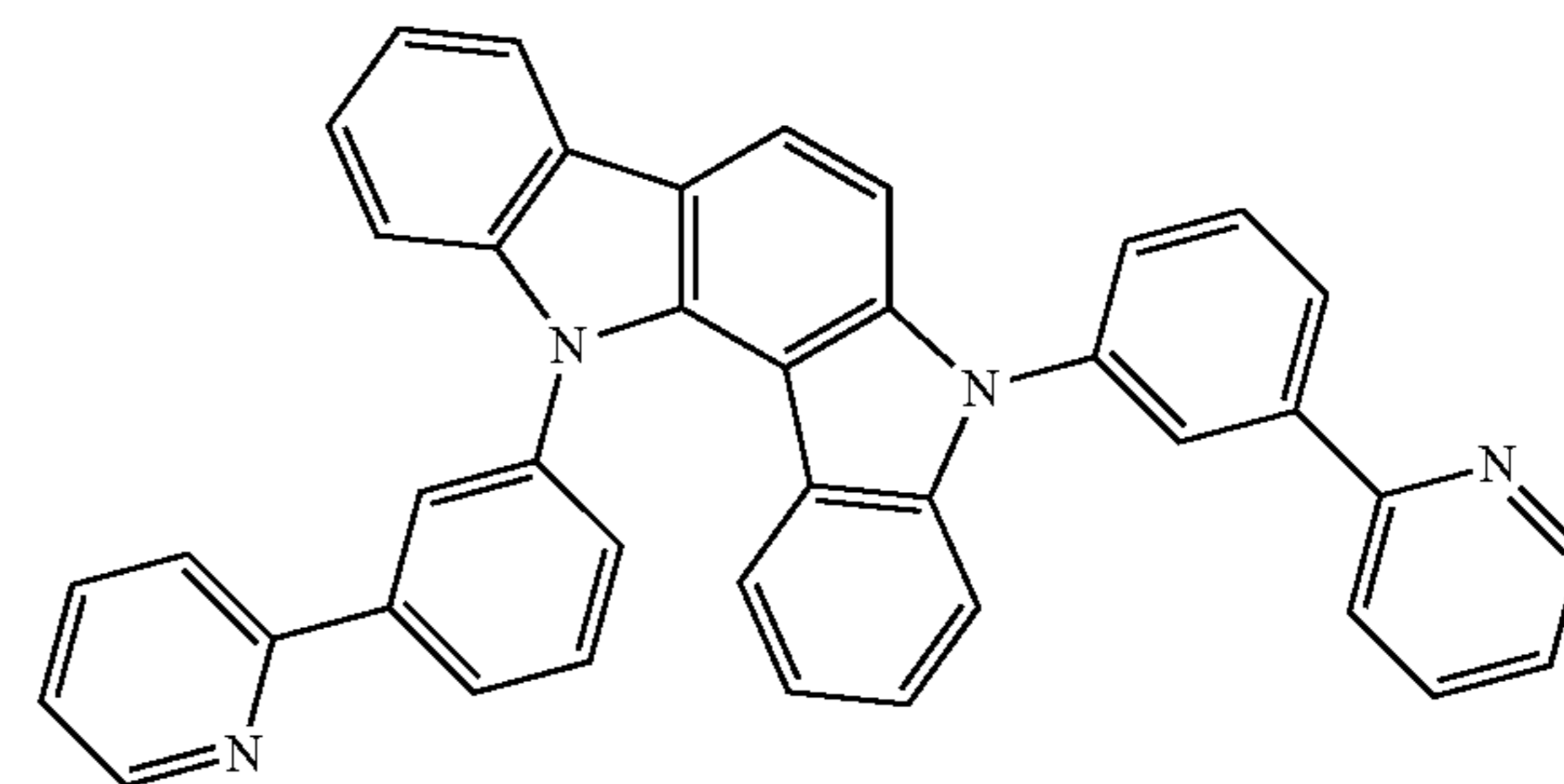
Compound H19
