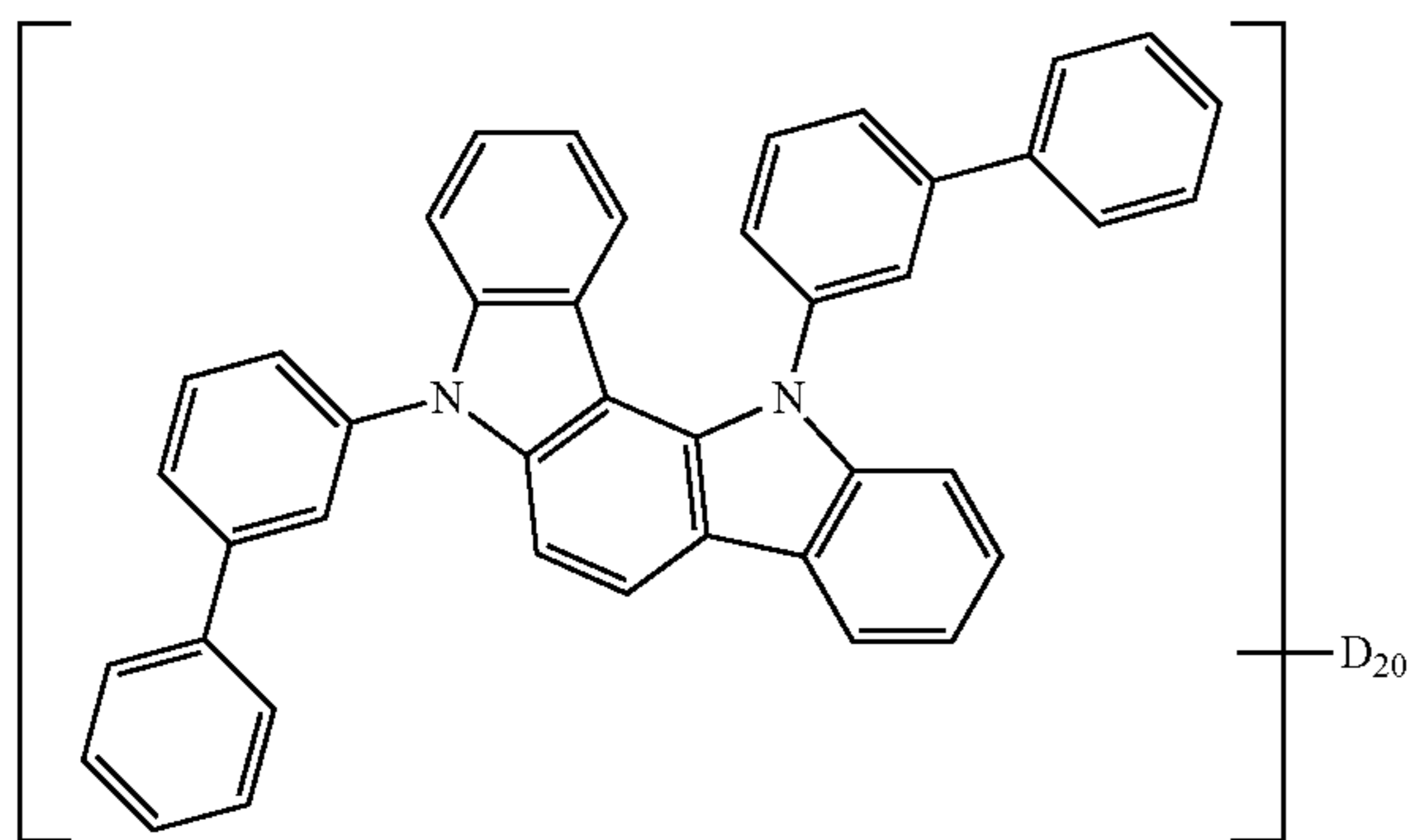
Compound H10
