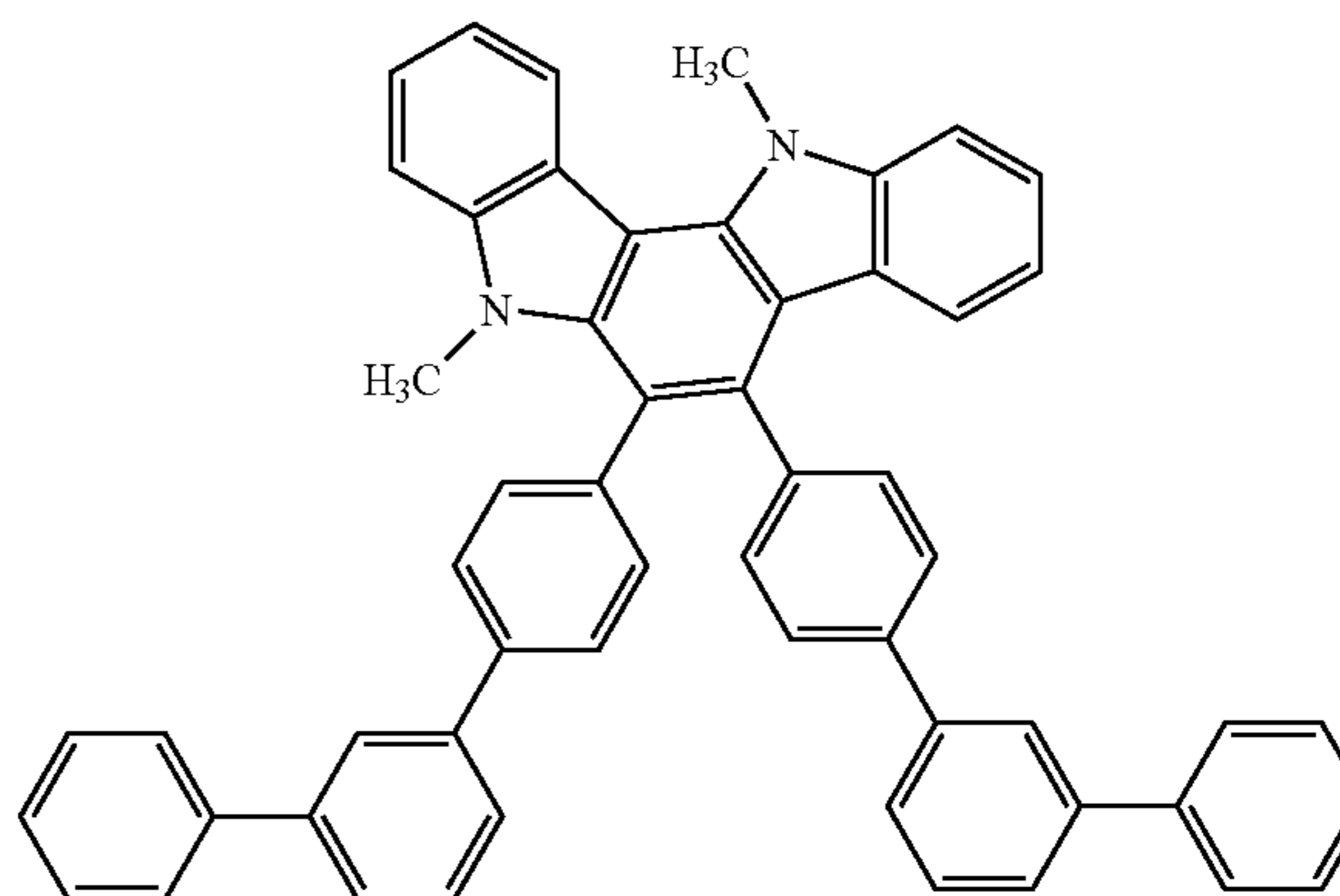
Compound H21
