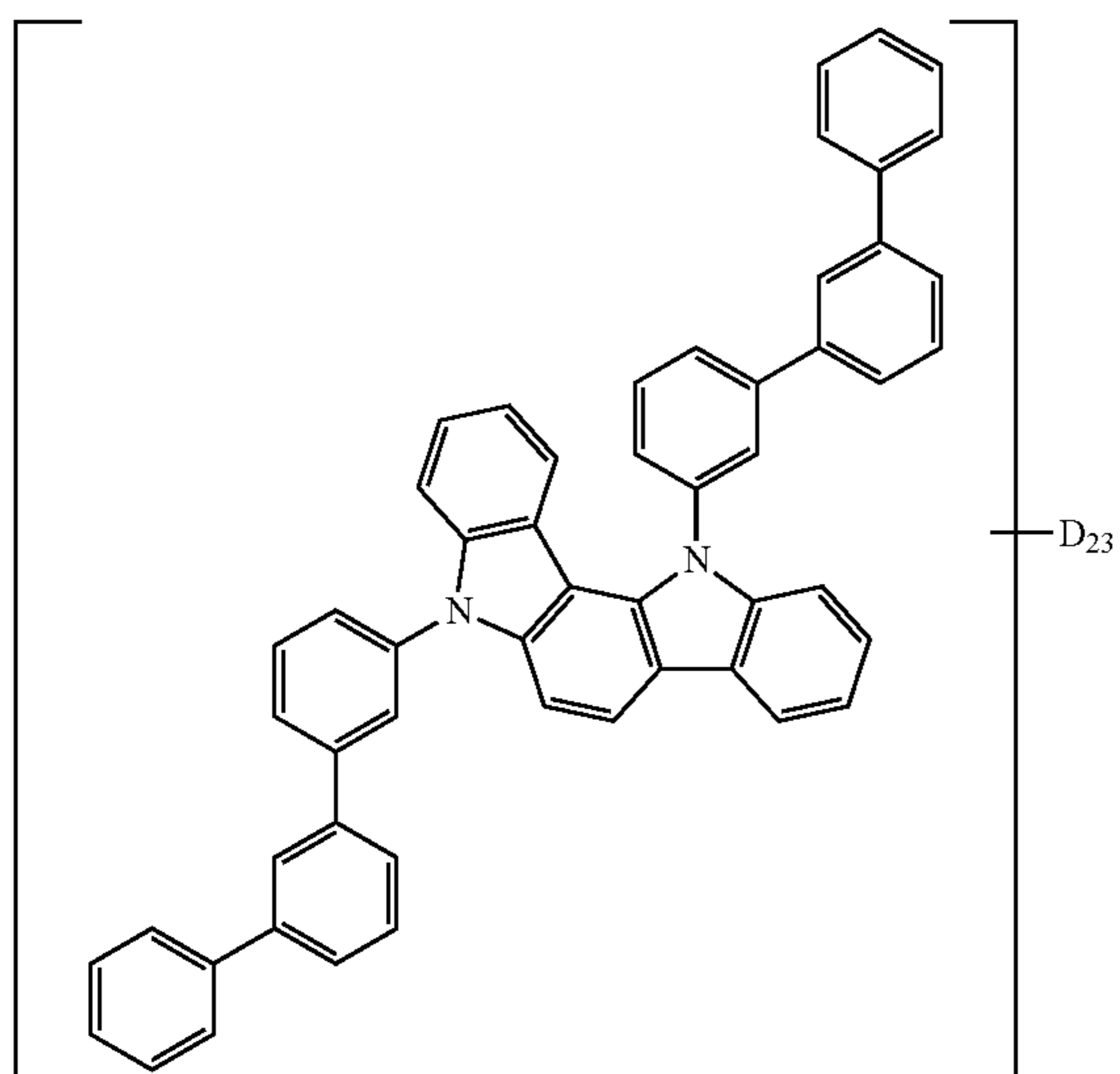
Compound H17
