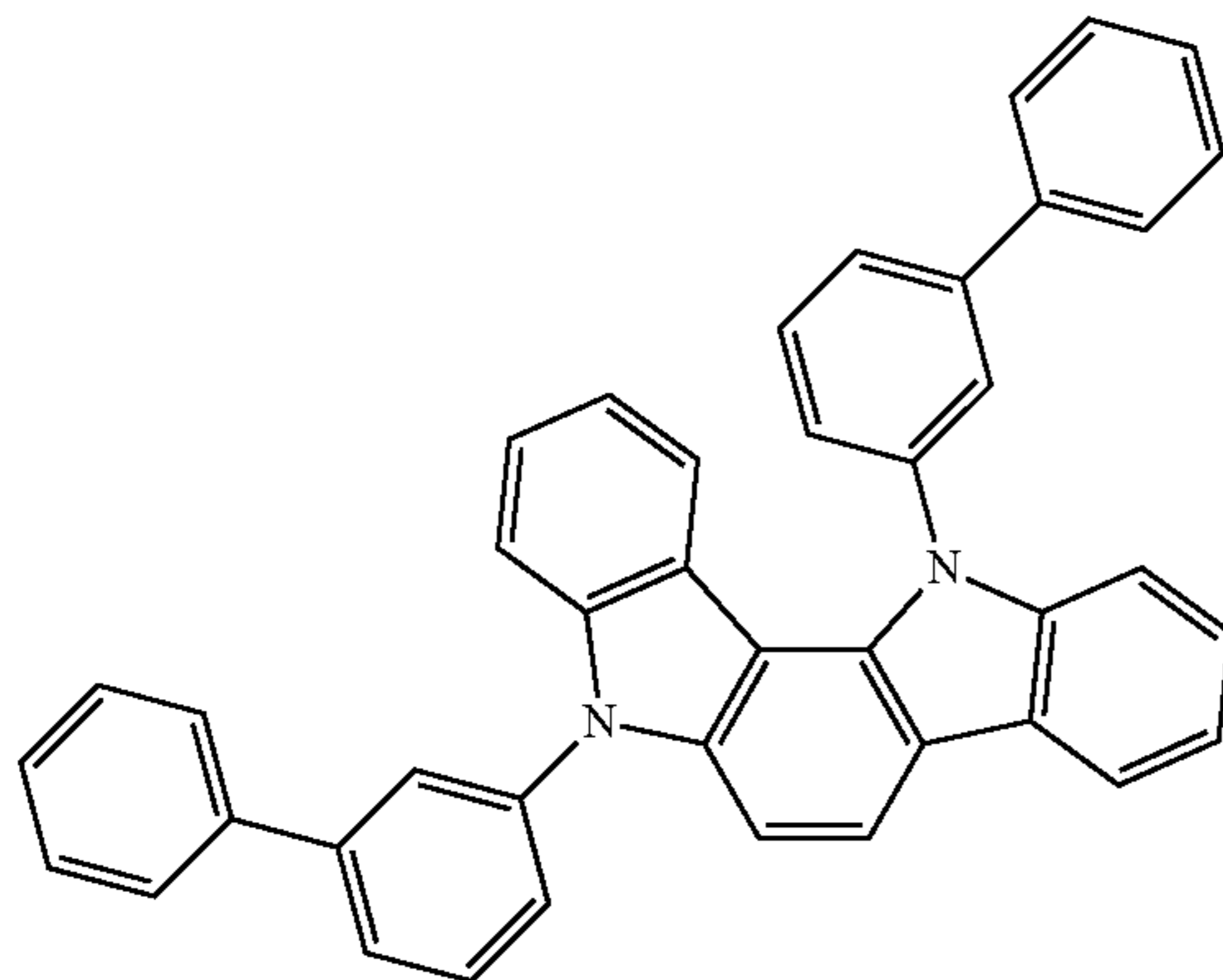
Compound H25
