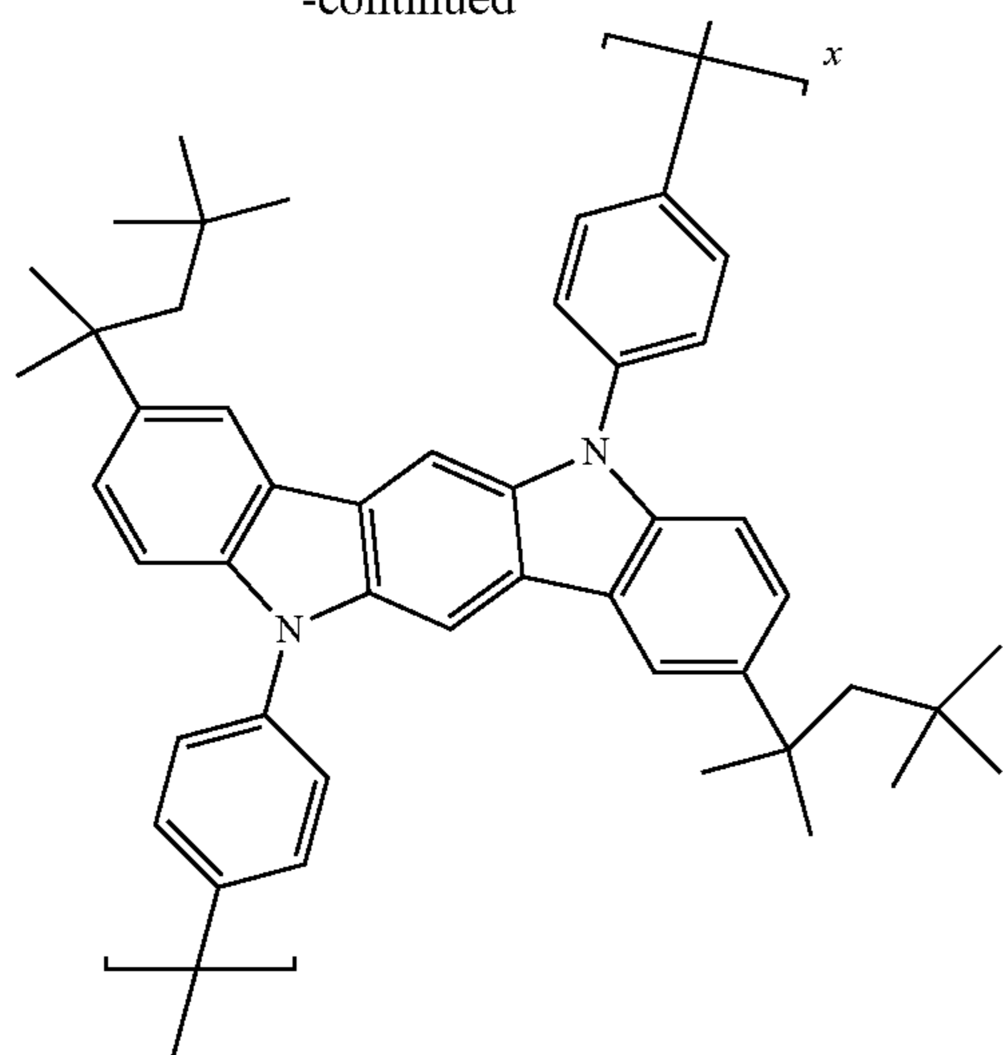
Compound H27
