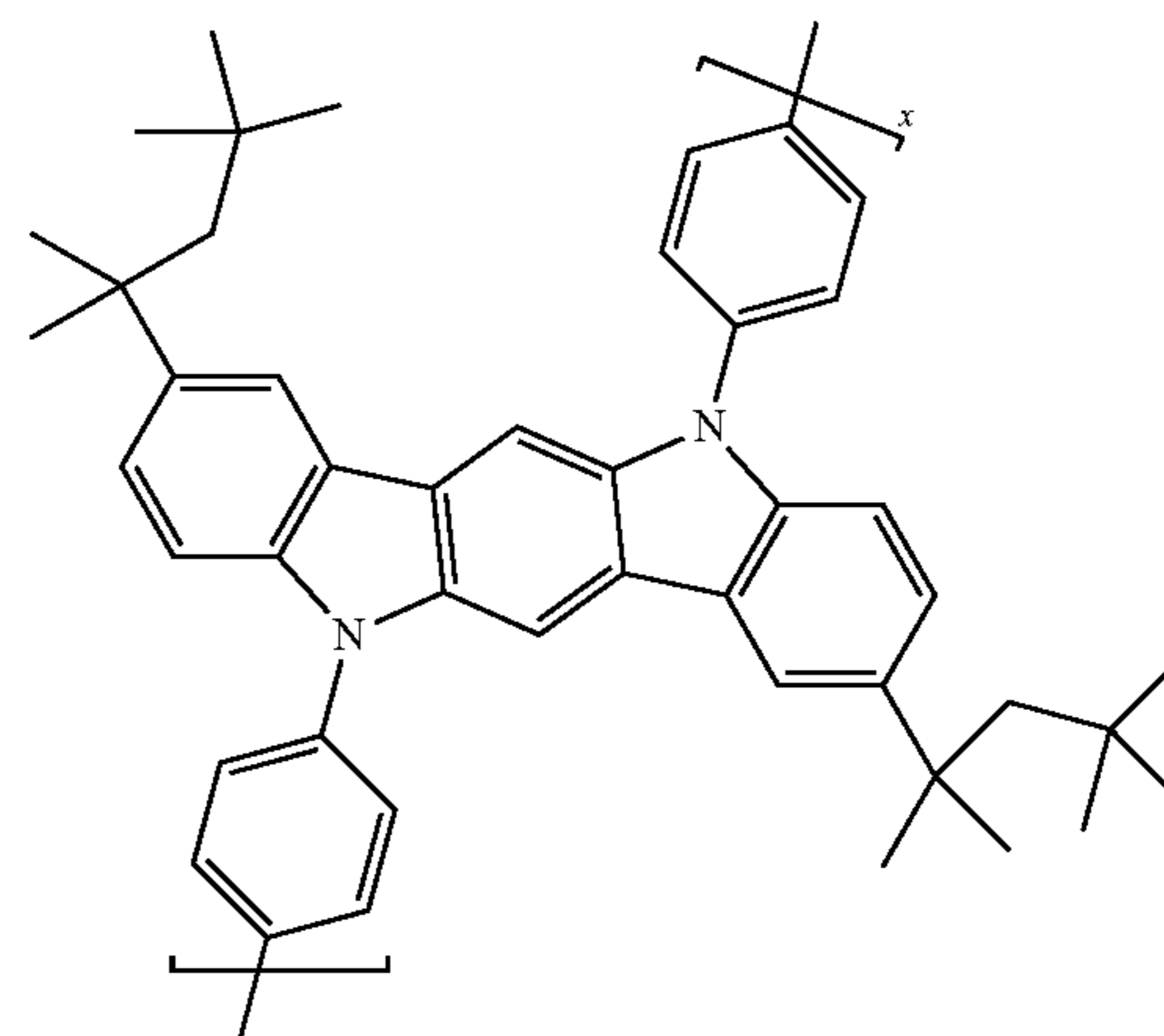
Compound H27
