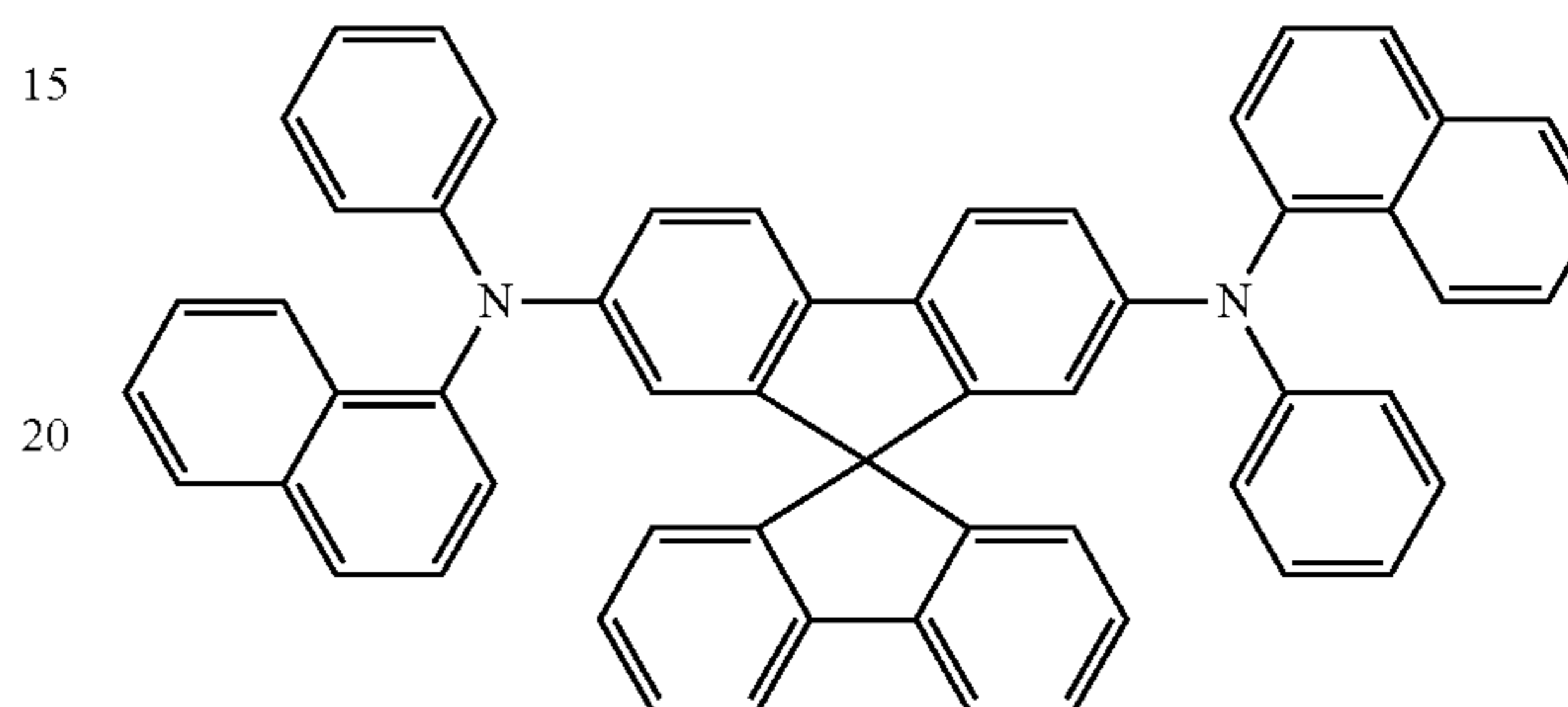
Spiro-NPD
