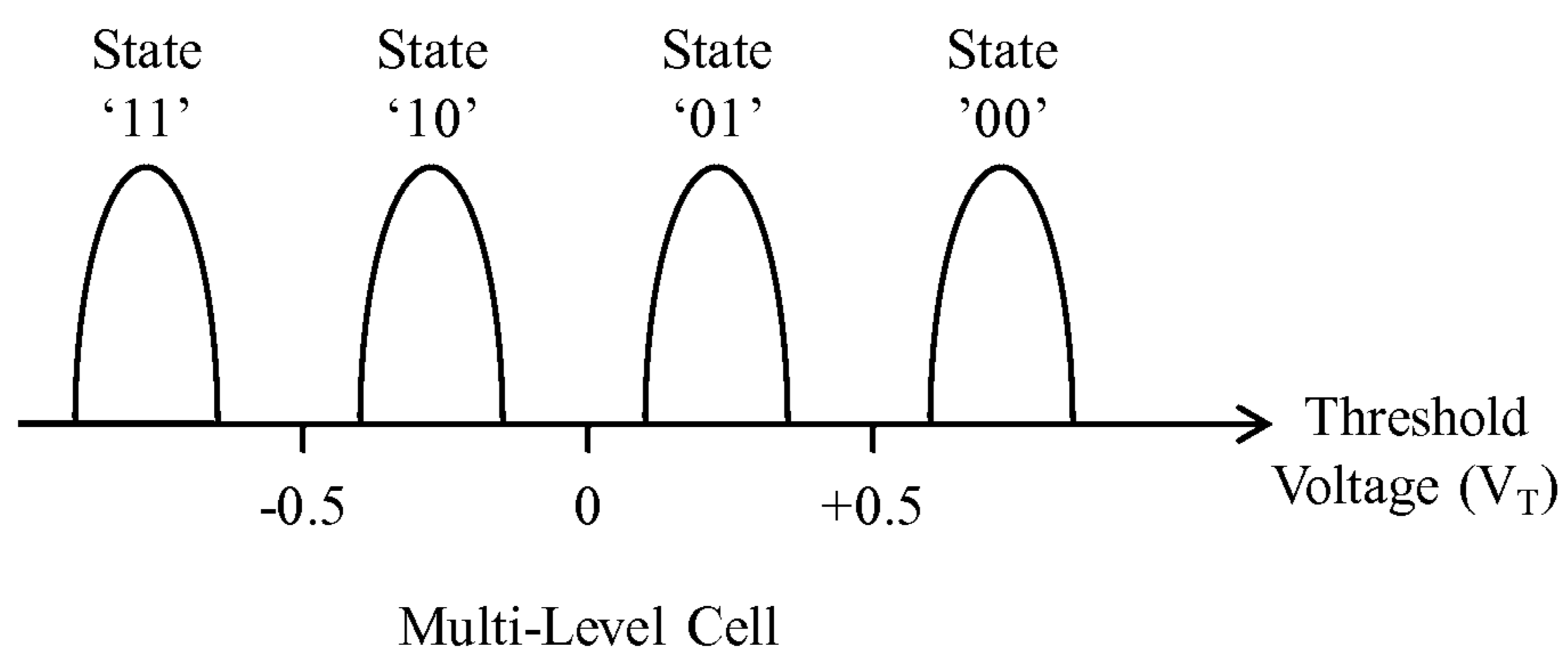
Multi-Level Cell FIG. 22
