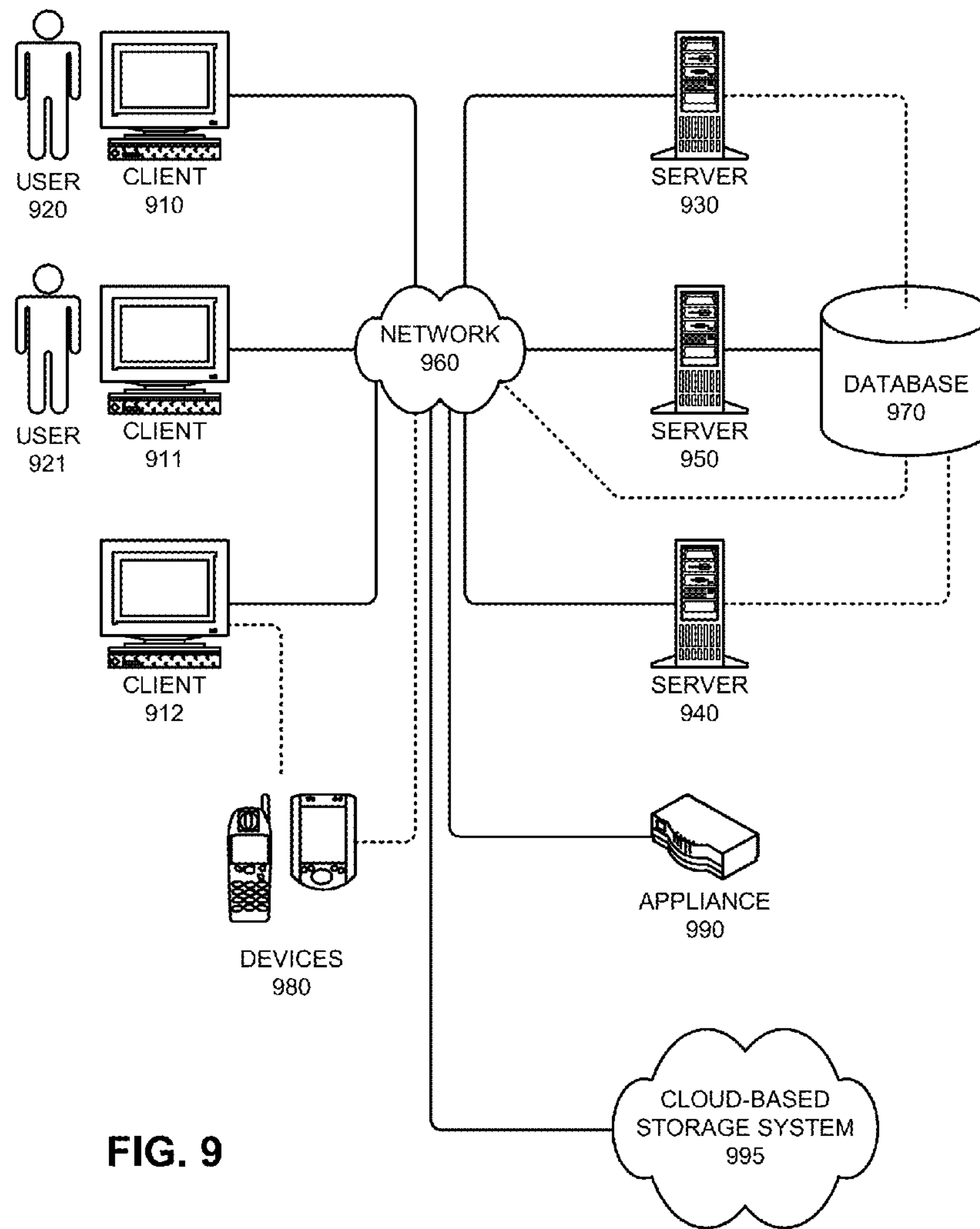
COMPUTING ENVIRONMENT 900
