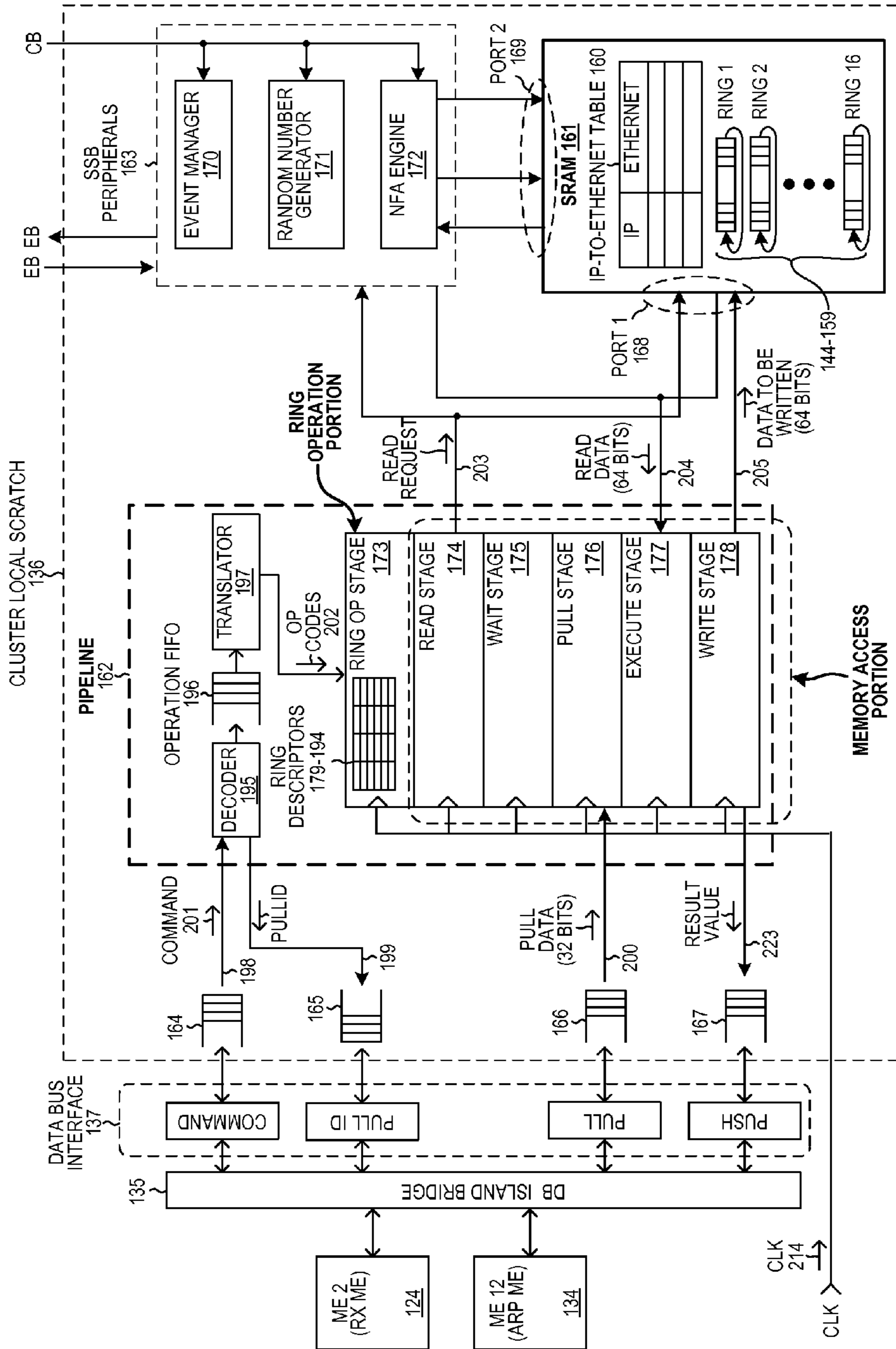
CLUSTER LOCAL SCRATCH
