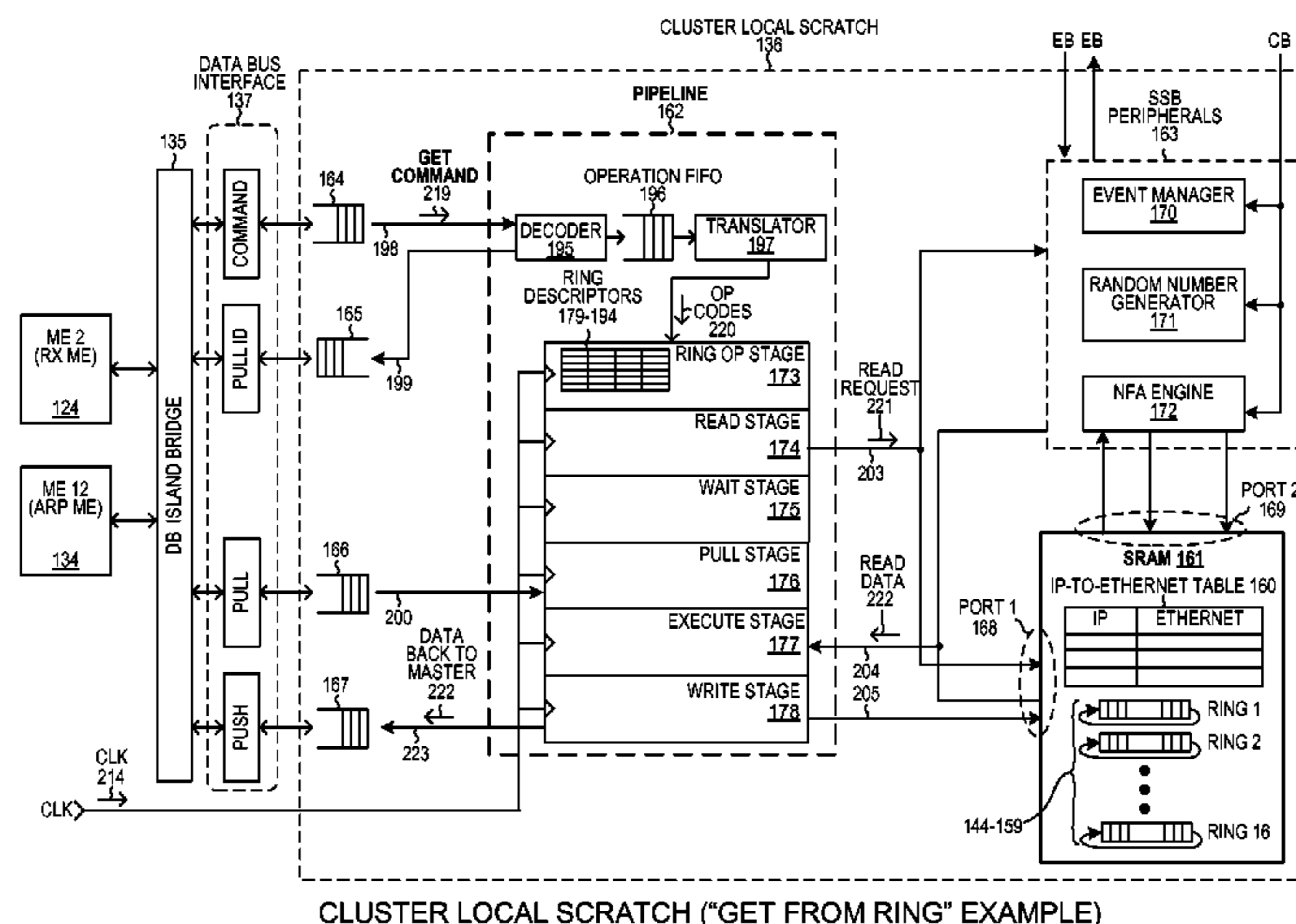
CLUSTER LOCAL SCRATCH ("GET FROM RING" EXAMPLE)
