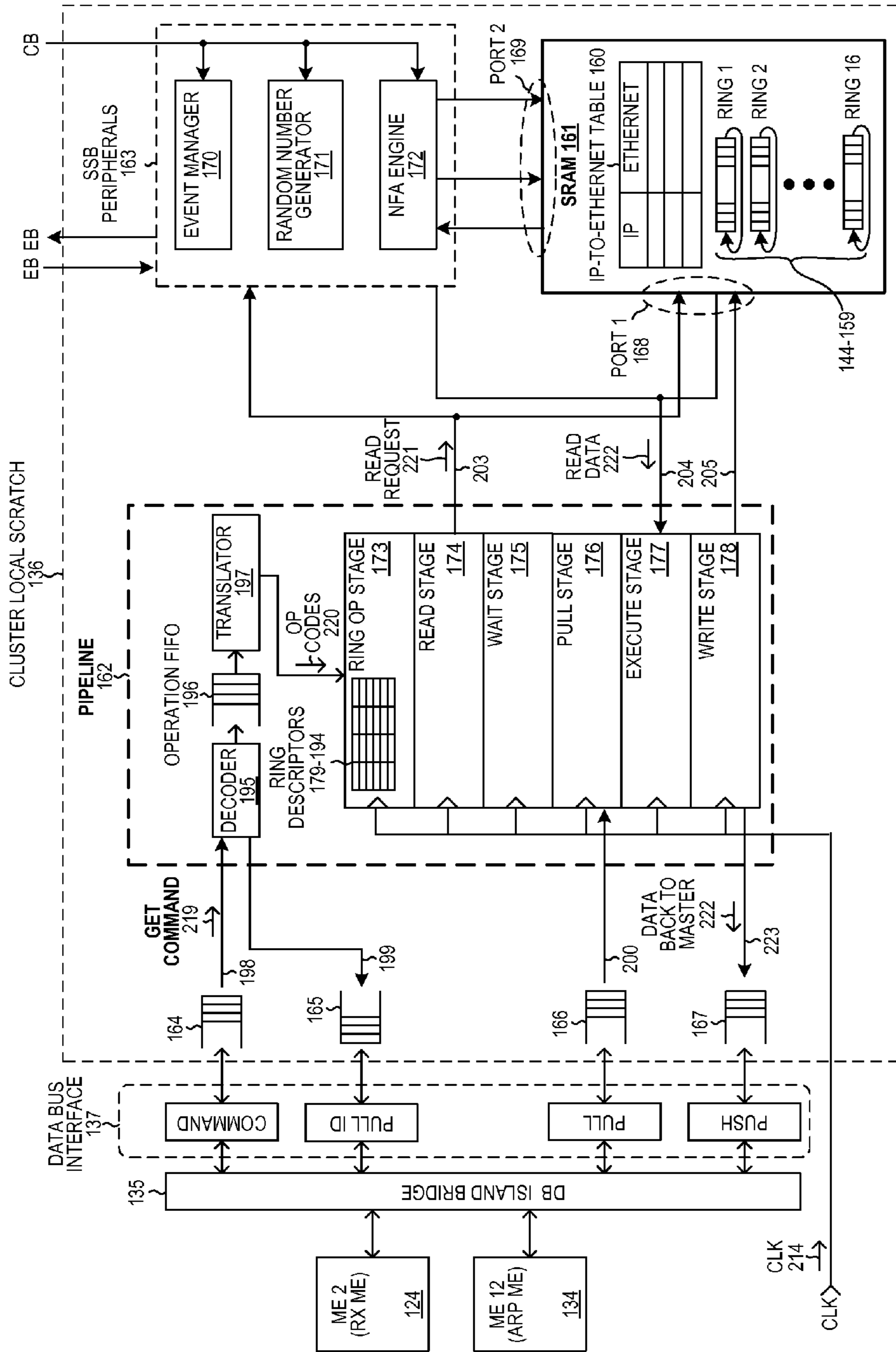
CLUSTER LOCAL SCRATCH ("GET FROM RING" EXAMPLE)
