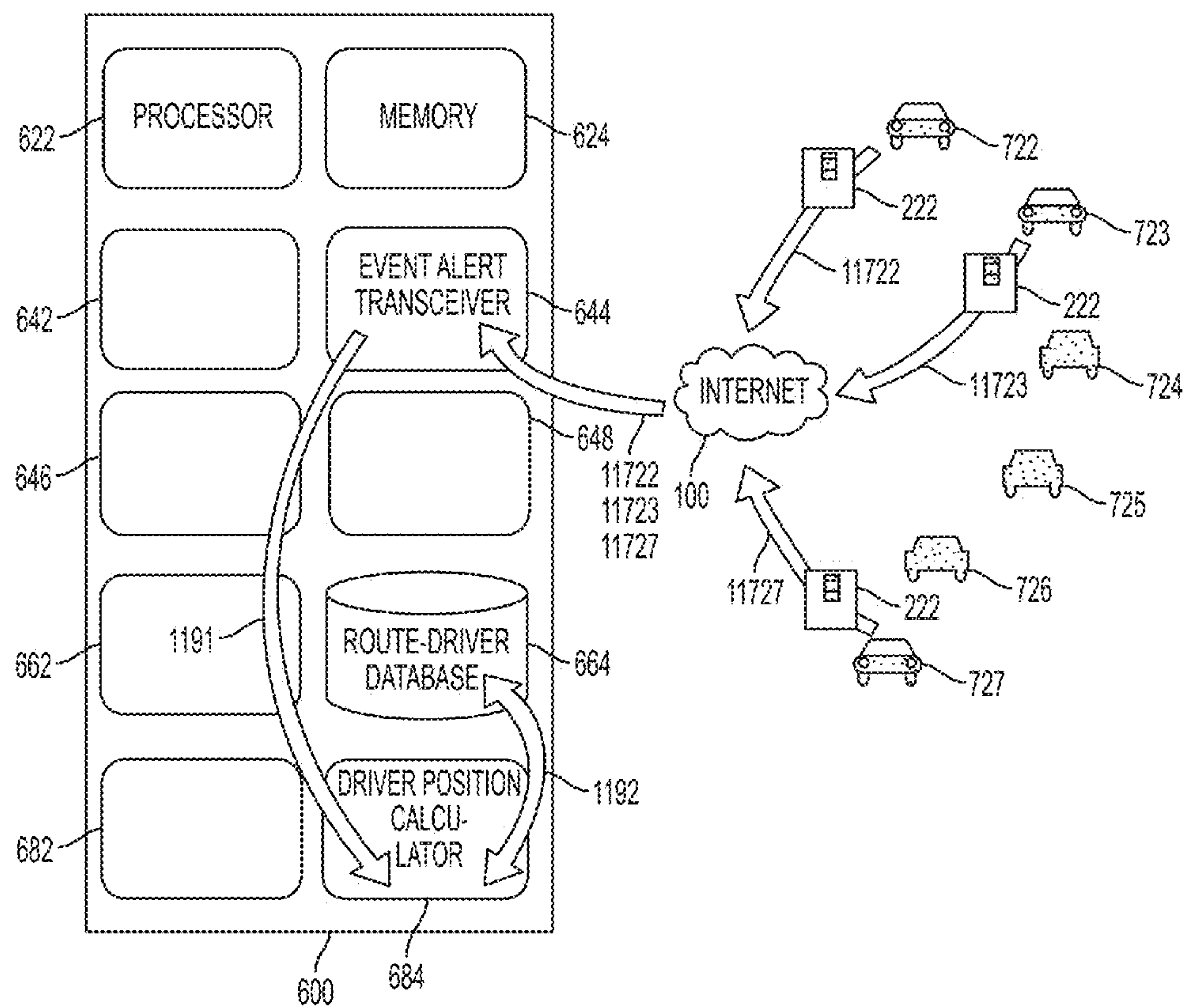
FIG. 11 PRIOR ART
