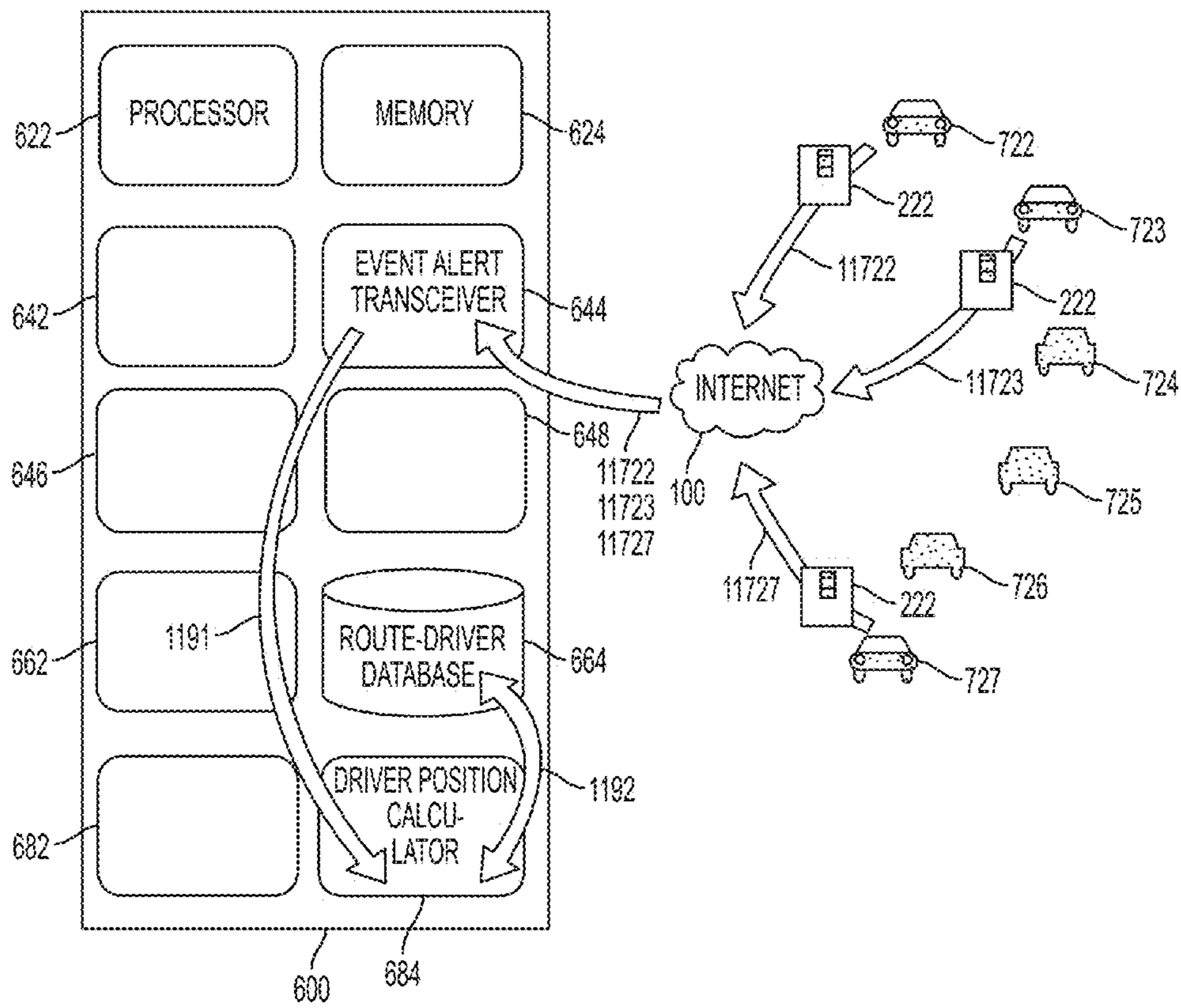
FIG. 11 PRIOR ART
