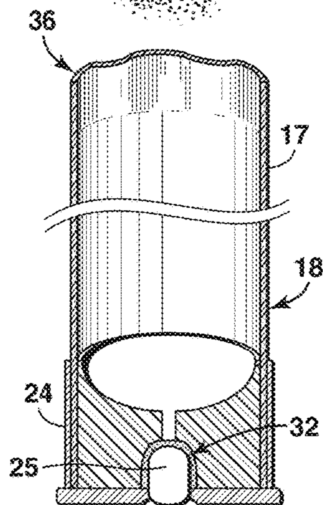
FIG. 2 (Prior Art)
