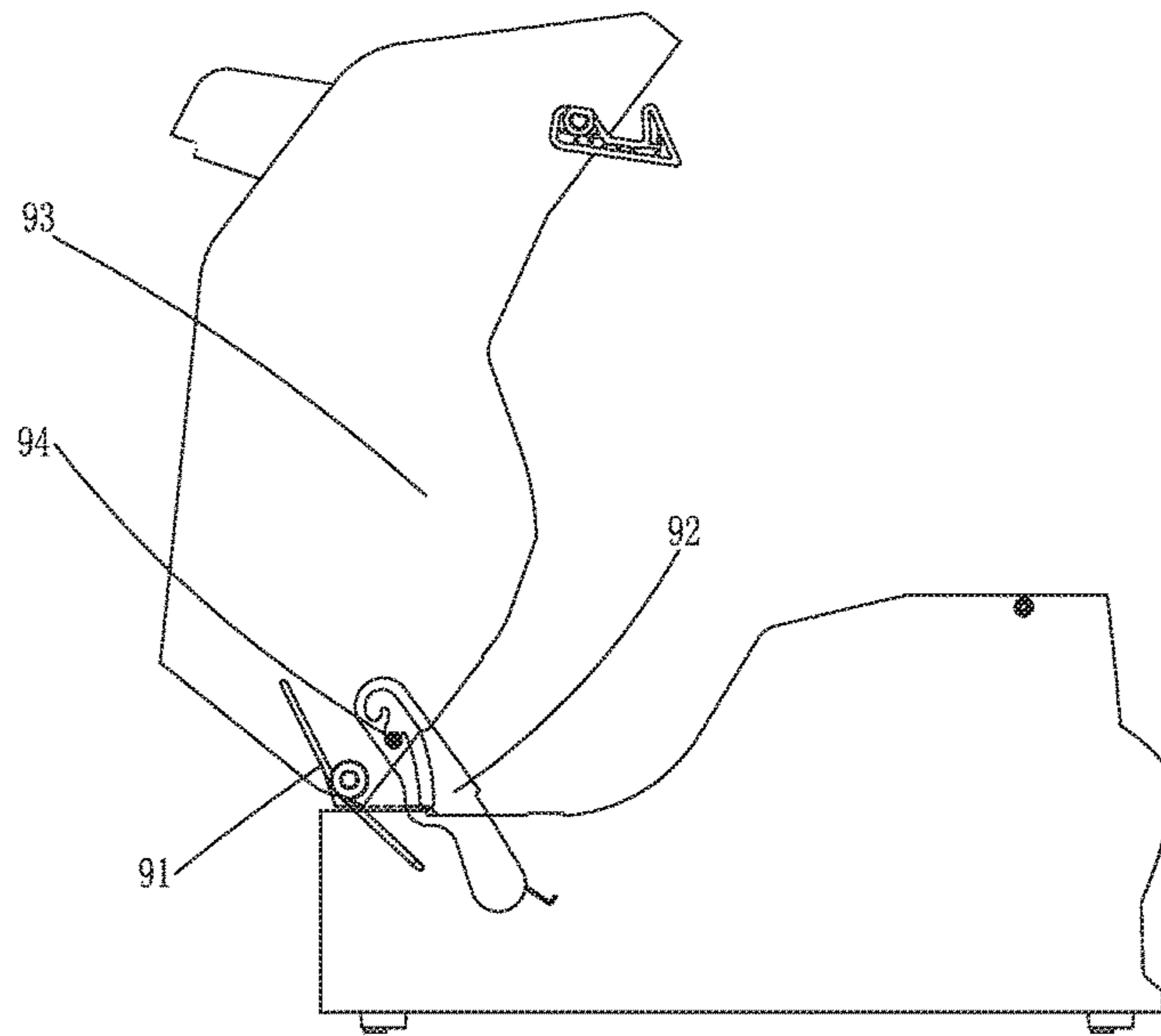
Fig. 1 Prior Art
