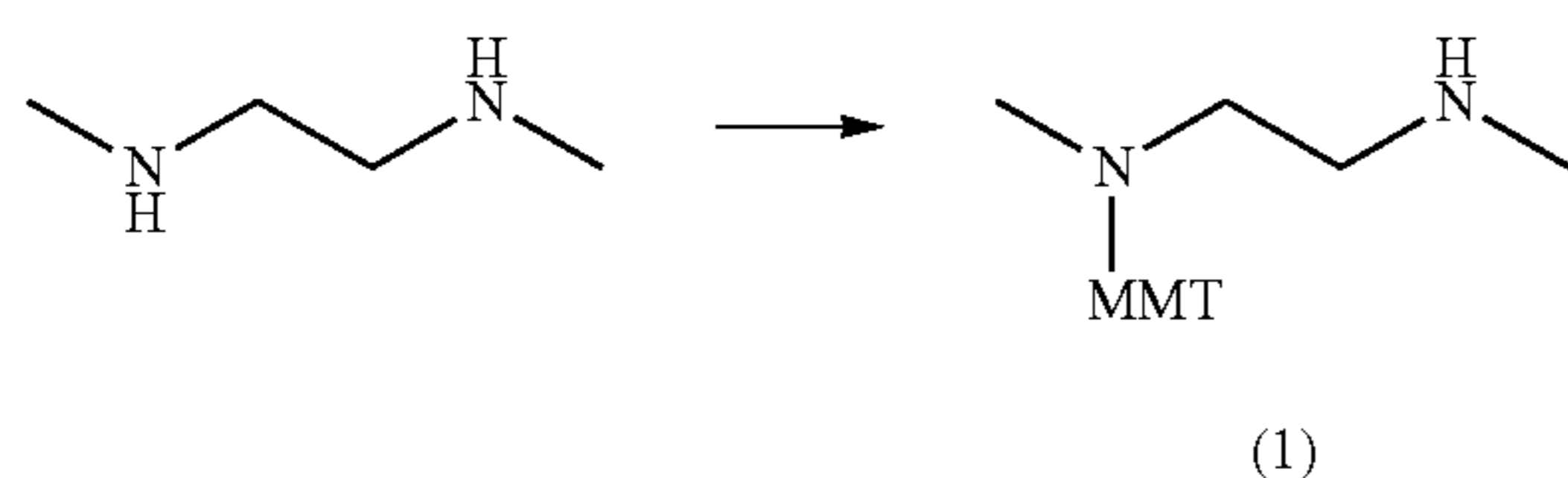
Scheme-4: Preparation of CL2E-SN-38
