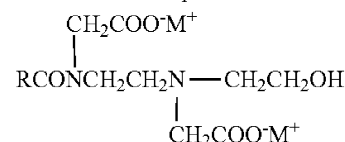
Diamphoacetate
