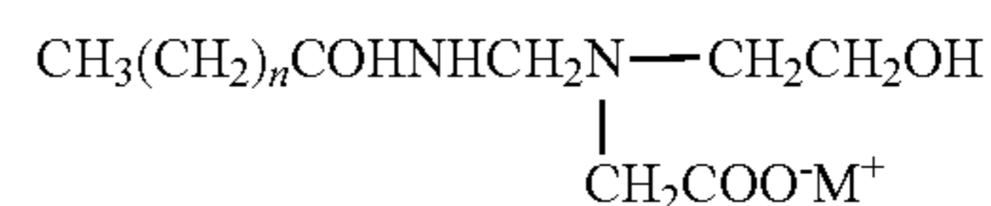
Amphoacetate
