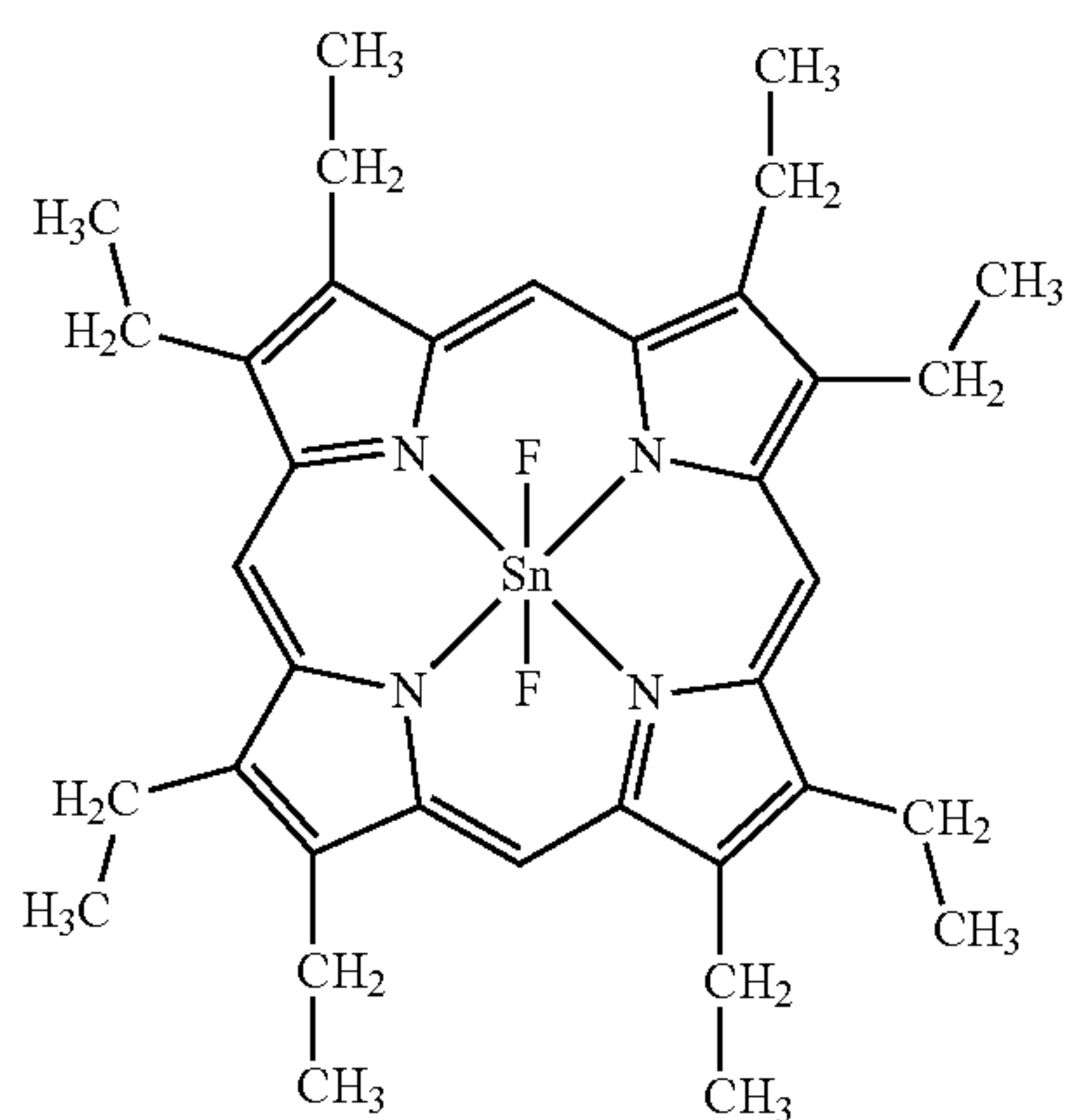
\text{SnF}_2(\text{OEP})
