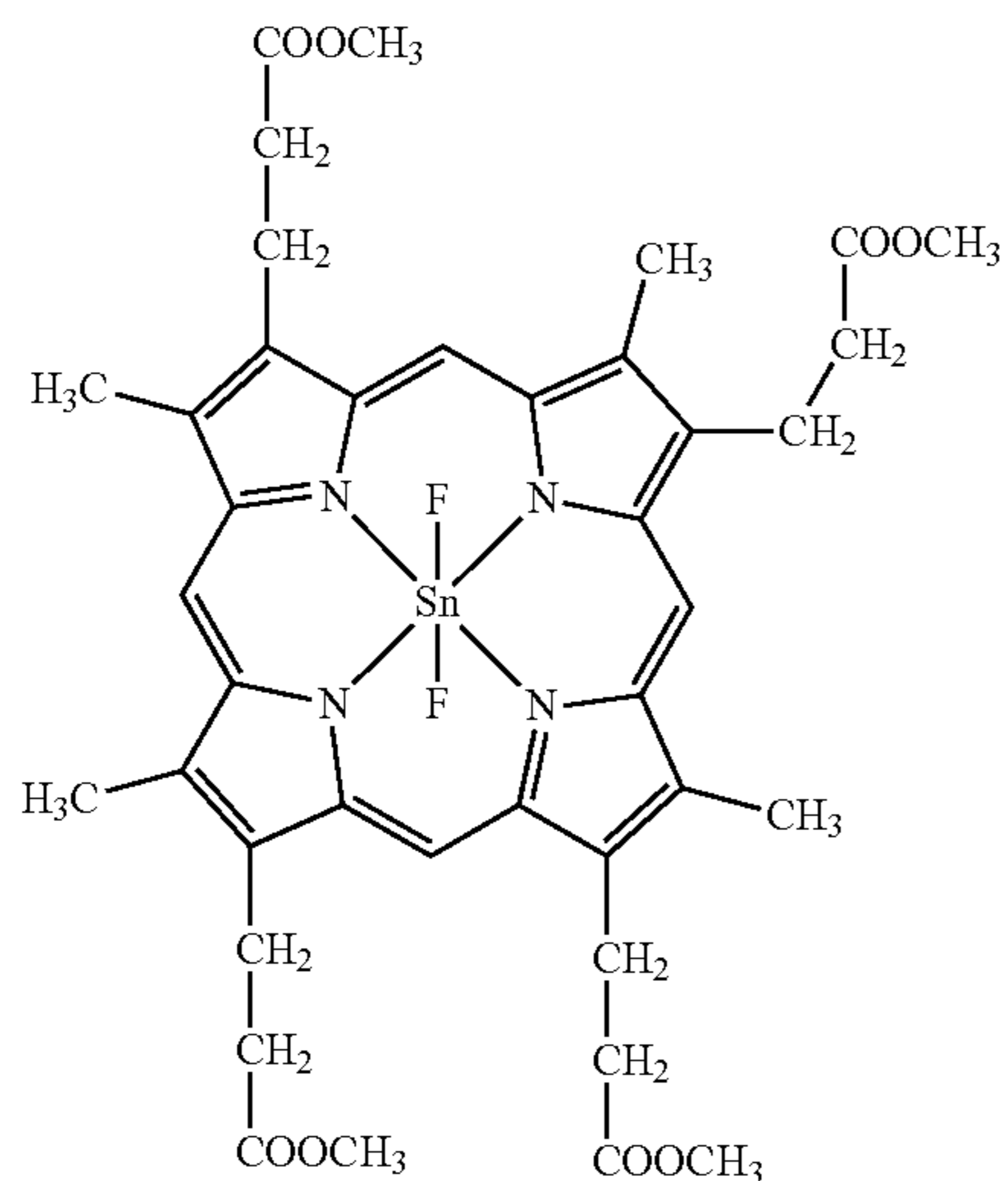
\text{SnF}_2(\text{Copro III-4Me})
