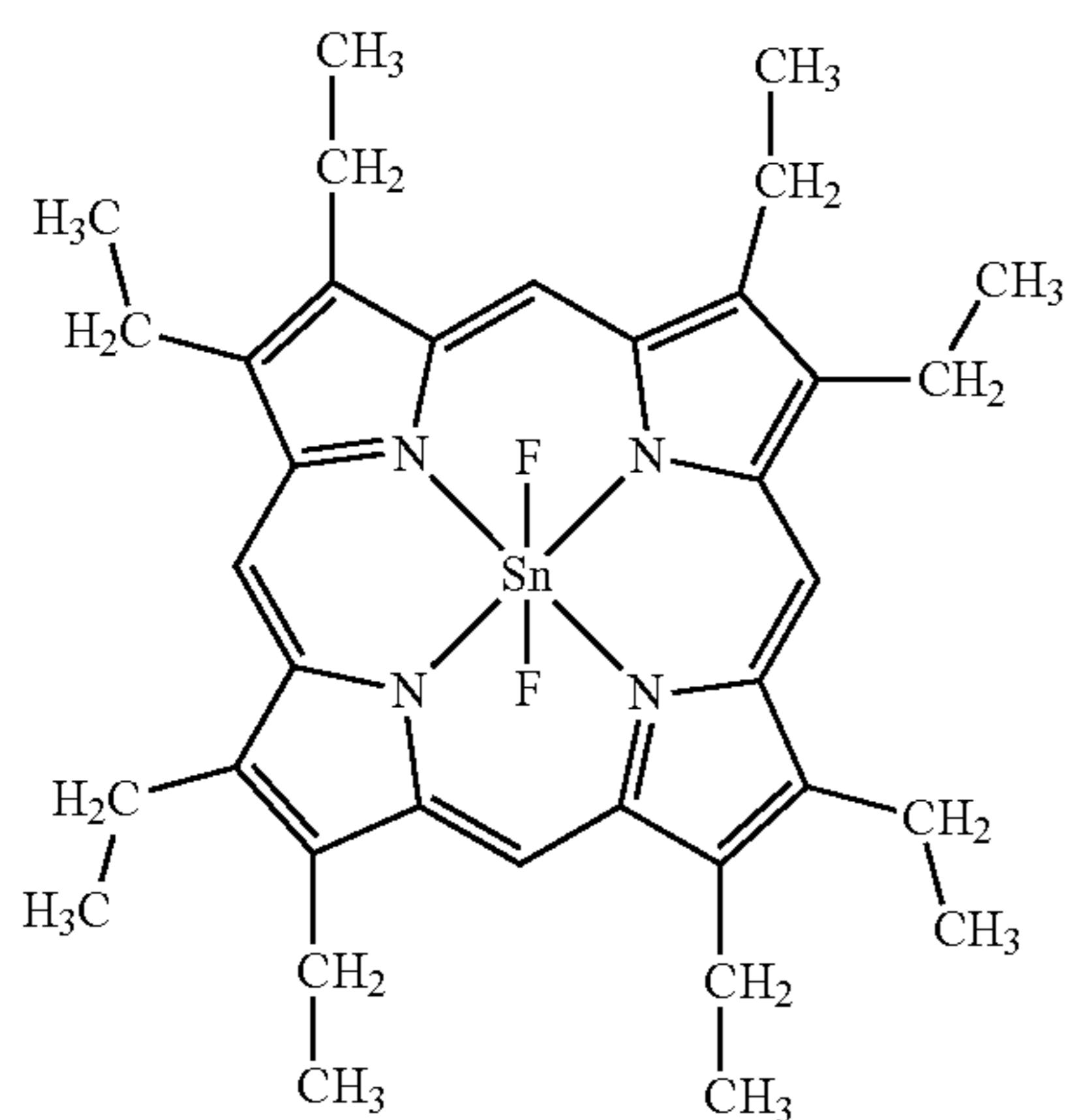
\text{SnF}_2(\text{OEP})
