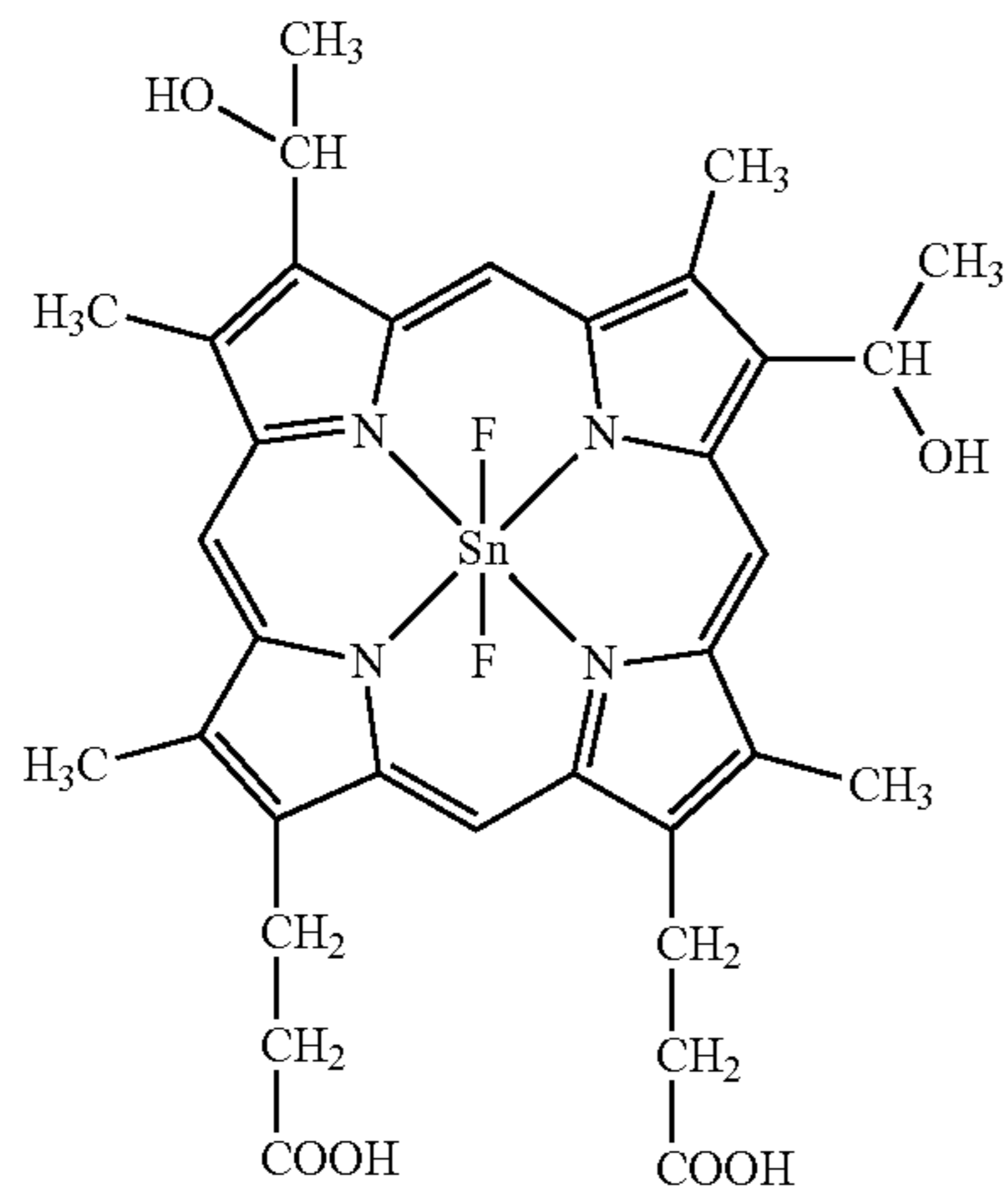
\text{SnF}_2(\text{Hemato IX})
