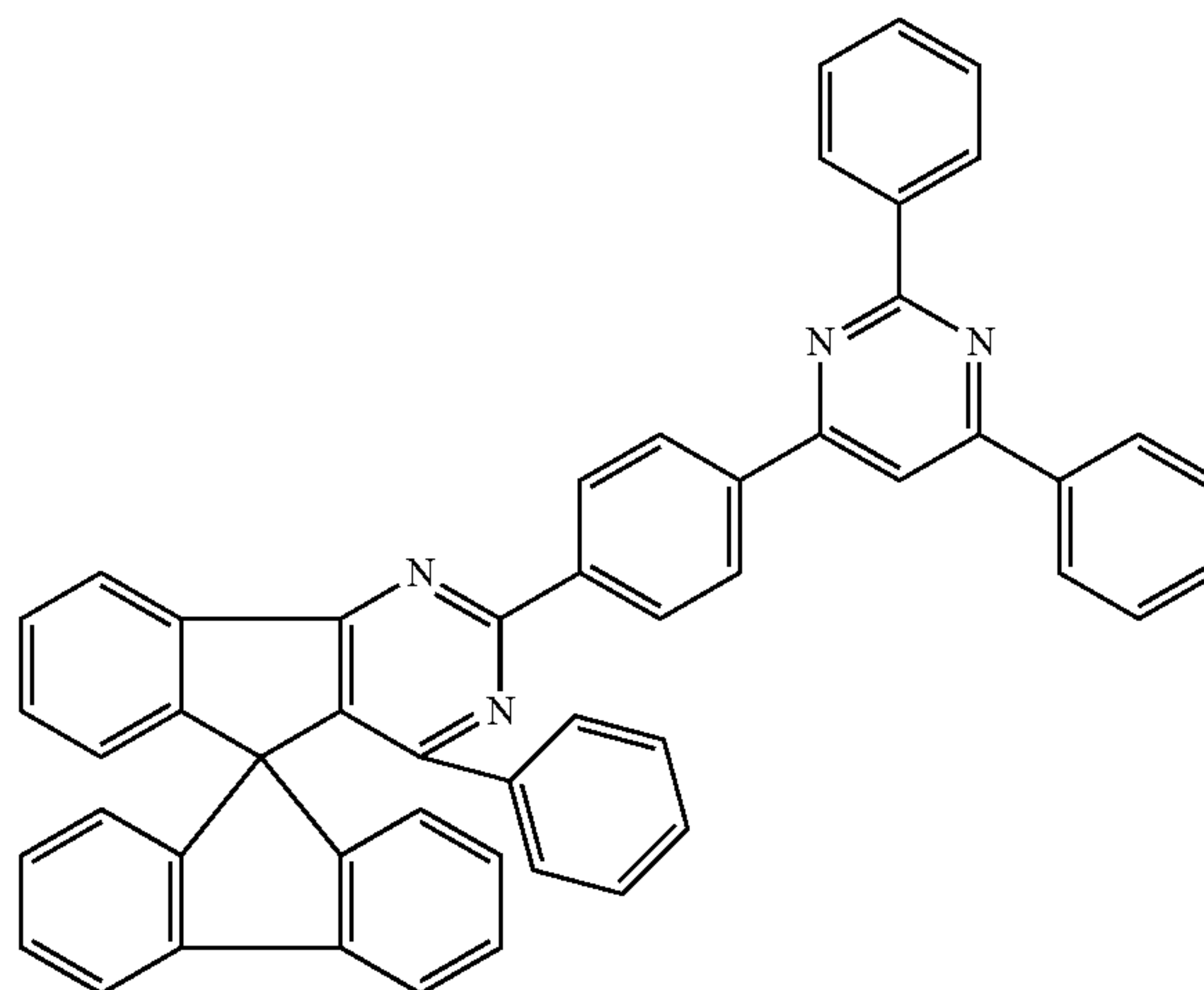
Chemical Formula 1-92
