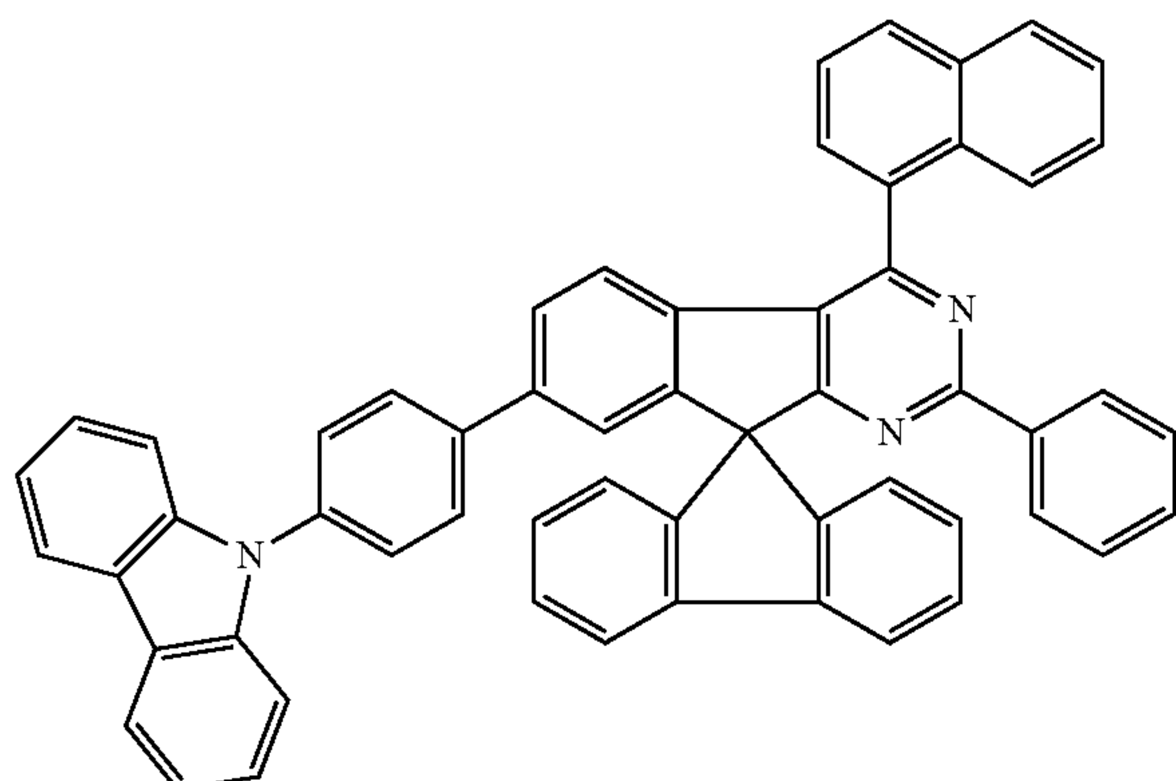
Chemical Formula 1-36
