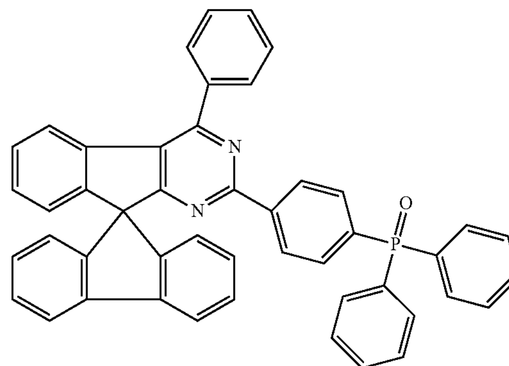
Chemical Formula 1-51
