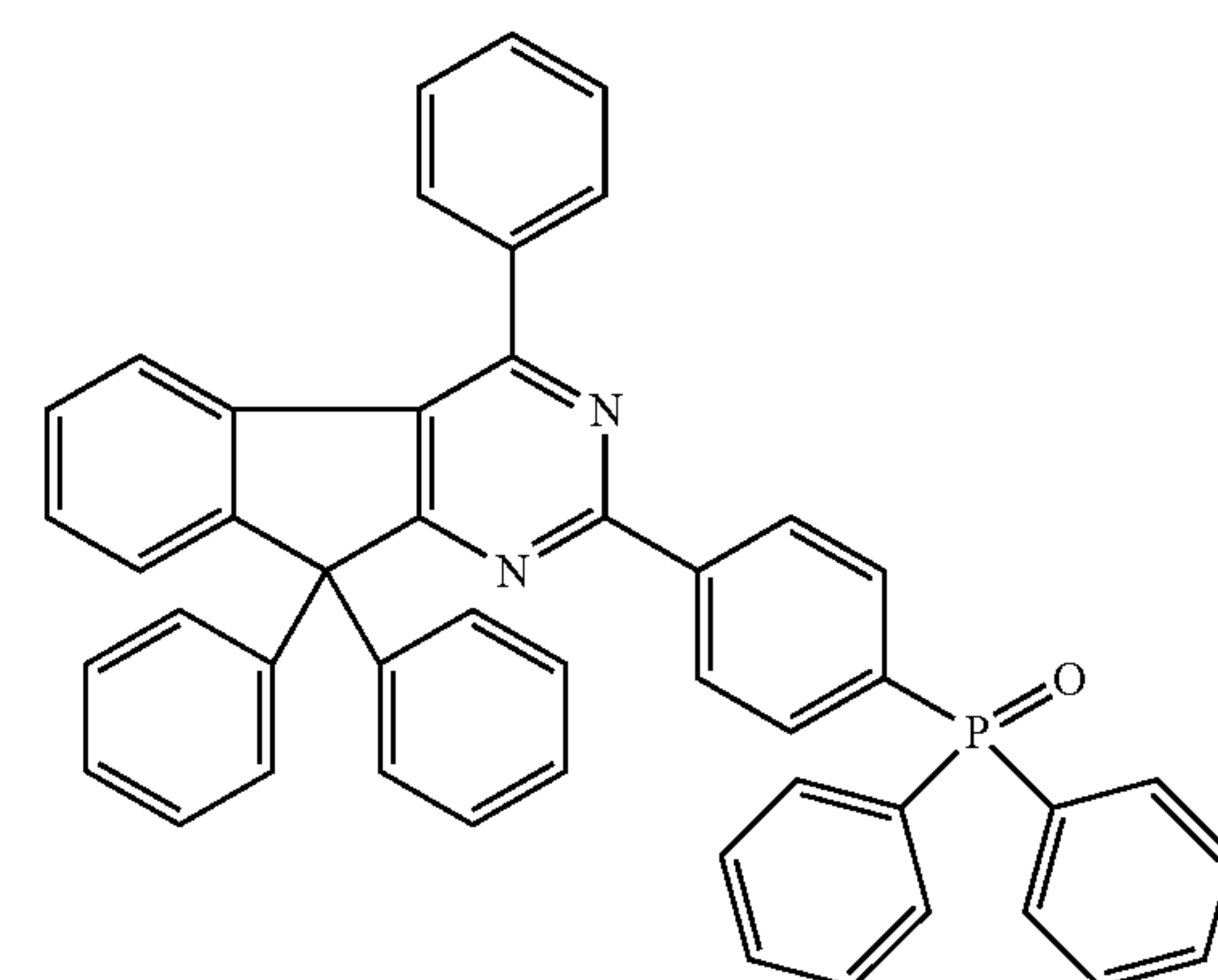
Chemical Formula 2-21
