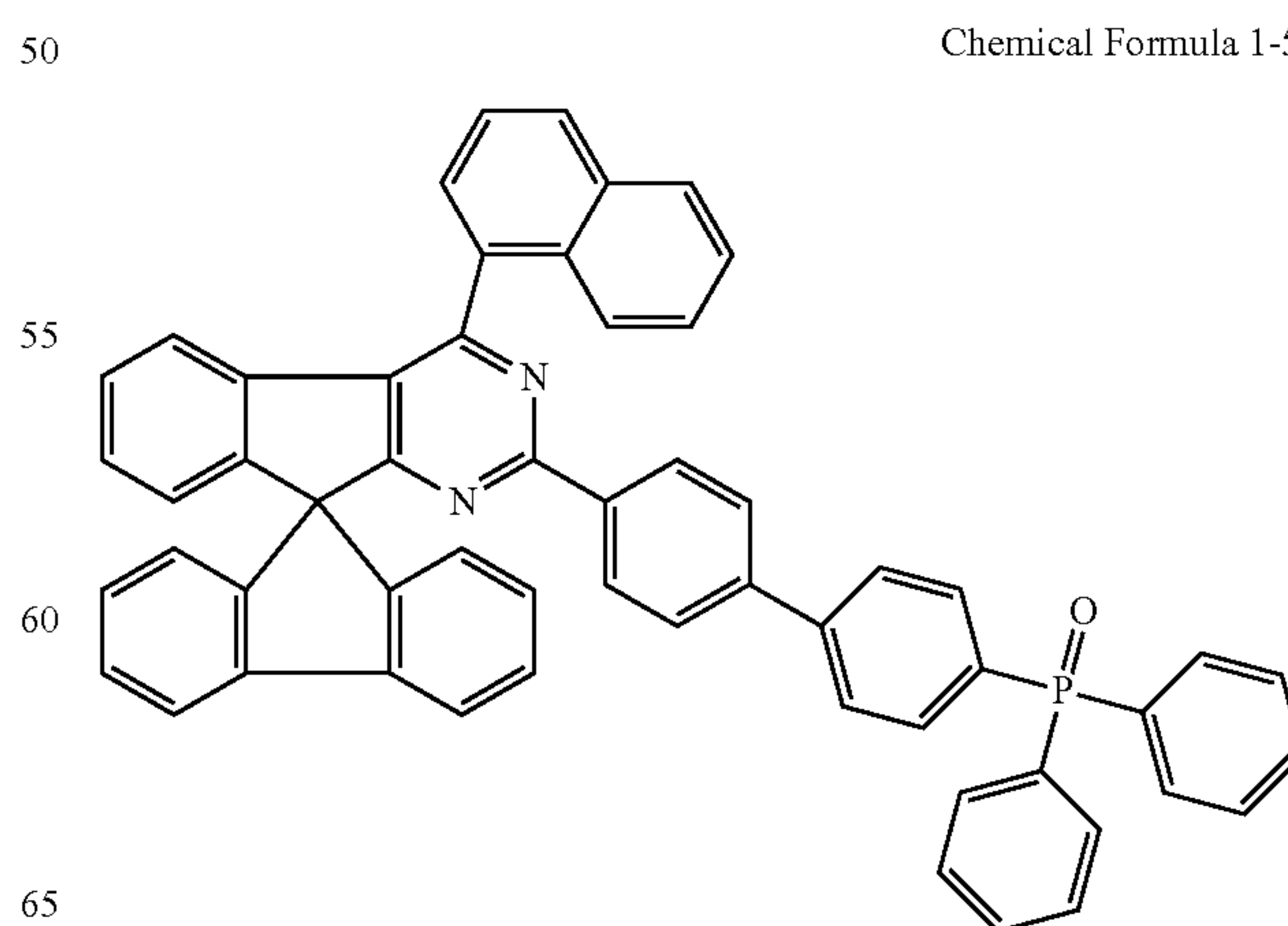
Chemical Formula 1-55
