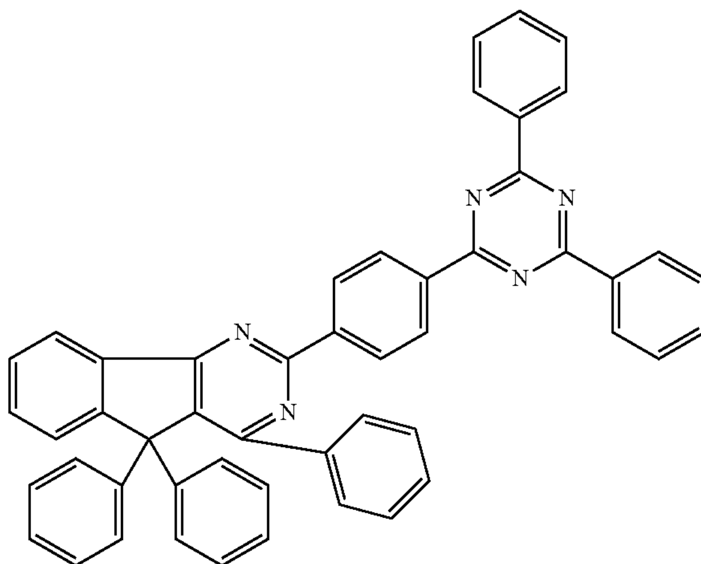
Chemical Formula 2-44
