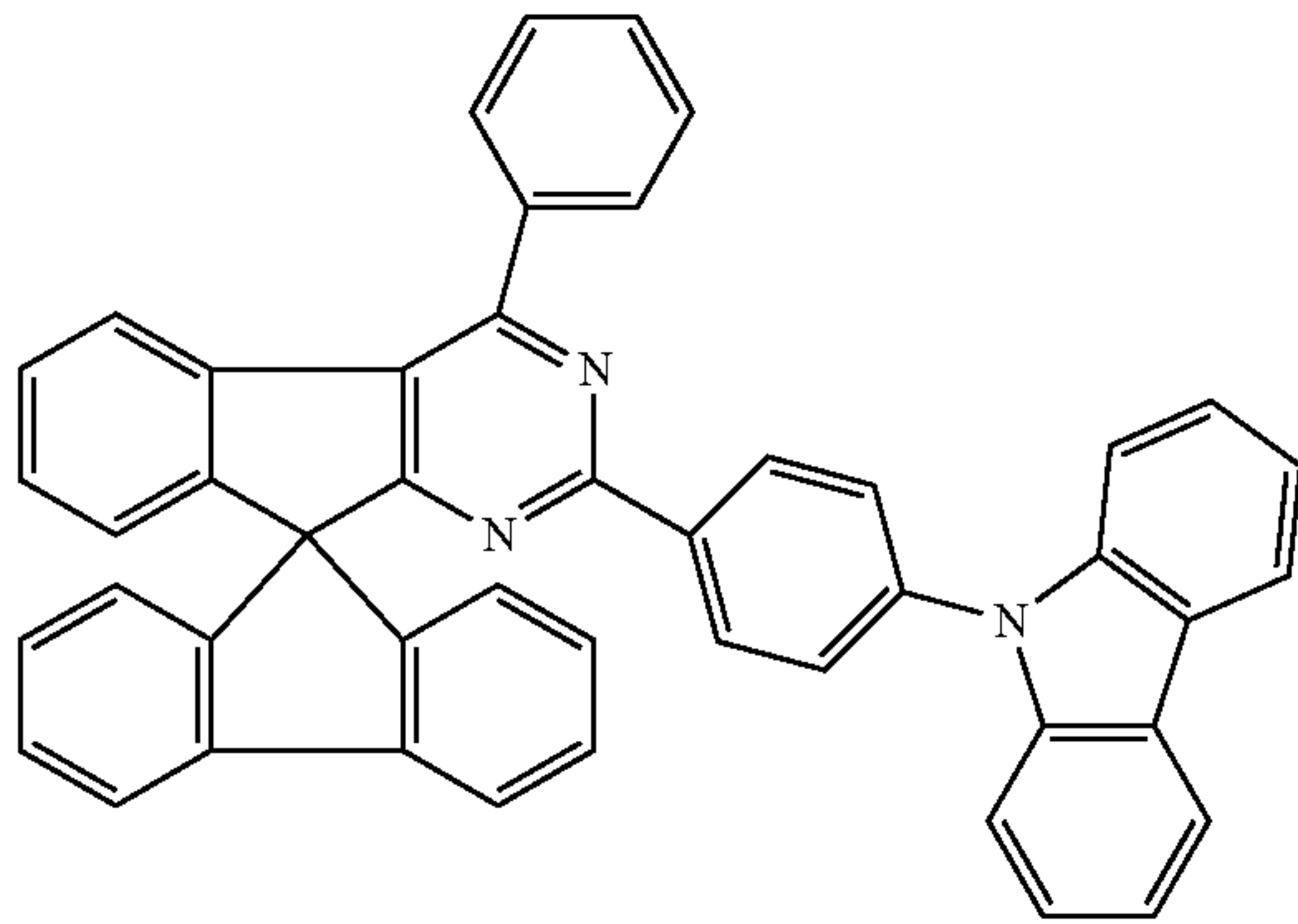
Chemical Formula 1-69
