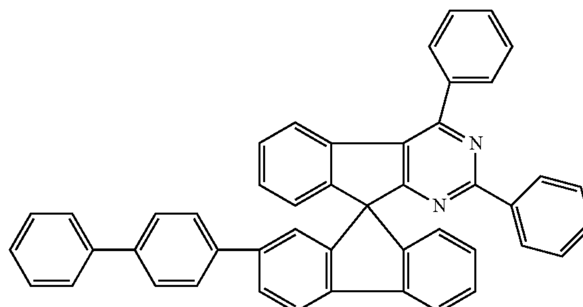
Chemical Formula 1-8
