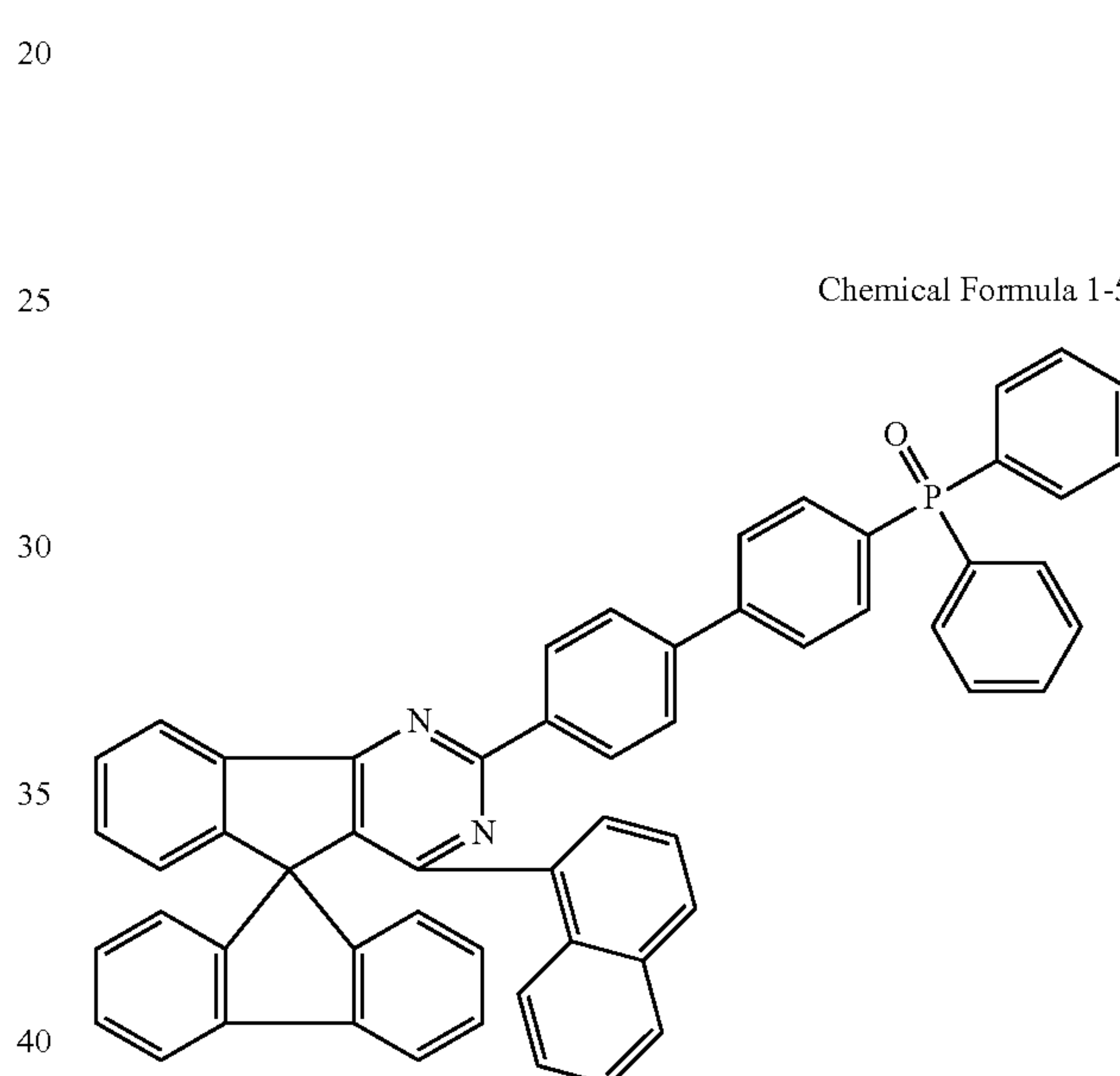
Chemical Formula 1-54
