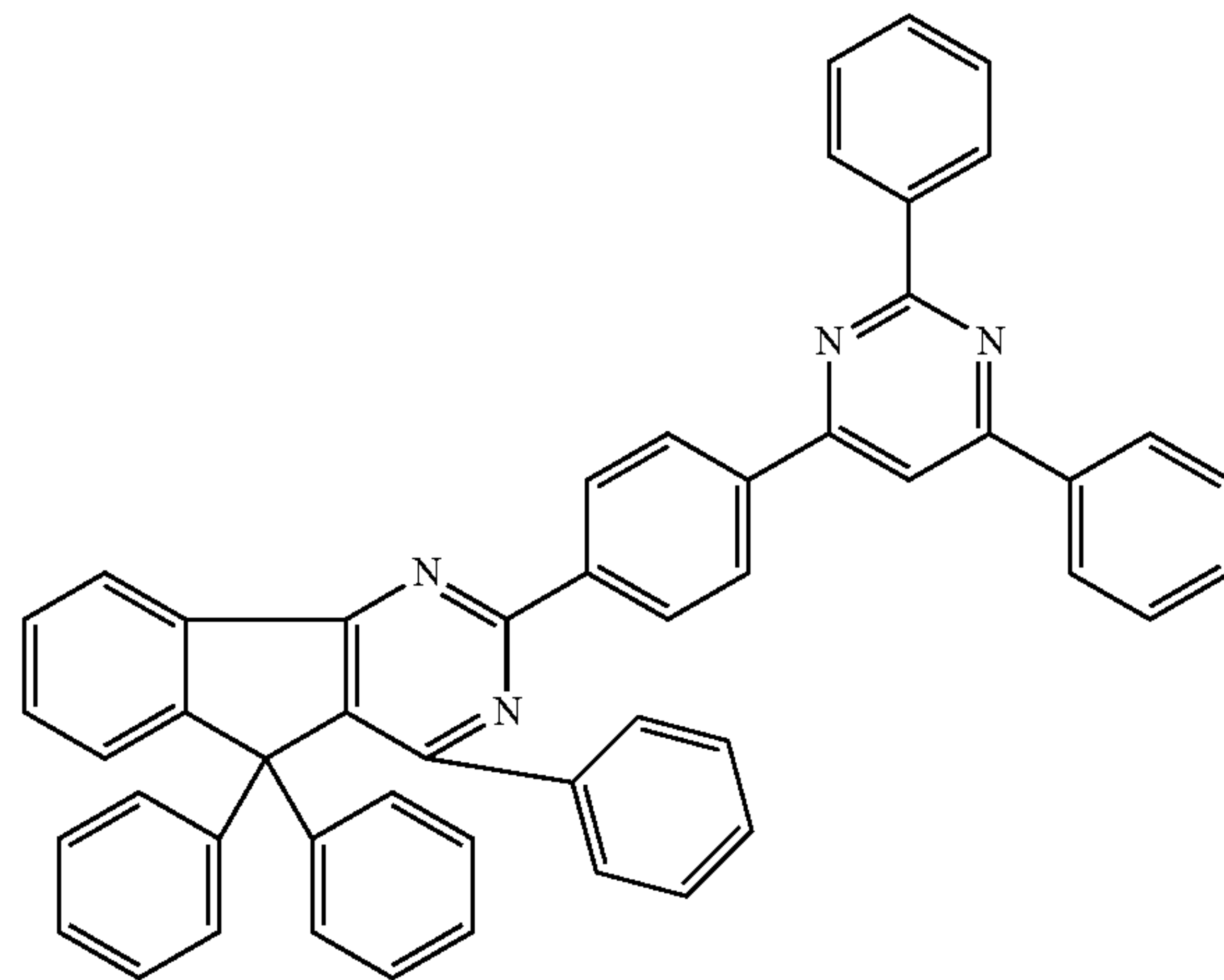
Chemical Formula 2-47
