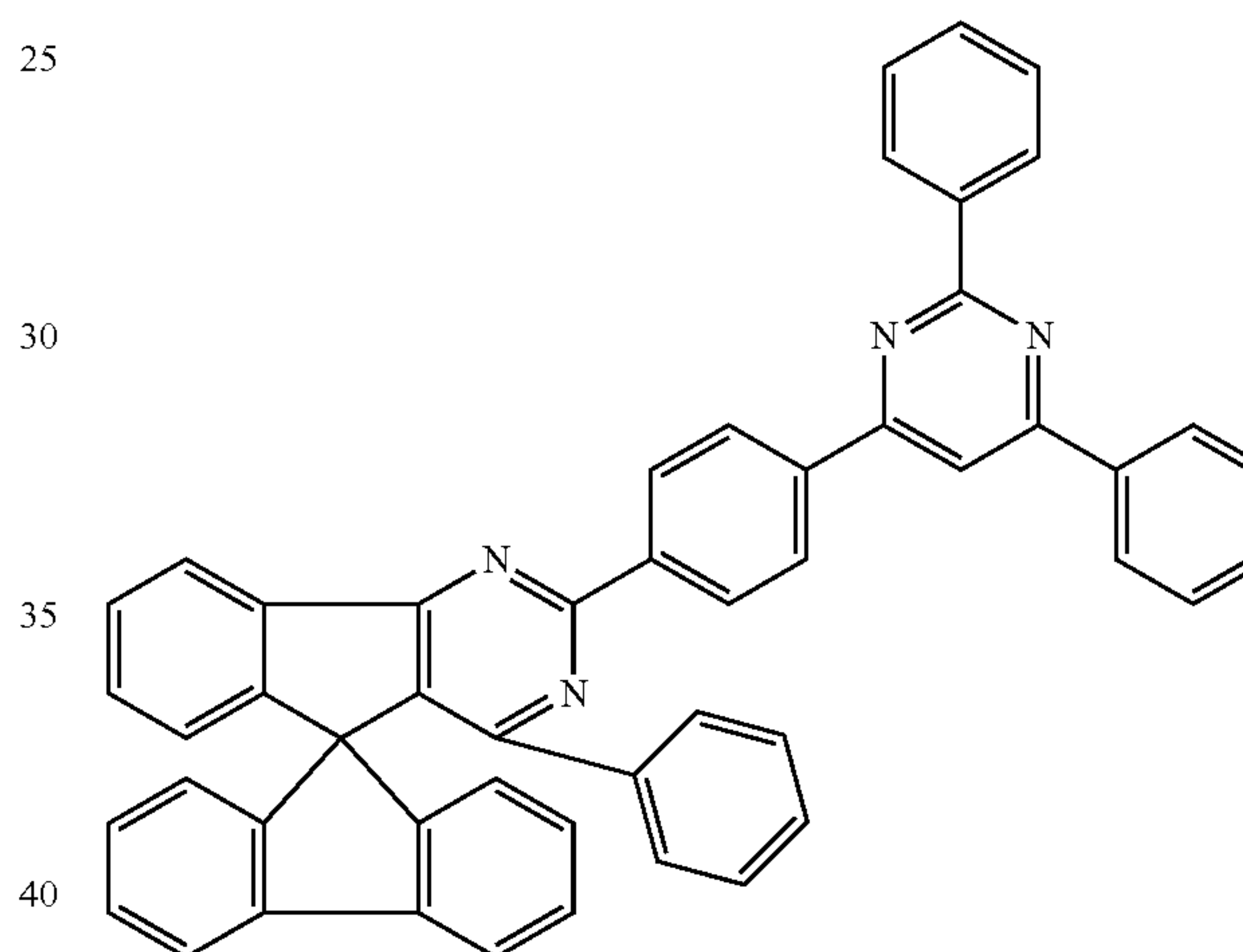
Chemical Formula 1-92
