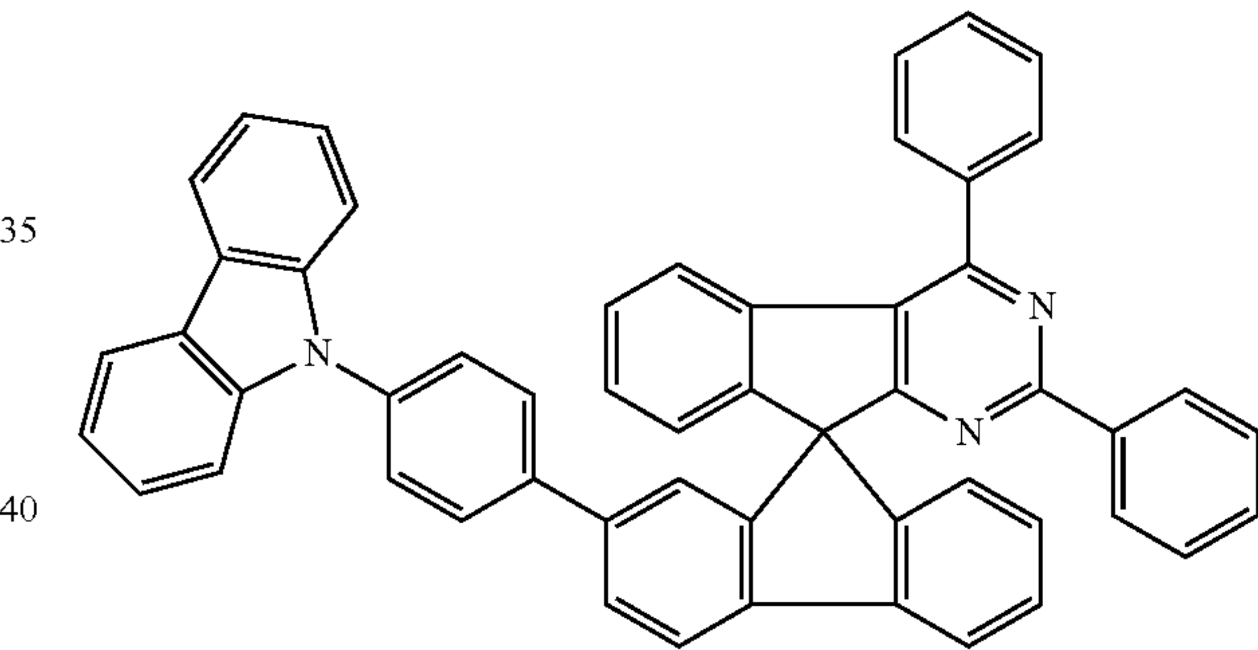
Chemical Formula 1-16
