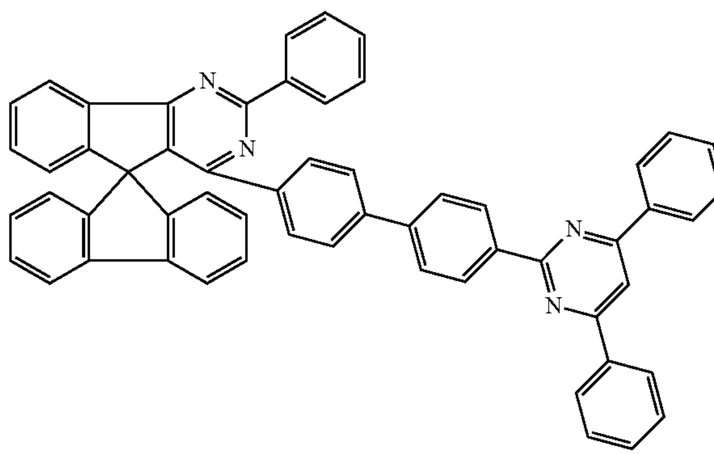
Chemical Formula 1-99
