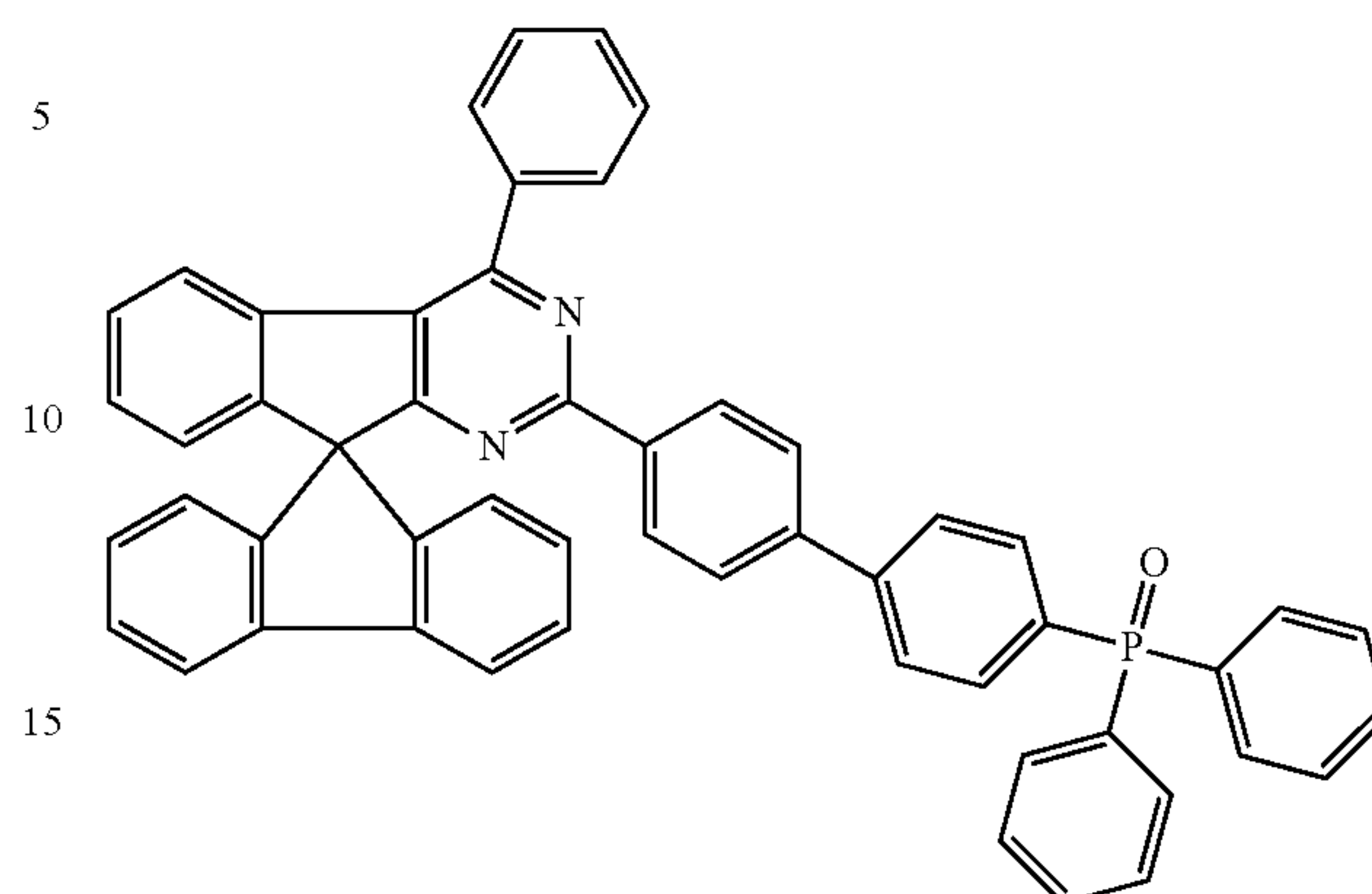
Chemical Formula 1-56
