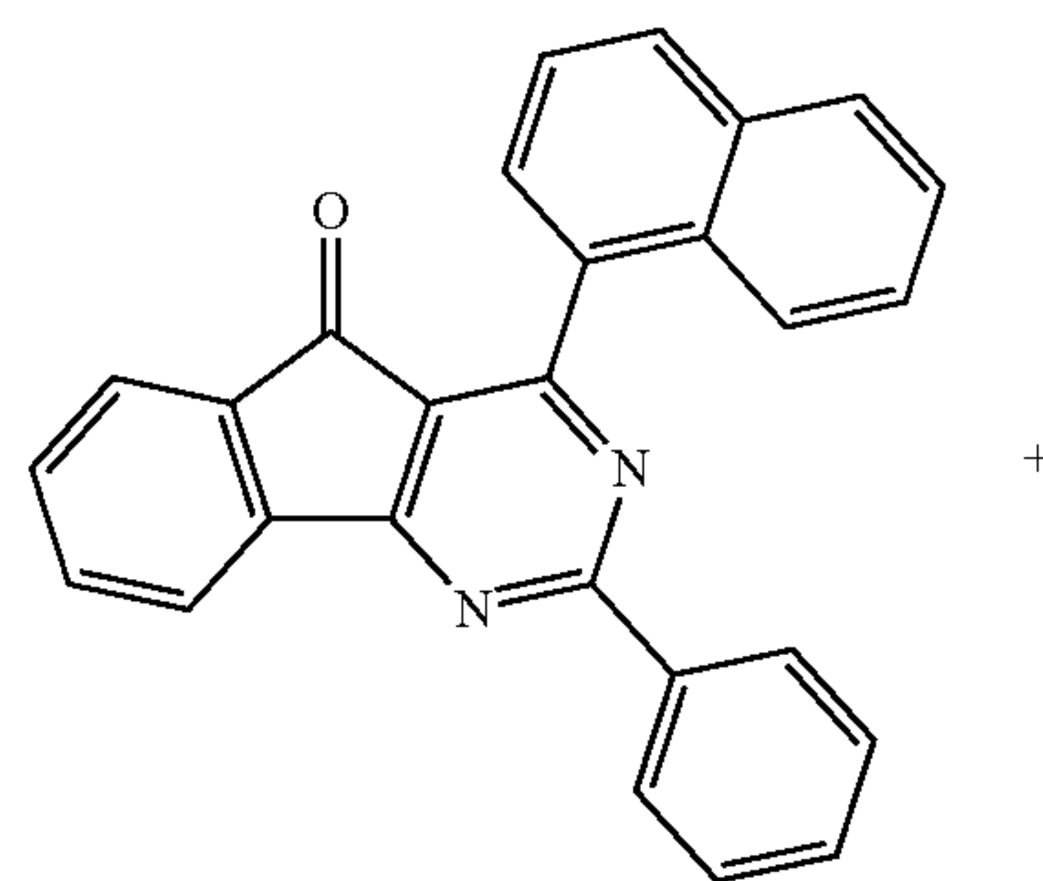
[Compound D]
