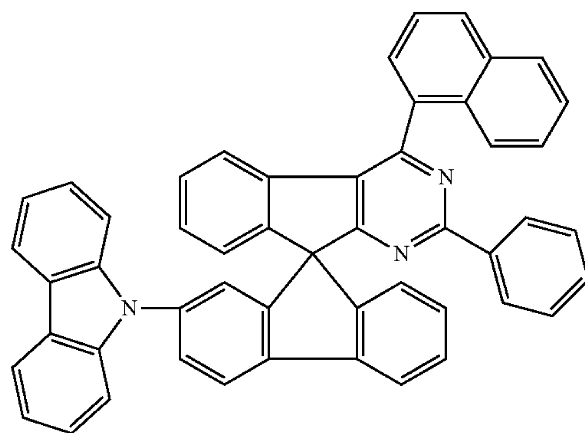
Chemical Formula 1-30
