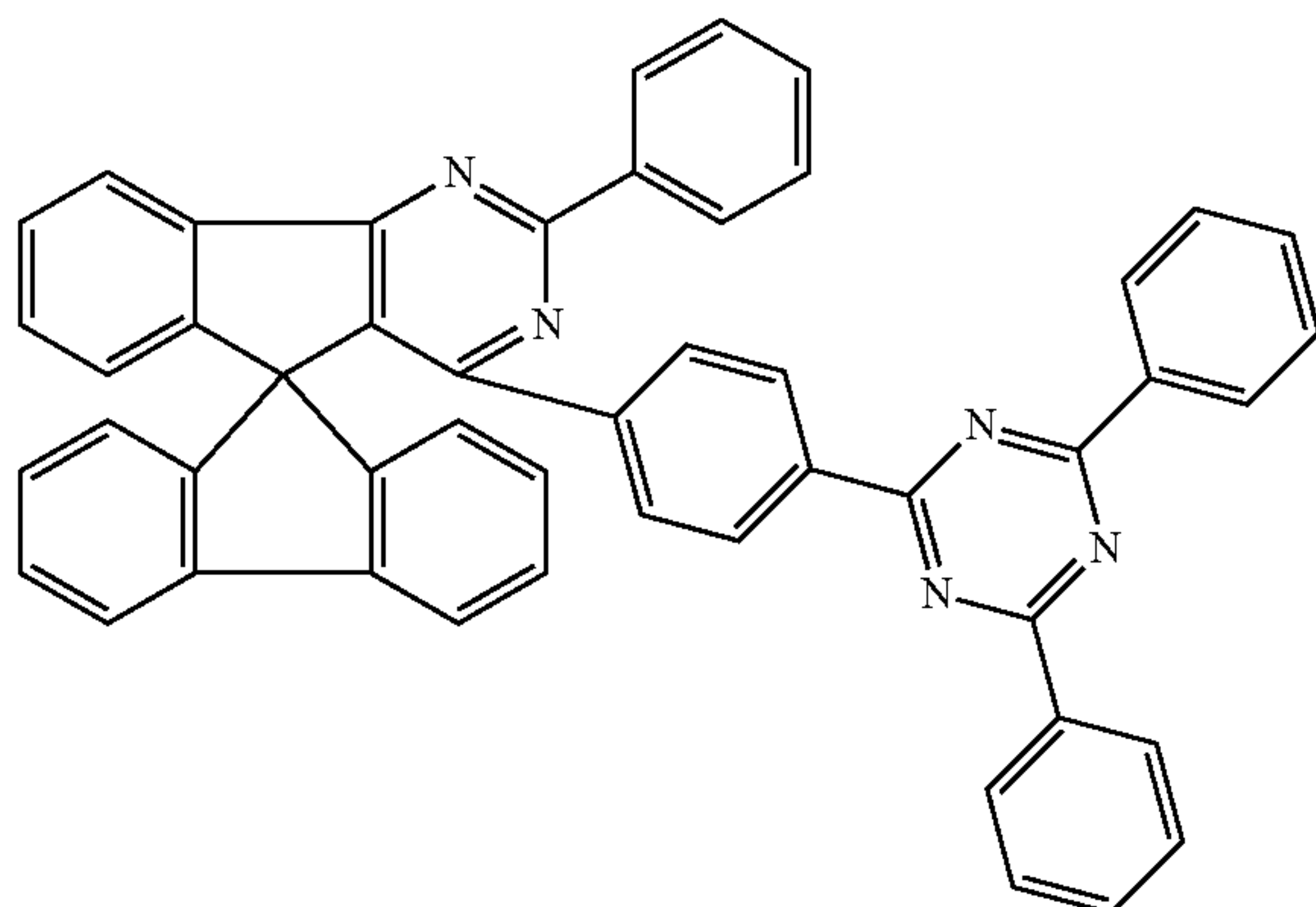
Chemical Formula 1-90
