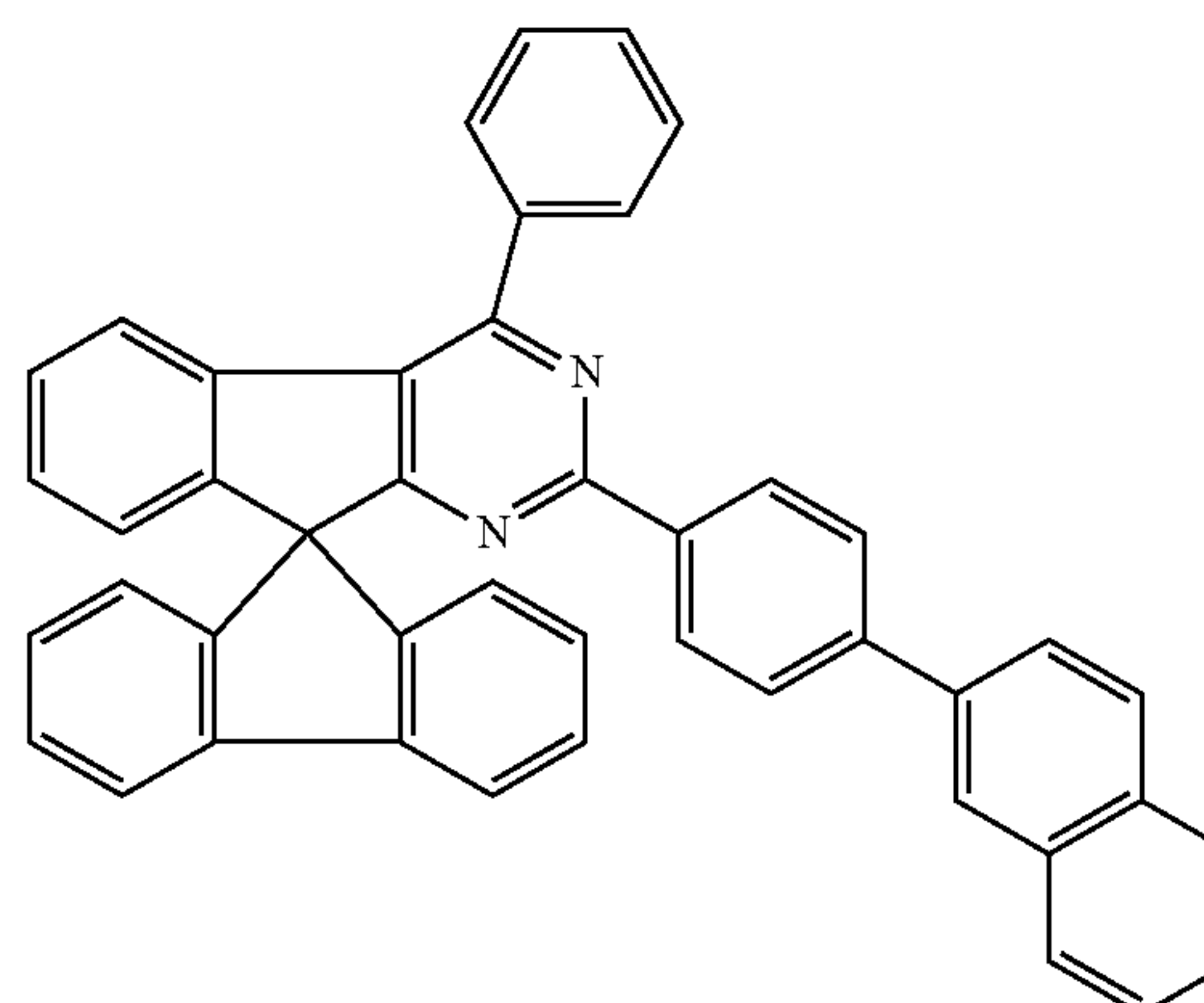
Chemical Formula 1-65
