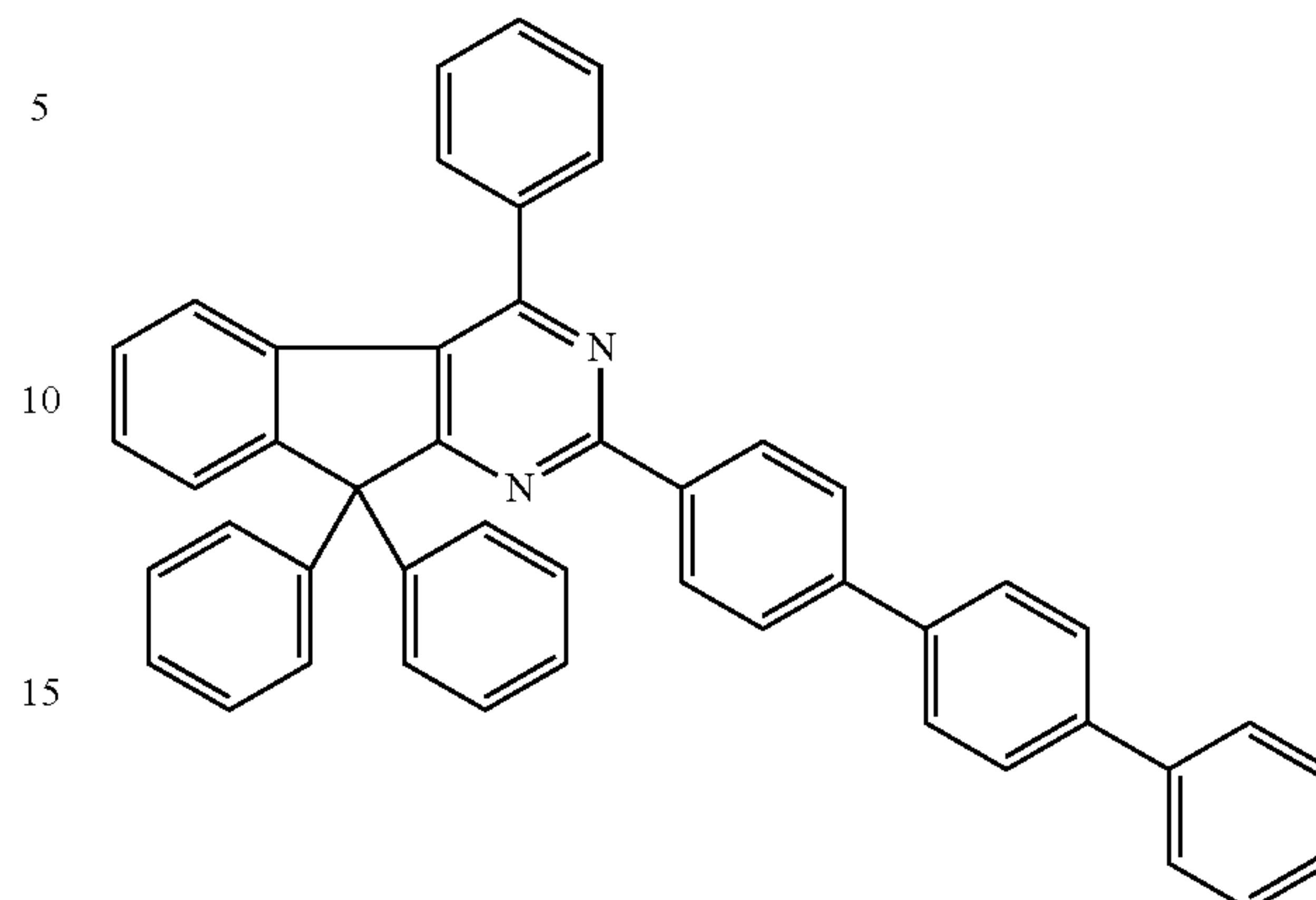
Chemical Formula 2-26
