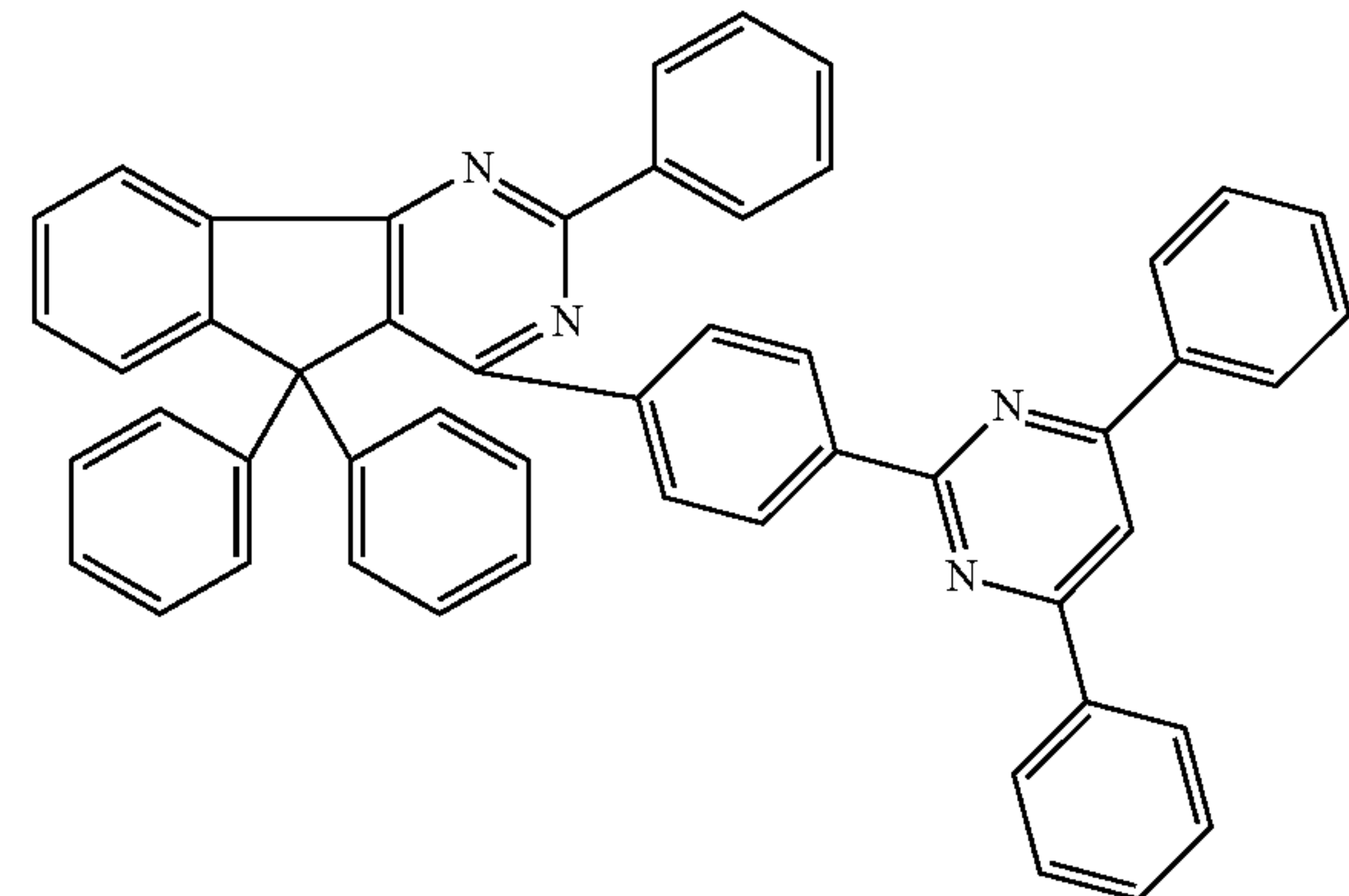
Chemical Formula 2-48
