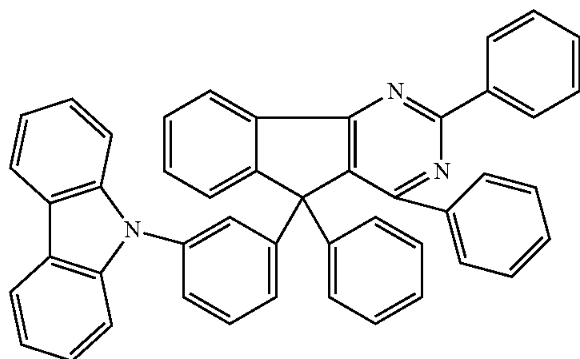
Chemical Formula 2-3
