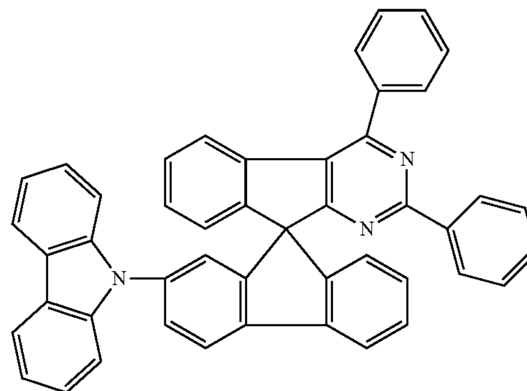
Chemical Formula 1-4
