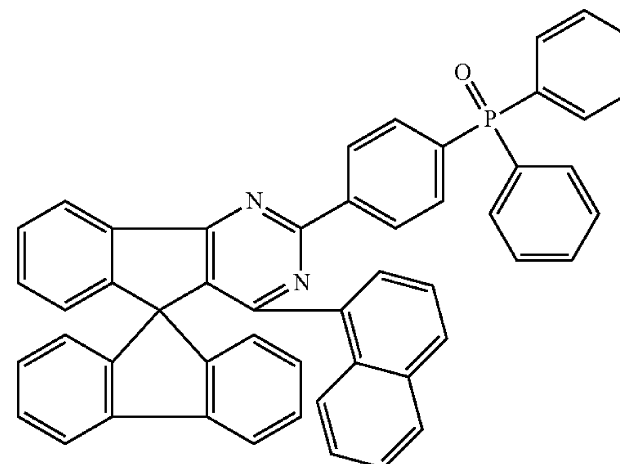
Chemical Formula 1-51
