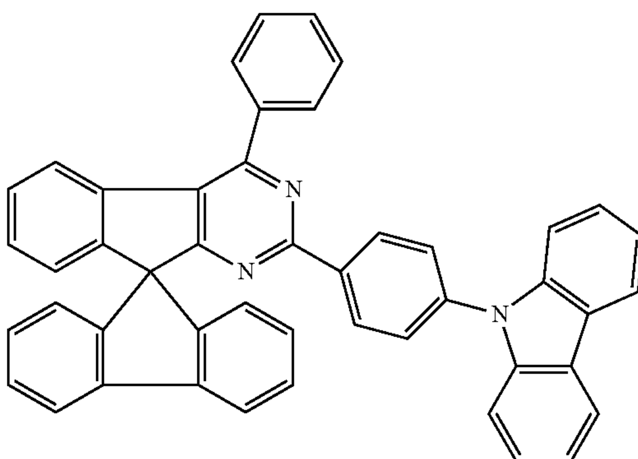
Chemical Formula 1-68
