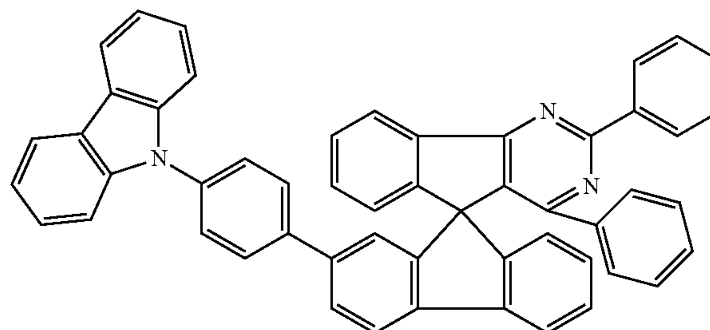
Chemical Formula 1-16
