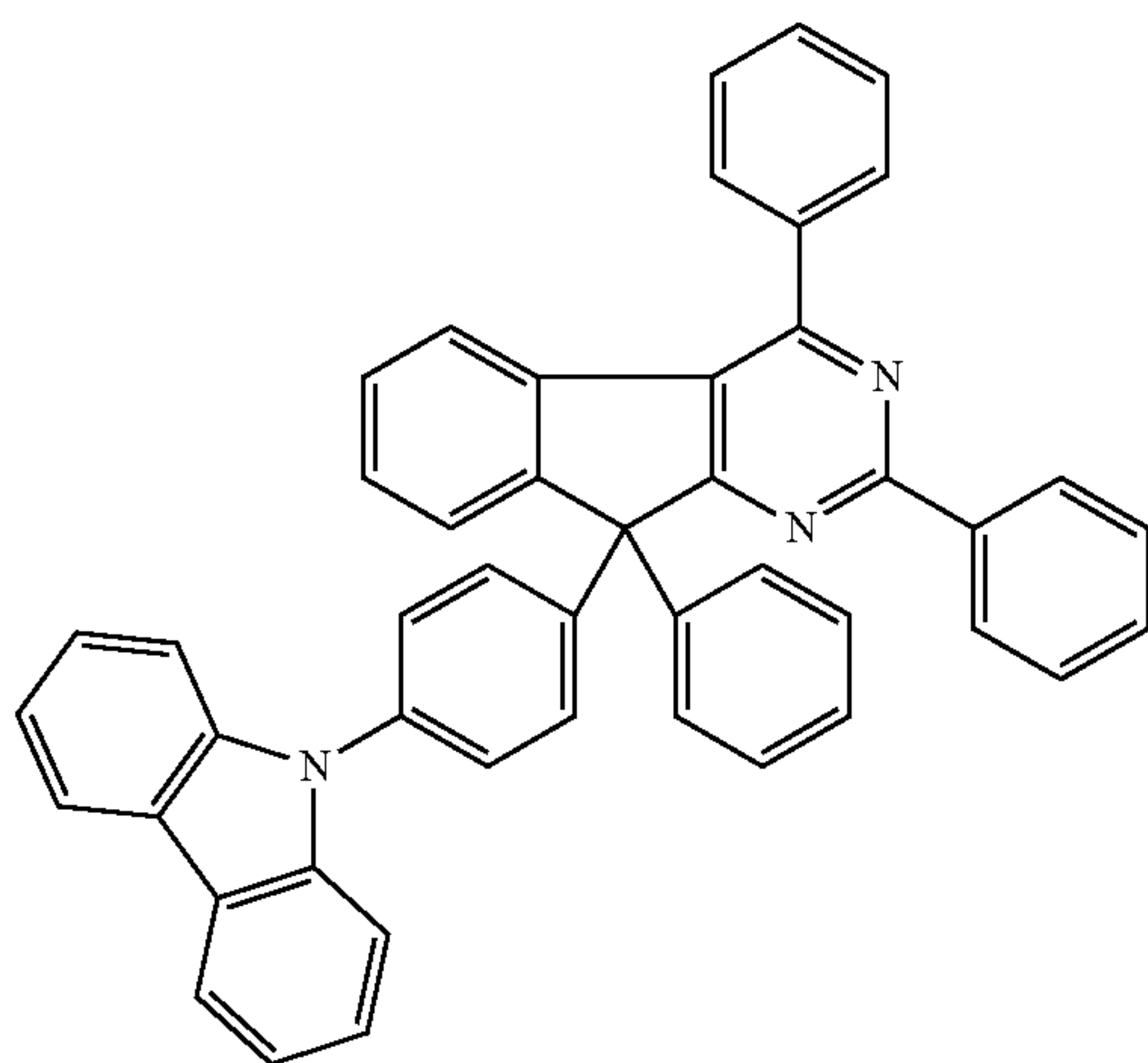
Chemical Formula 2-11
