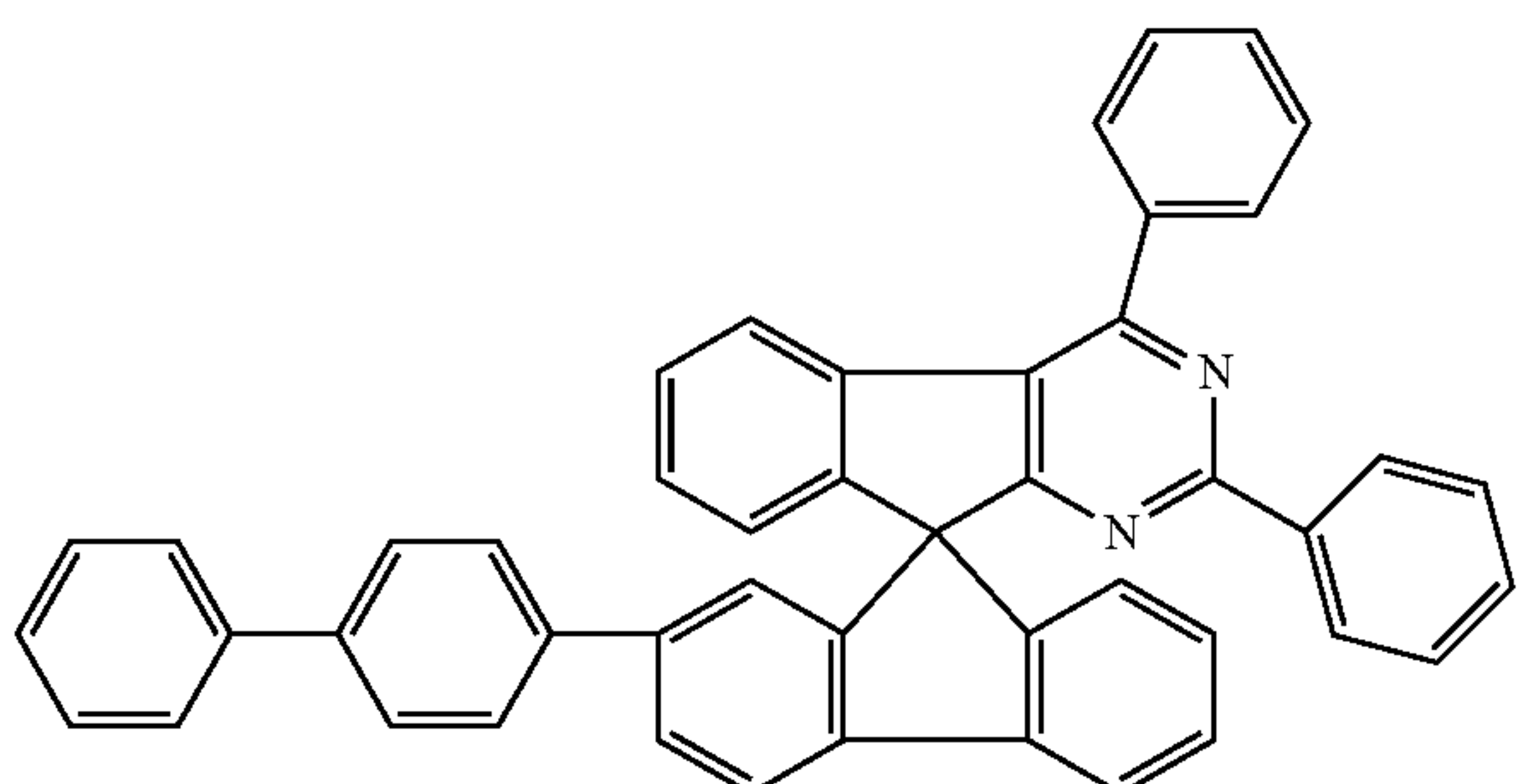
Chemical Formula 1-9
