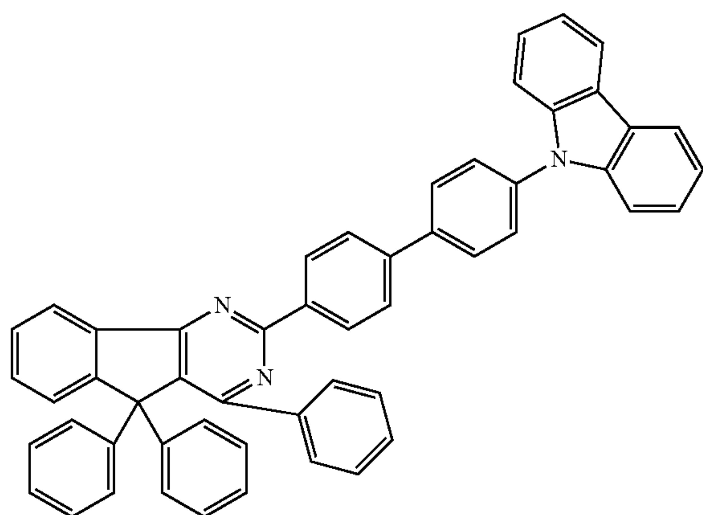
Chemical Formula 2-31
