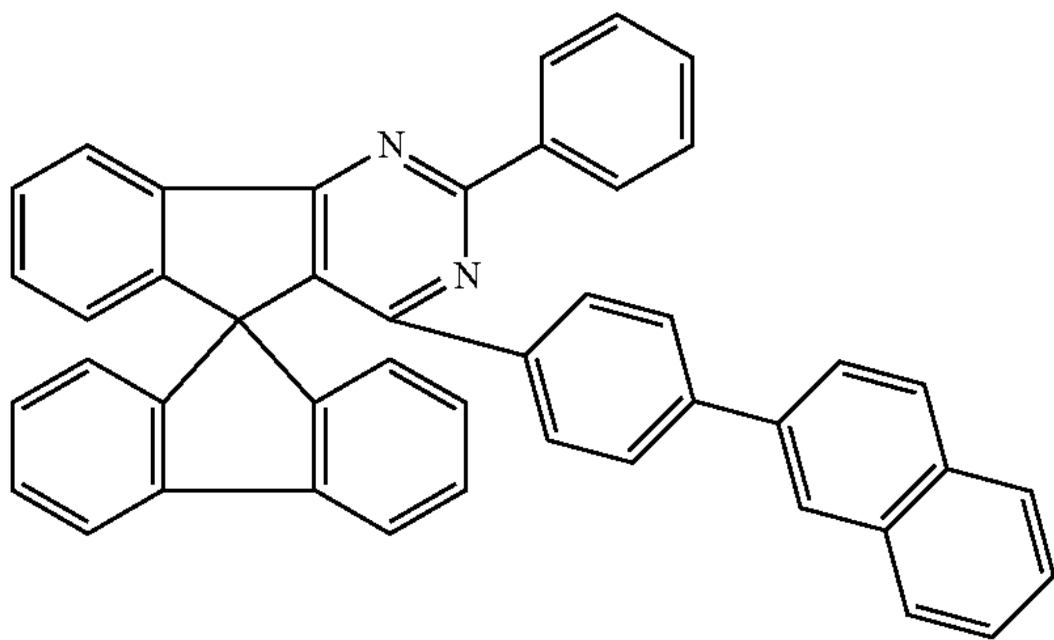
Chemical Formula 1-83
