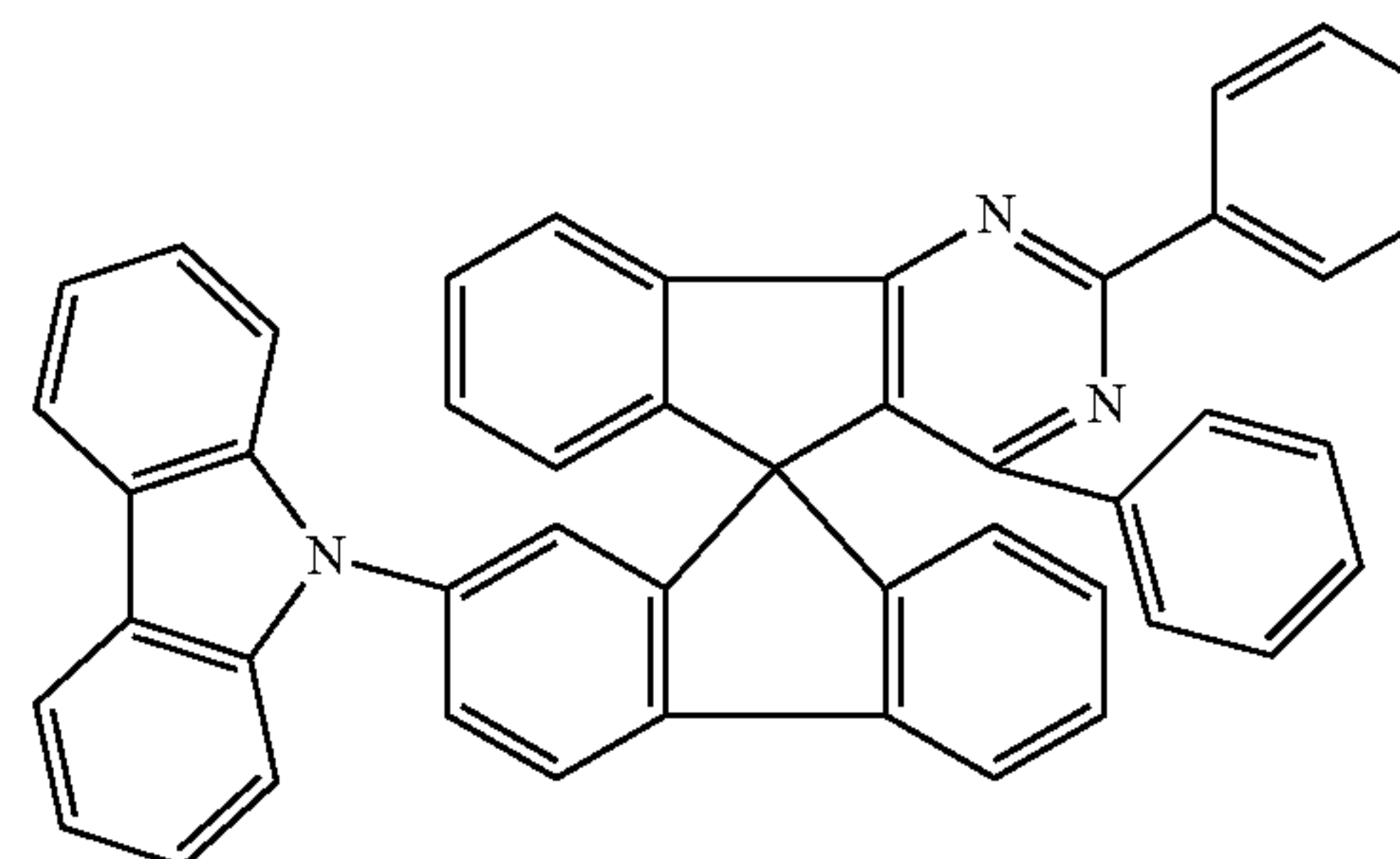
Chemical Formula 1-4
