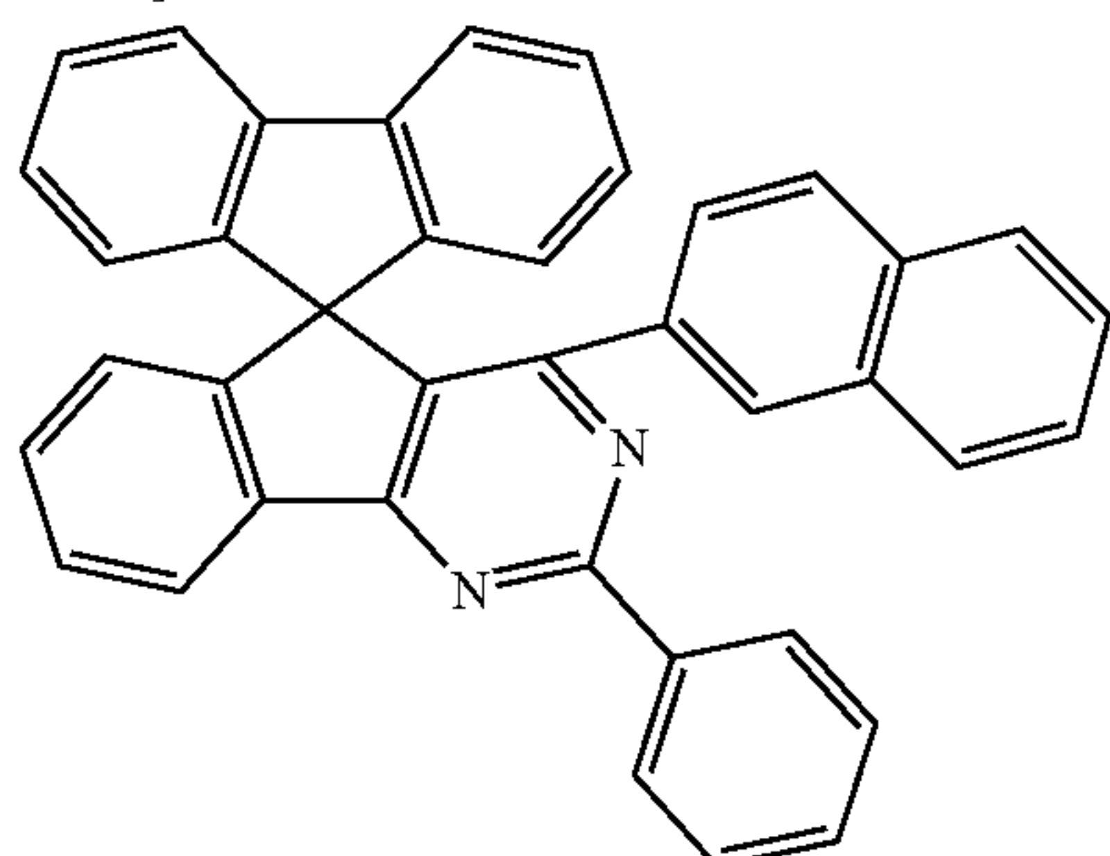
[Chemical Formula 1-73]
