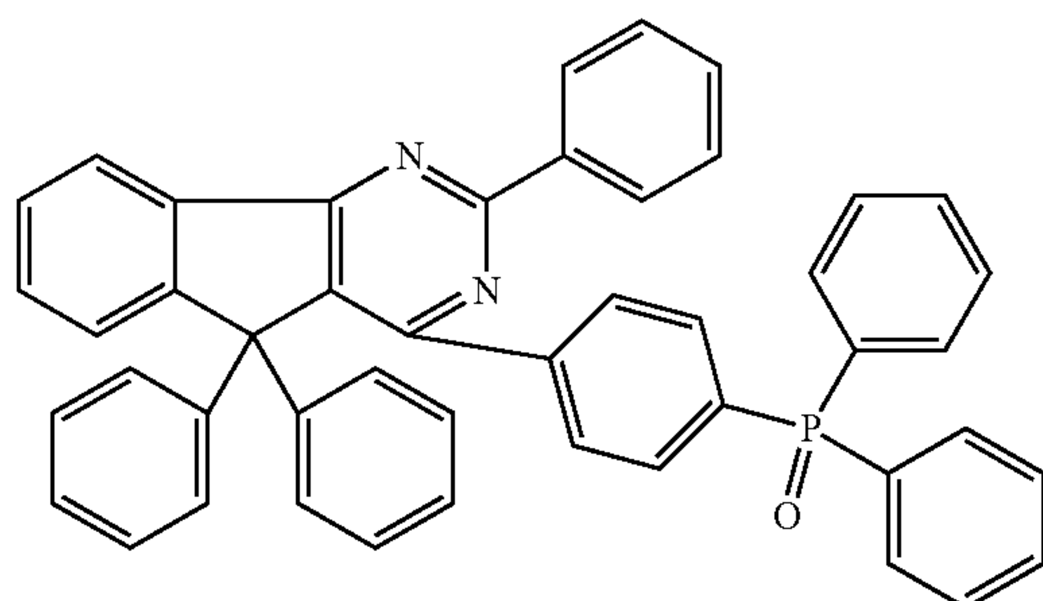
Chemical Formula 2-38
