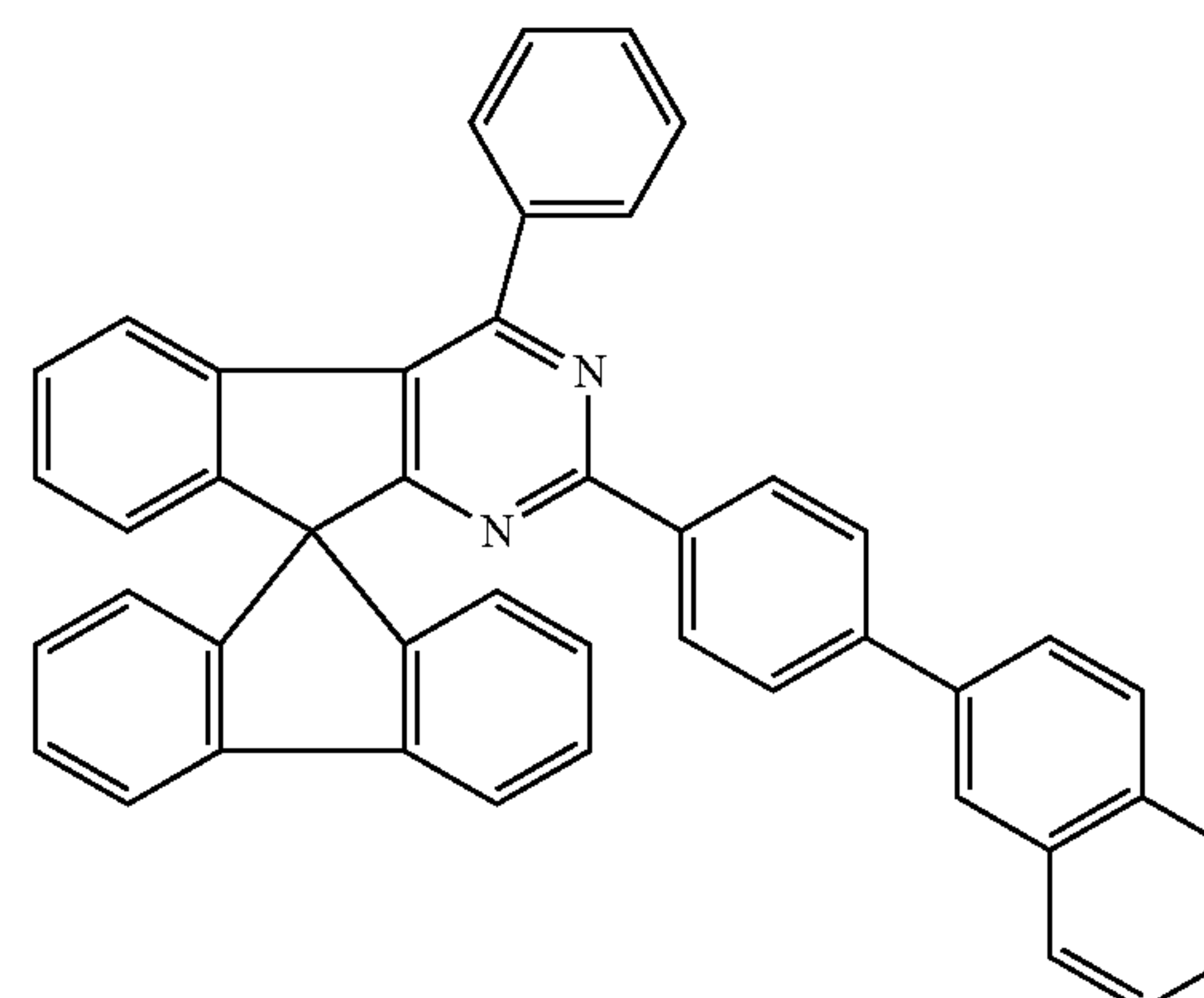
Chemical Formula 1-65
