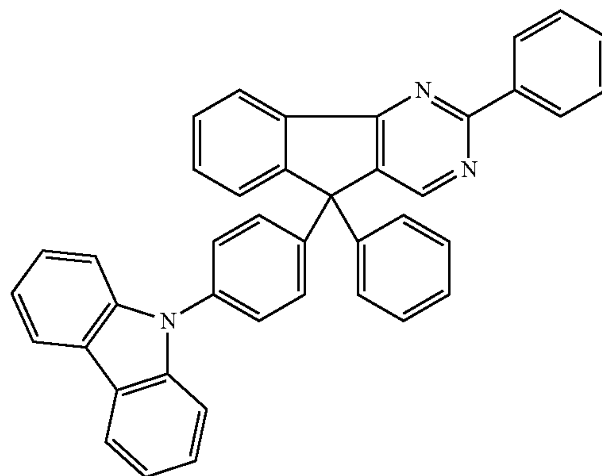
Chemical Formula 2-6
