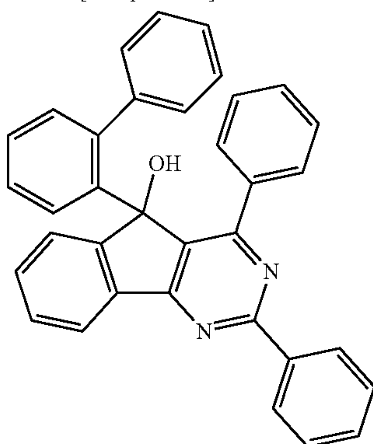
[Compound C-1]
