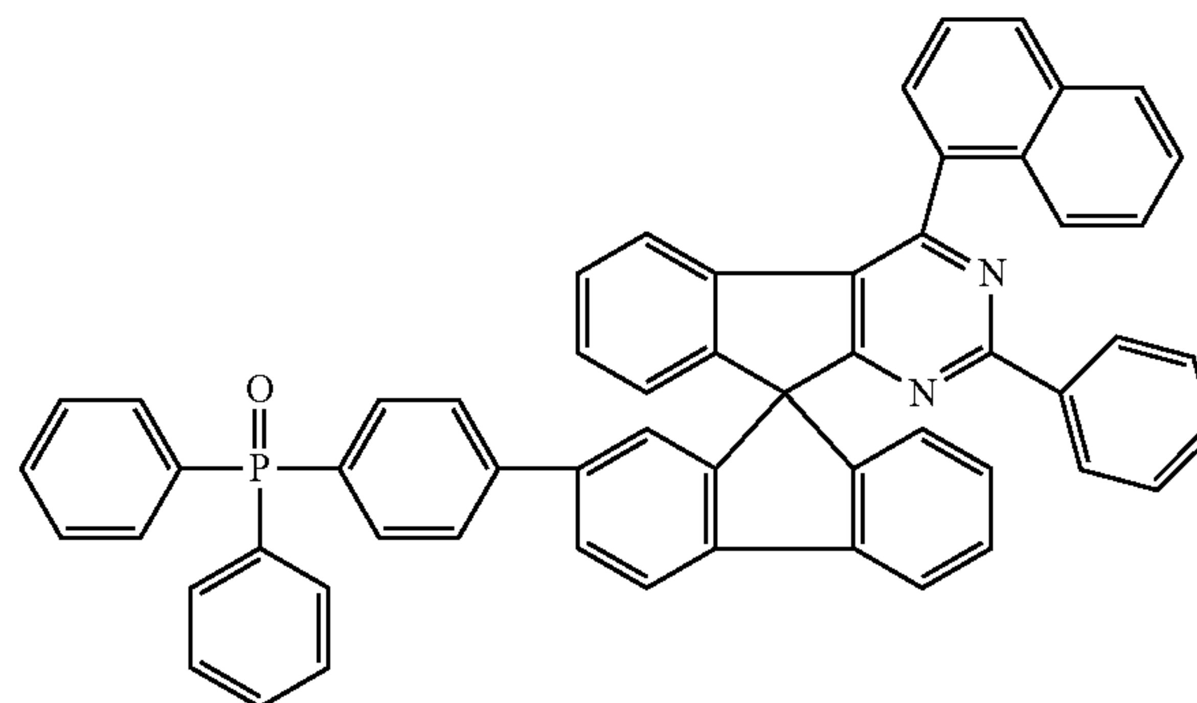
Chemical Formula 1-48
