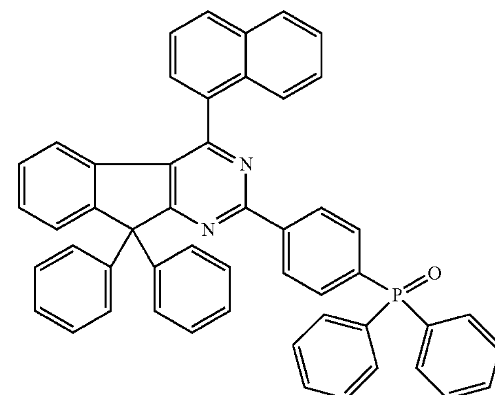
Chemical Formula 2-22
