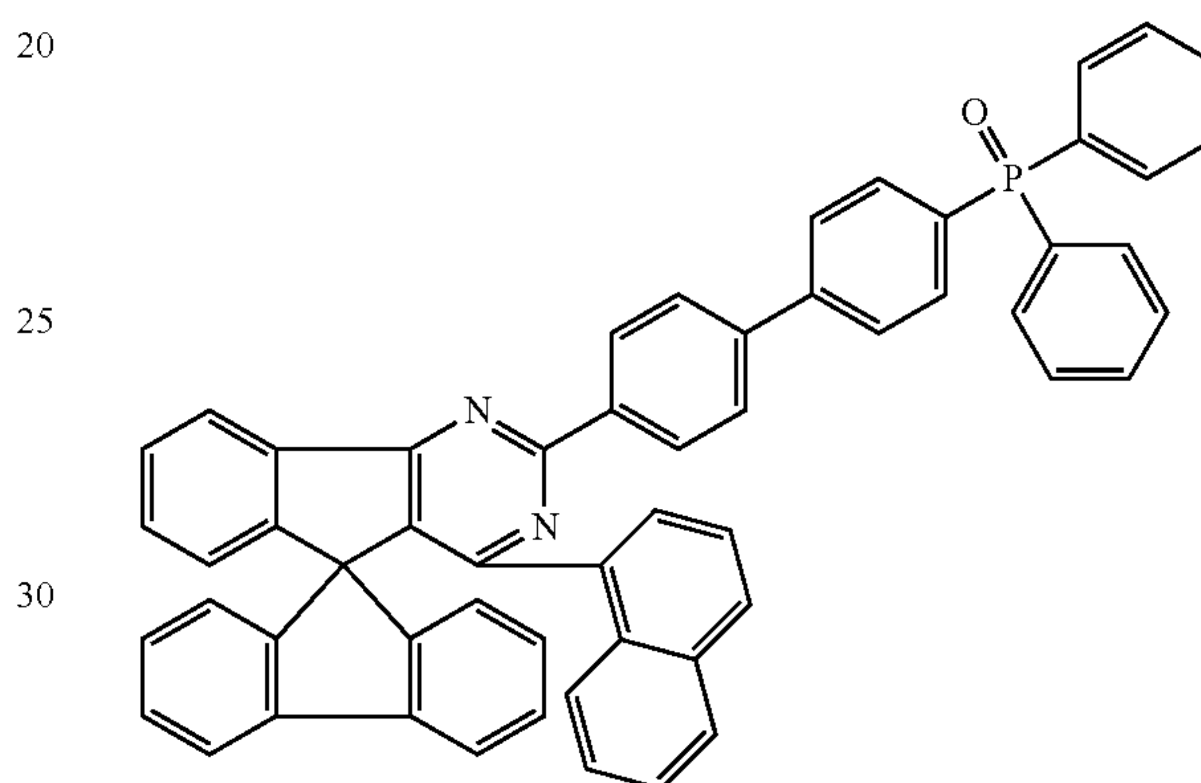
Chemical Formula 1-58
