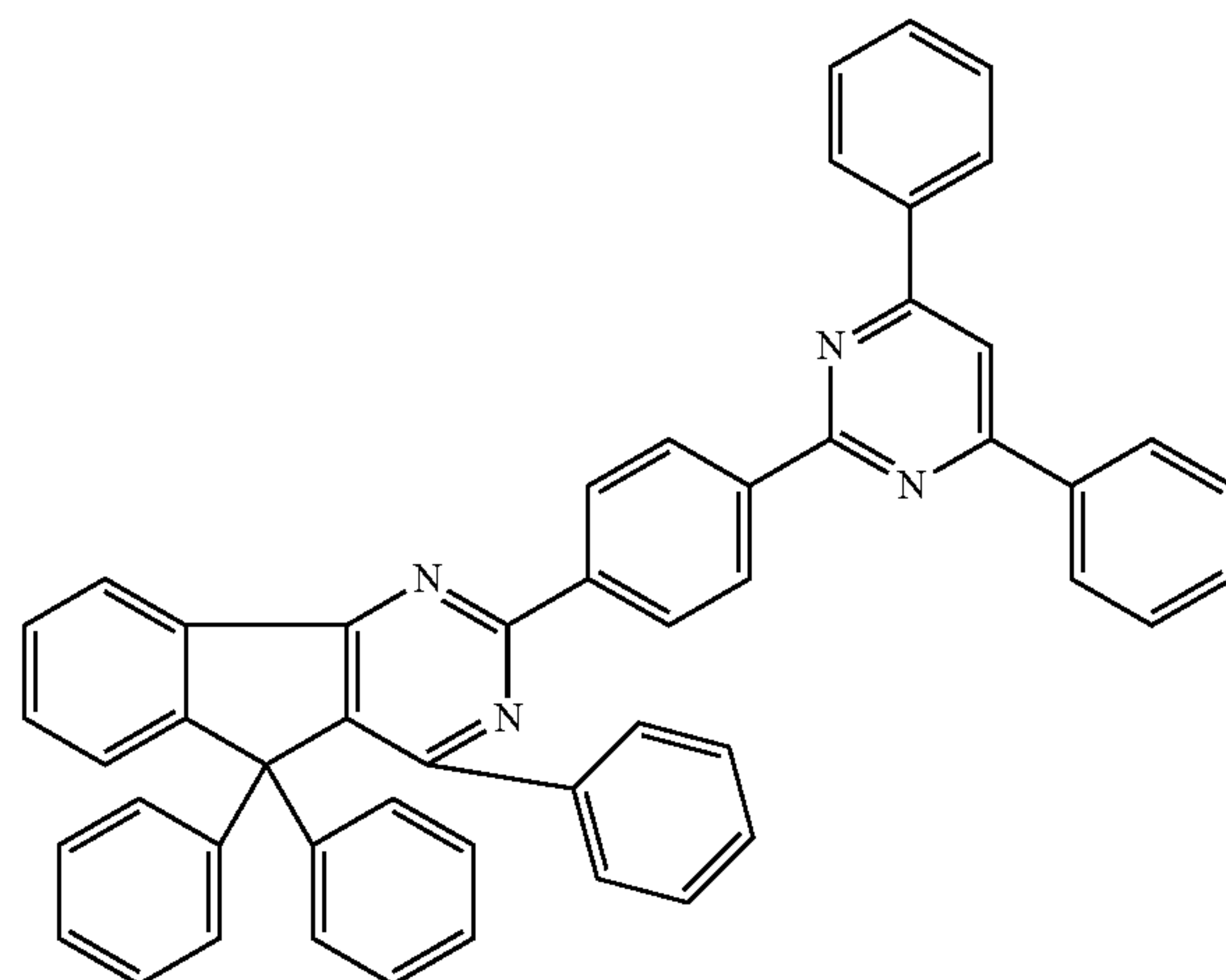
Chemical Formula 2-48
