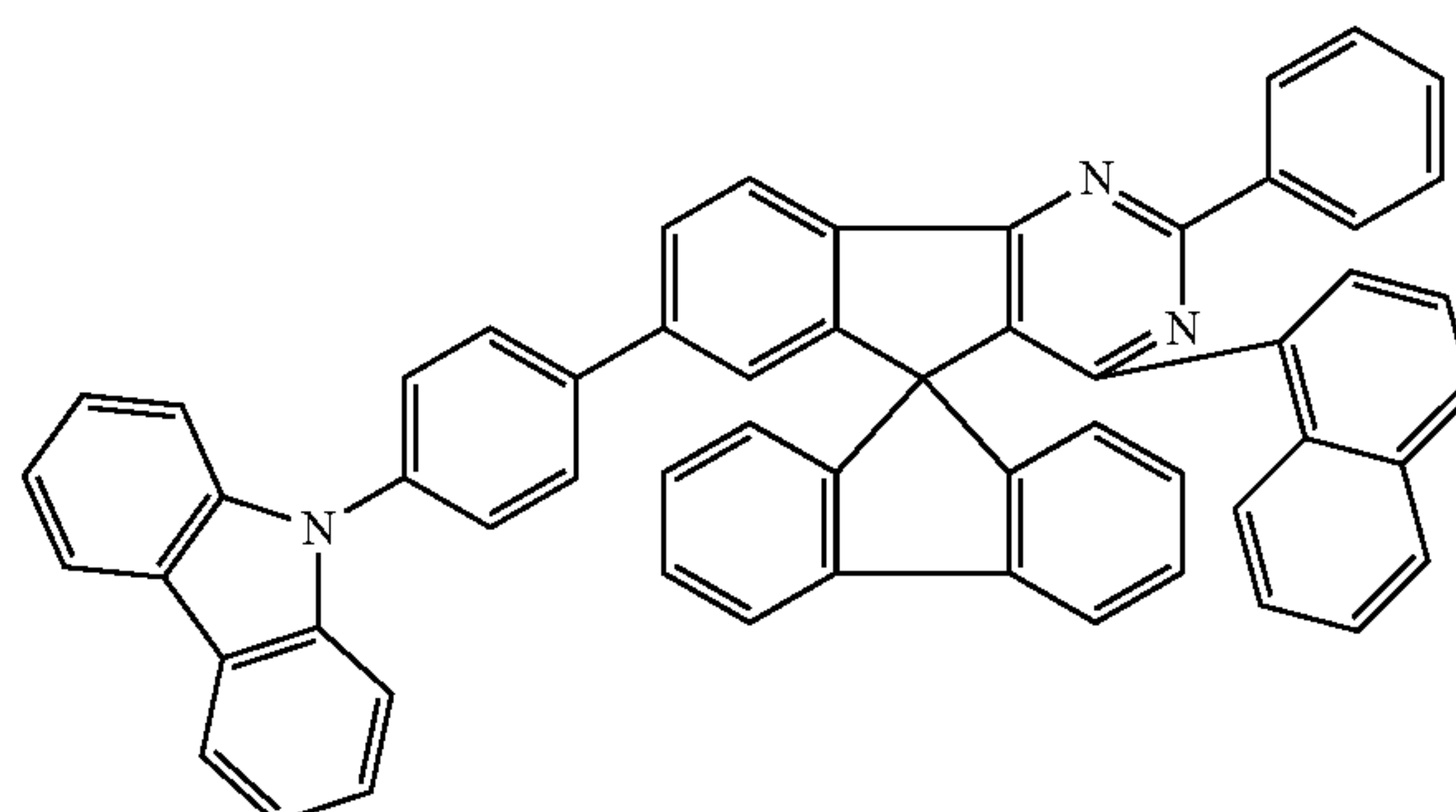
Chemical Formula 1-35
