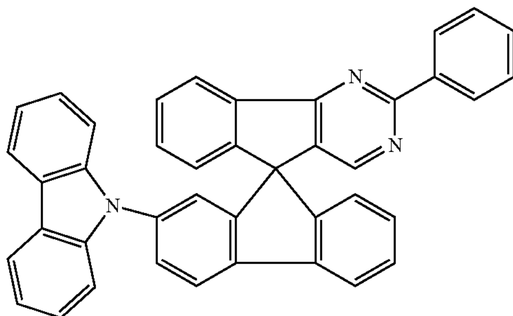
Chemical Formula 1-2
