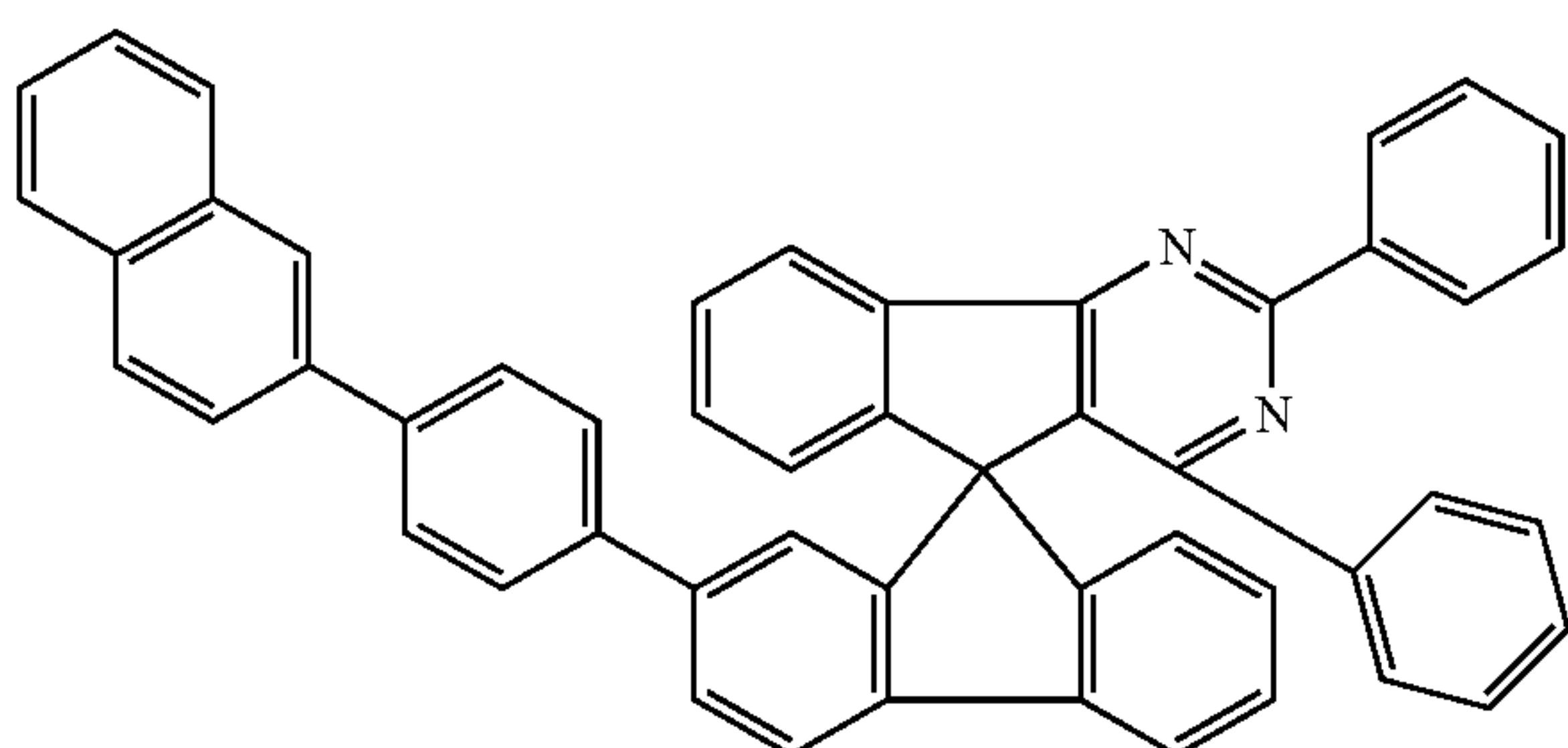
Chemical Formula 1-23
