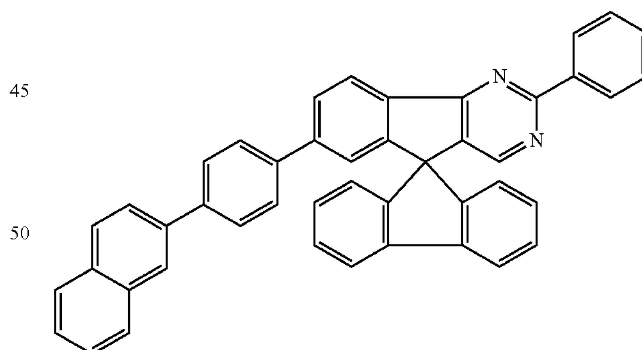
Chemical Formula 1-26
