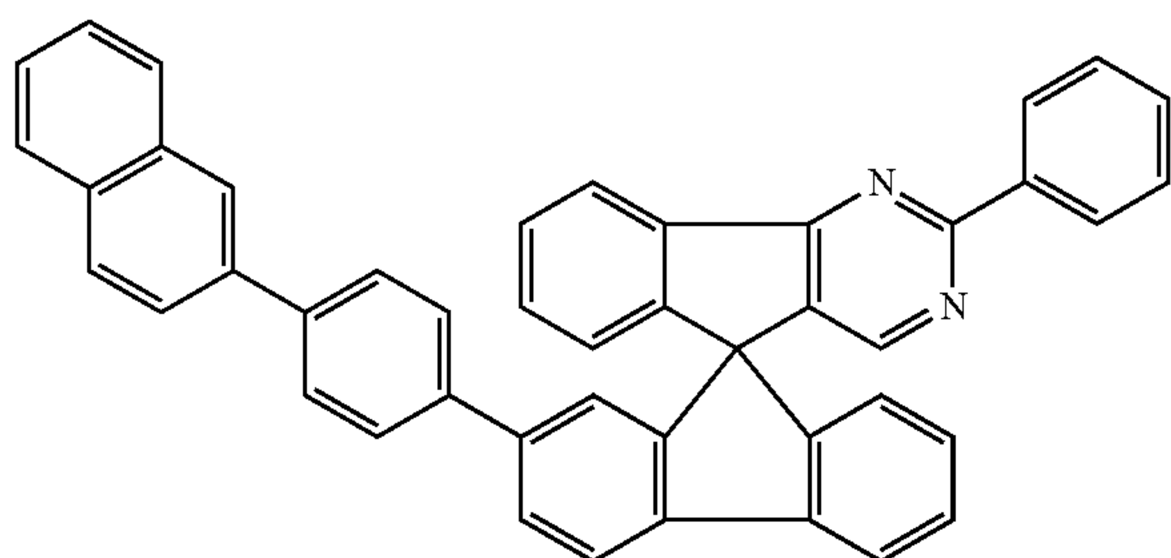
Chemical Formula 1-22
