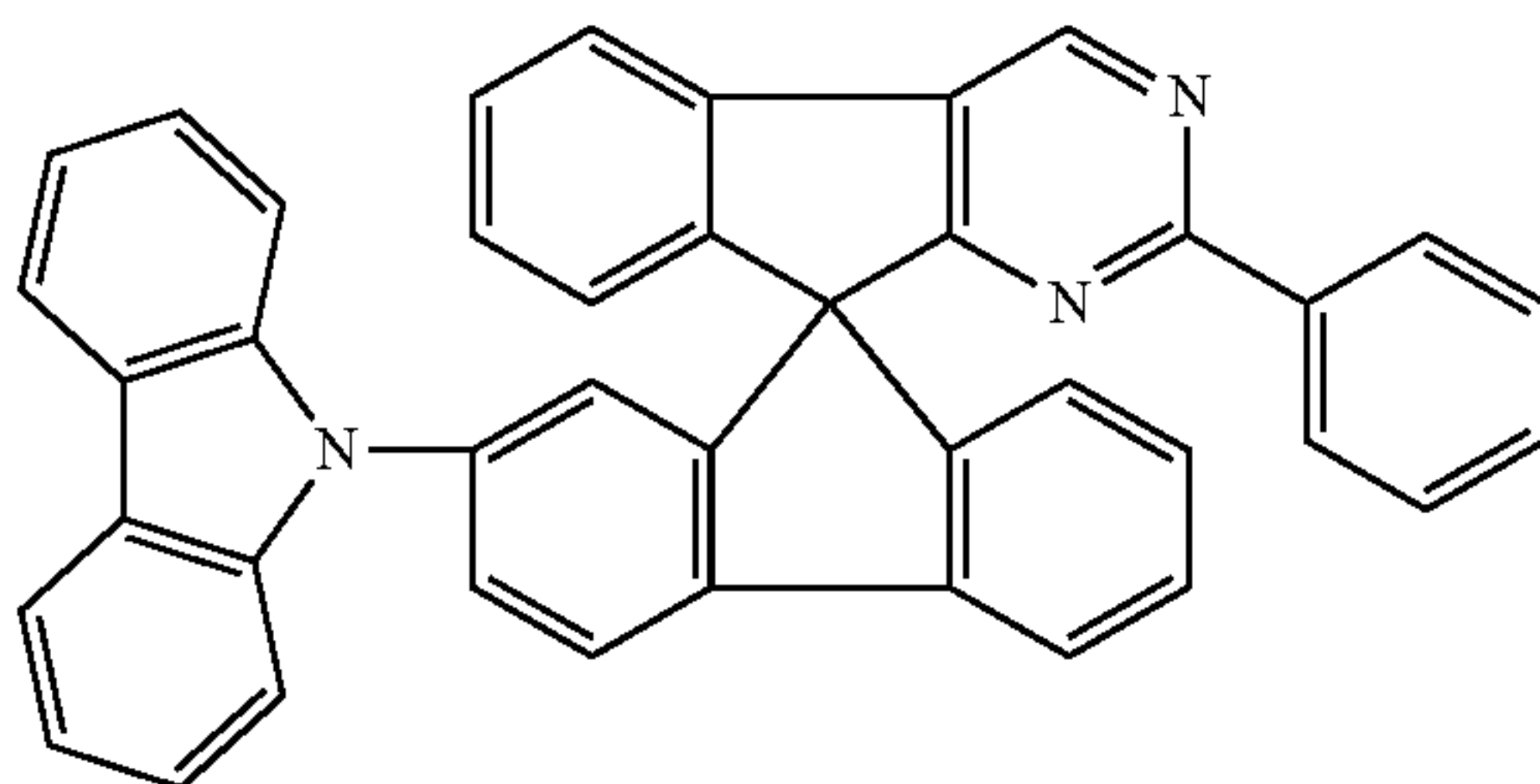
Chemical Formula 1-3
