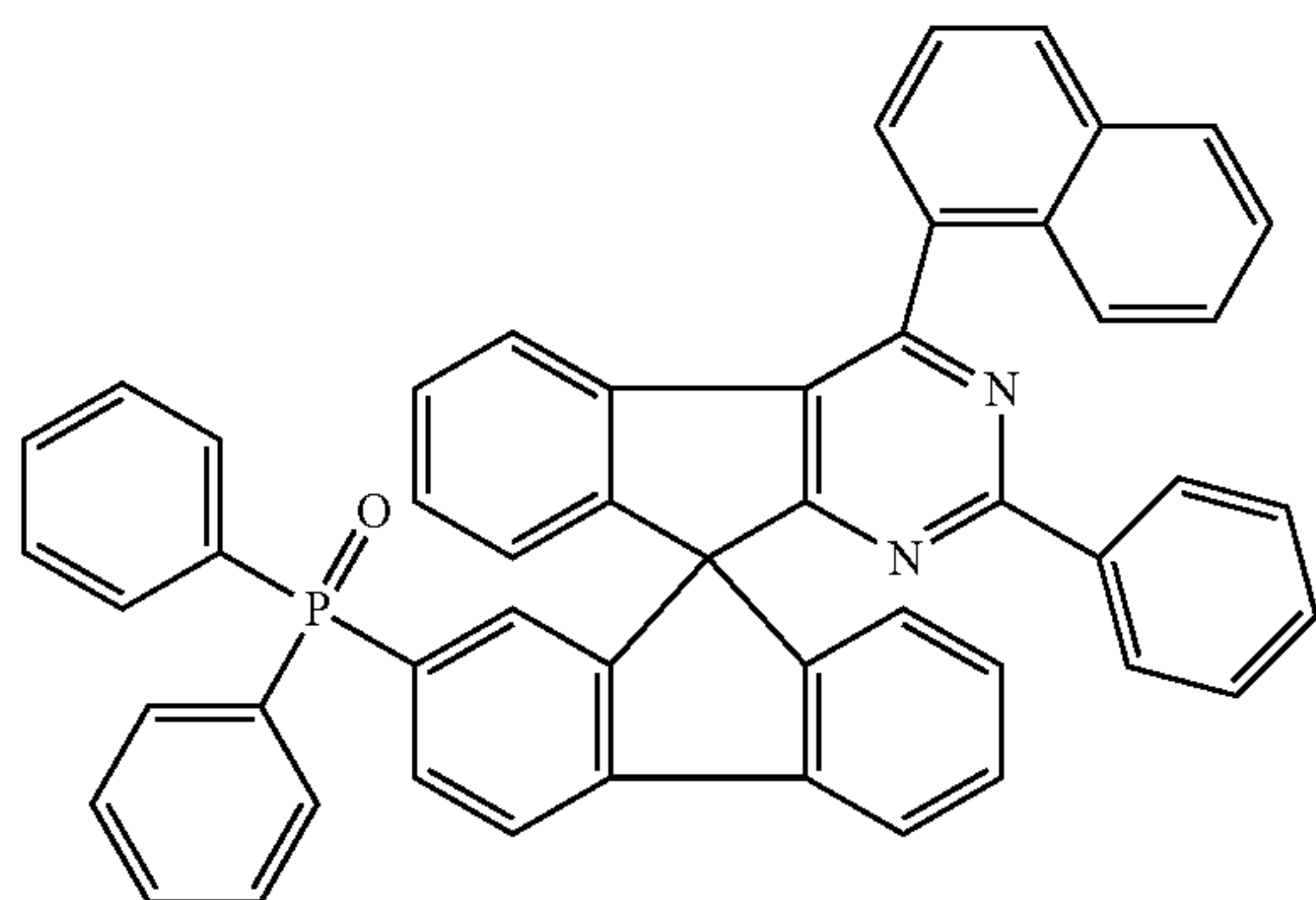
Chemical Formula 1-44
