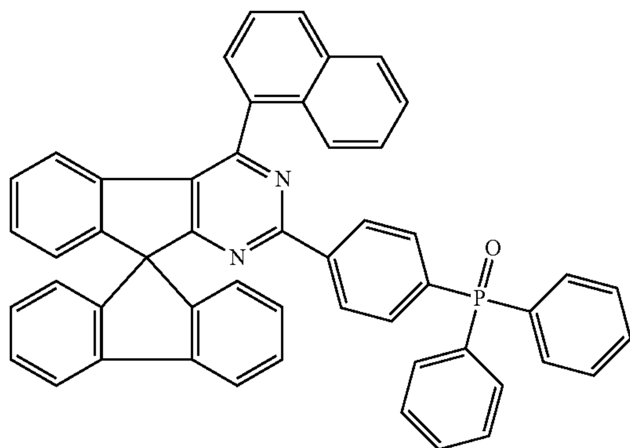
Chemical Formula 1-52
