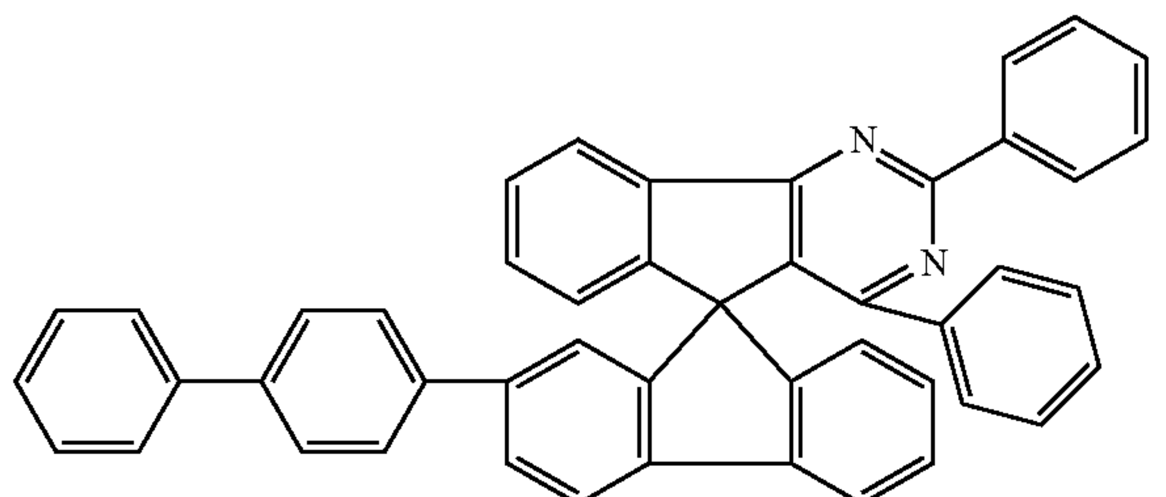
Chemical Formula 1-8
