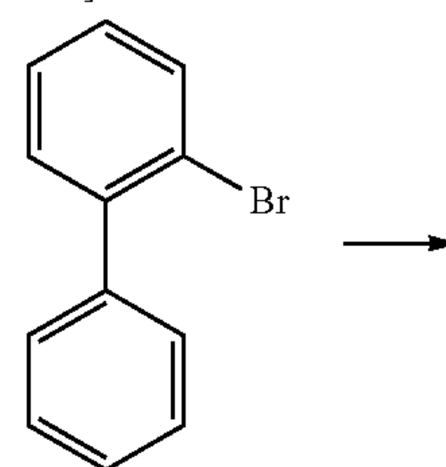
[Compound D]
