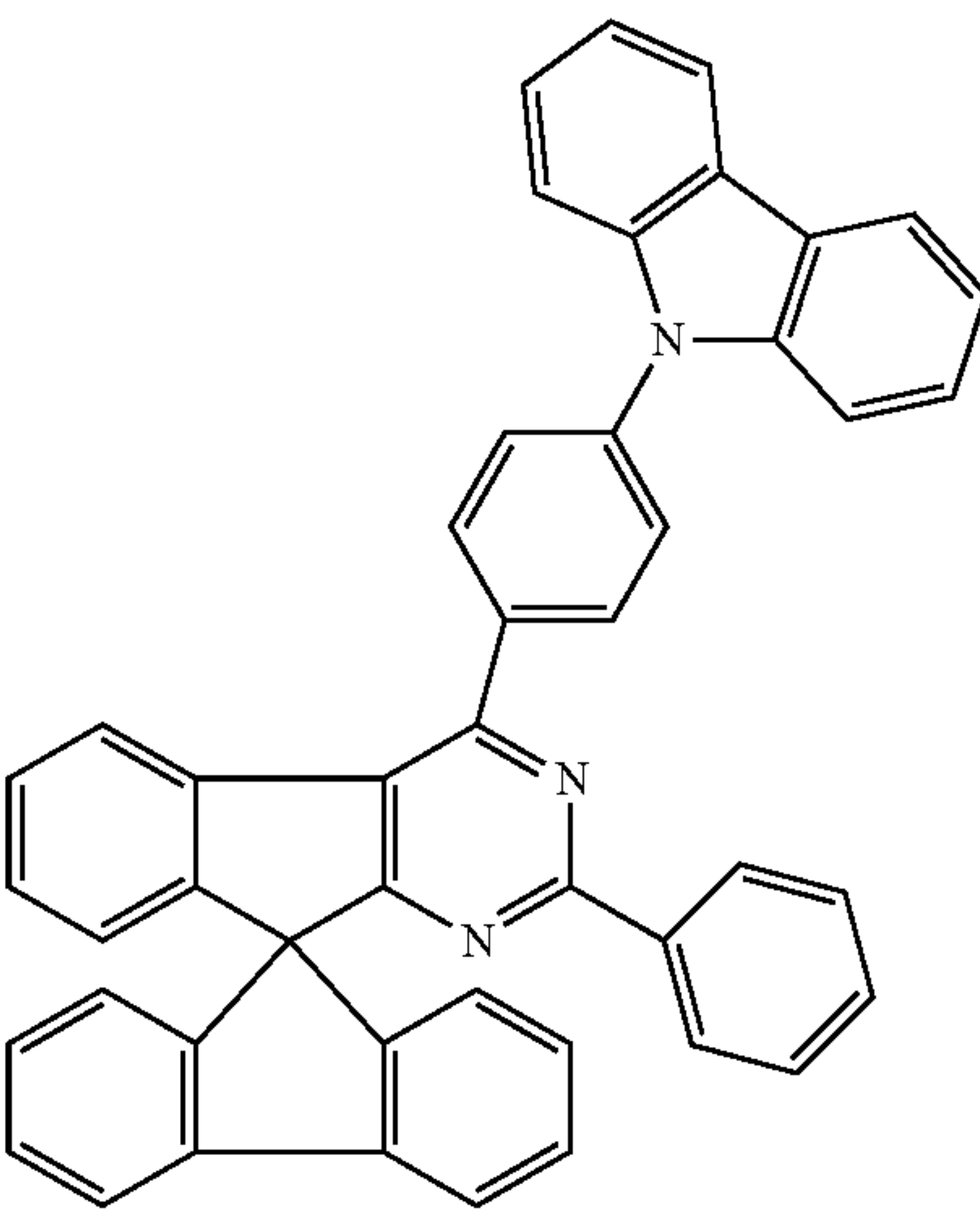
Chemical Formula 1-86
