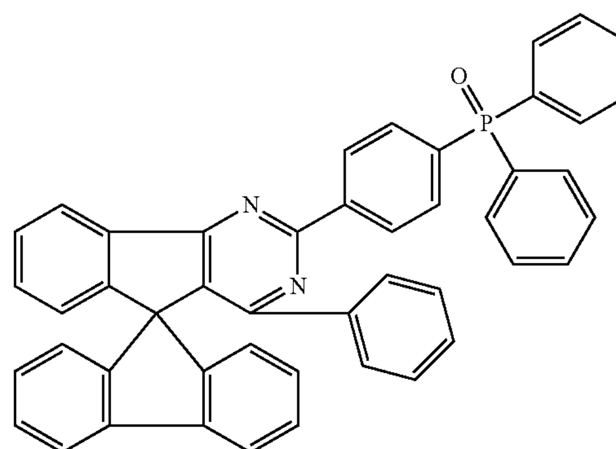
Chemical Formula 1-50
