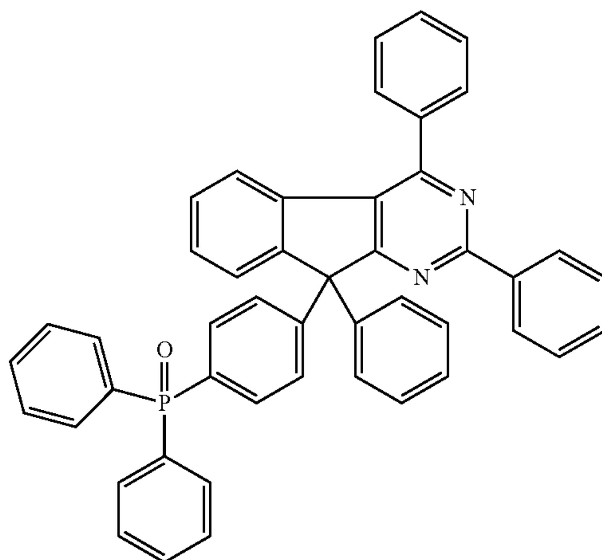
Chemical Formula 2-16
