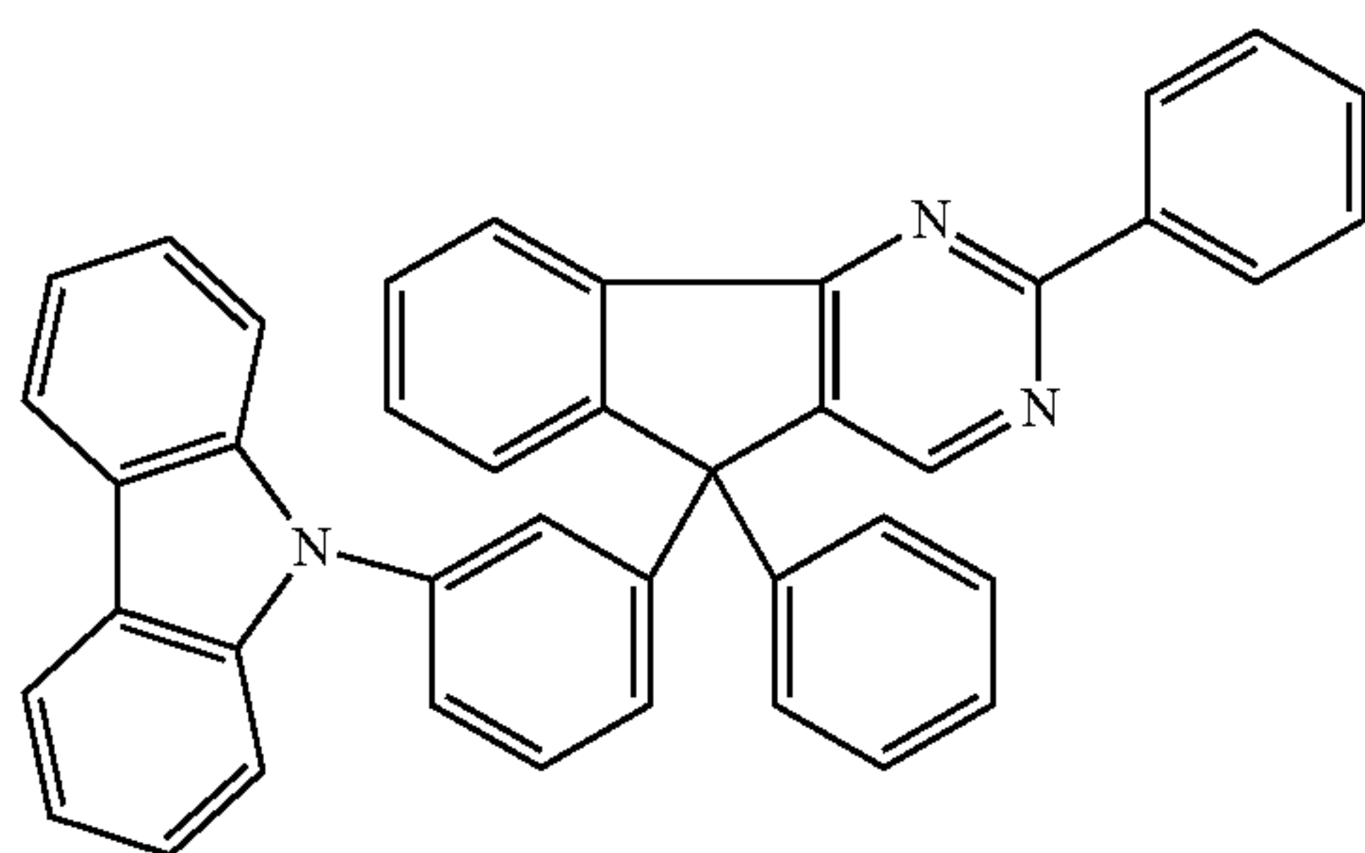
Chemical Formula 2-2
