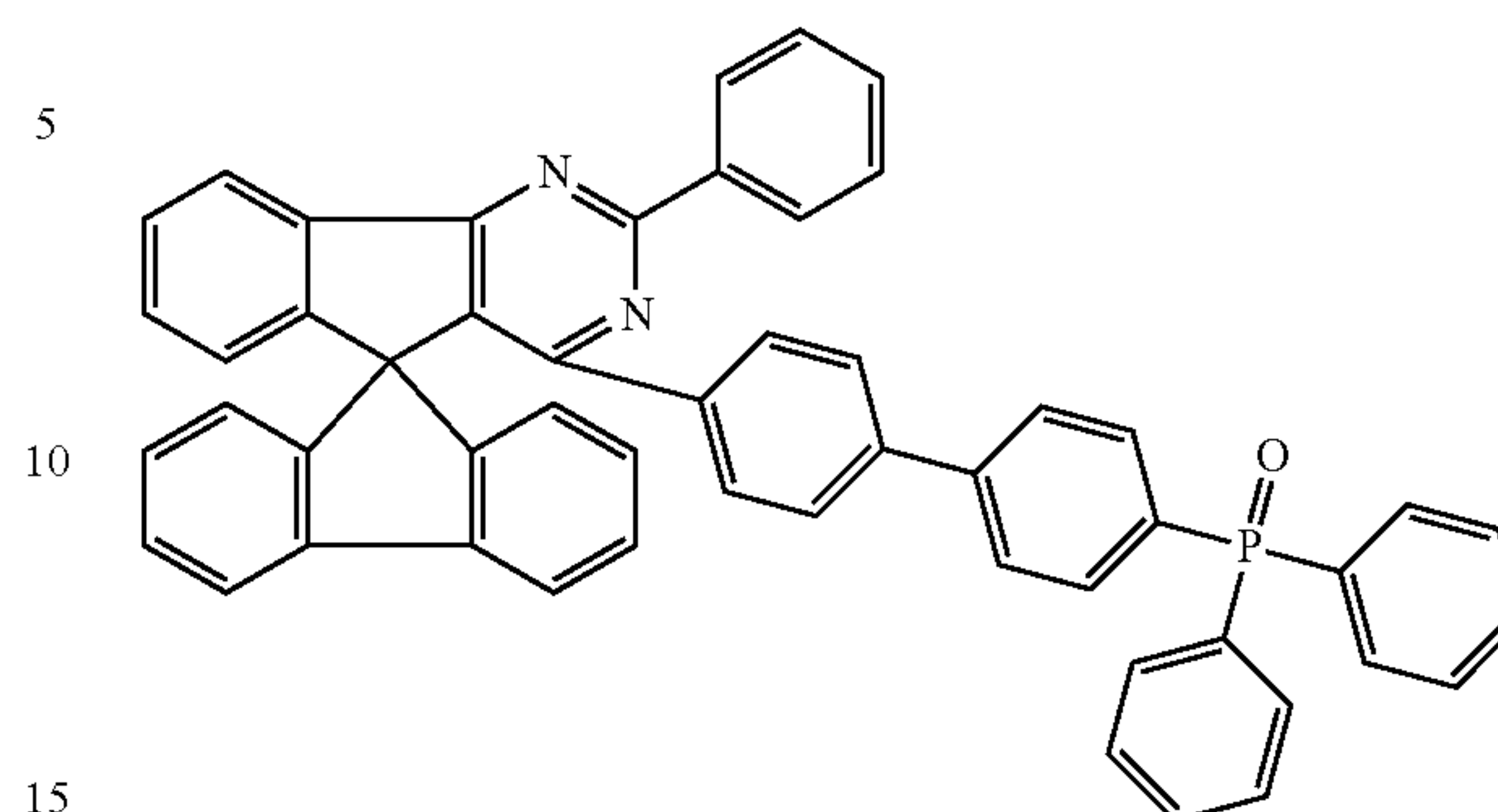
Chemical Formula 1-79
