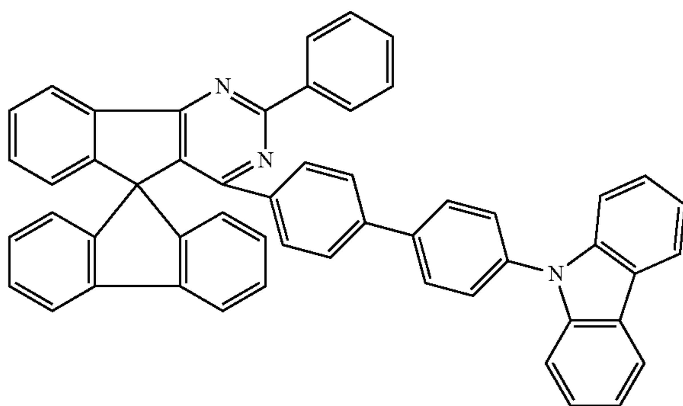
Chemical Formula 1-87
