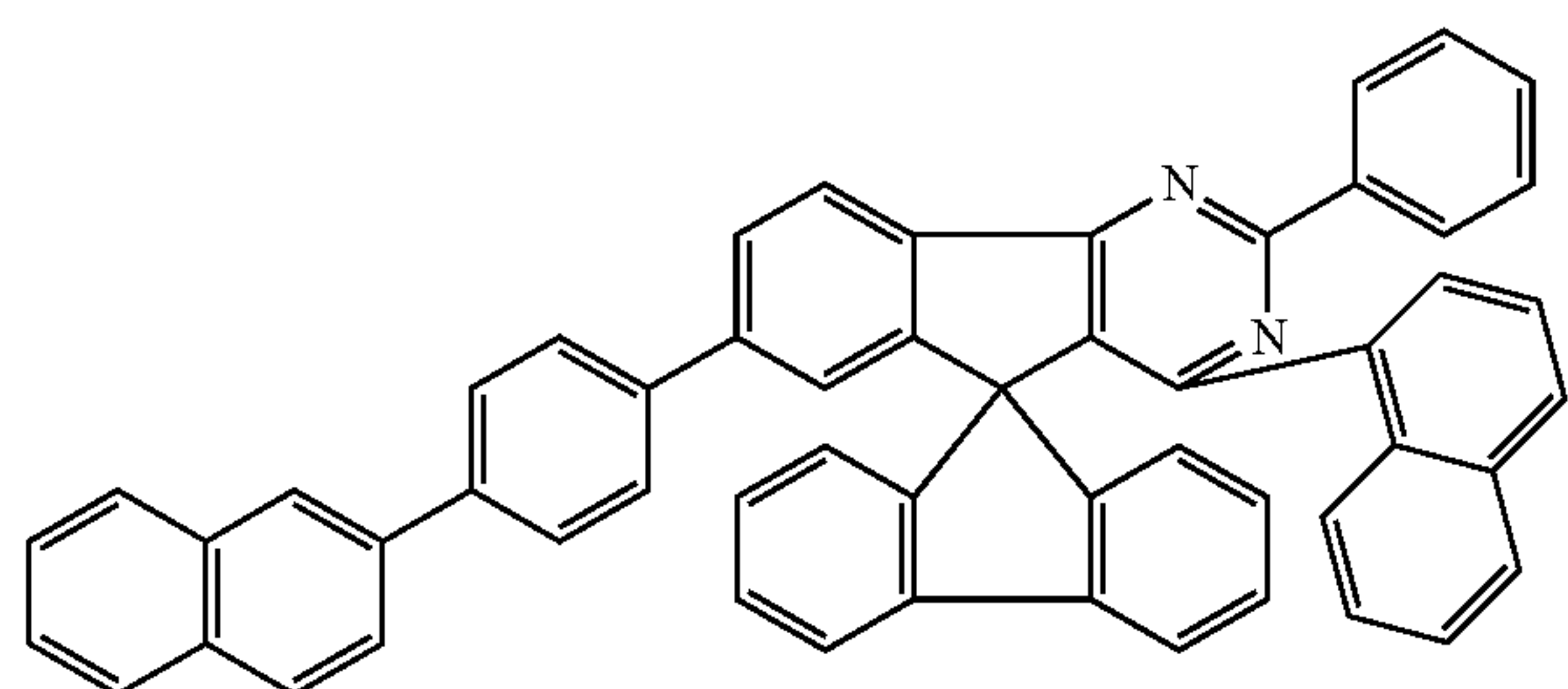
Chemical Formula 1-39
