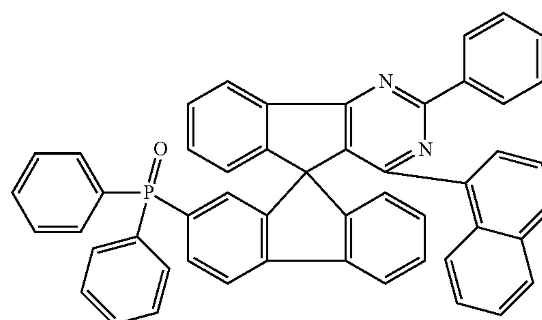
Chemical Formula 1-43
