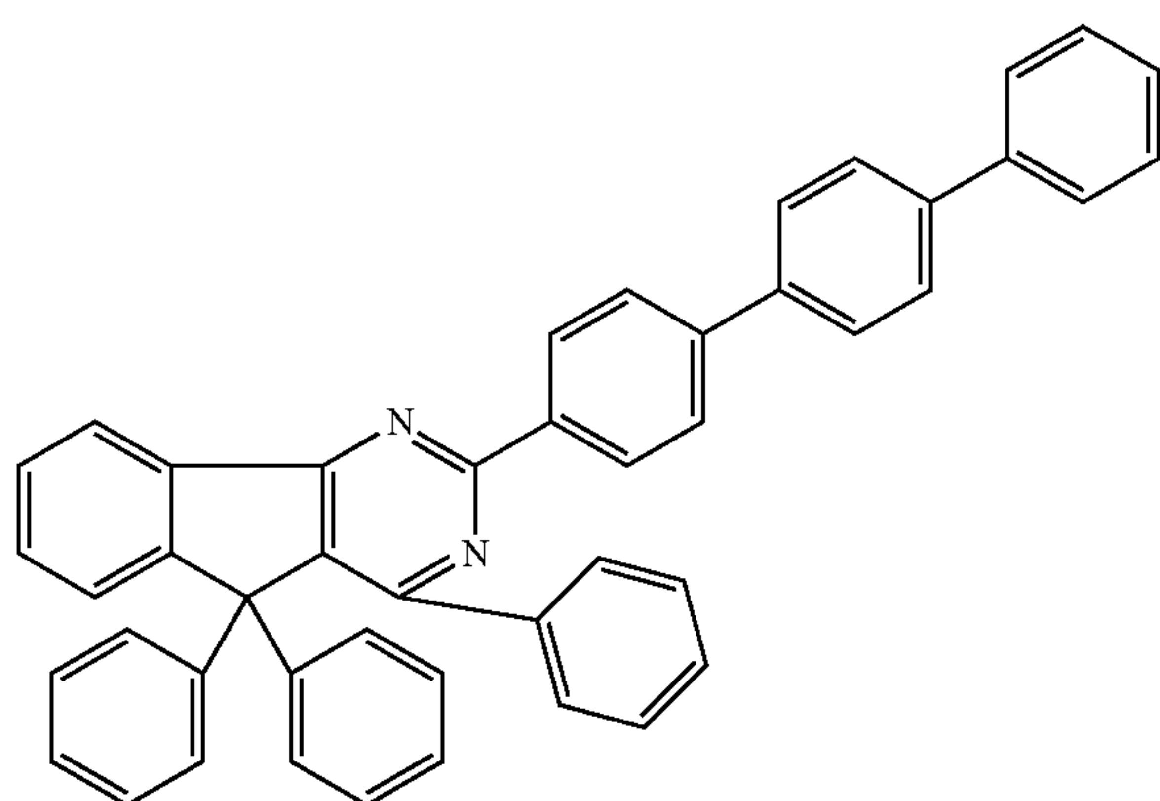
Chemical Formula 2-25
