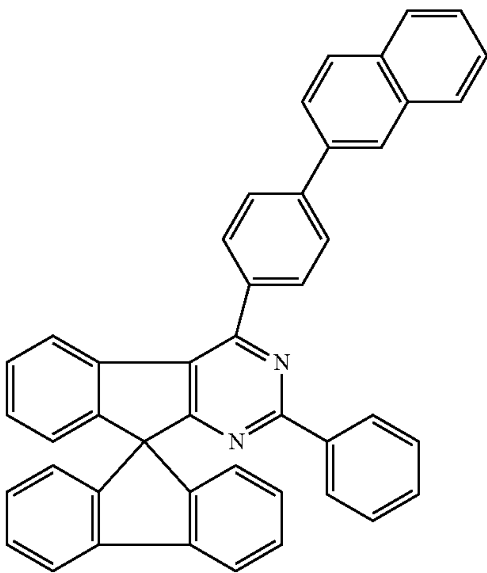
Chemical Formula 1-84
