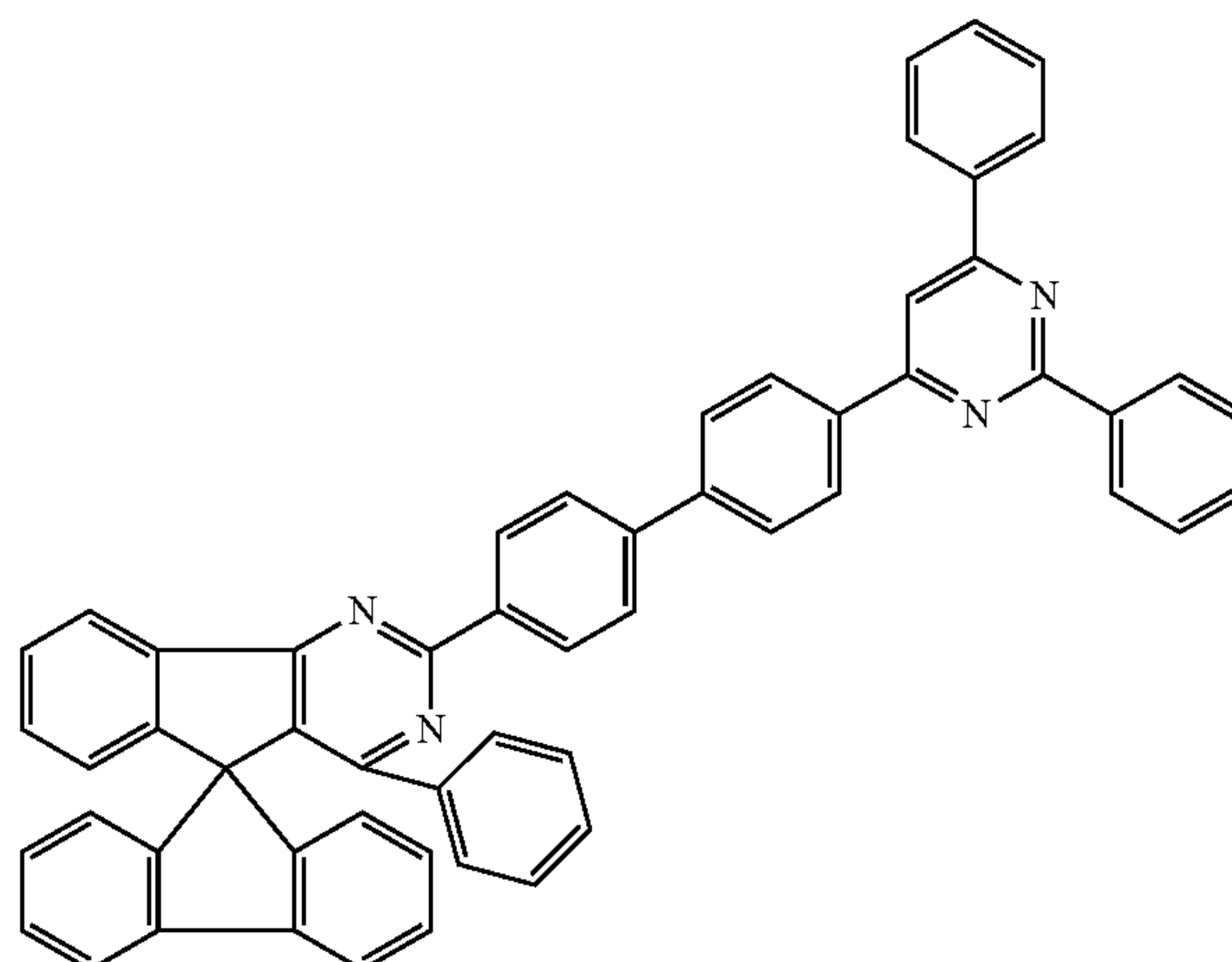
Chemical Formula 1-98
