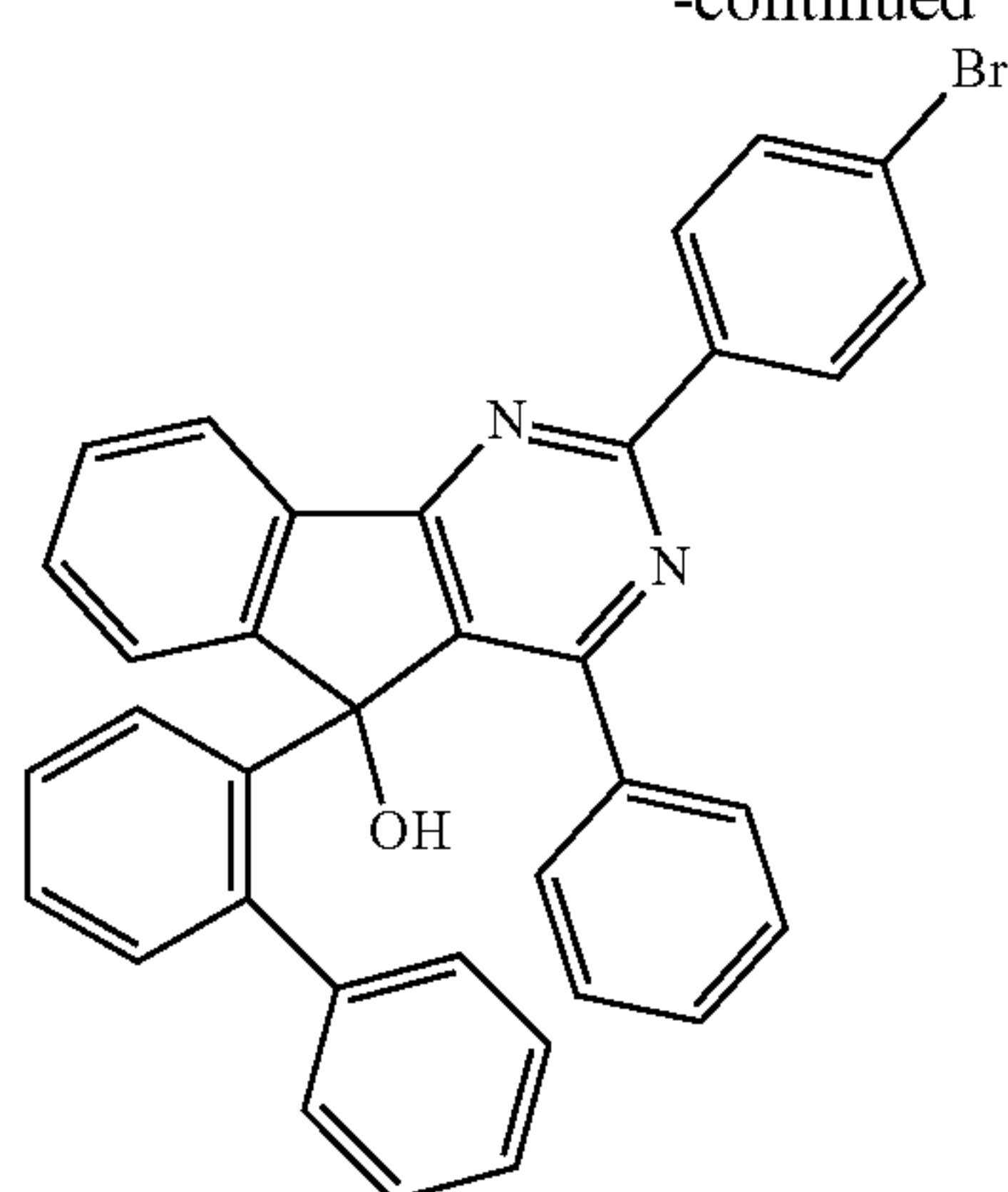
[Compound E-1]
