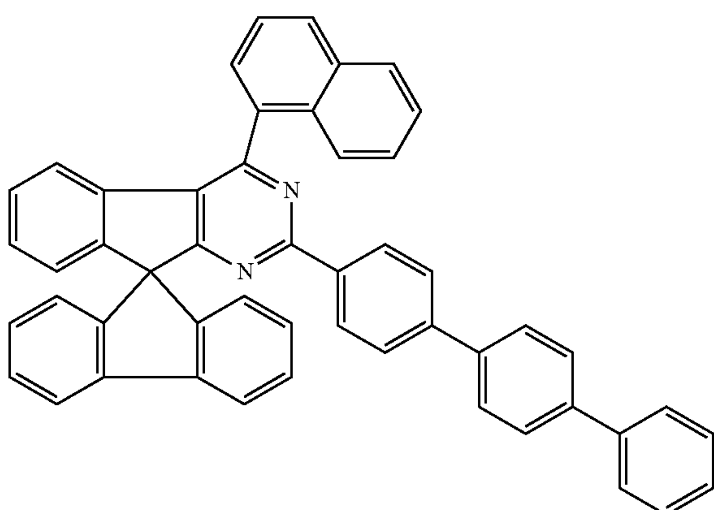
Chemical Formula 1-63
