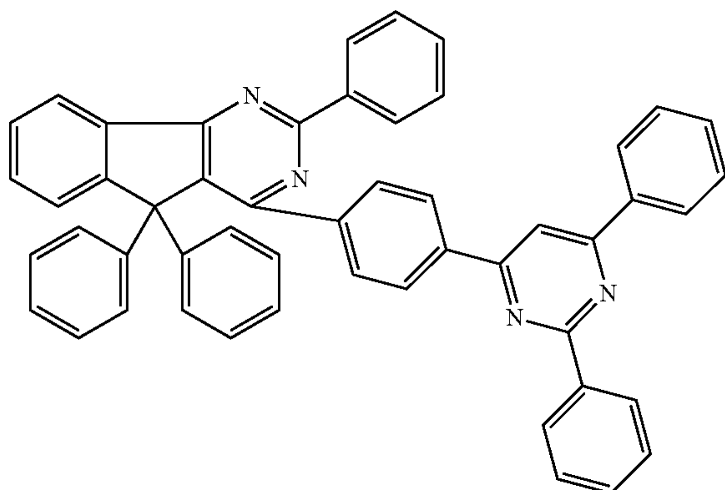
Chemical Formula 2-45
