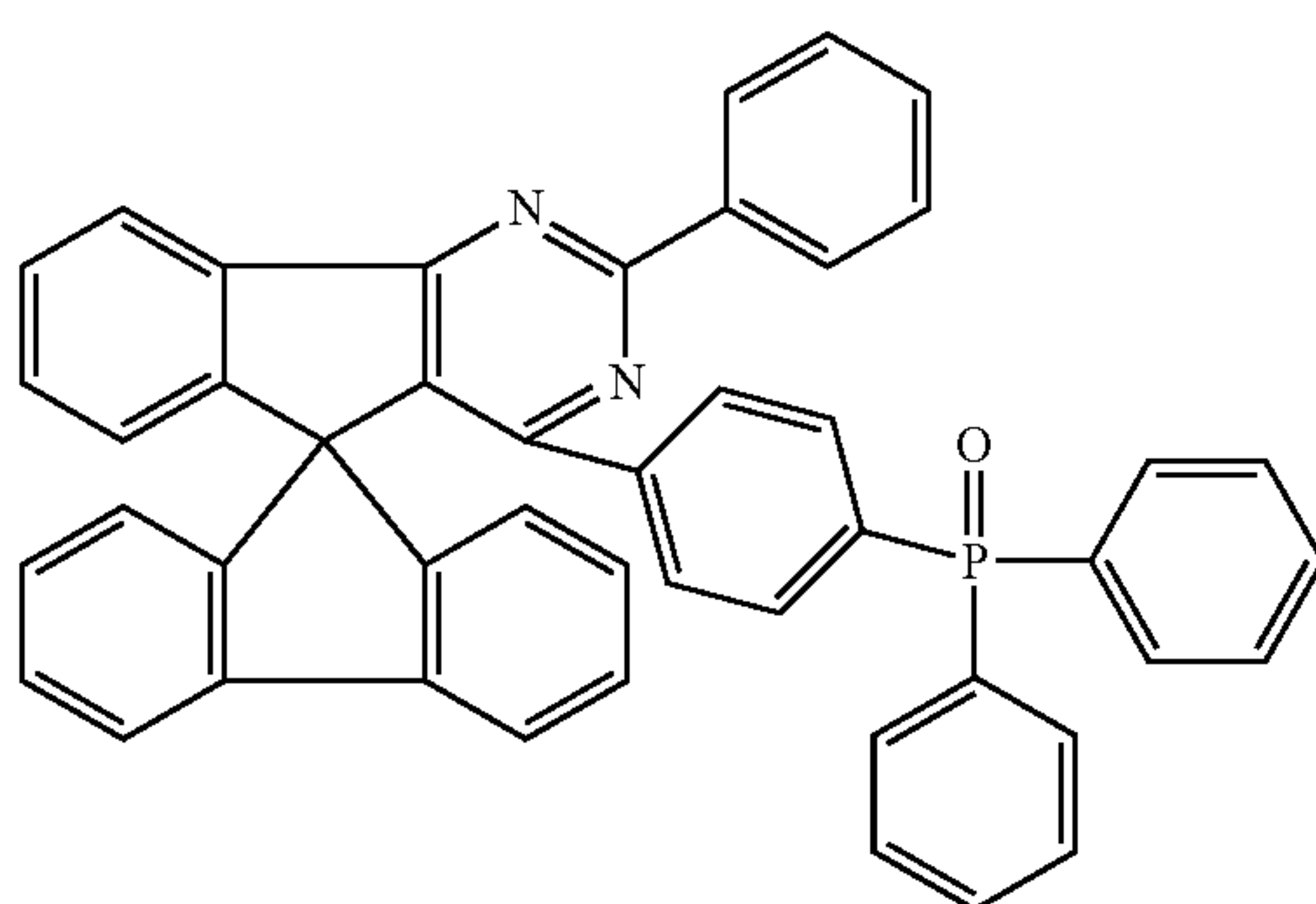
Chemical Formula 1-76
