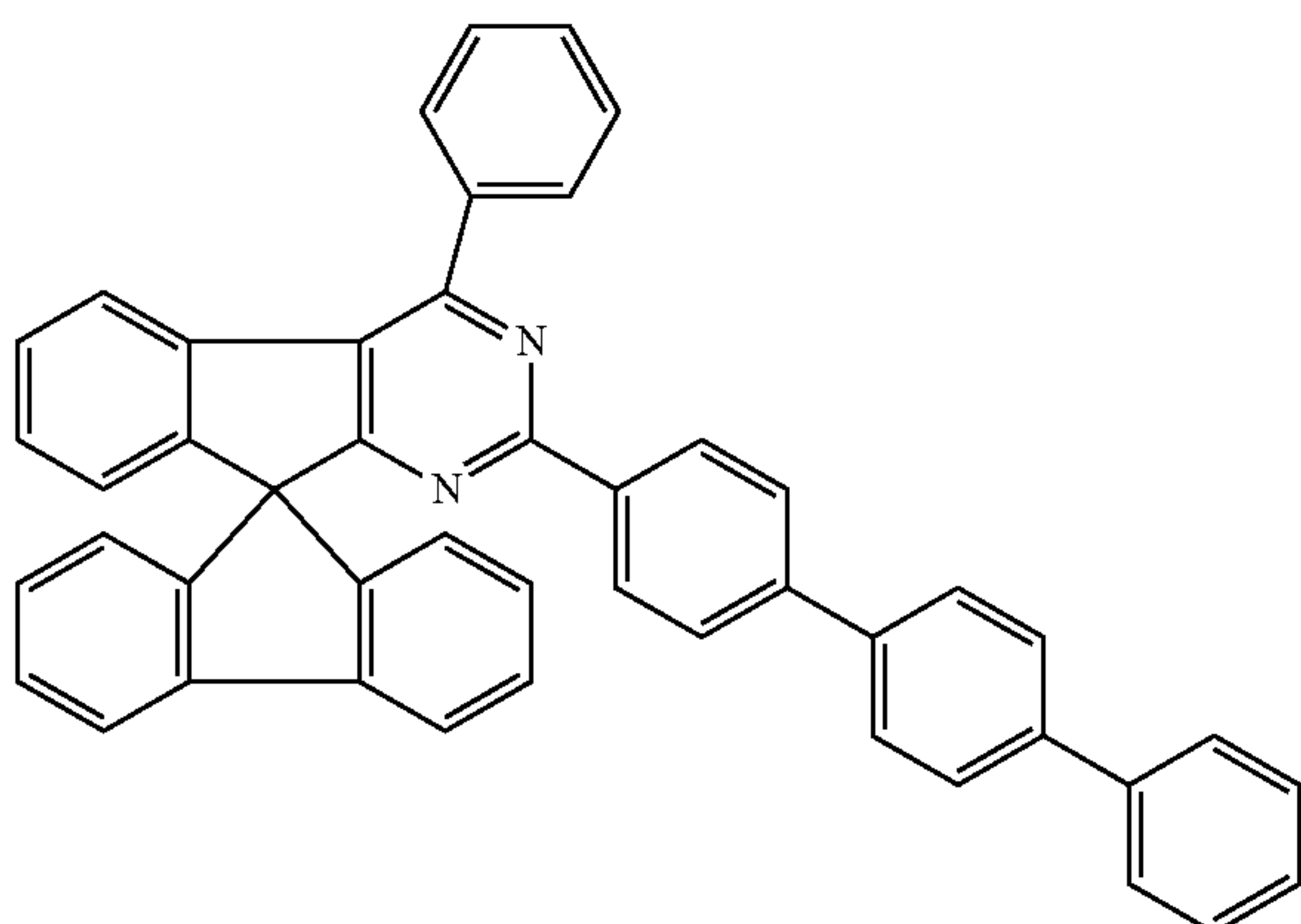
Chemical Formula 1-61
