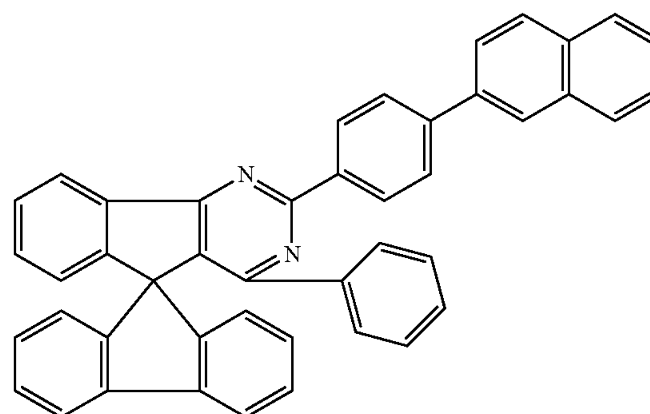
Chemical Formula 1-64
