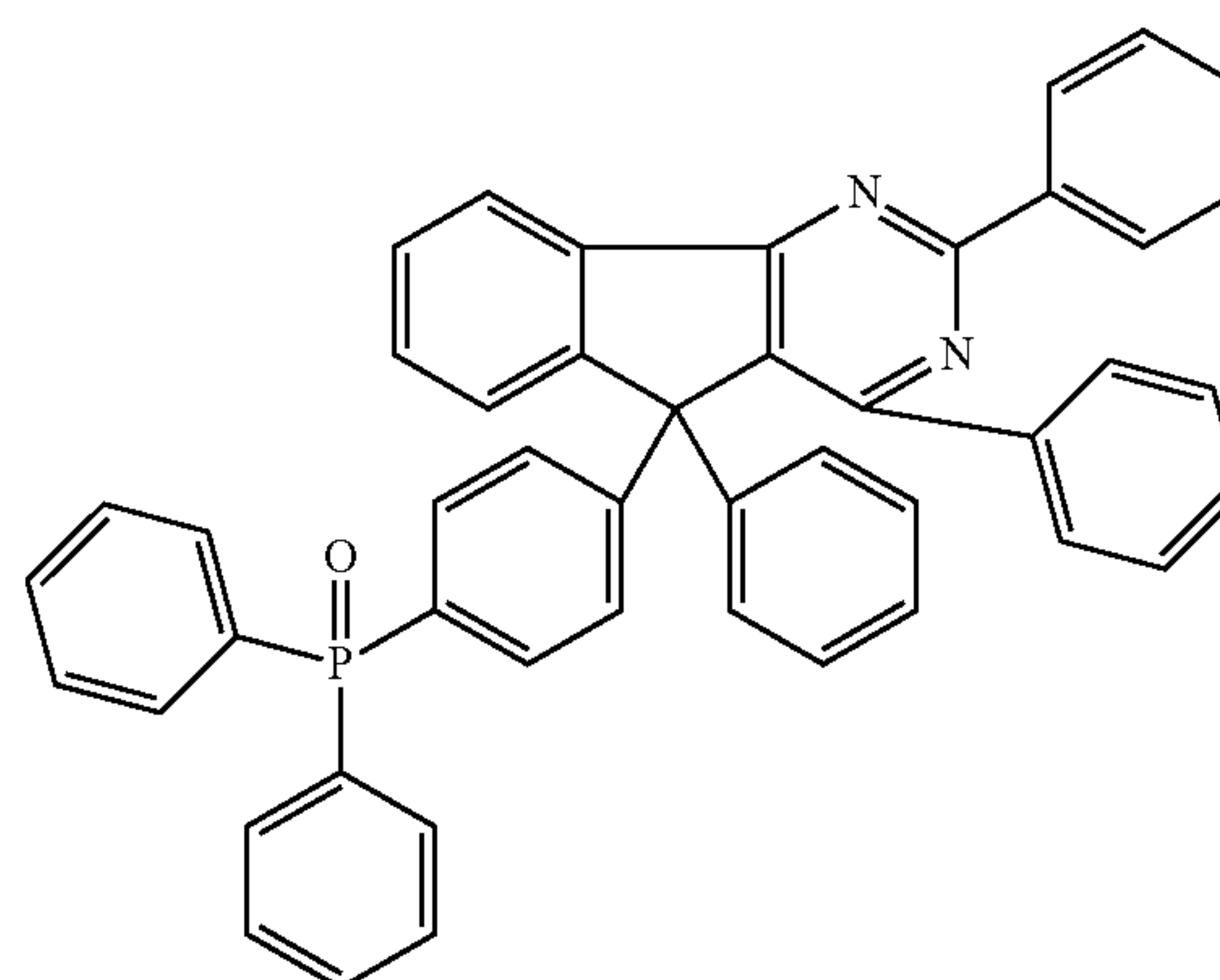
Chemical Formula 2-15
