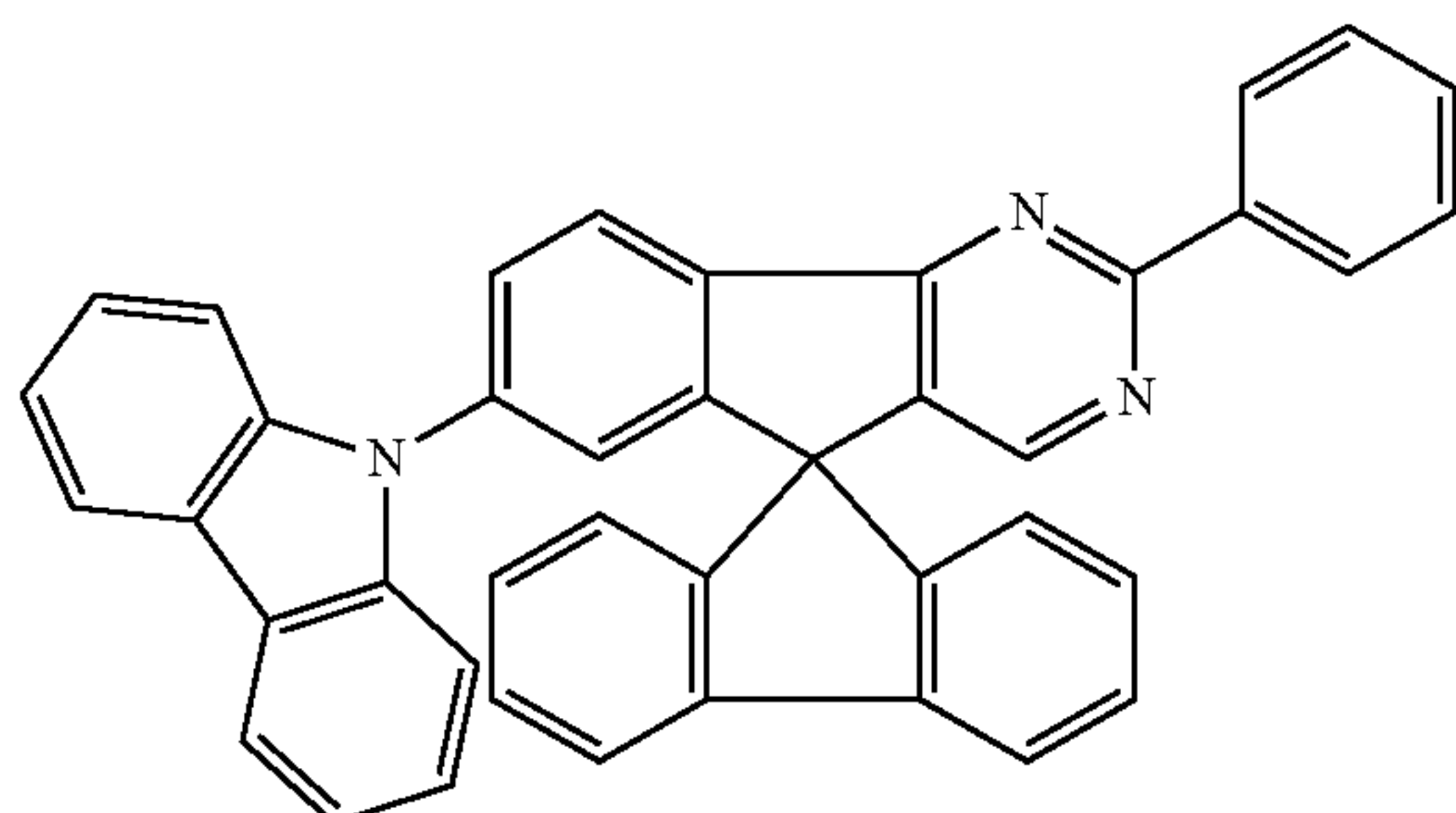
Chemical Formula 1-18
