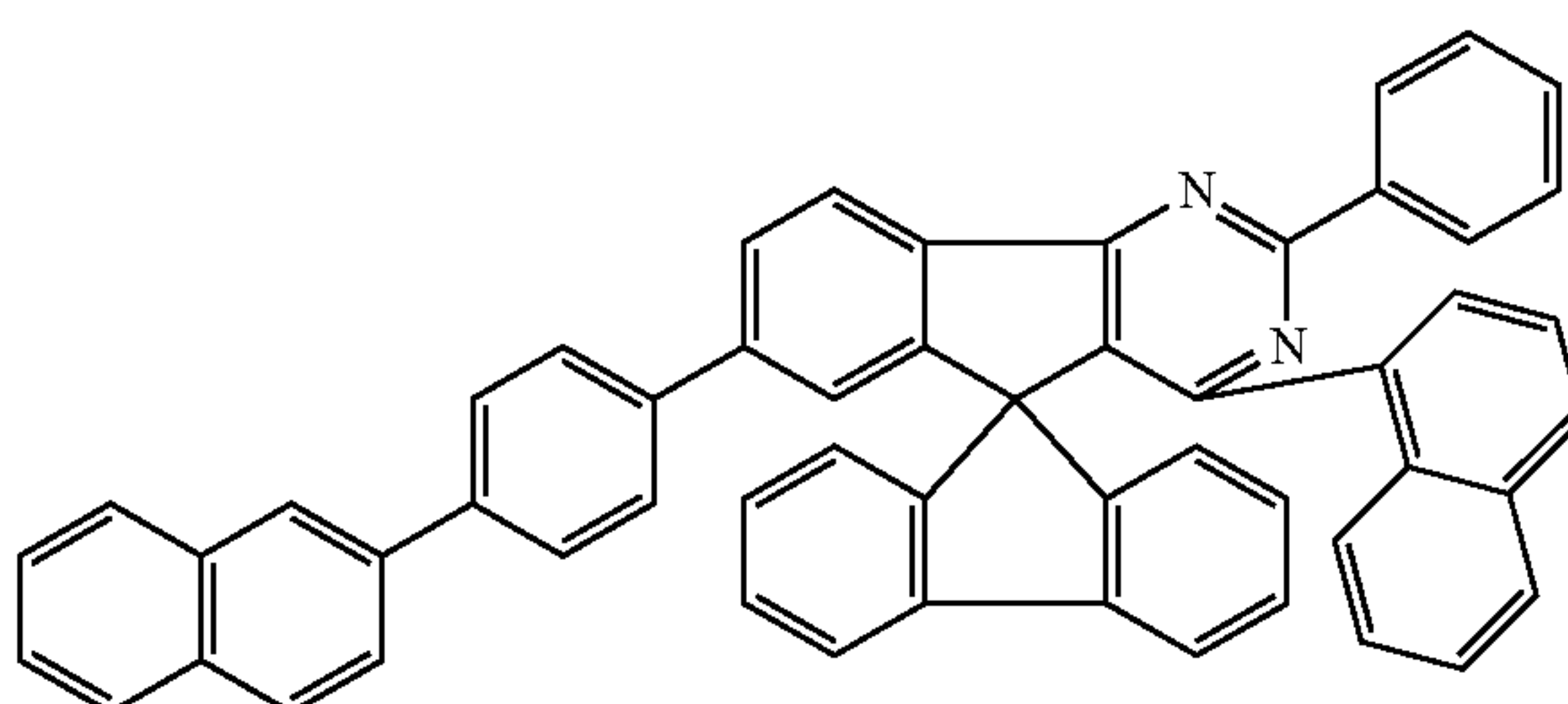
Chemical Formula 1-39
