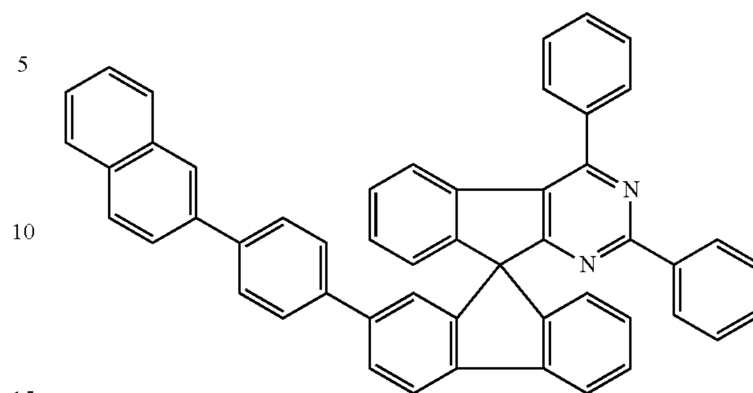
Chemical Formula 1-24
