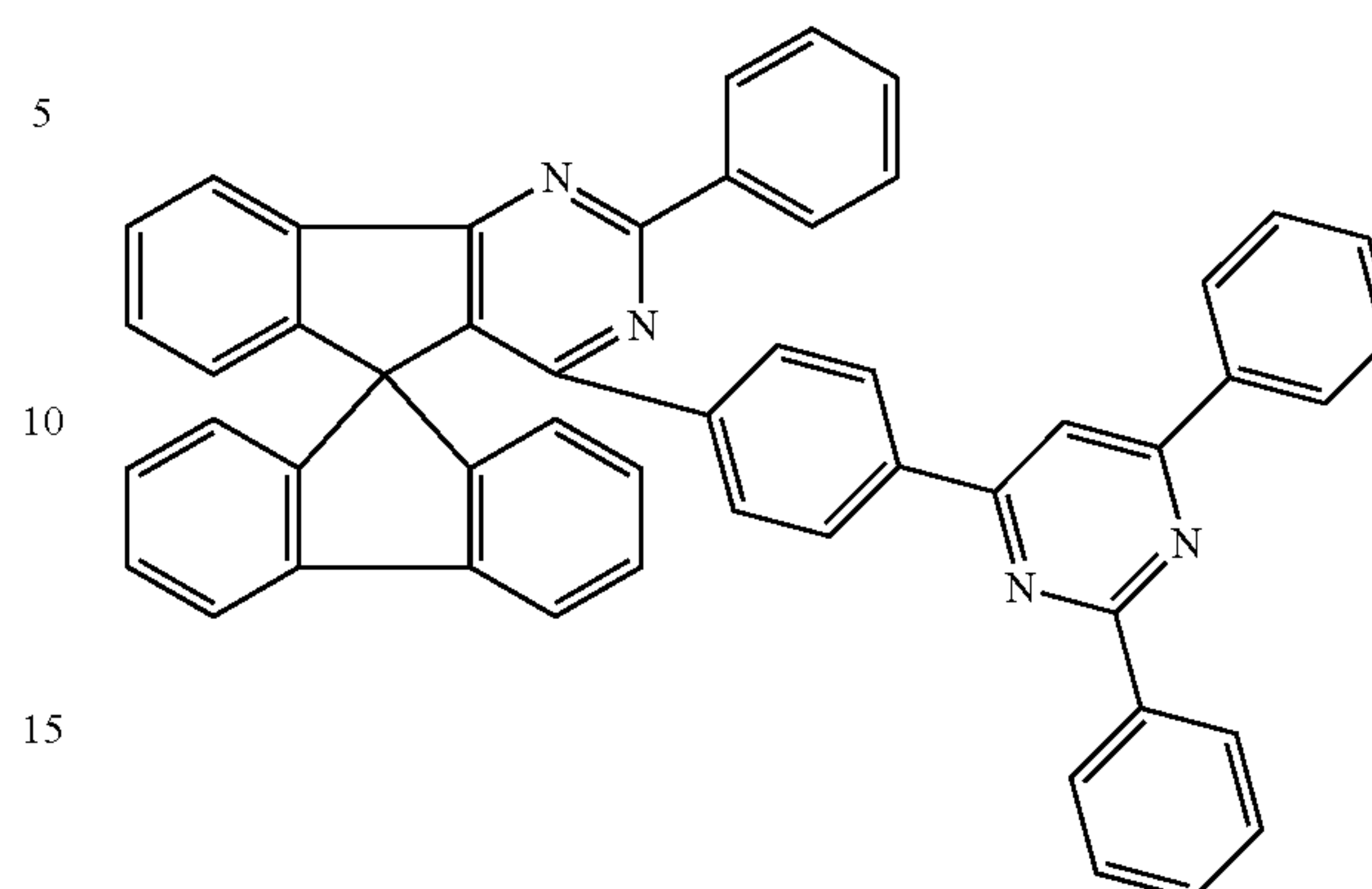
Chemical Formula 1-91
