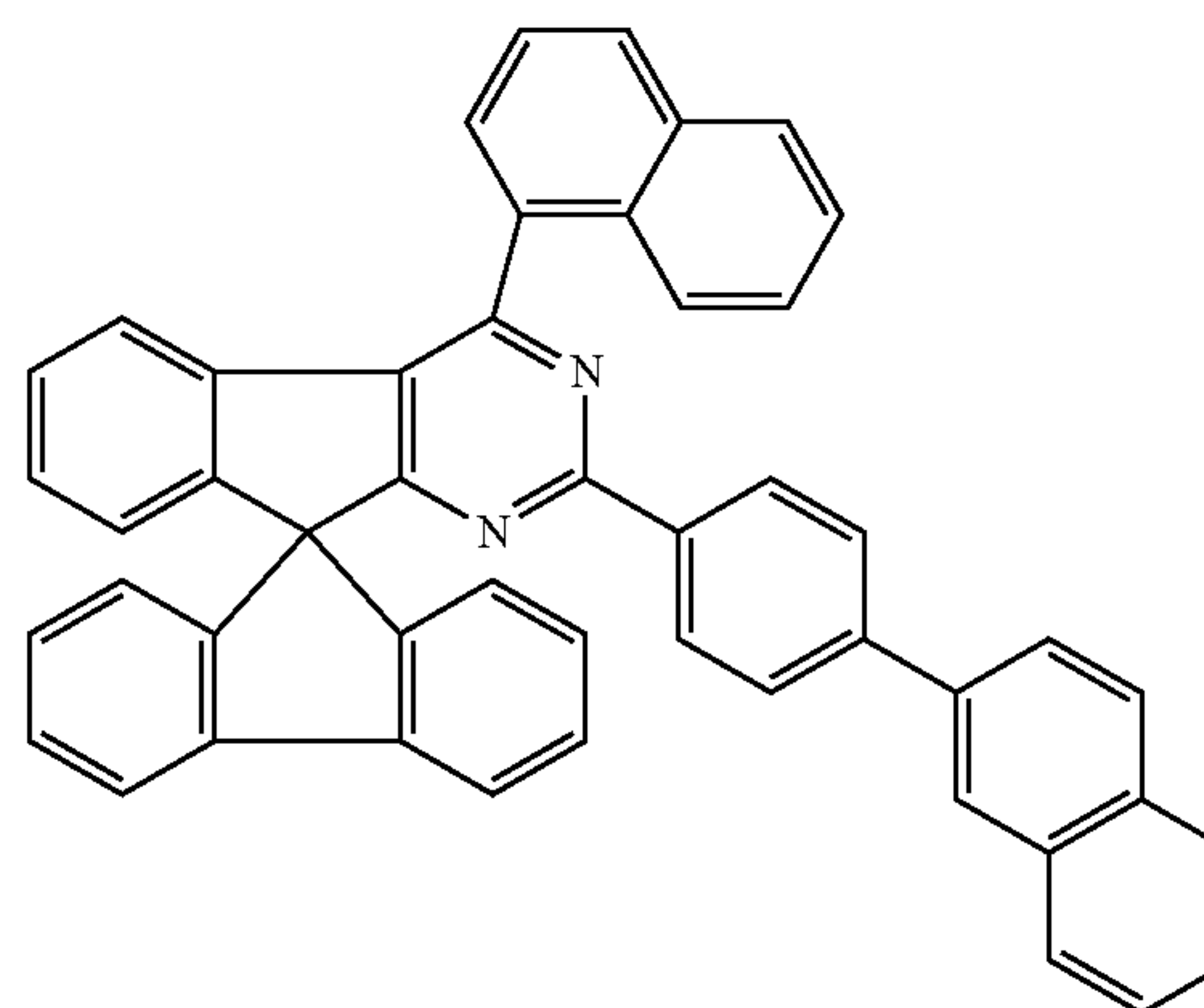
Chemical Formula 1-67
