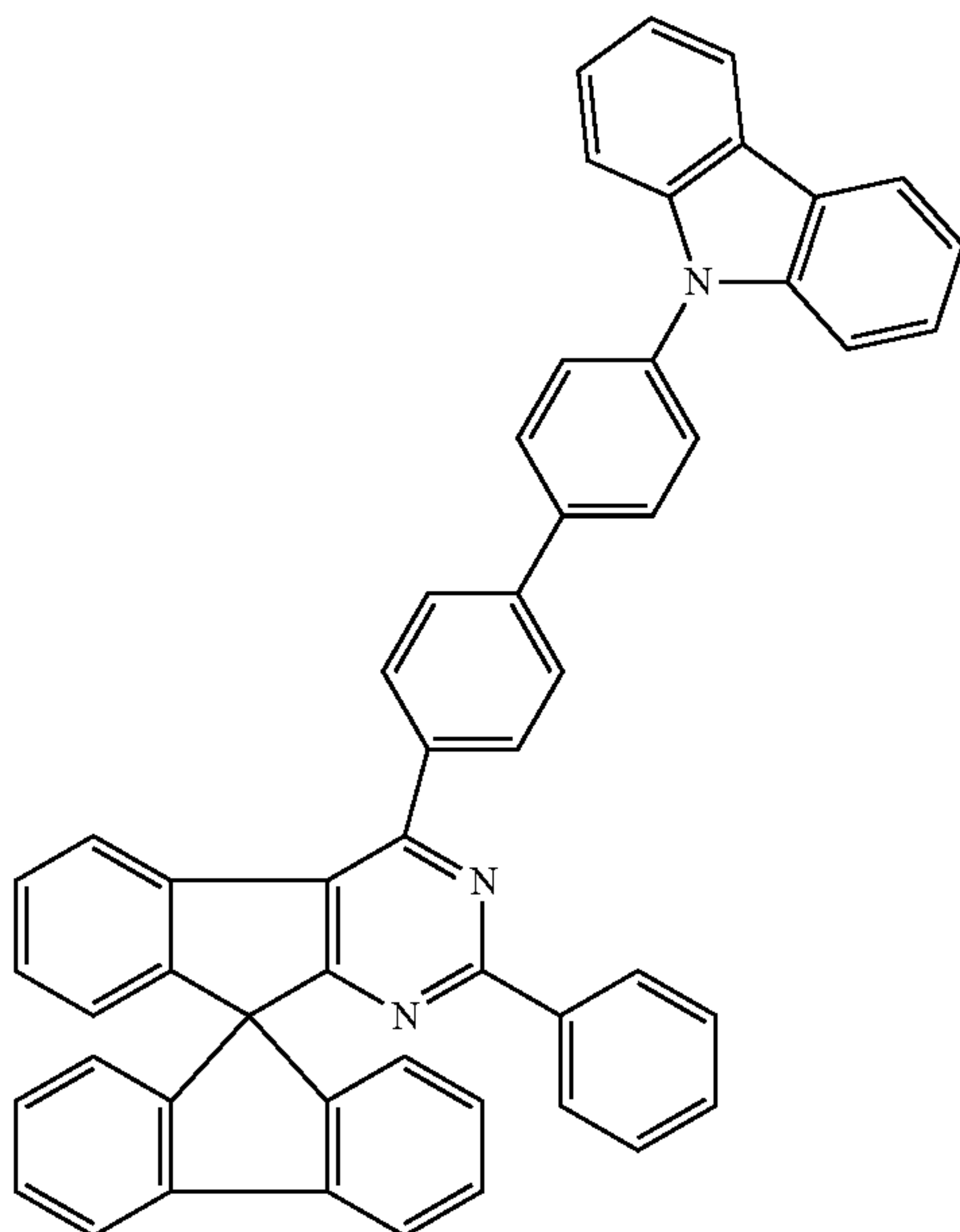
Chemical Formula 1-88
