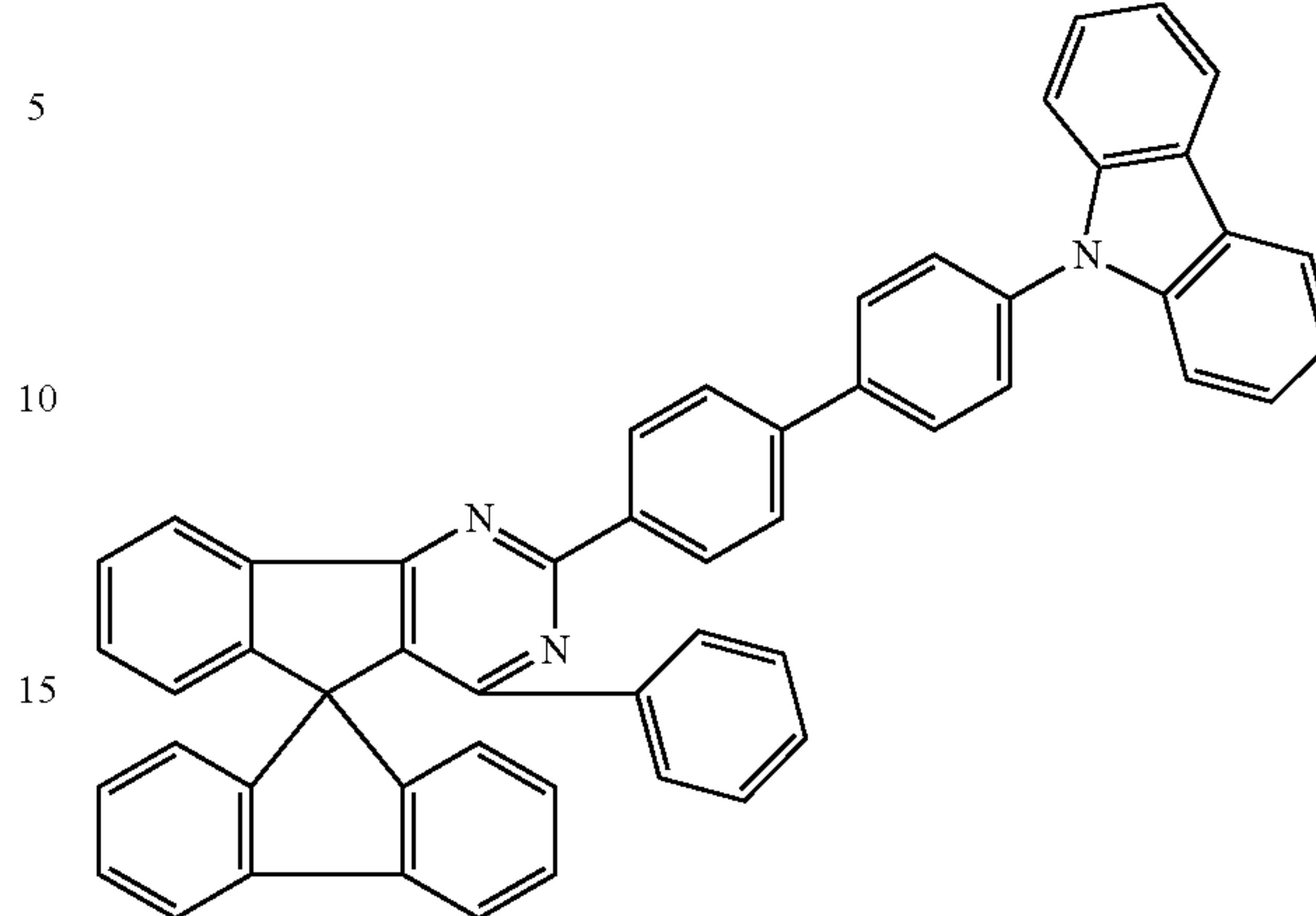
Chemical Formula 1-70
