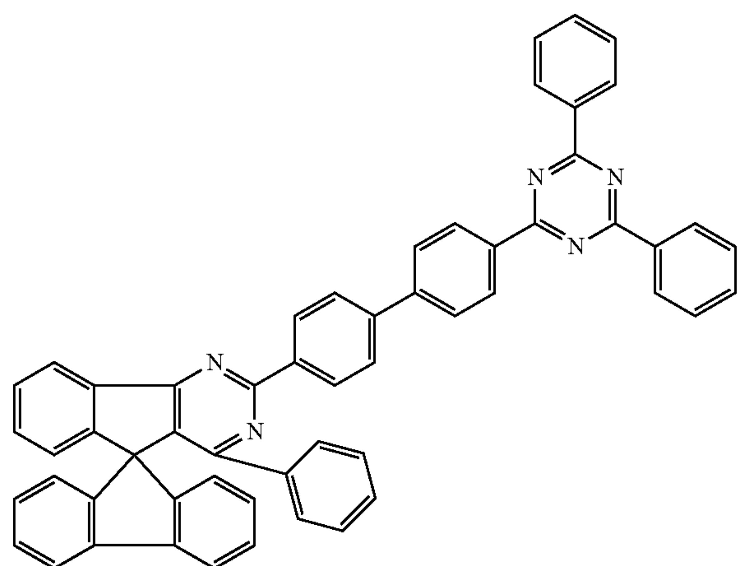
Chemical Formula 1-96
