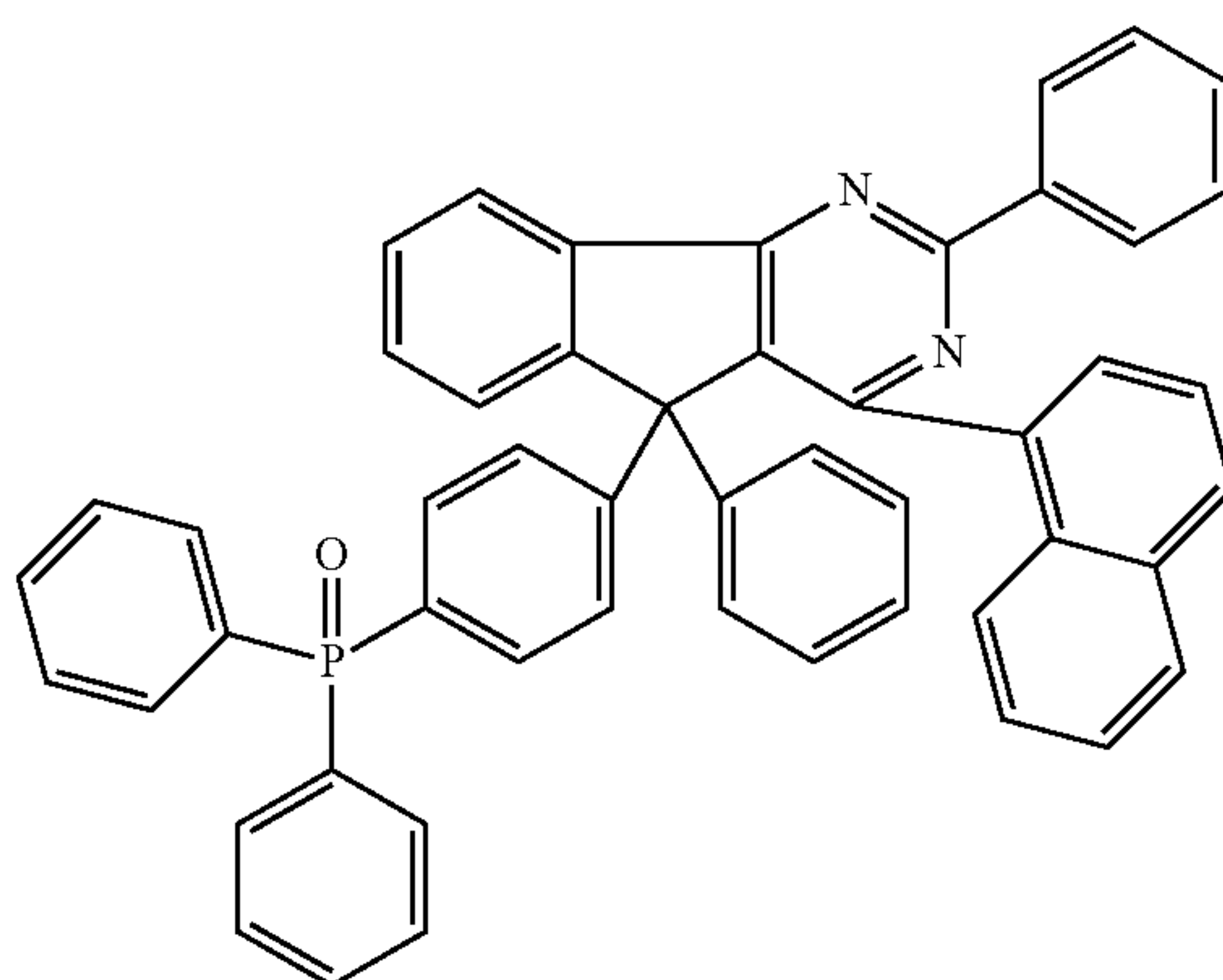
Chemical Formula 2-17
