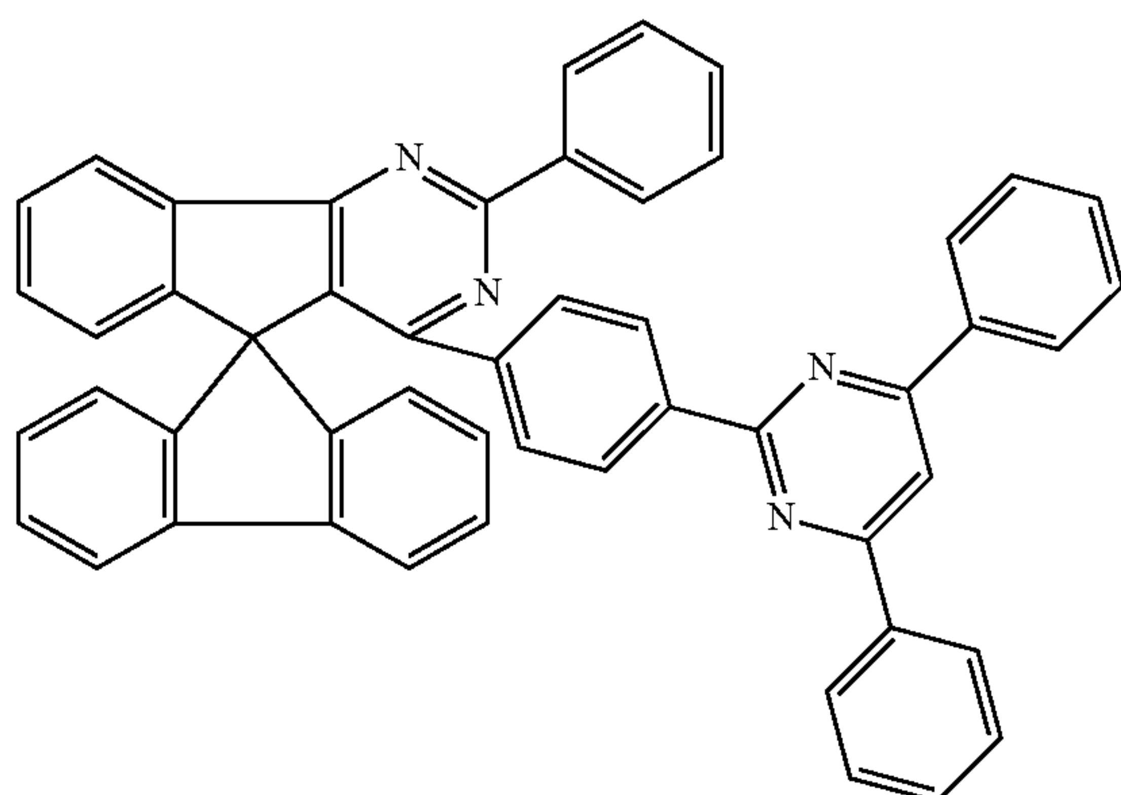
Chemical Formula 1-93
