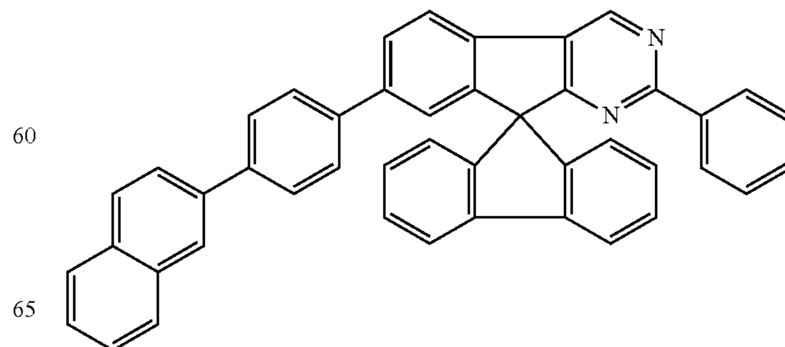
Chemical Formula 1-26
