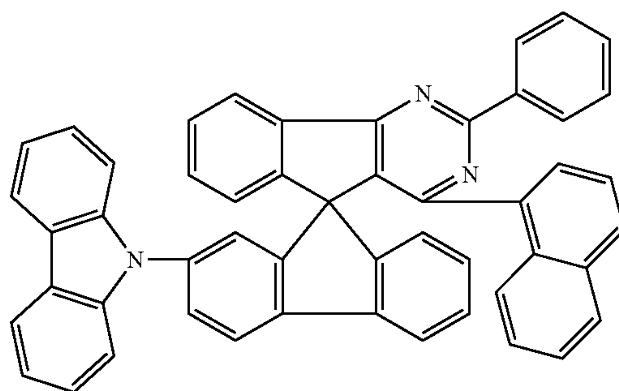
Chemical Formula 1-29
