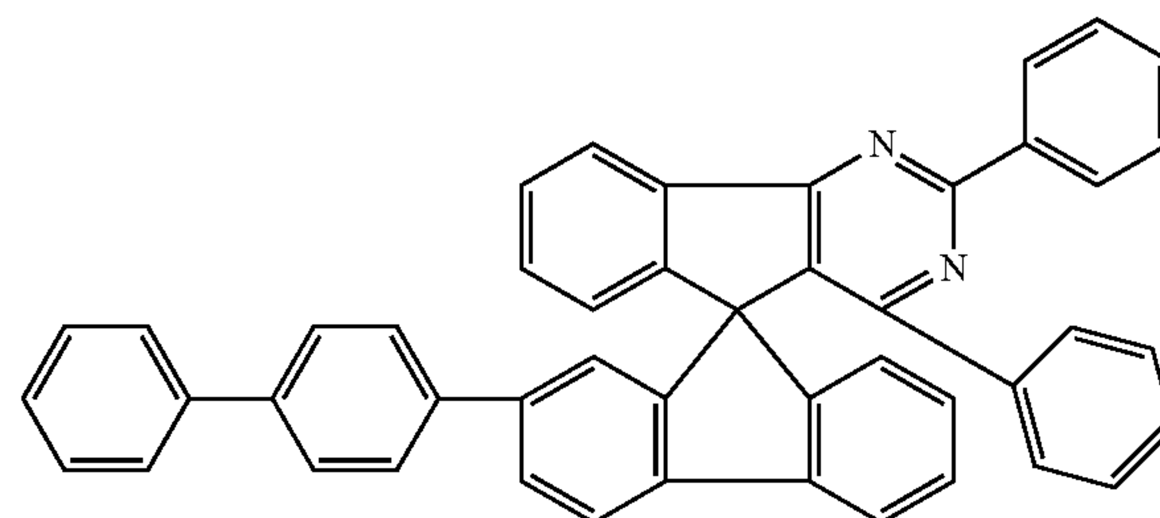
Chemical Formula 1-8
