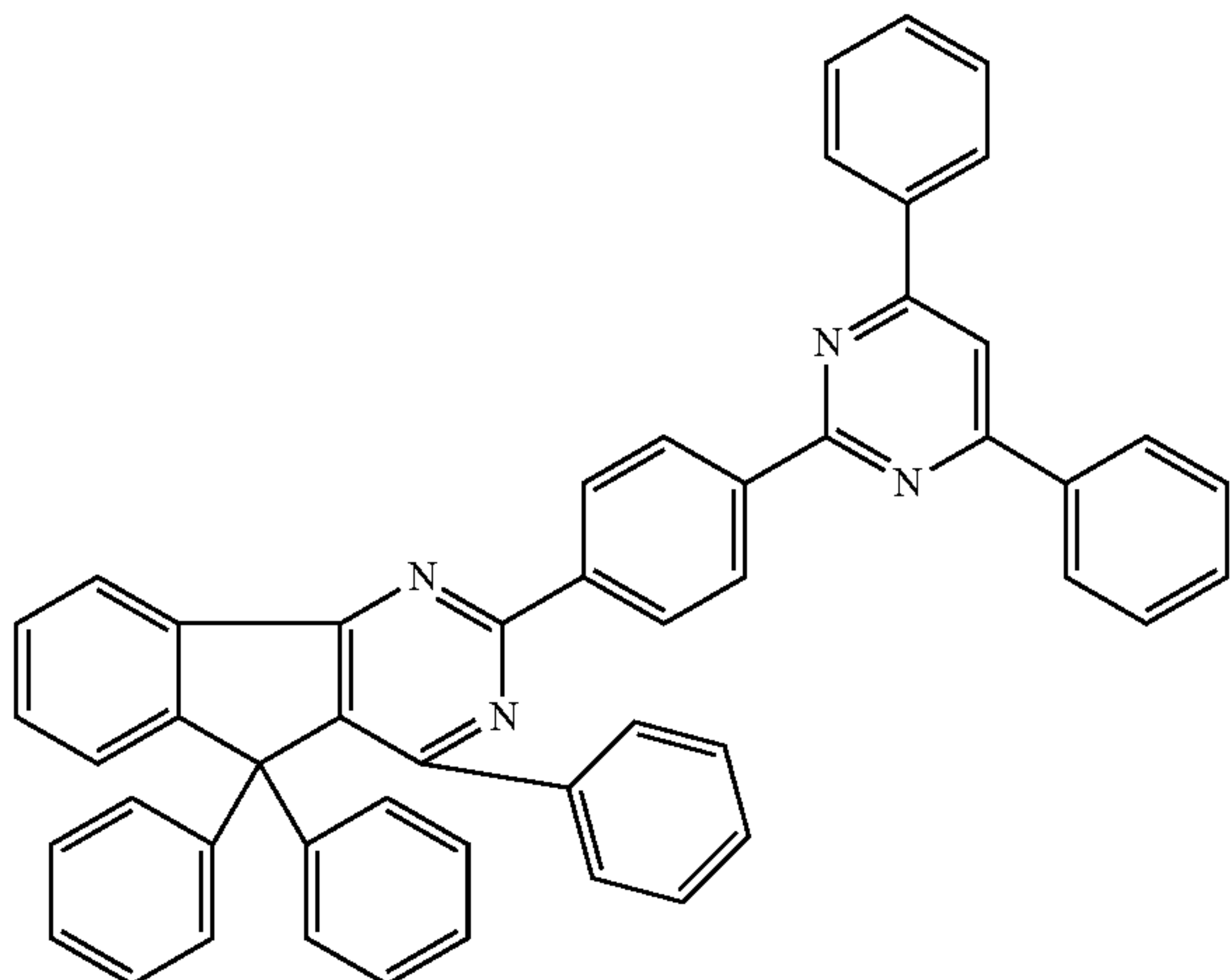
Chemical Formula 2-48
