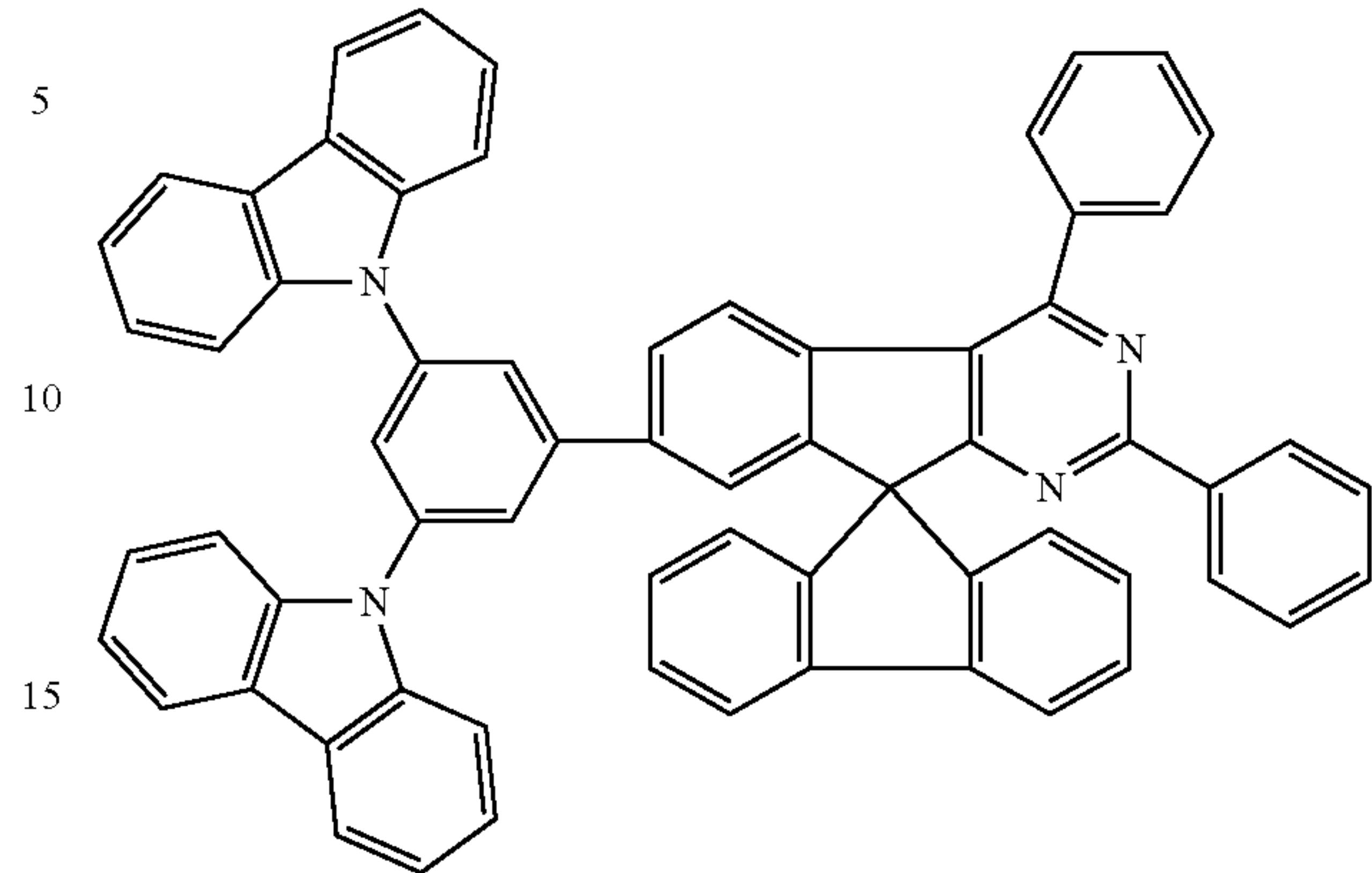
Chemical Formula 1-69
