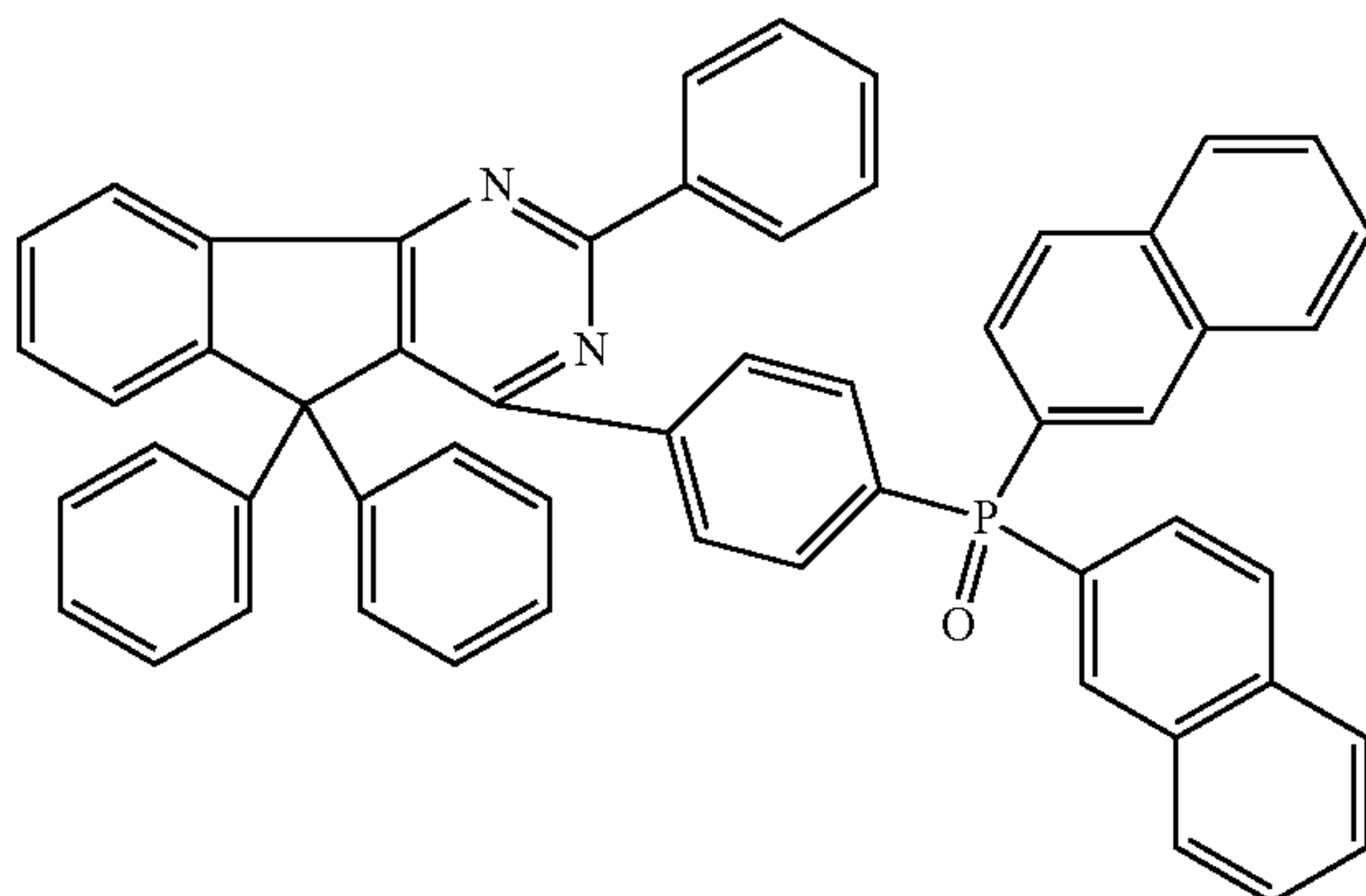
Chemical Formula 2-39
