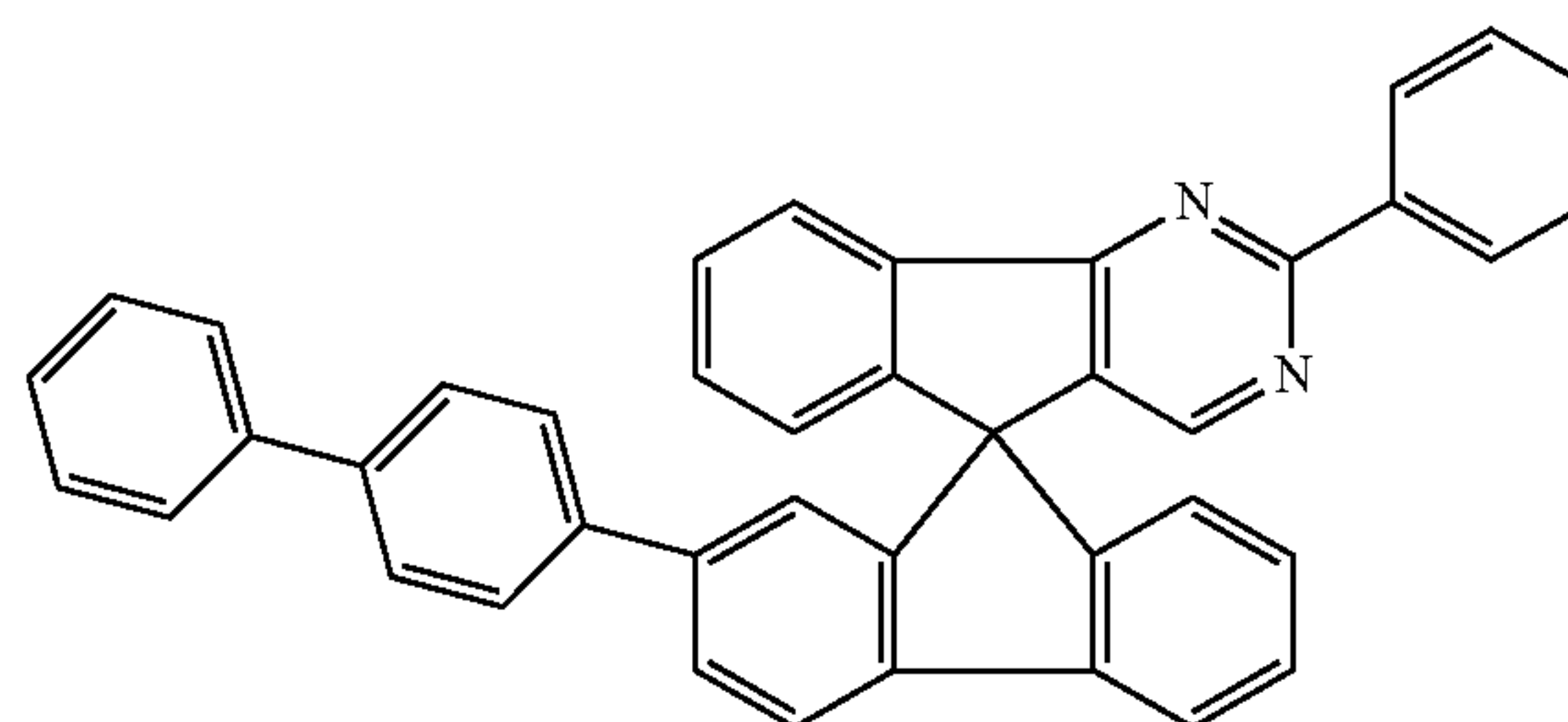
Chemical Formula 1-5
