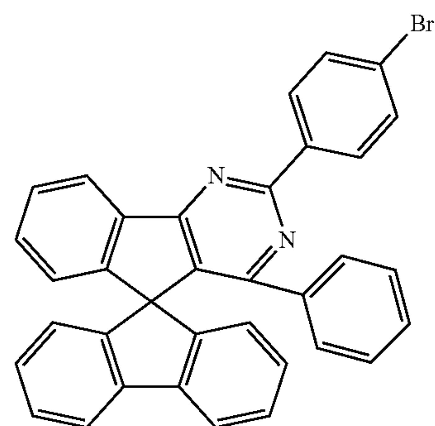
[Compound E-2]
