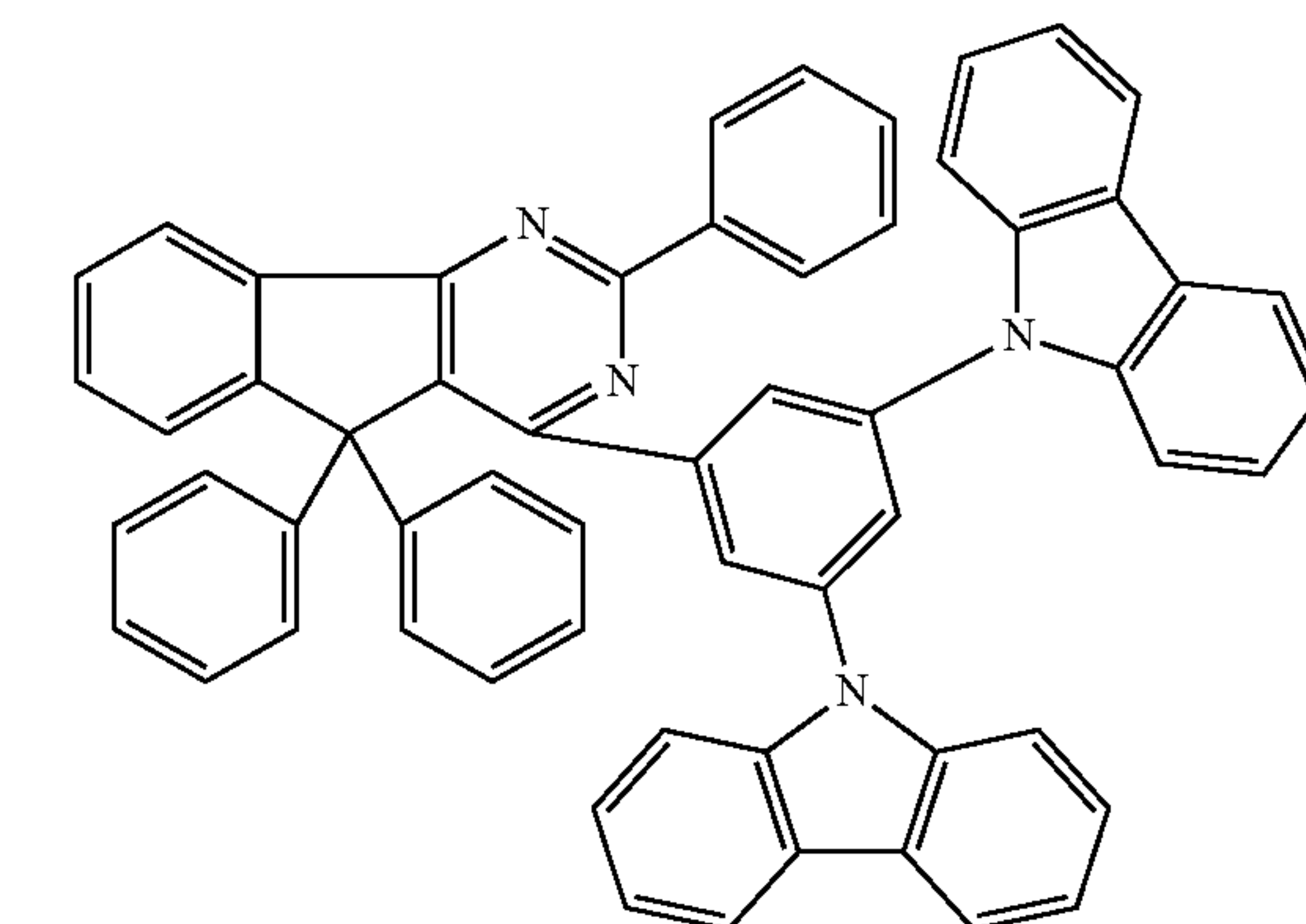
Chemical Formula 2-34
