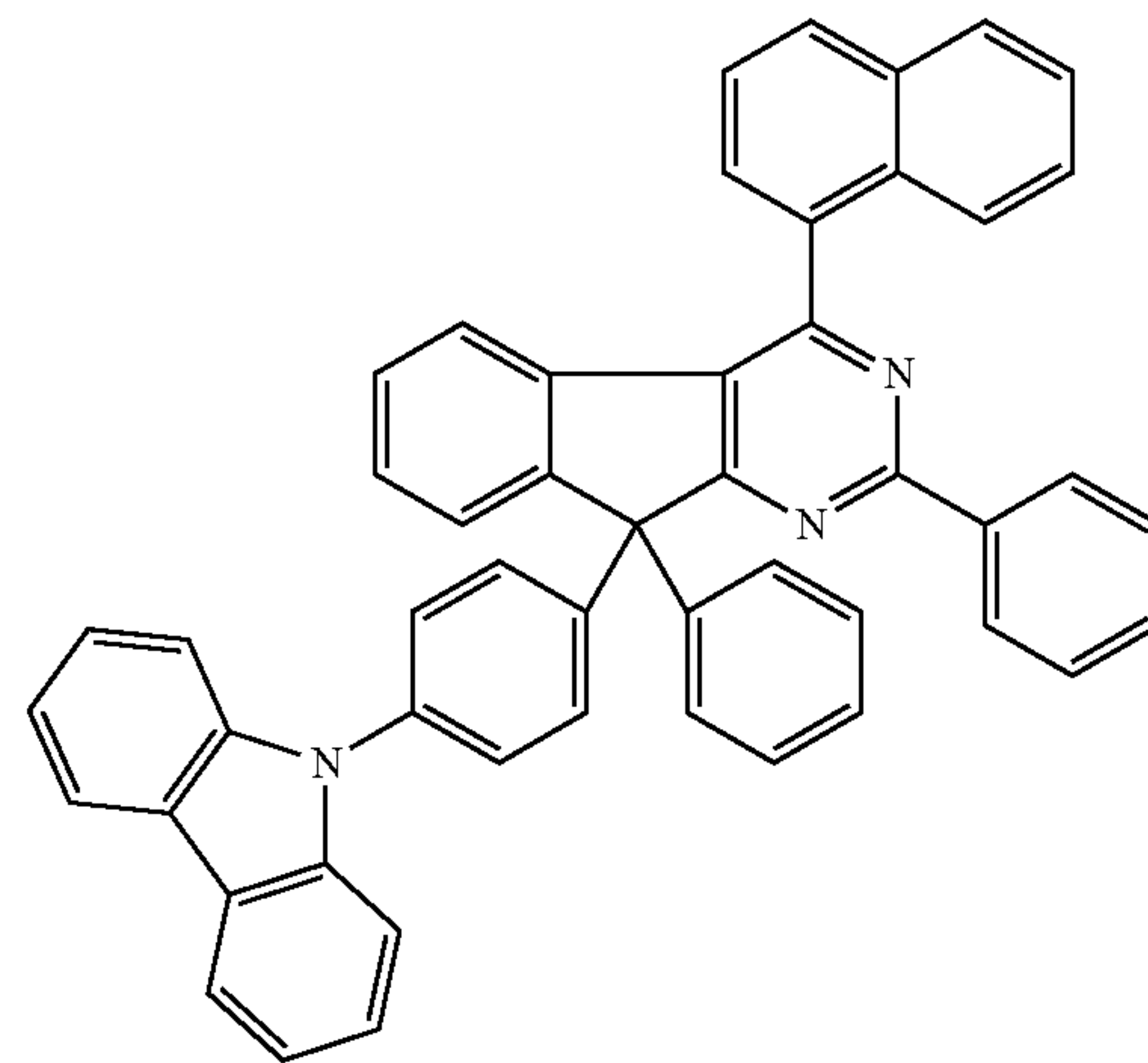
Chemical Formula 2-15
