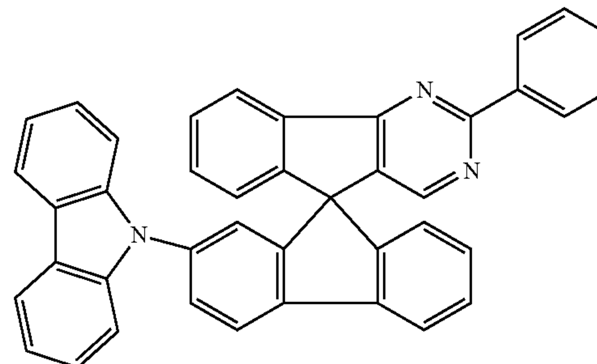
Chemical Formula 1-1
