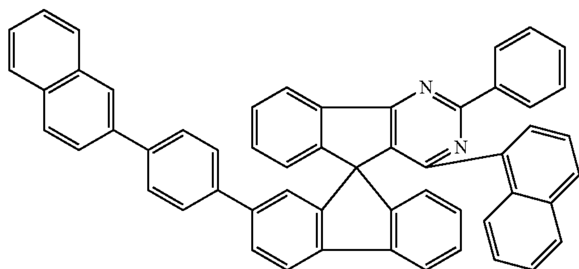
Chemical Formula 1-37
