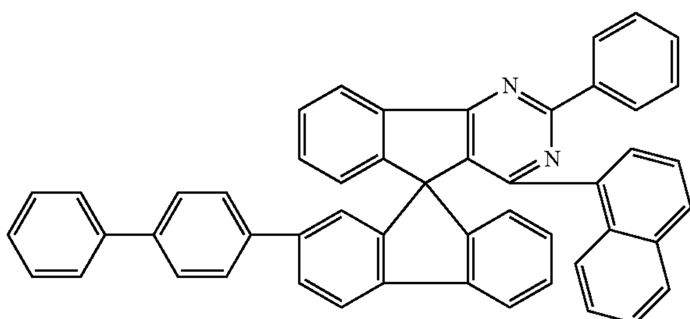
Chemical Formula 1-31
