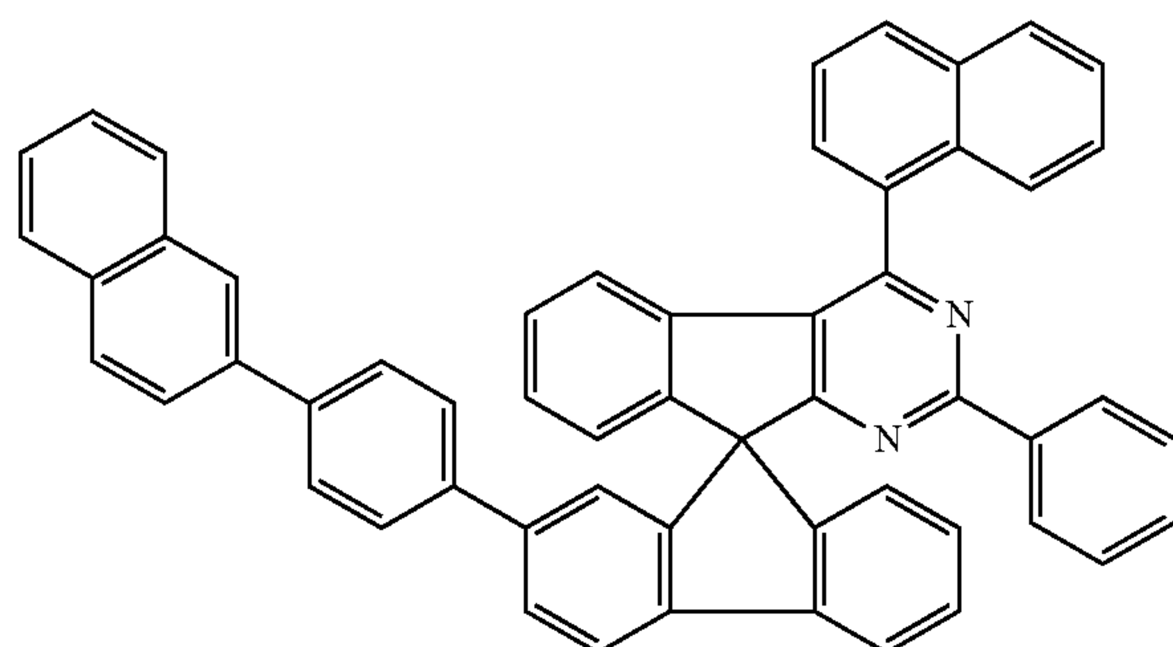
Chemical Formula 1-38
