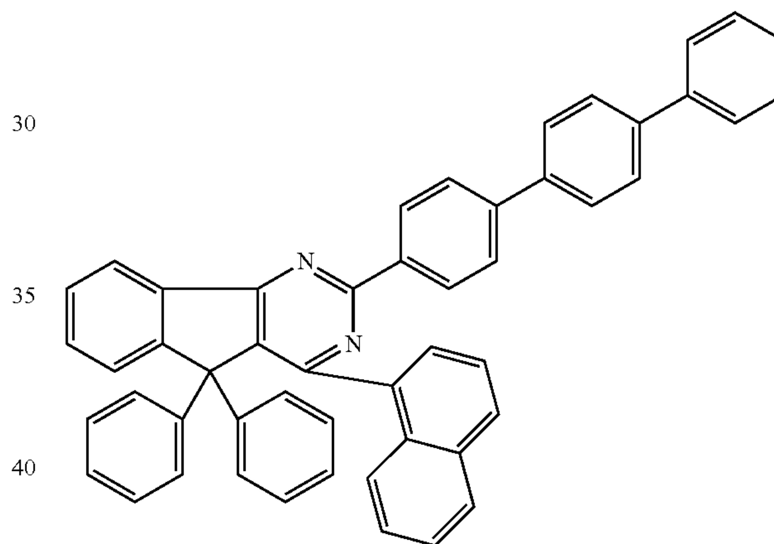
Chemical Formula 2-27
