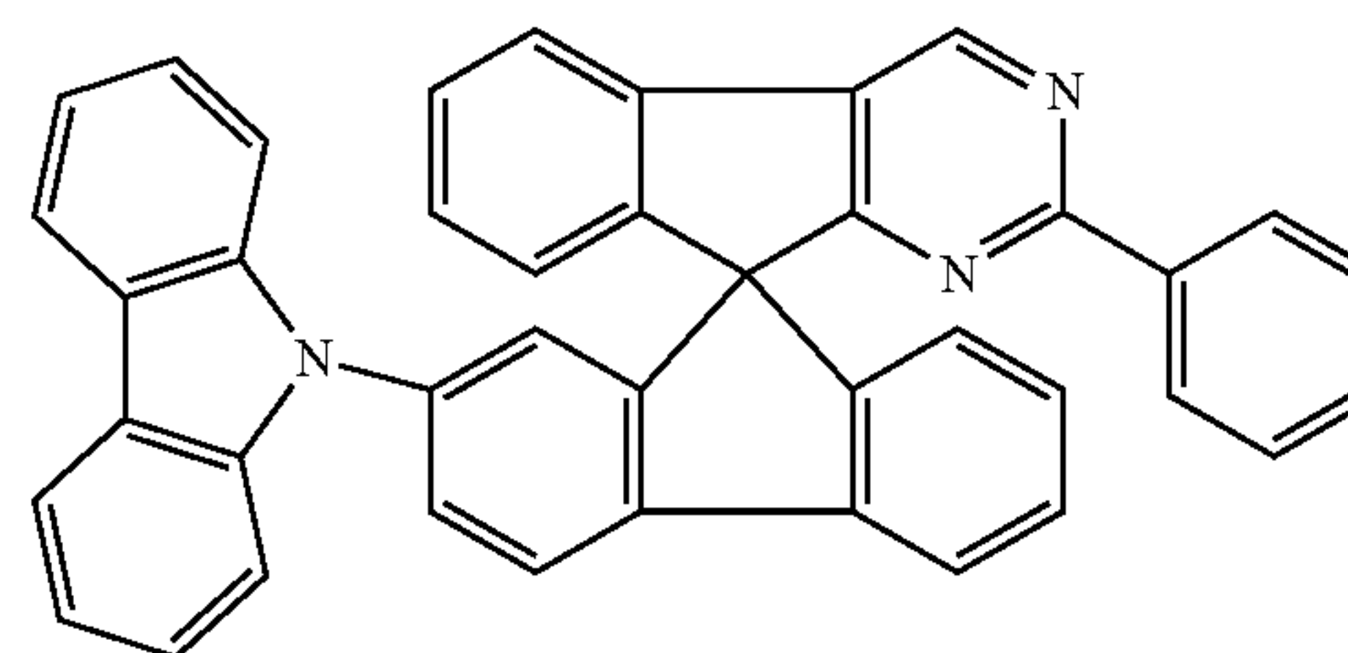
Chemical Formula 1-3
