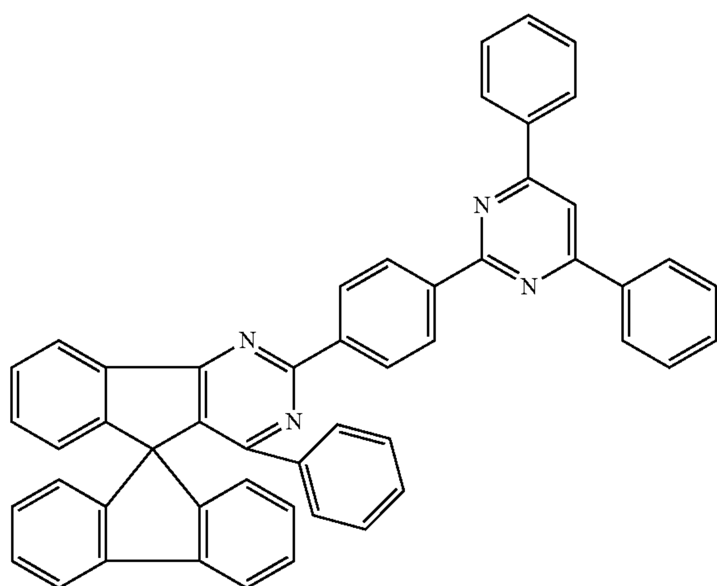
Chemical Formula 1-94
