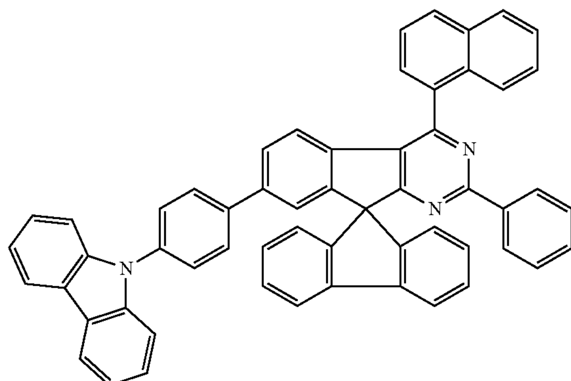
Chemical Formula 1-36
