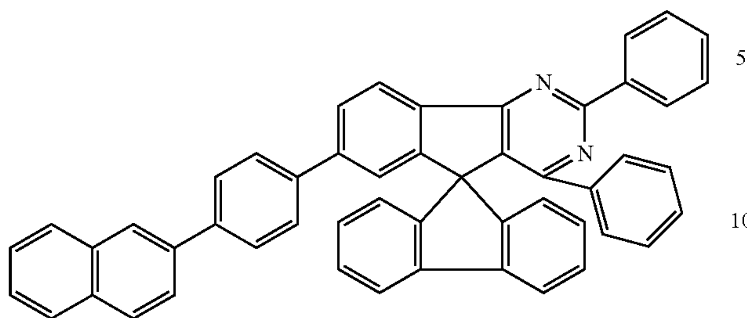
Chemical Formula 1-27
