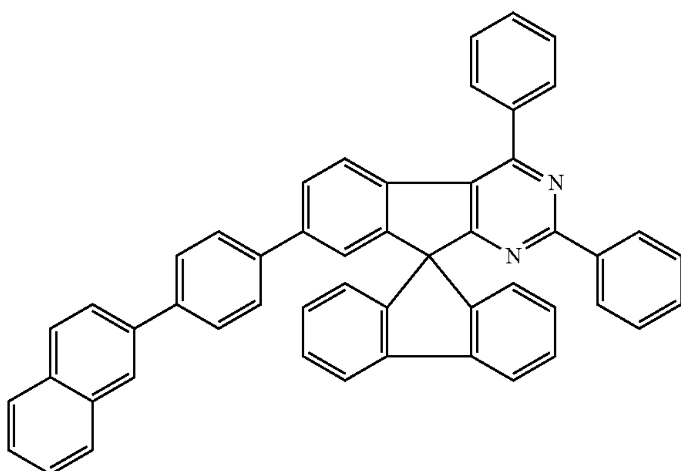
Chemical Formula 1-28
