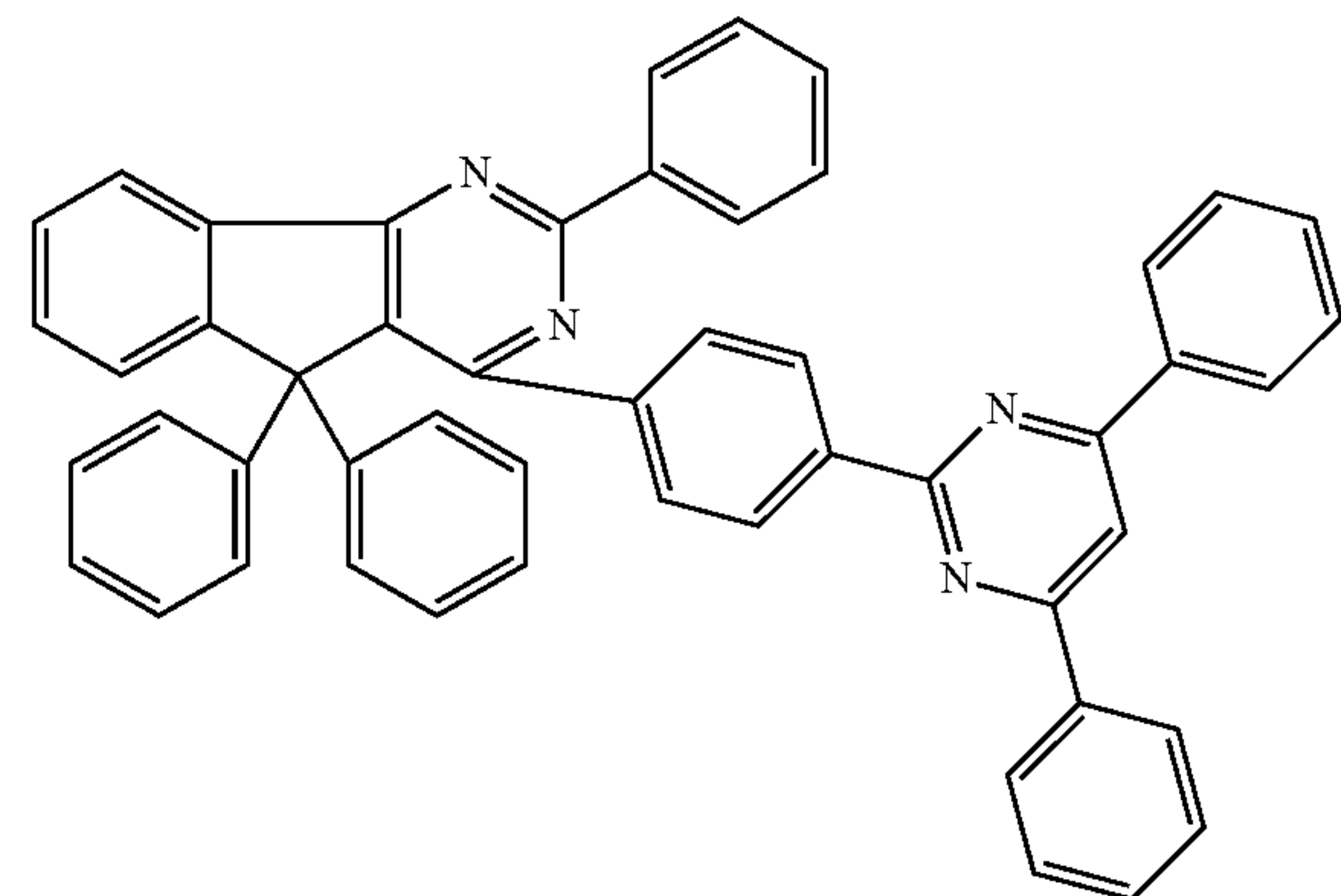
Chemical Formula 2-48
