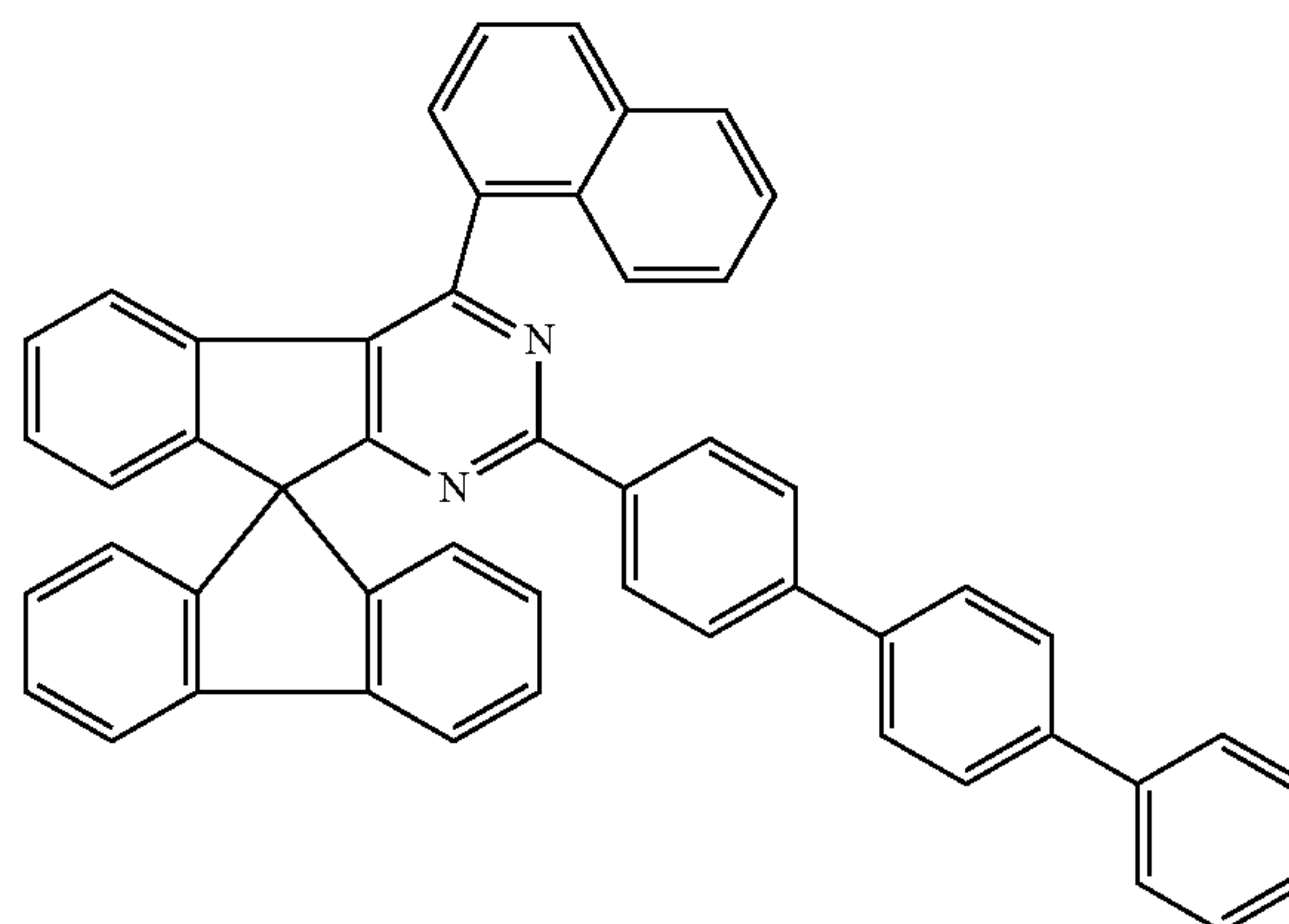
Chemical Formula 1-62
