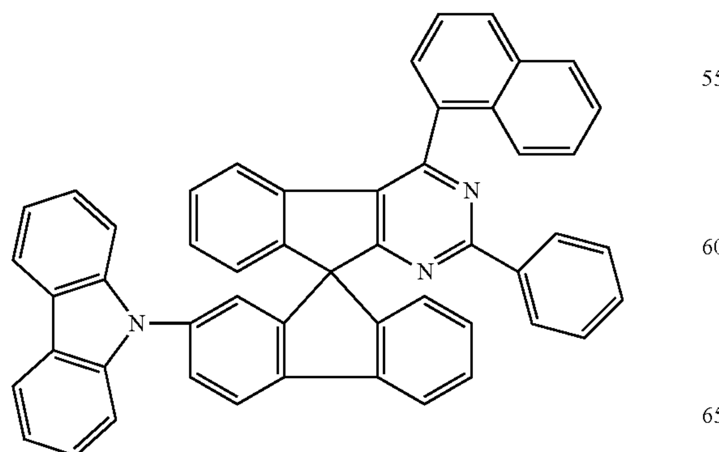
Chemical Formula 1-30
