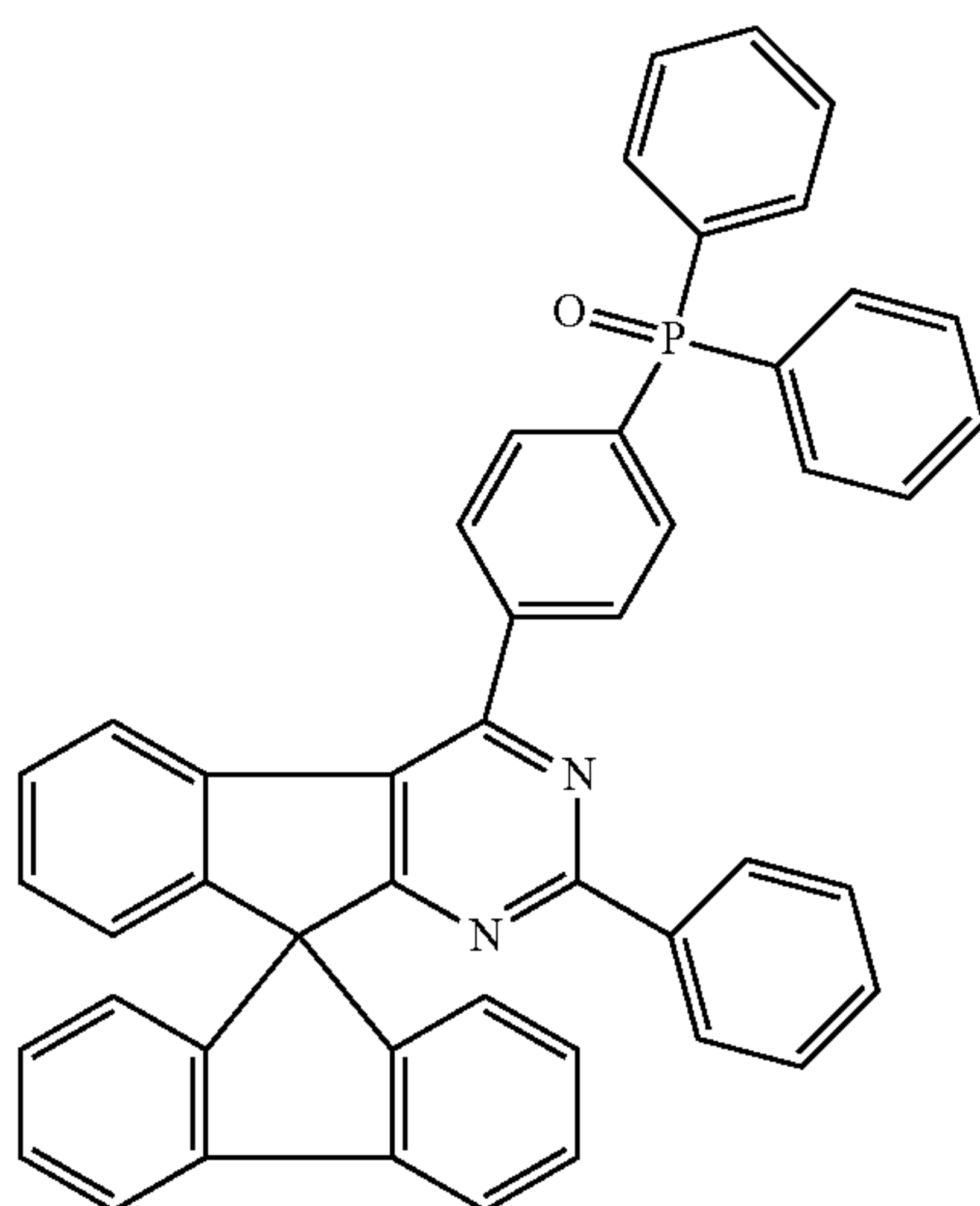
Chemical Formula 1-76
