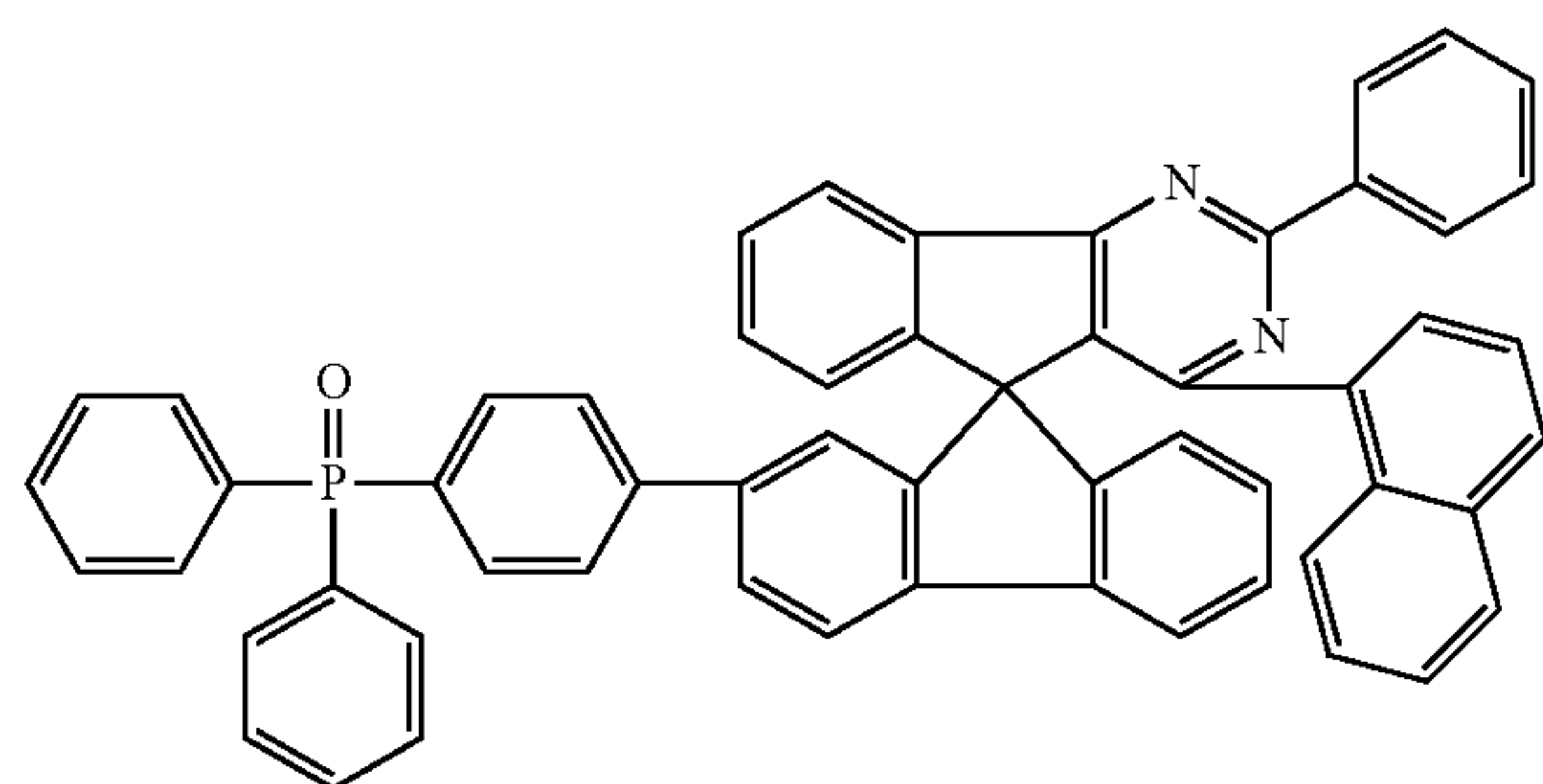
Chemical Formula 1-47
