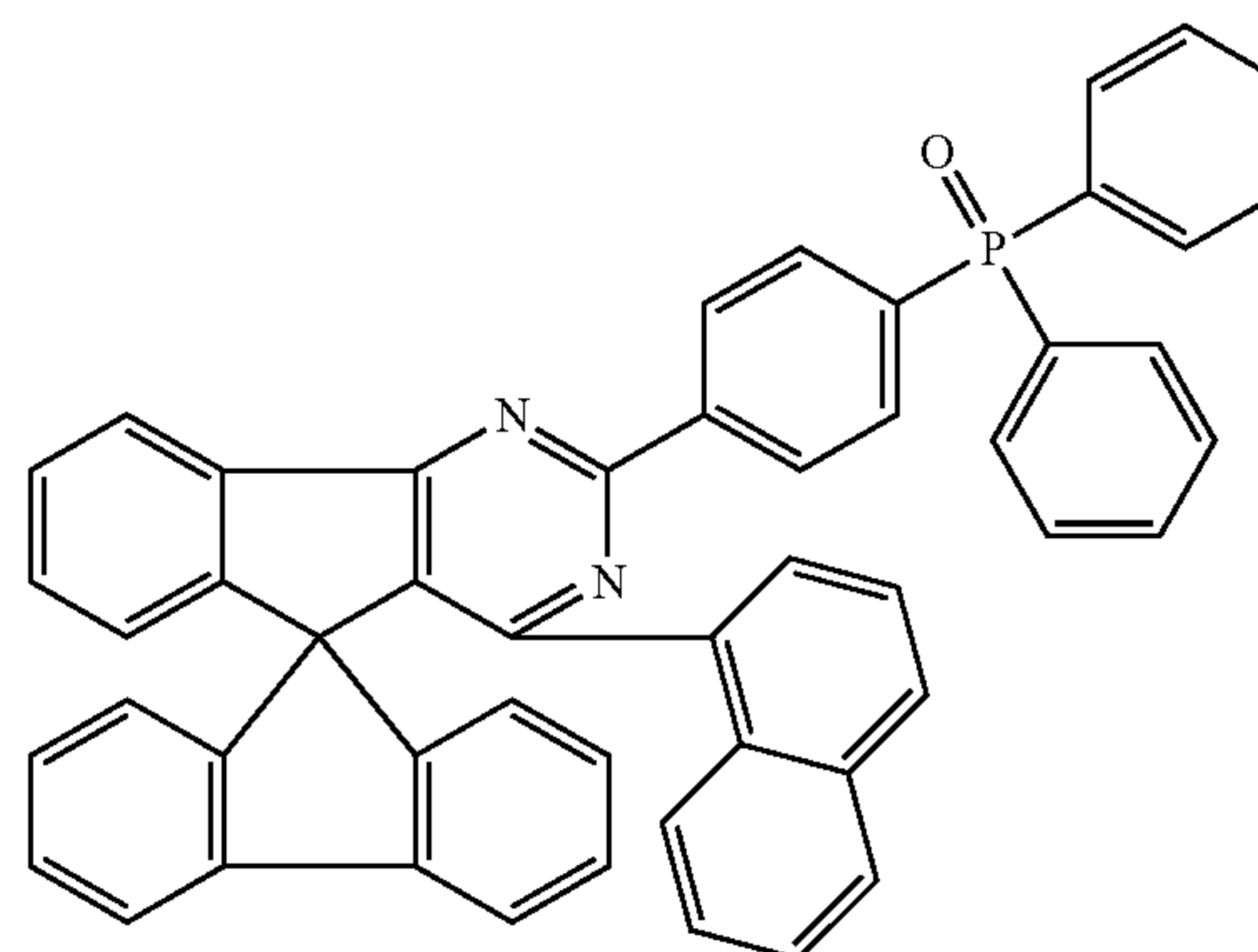
Chemical Formula 1-51
