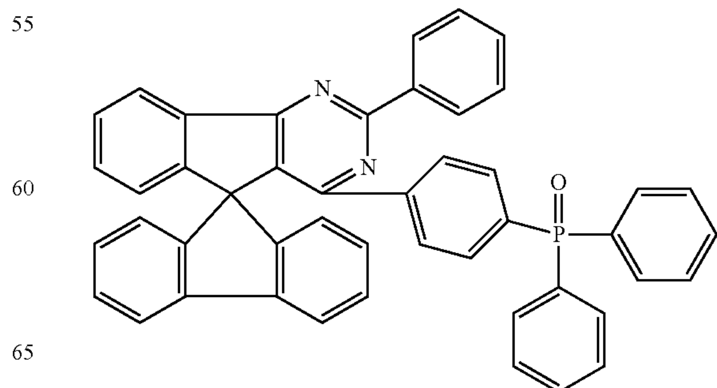
Chemical Formula 1-75
