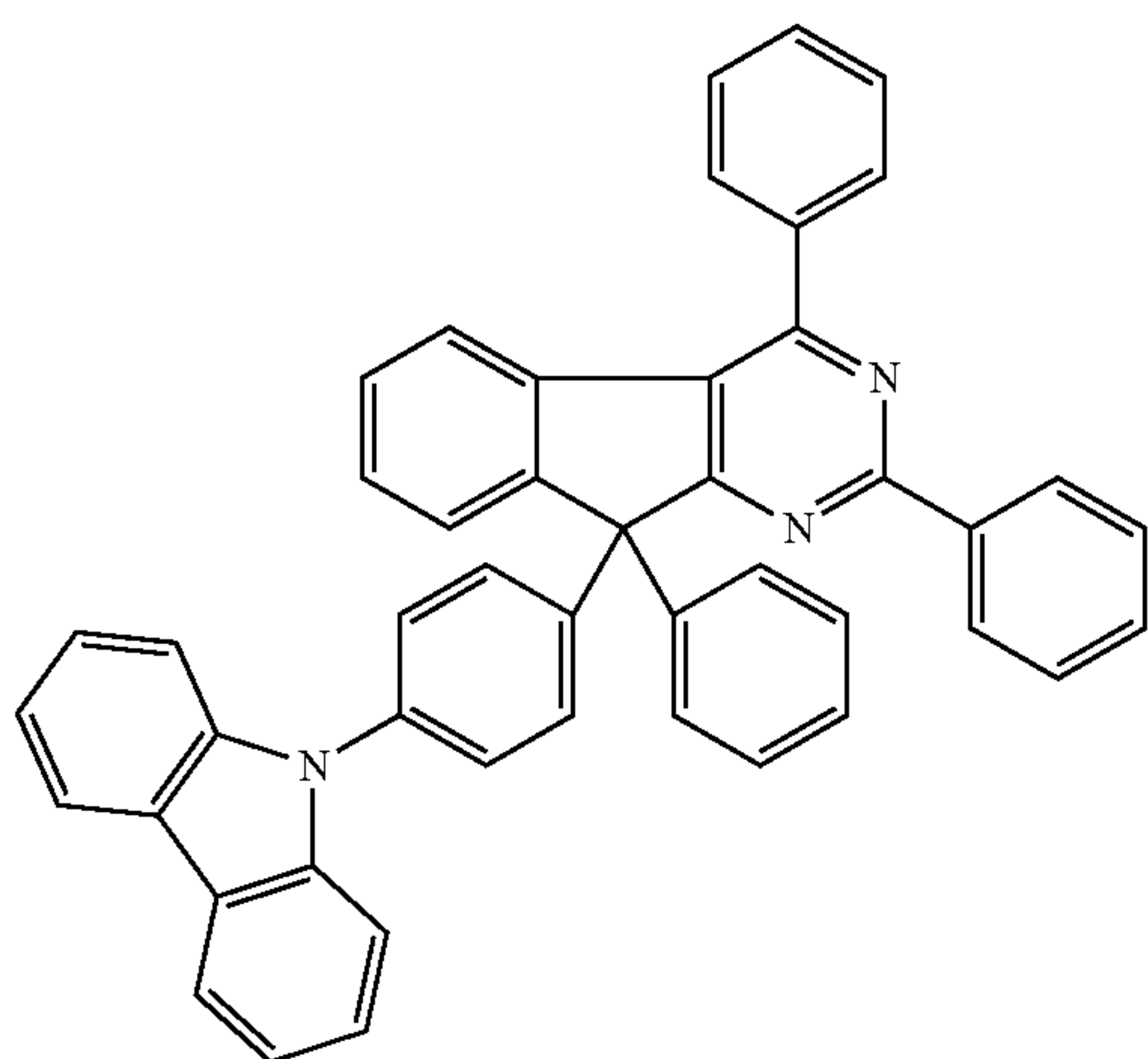
Chemical Formula 2-10
