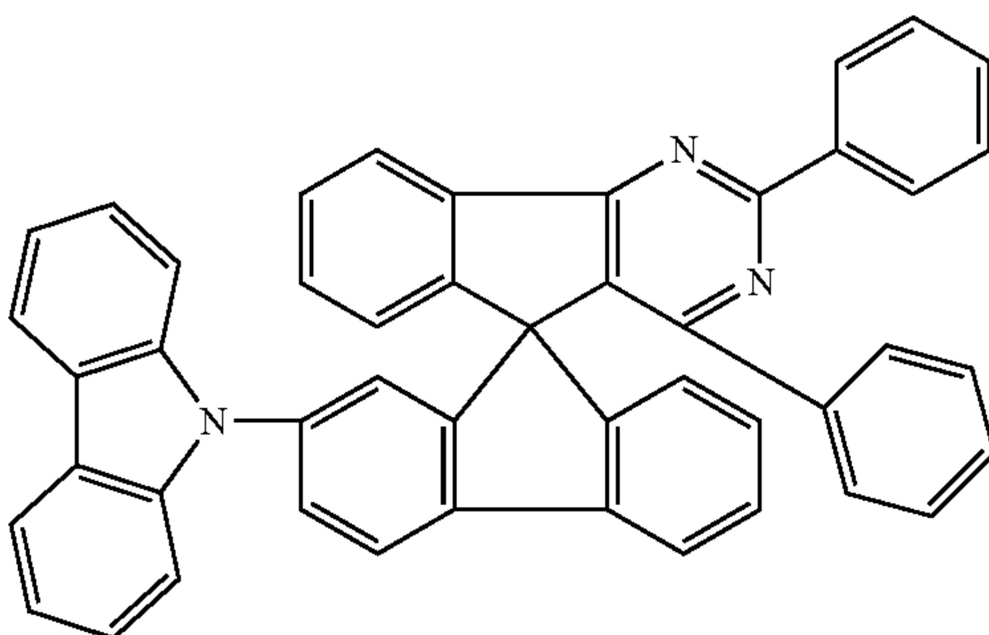
Chemical Formula 1-3
