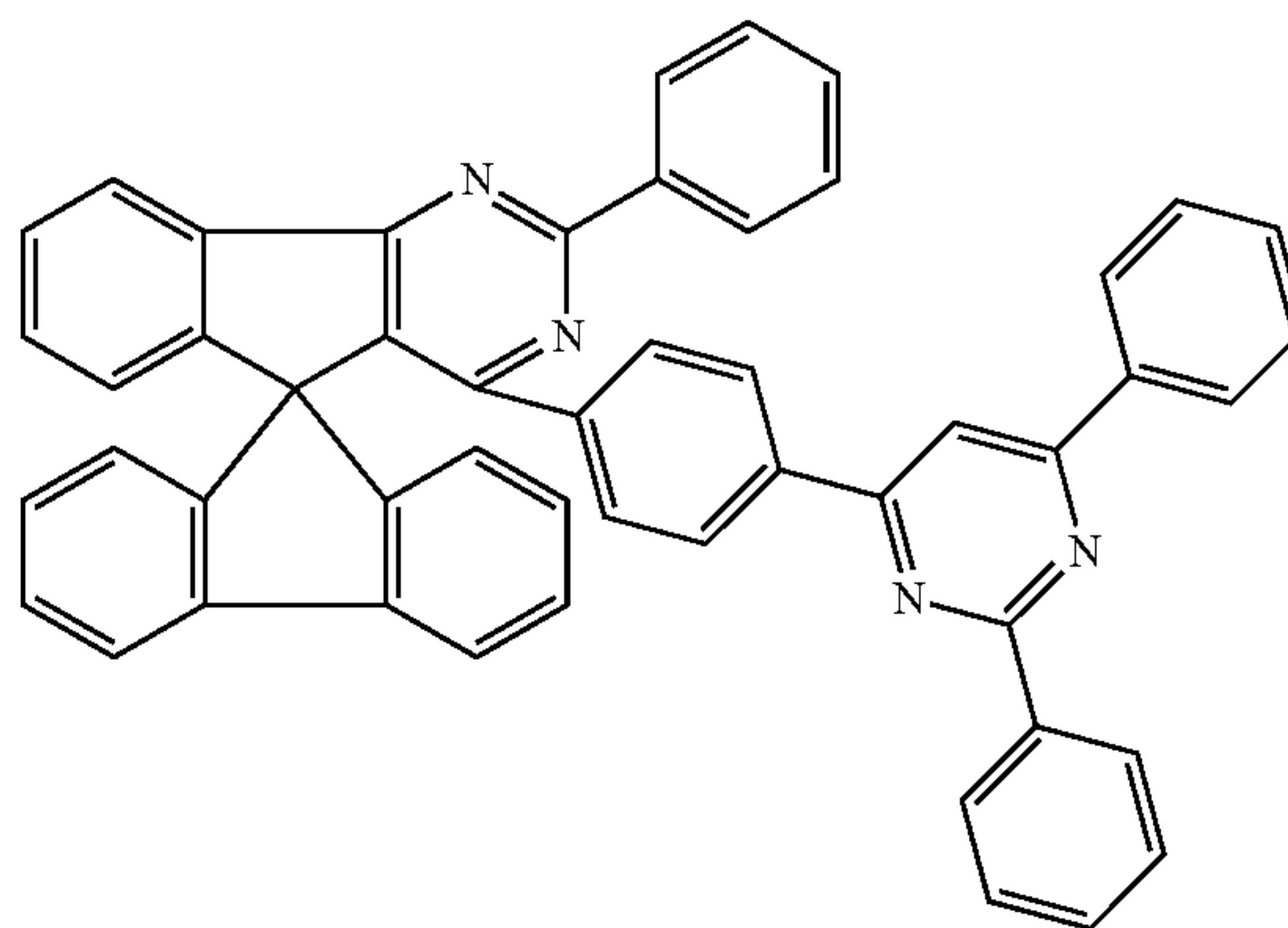
Chemical Formula 1-91
