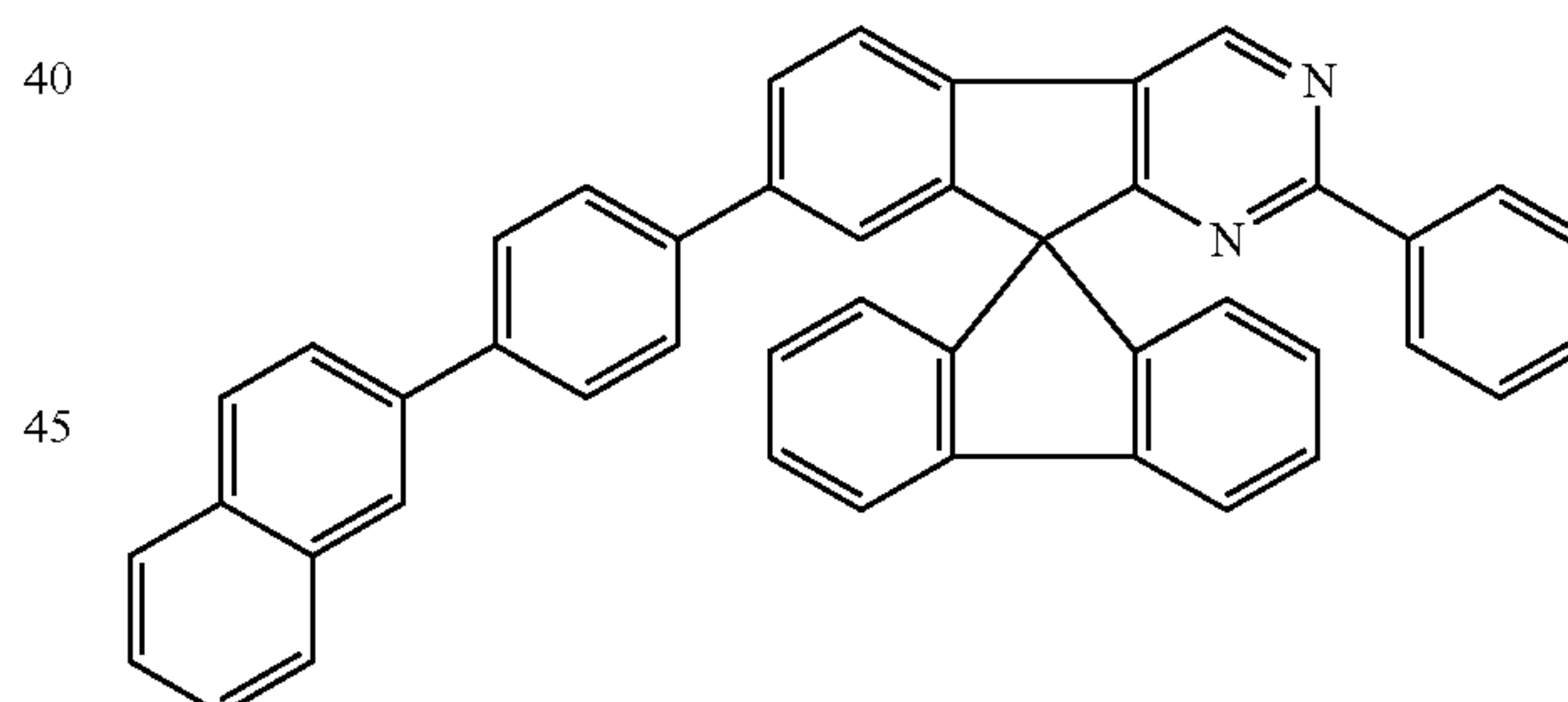
Chemical Formula 1-26
