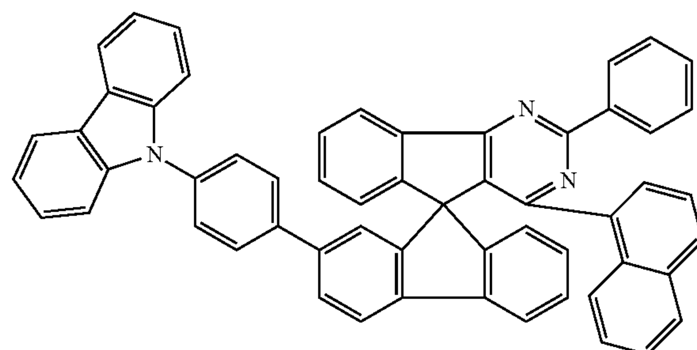
Chemical Formula 1-34
