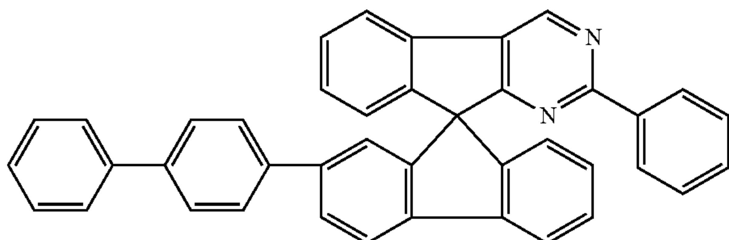
Chemical Formula 1-7
