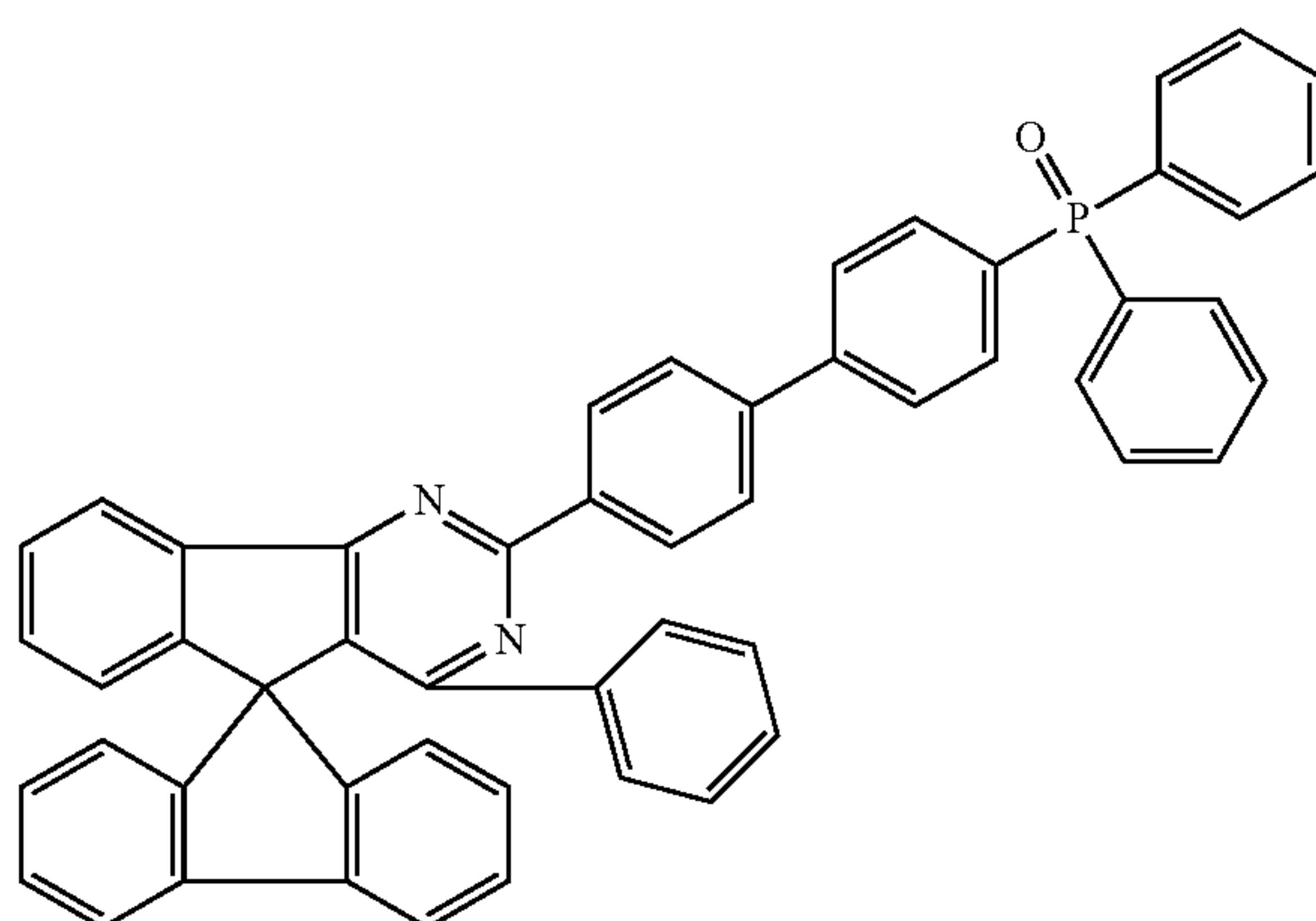
Chemical Formula 1-55
