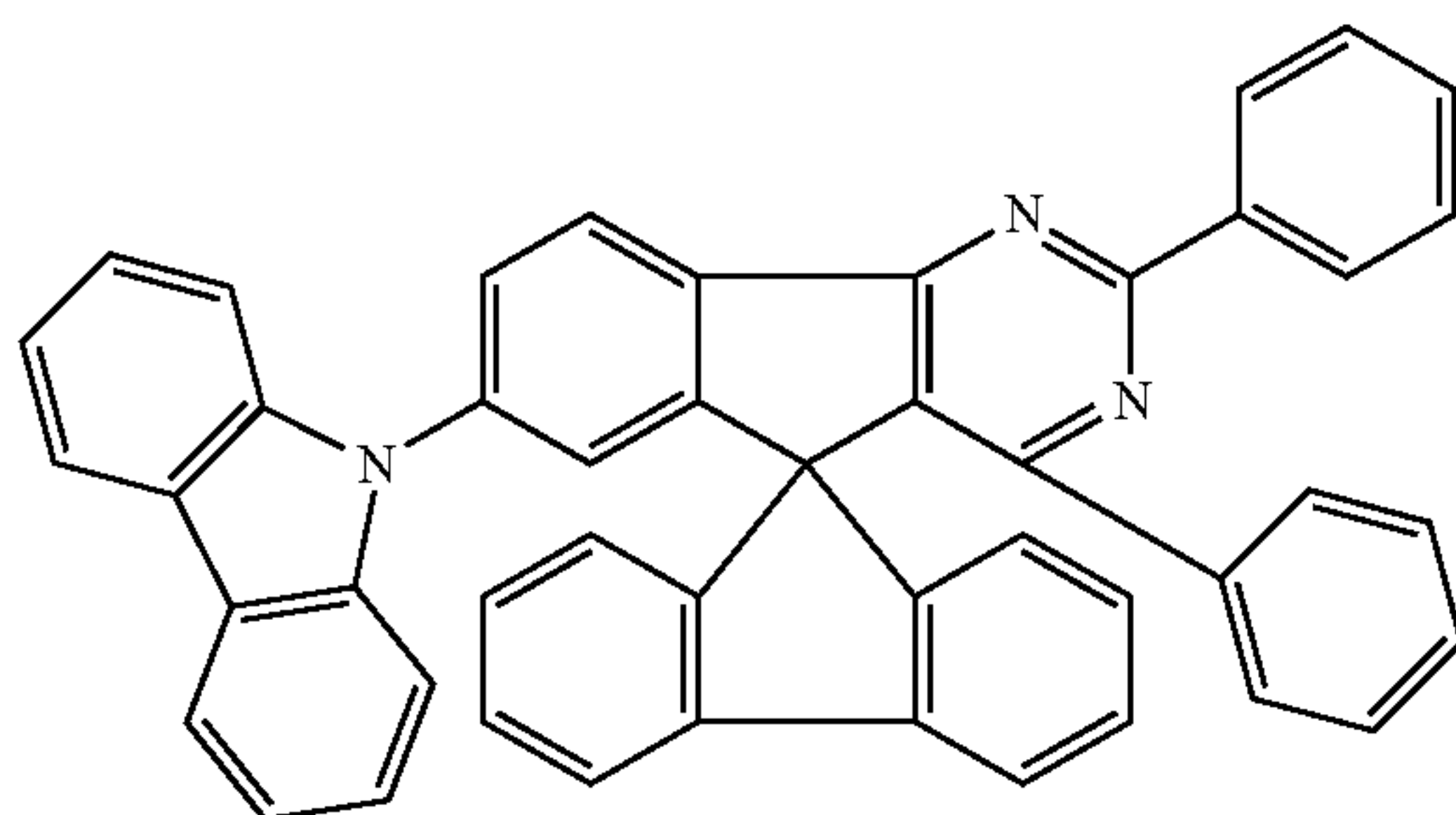
Chemical Formula 1-19
