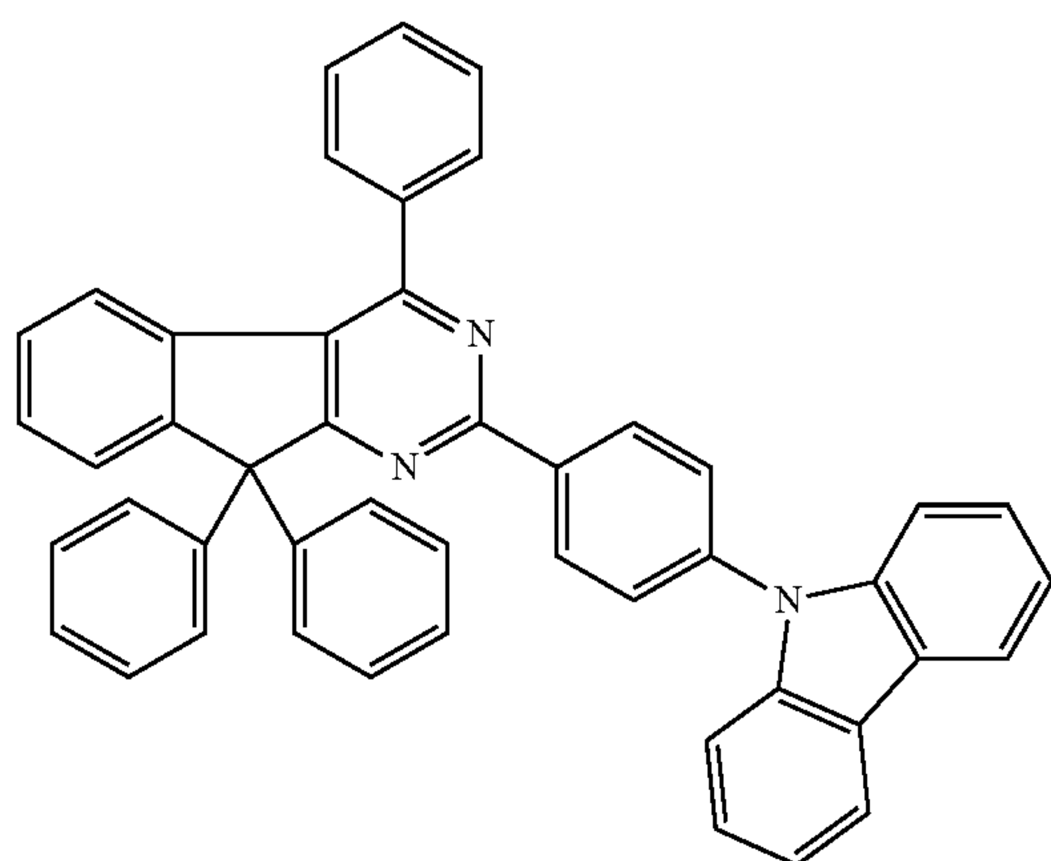
Chemical Formula 2-30
