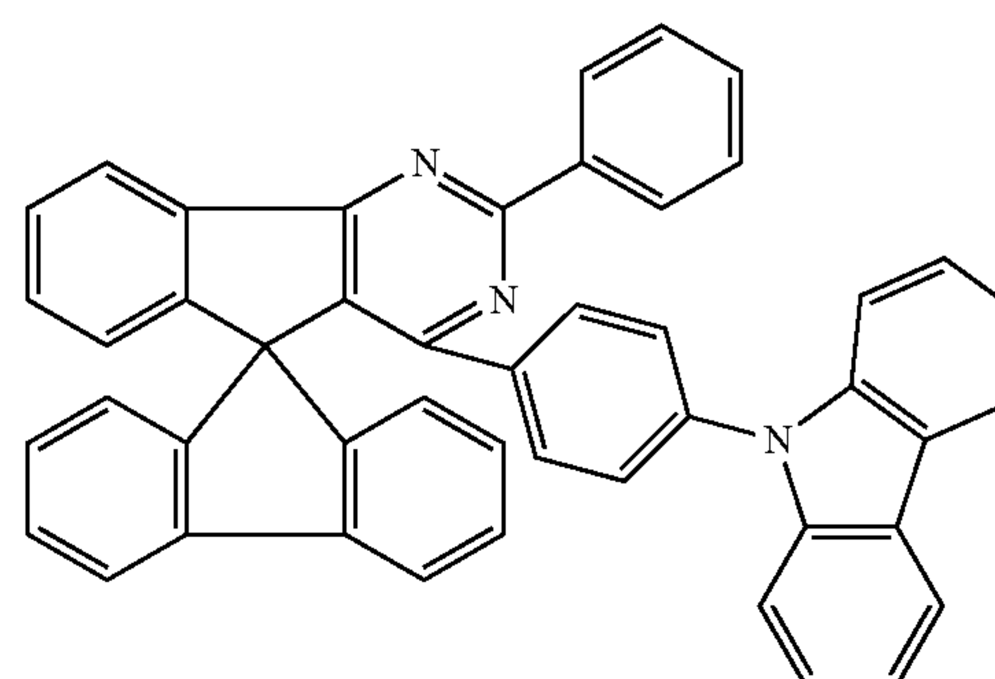
Chemical Formula 1-86
