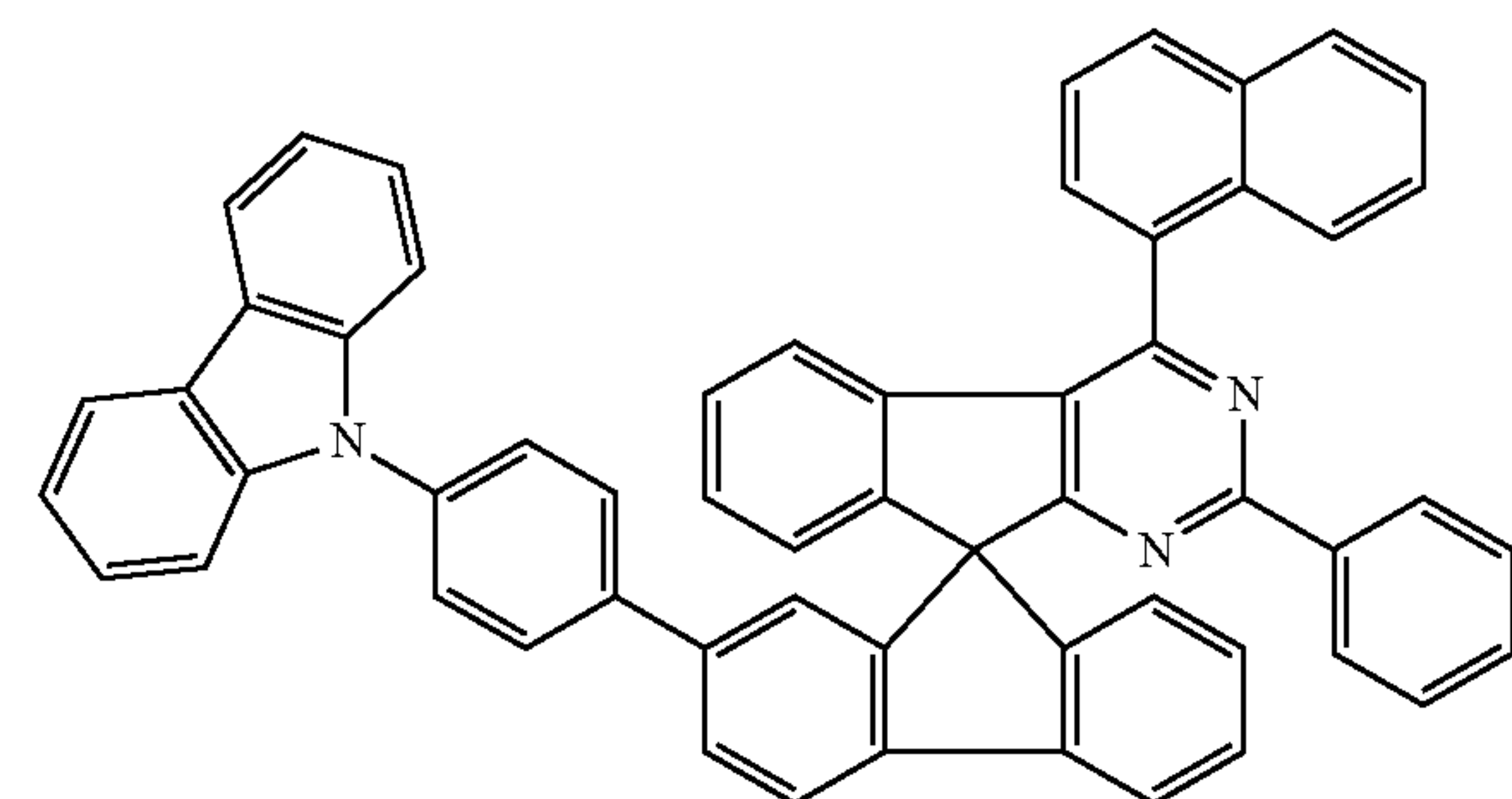
Chemical Formula 1-35
