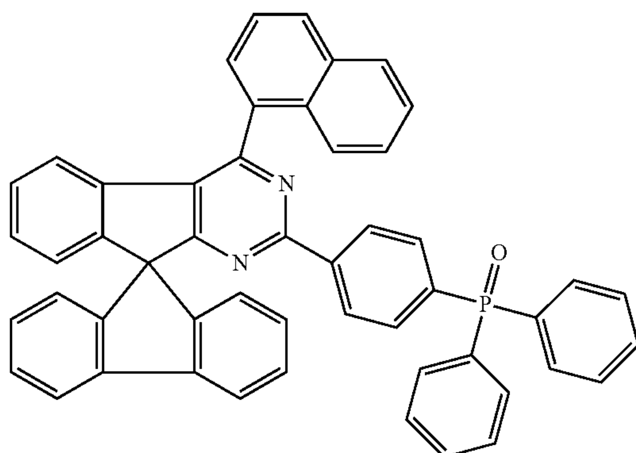
Chemical Formula 1-53
