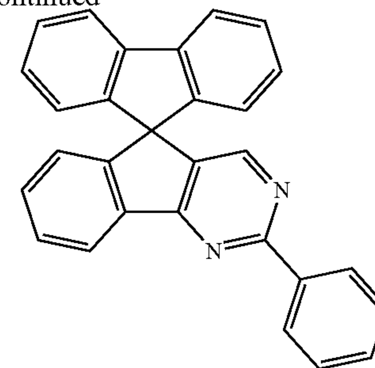
[Chemical Formula 1-9]
