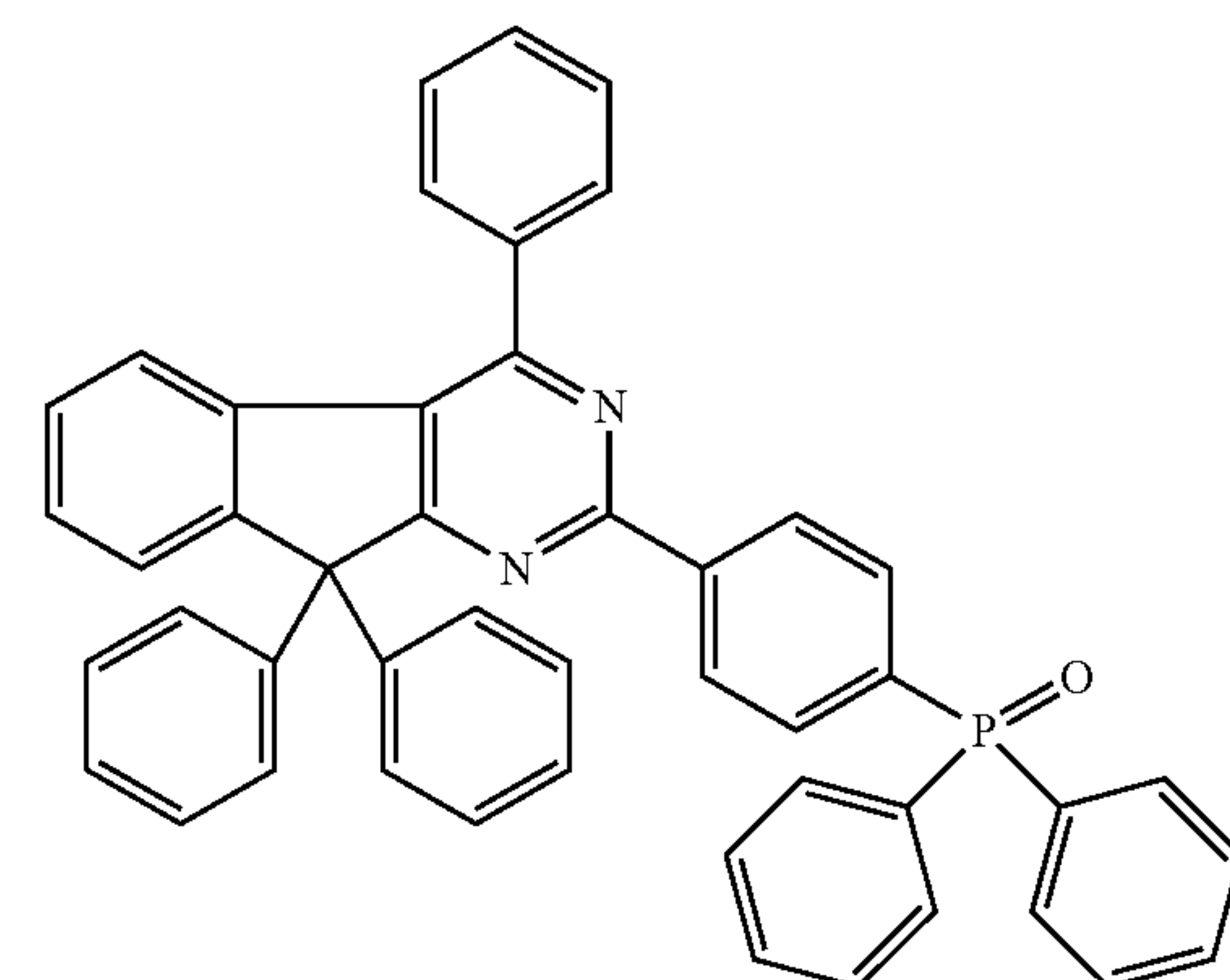
Chemical Formula 2-21
