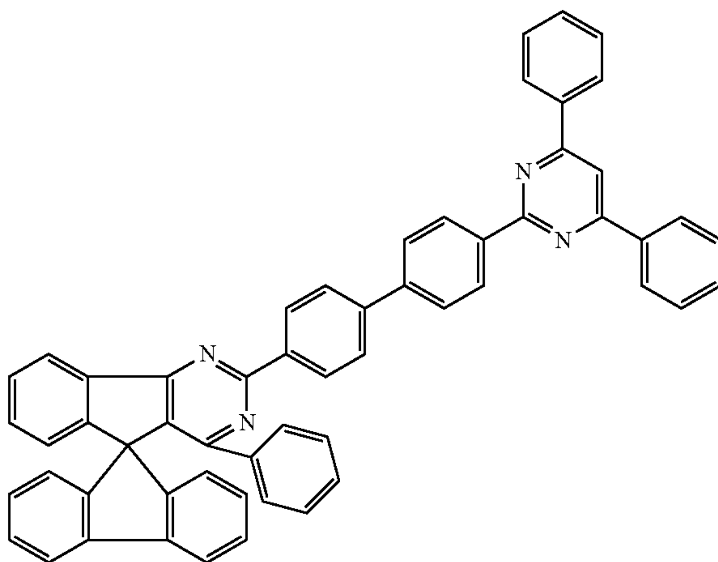
Chemical Formula 1-100
