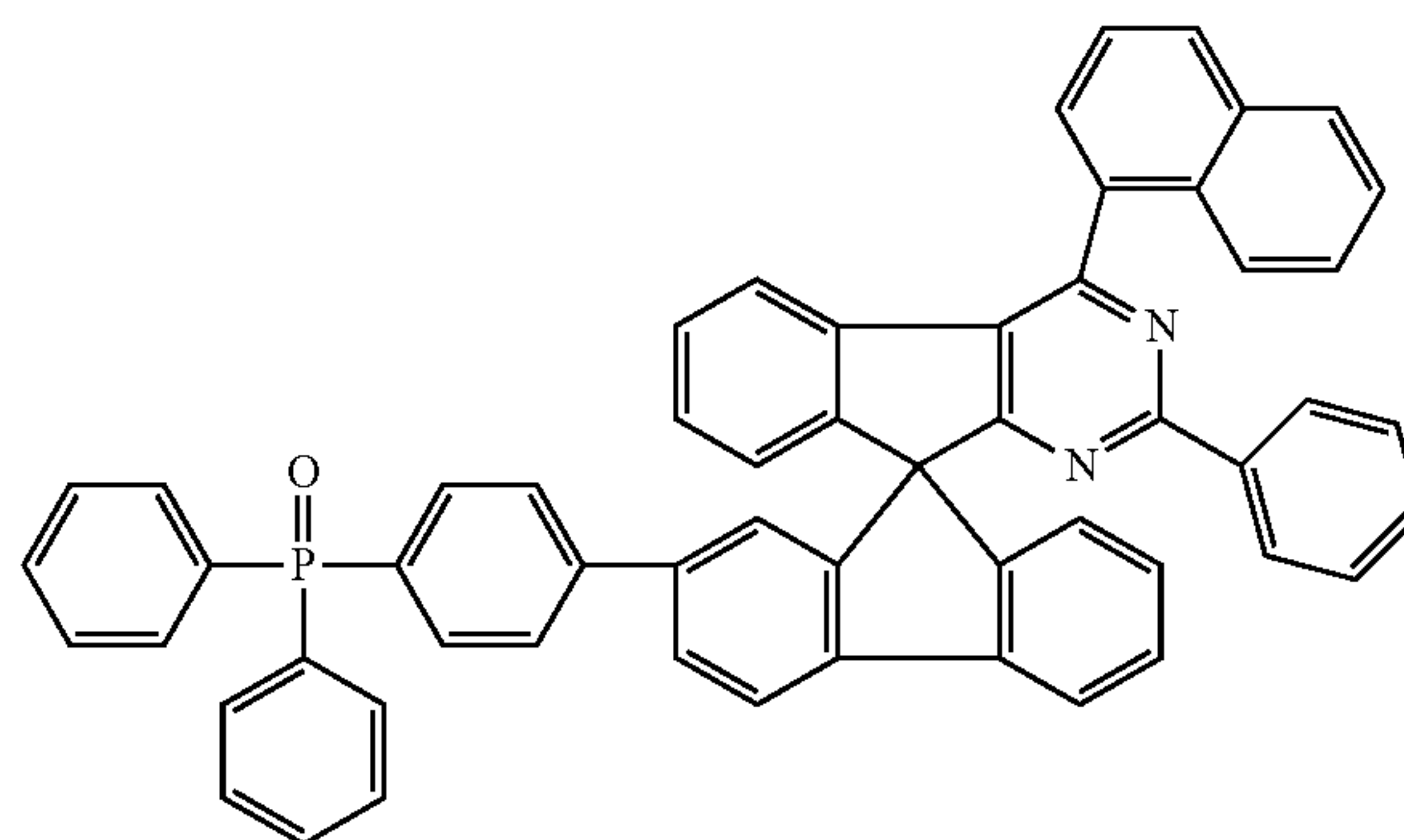
Chemical Formula 1-48
