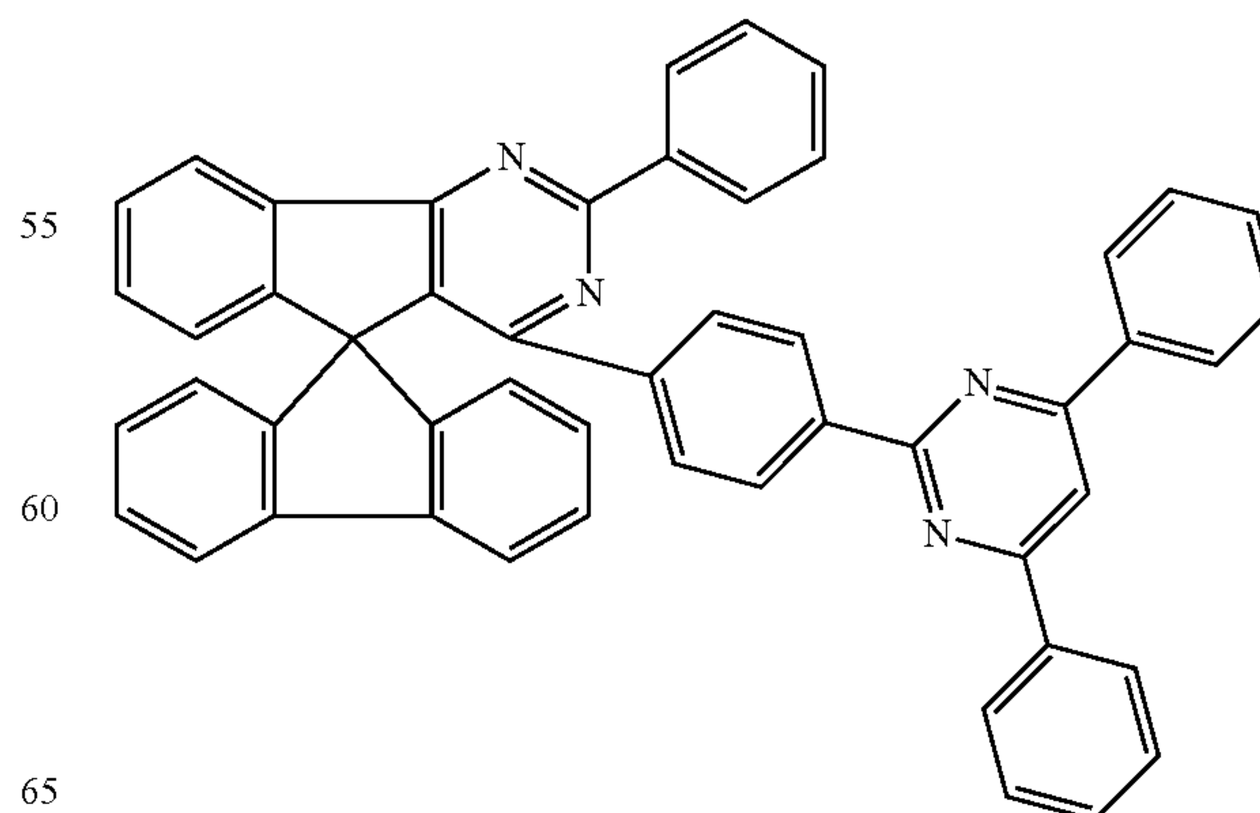
Chemical Formula 1-93
