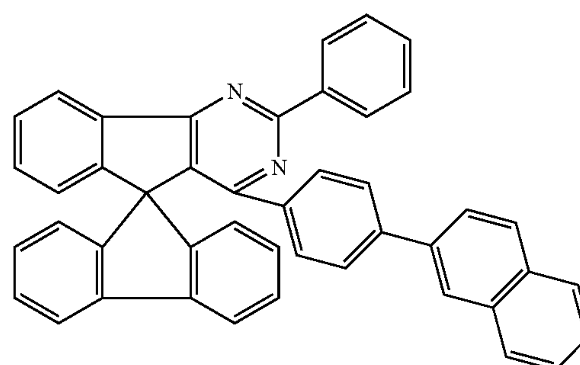
Chemical Formula 1-84
