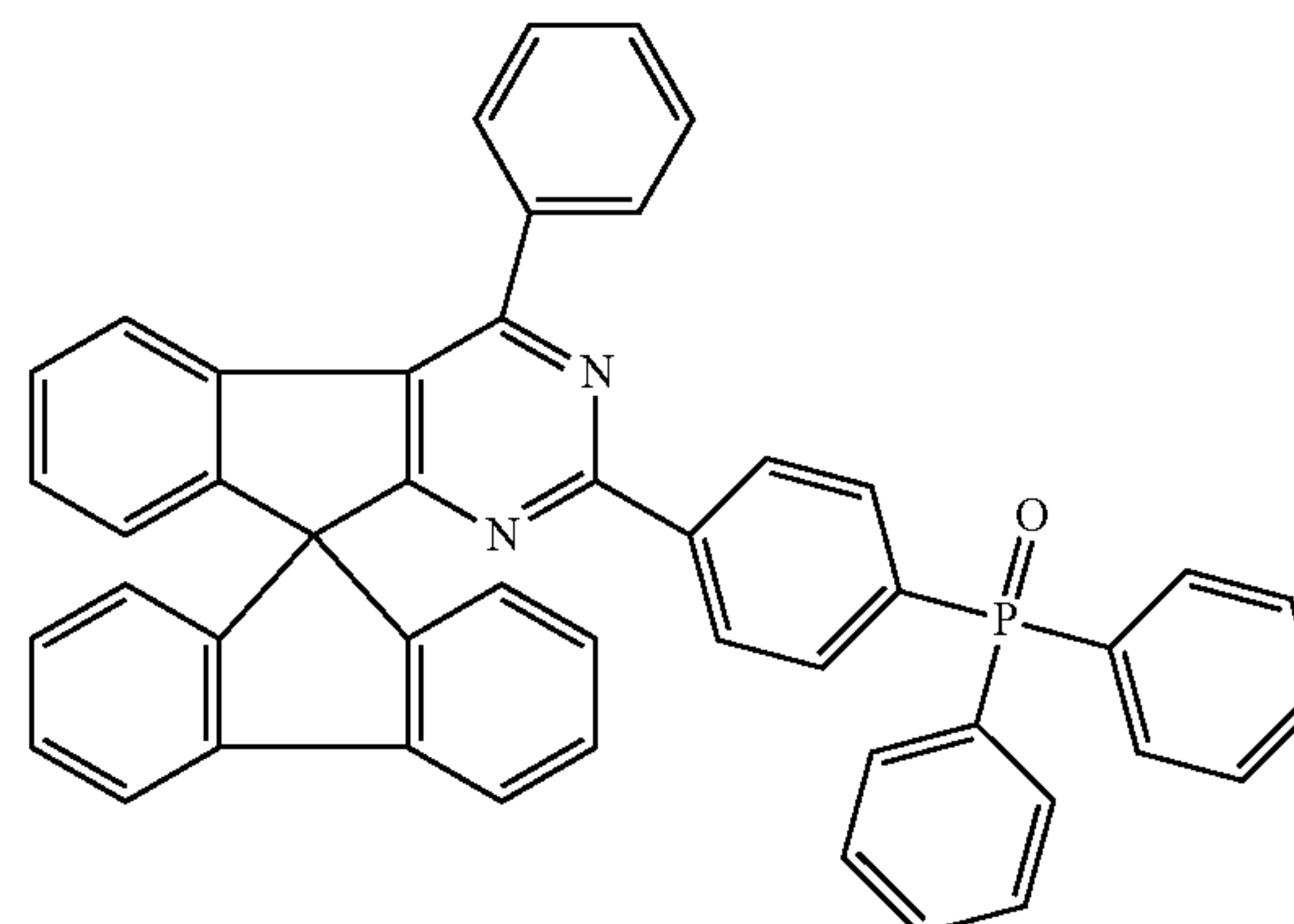
Chemical Formula 1-51
