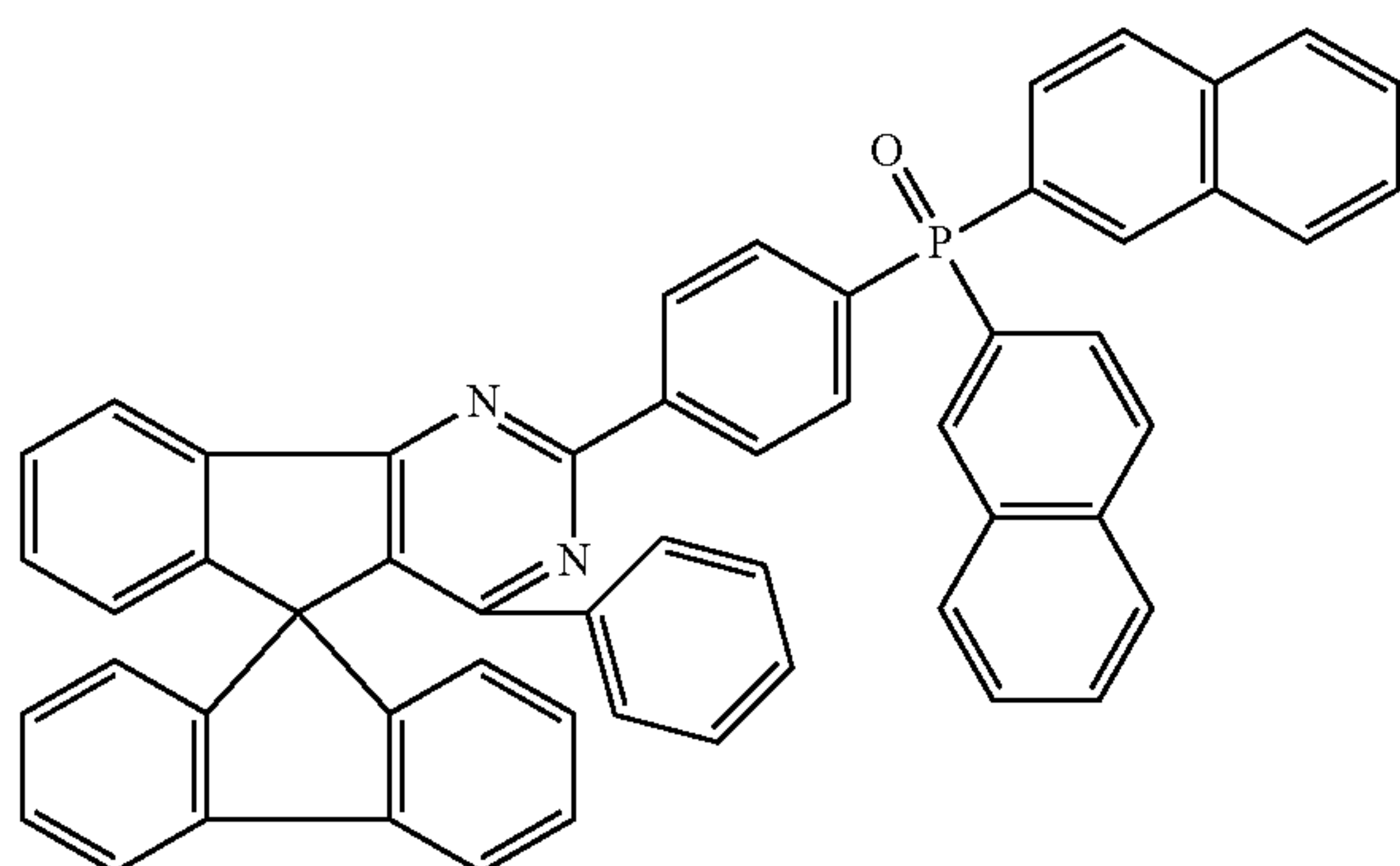
Chemical Formula 1-54
