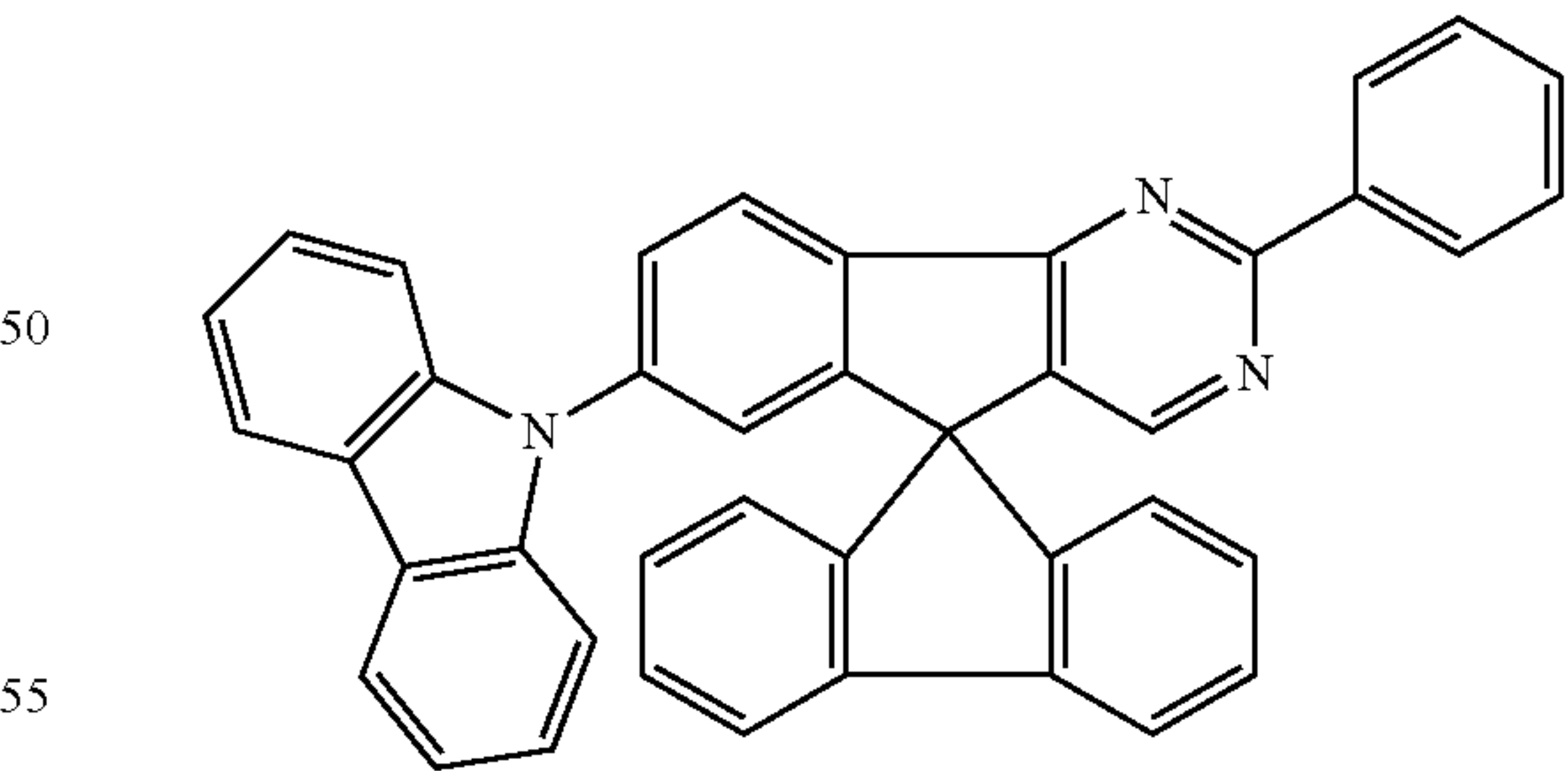
Chemical Formula 1-18
