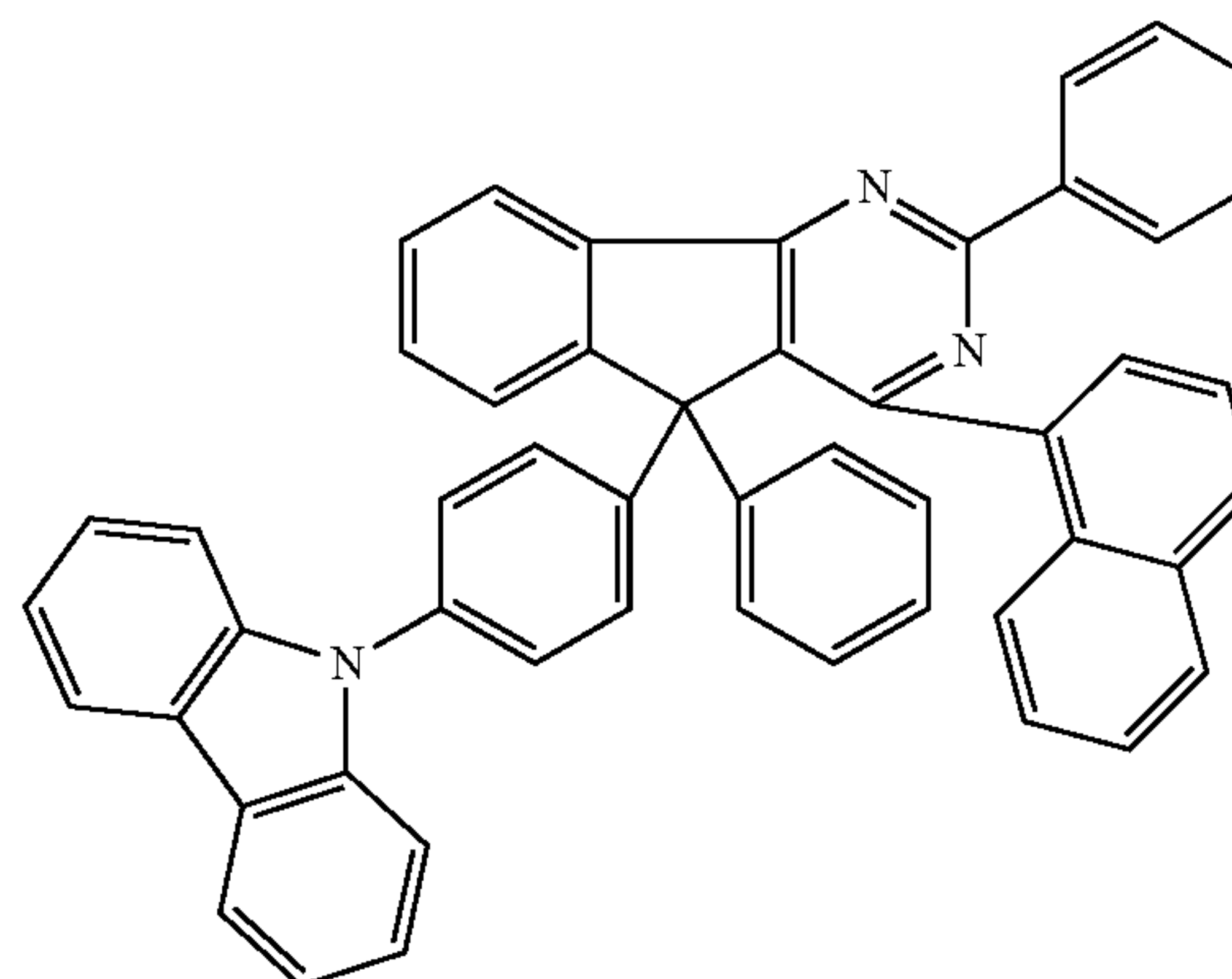
Chemical Formula 2-13
