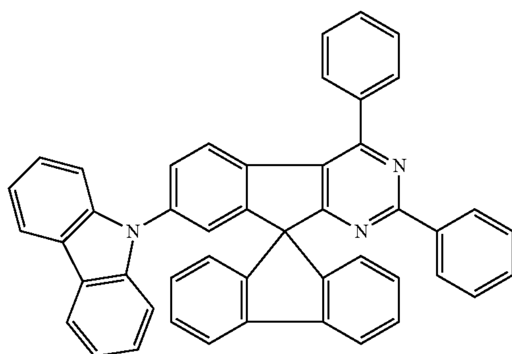
Chemical Formula 1-21
