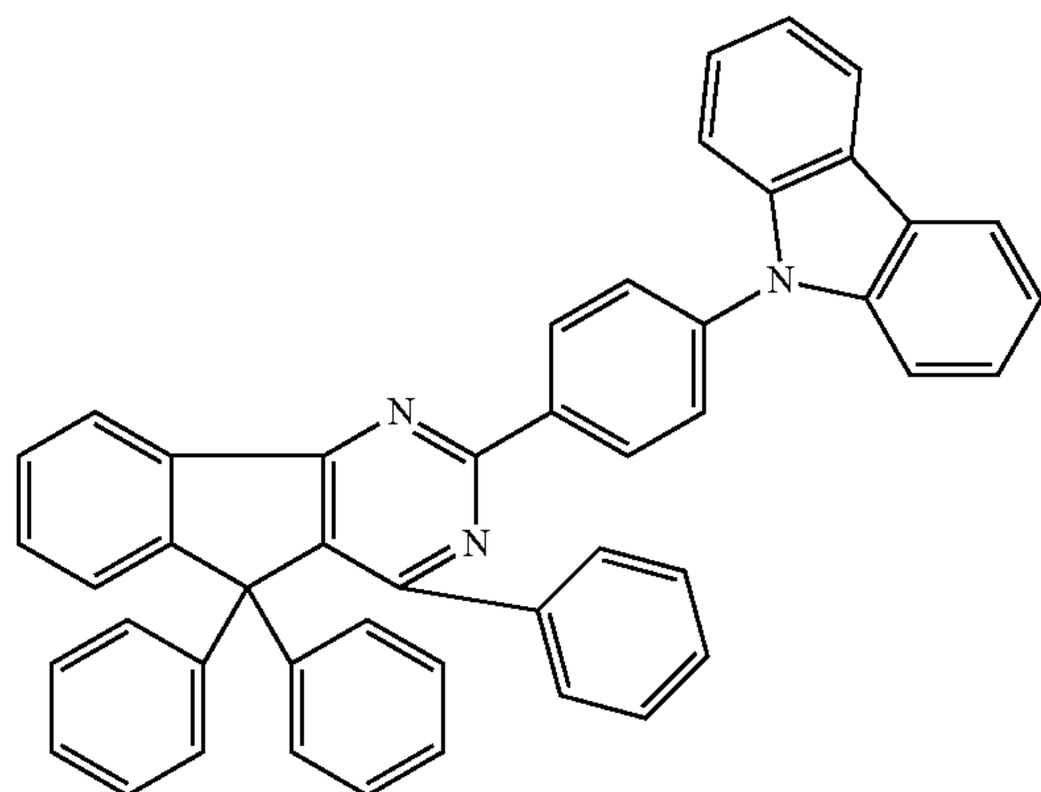
Chemical Formula 2-29
