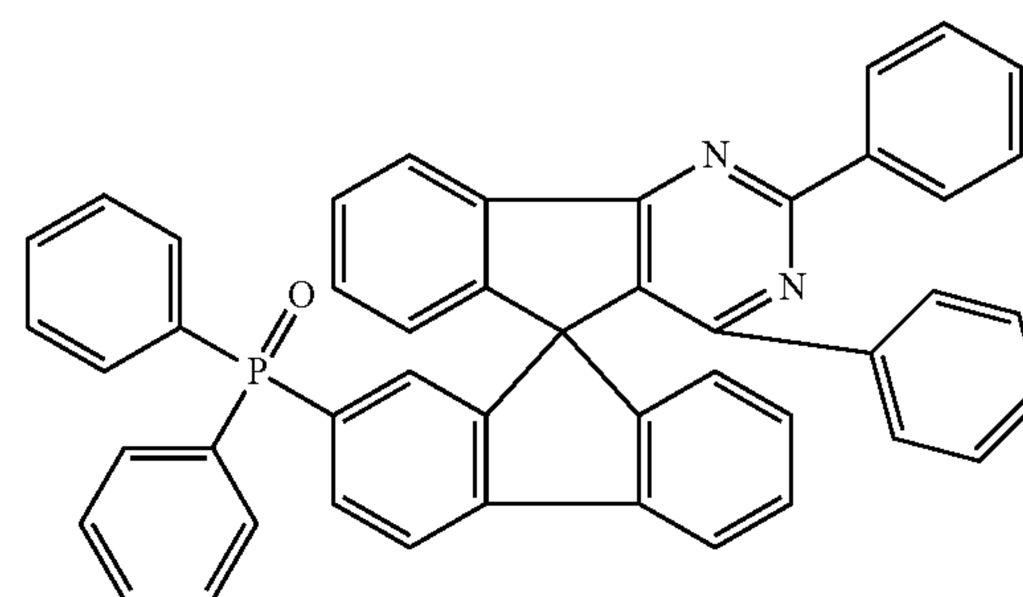
Chemical Formula 1-41
