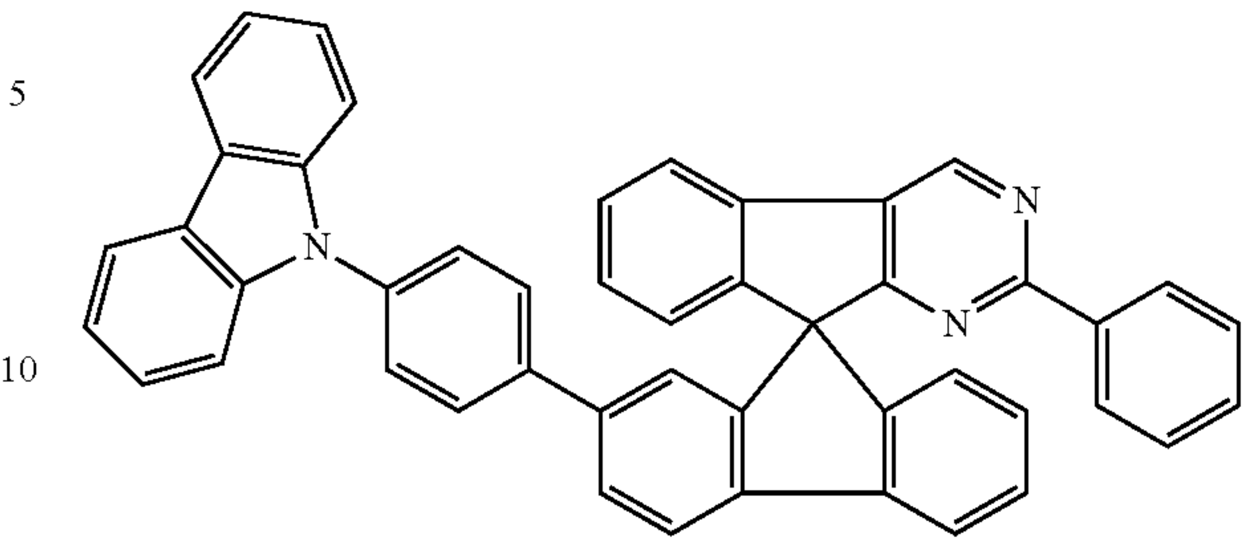
Chemical Formula 1-14
