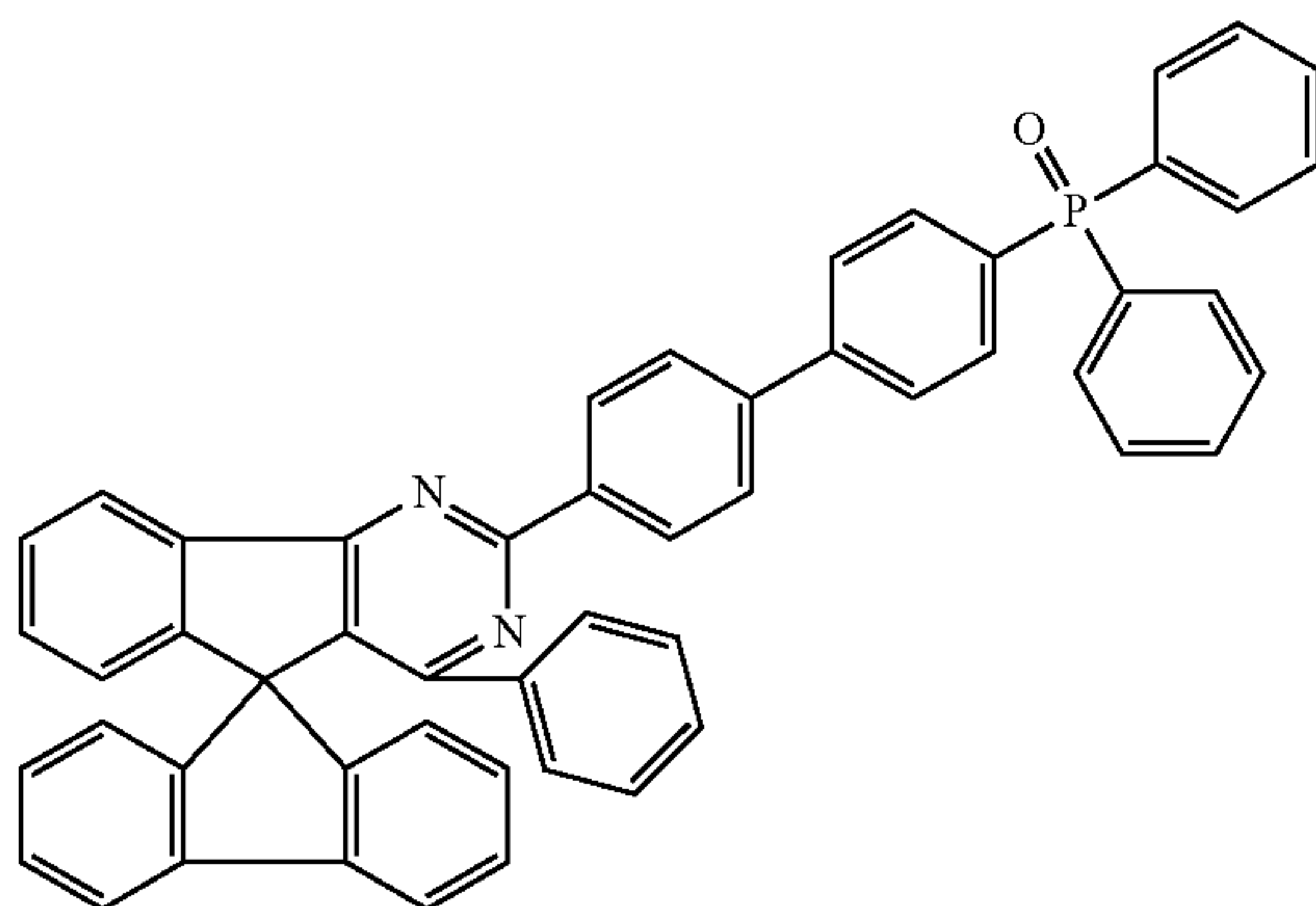
Chemical Formula 1-55
