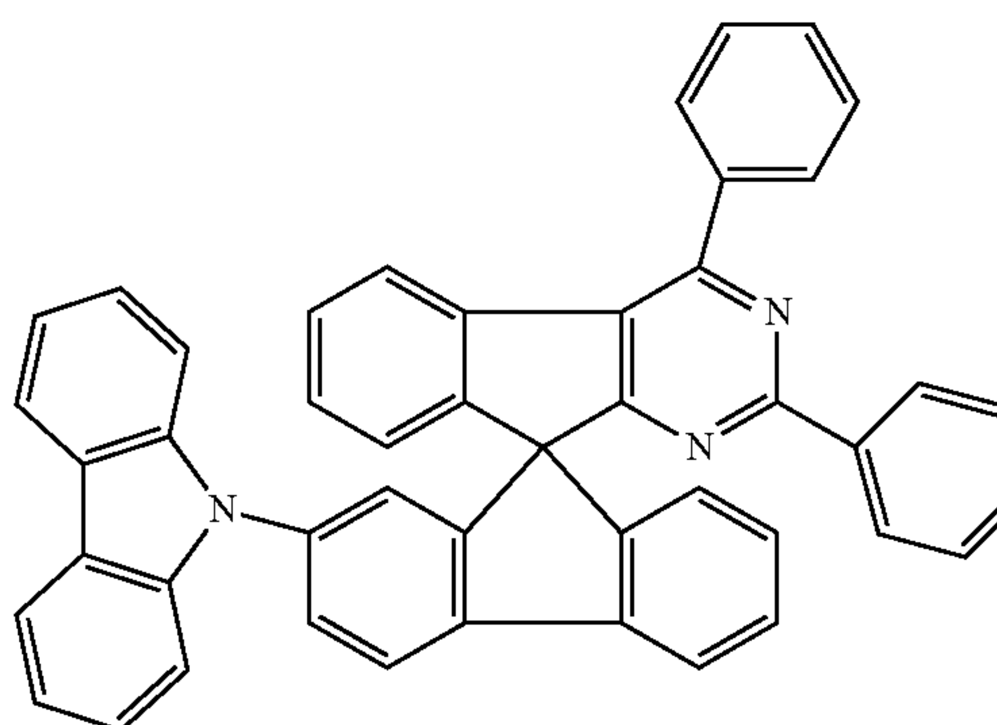
Chemical Formula 1-5
