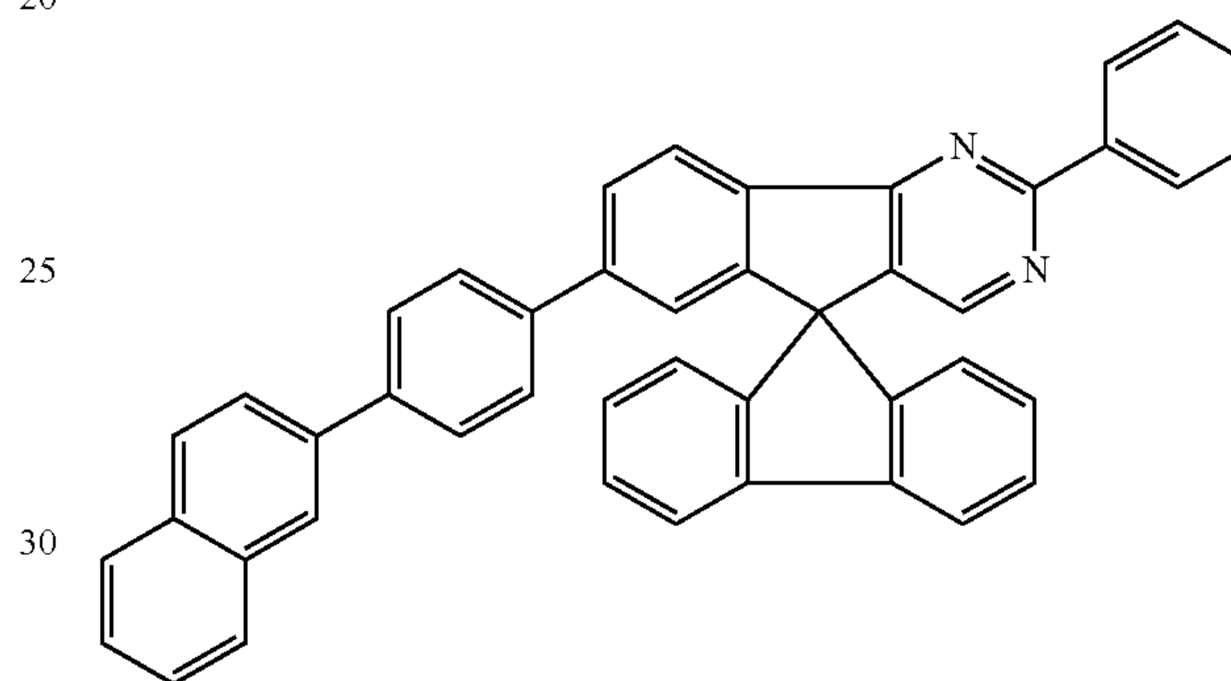
Chemical Formula 1-25
