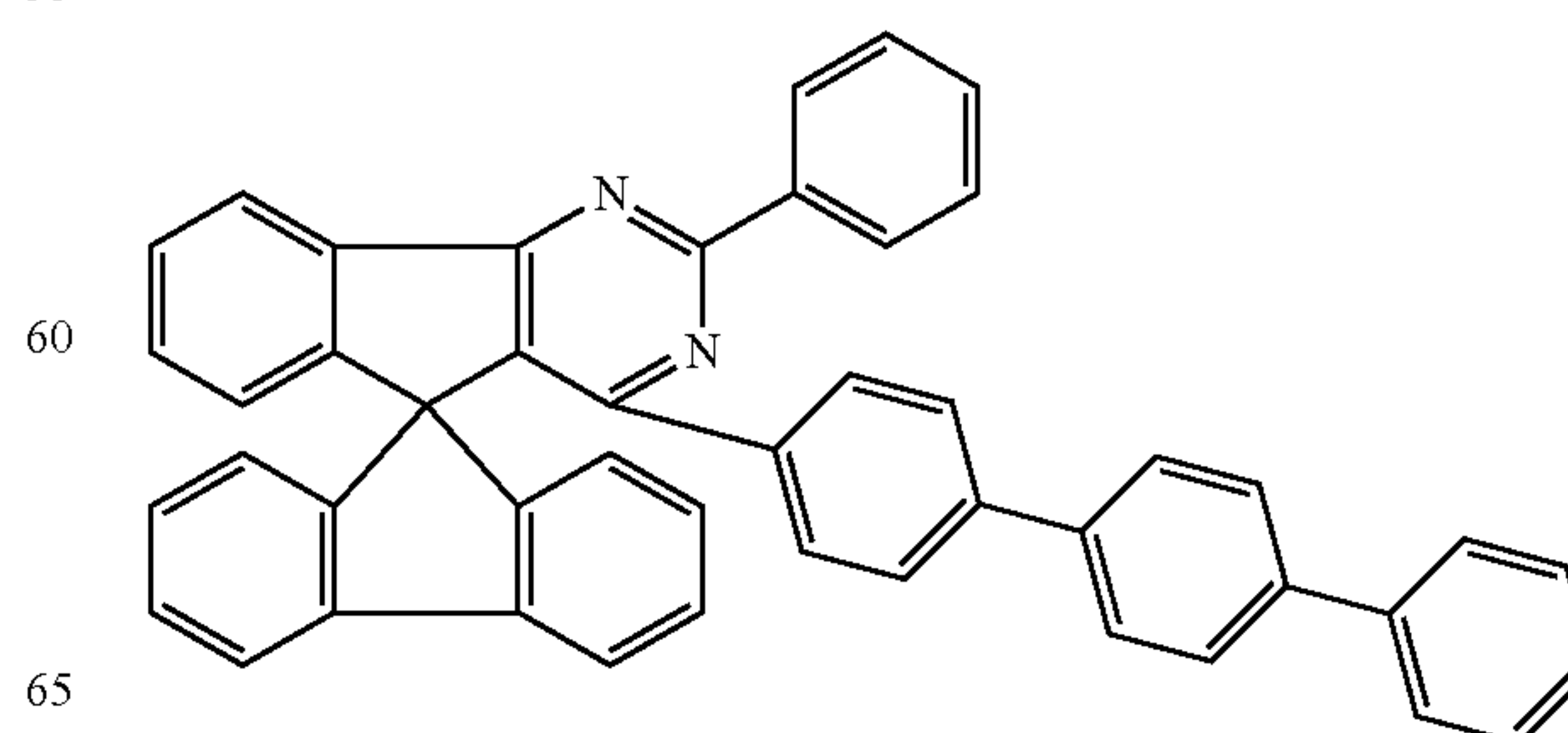
Chemical Formula 1-81
