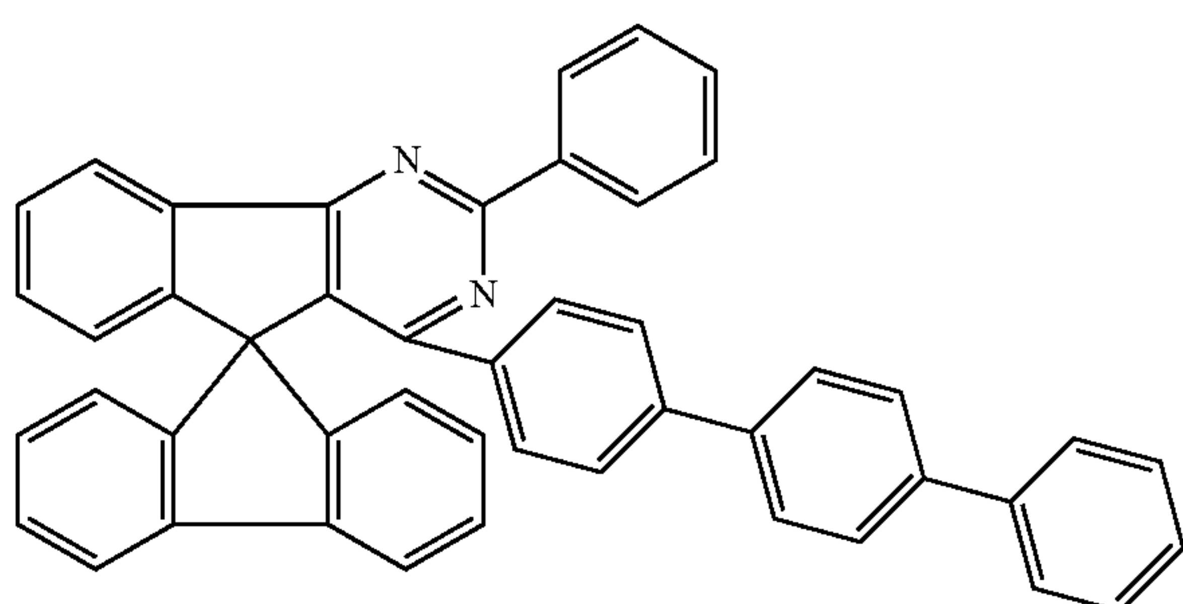
Chemical Formula 1-81
