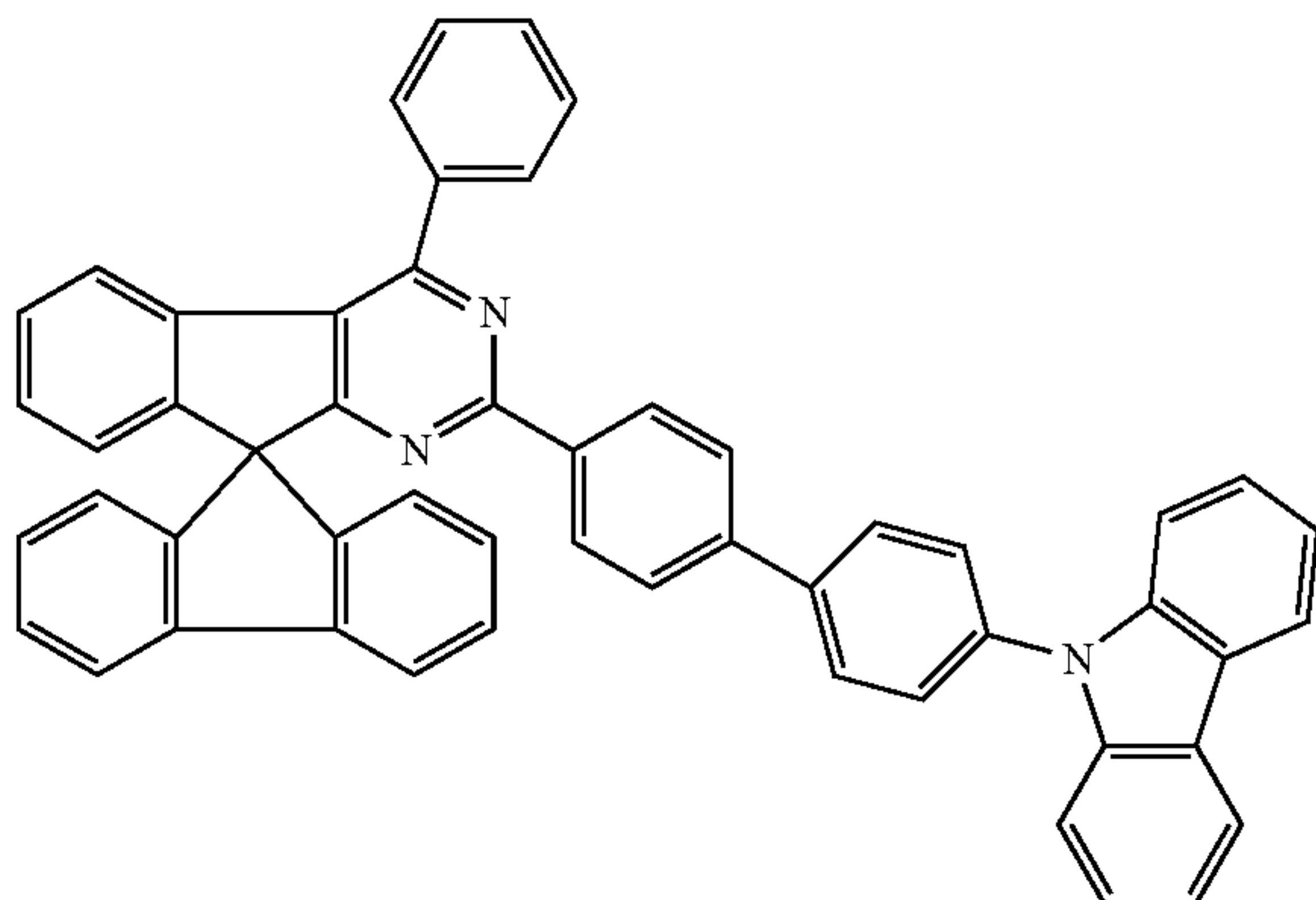
Chemical Formula 1-71
