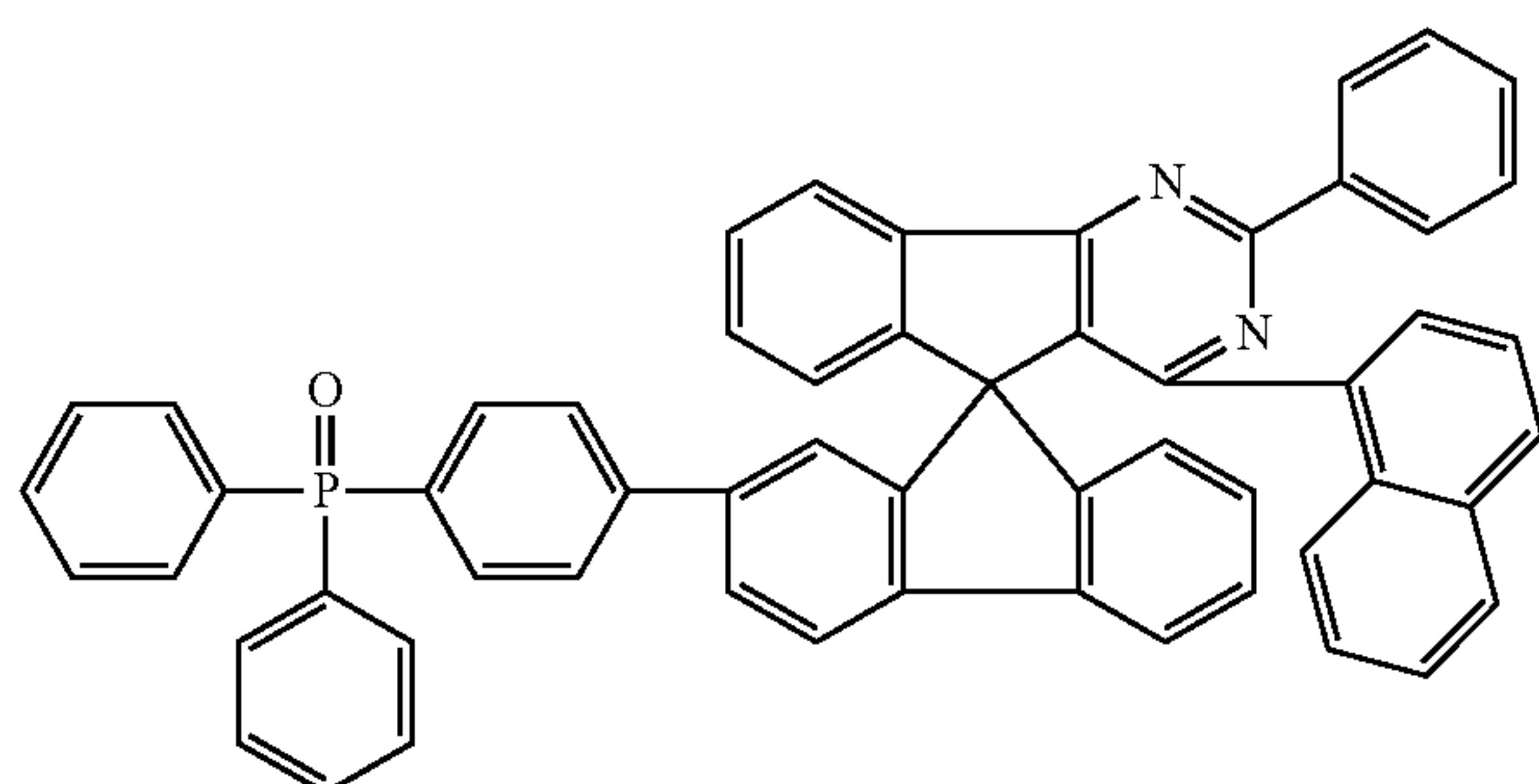
Chemical Formula 1-47
