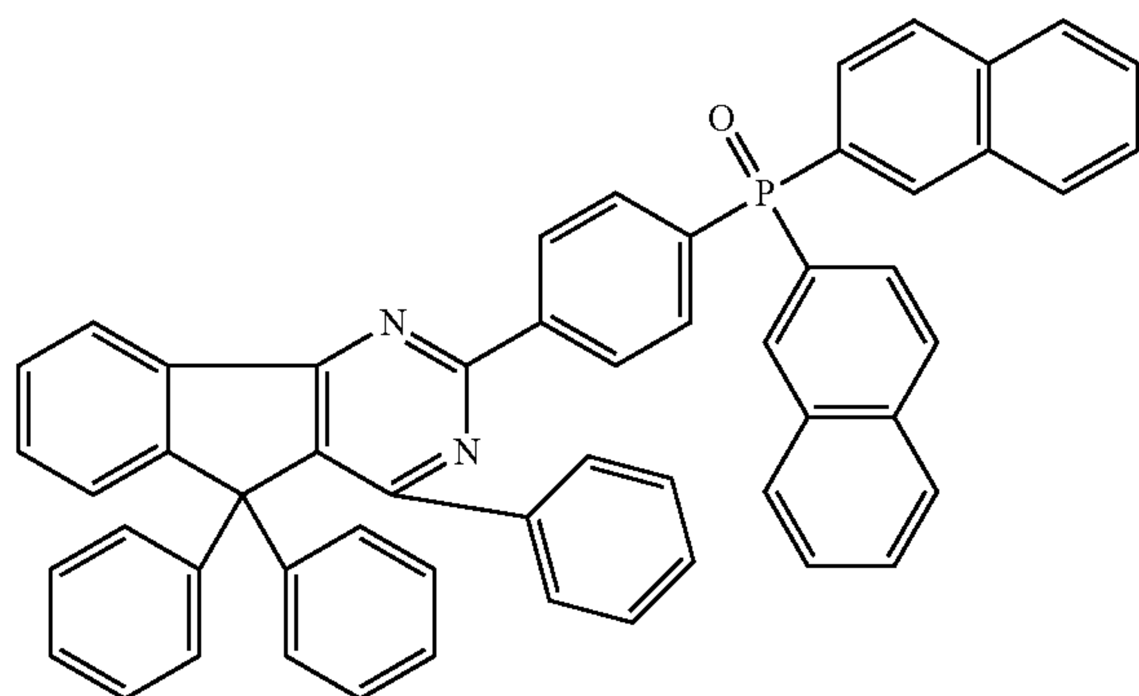
Chemical Formula 2-23
