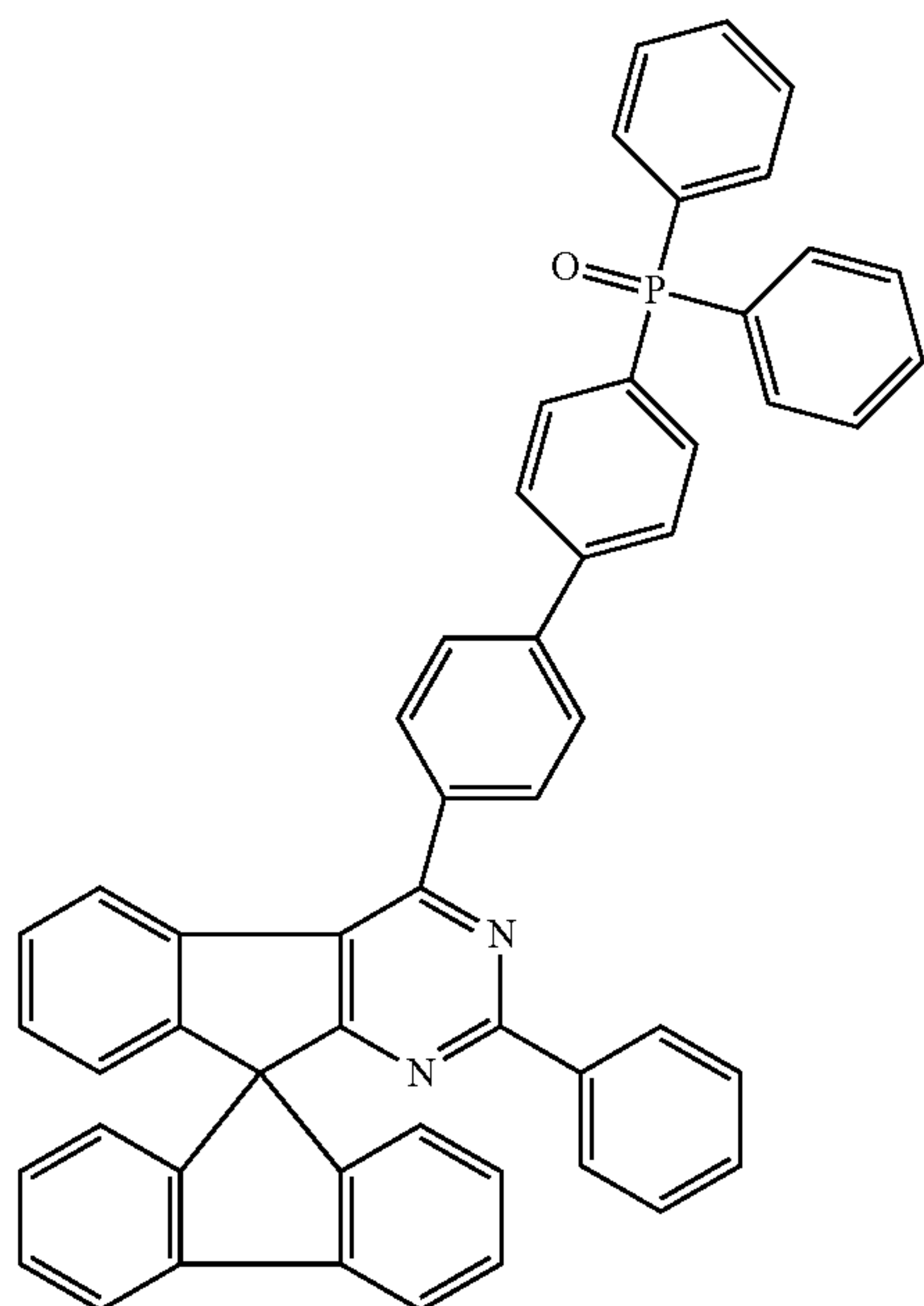
Chemical Formula 1-80
