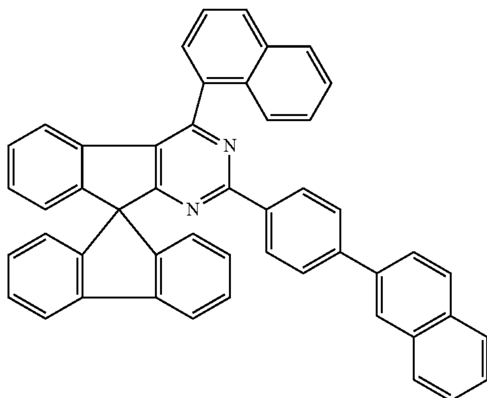
Chemical Formula 1-66
