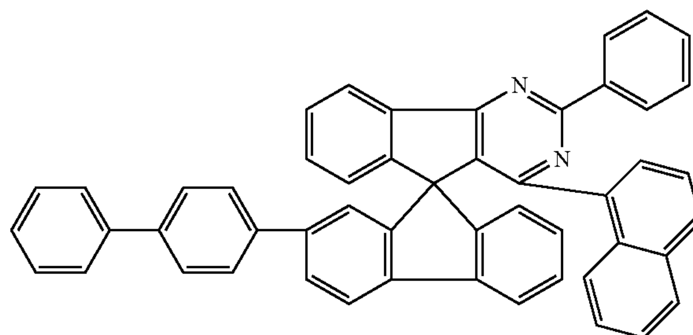
Chemical Formula 1-32
