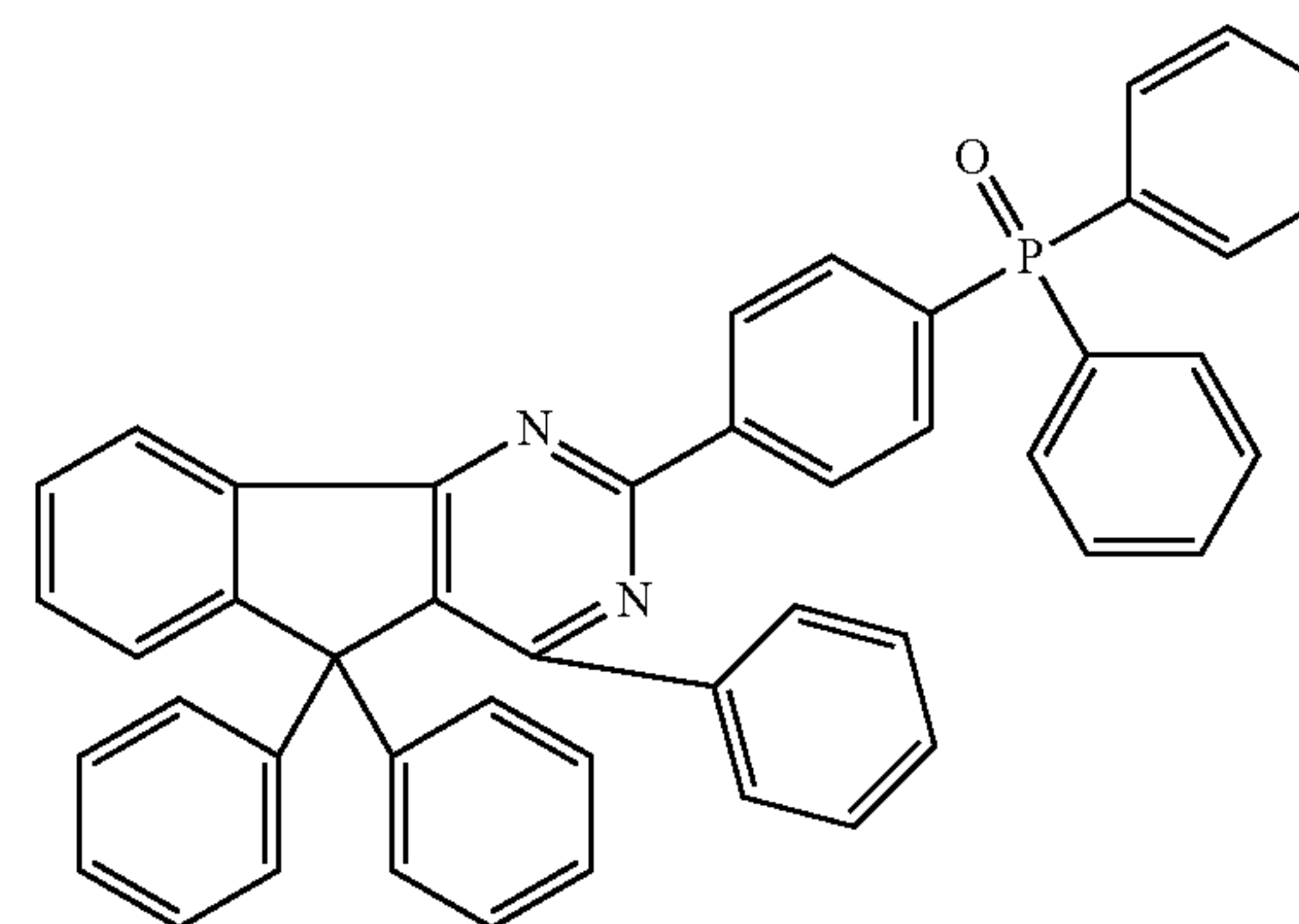
Chemical Formula 2-20
