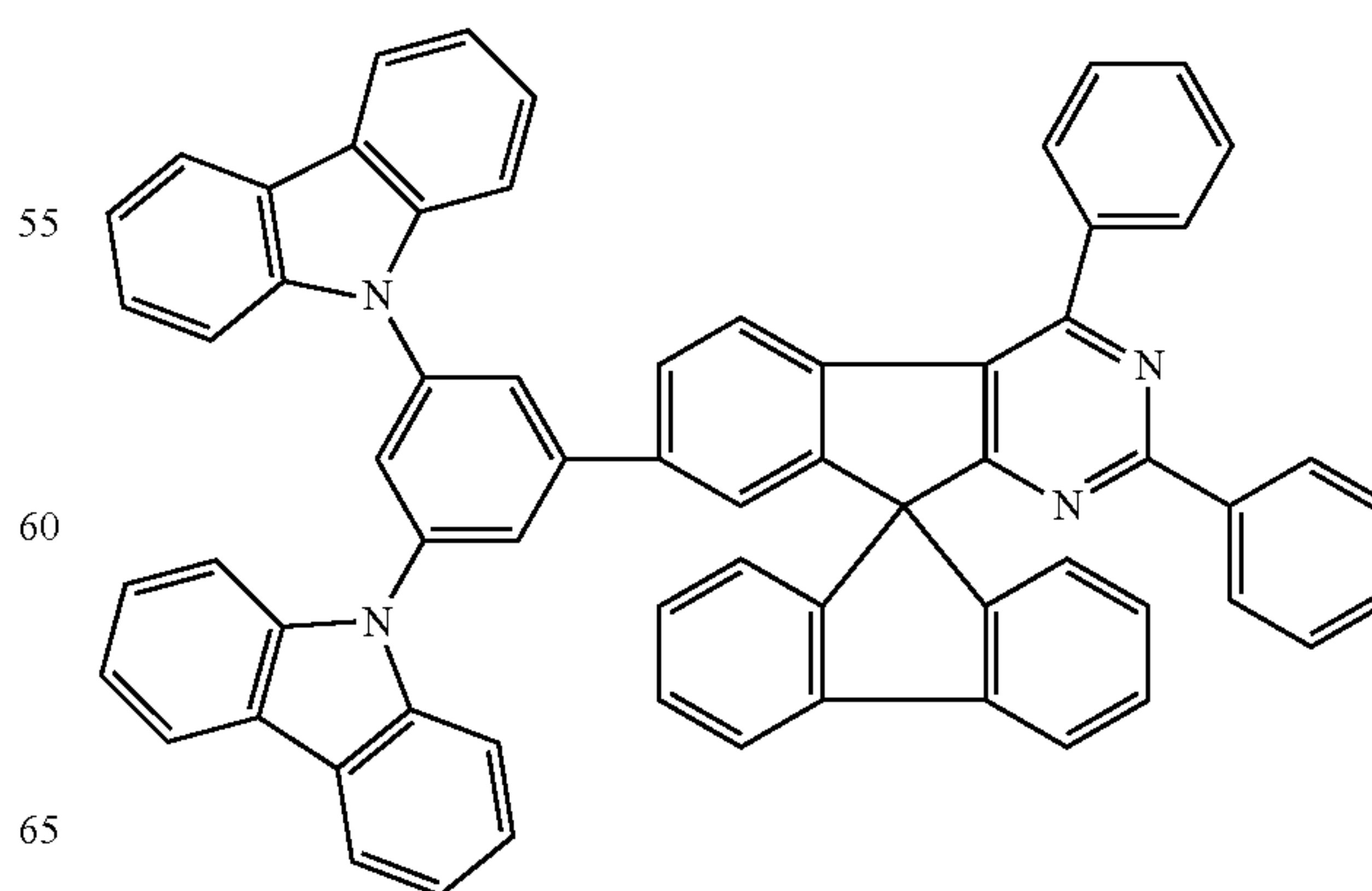
Chemical Formula 1-72
