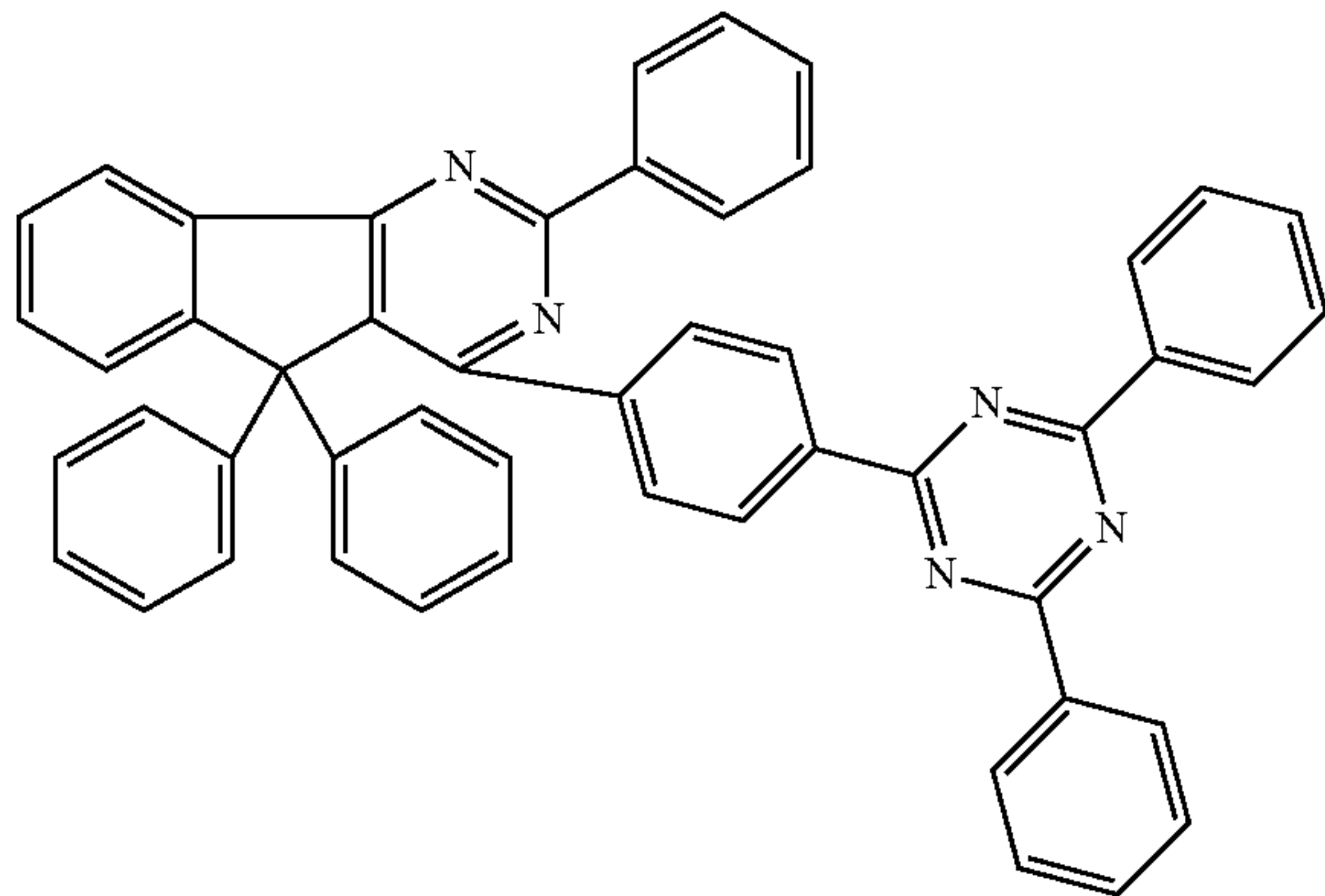
Chemical Formula 2-43
