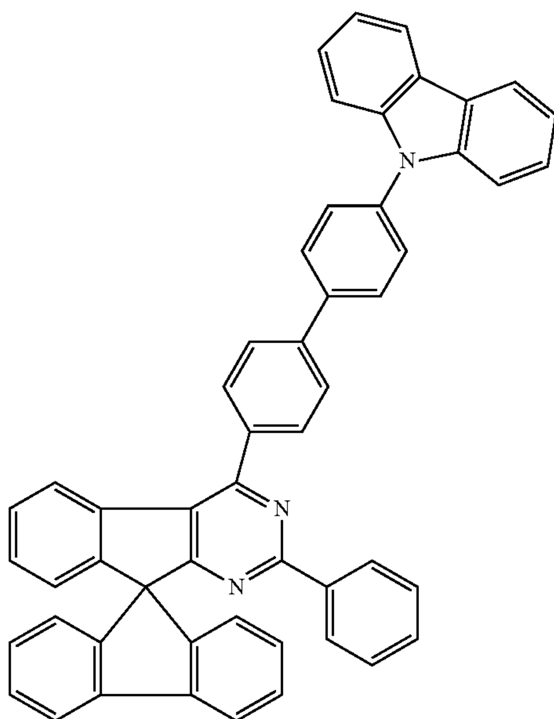
Chemical Formula 1-88
