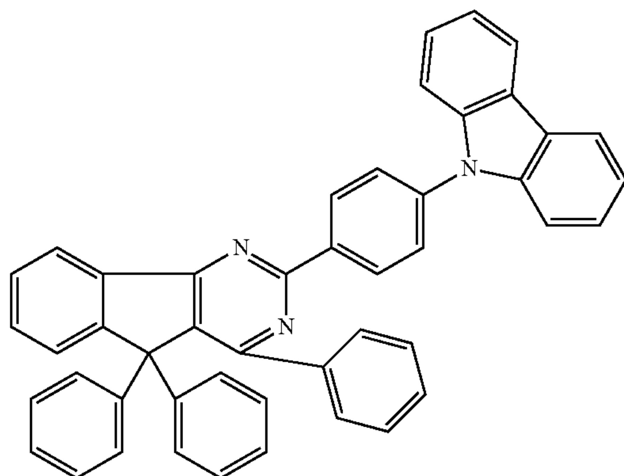
Chemical Formula 2-29
