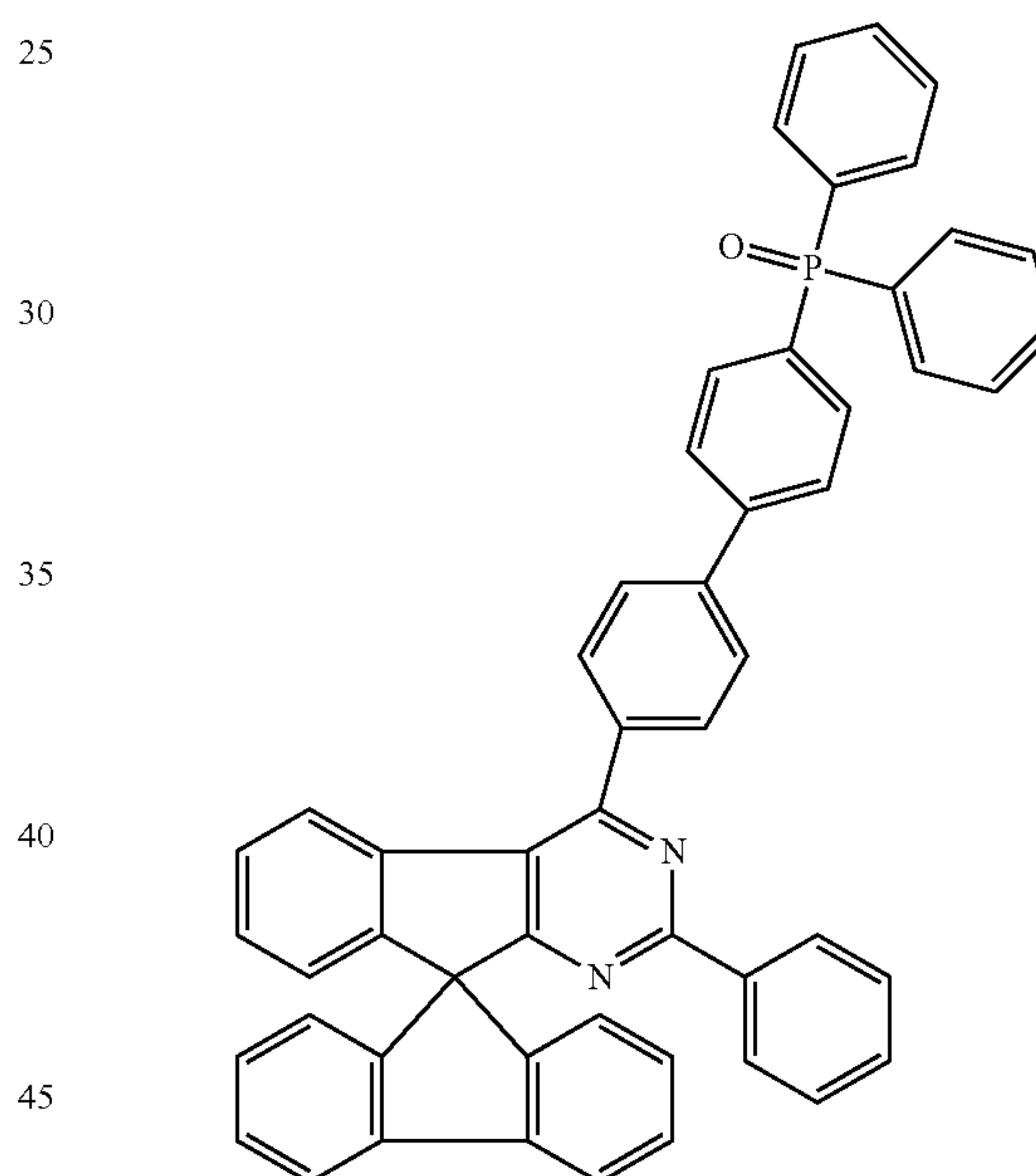
Chemical Formula 1-80
