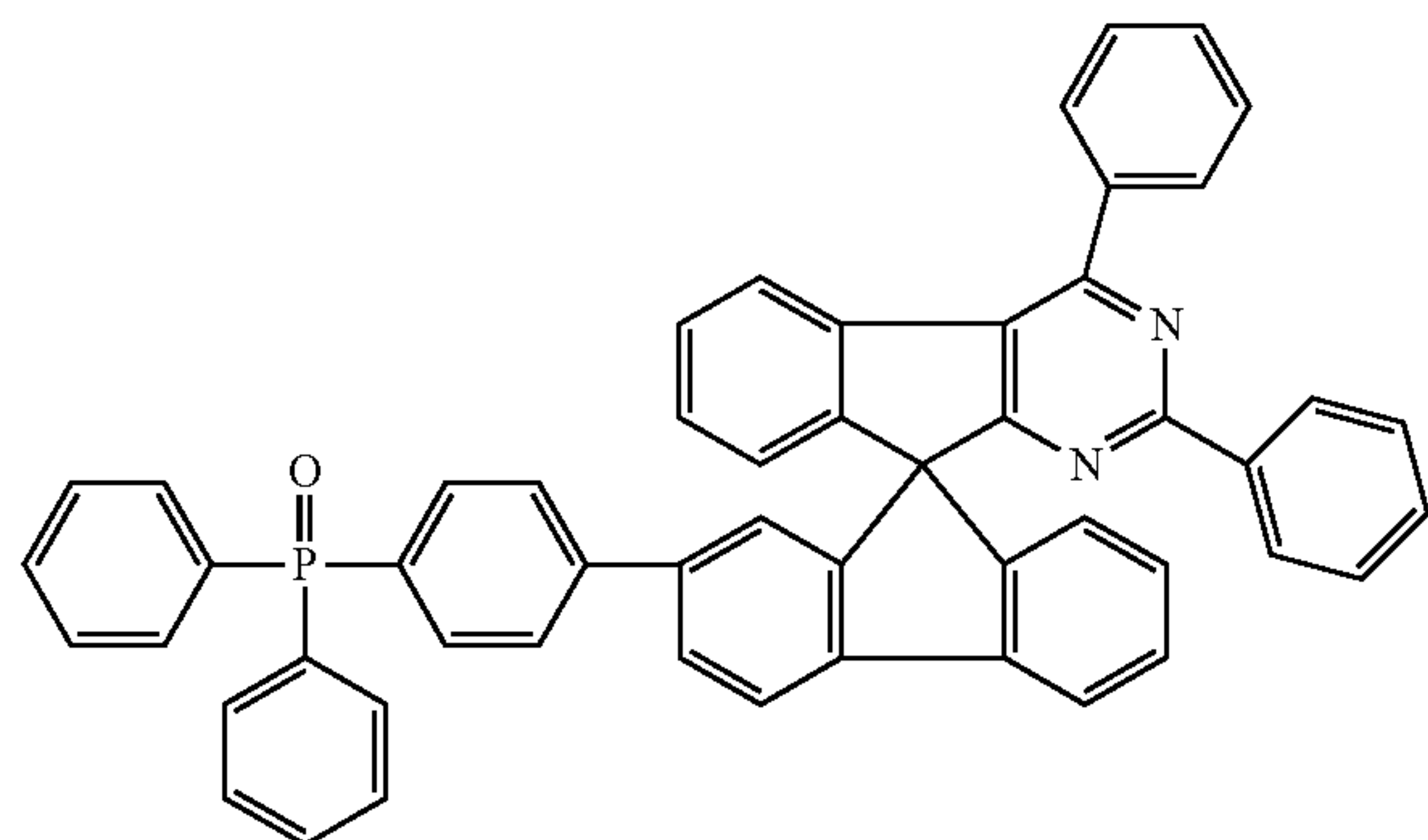
Chemical Formula 1-46
