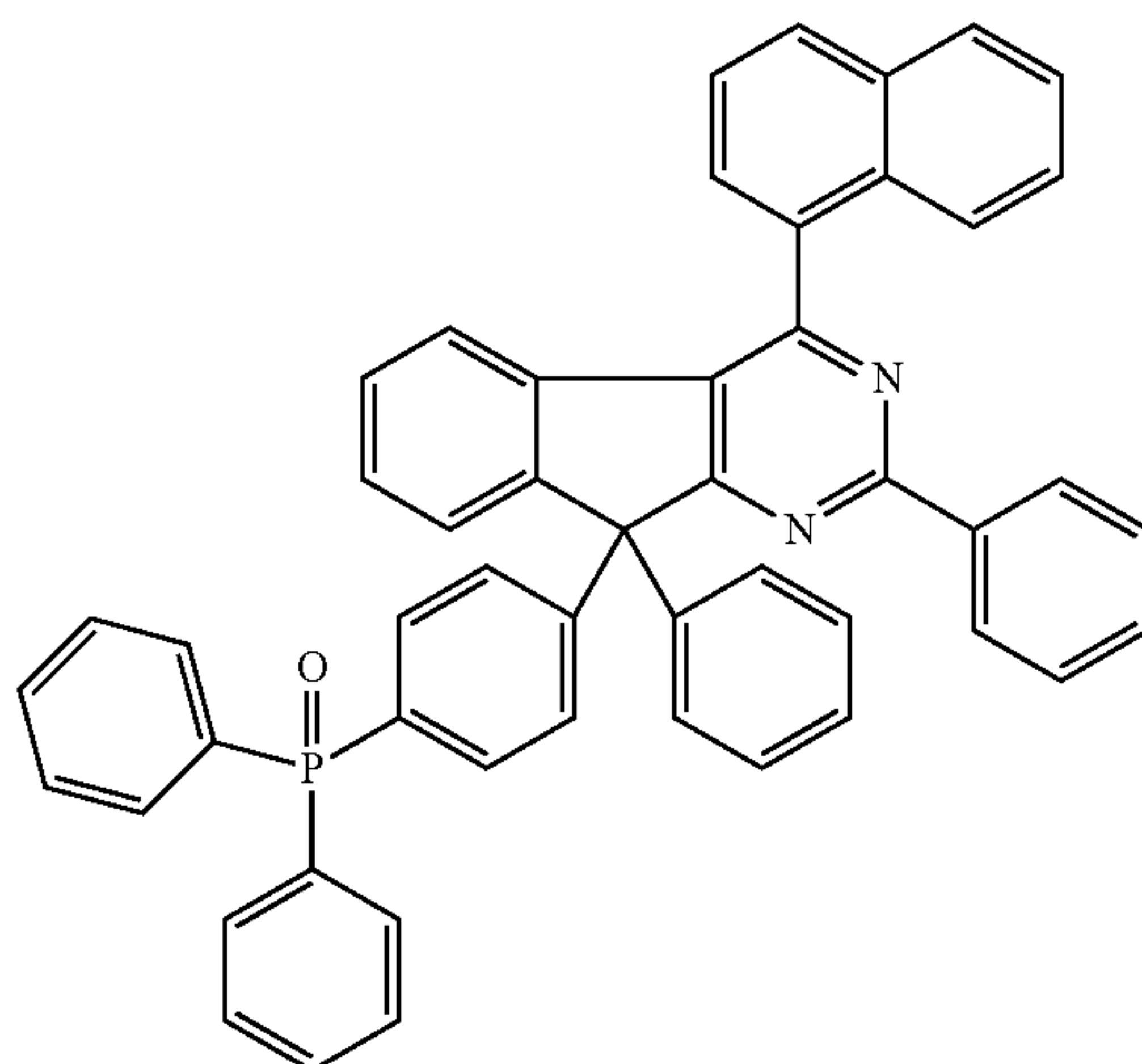
Chemical Formula 2-18
