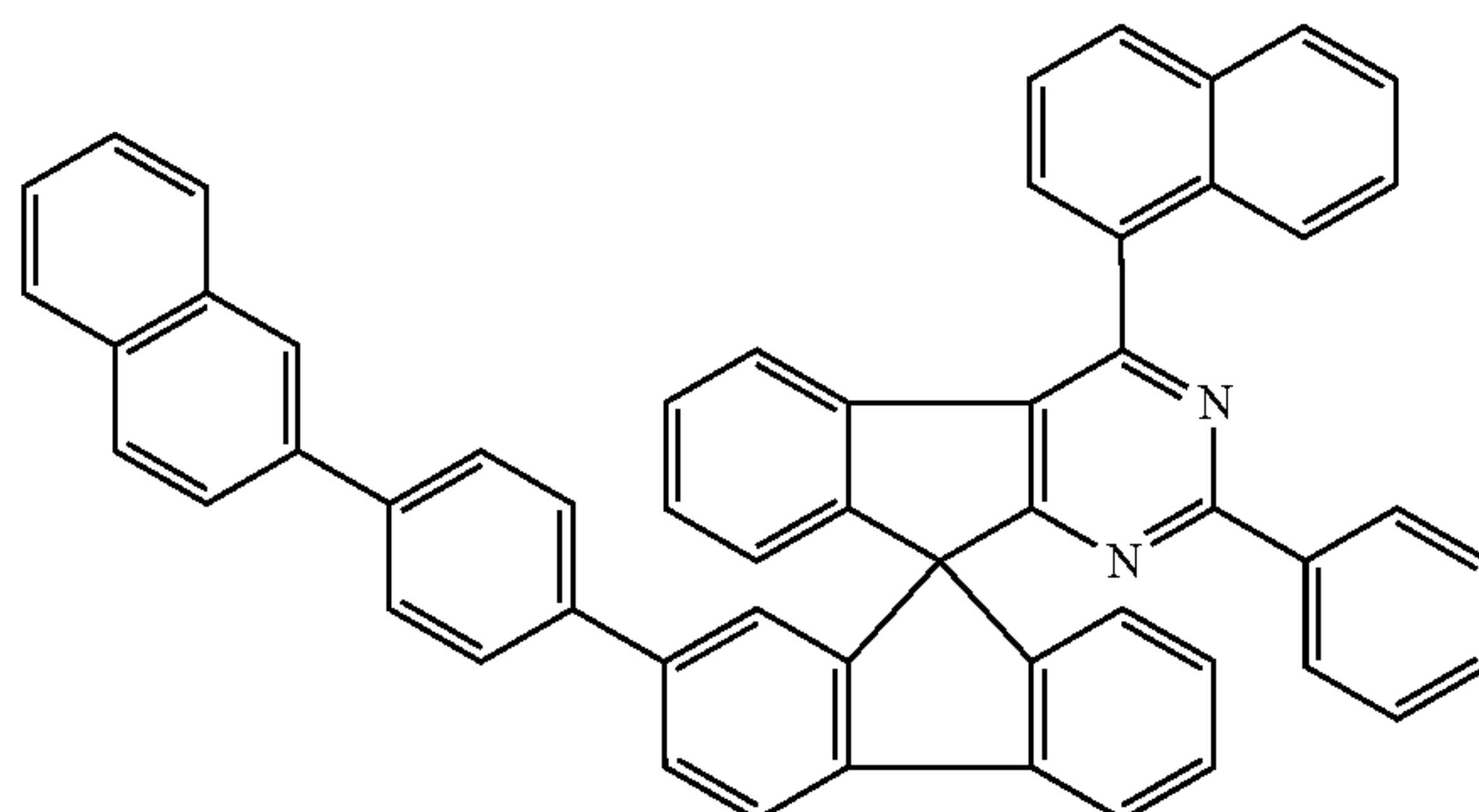
Chemical Formula 1-38
