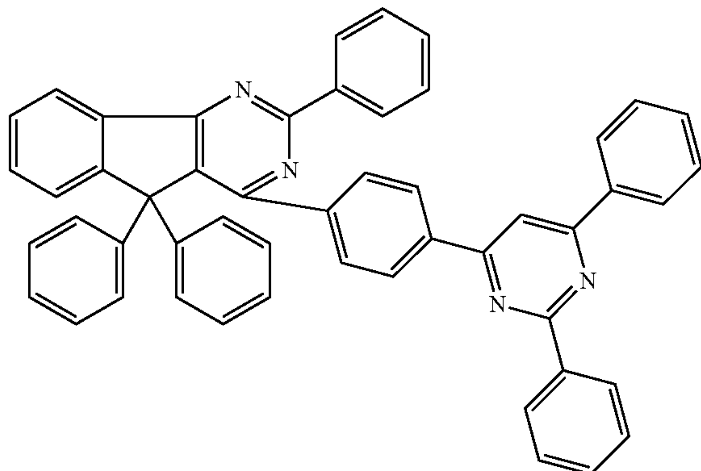
Chemical Formula 2-45
