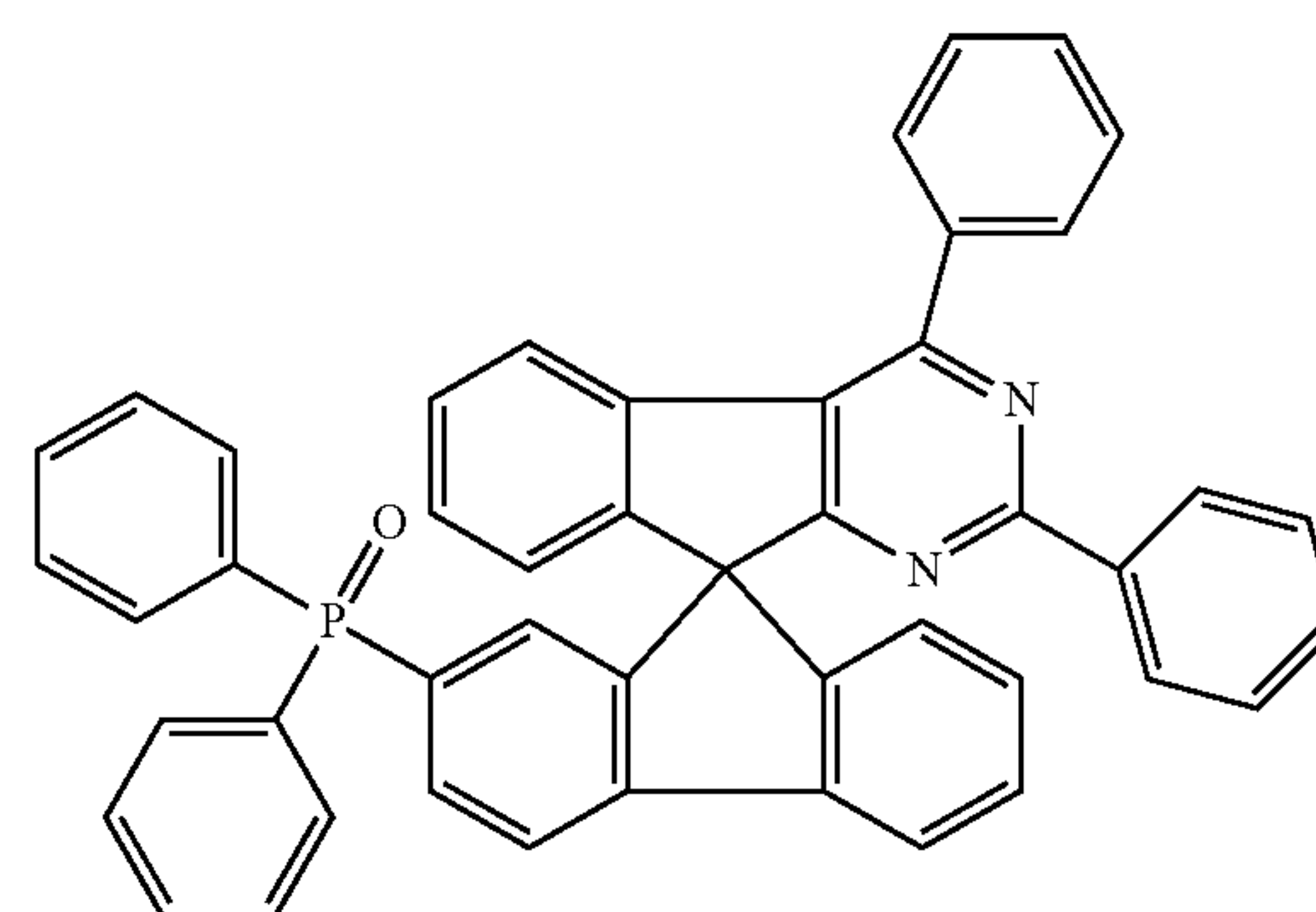
Chemical Formula 1-43
