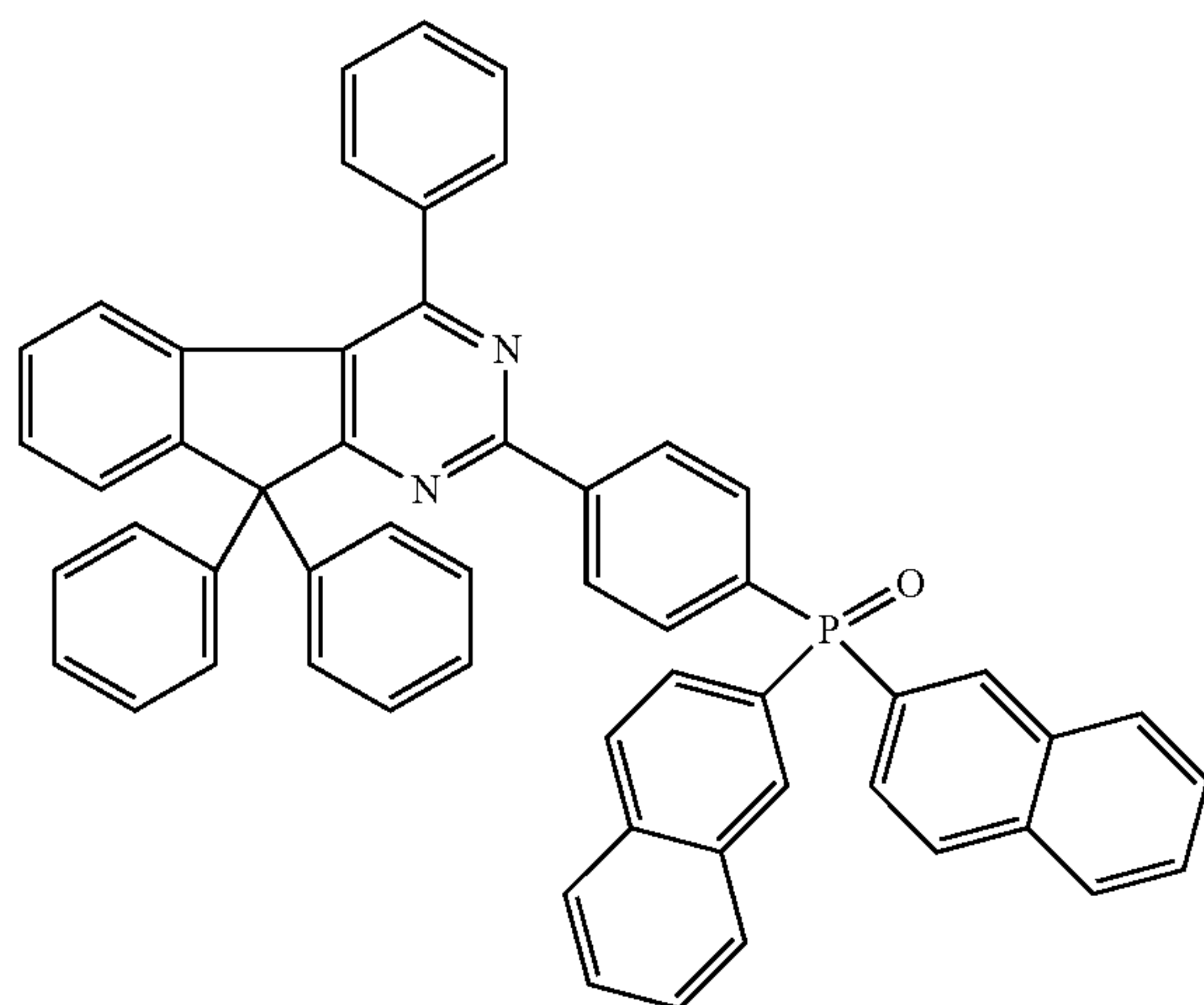
Chemical Formula 2-24
