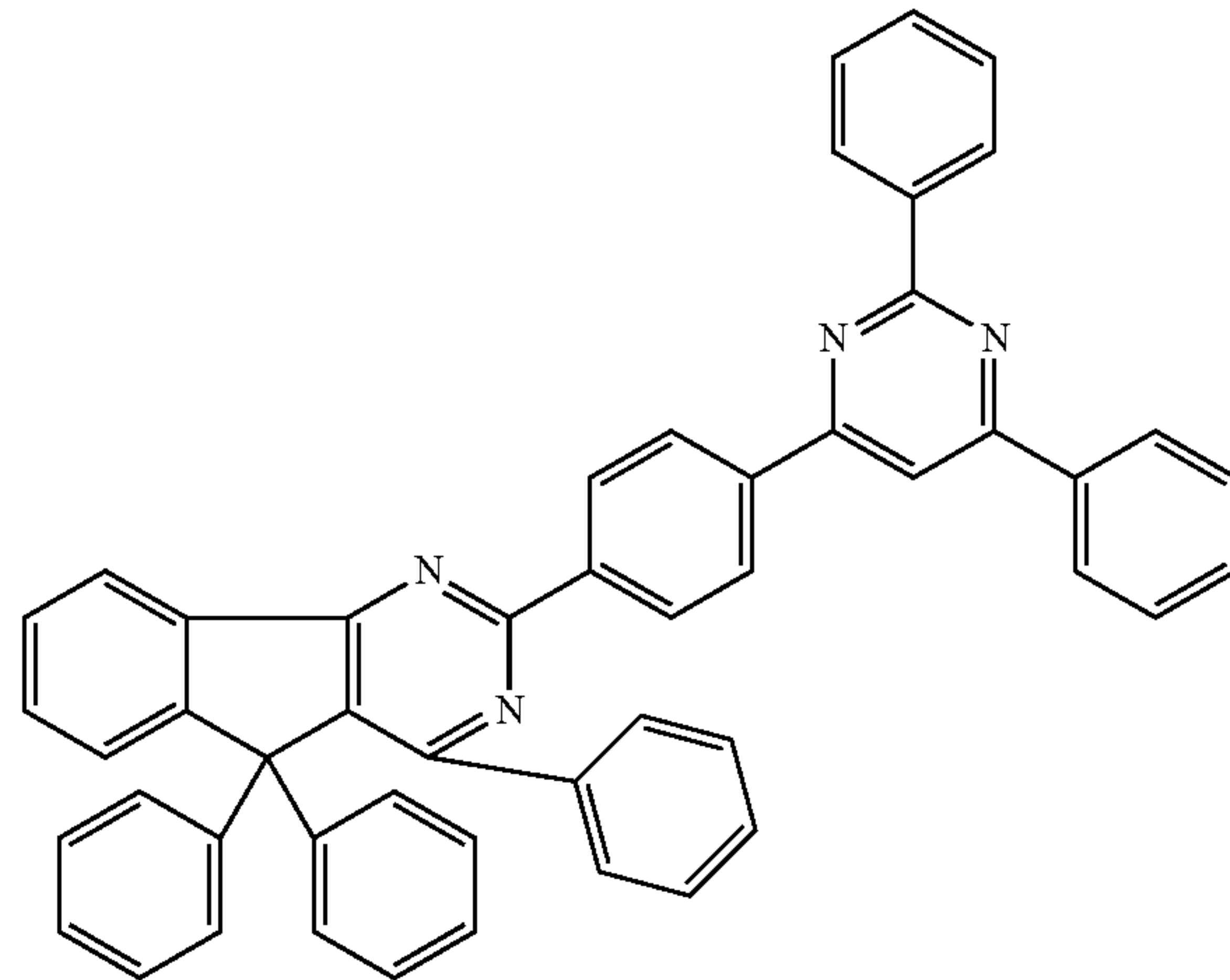
Chemical Formula 2-47
