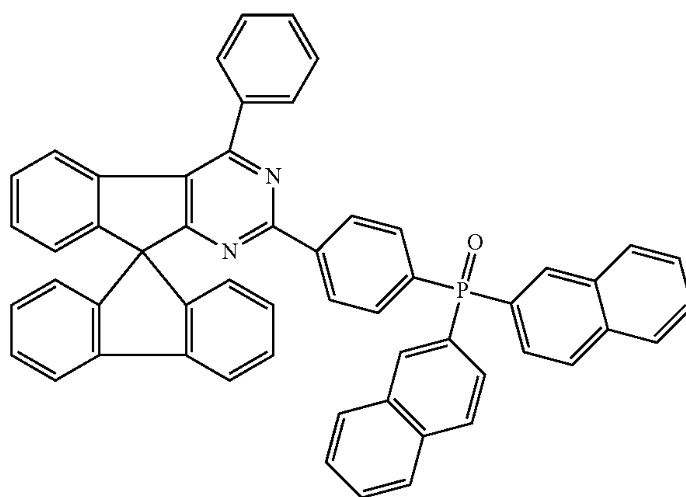
Chemical Formula 1-55
