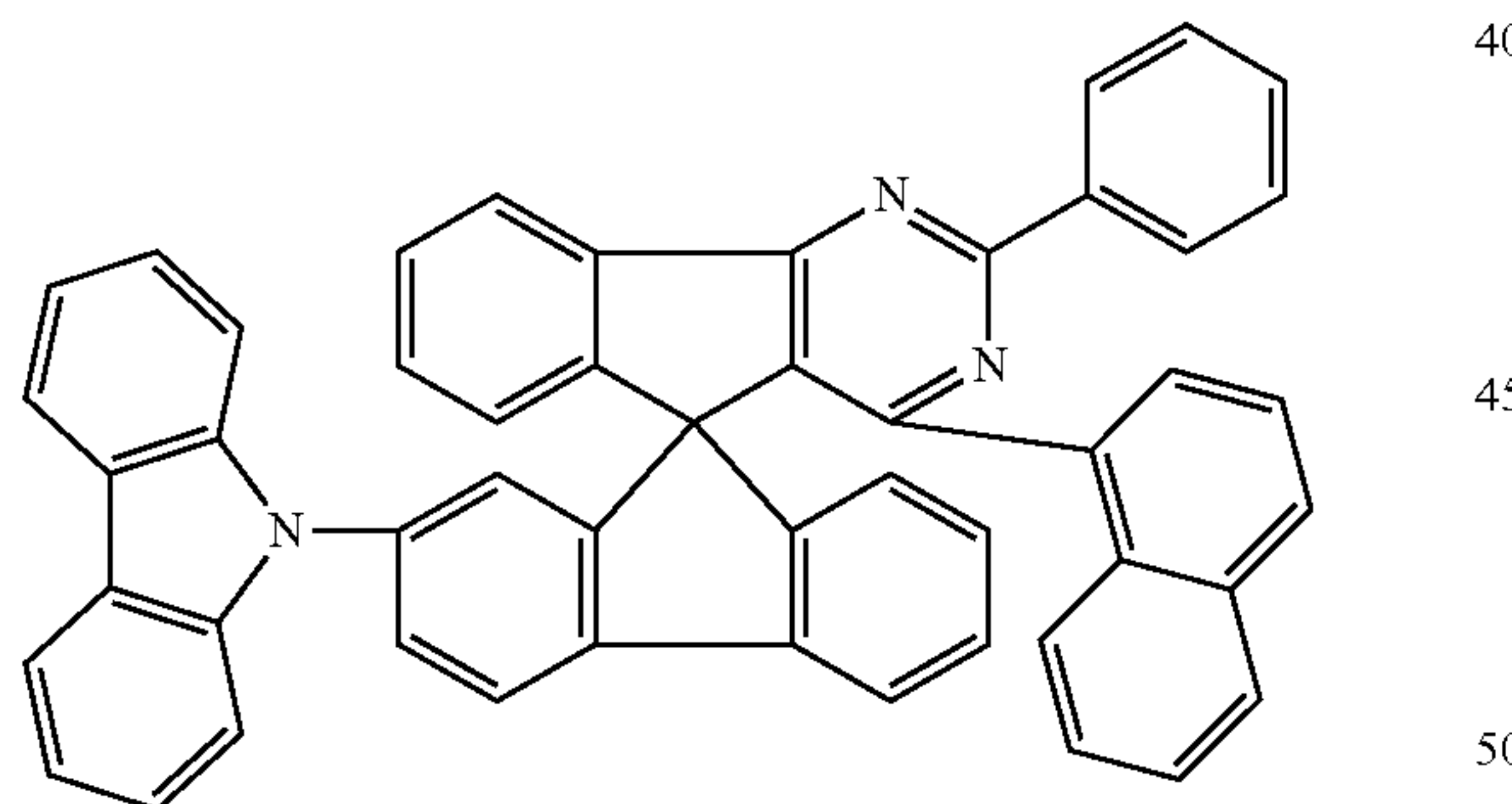
Chemical Formula 1-30
