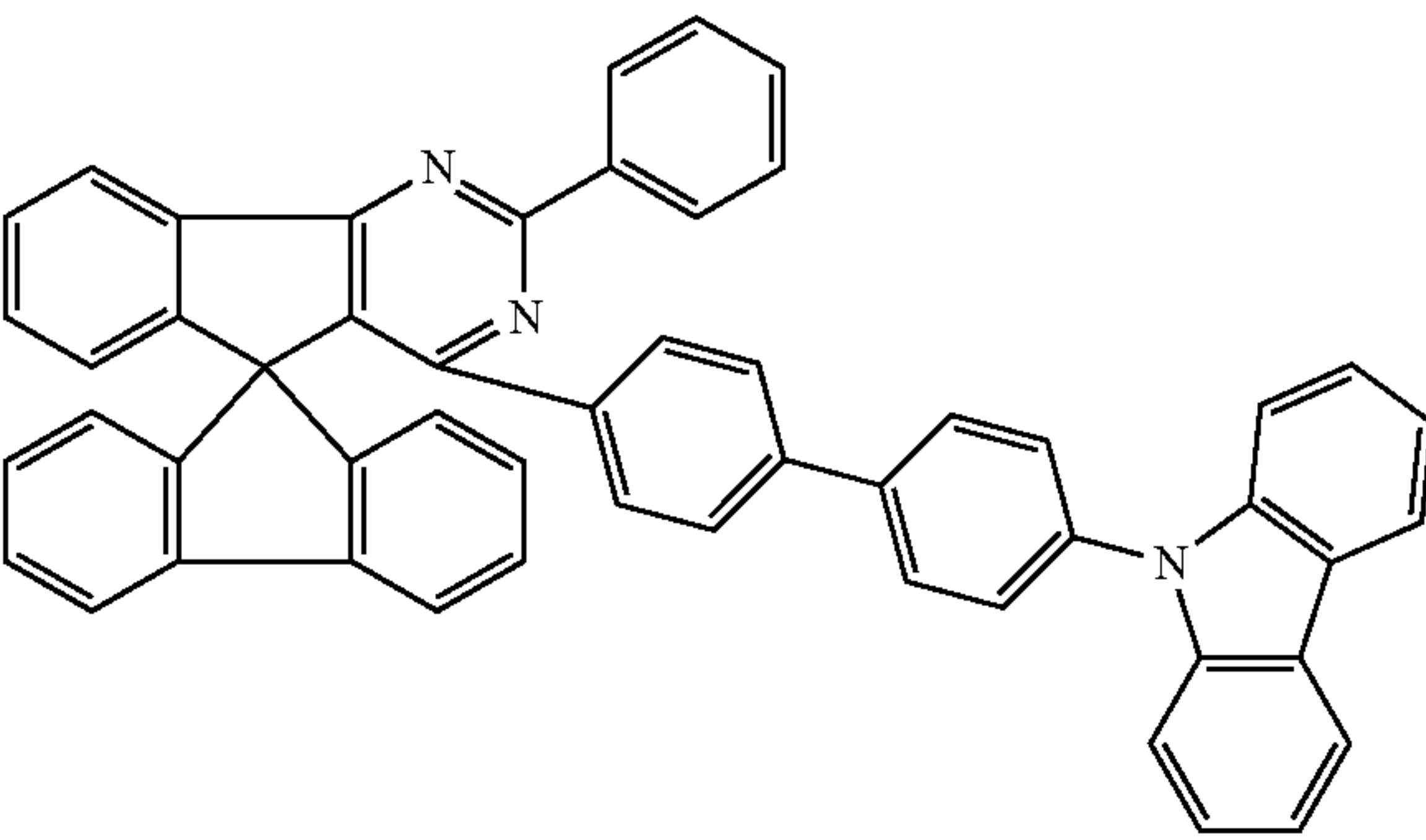
Chemical Formula 1-87
