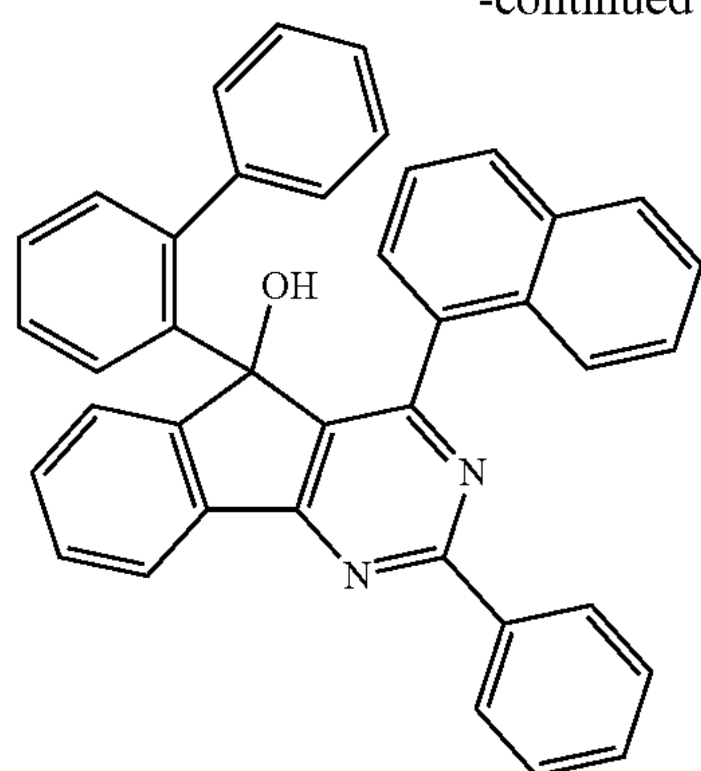
[Compound D-1]
