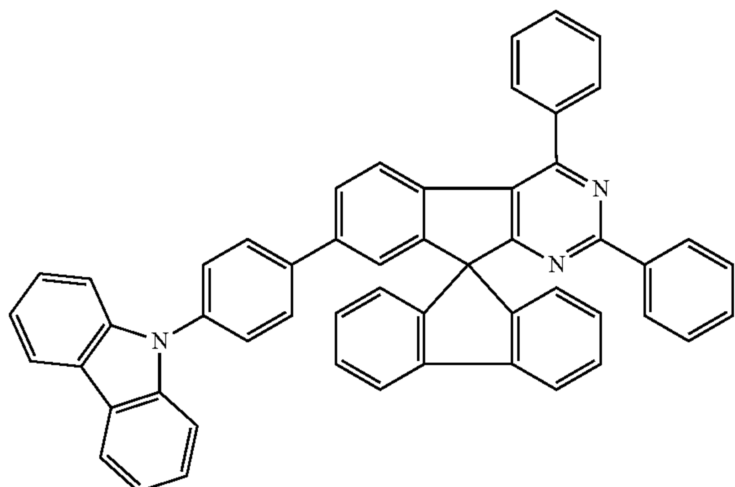
Chemical Formula 1-21
