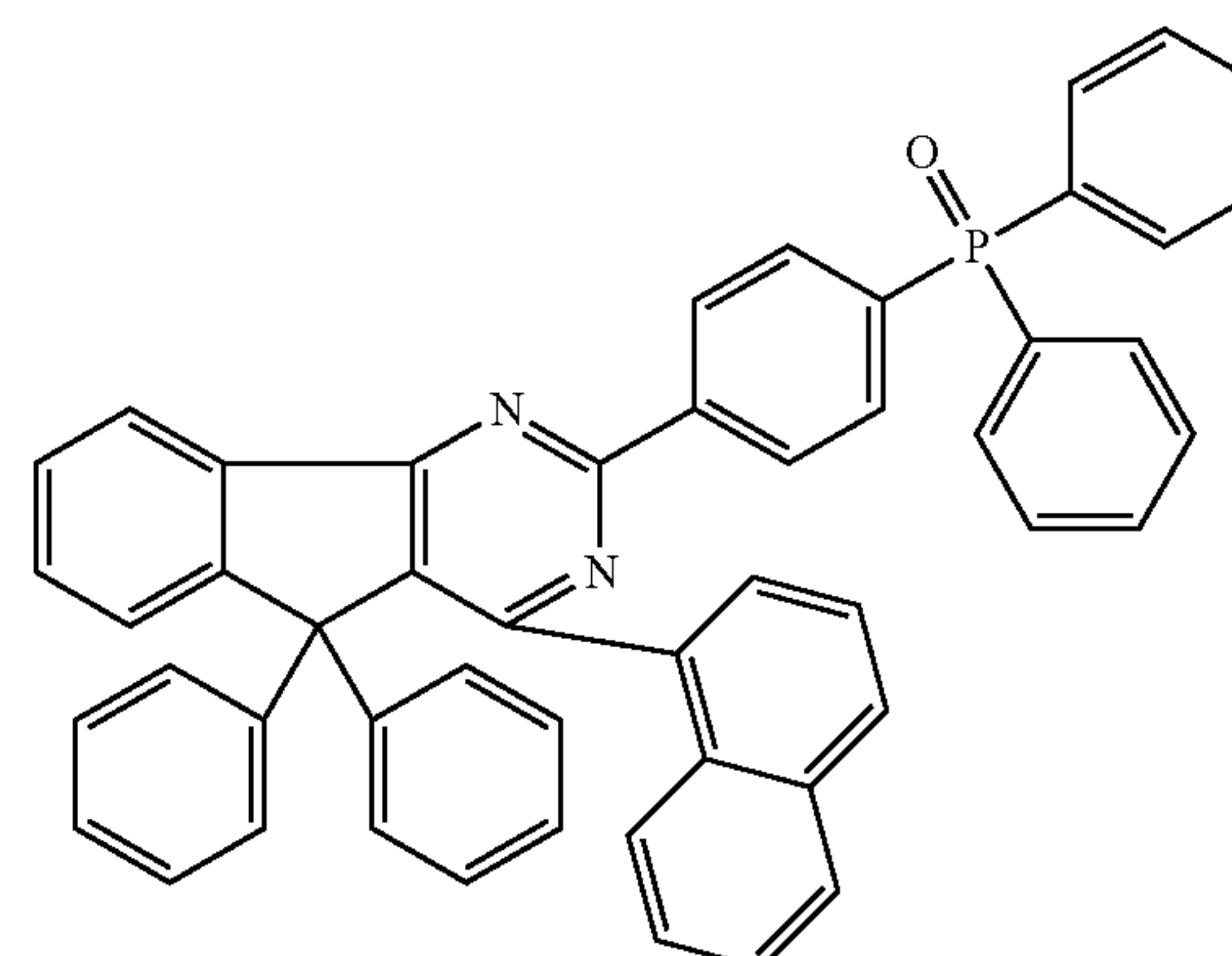
Chemical Formula 2-22
