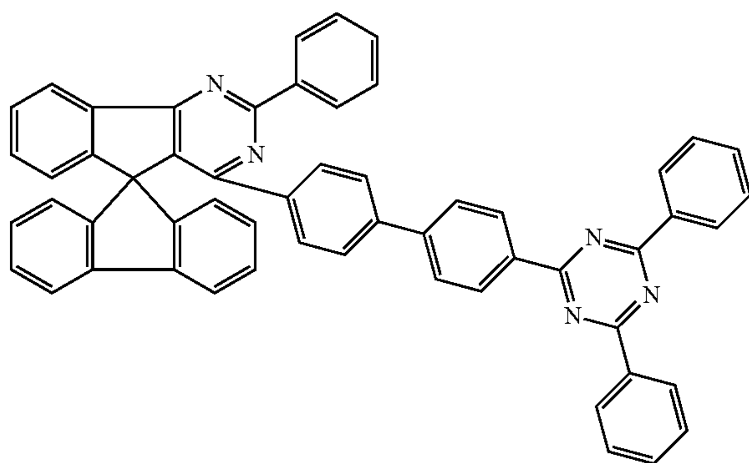
Chemical Formula 1-95
