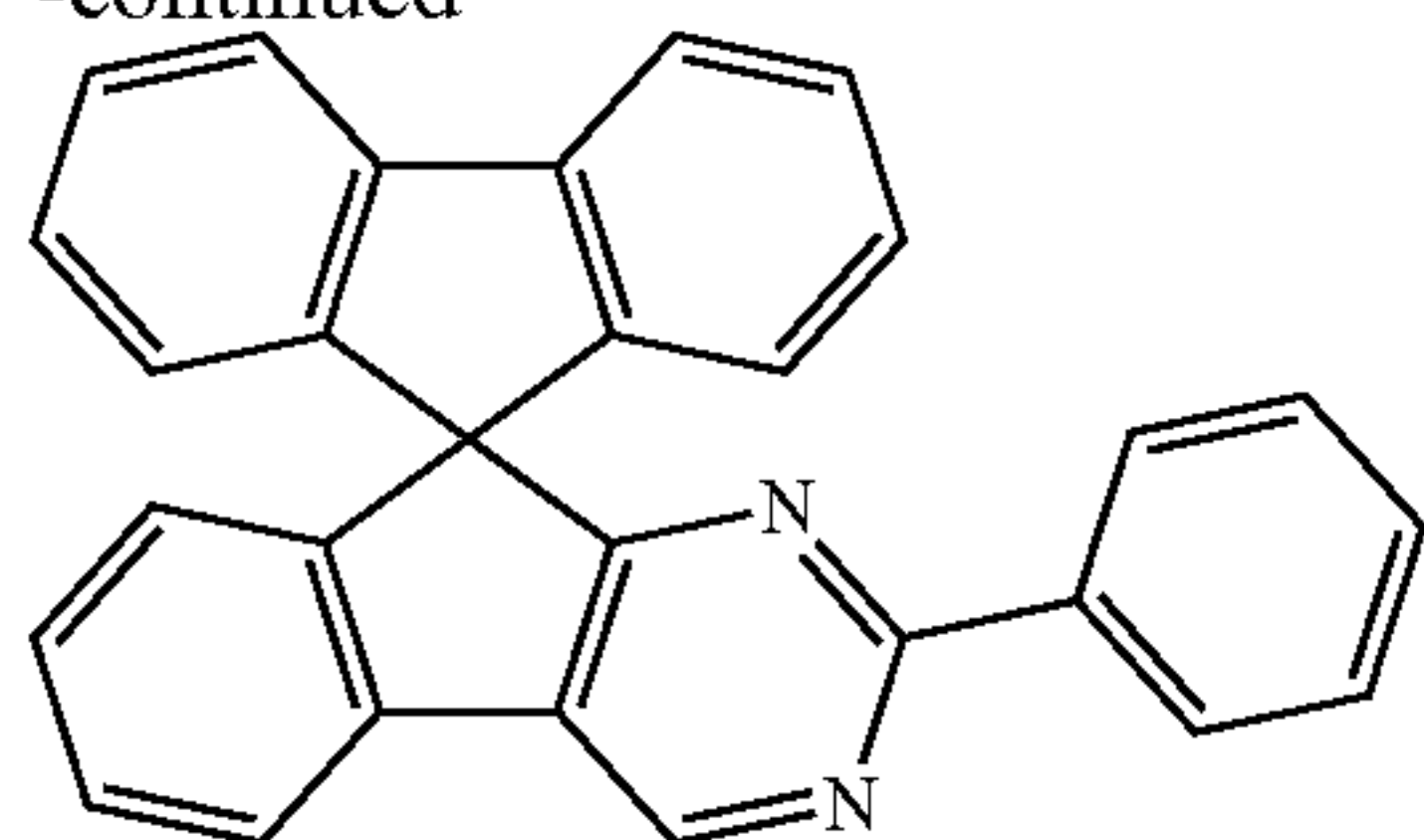
[Chemical Formula 1-10]
