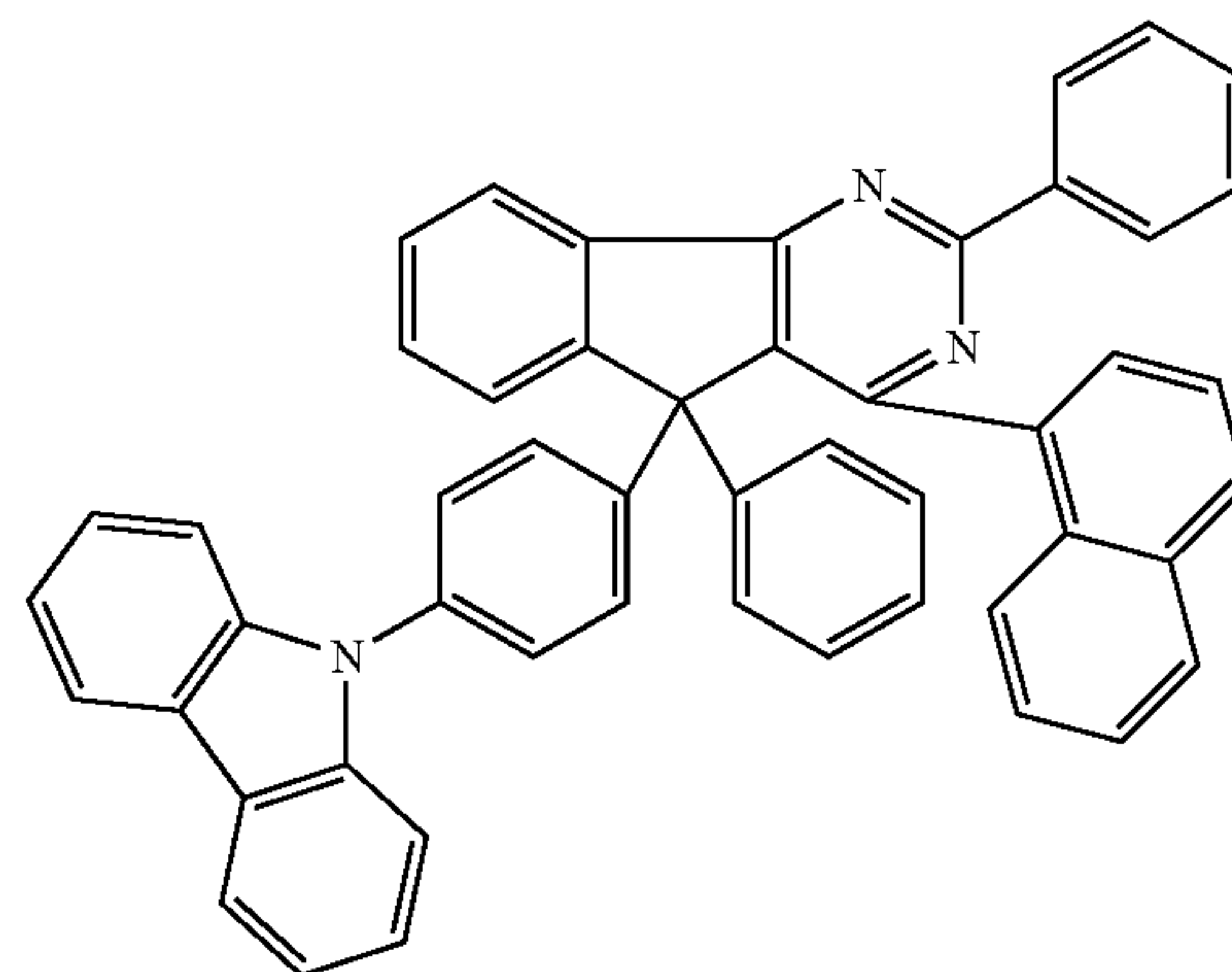
Chemical Formula 2-14
