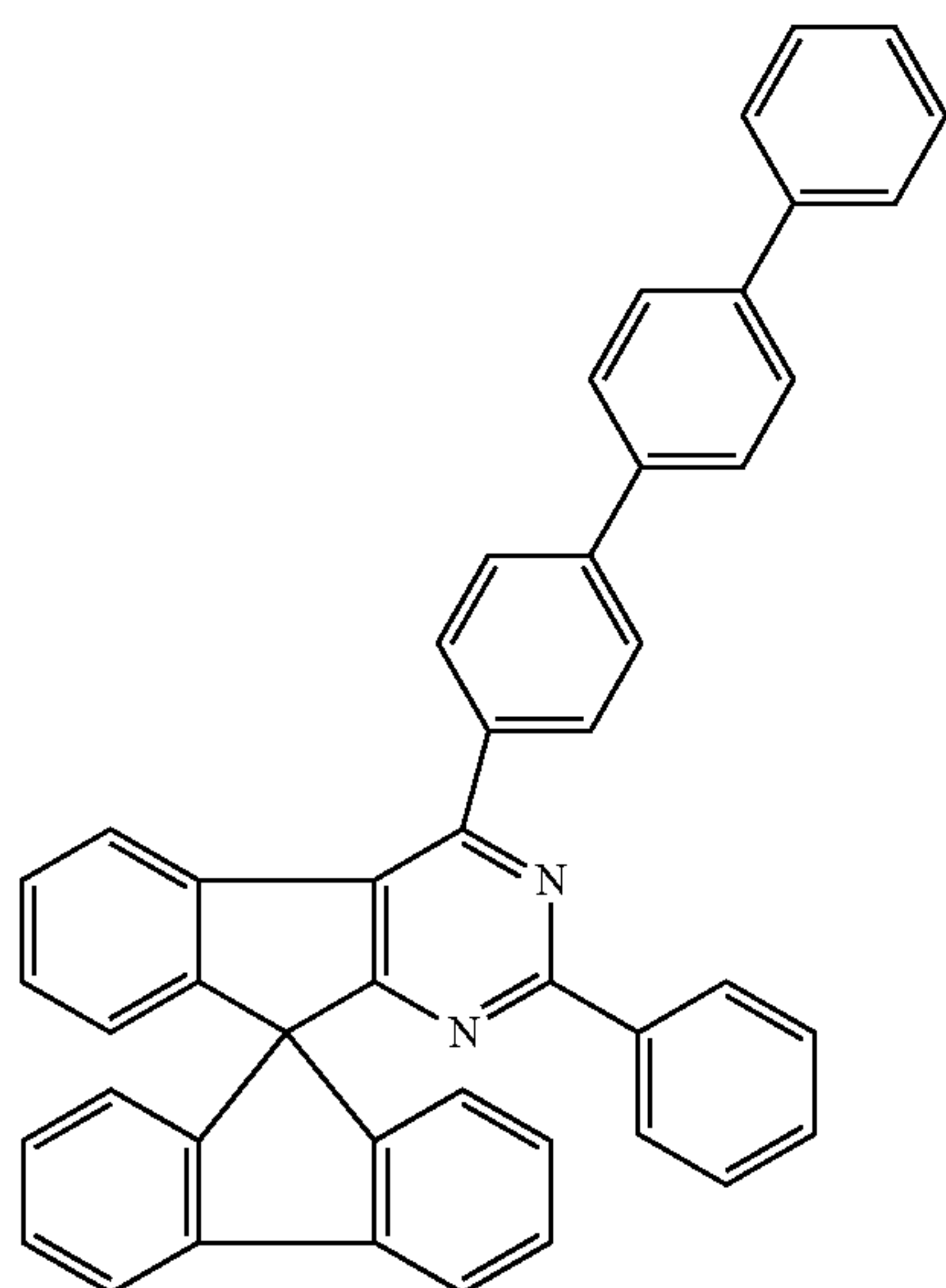
Chemical Formula 1-82
