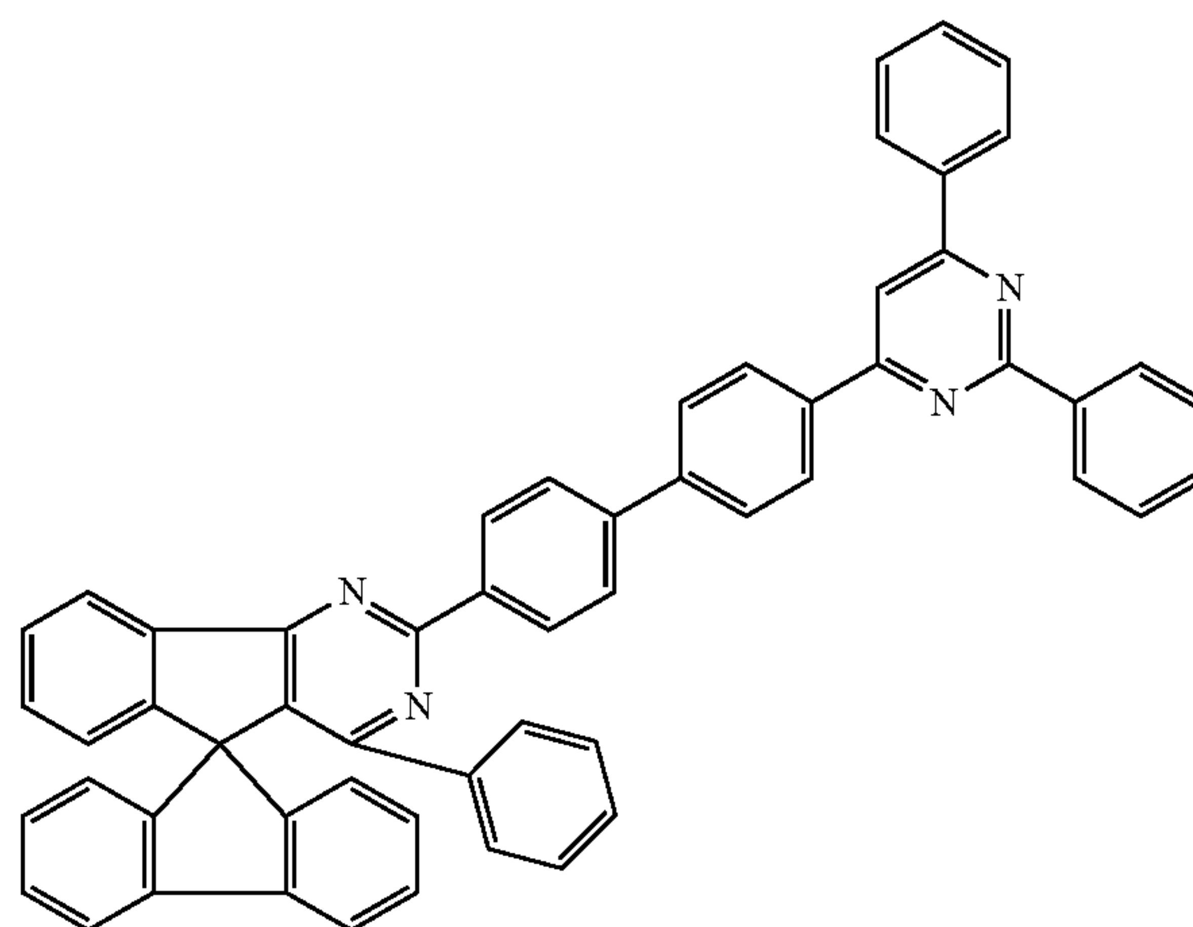
Chemical Formula 1-98
