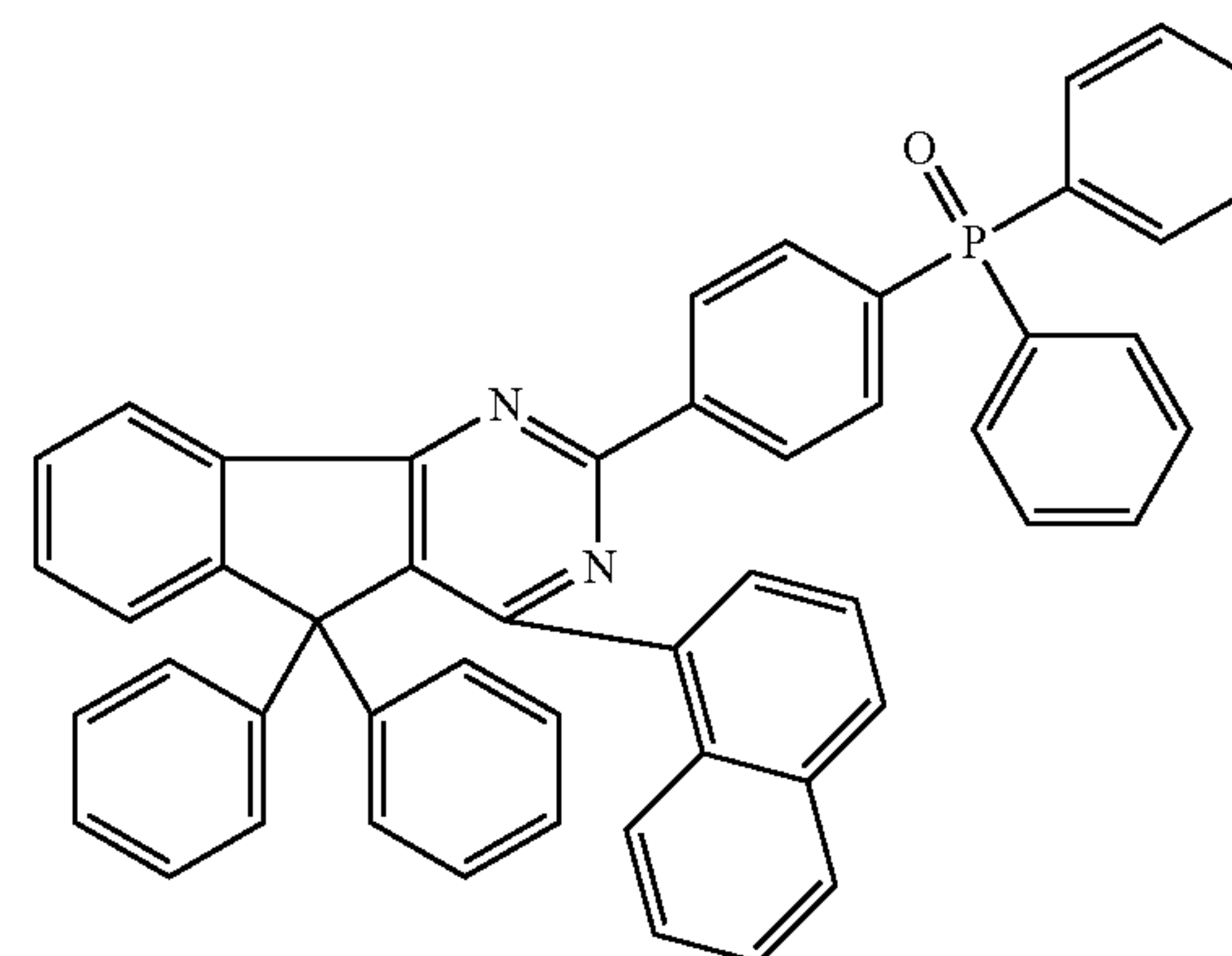
Chemical Formula 2-22
