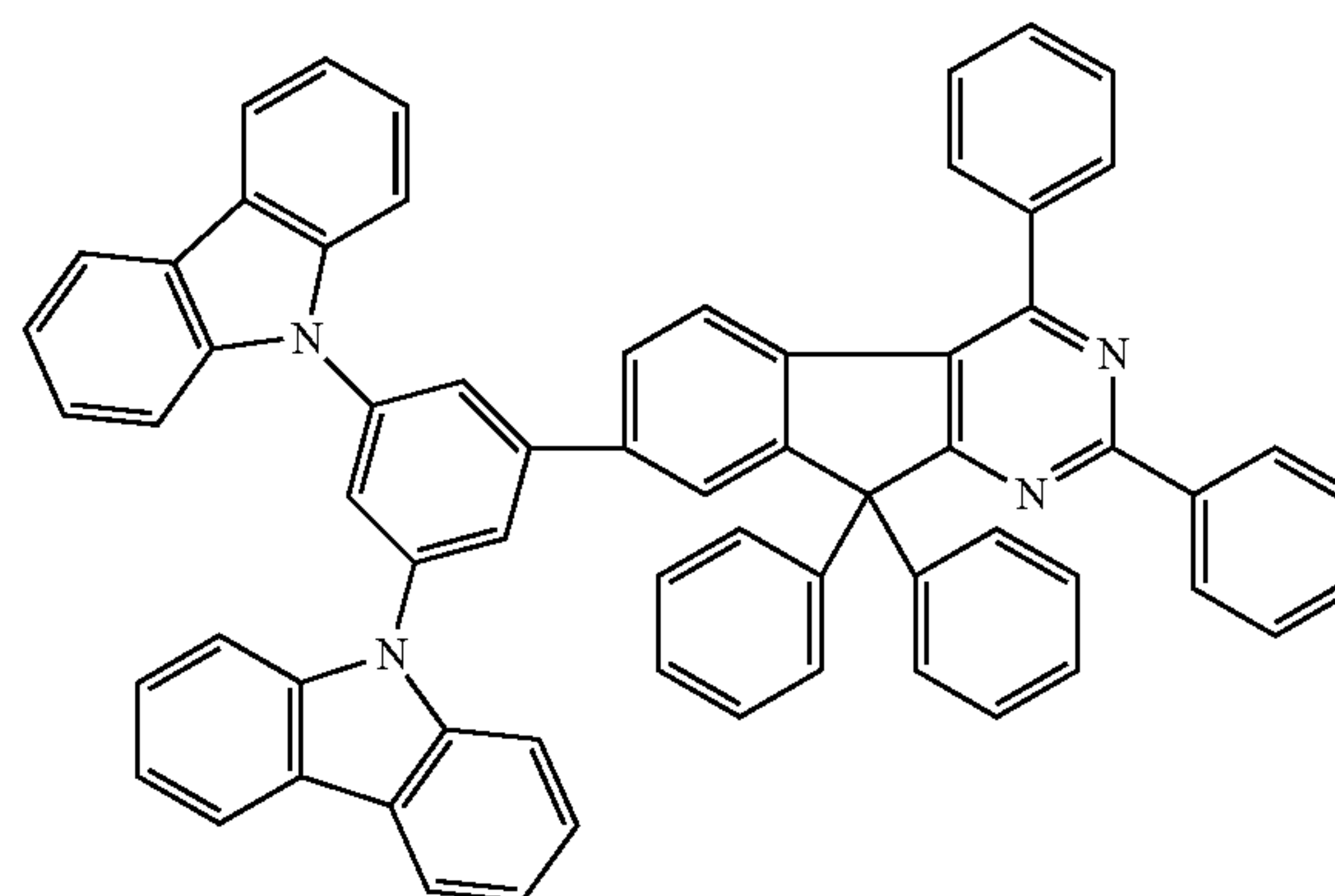
Chemical Formula 2-35
