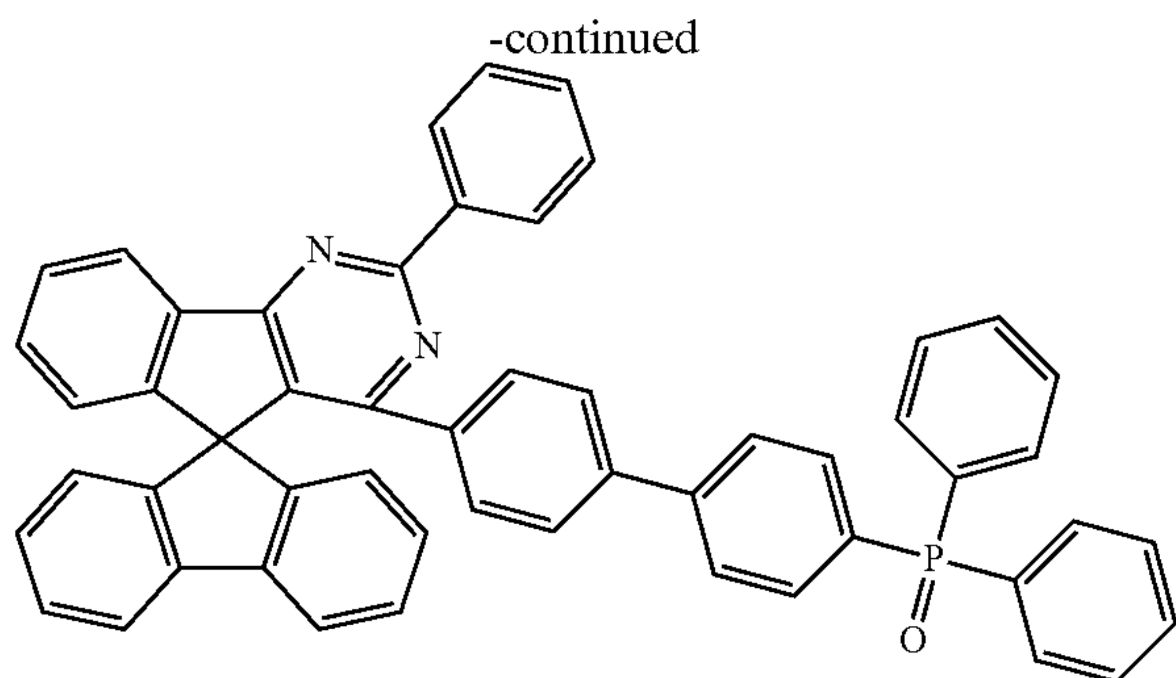
[Compound Formula 1-56]
