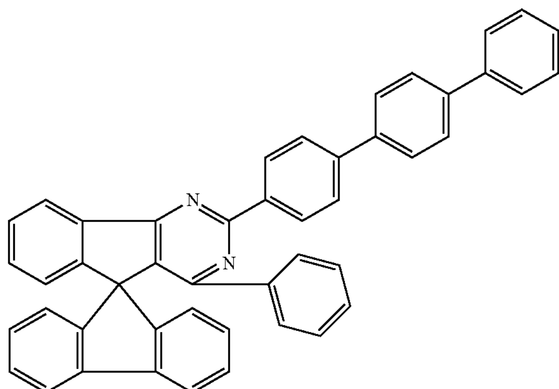
Chemical Formula 1-59
