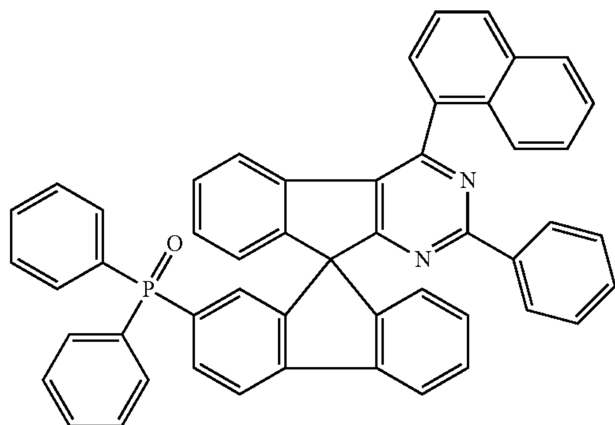
Chemical Formula 1-44
