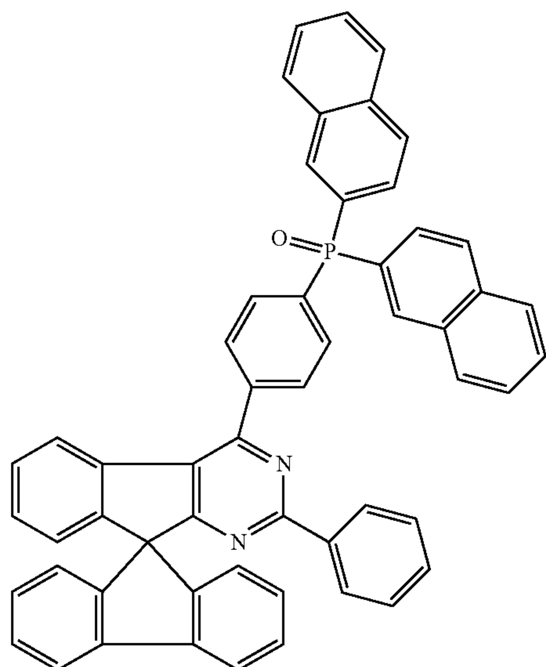
Chemical Formula 1-78
