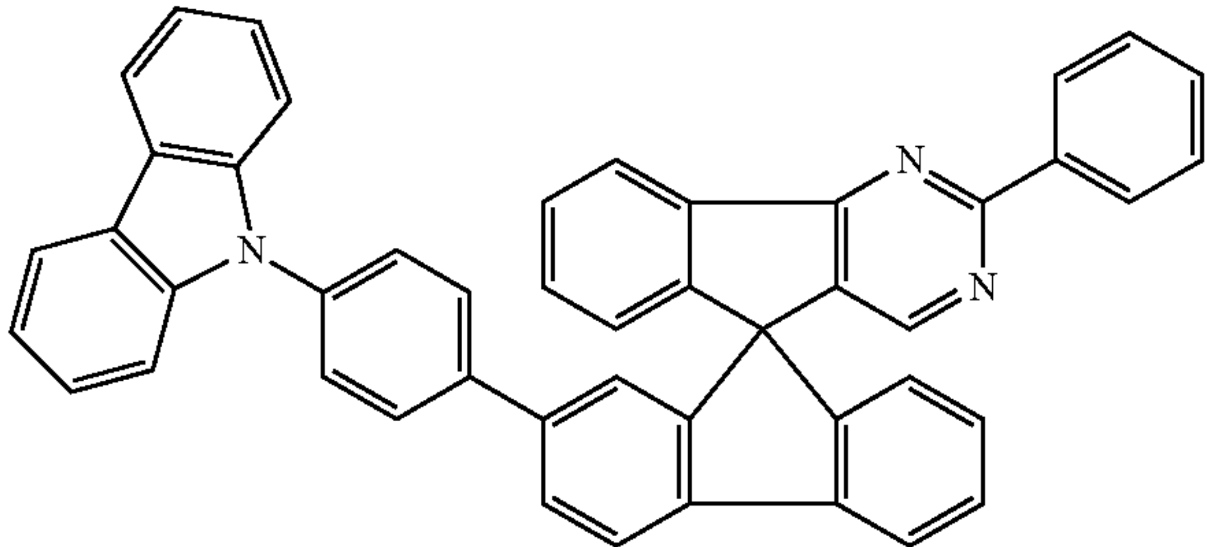
Chemical Formula 1-13
