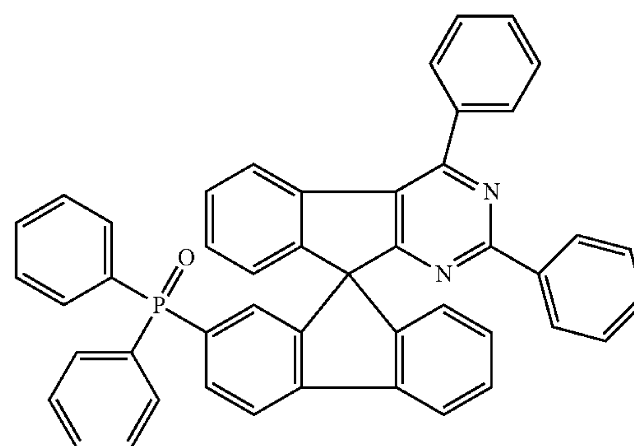
Chemical Formula 1-43
