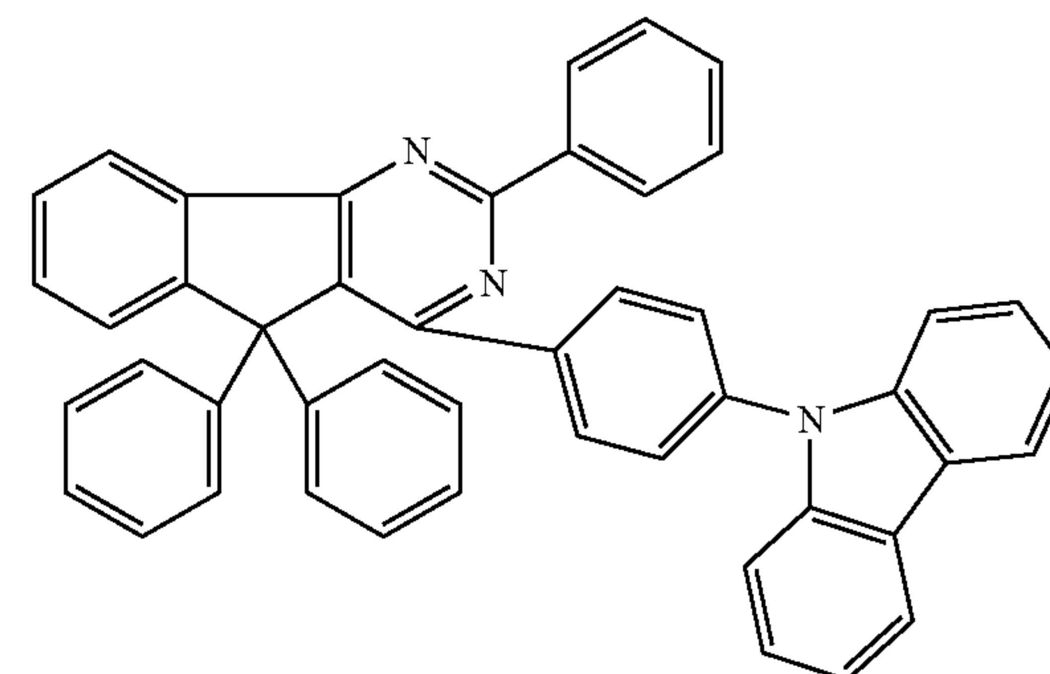
Chemical Formula 2-41
