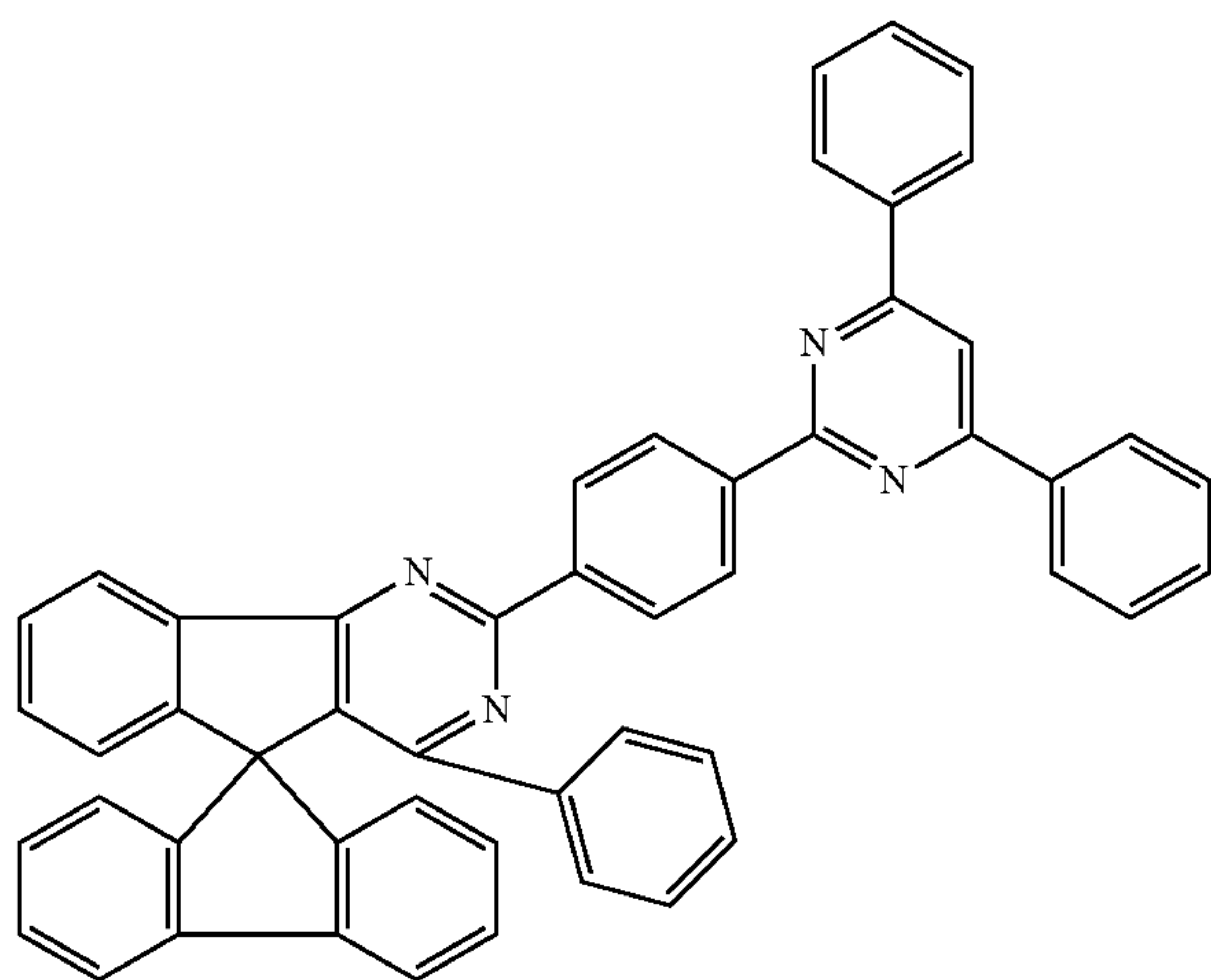
Chemical Formula 1-94
