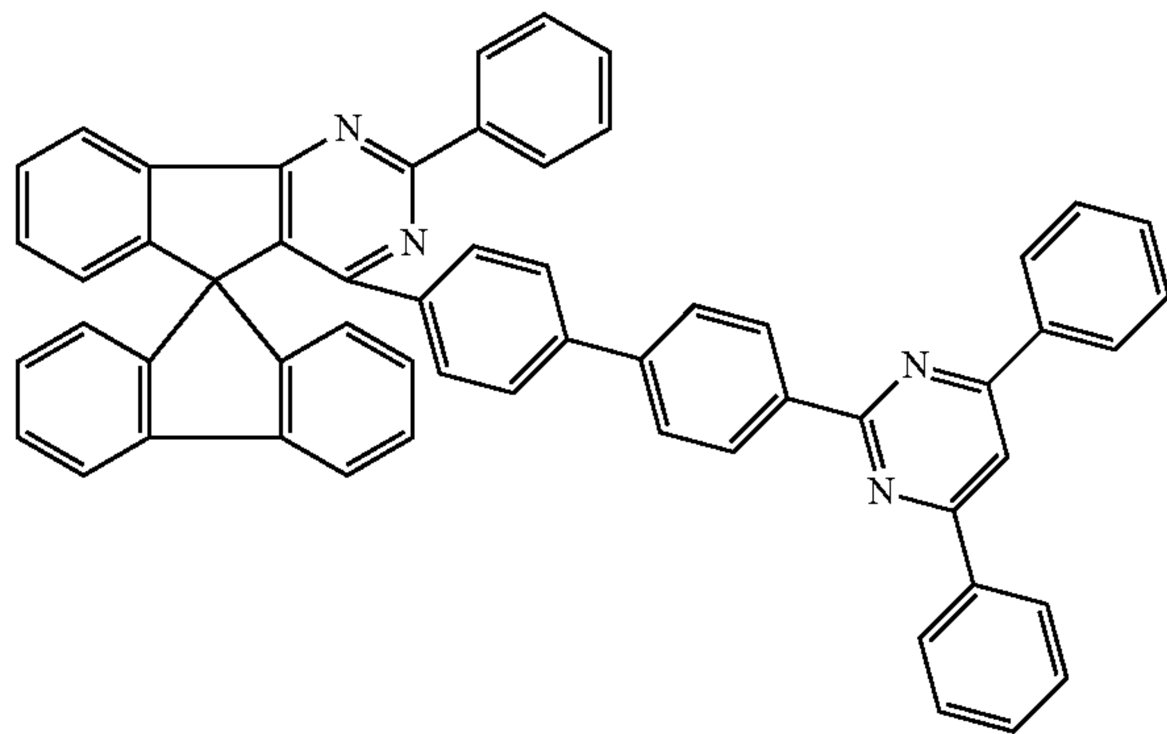
Chemical Formula 1-100
