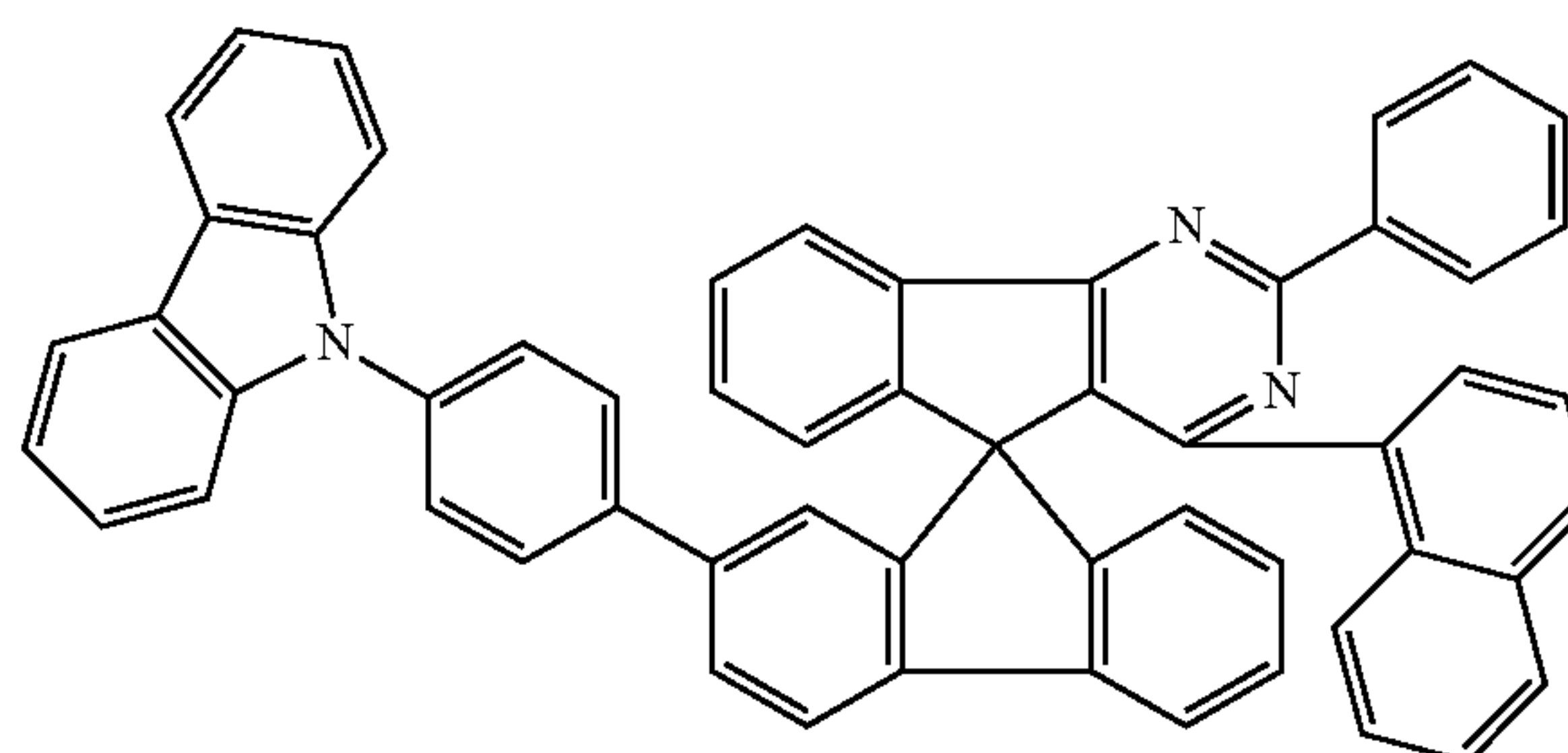
Chemical Formula 1-33
