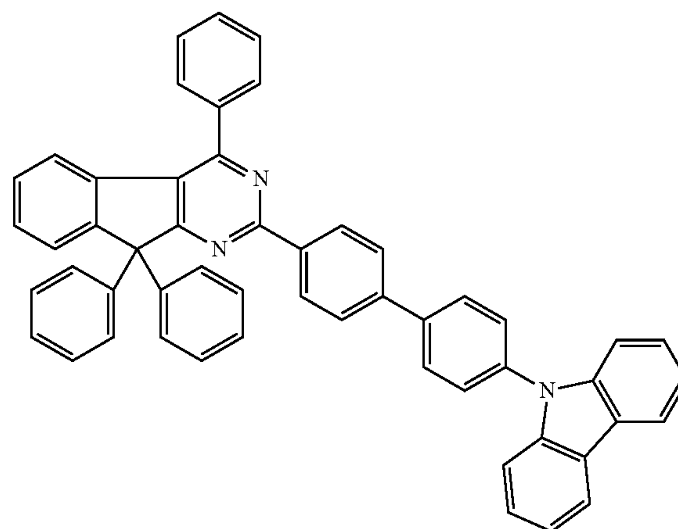
Chemical Formula 2-32
