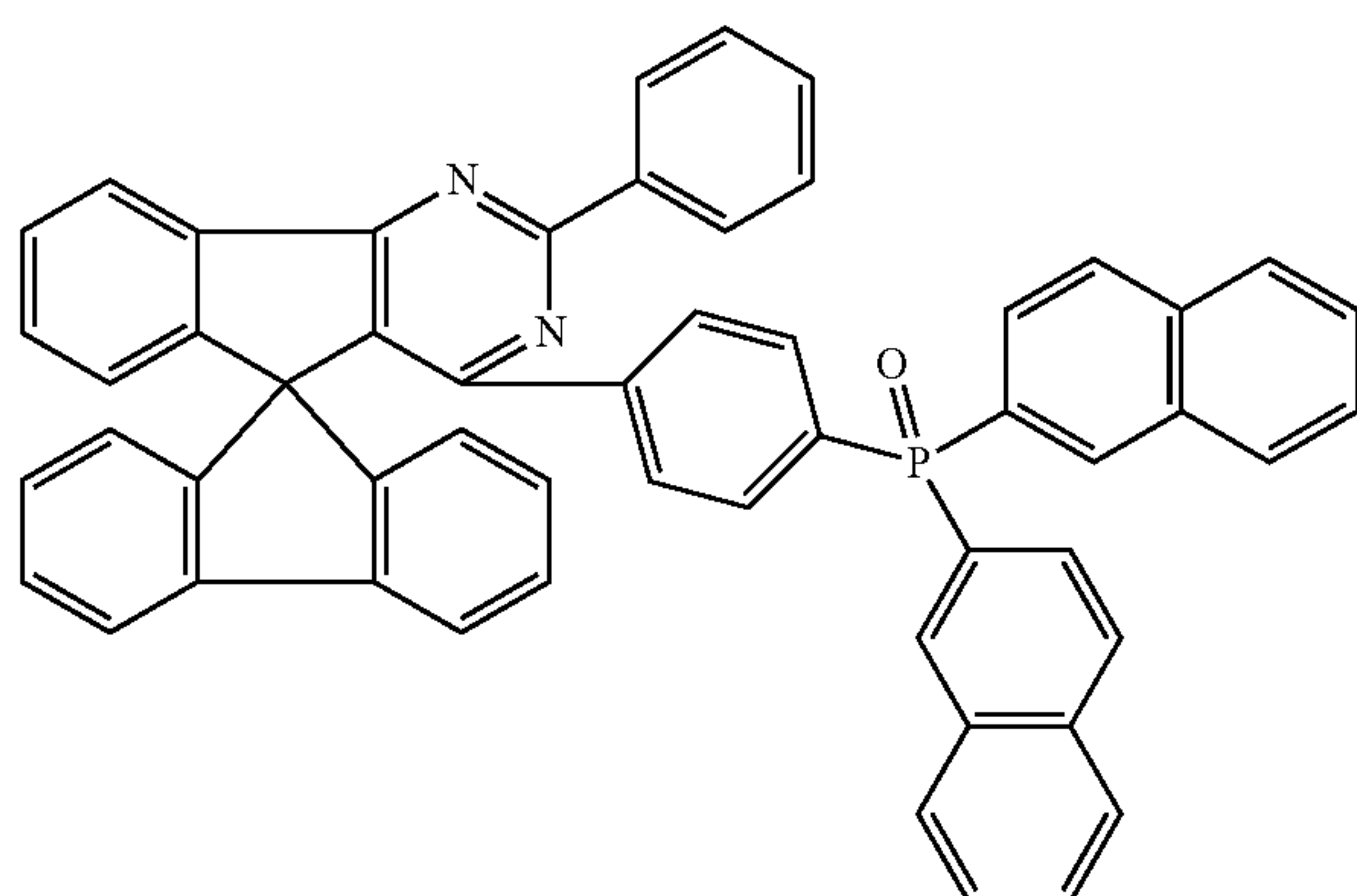
Chemical Formula 1-77
