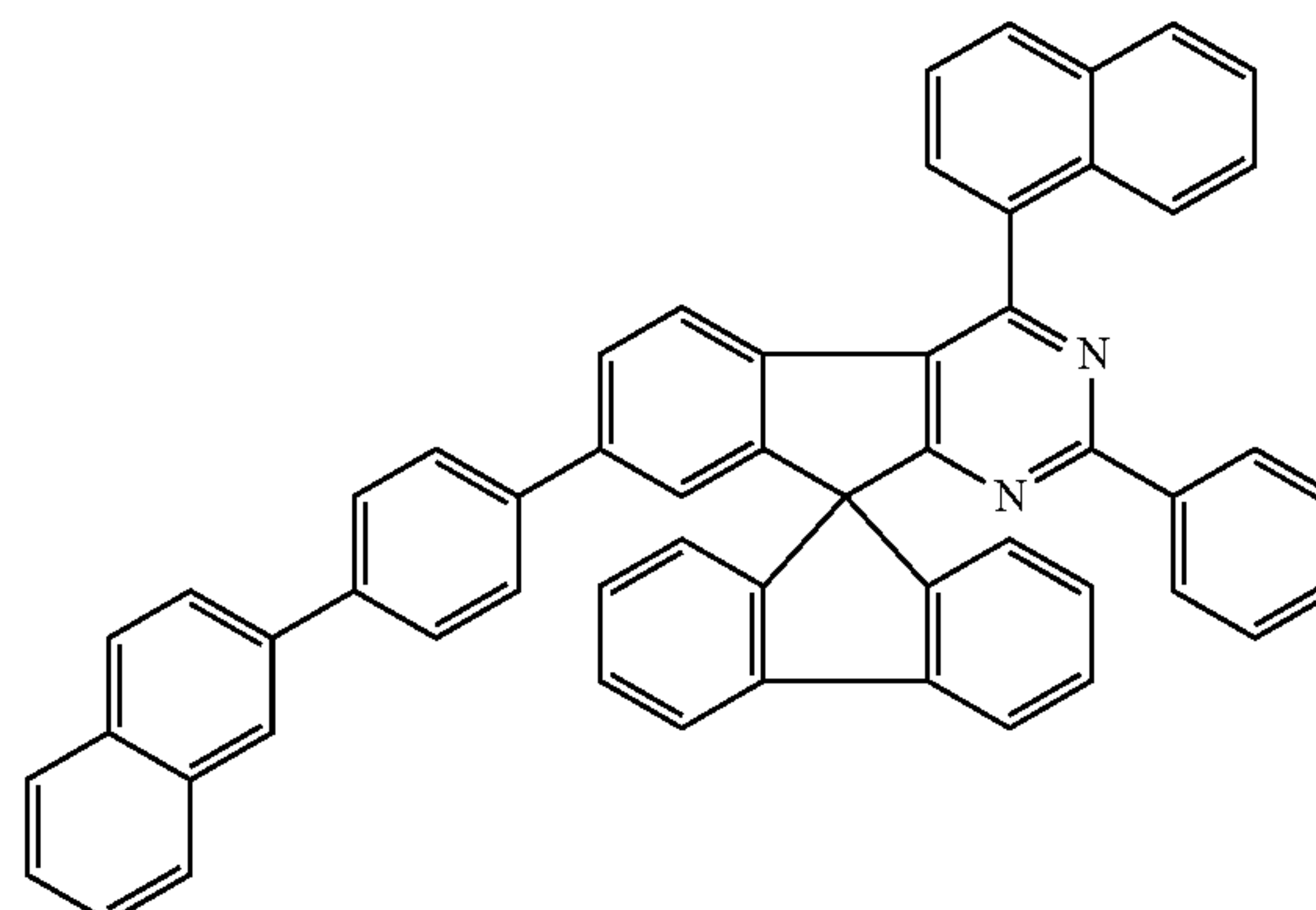
Chemical Formula 1-40
