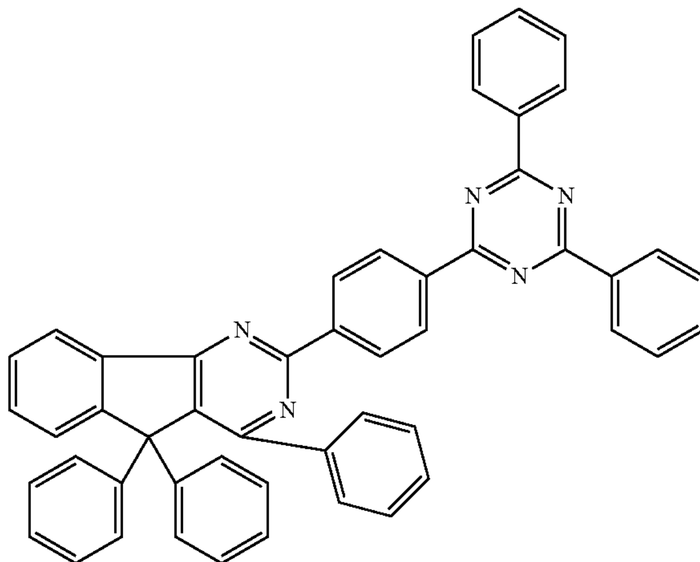
Chemical Formula 2-44
