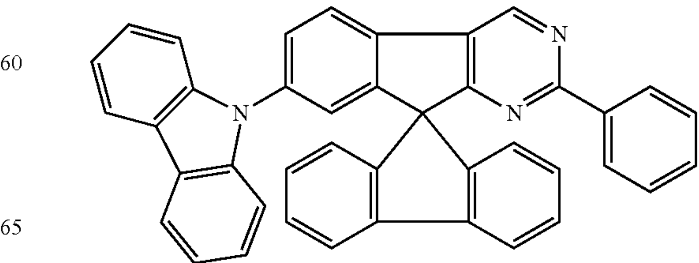
Chemical Formula 1-18
