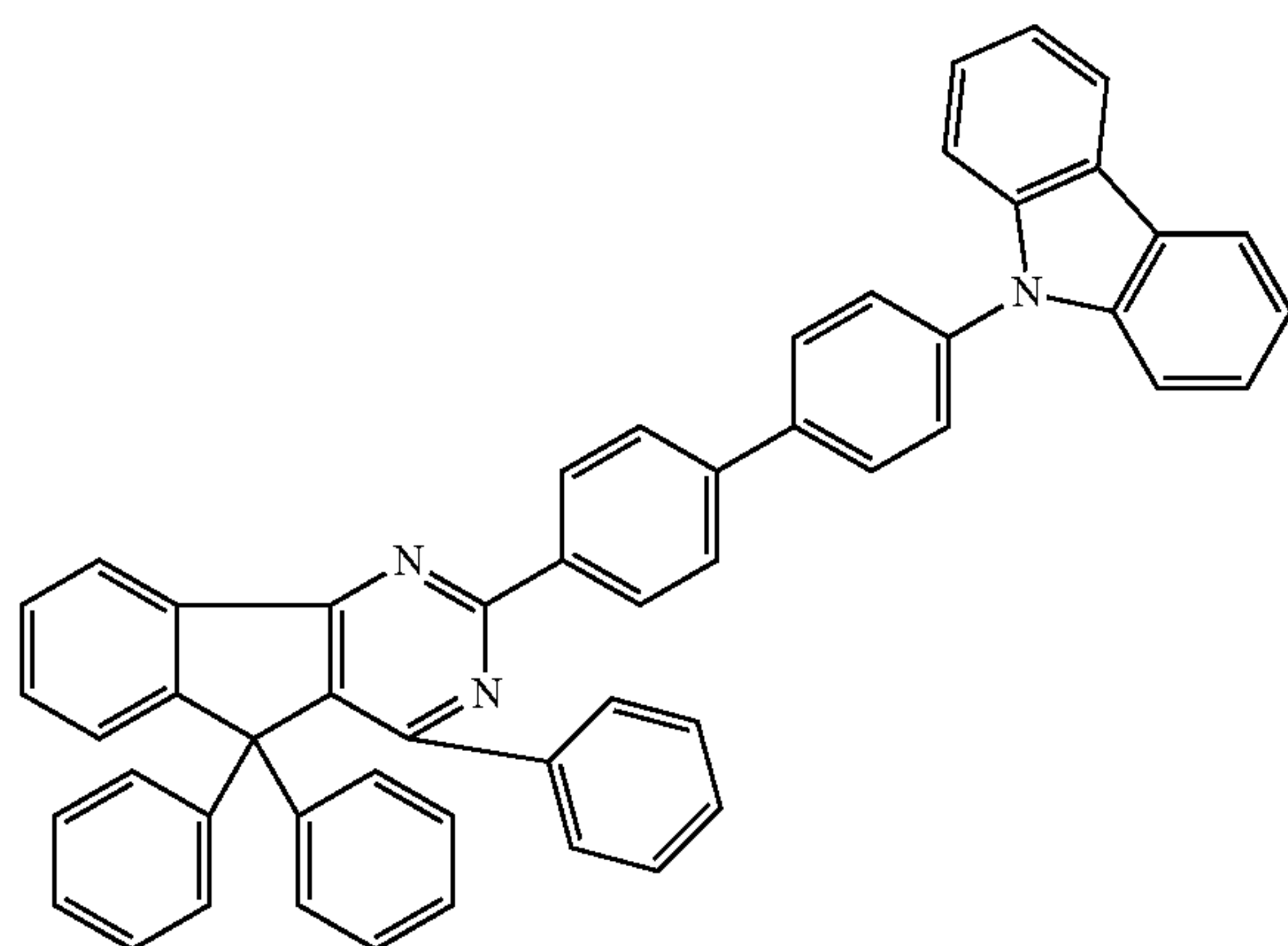
Chemical Formula 2-31
