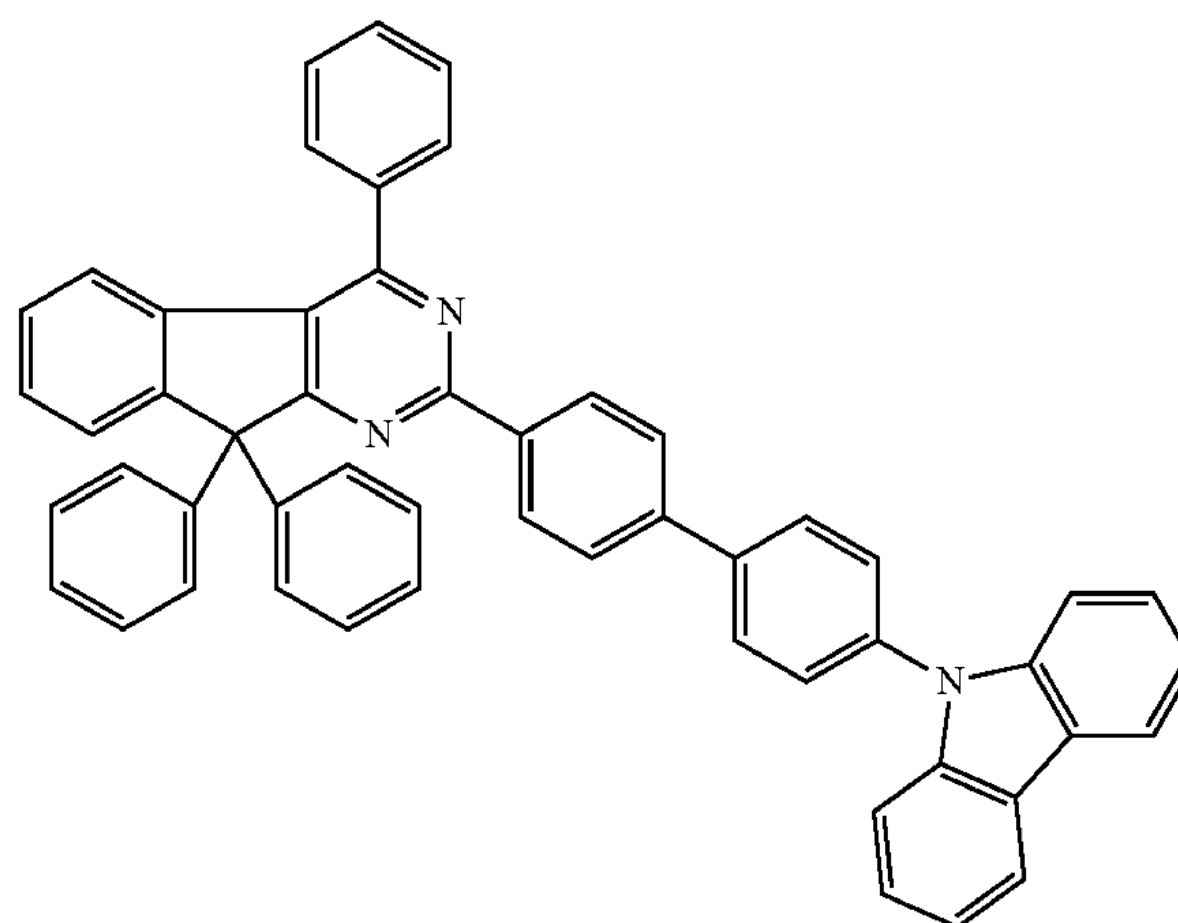
Chemical Formula 2-32
