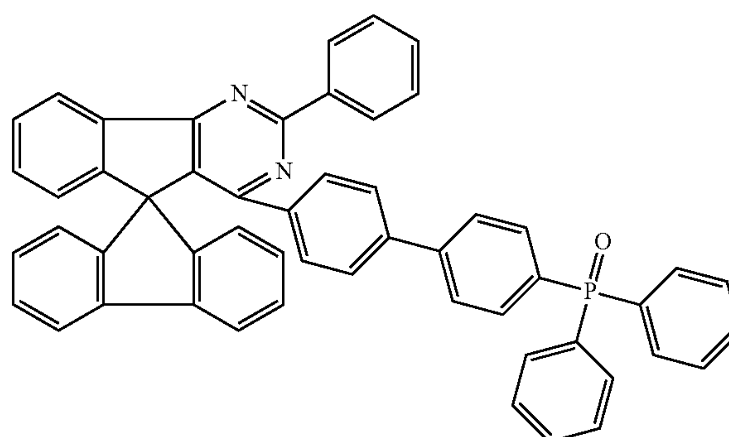
Chemical Formula 1-79
