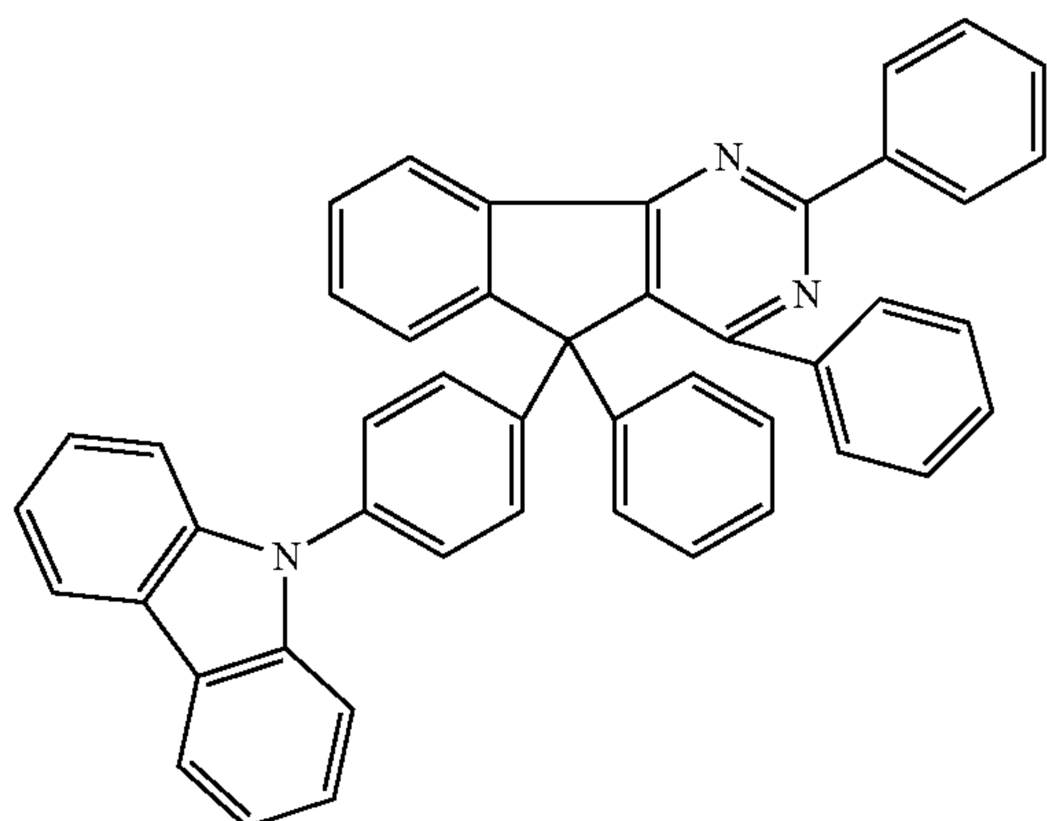
Chemical Formula 2-9
