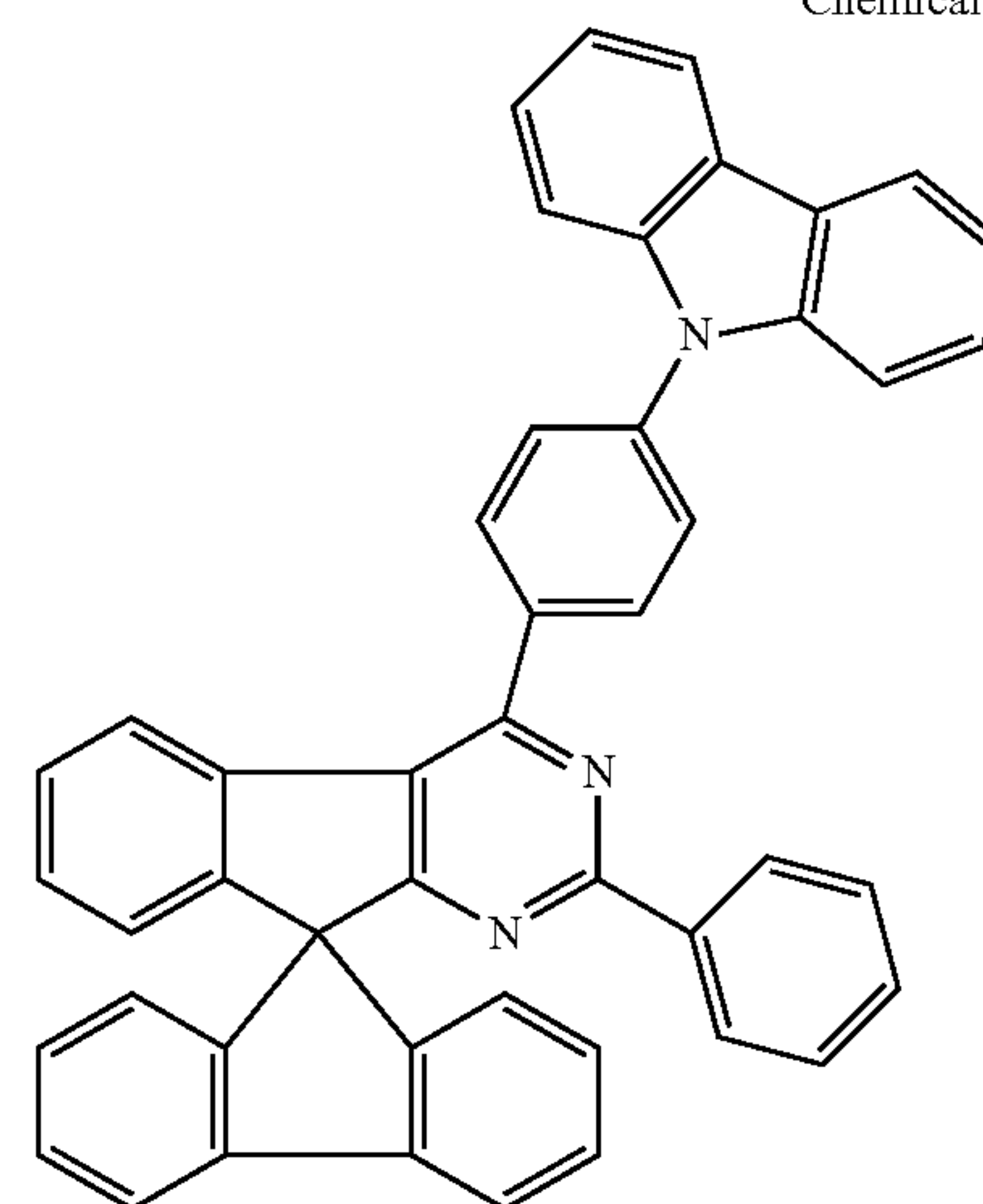
Chemical Formula 1-86
