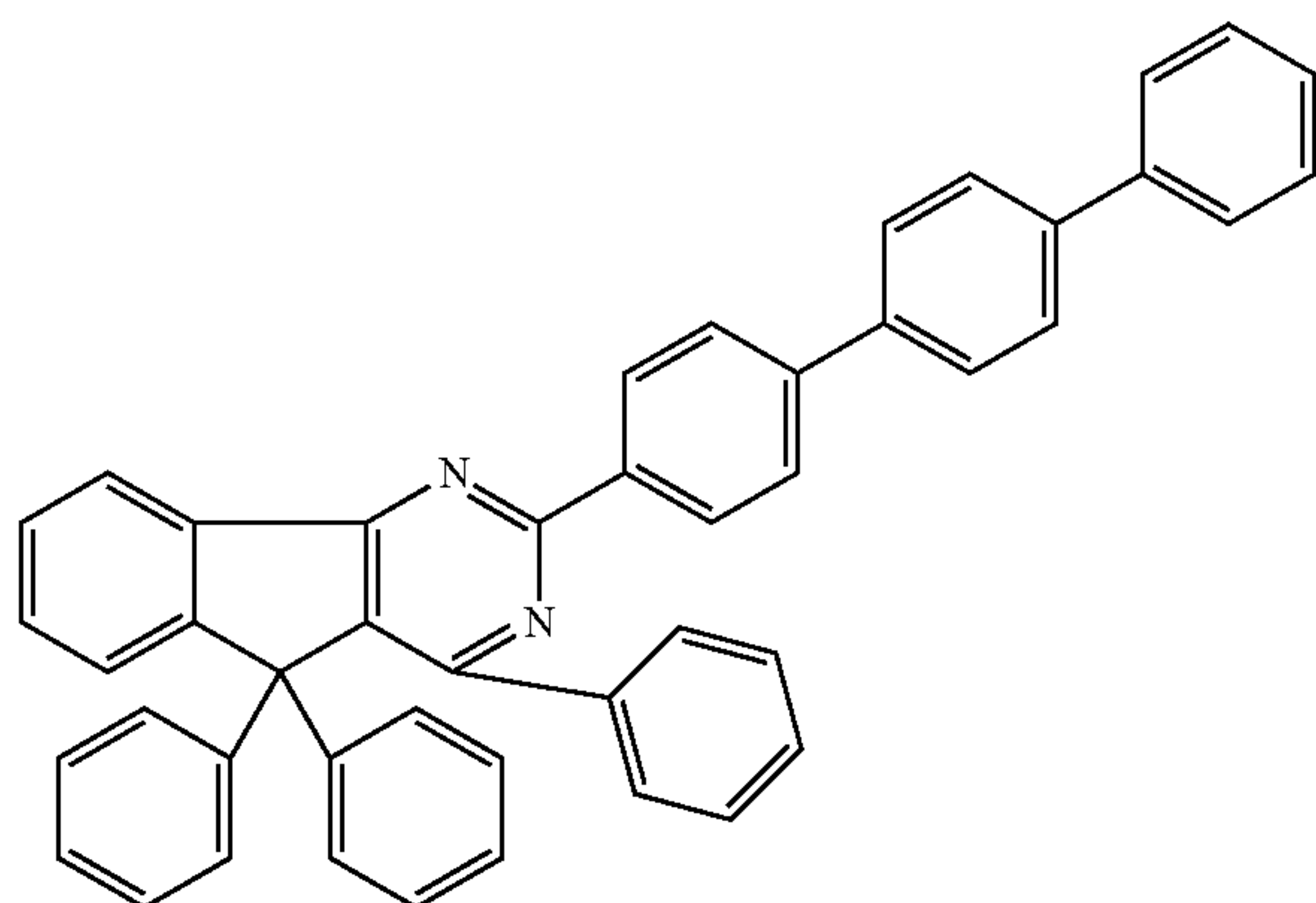
Chemical Formula 2-25
