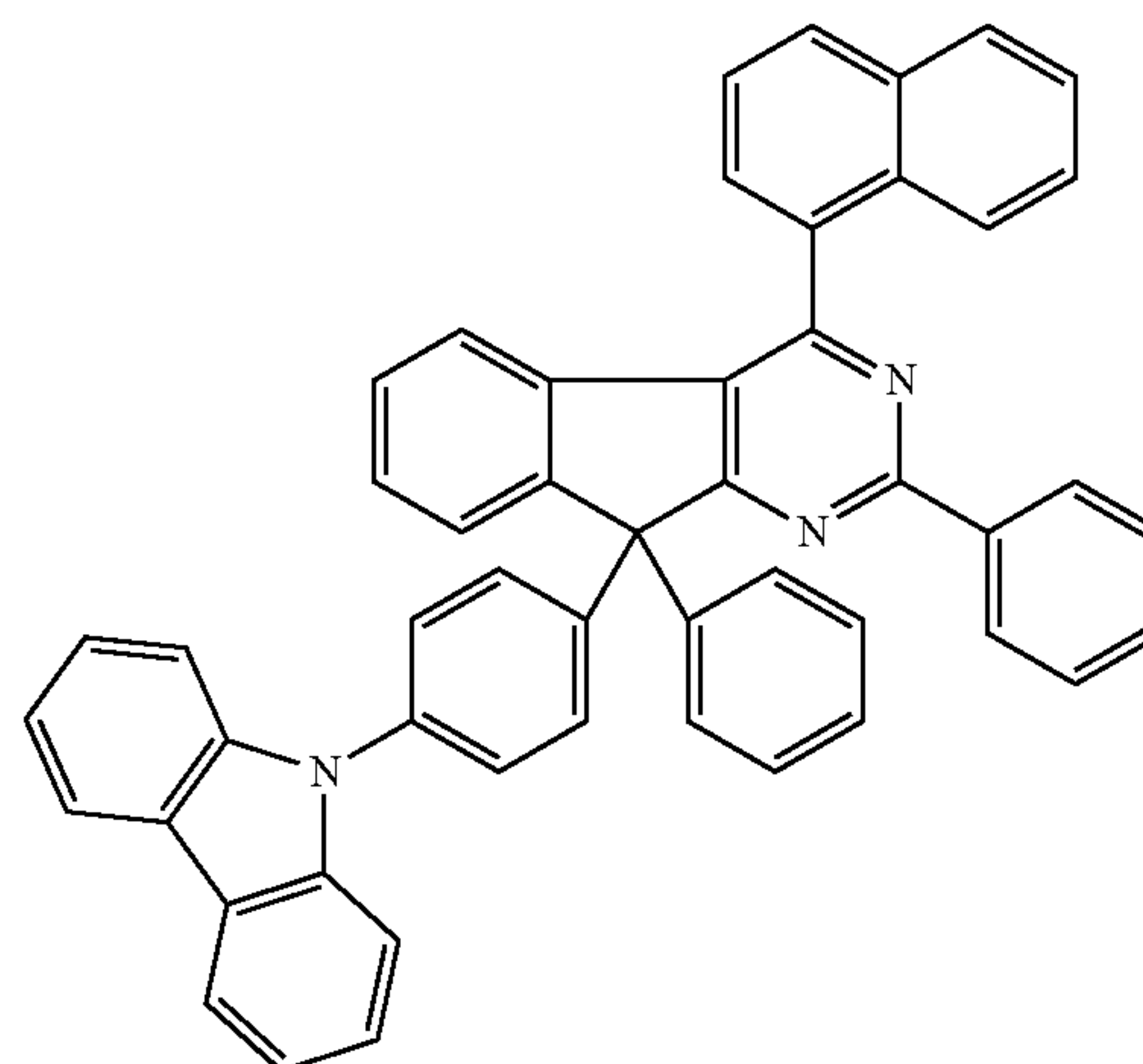
Chemical Formula 2-14
