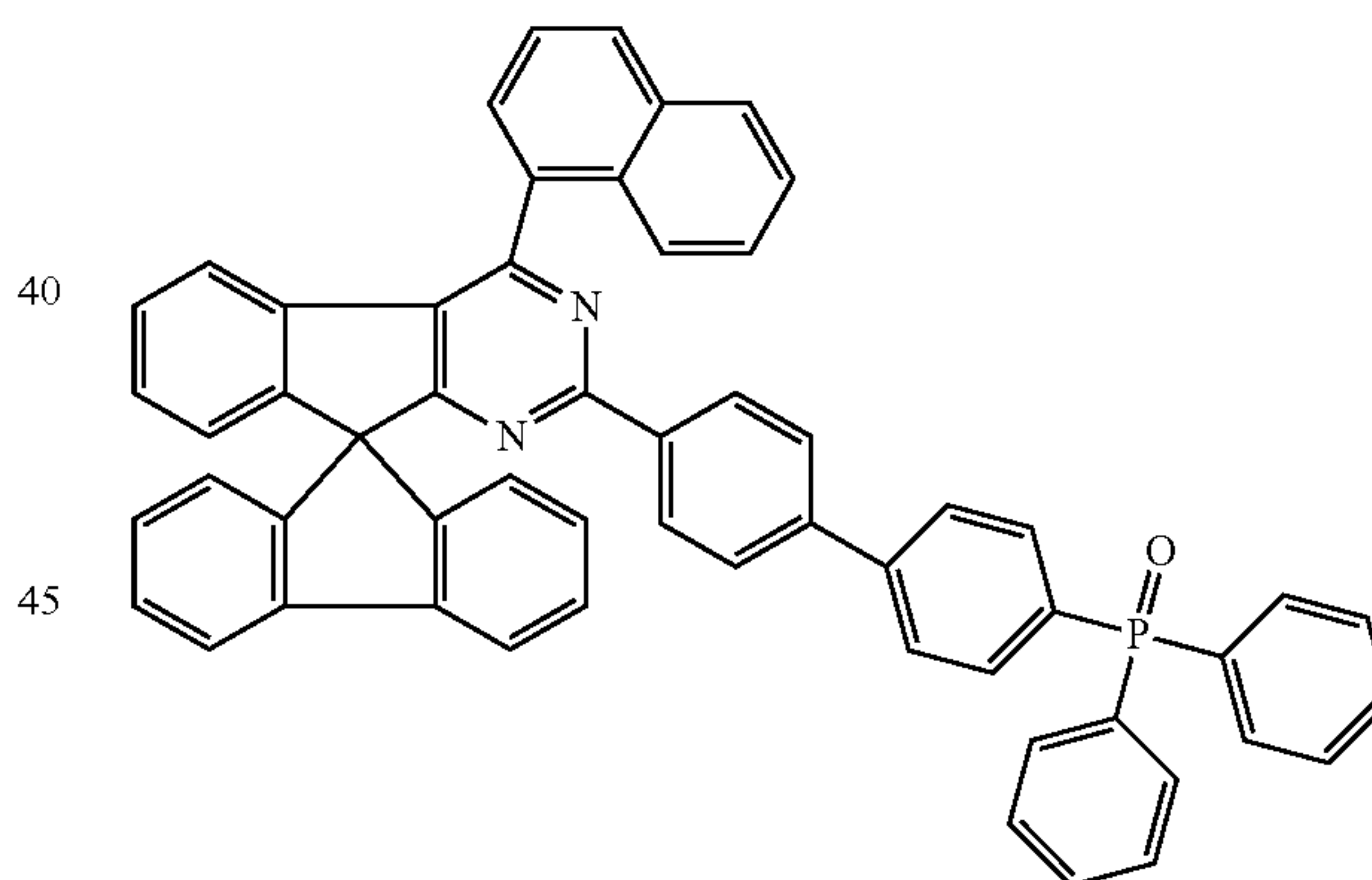
Chemical Formula 1-59
