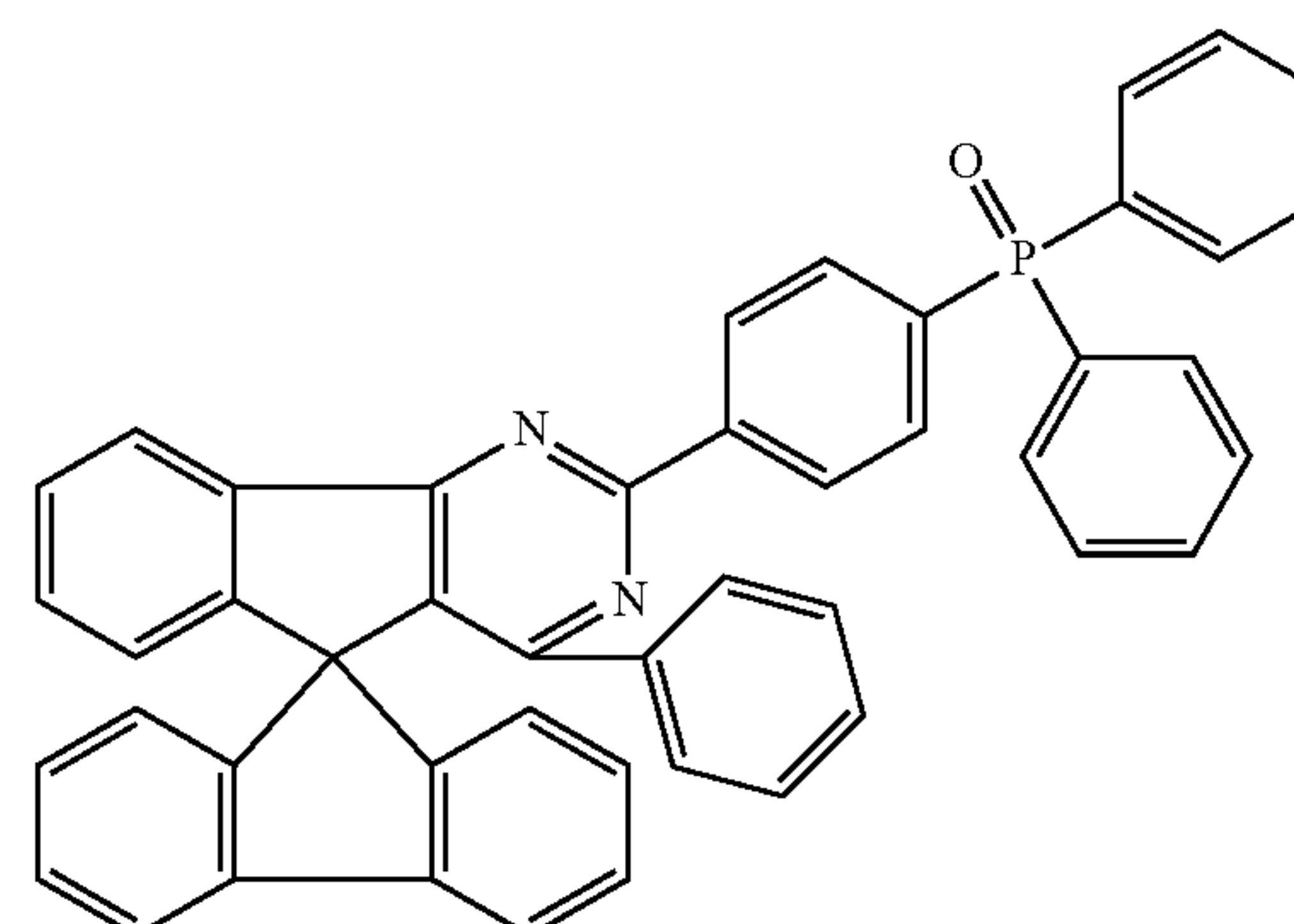
Chemical Formula 1-50
