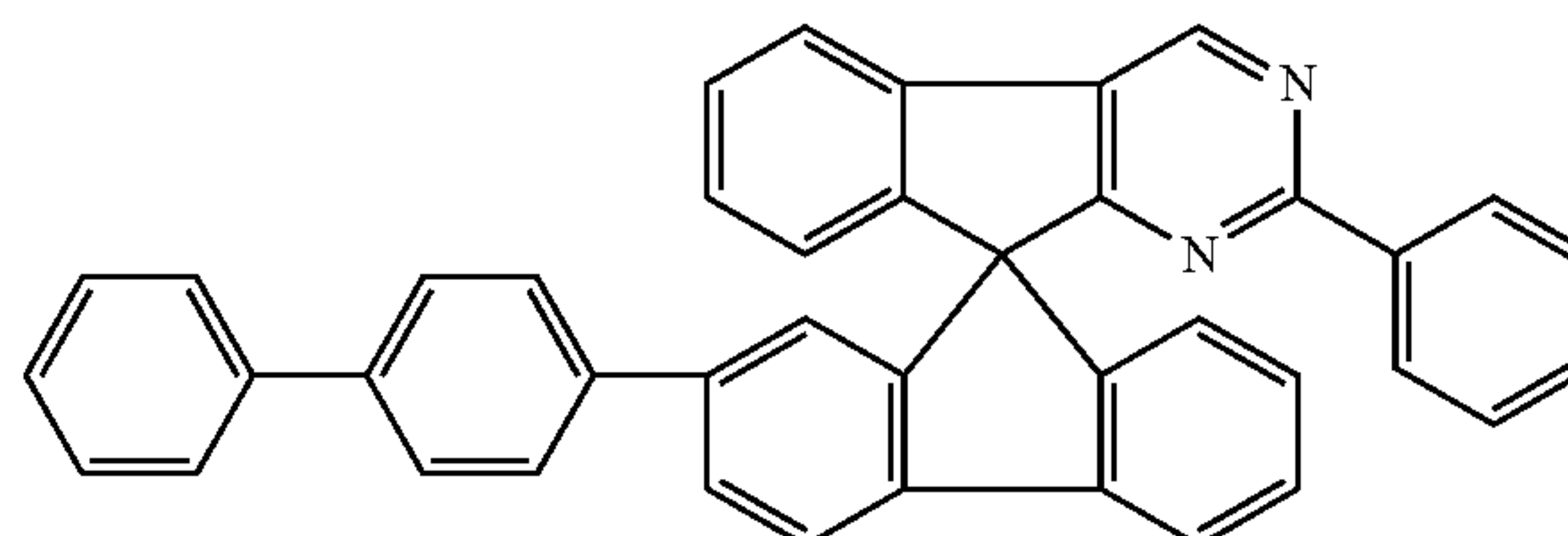
Chemical Formula 1-7
