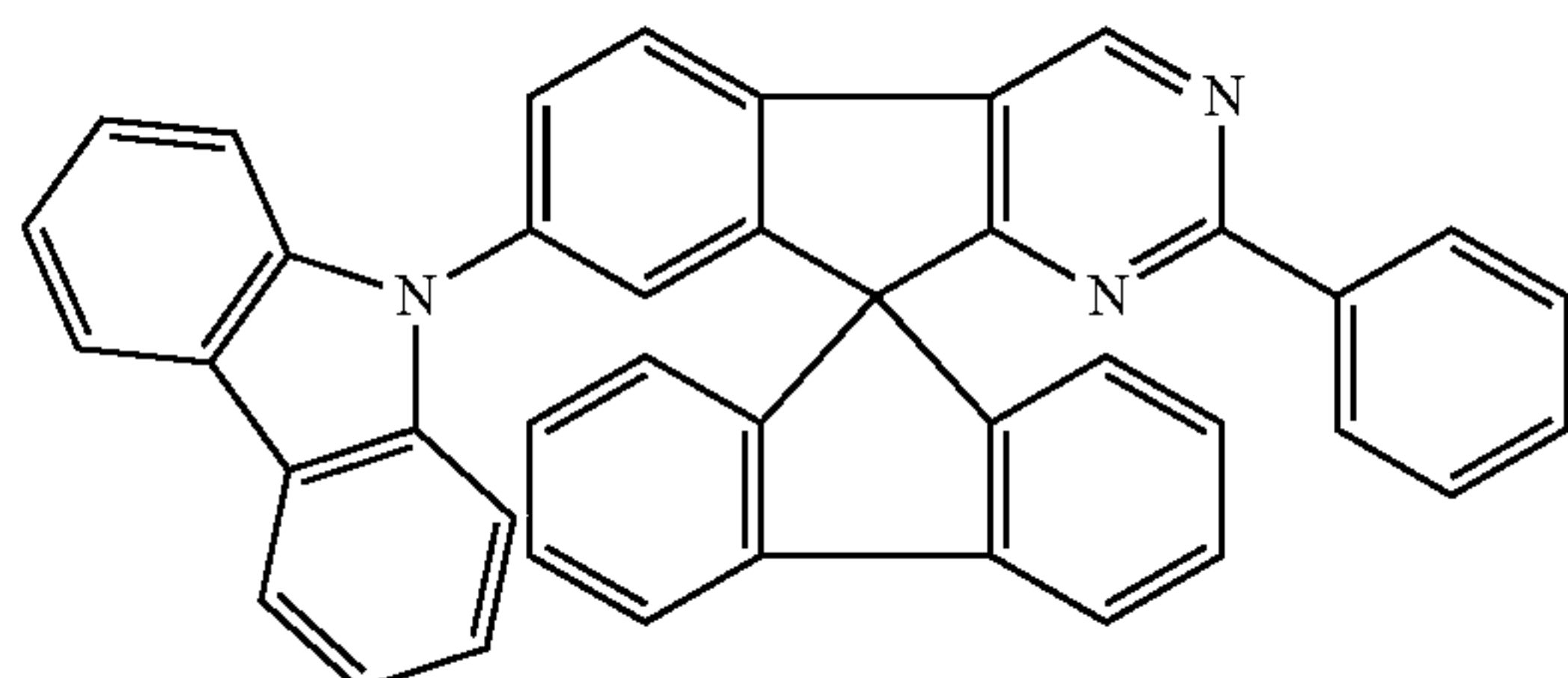
Chemical Formula 1-19
