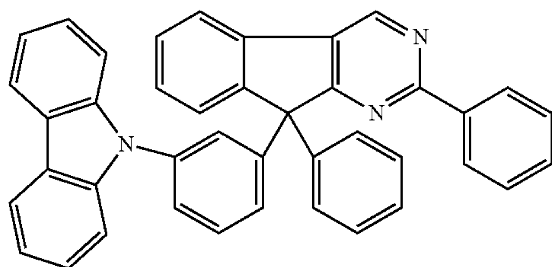
Chemical Formula 2-3
