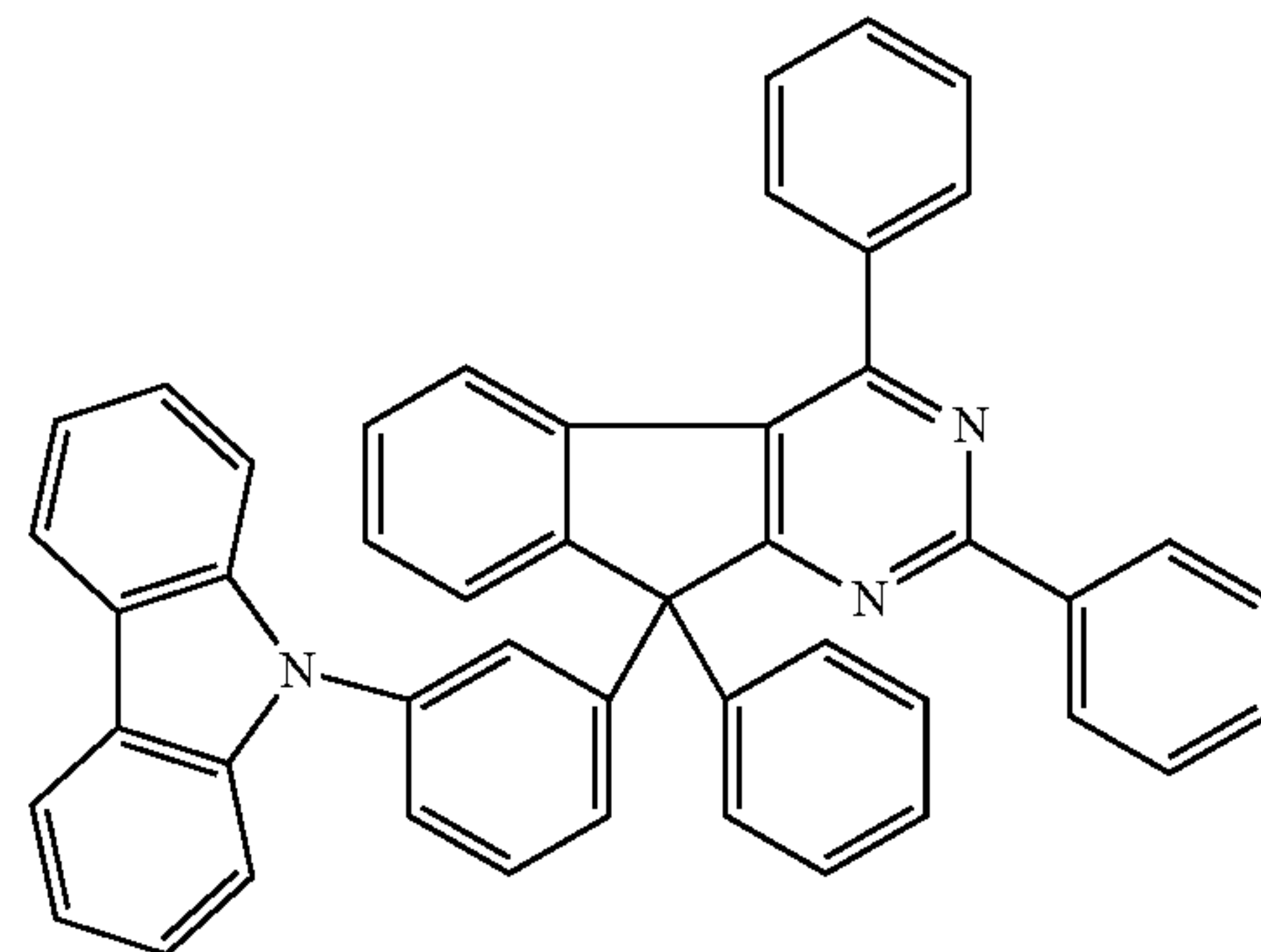
Chemical Formula 2-4
