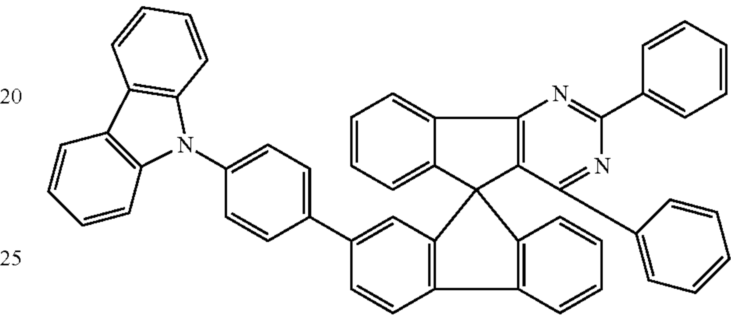
Chemical Formula 1-15
