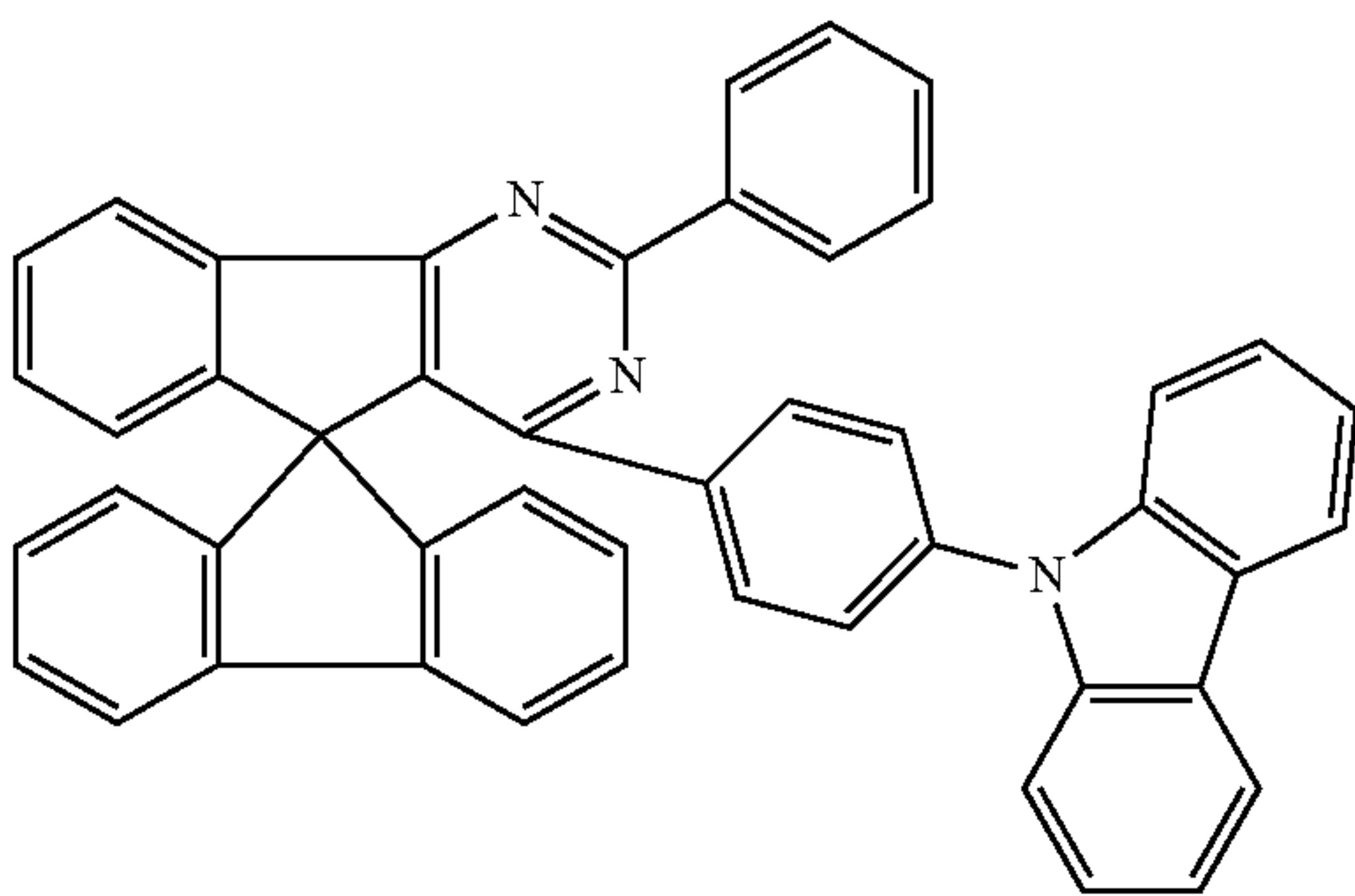
Chemical Formula 1-85
