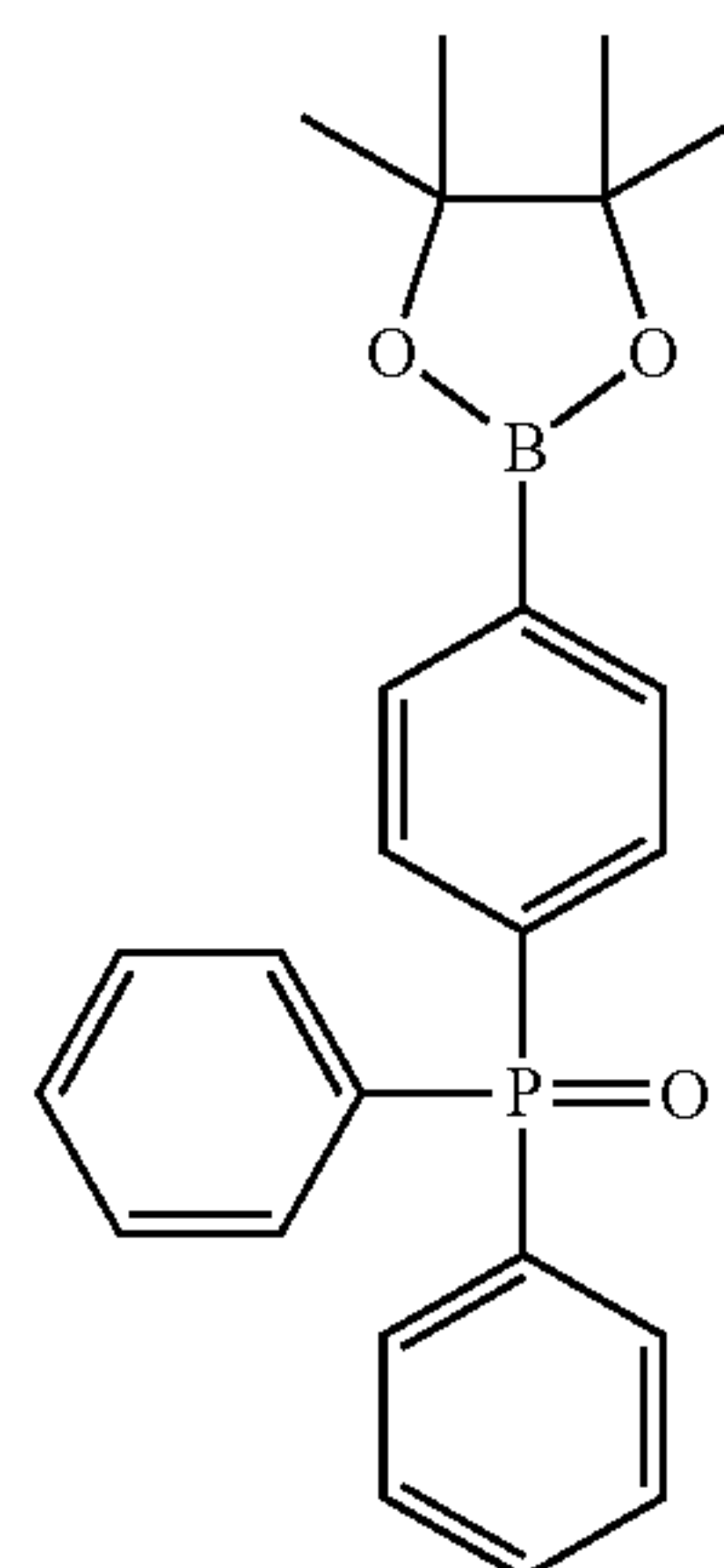
[Compound E-3]
