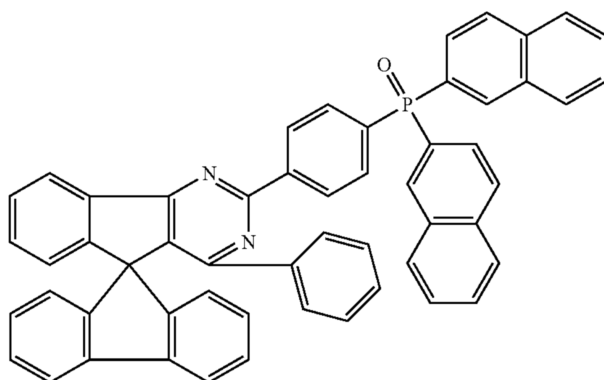
Chemical Formula 1-54
