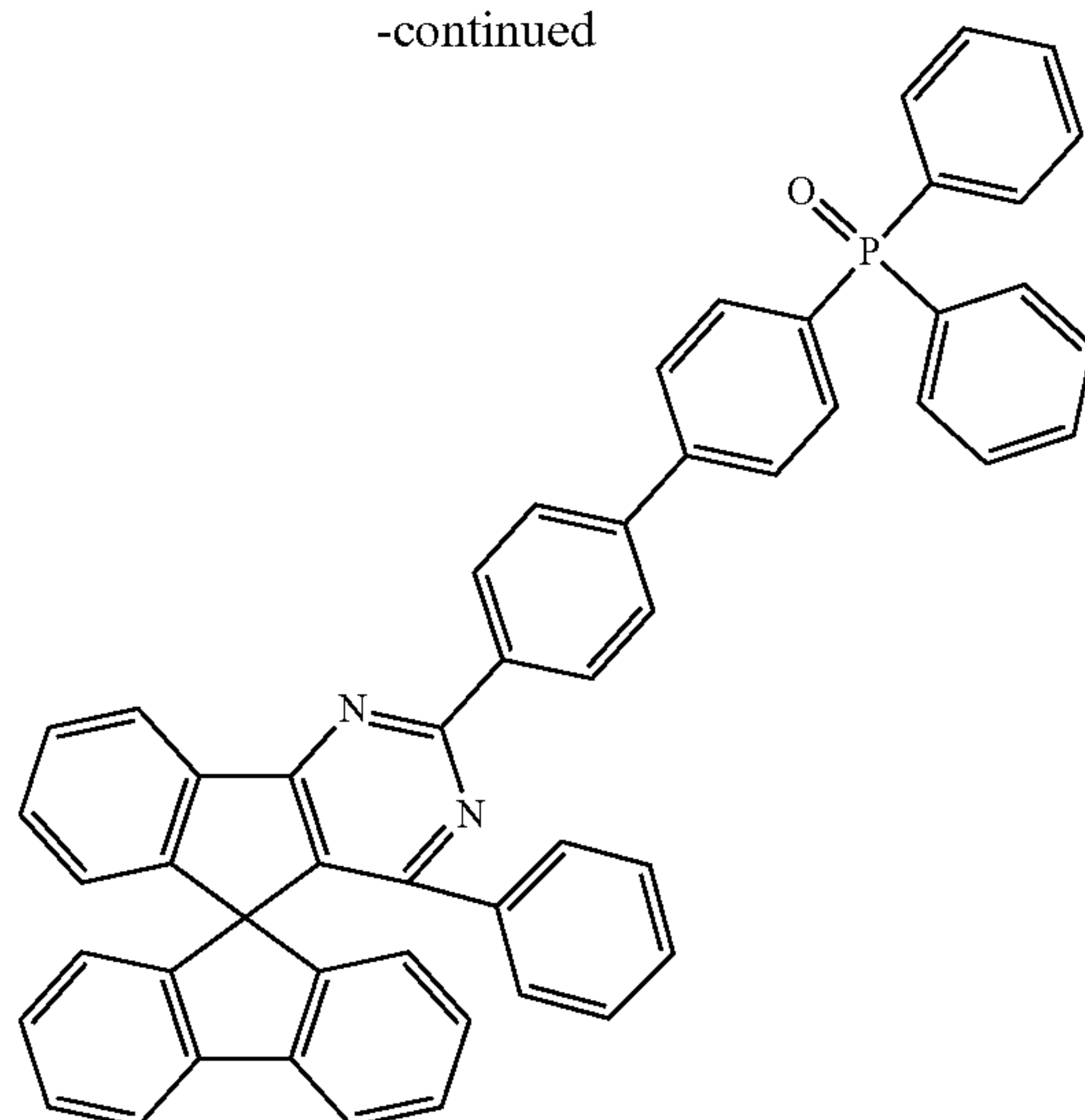
[Compound Formula 1-55]
