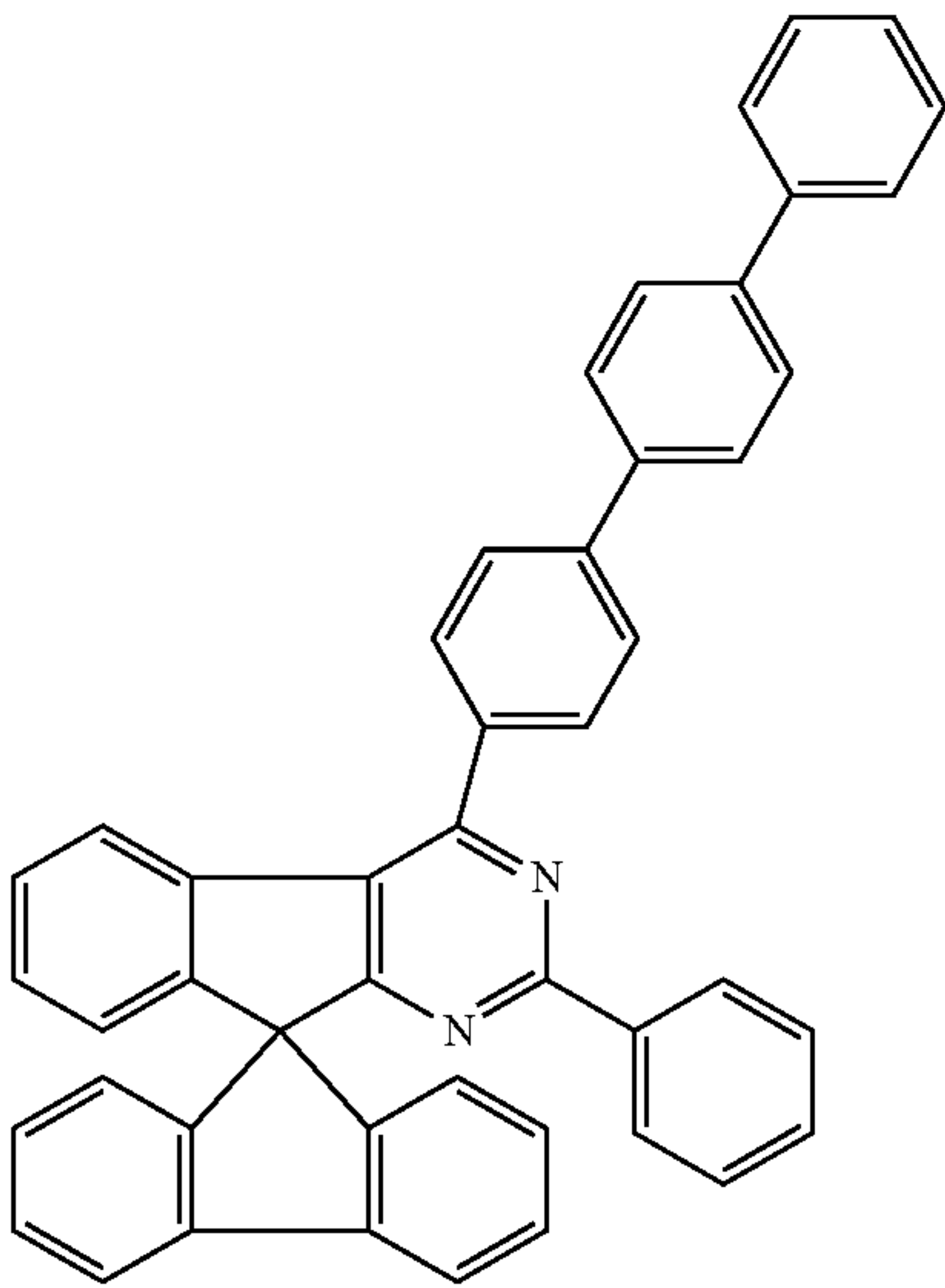
Chemical Formula 1-82
