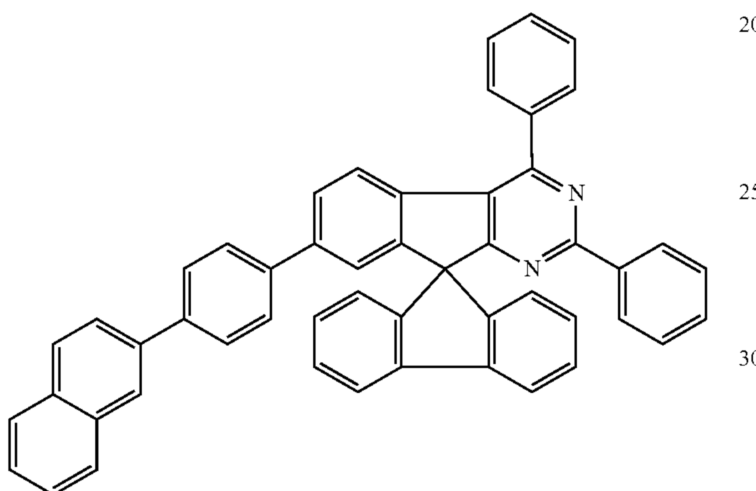
Chemical Formula 1-28
