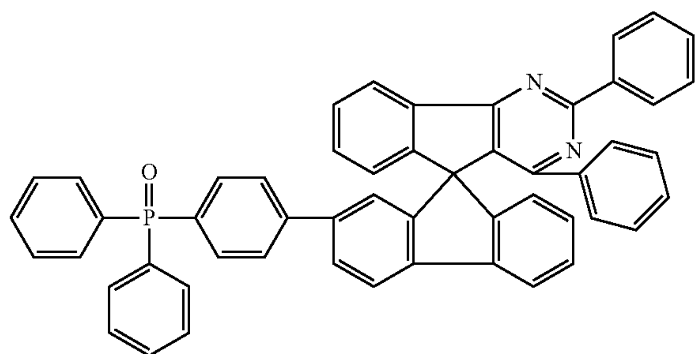
Chemical Formula 1-45
