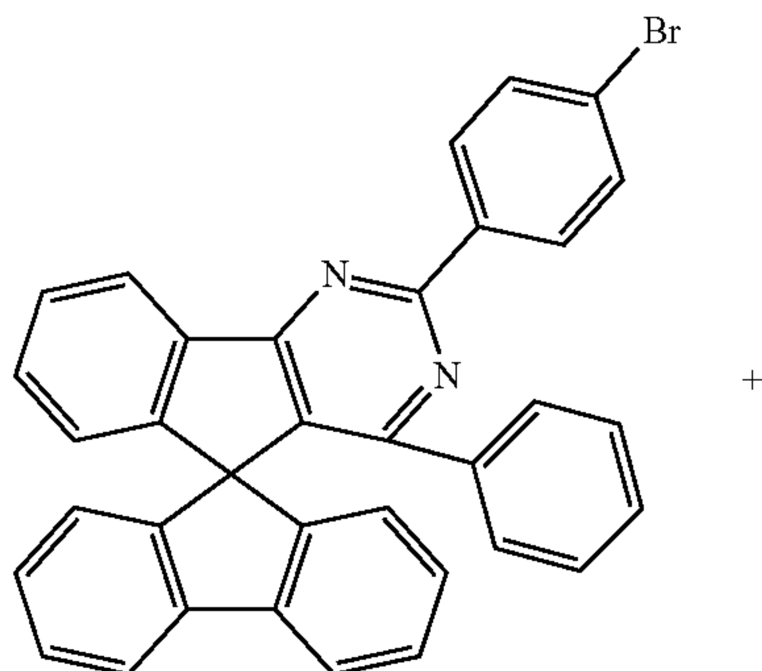
[Compound E-2]
