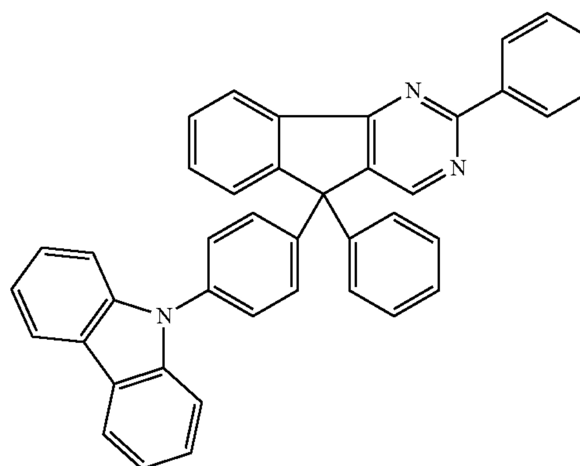
Chemical Formula 2-6
