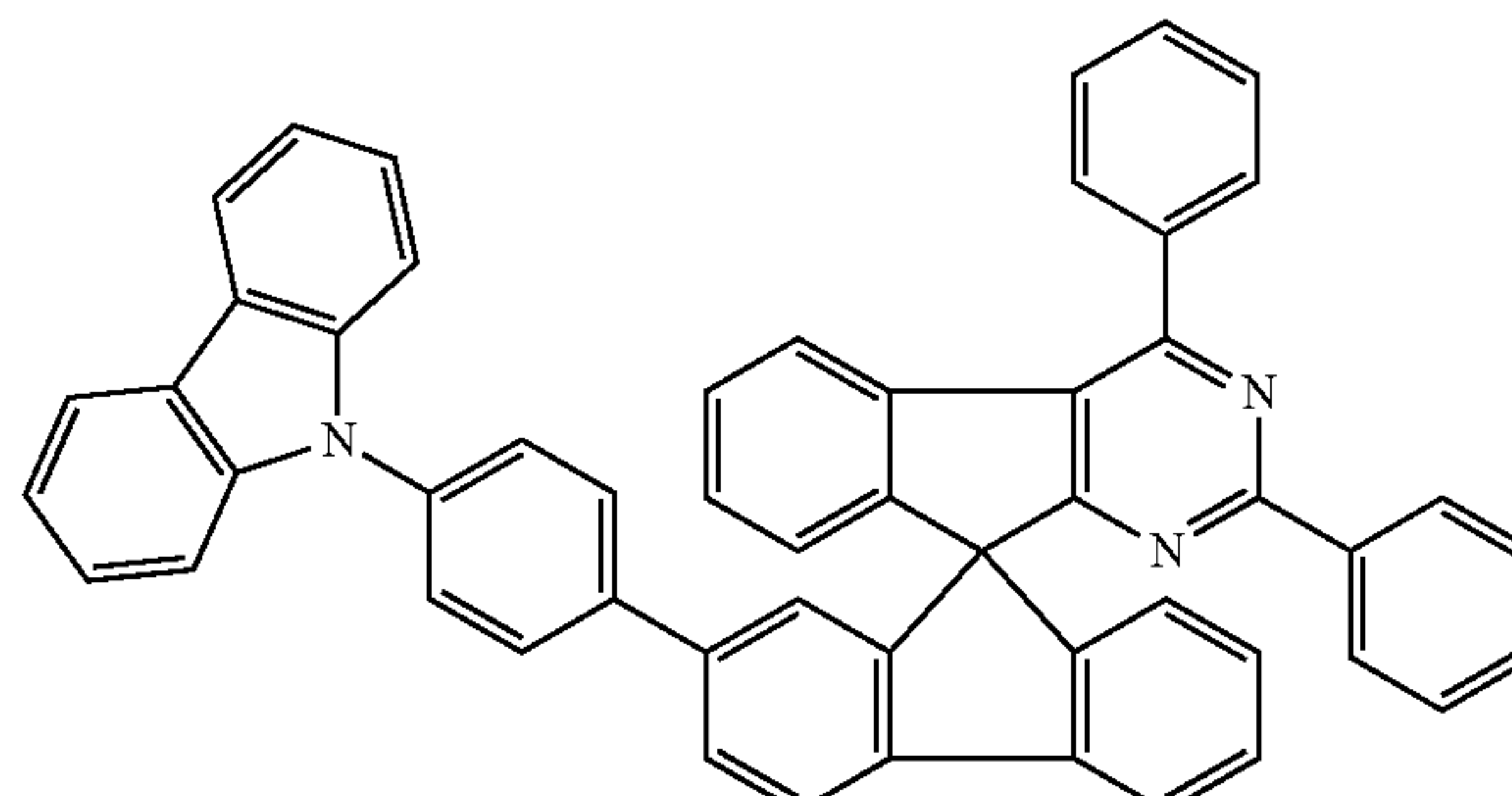
Chemical Formula 1-16
