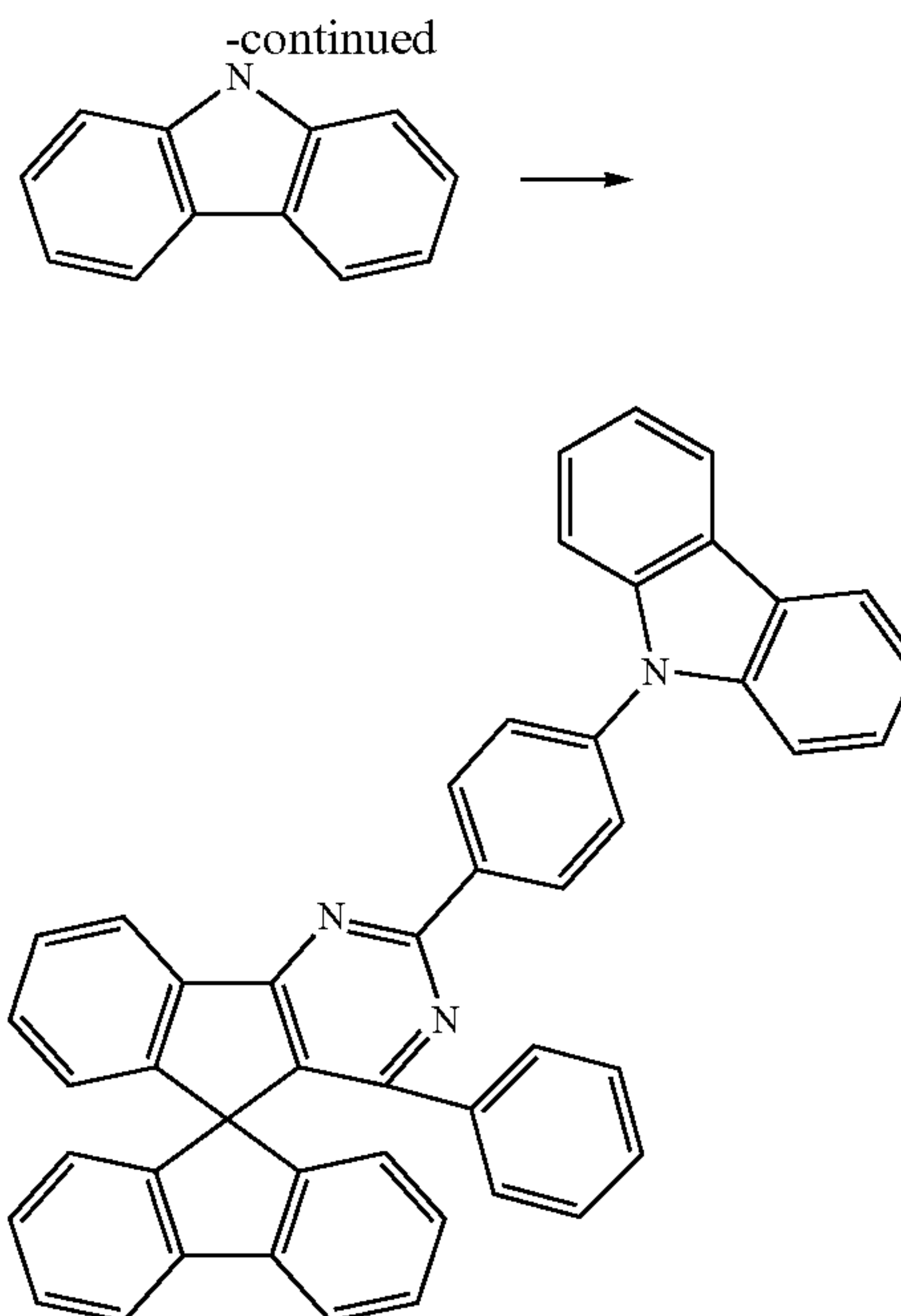
[Chemical Formula 1-67]
