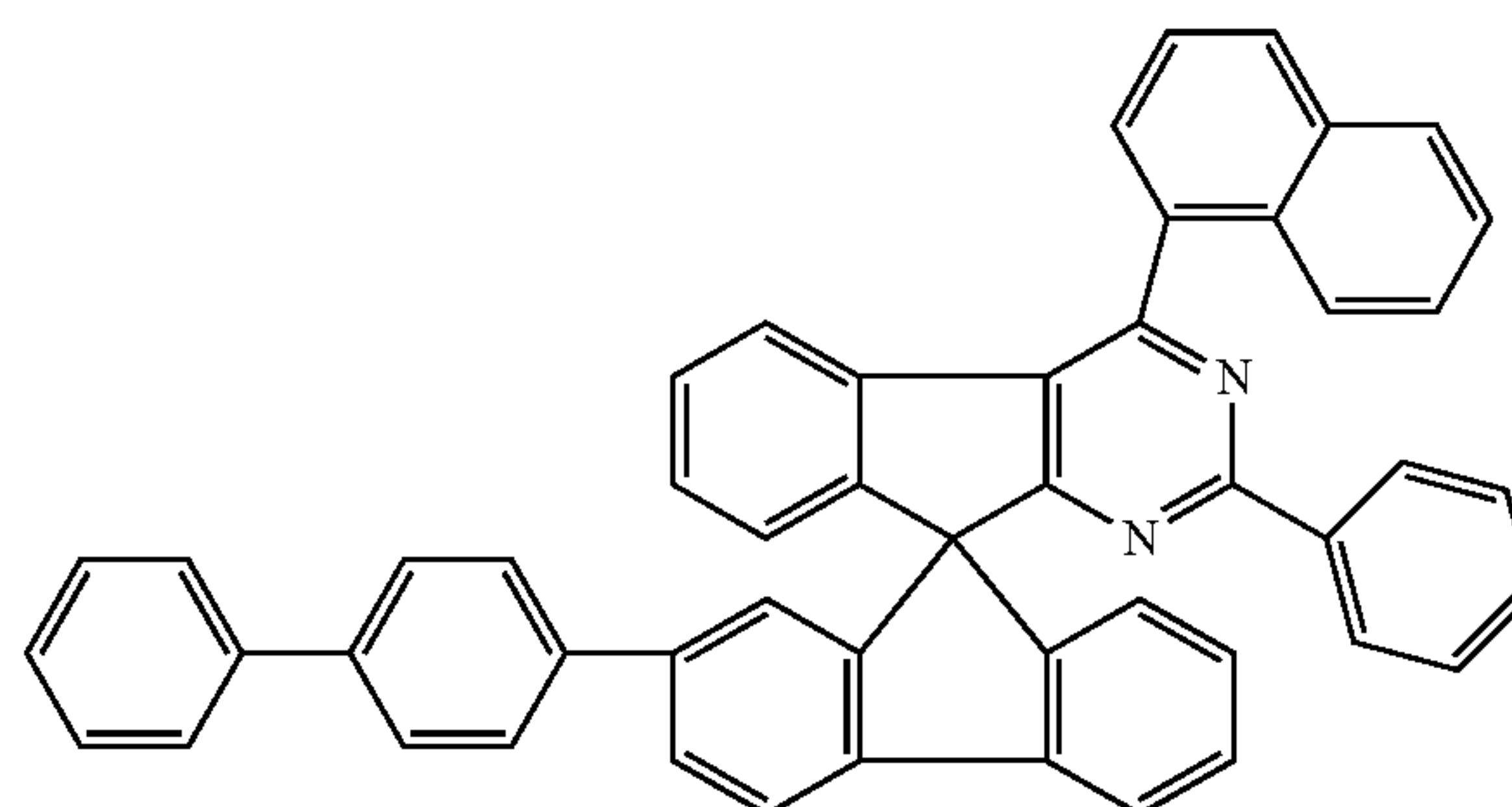
Chemical Formula 1-32
