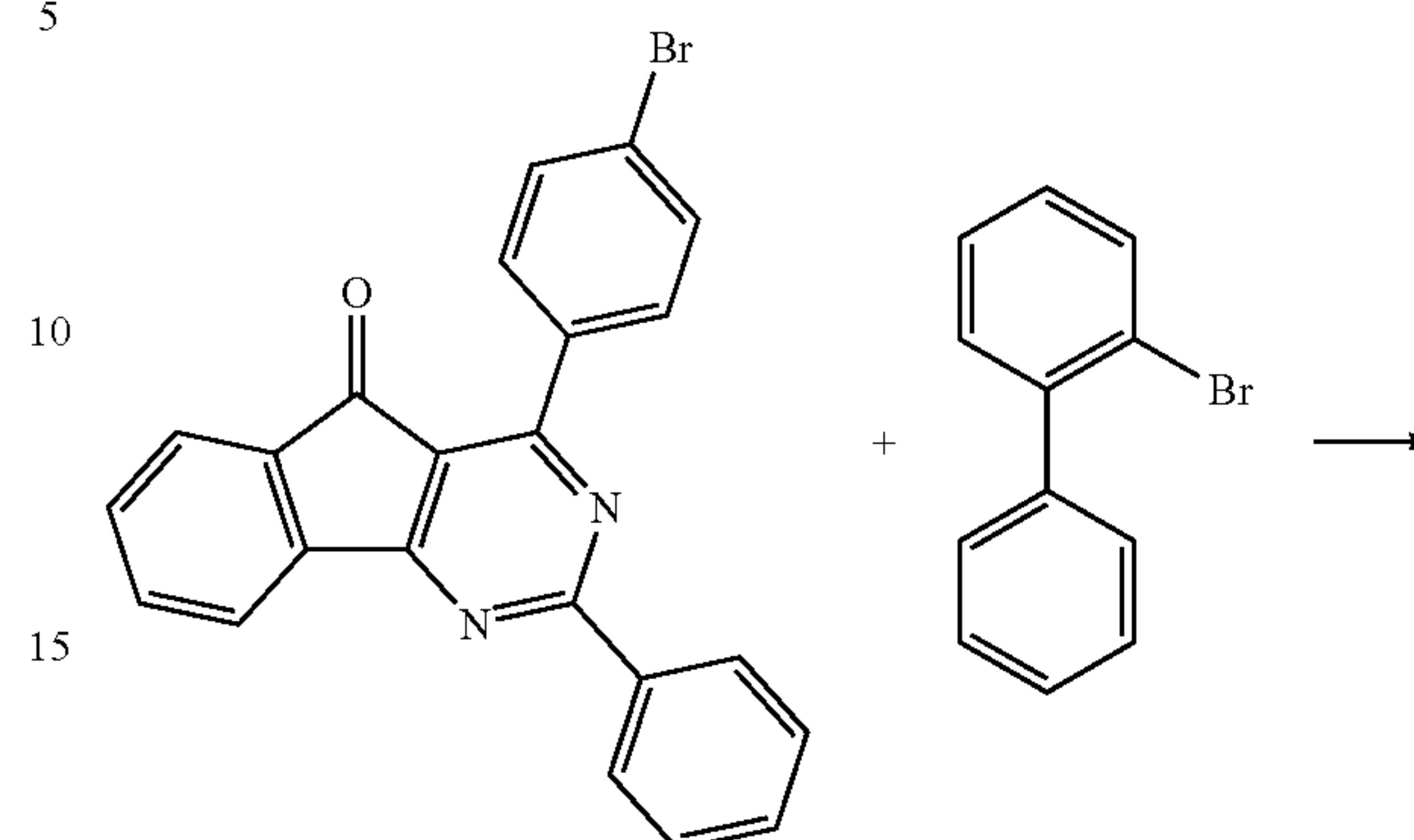
[Compound F]
