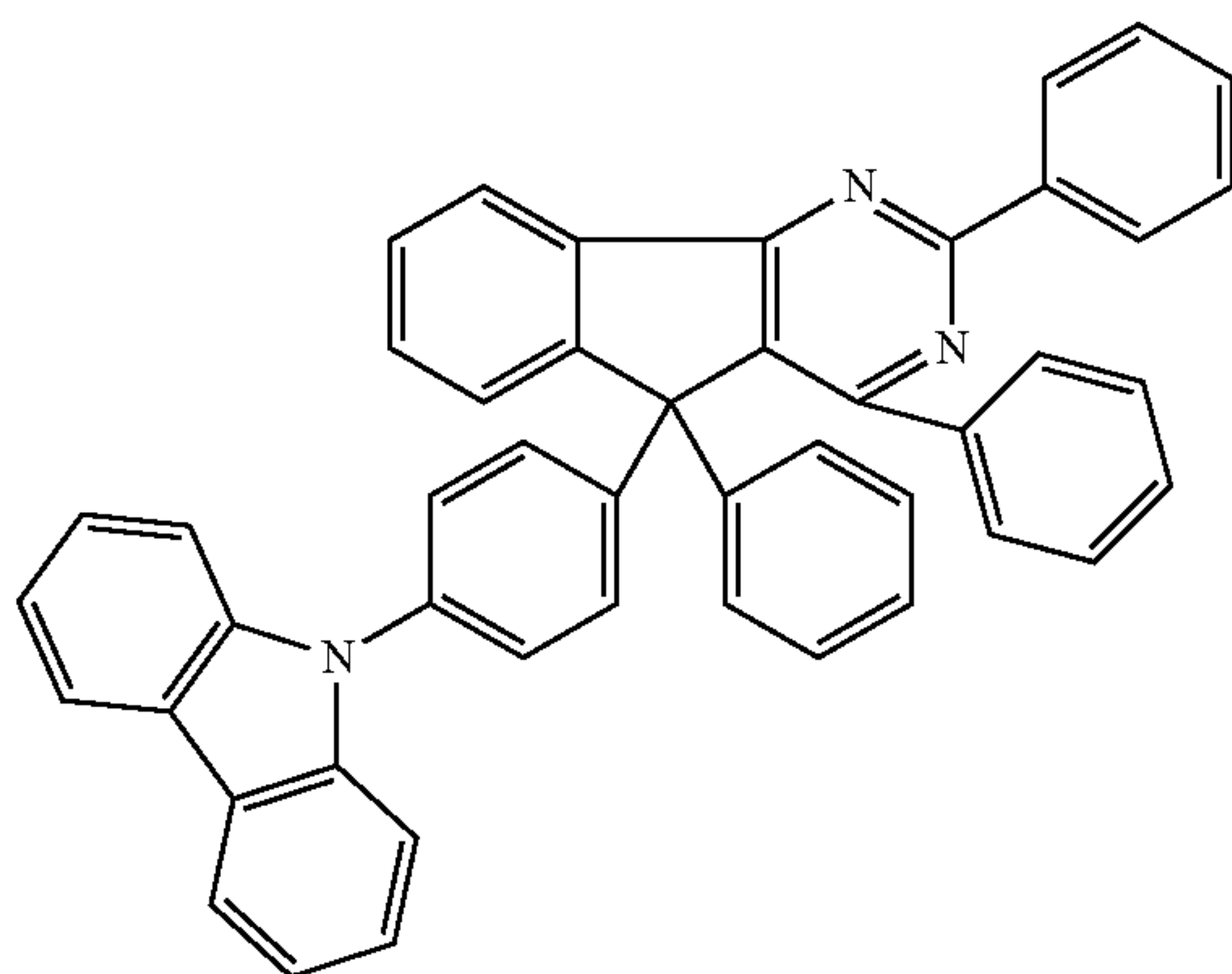
Chemical Formula 2-10
