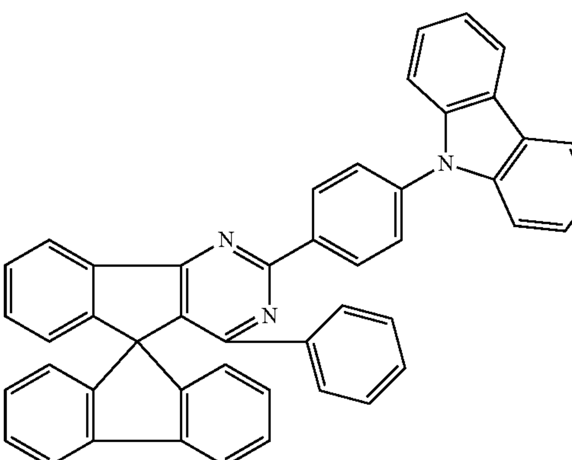
Chemical Formula 1-67
