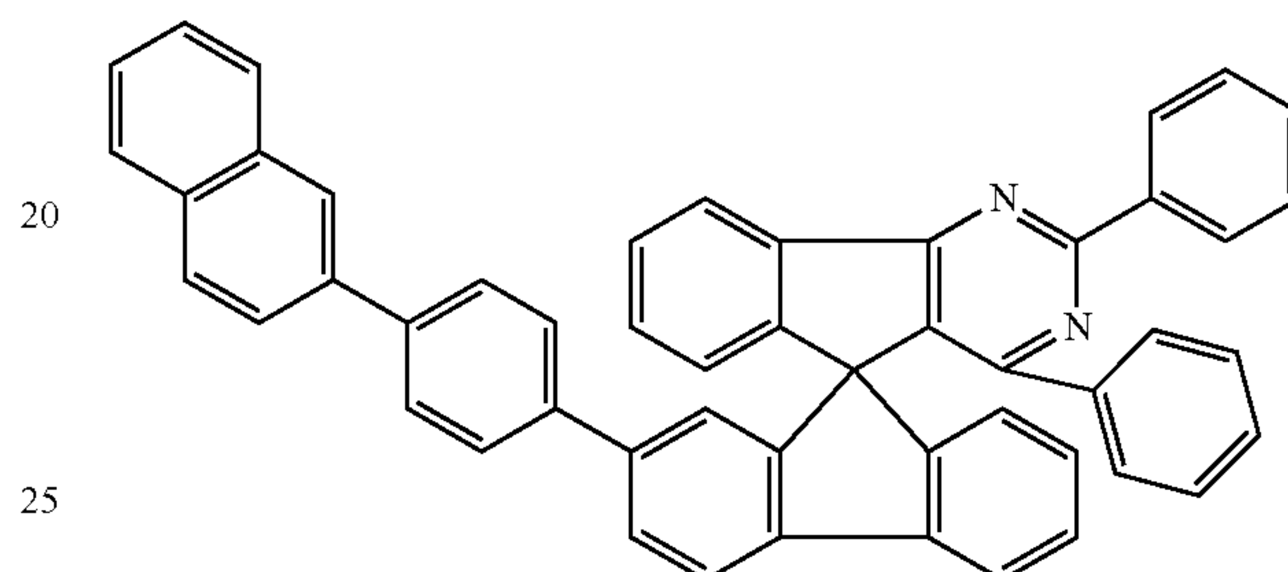
Chemical Formula 1-24
