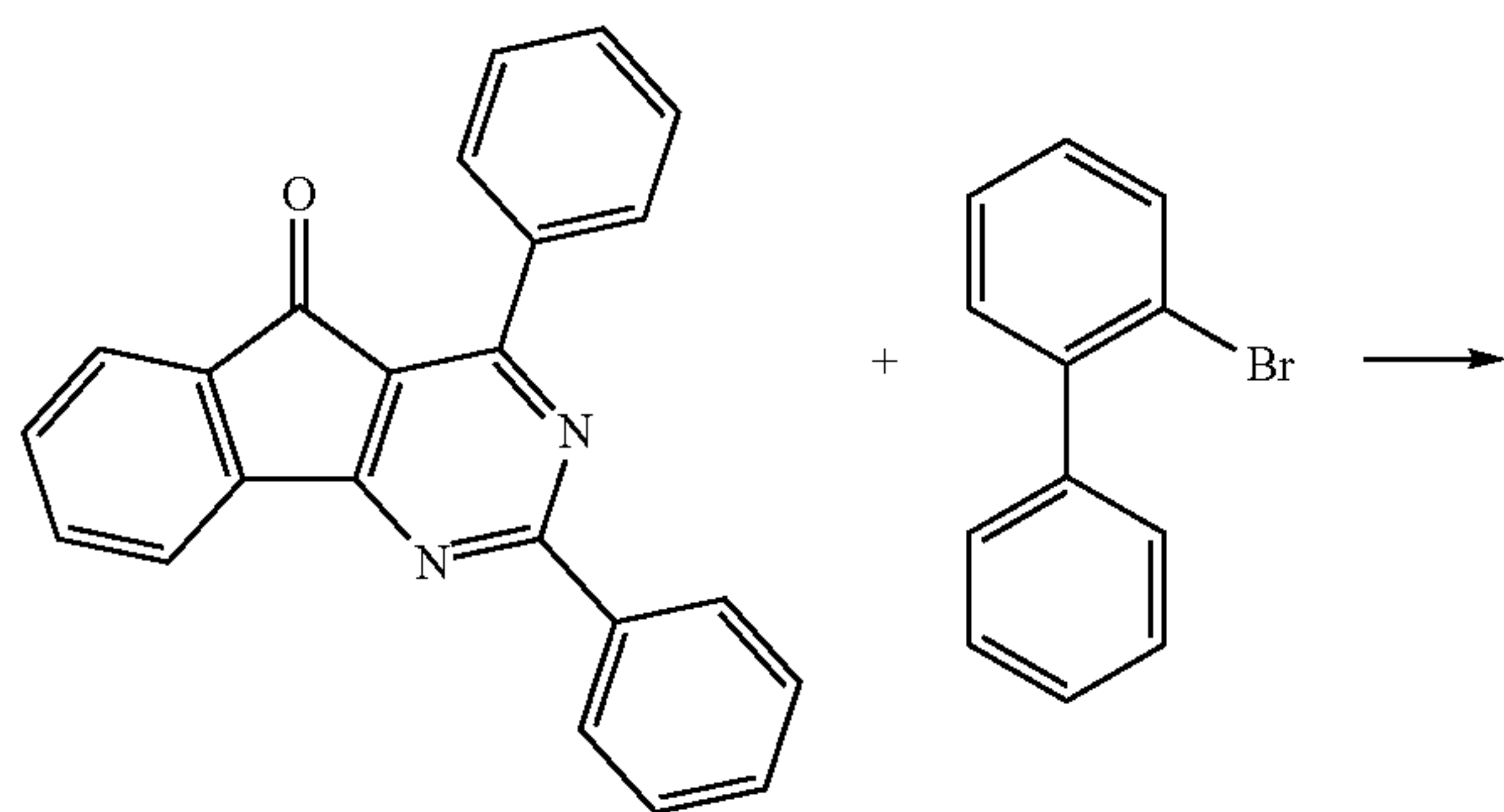
[Compound C]
