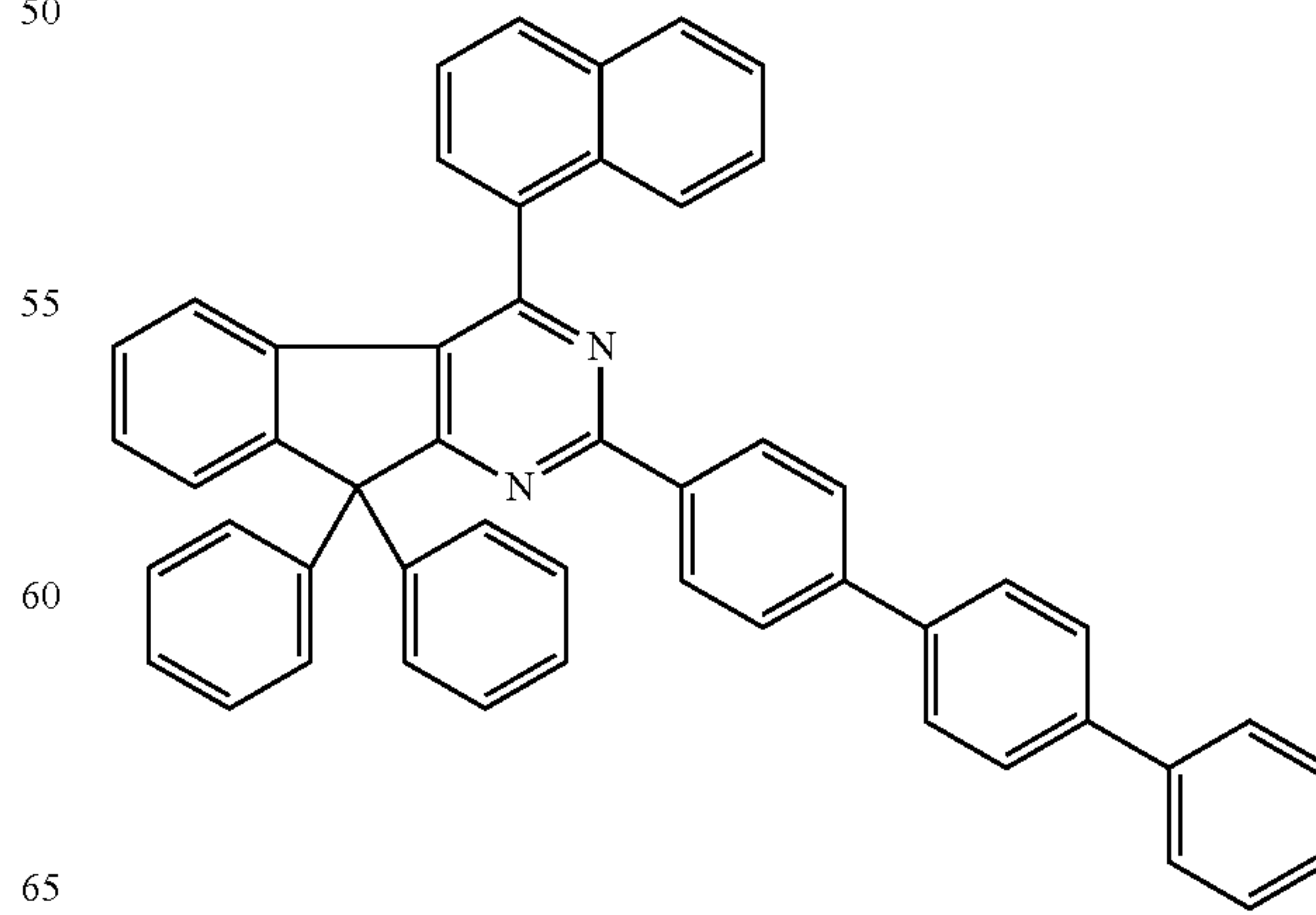
Chemical Formula 2-25
