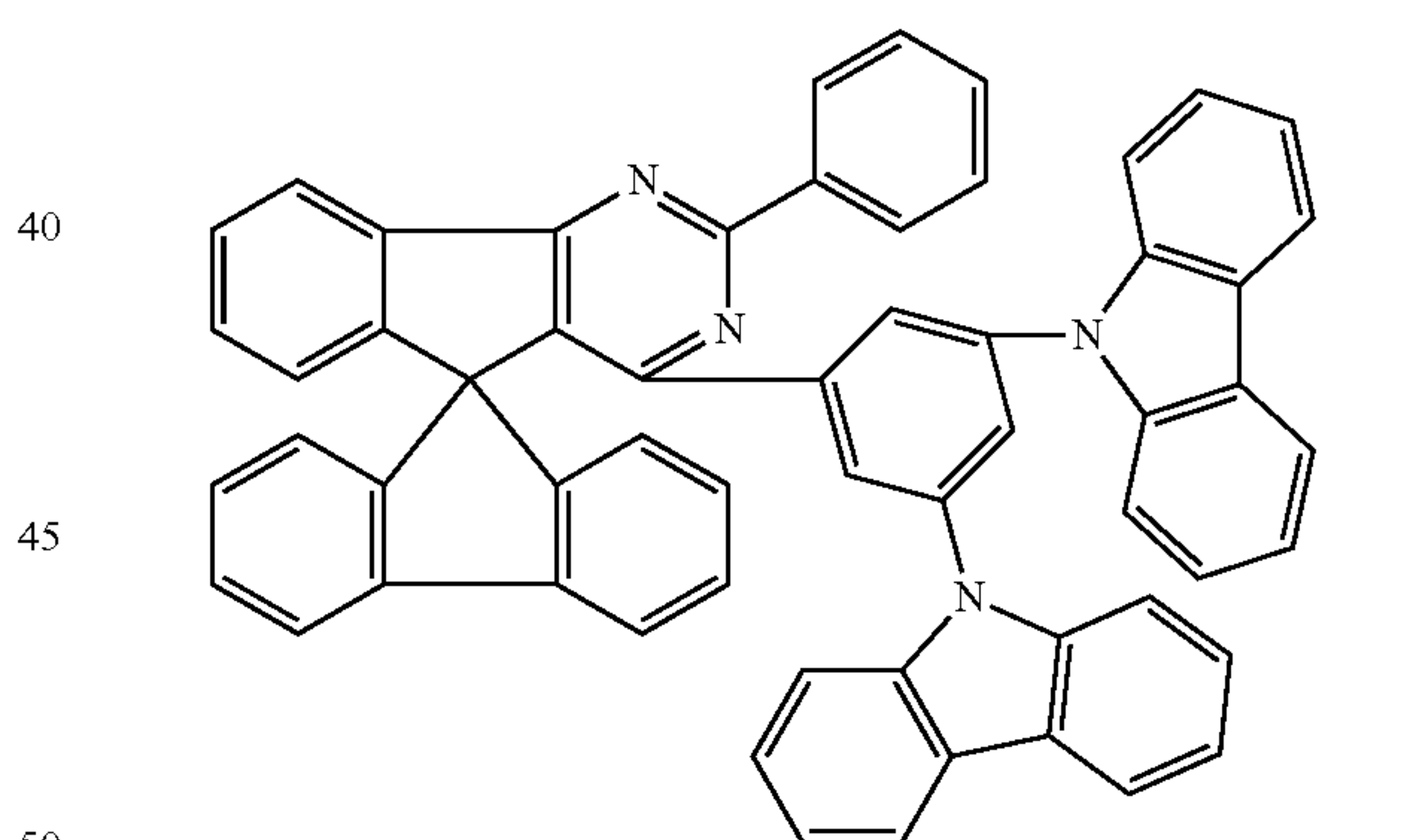
Chemical Formula 1-72
