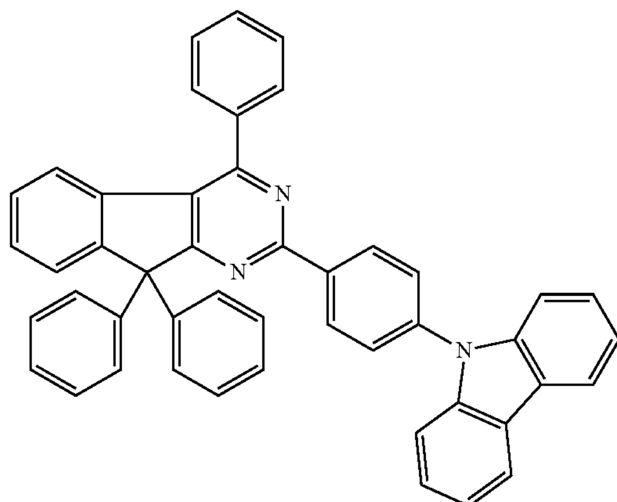
Chemical Formula 2-30
