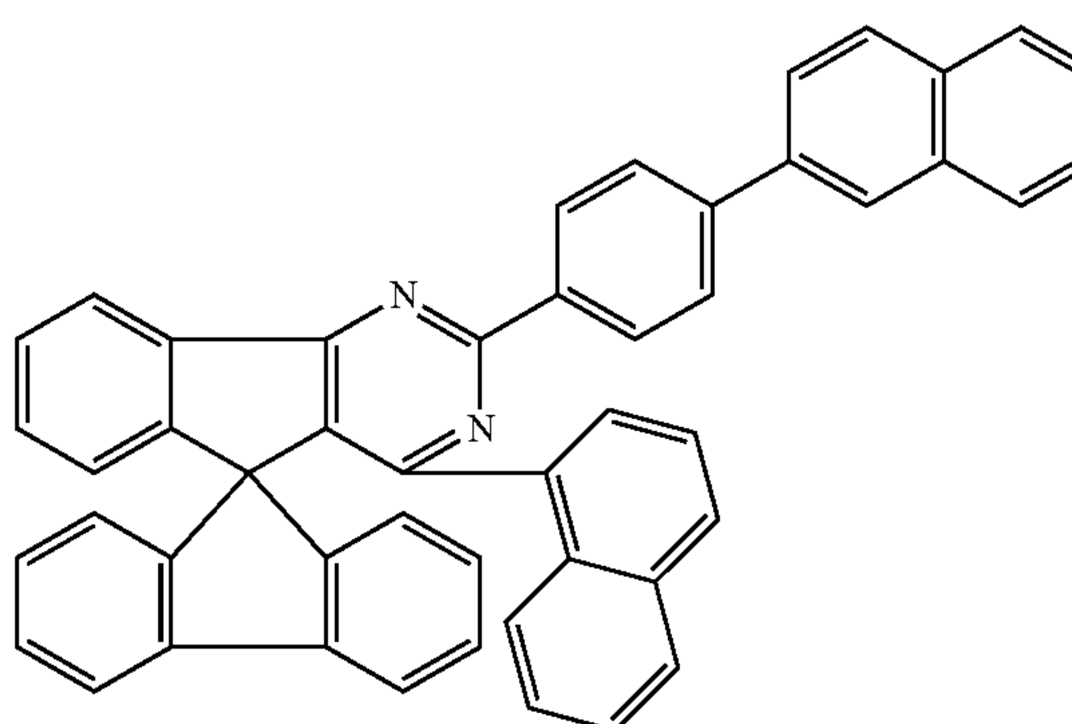
Chemical Formula 1-66
