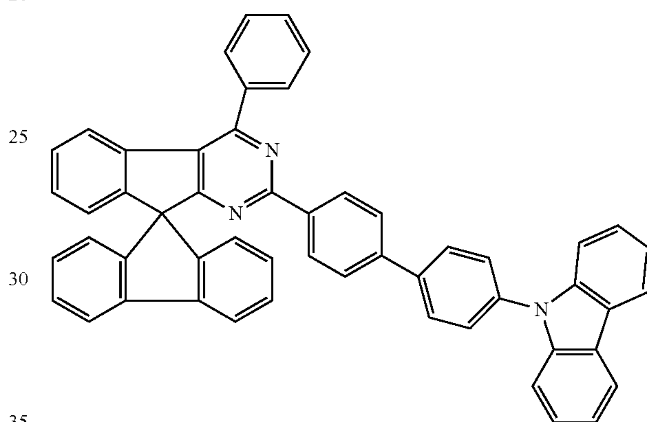
Chemical Formula 1-71
