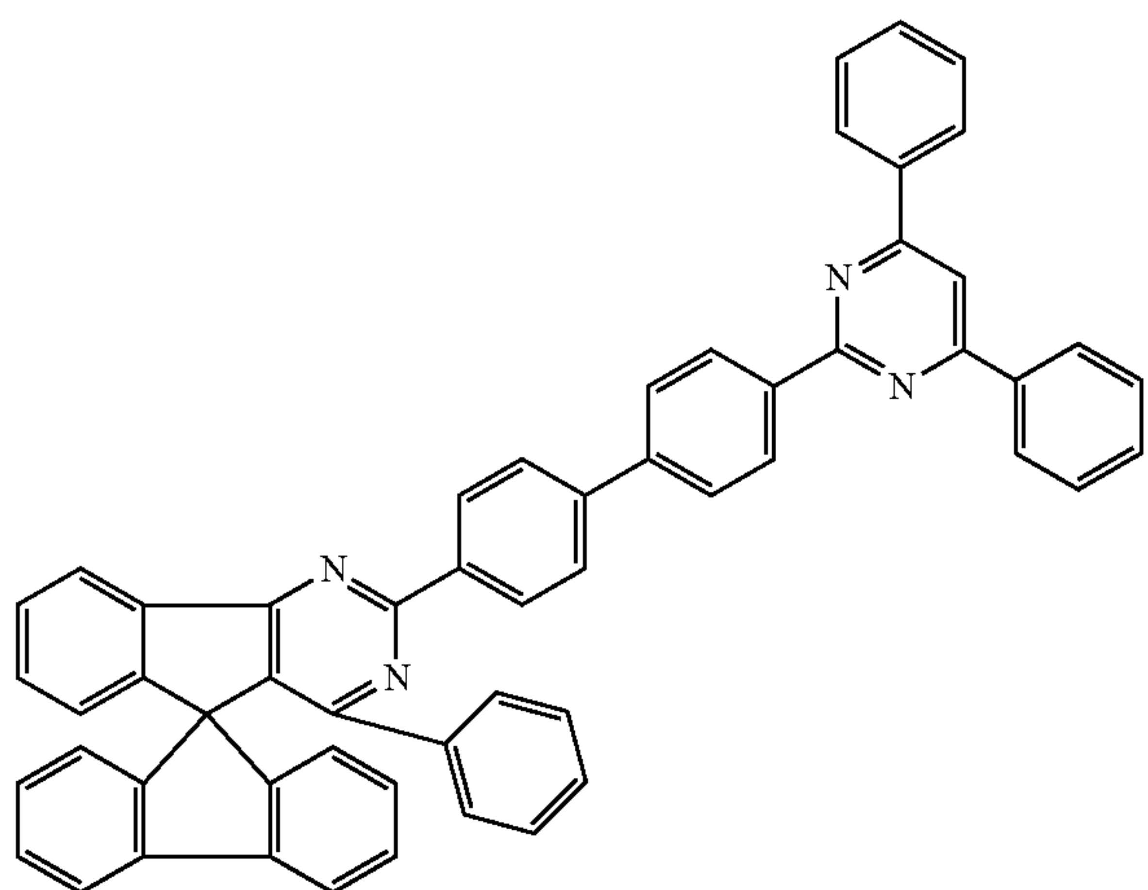
Chemical Formula 1-100
