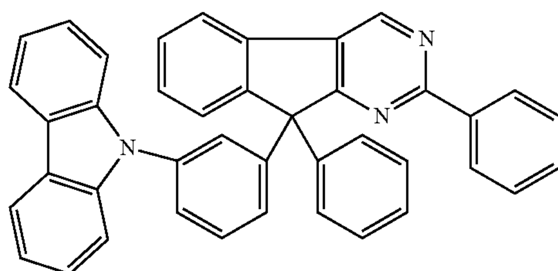
Chemical Formula 2-2
