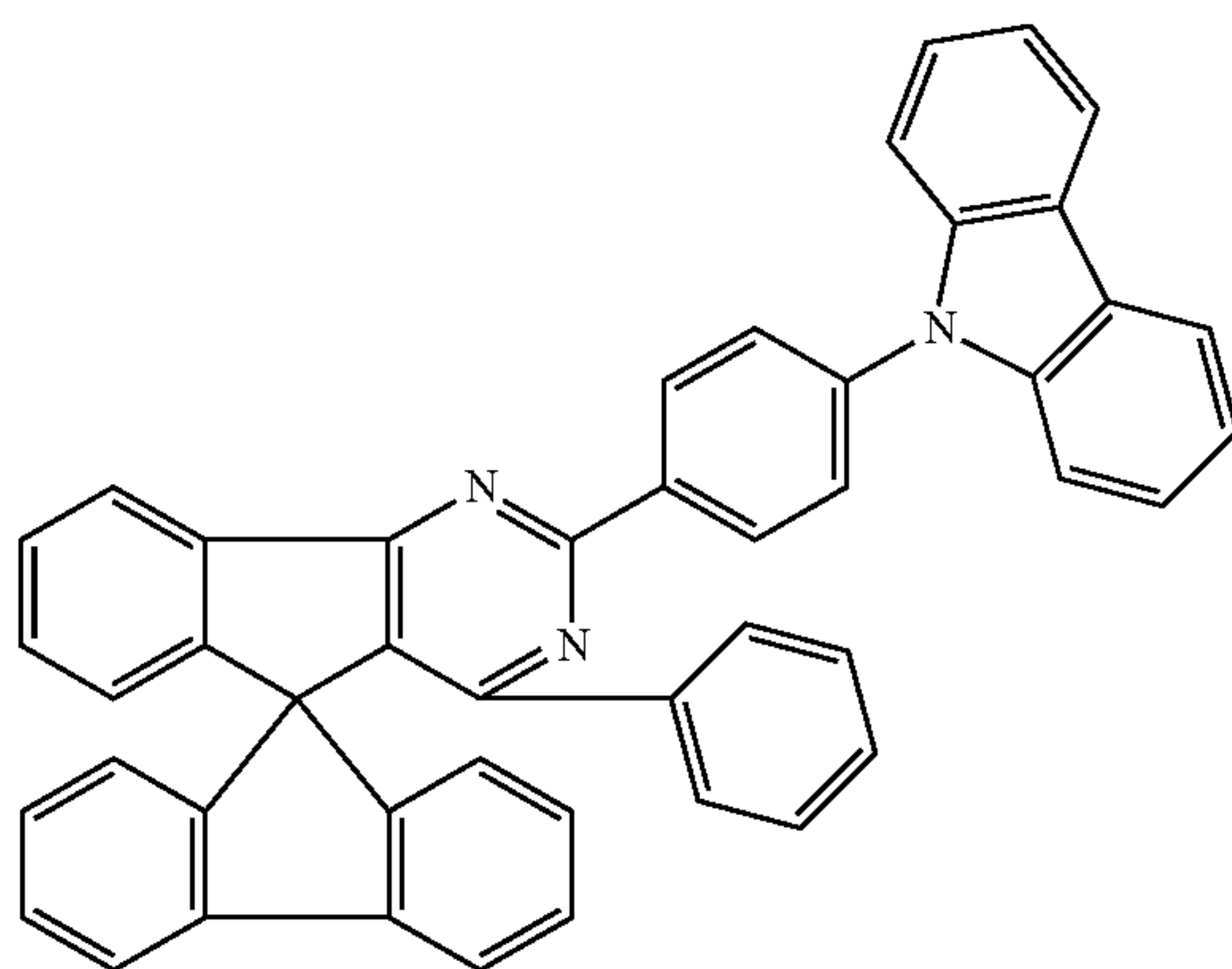
Chemical Formula 1-67
