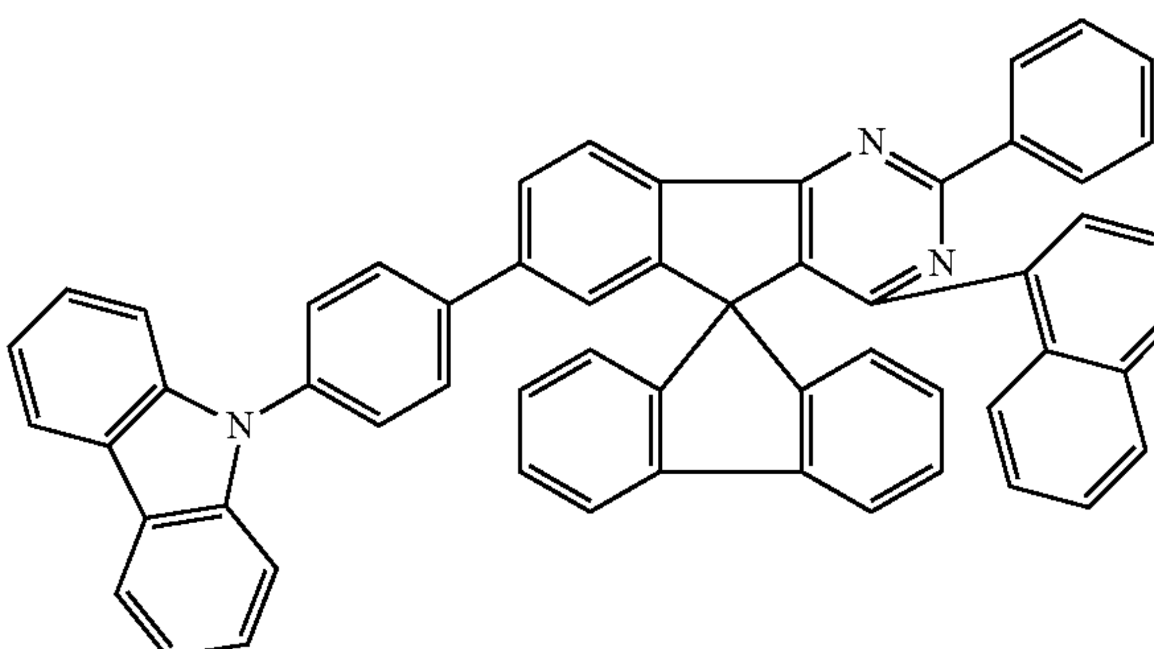
Chemical Formula 1-35
