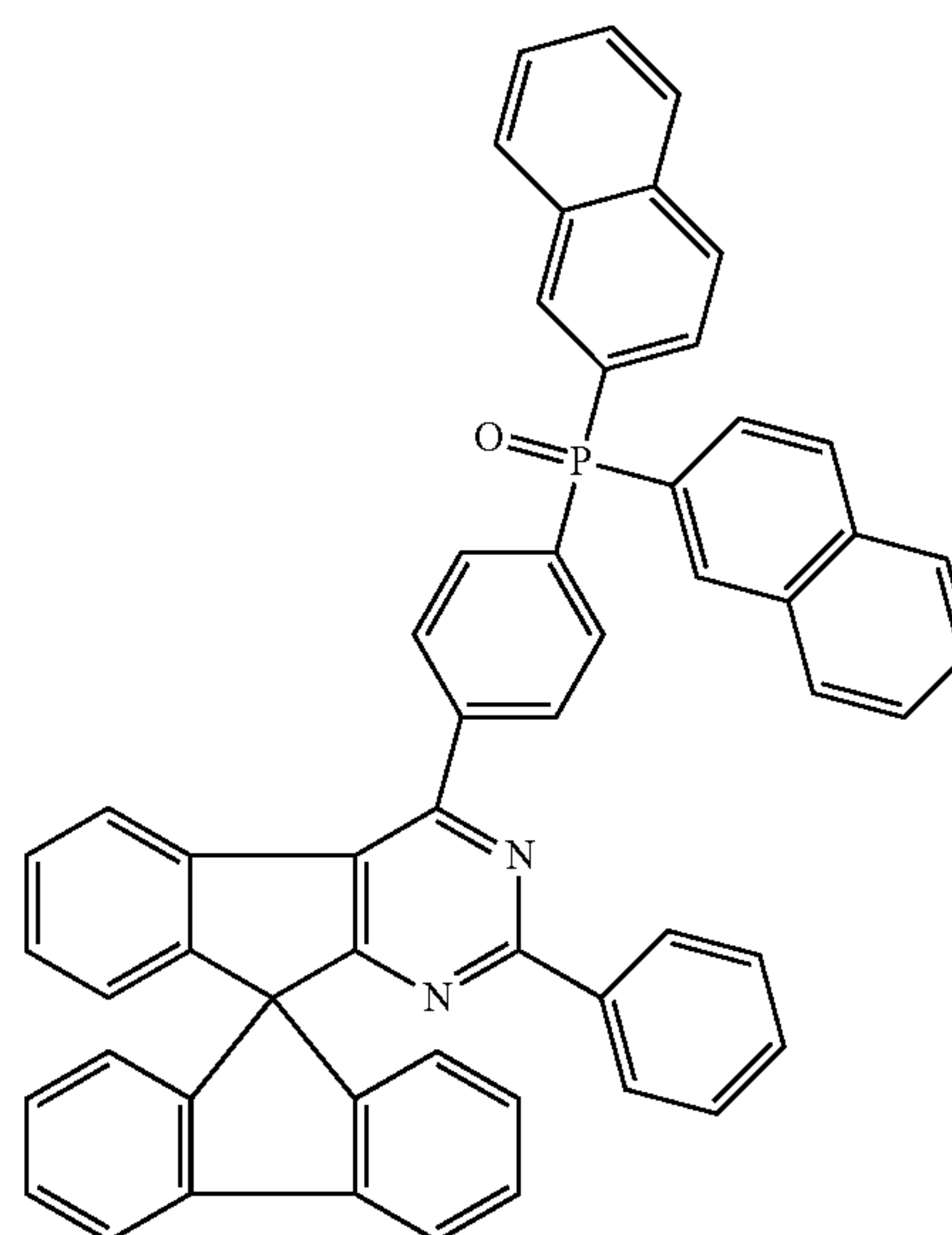
Chemical Formula 1-78
