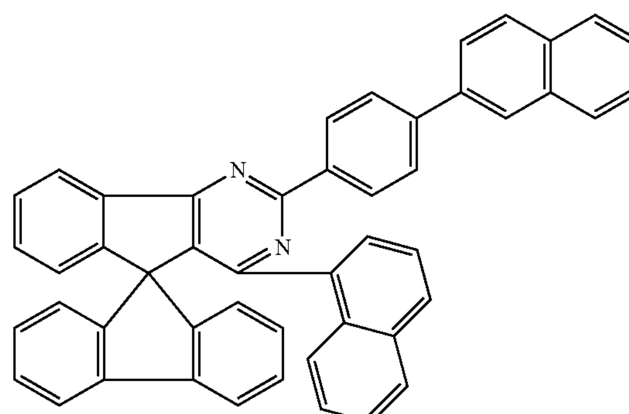
Chemical Formula 1-65
