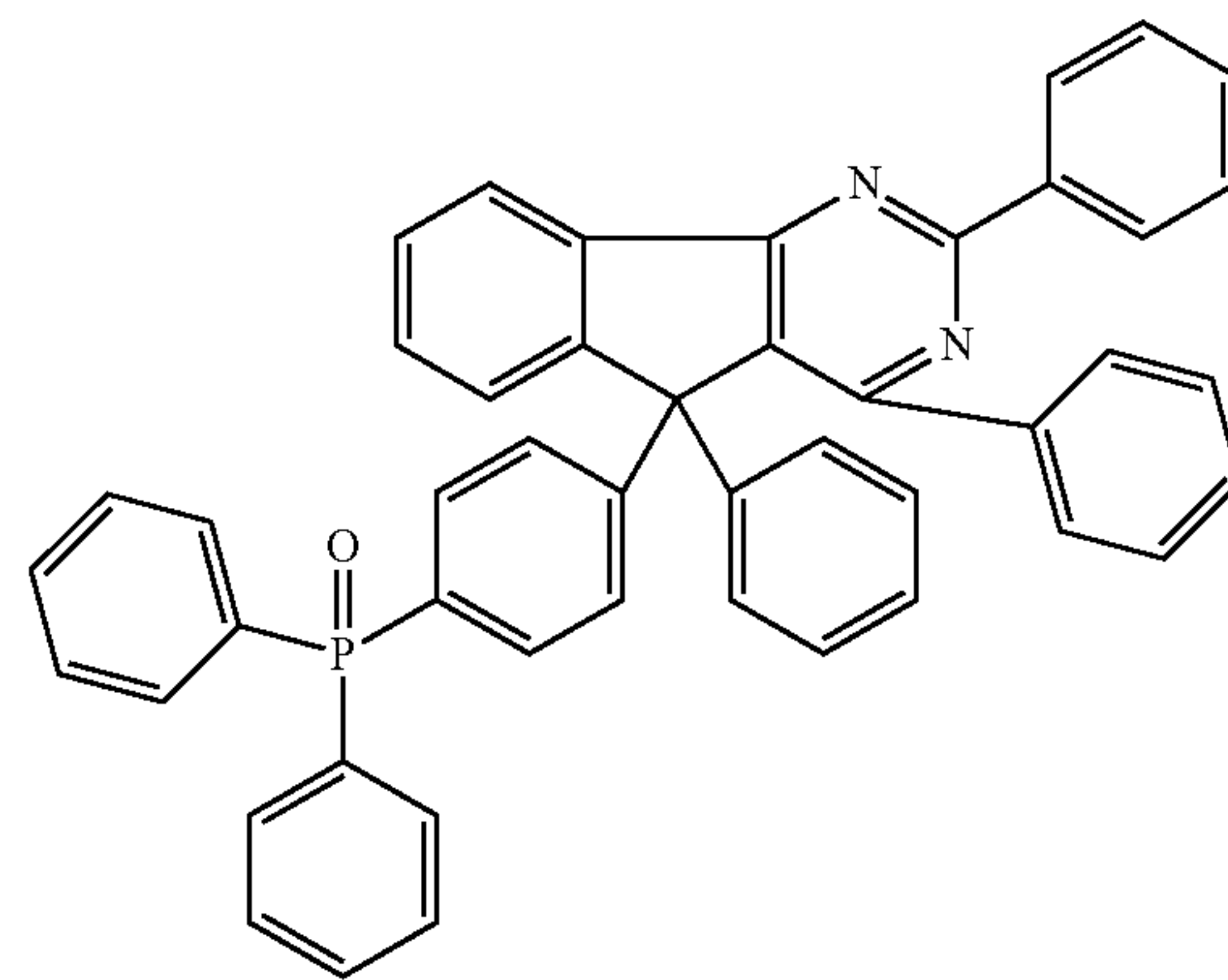
Chemical Formula 2-15
