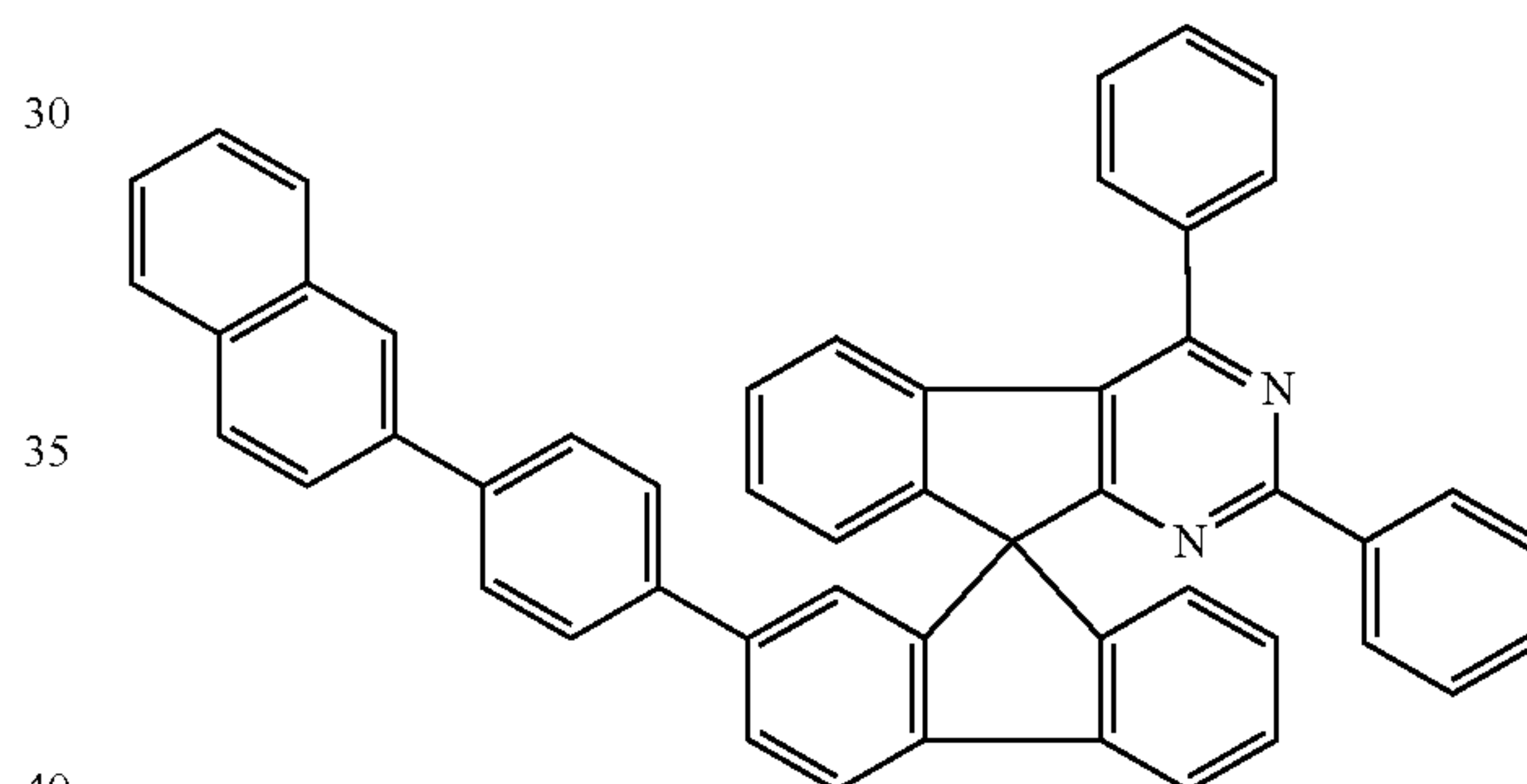
Chemical Formula 1-25
