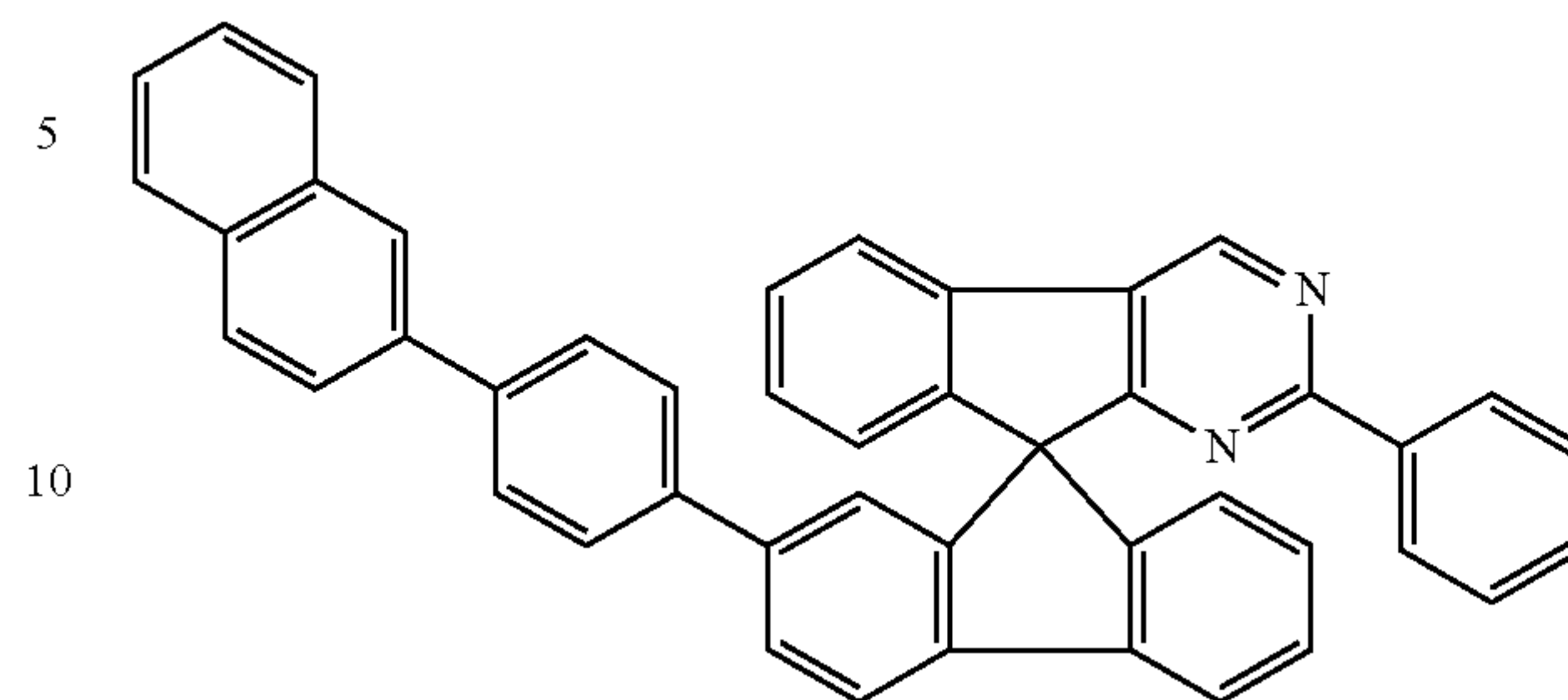
Chemical Formula 1-22
