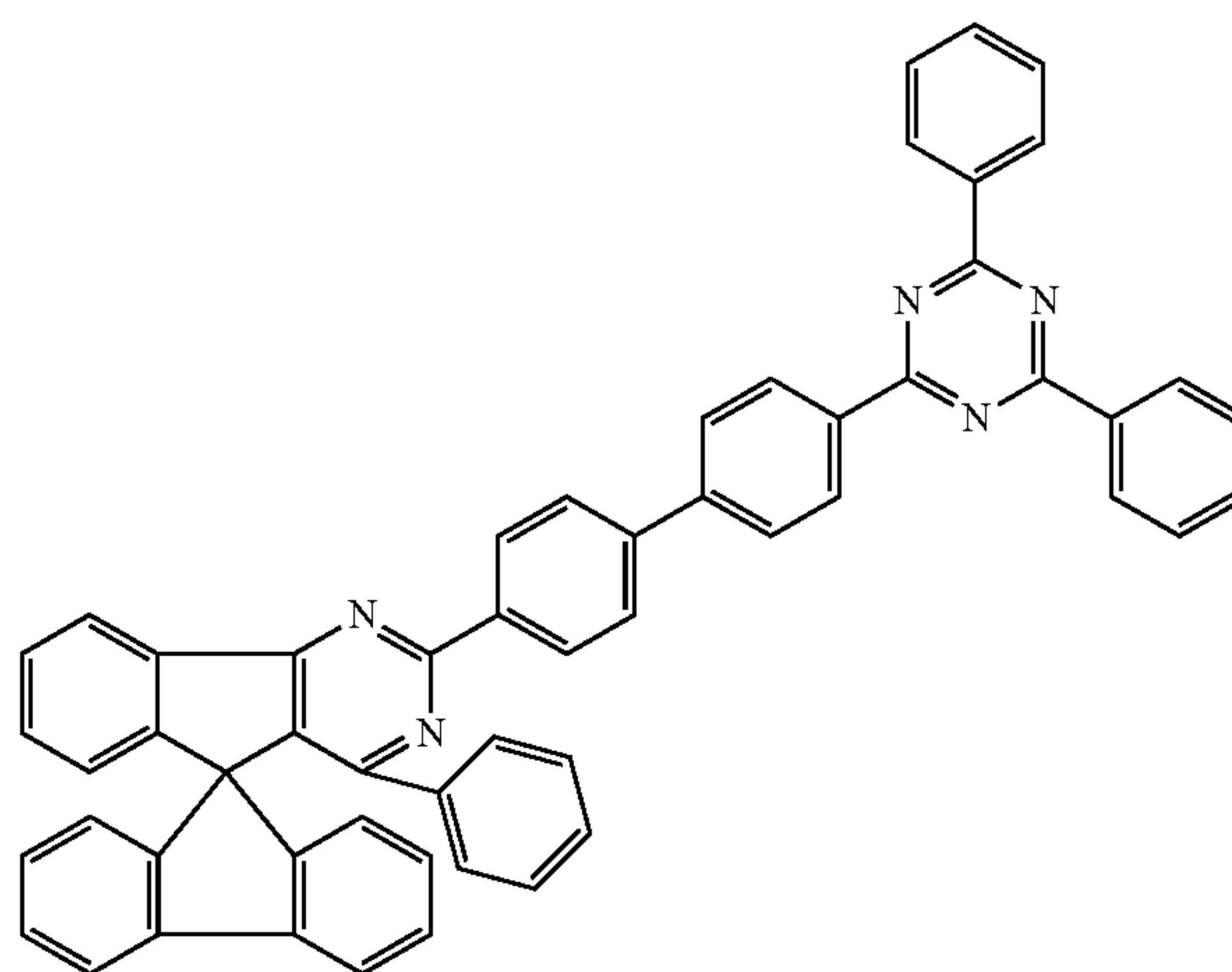
Chemical Formula 1-96
