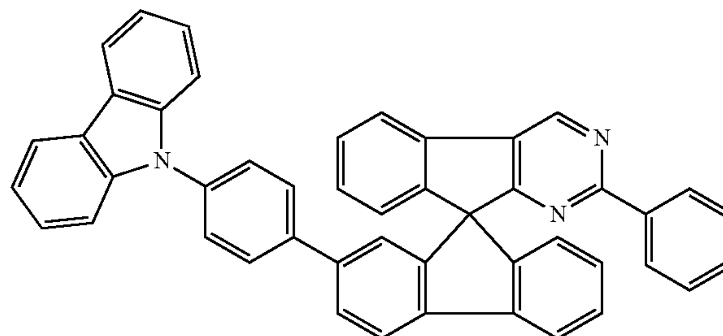
Chemical Formula 1-15
