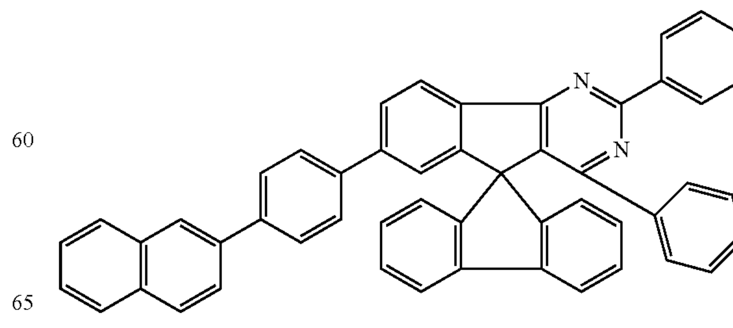
Chemical Formula 1-27
