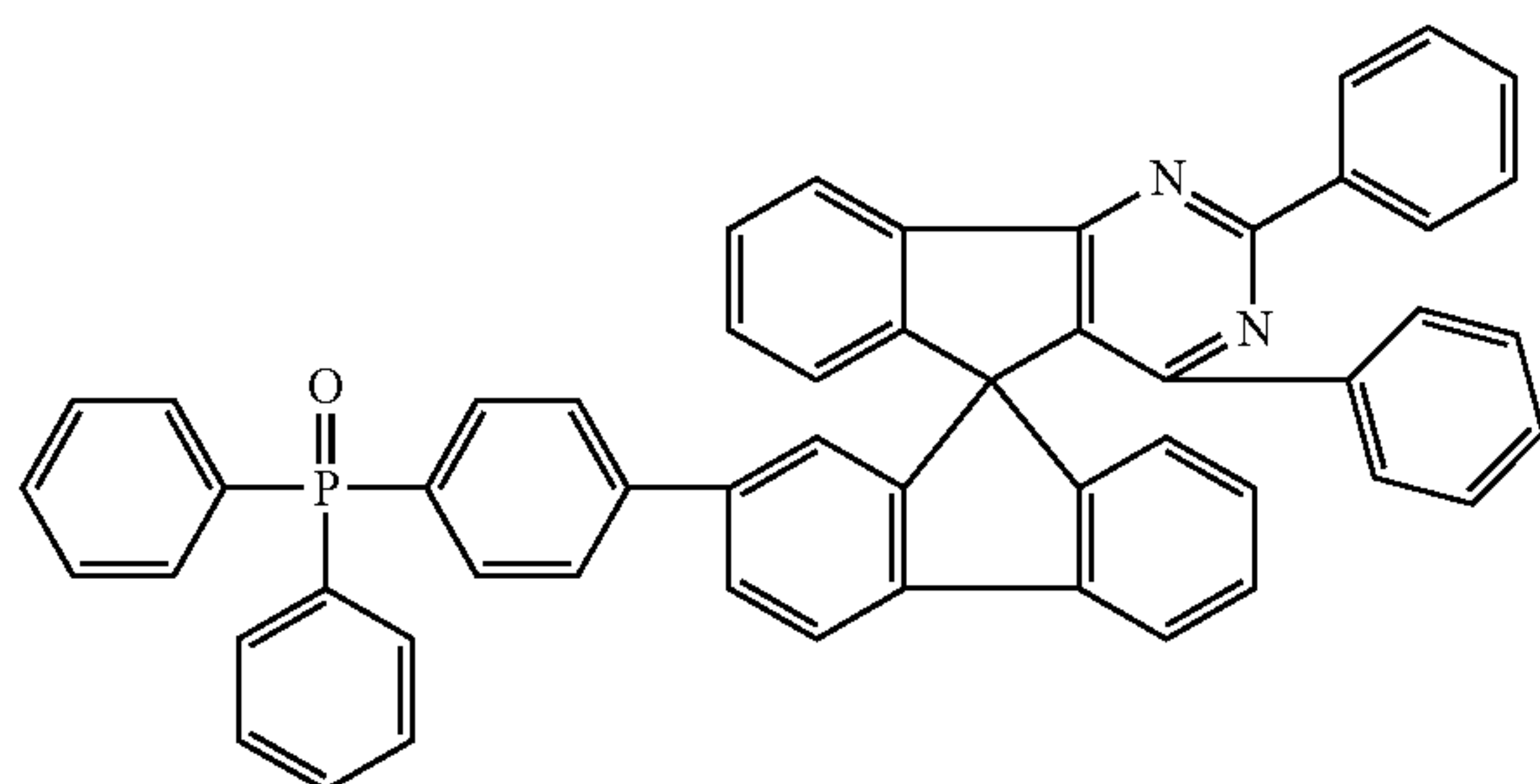
Chemical Formula 1-45
