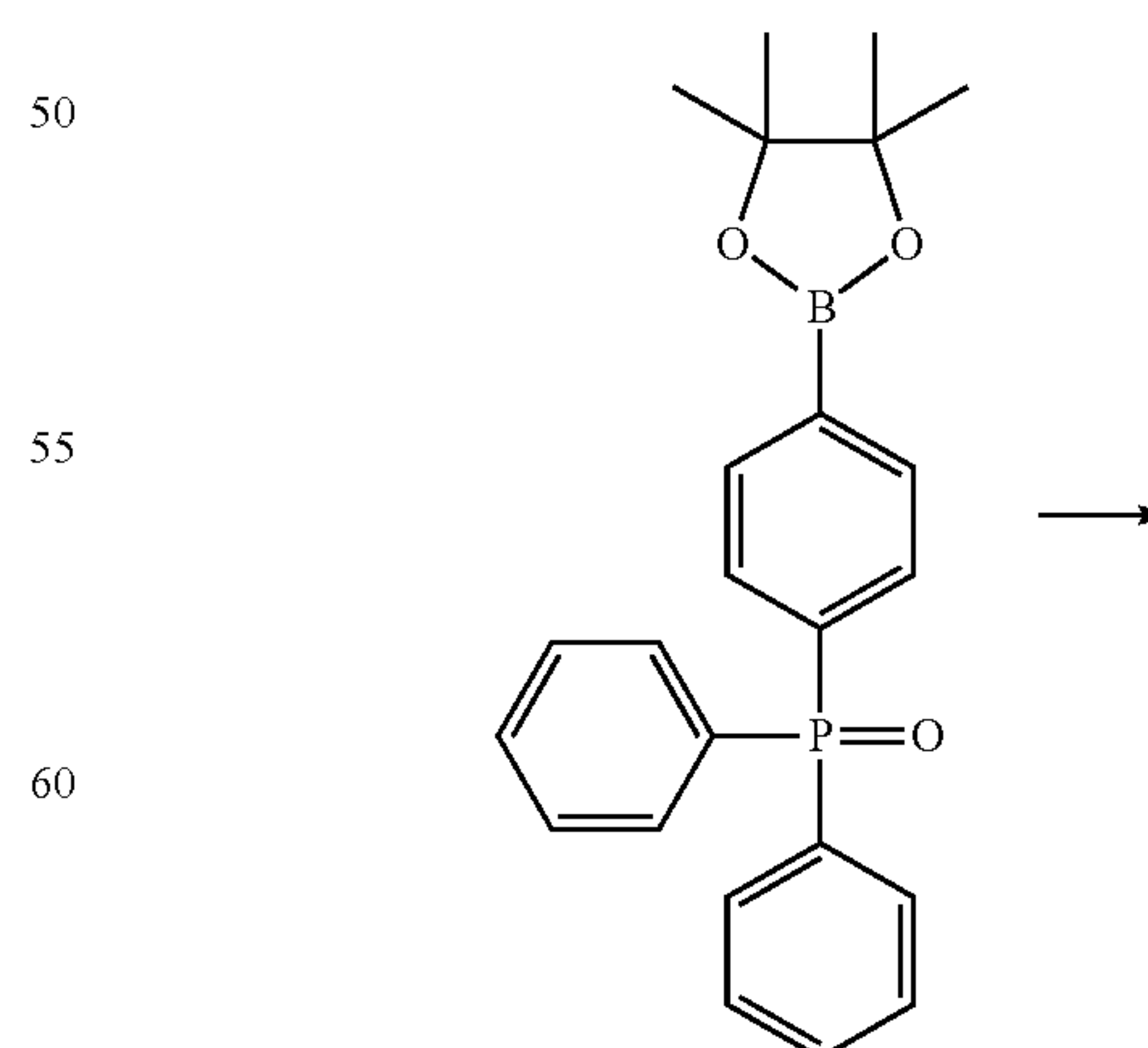
[Compound E-3]
