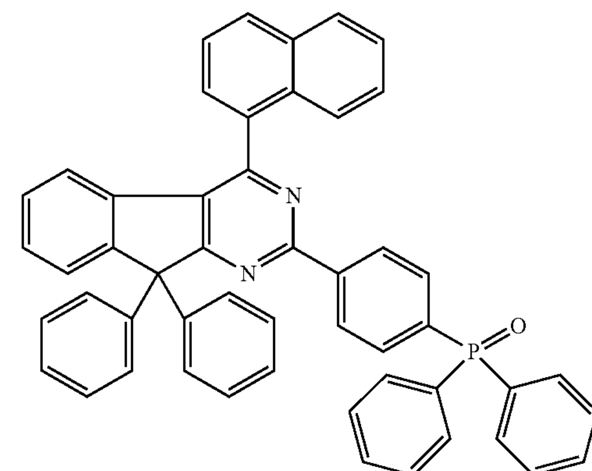
Chemical Formula 2-22
