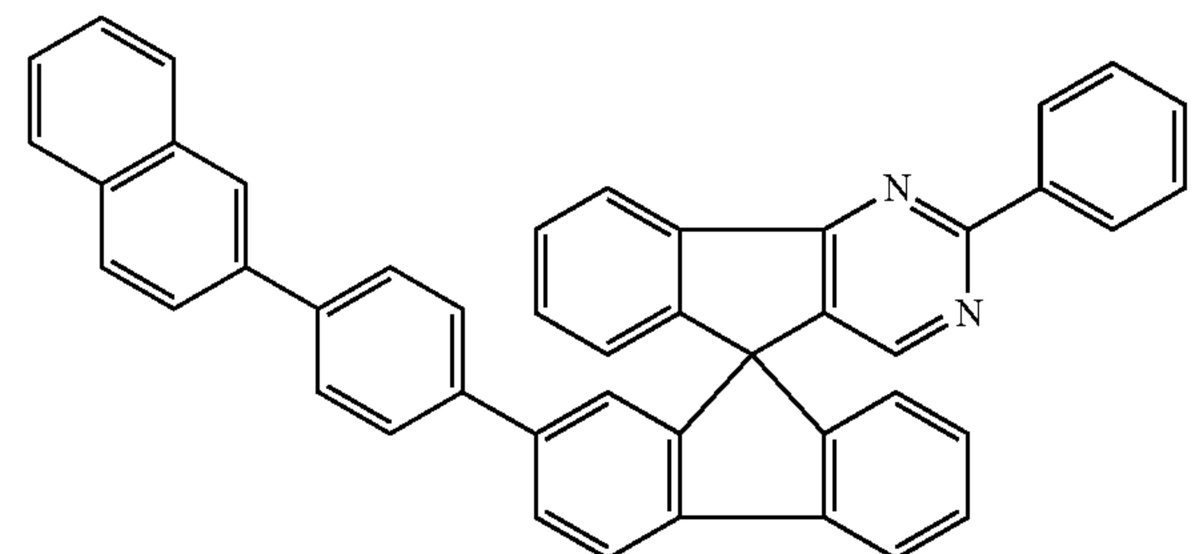
Chemical Formula 1-21
