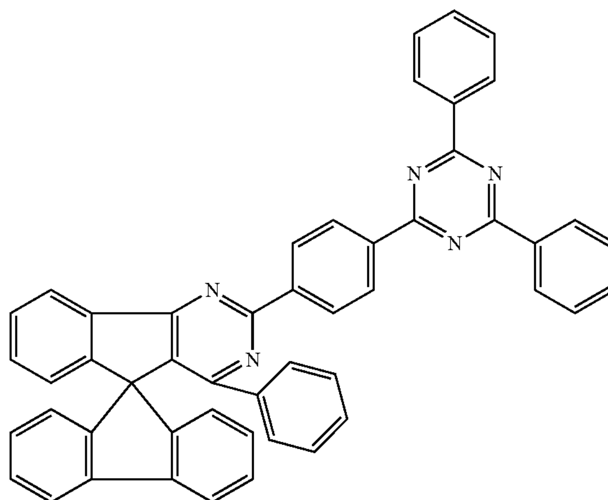
Chemical Formula 1-90
