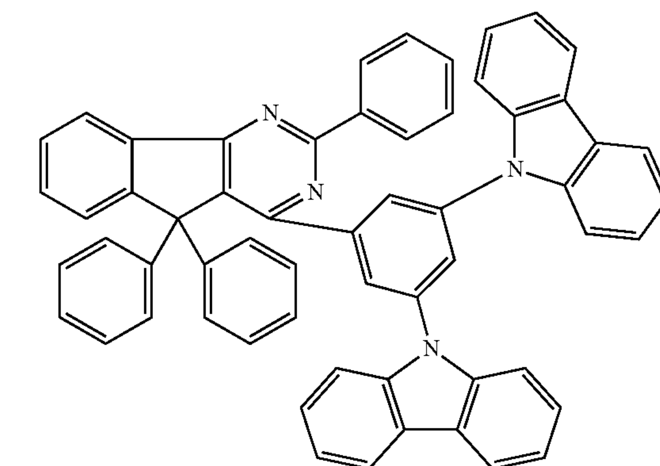
Chemical Formula 2-34
