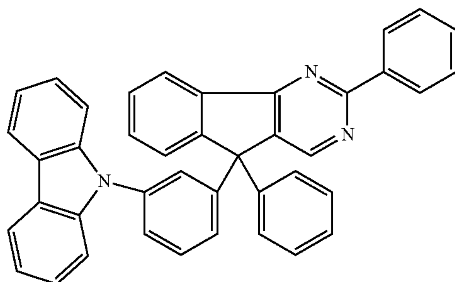
Chemical Formula 2-2
