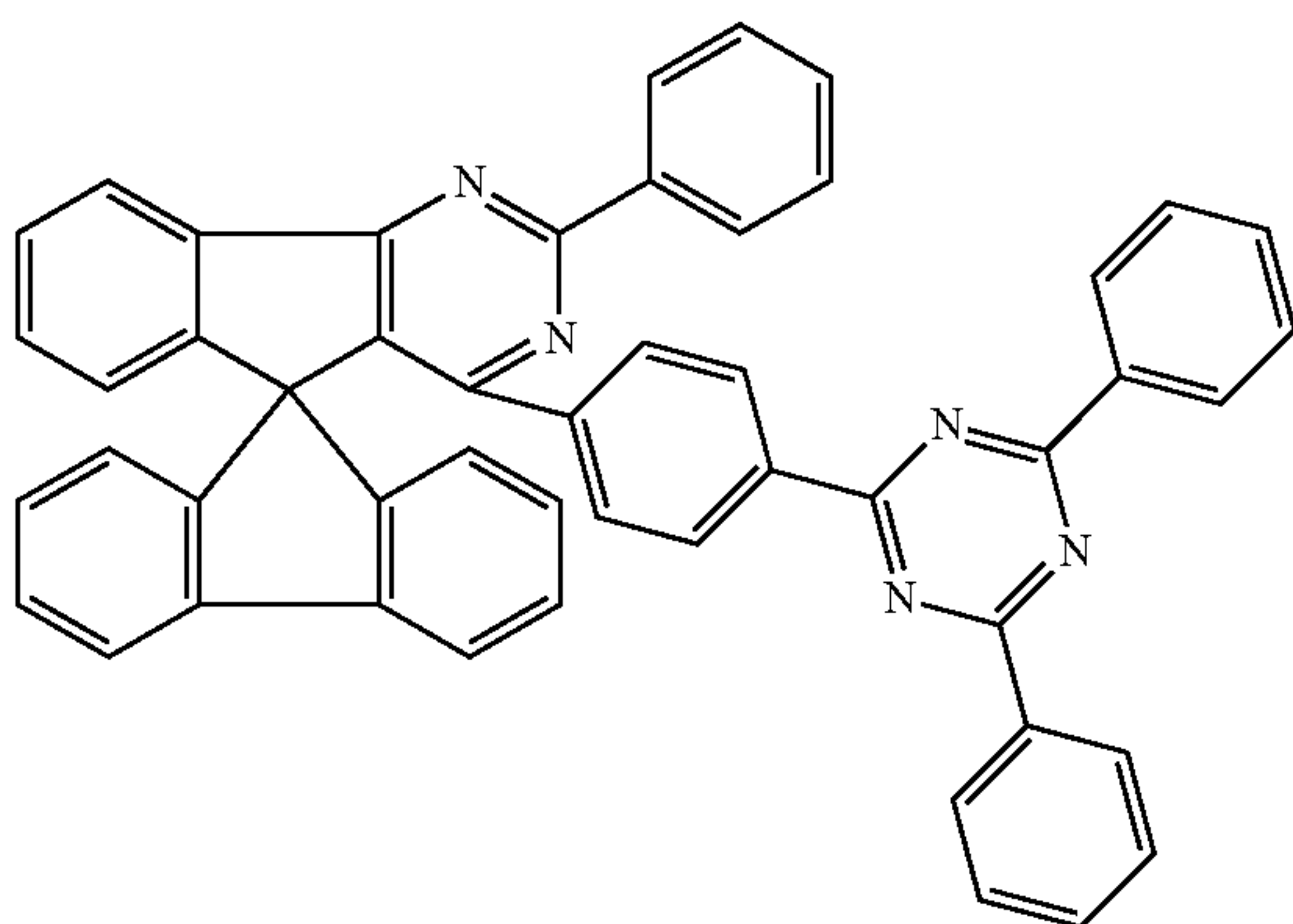
Chemical Formula 1-89
