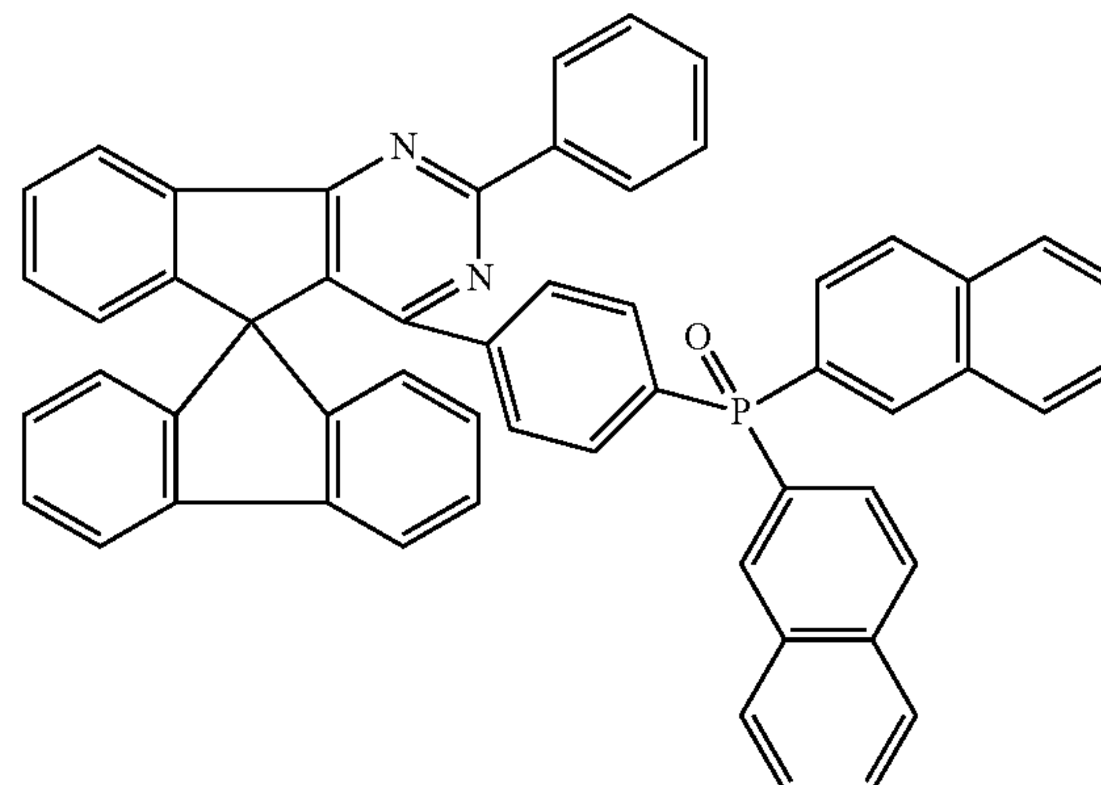
Chemical Formula 1-77
