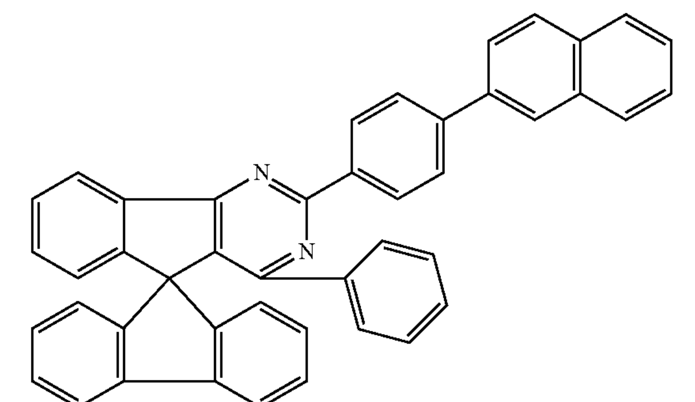
Chemical Formula 1-63
