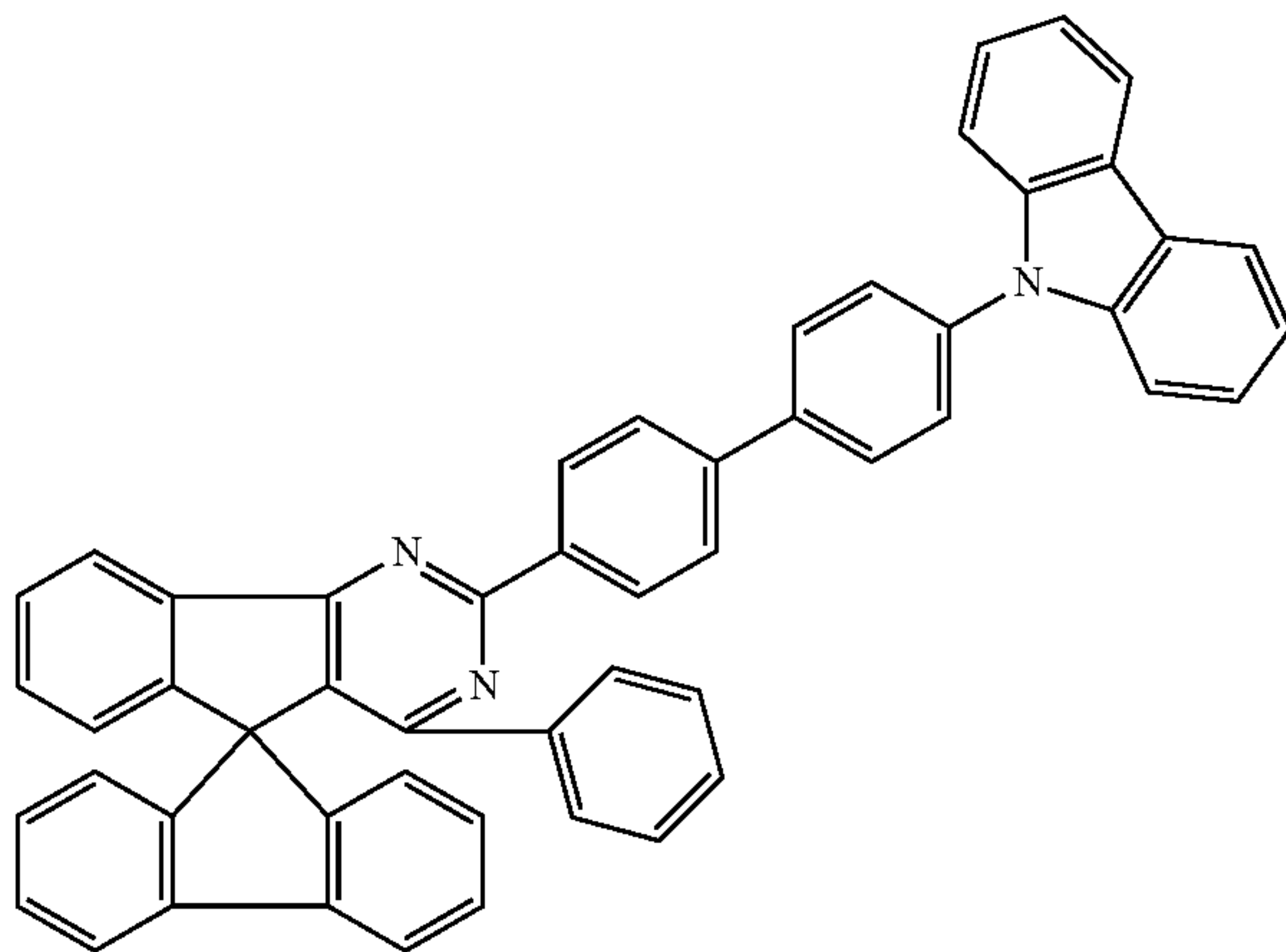
Chemical Formula 1-70
