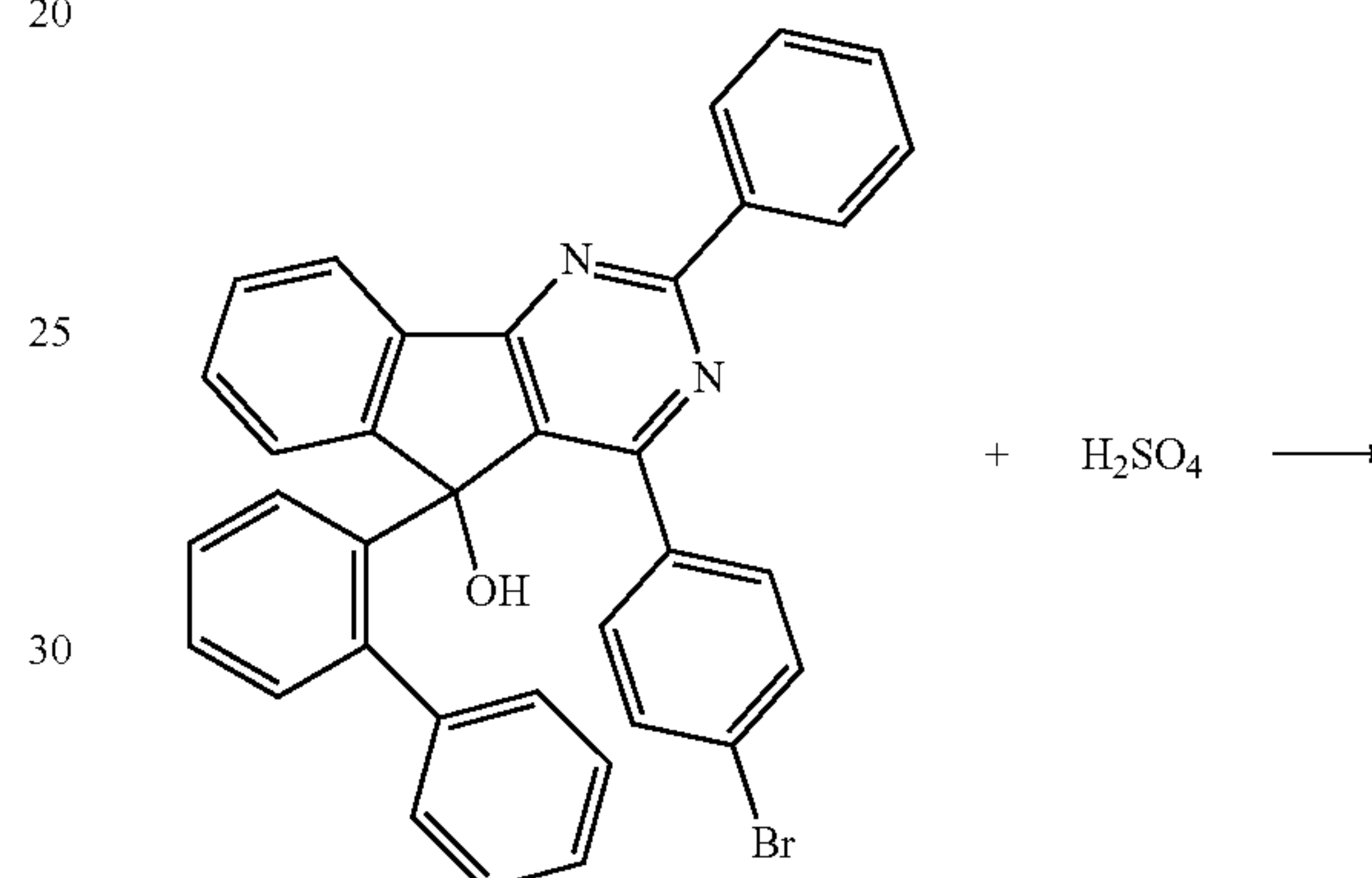
[Compound F-1]
