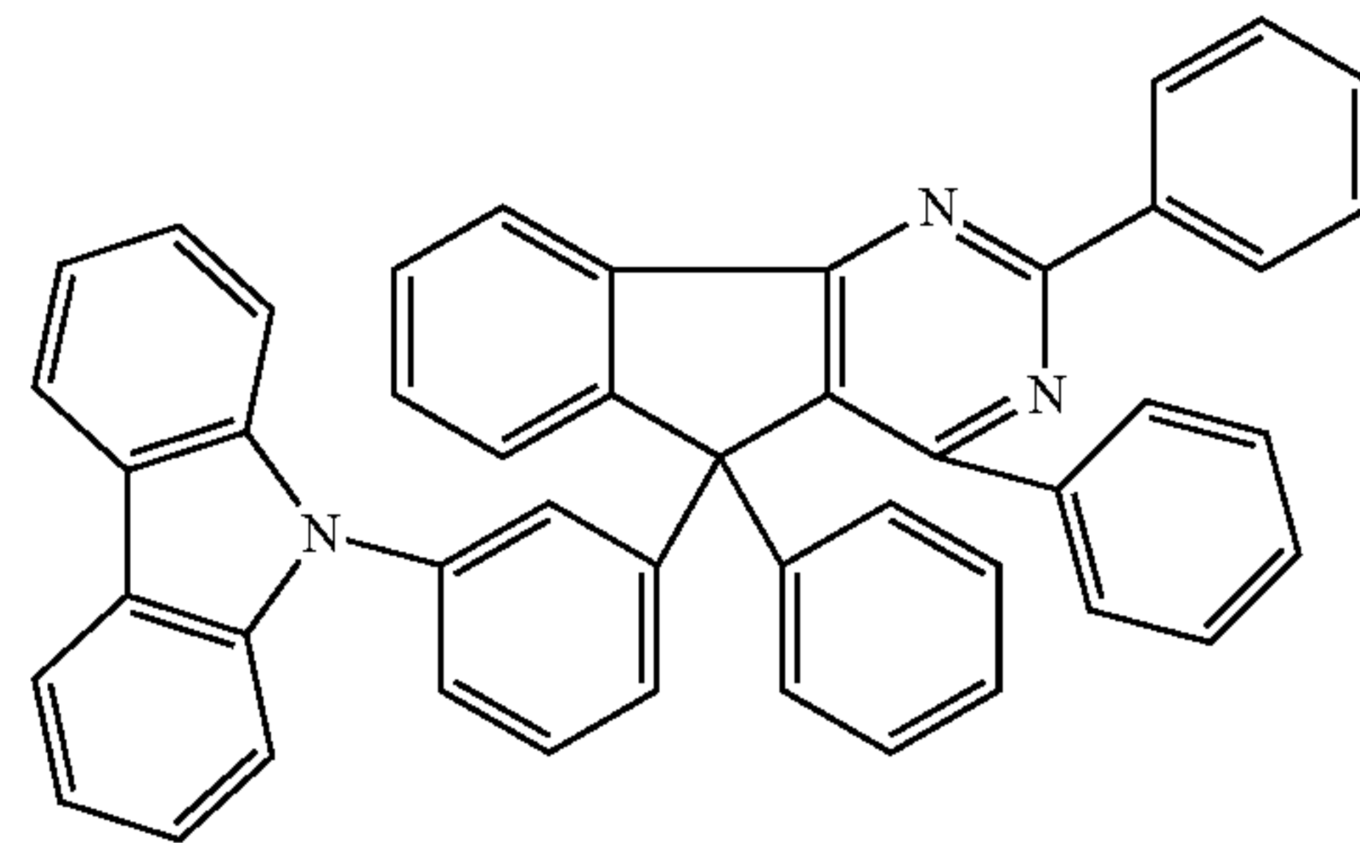
Chemical Formula 2-3
