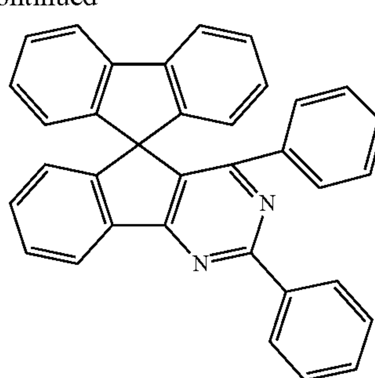
[Chemical Formula 1-11]
