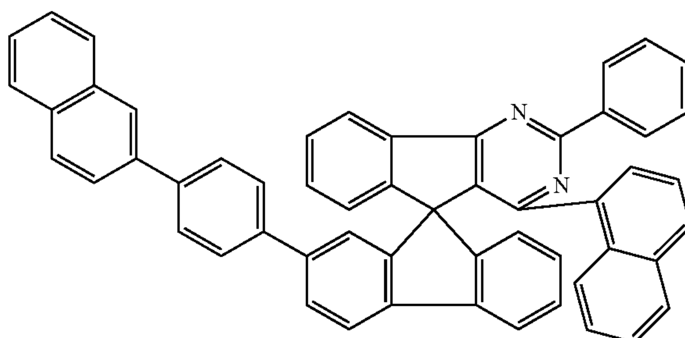
Chemical Formula 1-37
