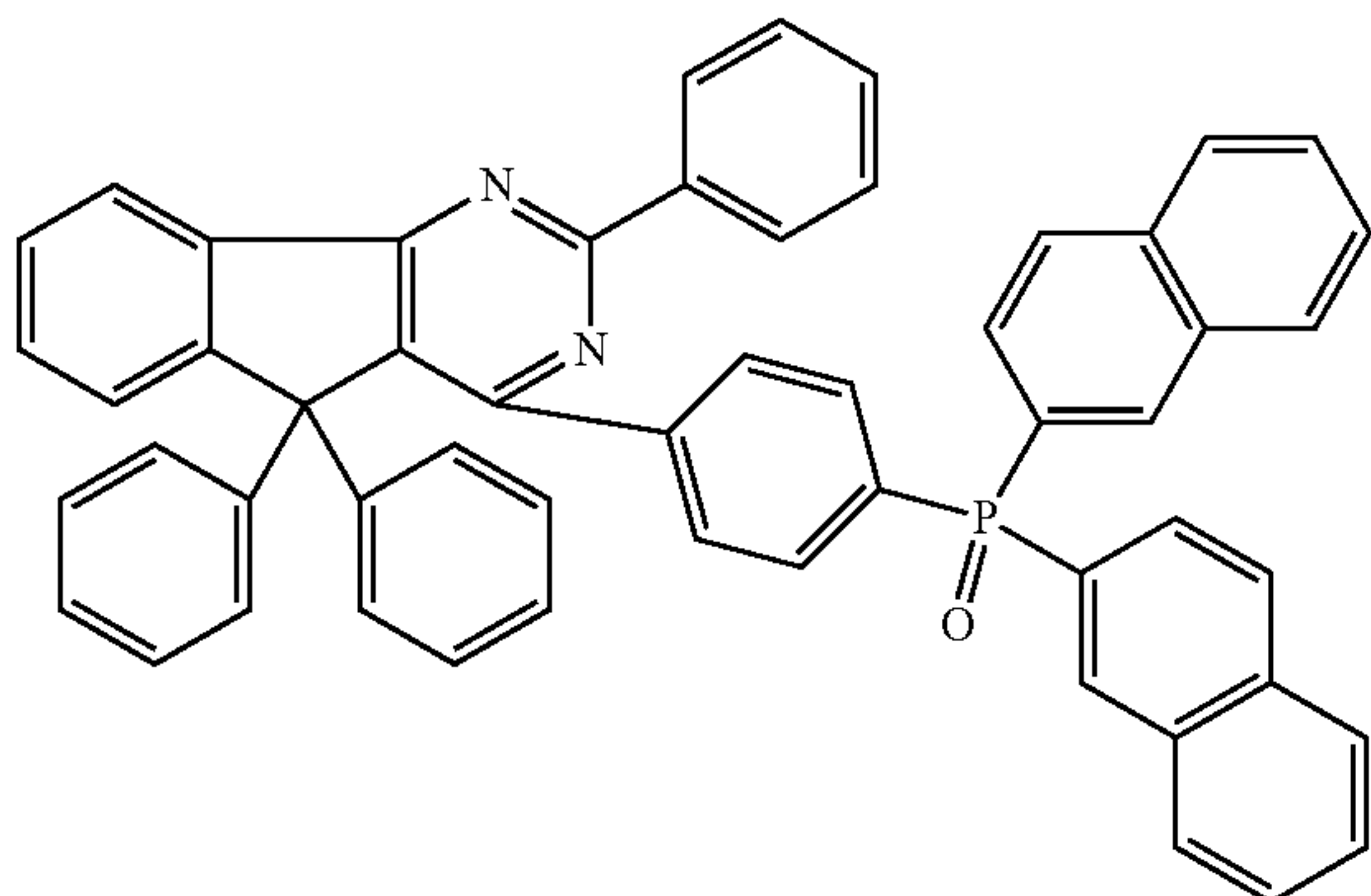
Chemical Formula 2-39
