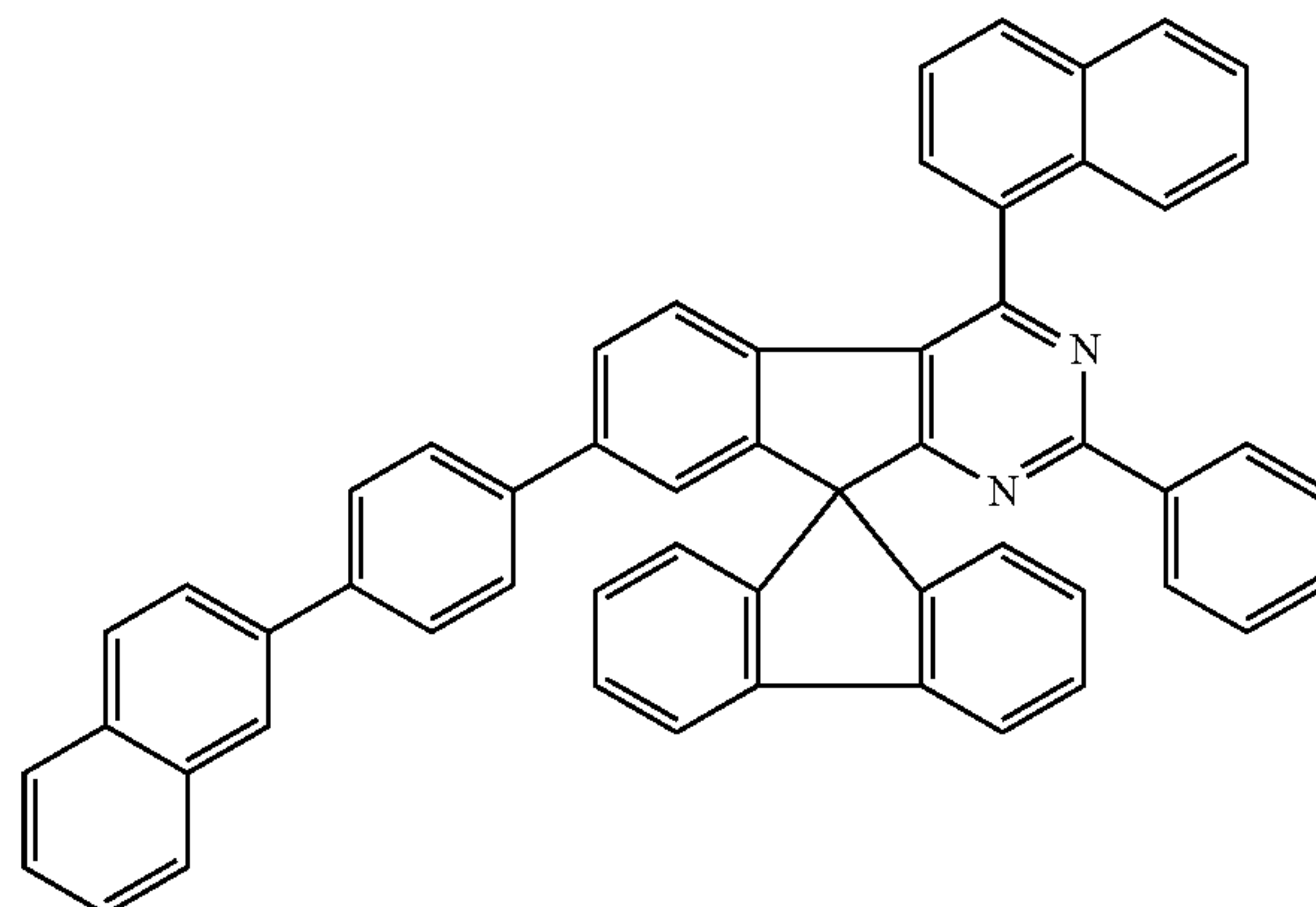
Chemical Formula 1-40
