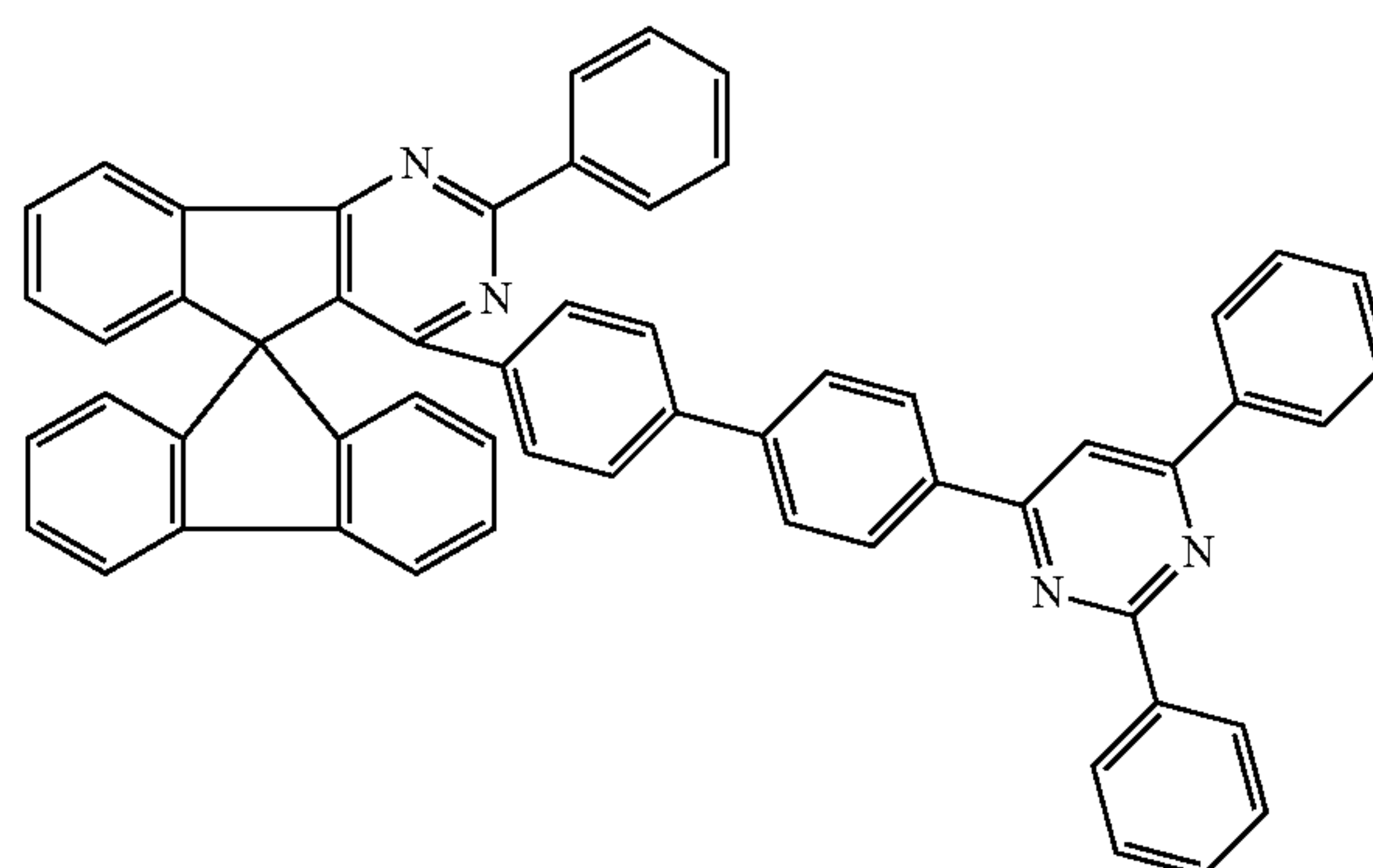
Chemical Formula 1-97
