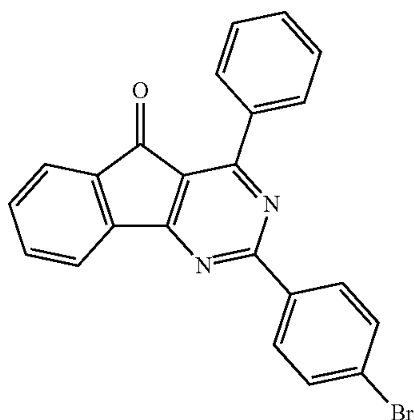
[Compound E]
