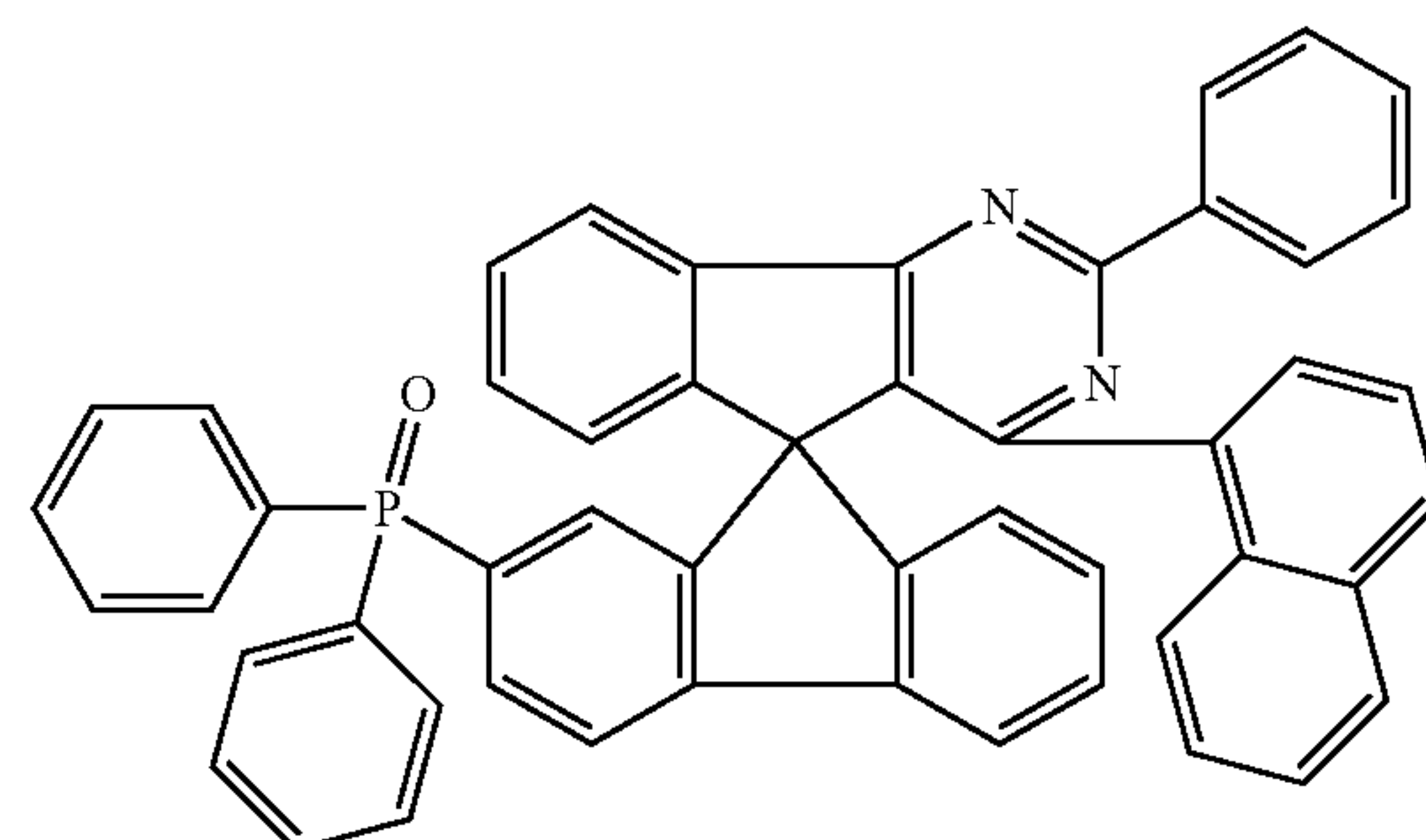
Chemical Formula 1-43
