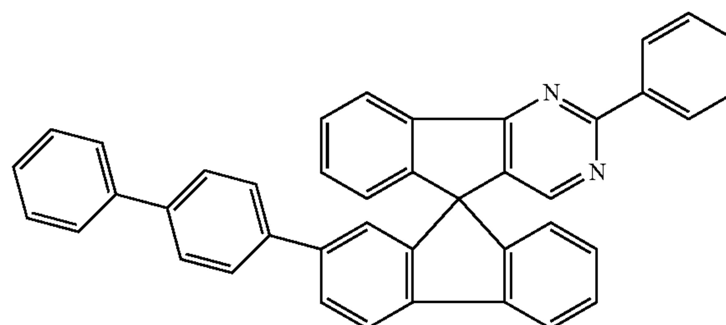
Chemical Formula 1-5
