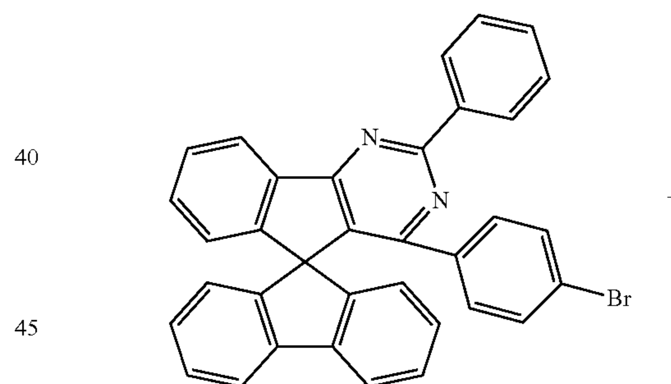
[Compound F-2]
