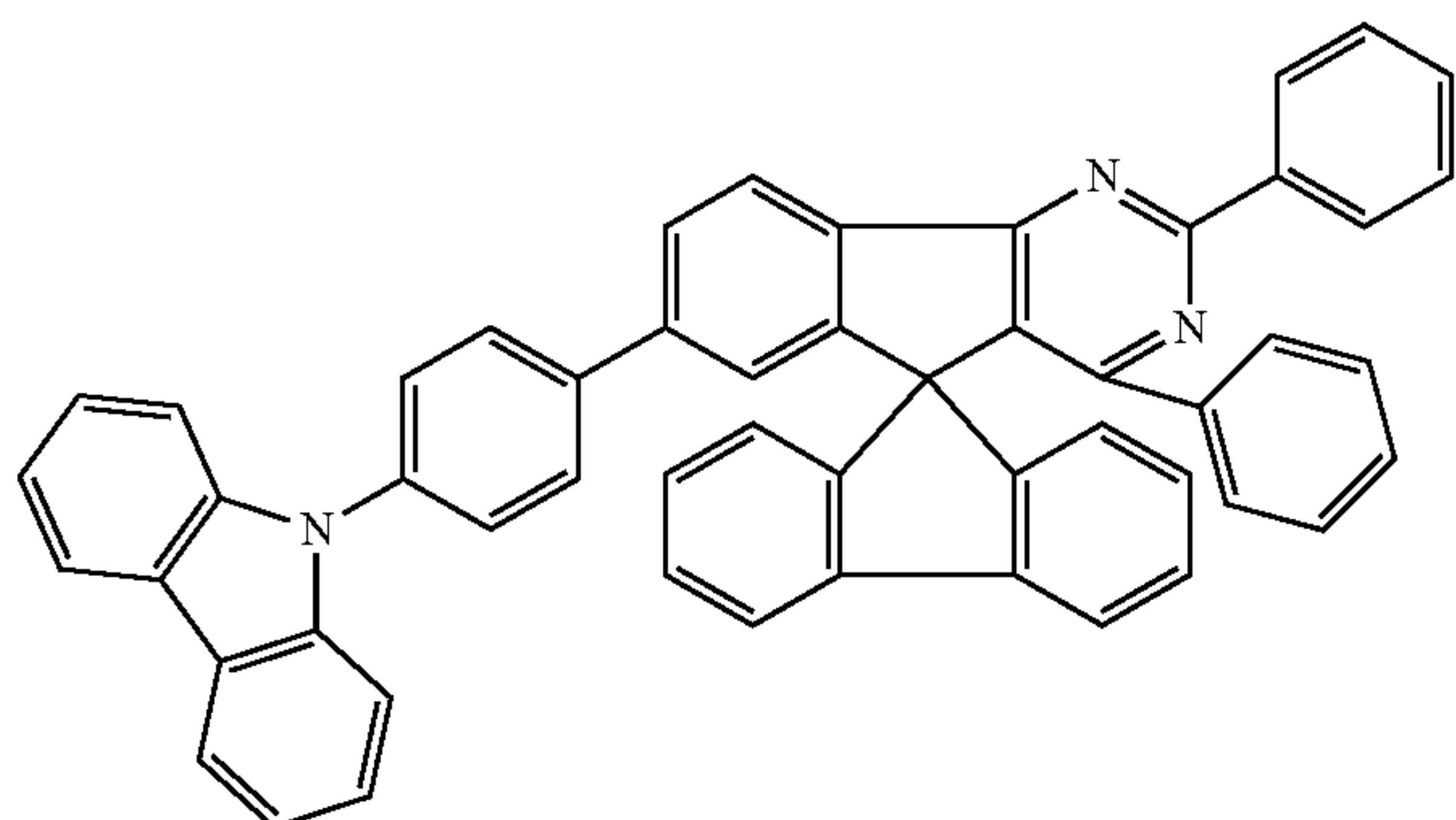
Chemical Formula 1-20
