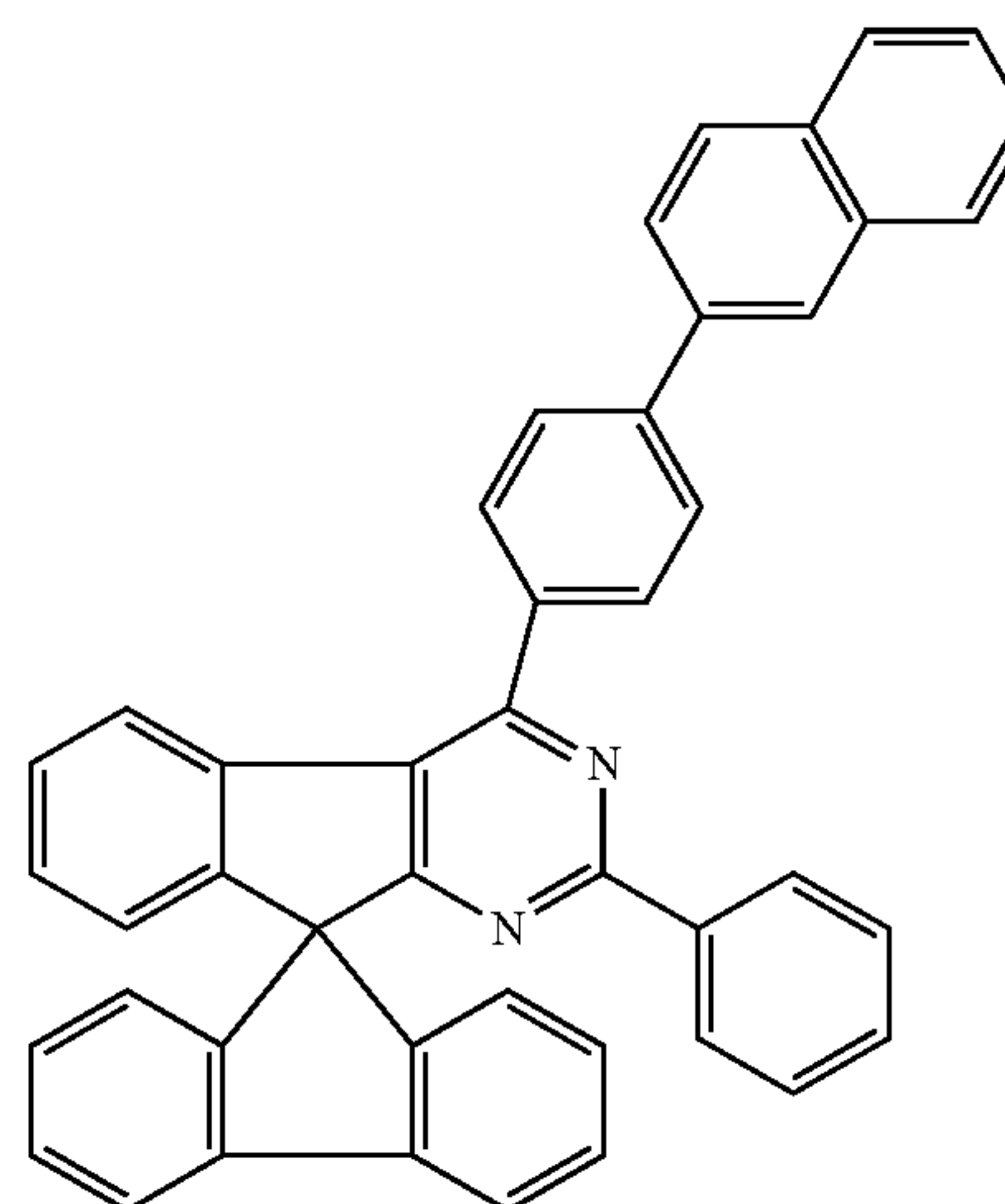
Chemical Formula 1-85
