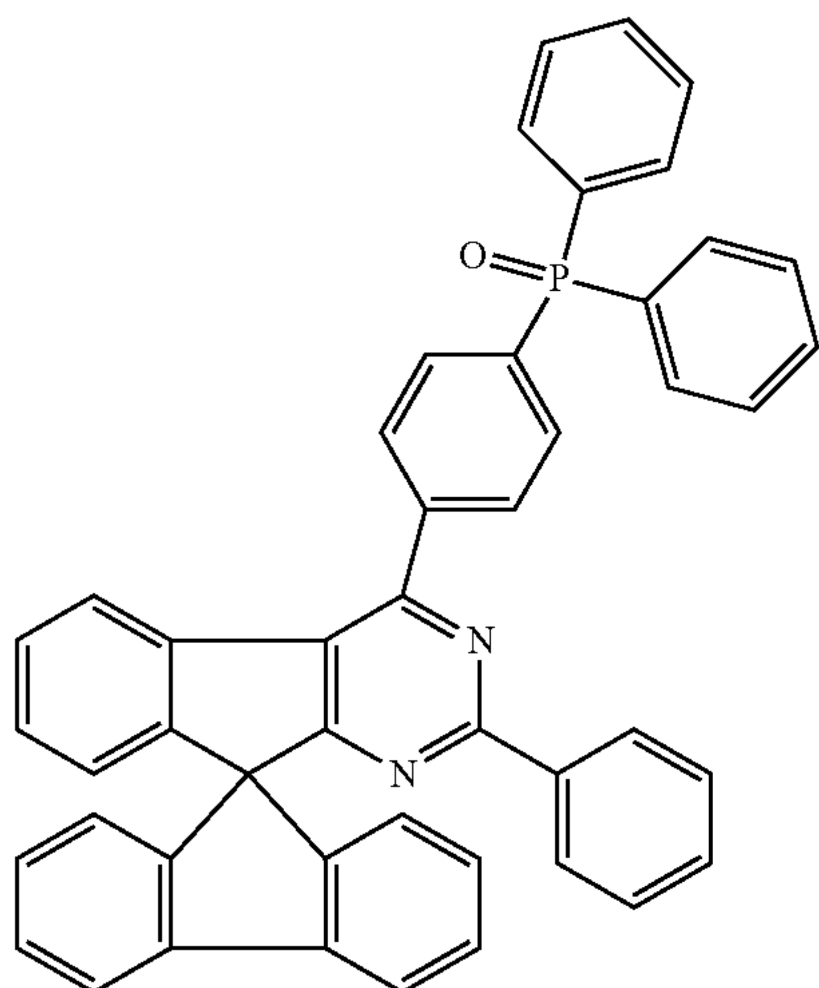
Chemical Formula 1-76
