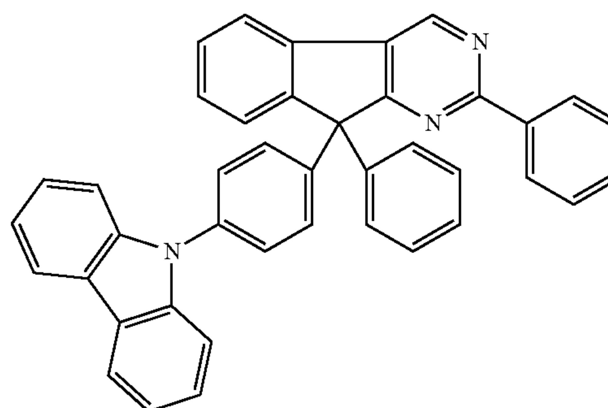
Chemical Formula 2-7
