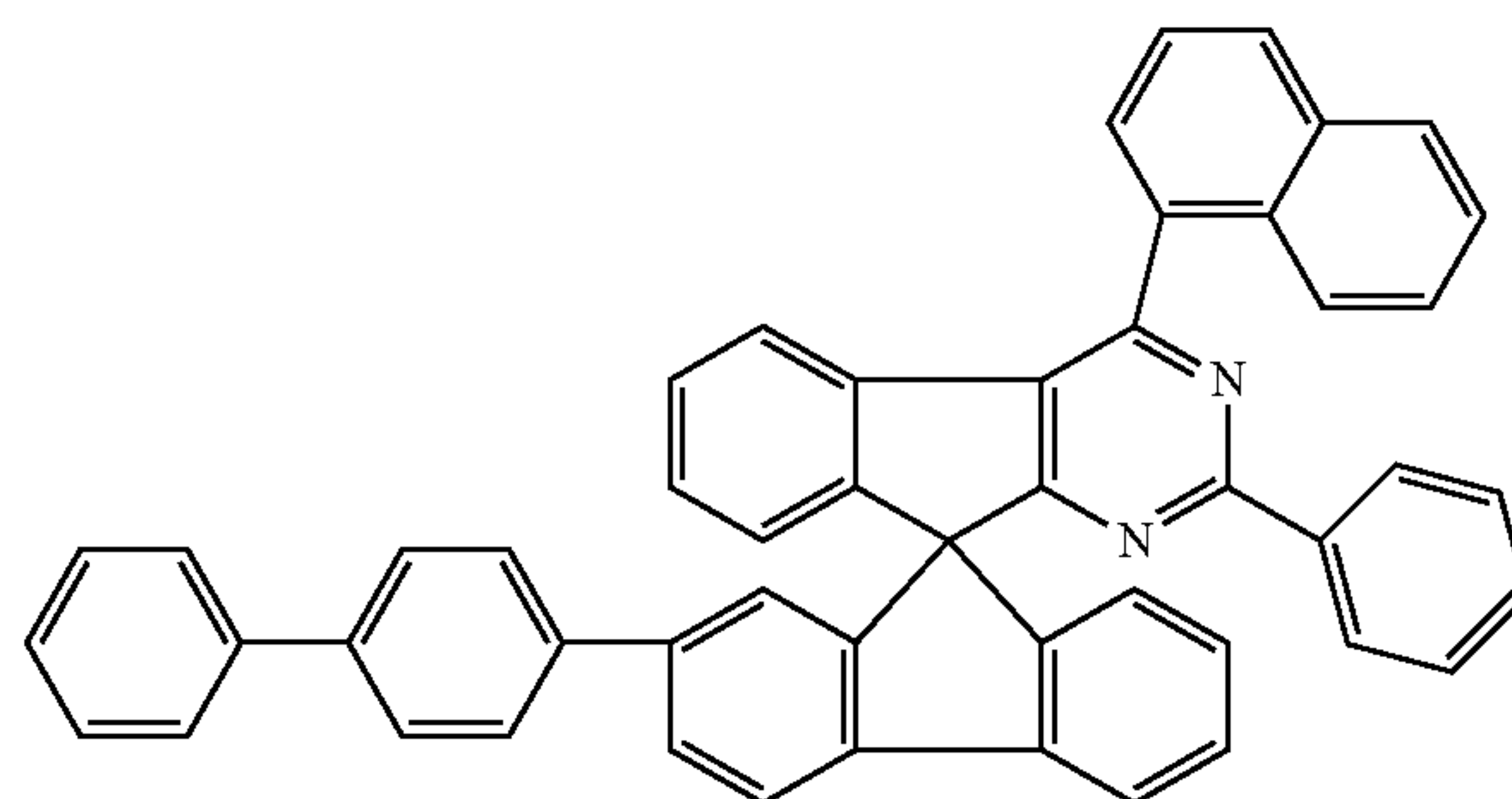
Chemical Formula 1-33
