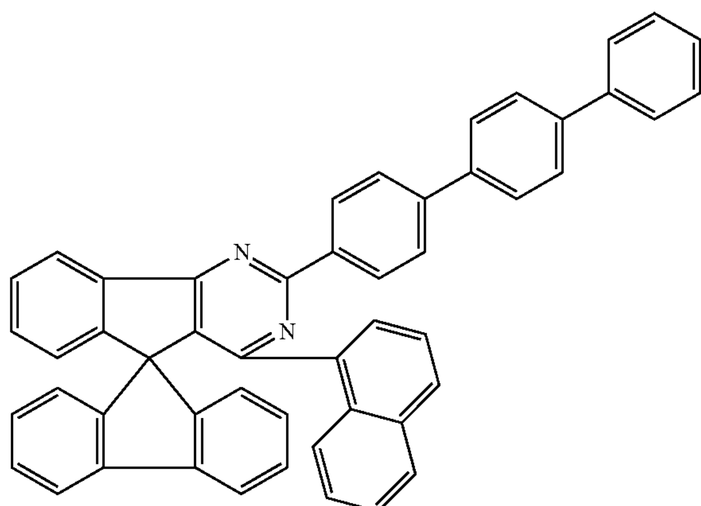
Chemical Formula 1-61
