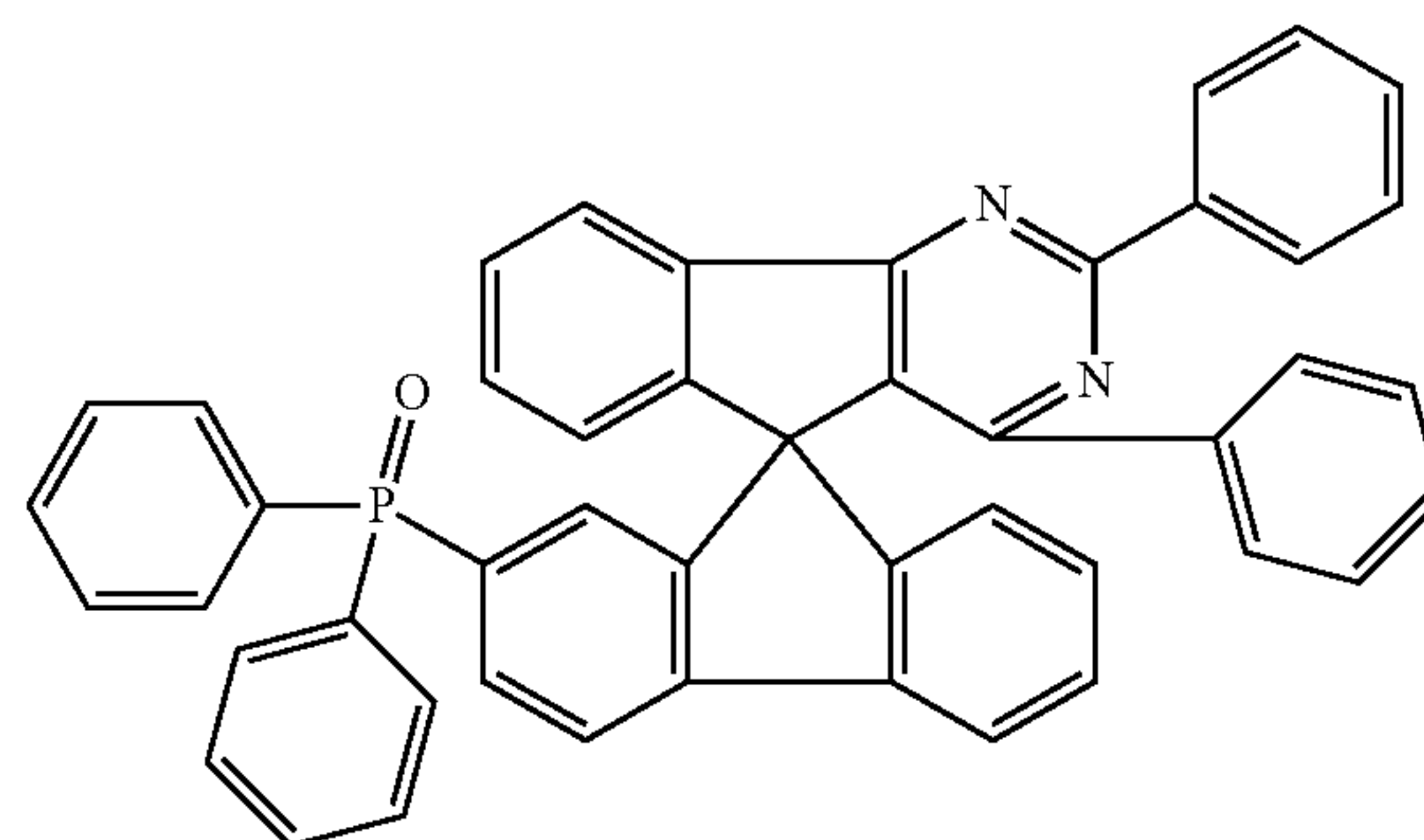
Chemical Formula 1-41
