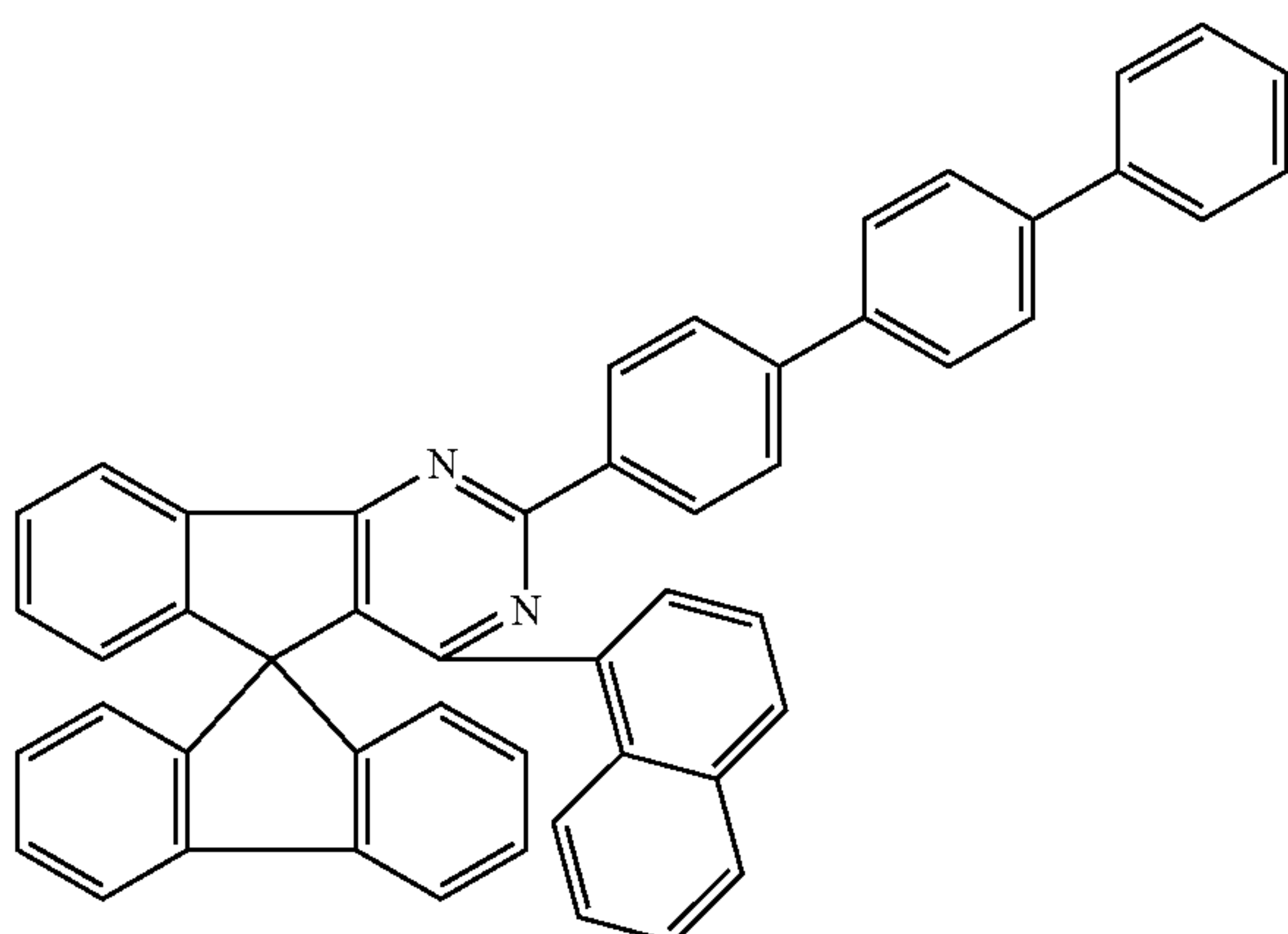
Chemical Formula 1-62
