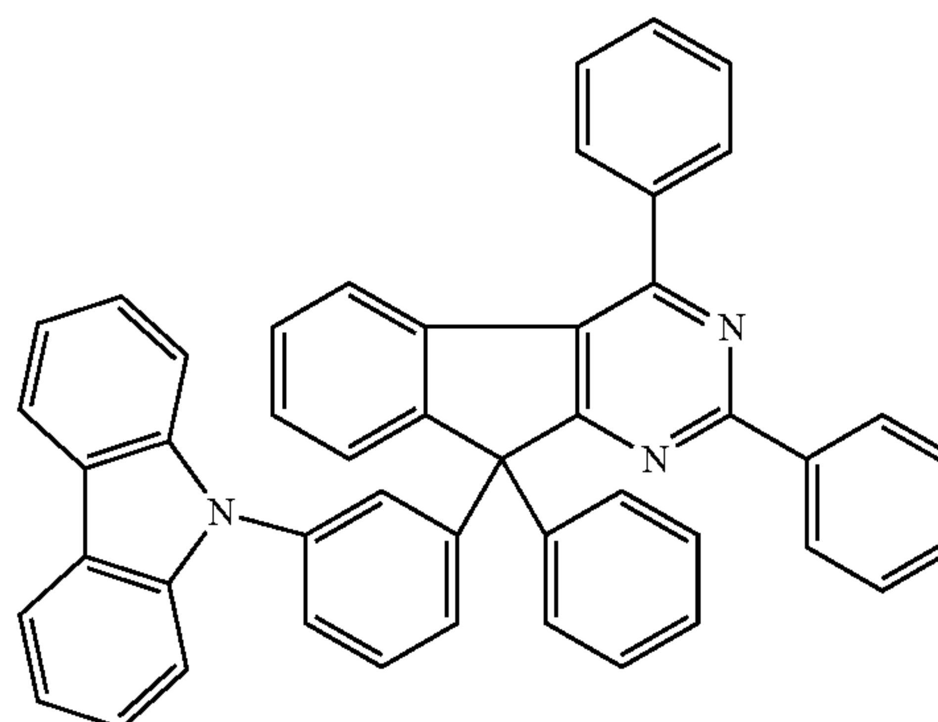
Chemical Formula 2-5
