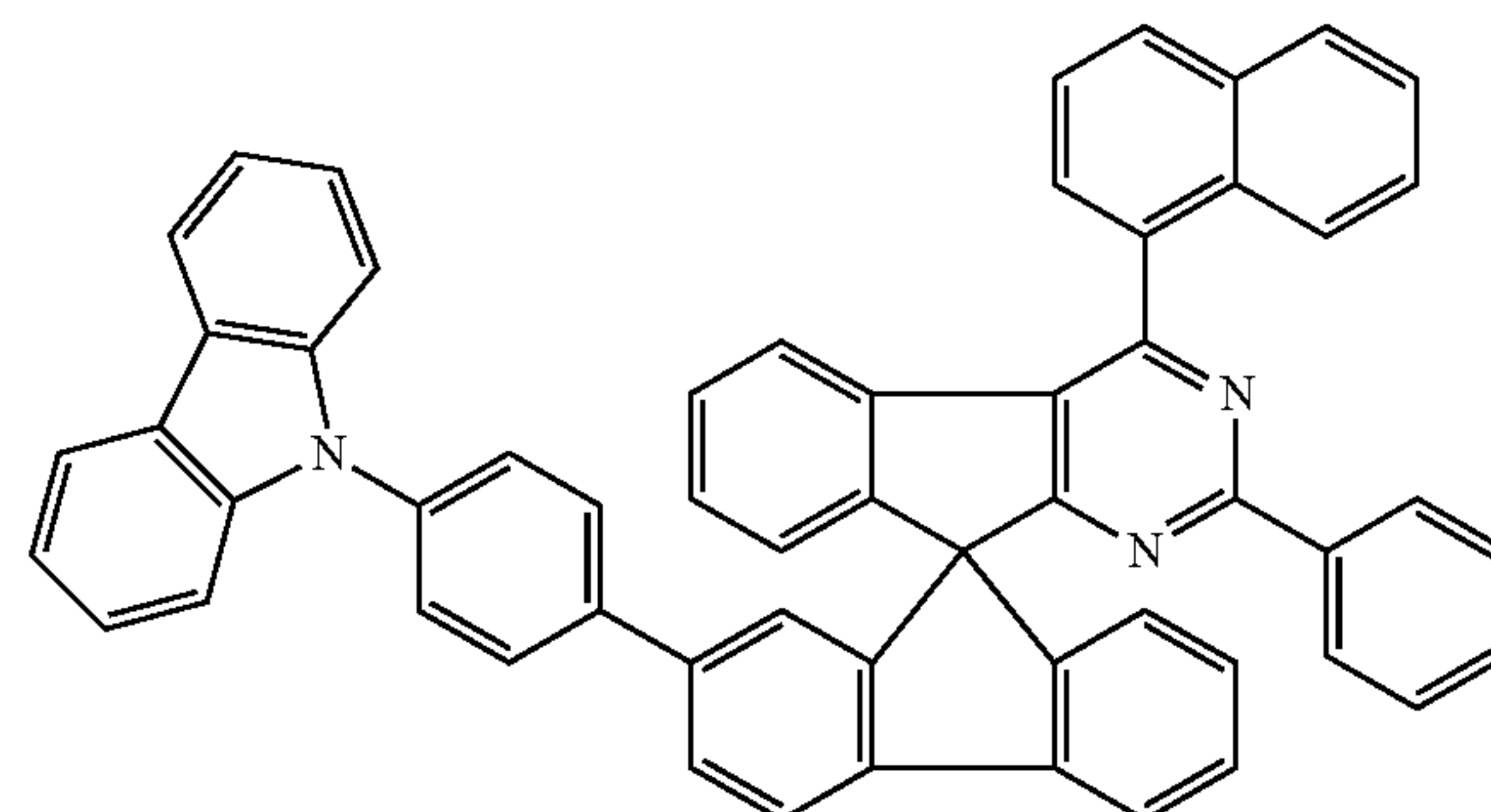
Chemical Formula 1-34
