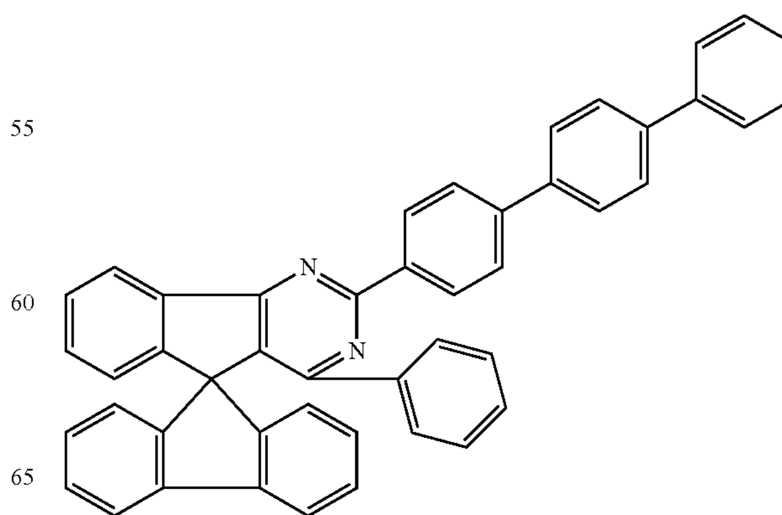
Chemical Formula 1-59
