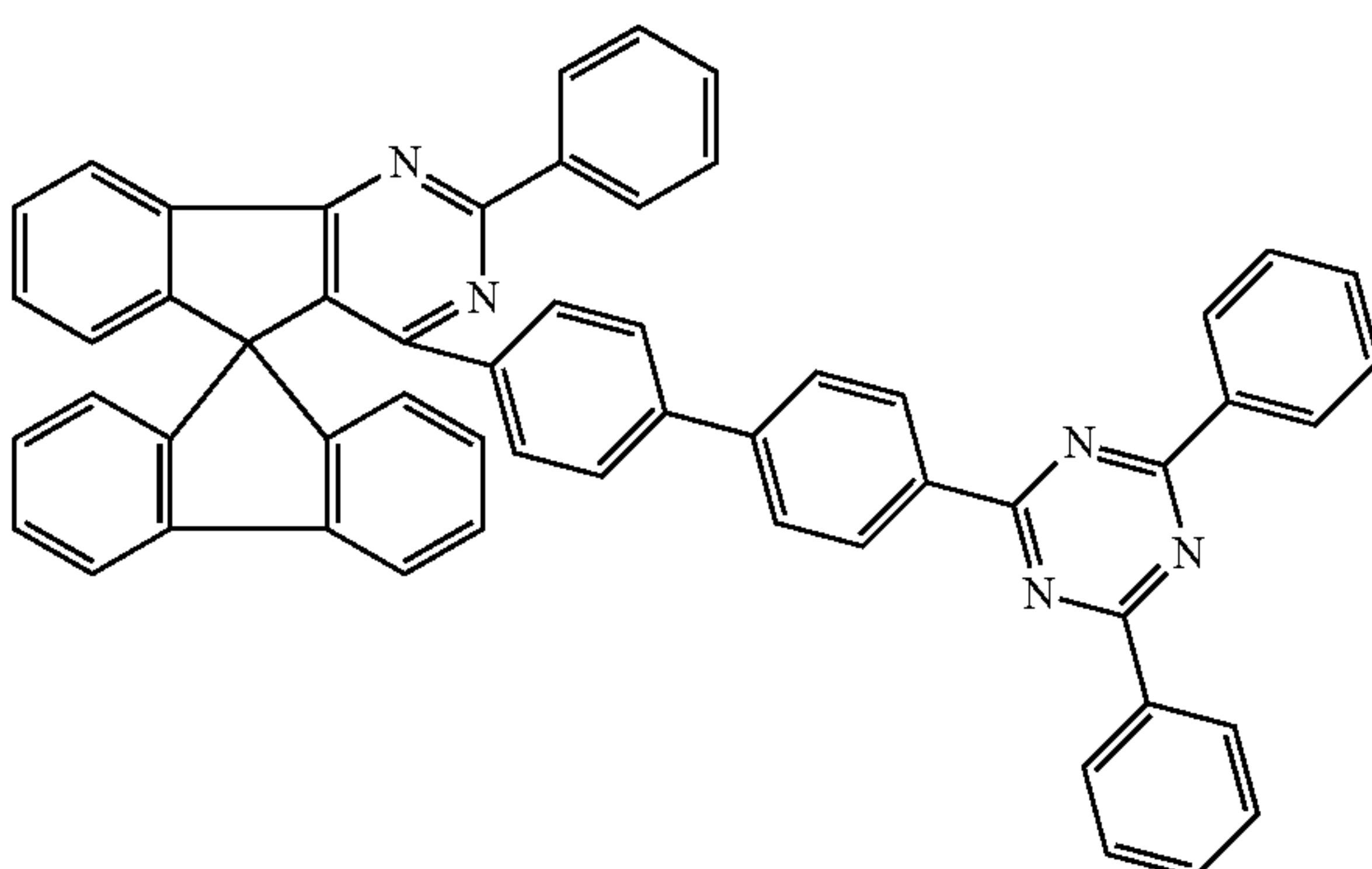
Chemical Formula 1-95
