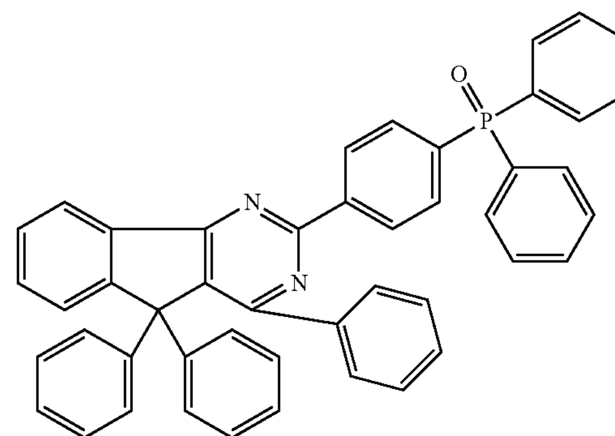
Chemical Formula 2-20
