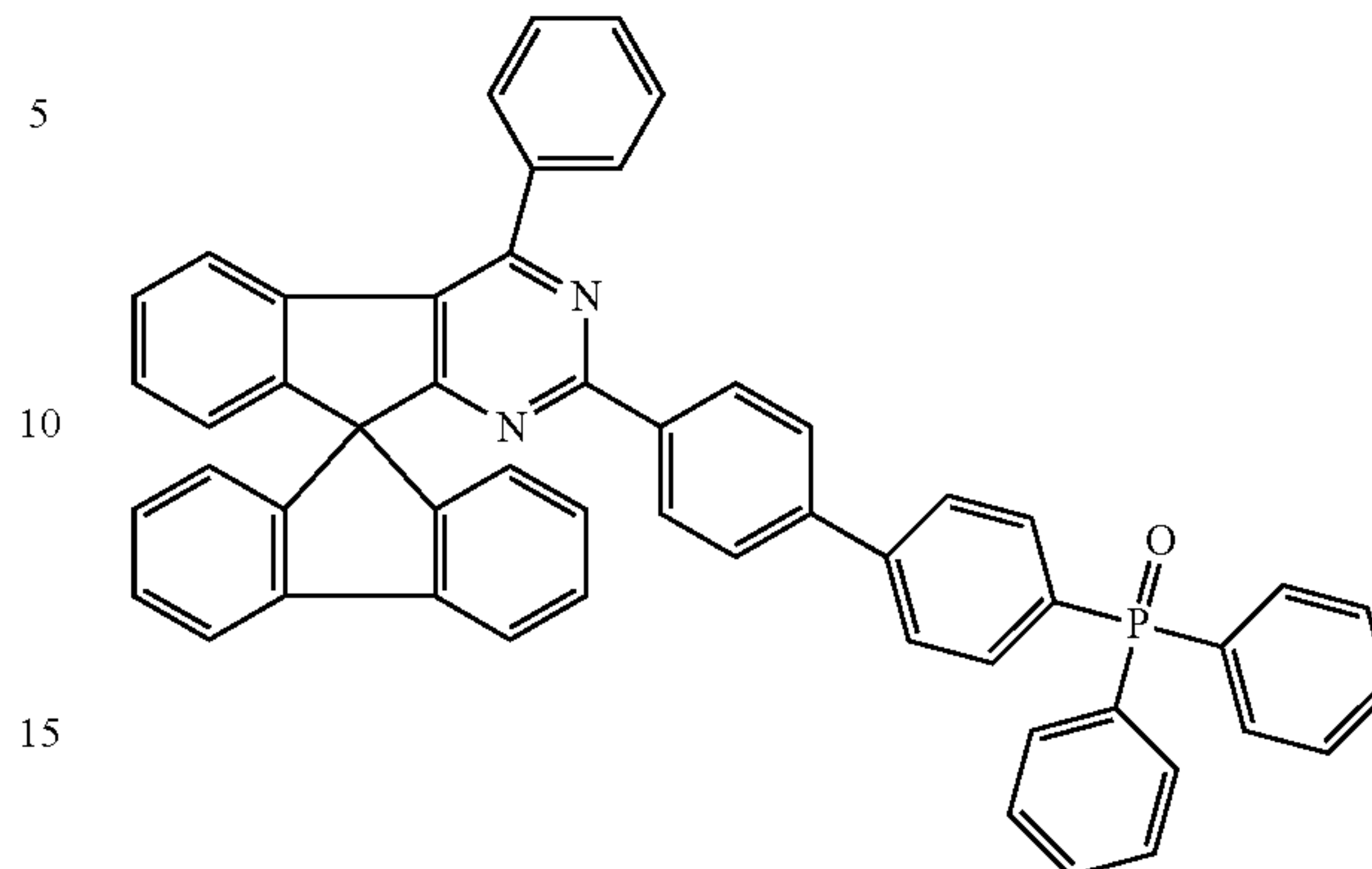
Chemical Formula 1-57
