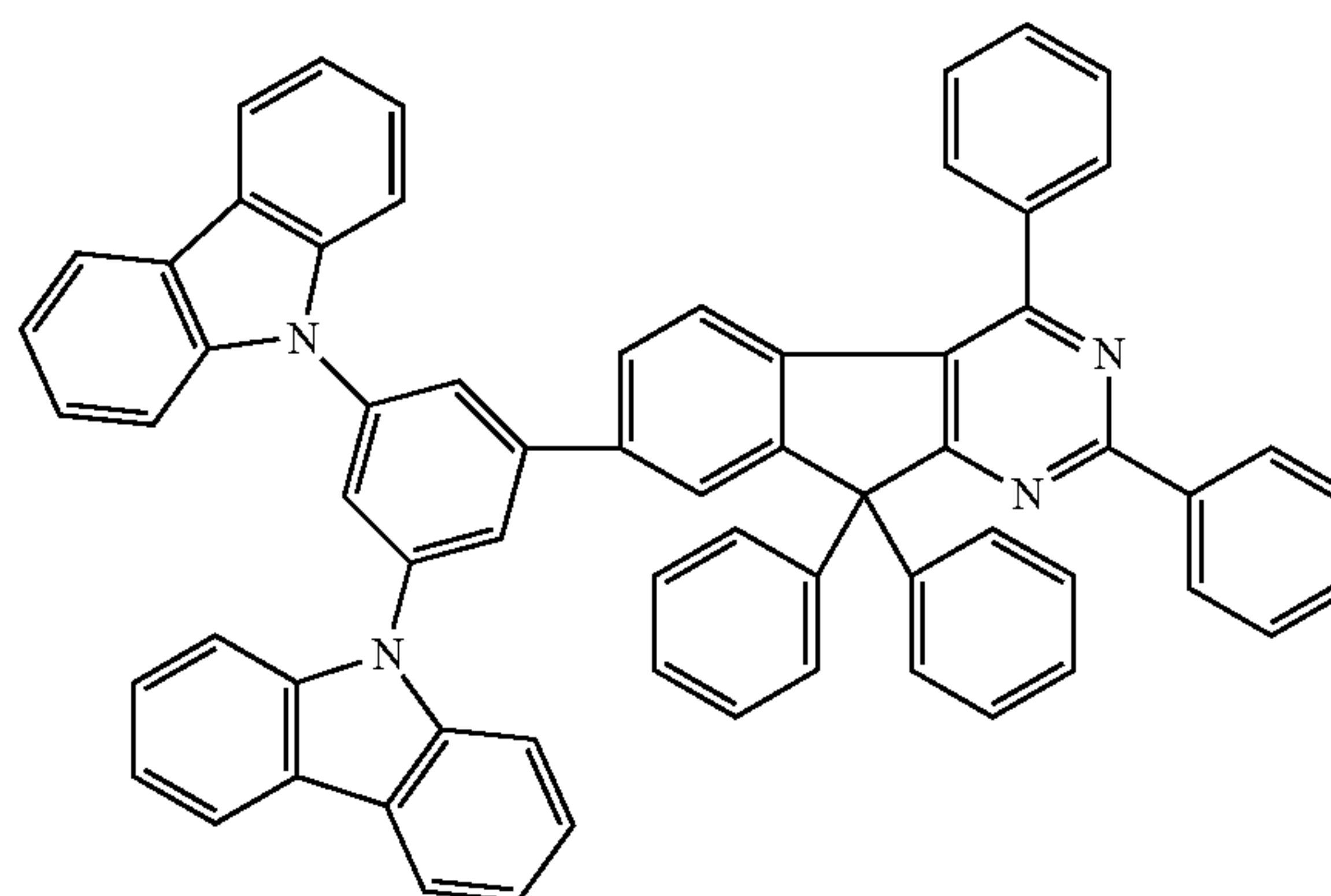
Chemical Formula 2-35
