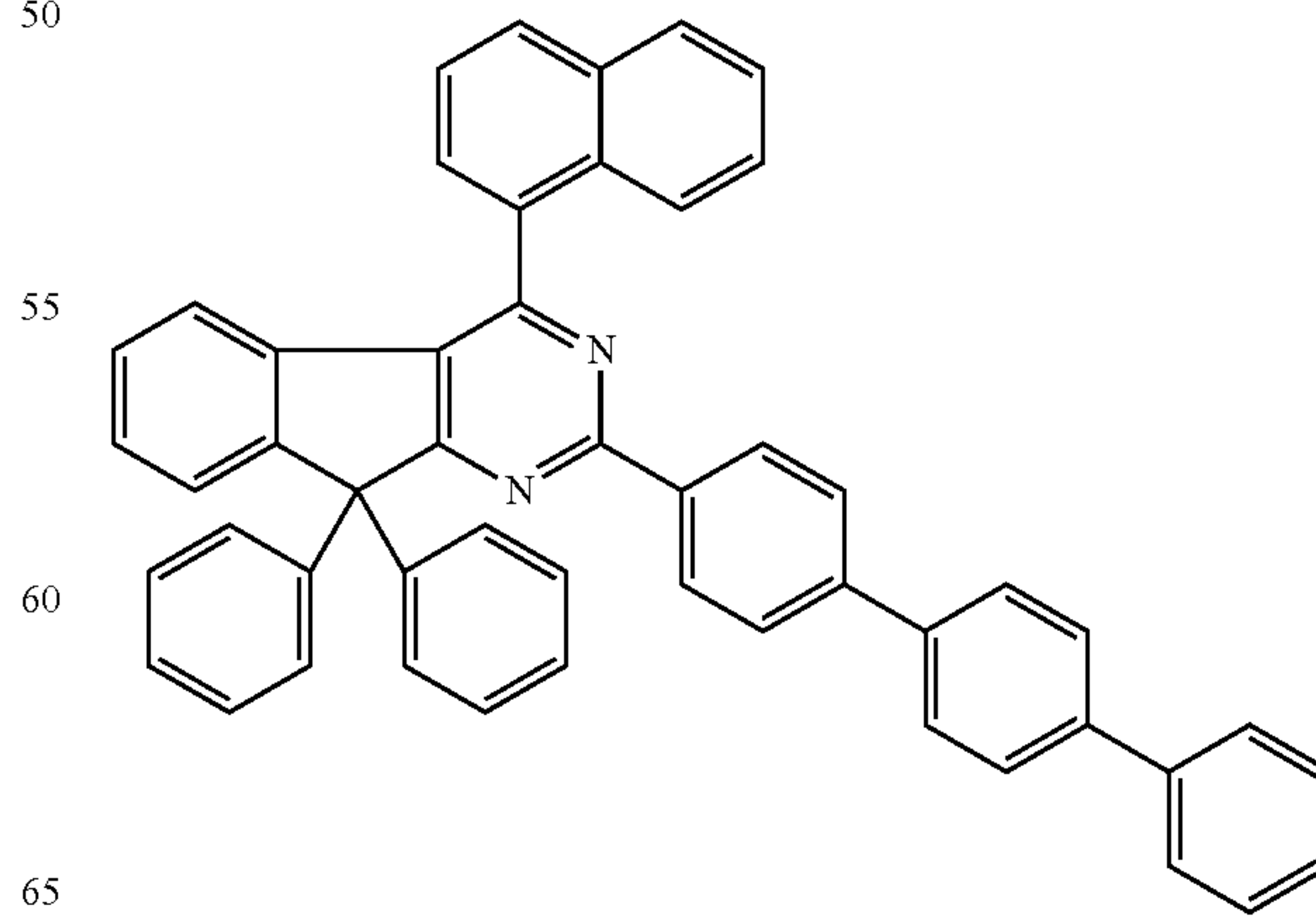
Chemical Formula 2-28
