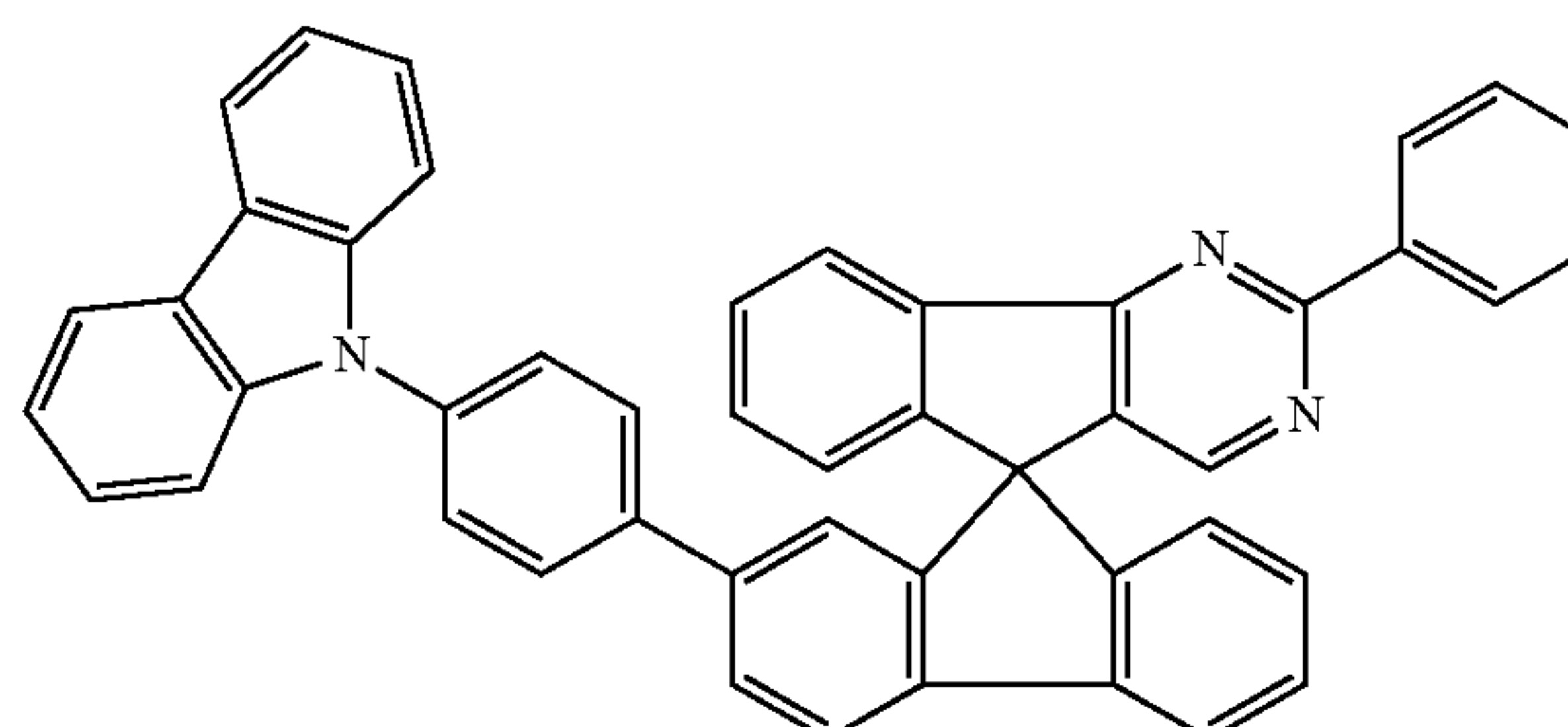
Chemical Formula 1-14
