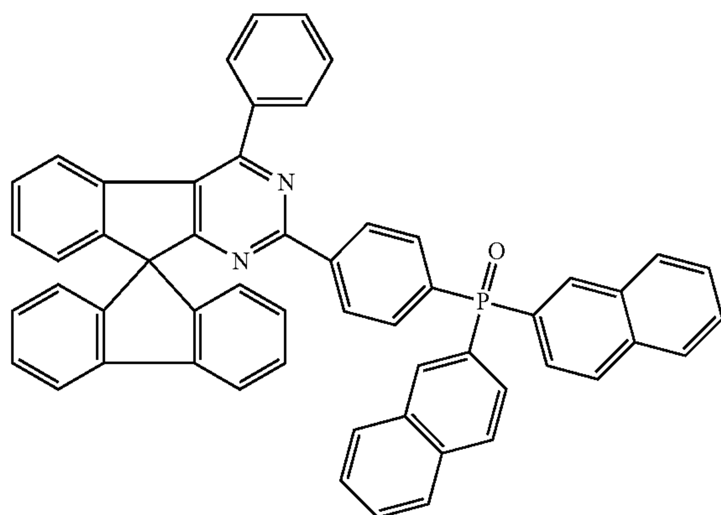
Chemical Formula 1-55
