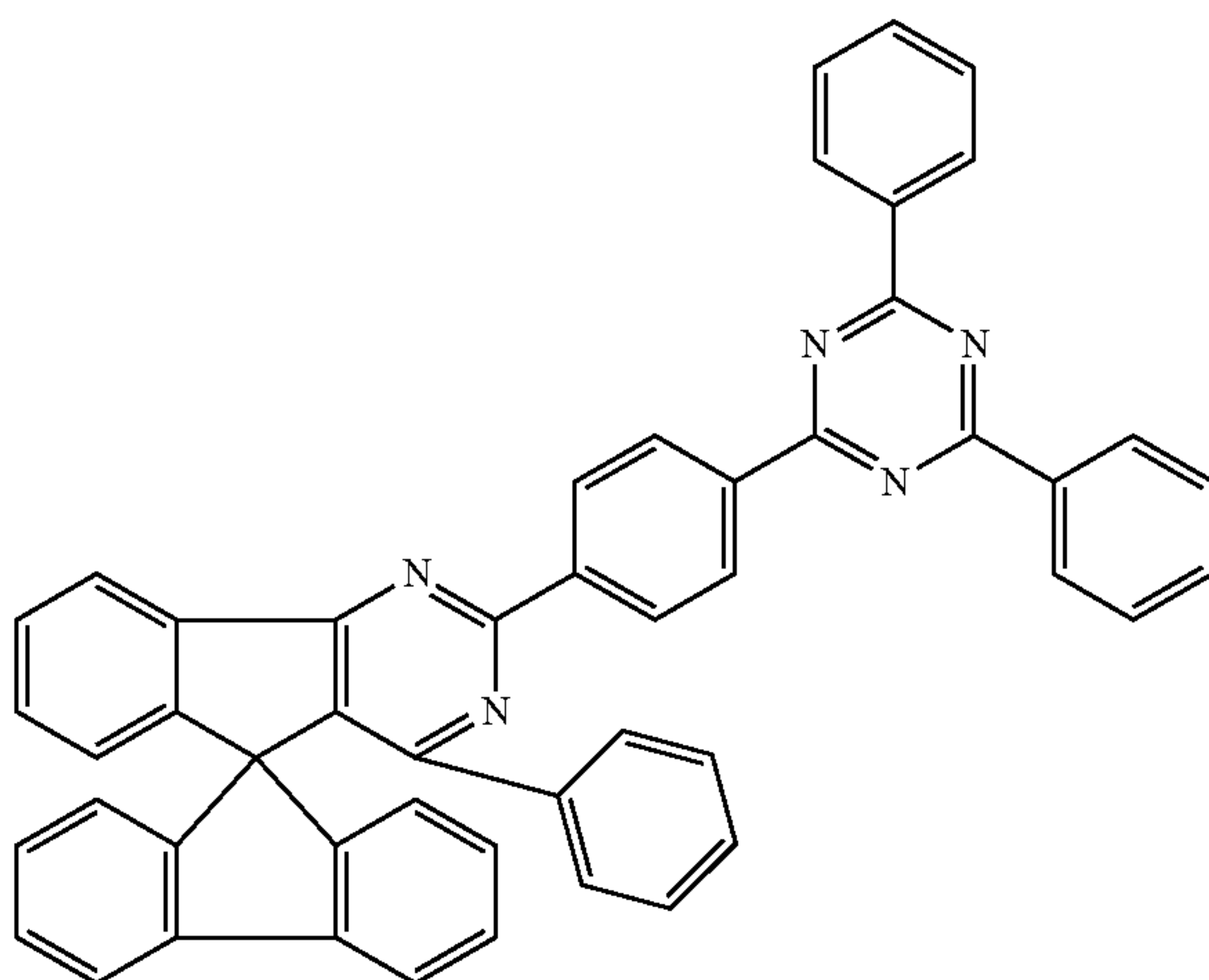
Chemical Formula 1-90
