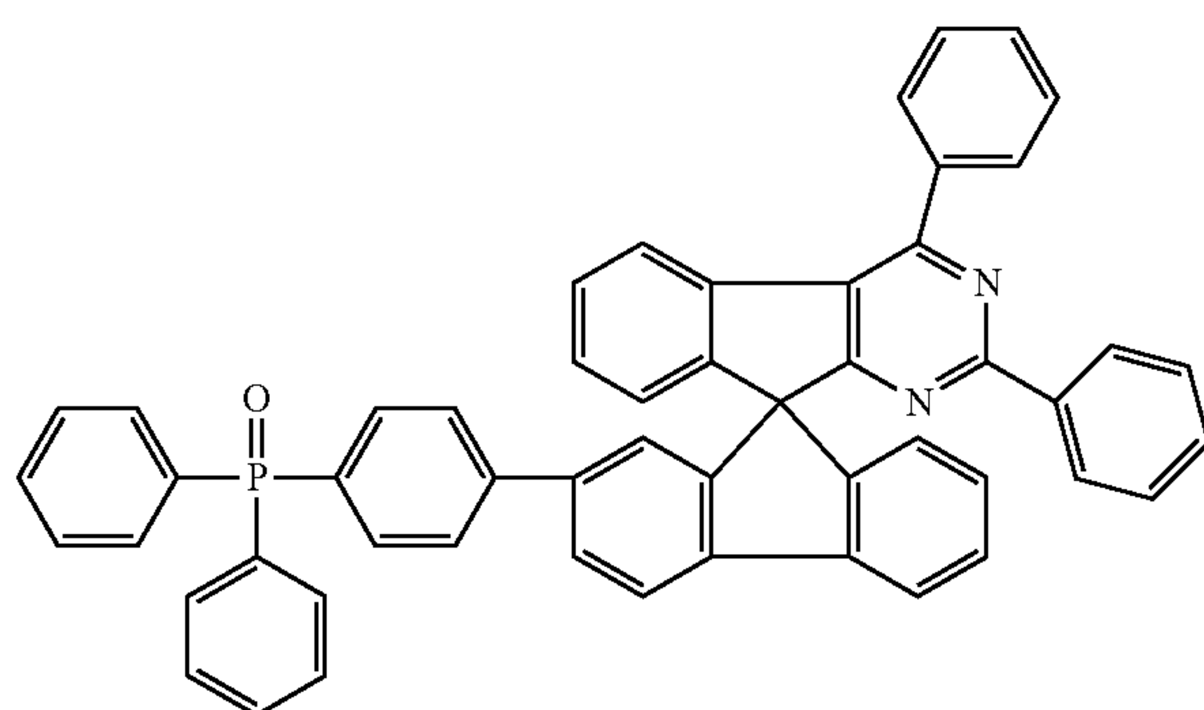
Chemical Formula 1-46
