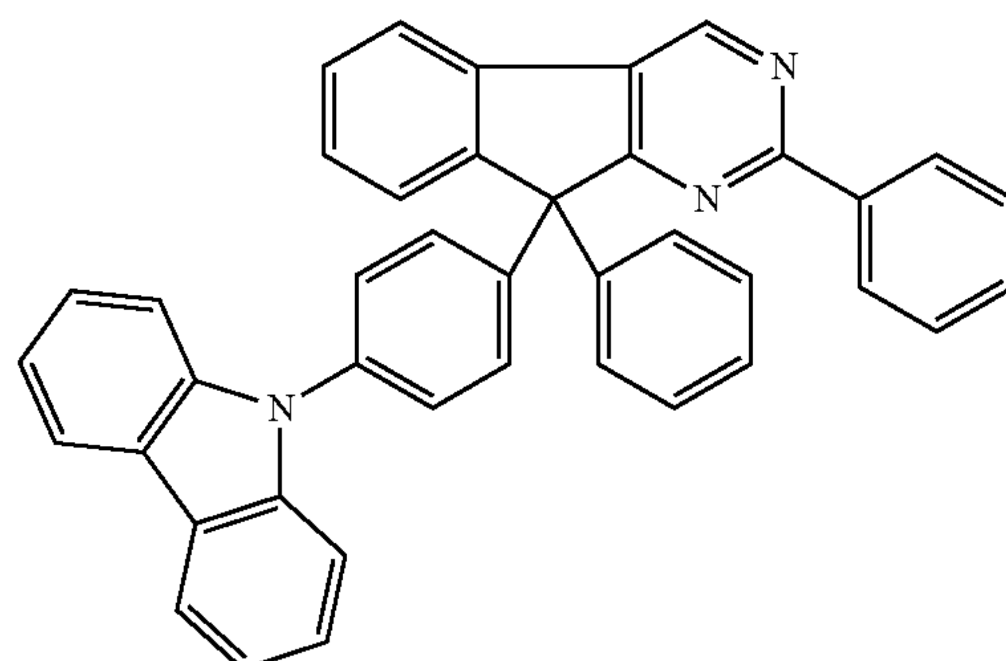
Chemical Formula 2-6
