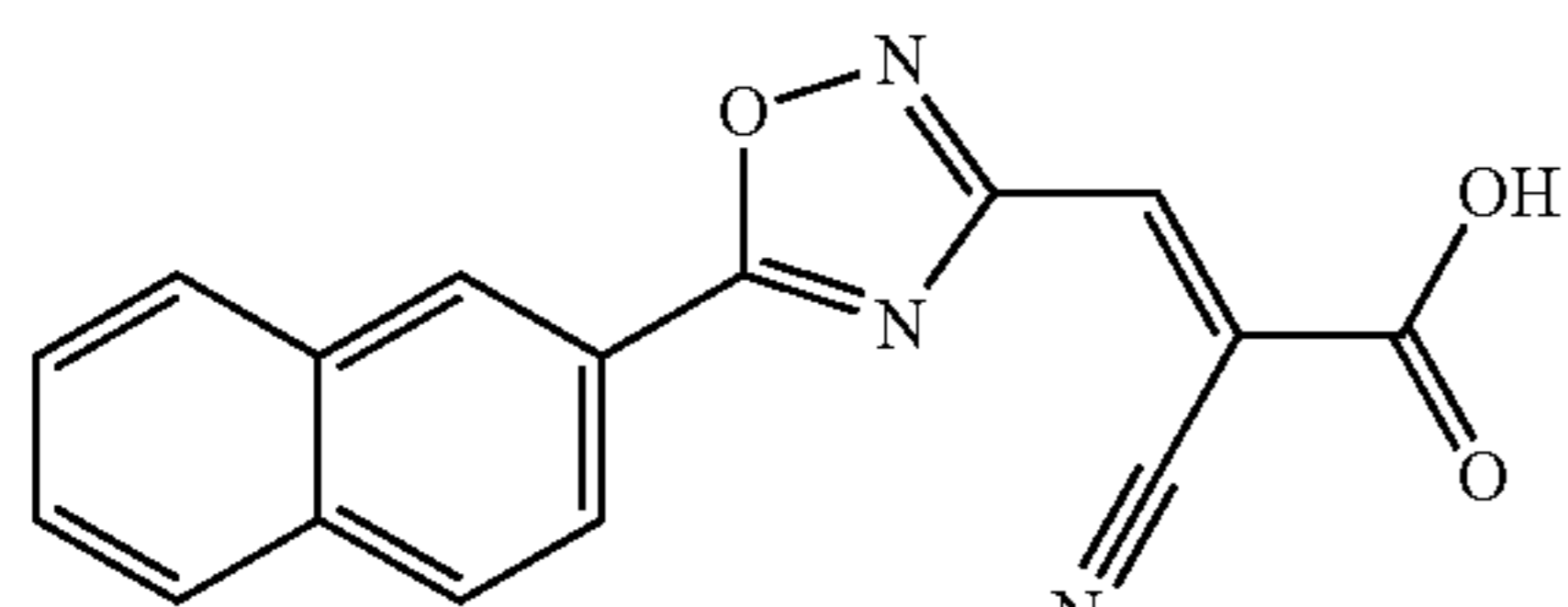
(E)-2-cyano-3-(5-(naphthalen-2-yl)-1,2,4-oxadiazol-3-yl)acrylic acid
