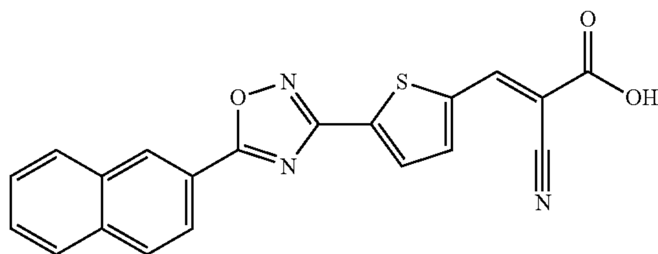
(E)-2-cyano-3-(5-(5-(naphthalen-2-yl)-1,2,4-oxadiazol-3-yl)thiophen-2-yl)cyanoacrylic acid
