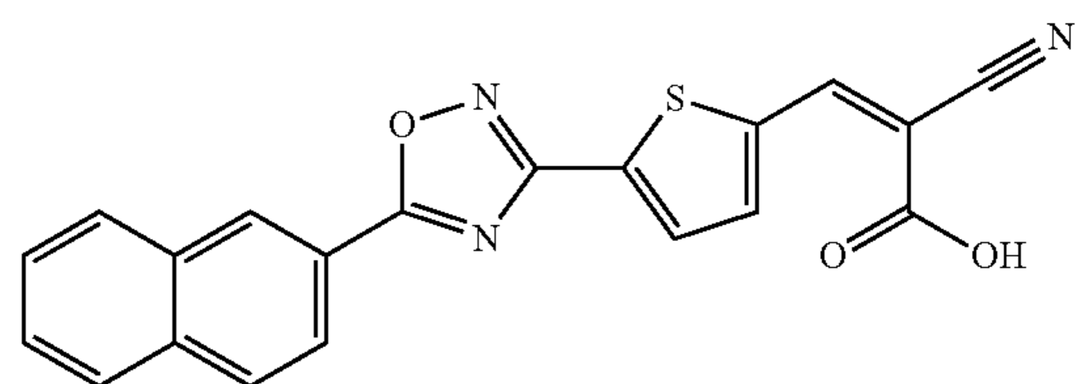
(Z)-2-cyano-3-(5-(5-(naphthalen-2-yl)-1,2,4-oxadiazol-3-yl)thiophen-2-yl)acrylic acid
