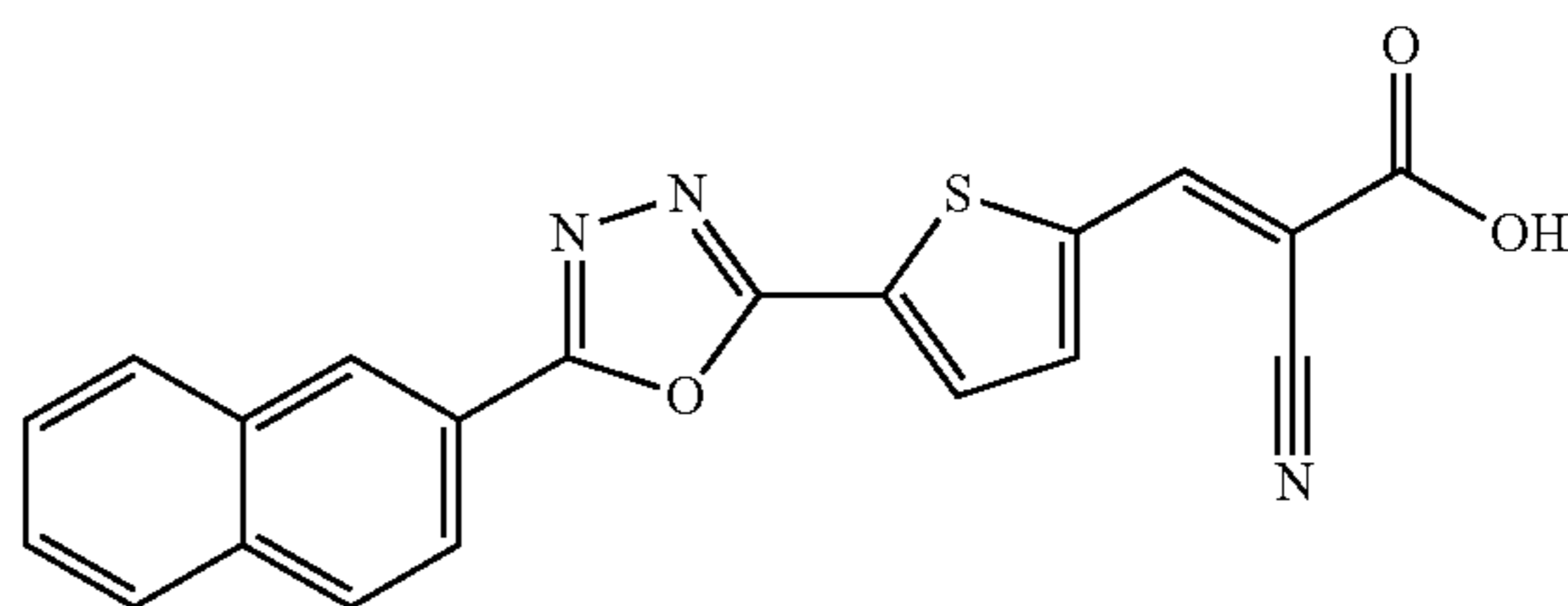
(E)-2-cyano-3-(5-(5-(naphthalen-2-yl)-1,3,4-oxadiazol-2-yl)thiophen-2-yl)cyanoacrylic acid
