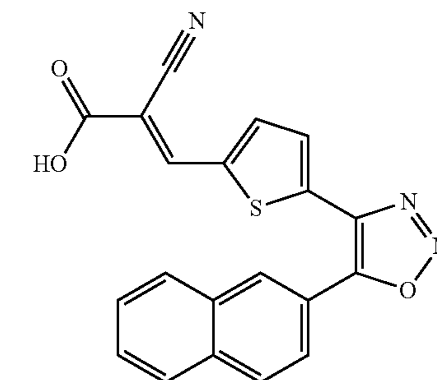
(E)-2-cyano-3-(5-(5-(naphthalen-2-yl)-1,2,3-oxadiazol-4-yl)thiophen-2-yl)cyanoacrylic acid
