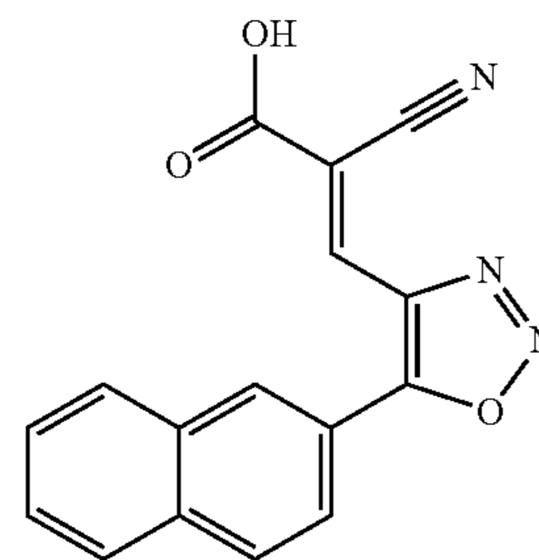
(E)-2-cyano-3-(5-naphthalen-2-yl)-1,2,3-oxadiazol-4-yl)-acrylic acid
