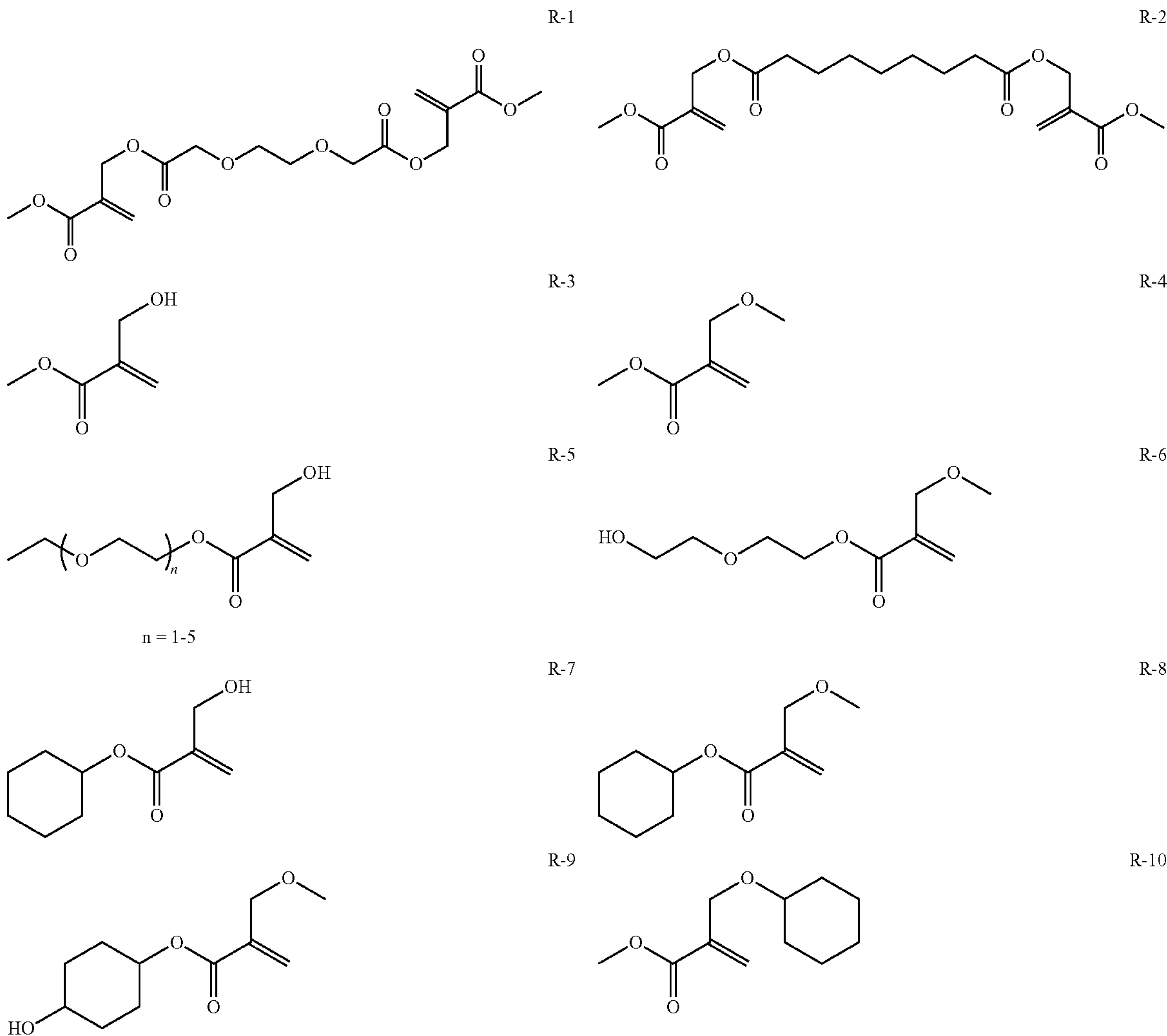
[Chemical Formula 6]
