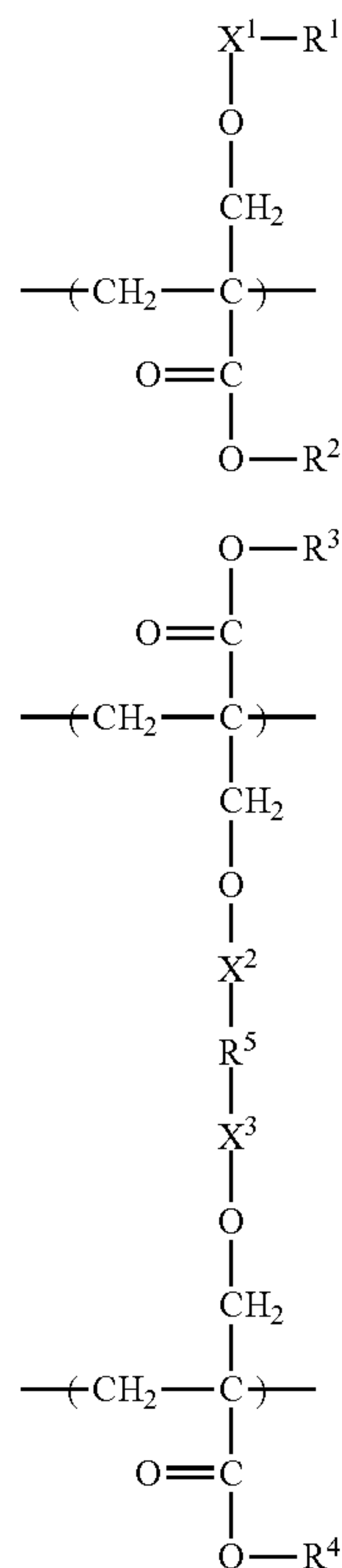
[Chemical Formula 1]
