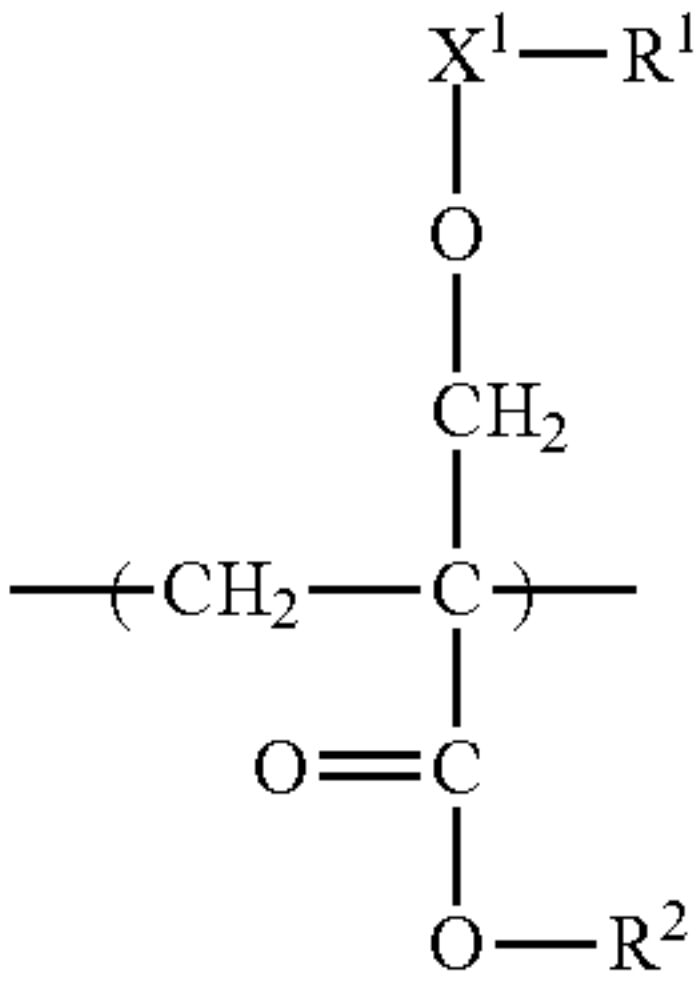
[Chemical Formula 1]
