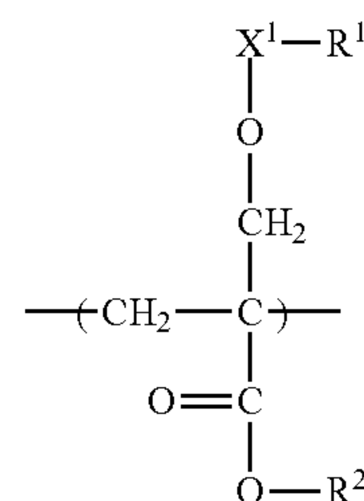
[Chemical Formula 3]
