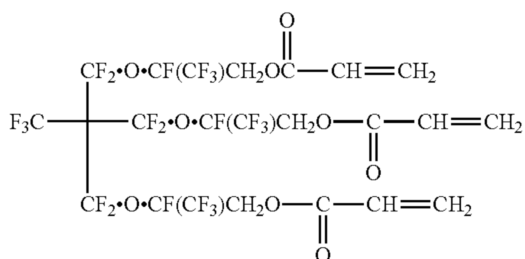
[Chemical Formula 2]
