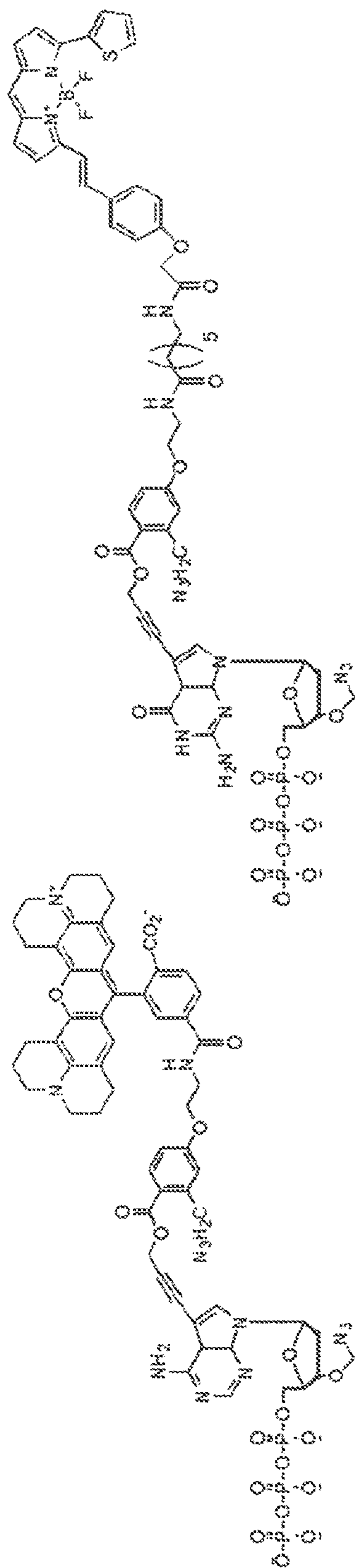
3'-O-Azido-dGTP-Azido-Bodipy650
