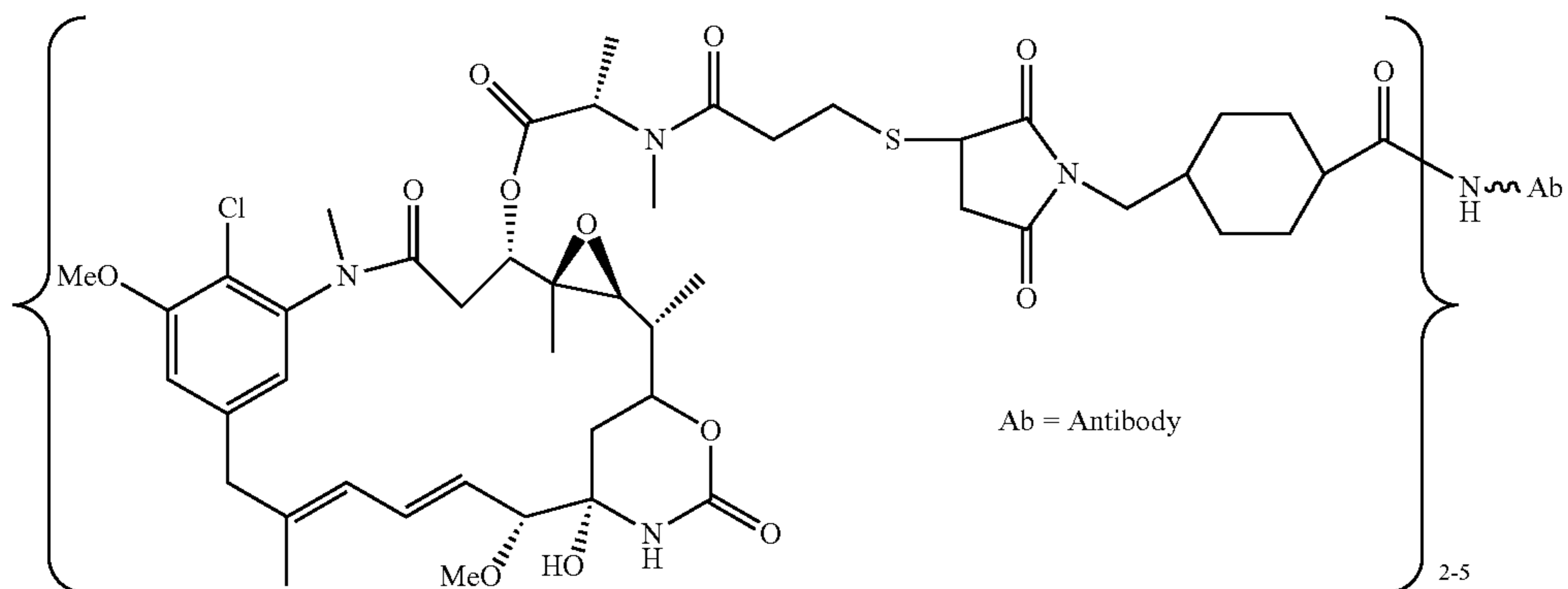
Ab-SMCC-DM1
