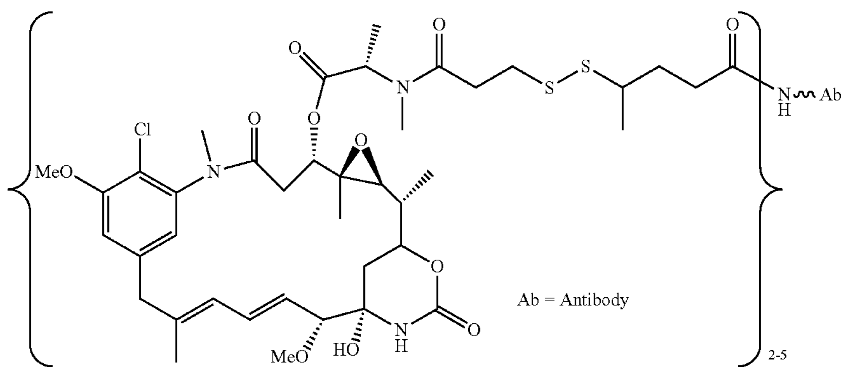
Ab-SPP-DM1
