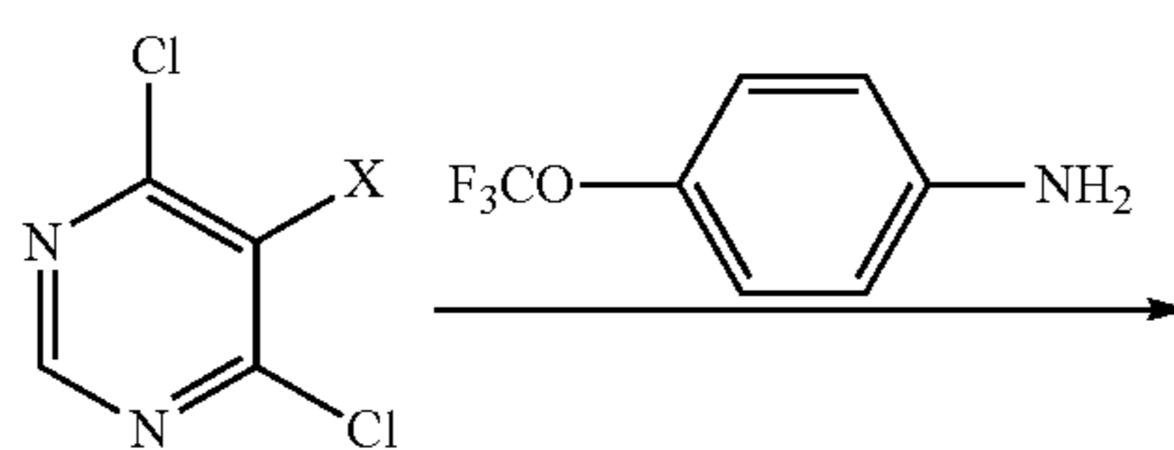
Scheme 5
