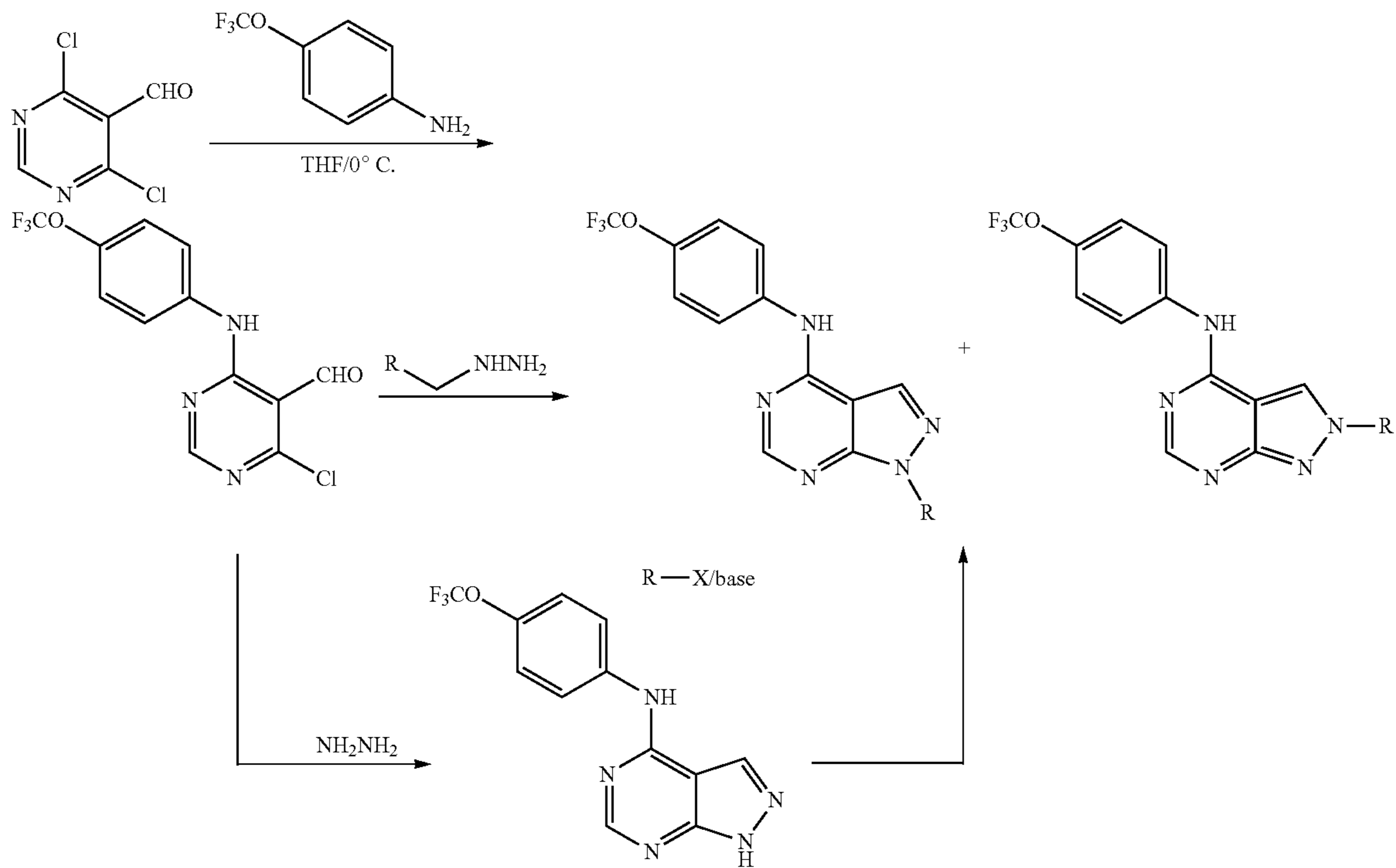
Scheme 1
