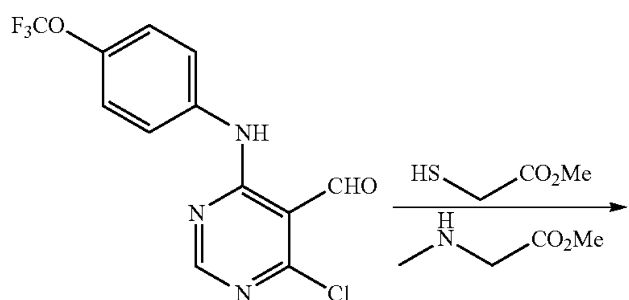
Scheme 3
