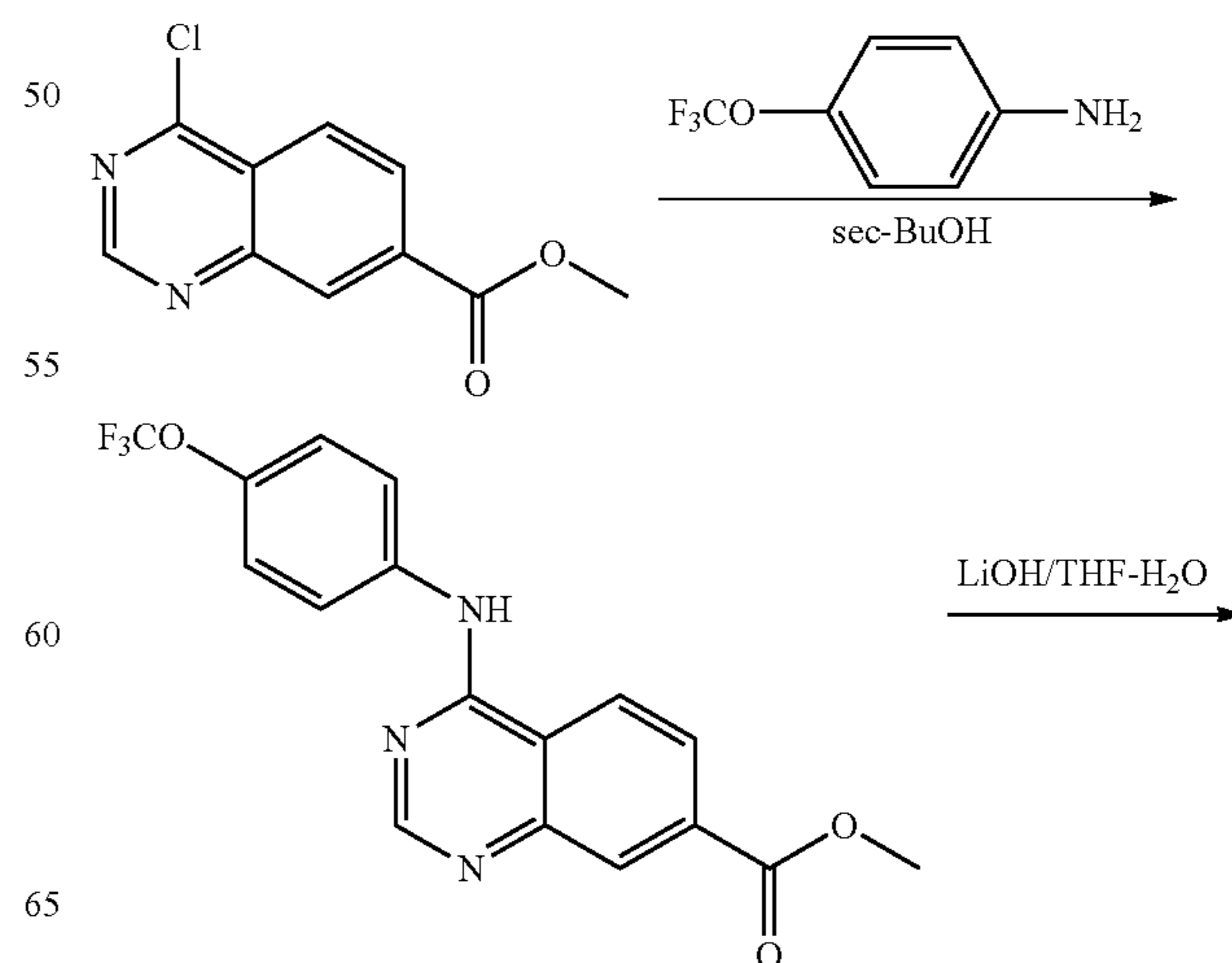
Scheme 4
