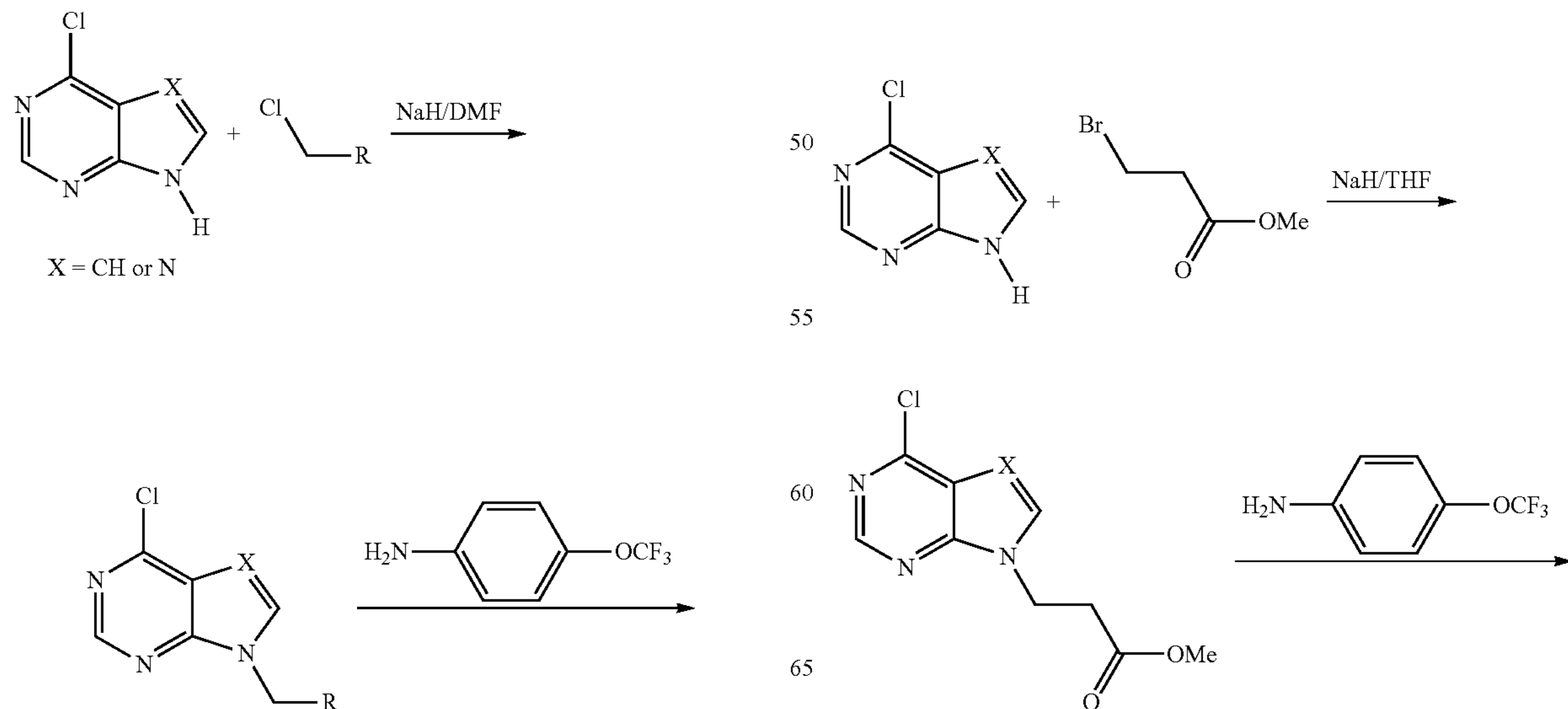
Scheme 2
