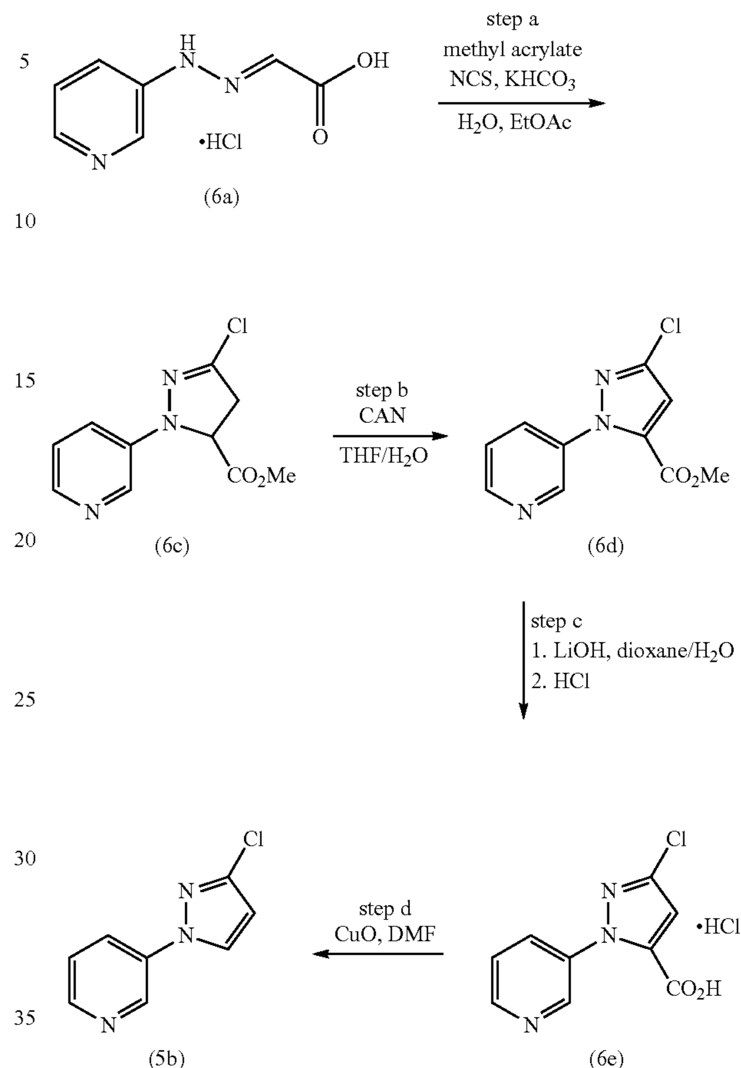
Scheme 2
