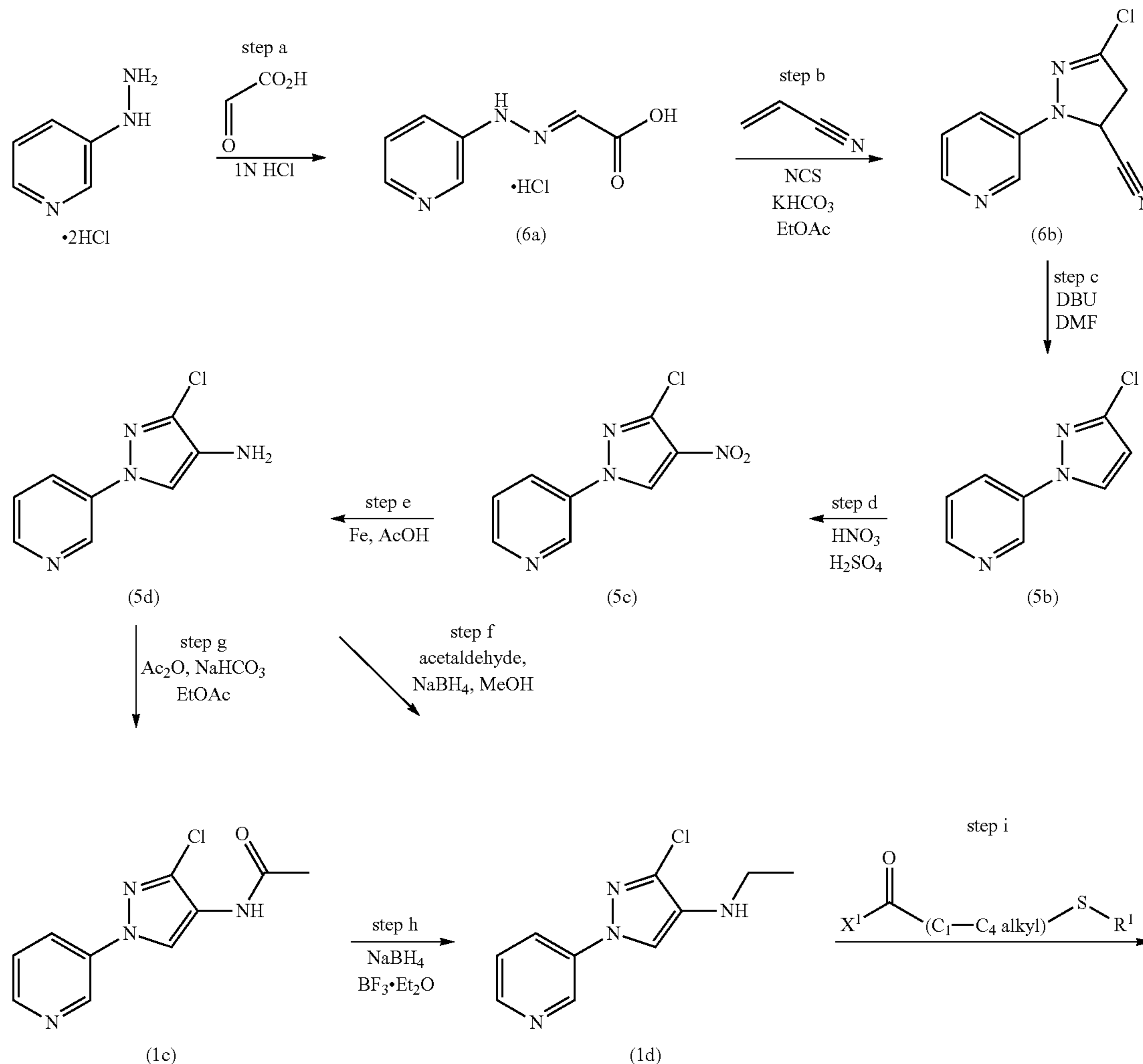
Scheme 1
