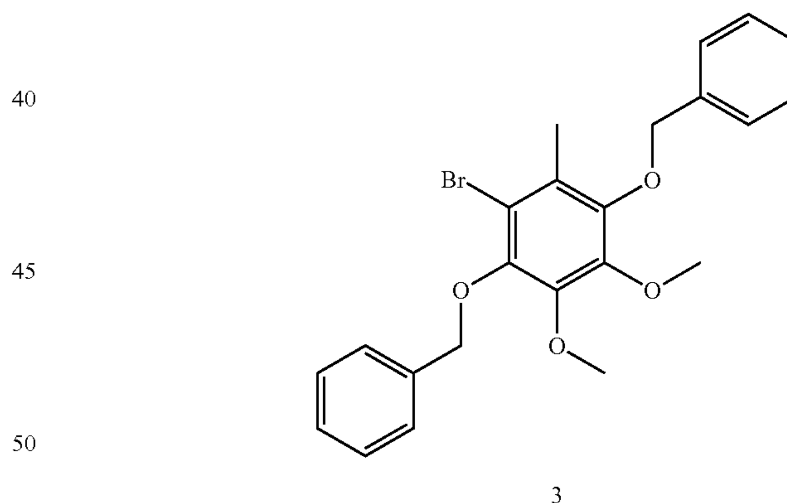
2-bromo-3,6-bis(benzyloxy)-4,5-dimethoxytoluene (3)
