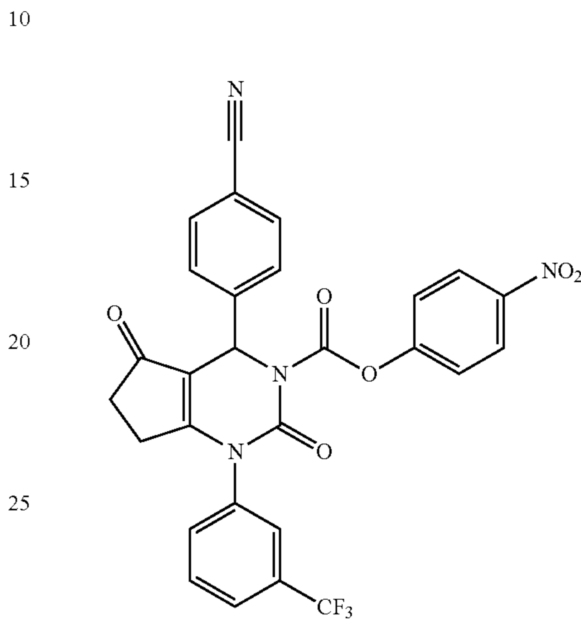
Intermediate 4
