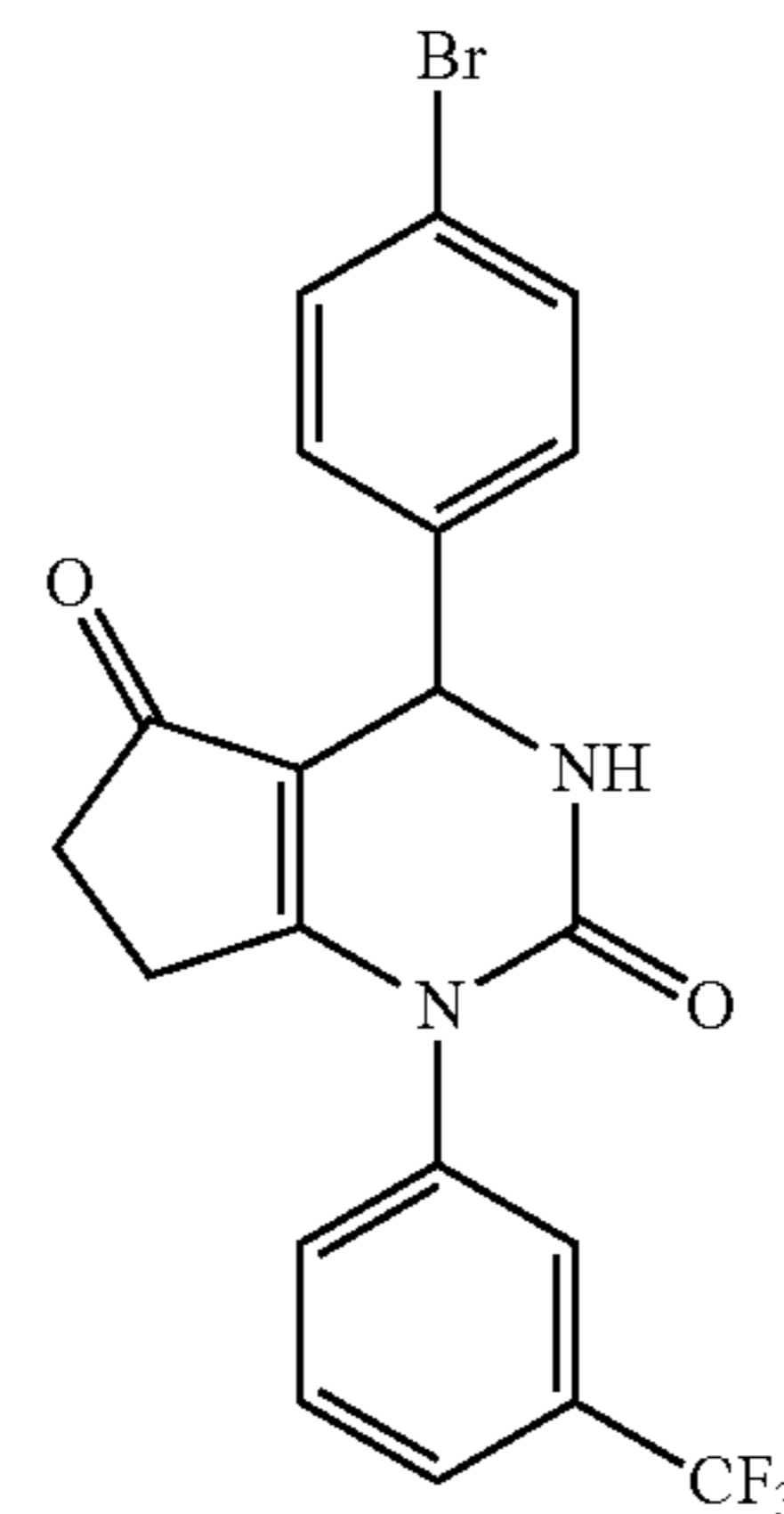
4-(4-Bromophenyl)-1-(3-(trifluoromethyl)phenyl)-3,4,6,7-tetrahydro-1H-cyclopenta[d]pyrimidine-2,5-dione
