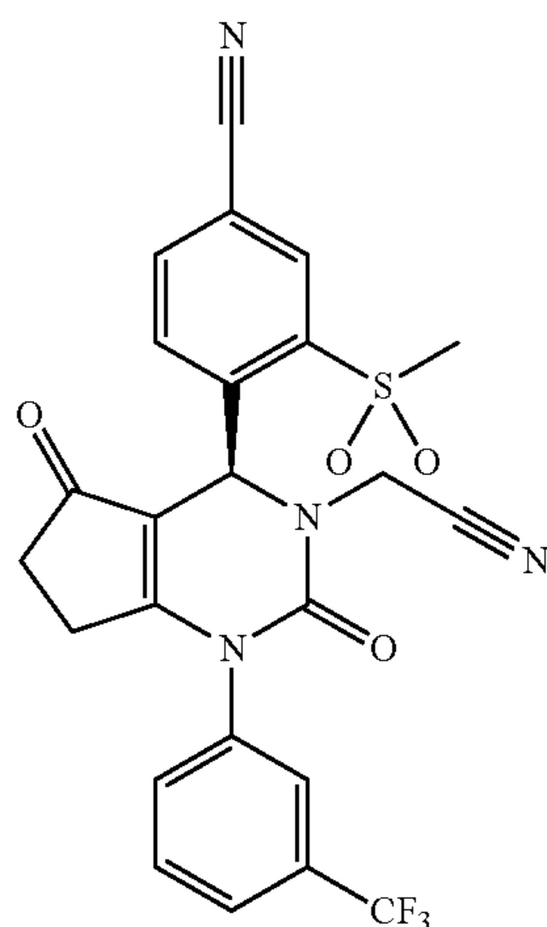
(S)-4-(3-(Cyanomethyl)-2,5-dioxo-1-(3-(trifluoromethyl)phenyl)-2,3,4,5,6,7-hexahydro-1H-cyclopenta[d]pyrimidin-4-yl)-3-(methylsulfonyl)benzonitrile
