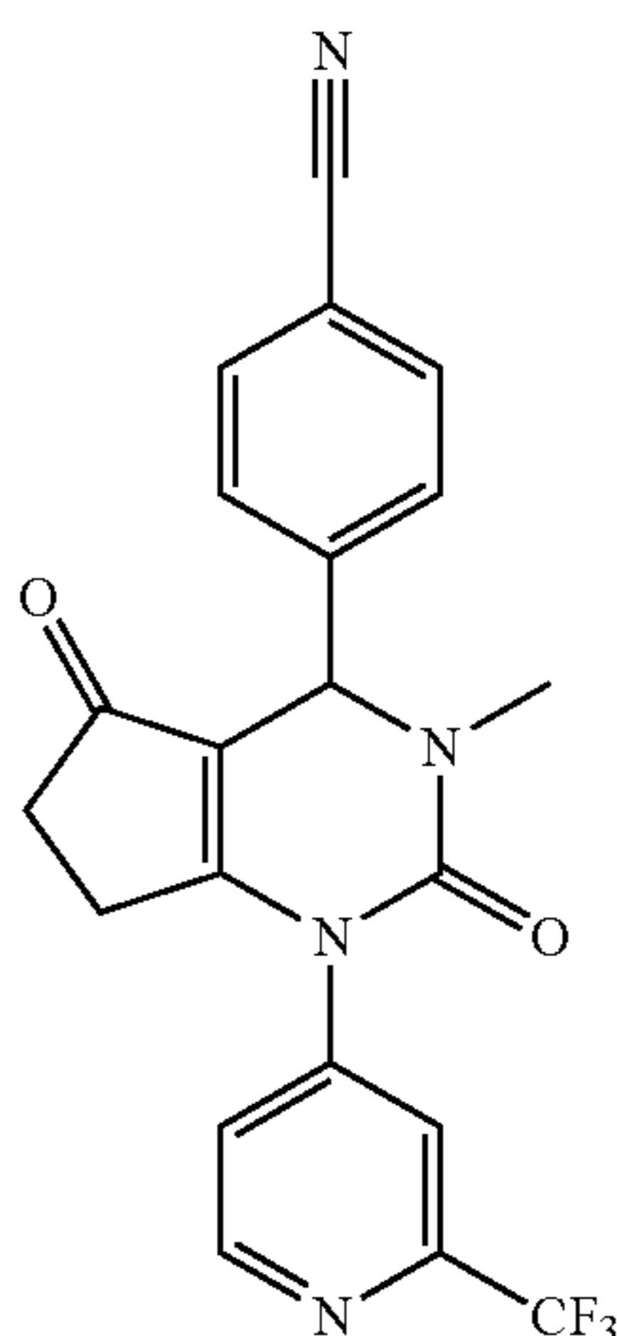
4-(3-Methyl-2,5-dioxo-1-(2-(trifluoromethyl)pyridin-4-yl)-2,3,4,5,6,7-hexahydro-1H-cyclopenta[d]pyrimidin-4-yl)benzonitrile
