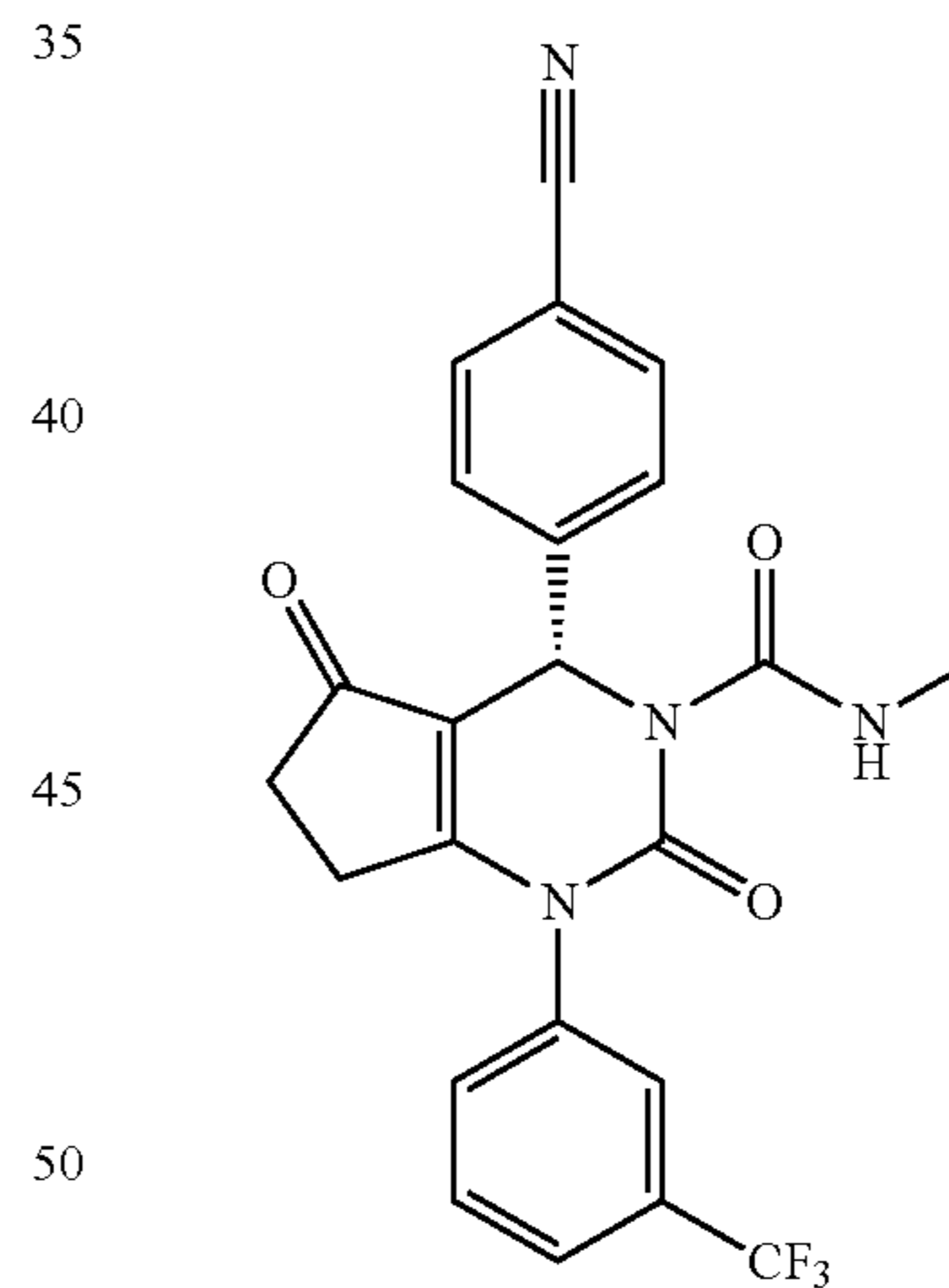
(S)-4-(4-Cyanophenyl)-N-methyl-2,5-dioxo-1-(3-(trifluoromethyl)phenyl)-4,5,6,7-tetrahydro-1H-cyclopenta[d]pyrimidine-3(2H)-carboxamide
