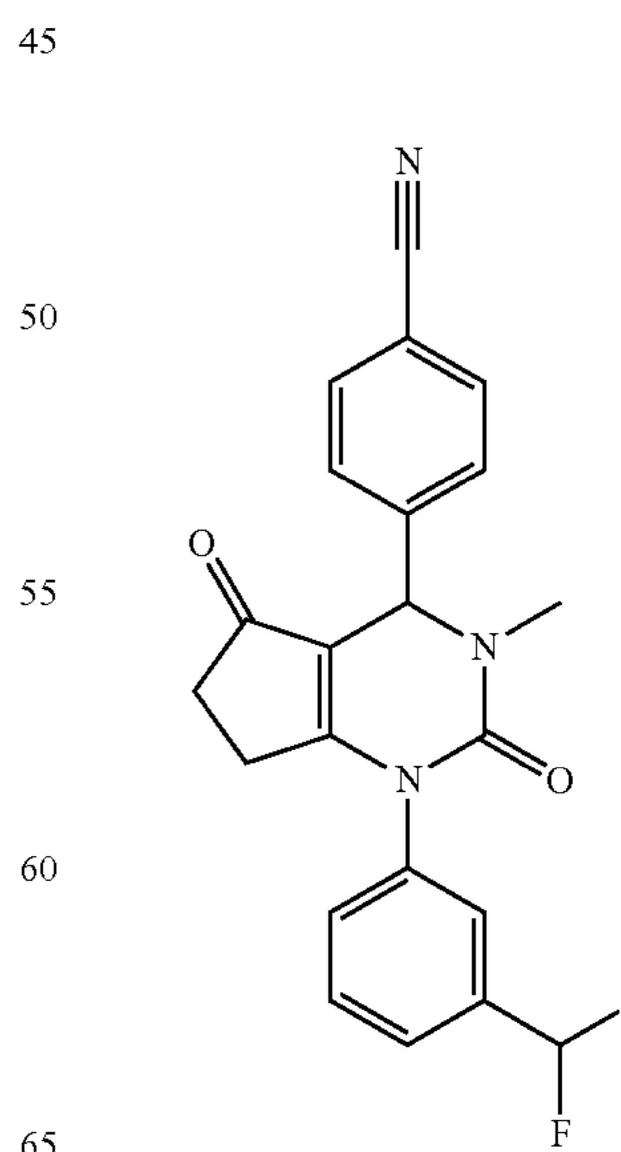
Example 26
