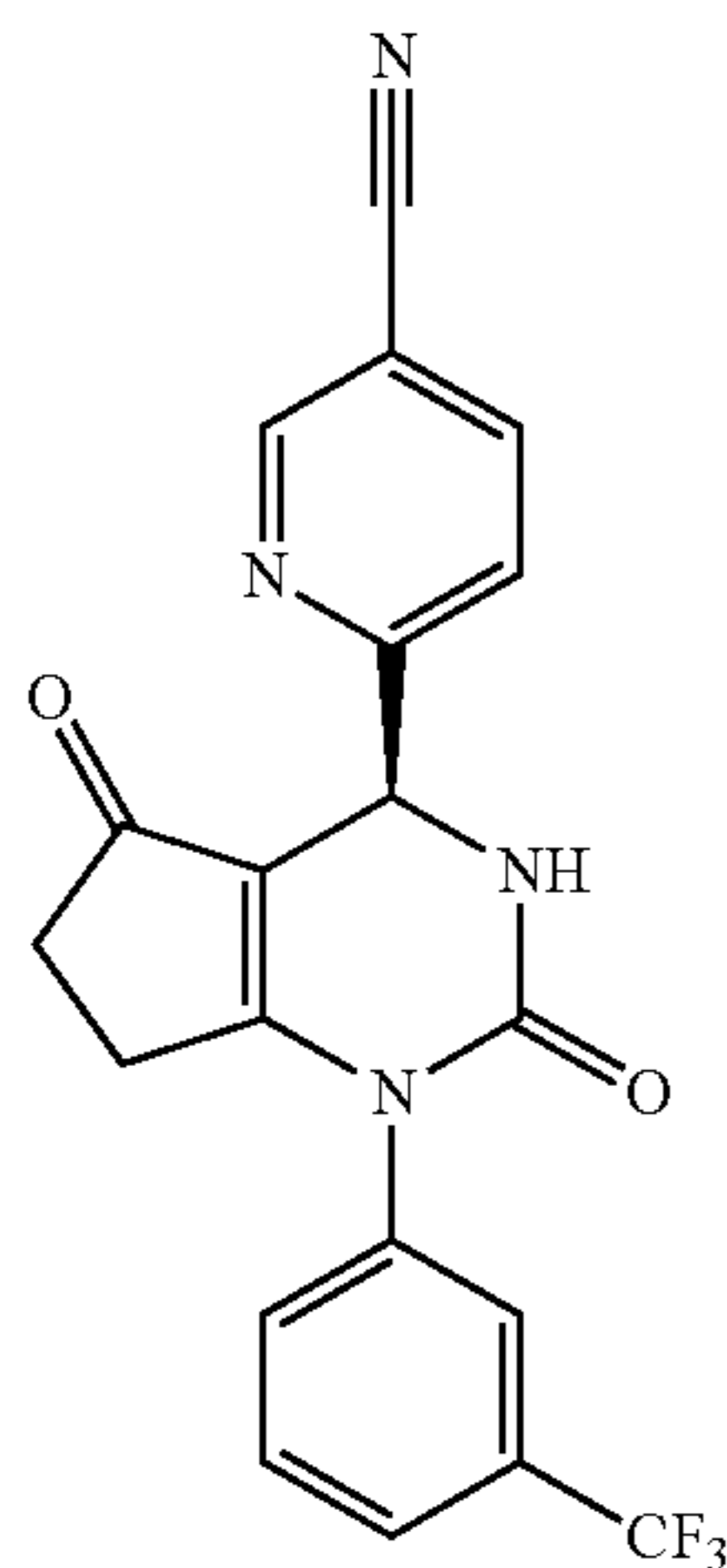
(S)-6-(2,5-Dioxo-1-(3-(trifluoromethyl)phenyl)-2,3,4,5,6,7-hexahydro-1H-cyclopenta[d]pyrimidin-4-yl)nicotinonitrile
