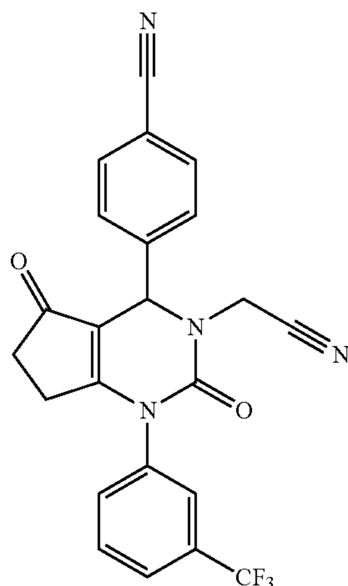
4-(3-(Cyanomethyl)-2,5-dioxo-1-(3-(trifluoromethyl)phenyl)-2,3,4,5,6,7-hexahydro-1H-cyclopenta[d]pyrimidin-4-yl)benzonitrile
