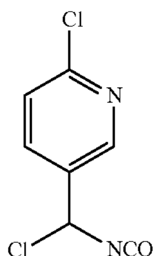
2-Chloro-5-(chloro(isocyanato)methyl)pyridine
