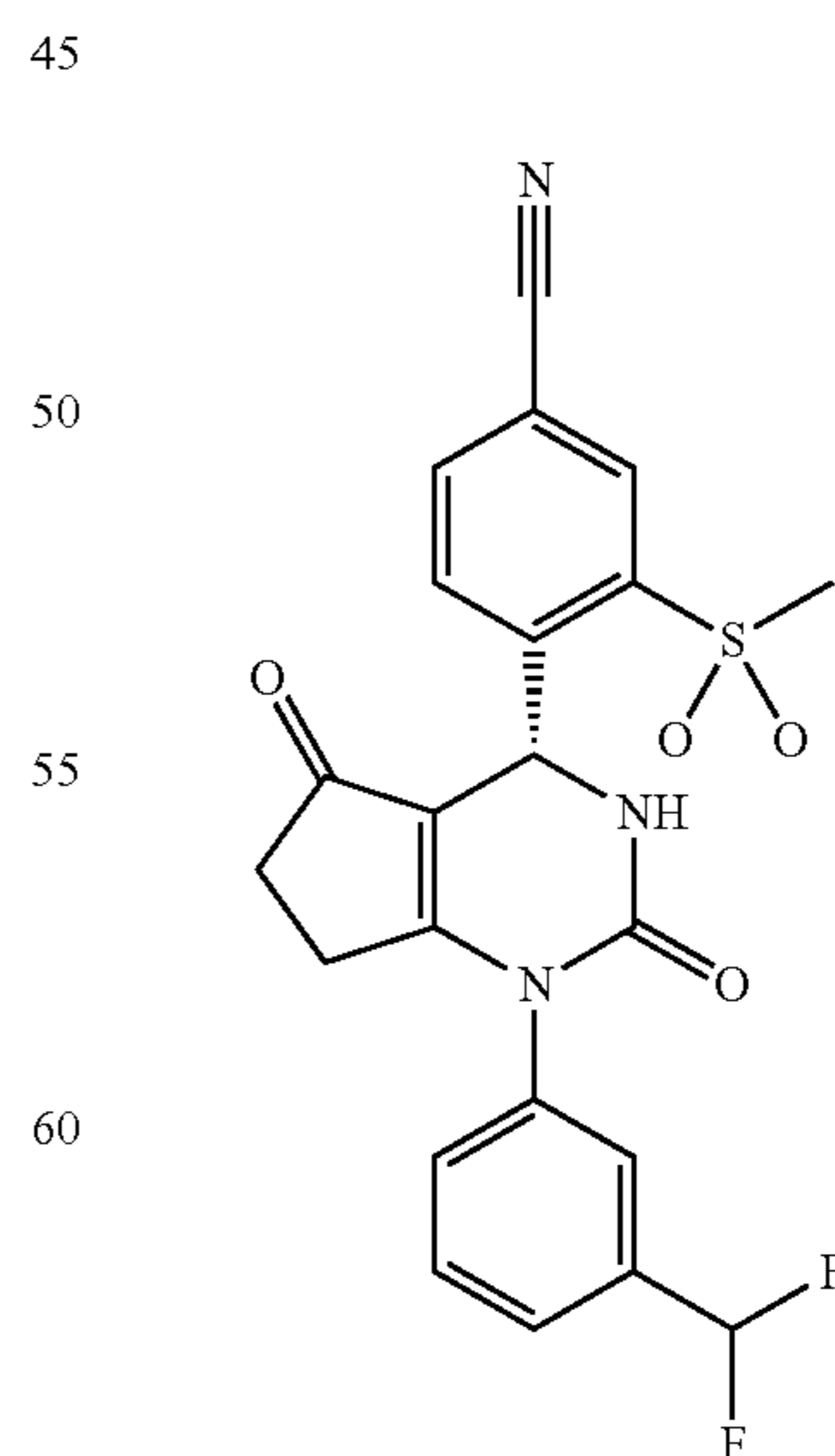
(R)-6-(2,5-Dioxo-1-(3-(trifluoromethyl)phenyl)-2,3,4,5,6,7-hexahydro-1H-cyclopenta[d]pyrimidin-4-yl)nicotinonitrile
