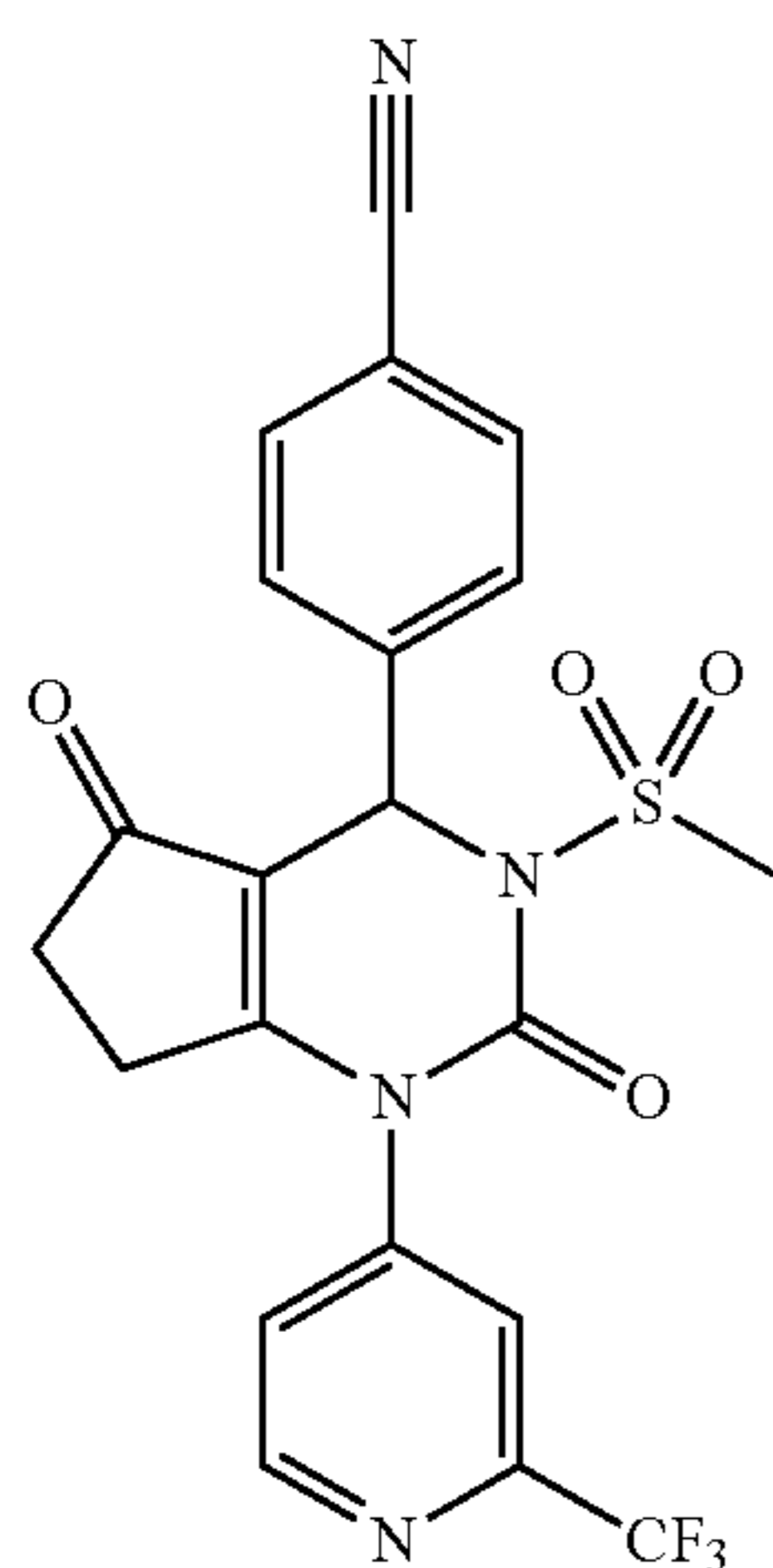
4-(3-(Methylsulfonyl)-2,5-dioxo-1-(2-(trifluoromethyl)pyridin-4-yl)-2,3,4,5,6,7-hexahydro-1H-cyclopenta[d]pyrimidin-4-yl)benzonitrile
