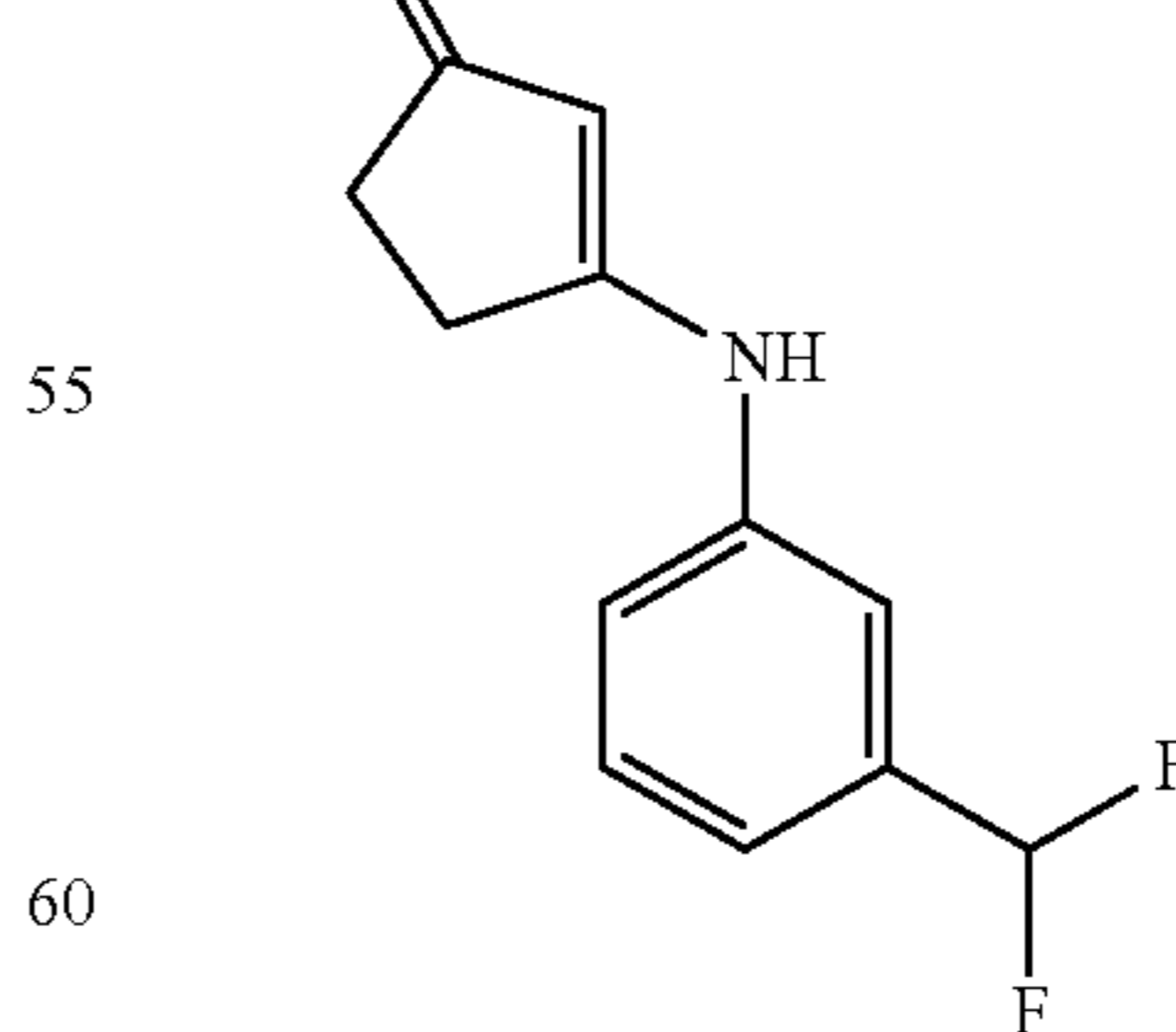
3-(3-(Difluoromethyl)phenylamino)cyclopent-2-enone
