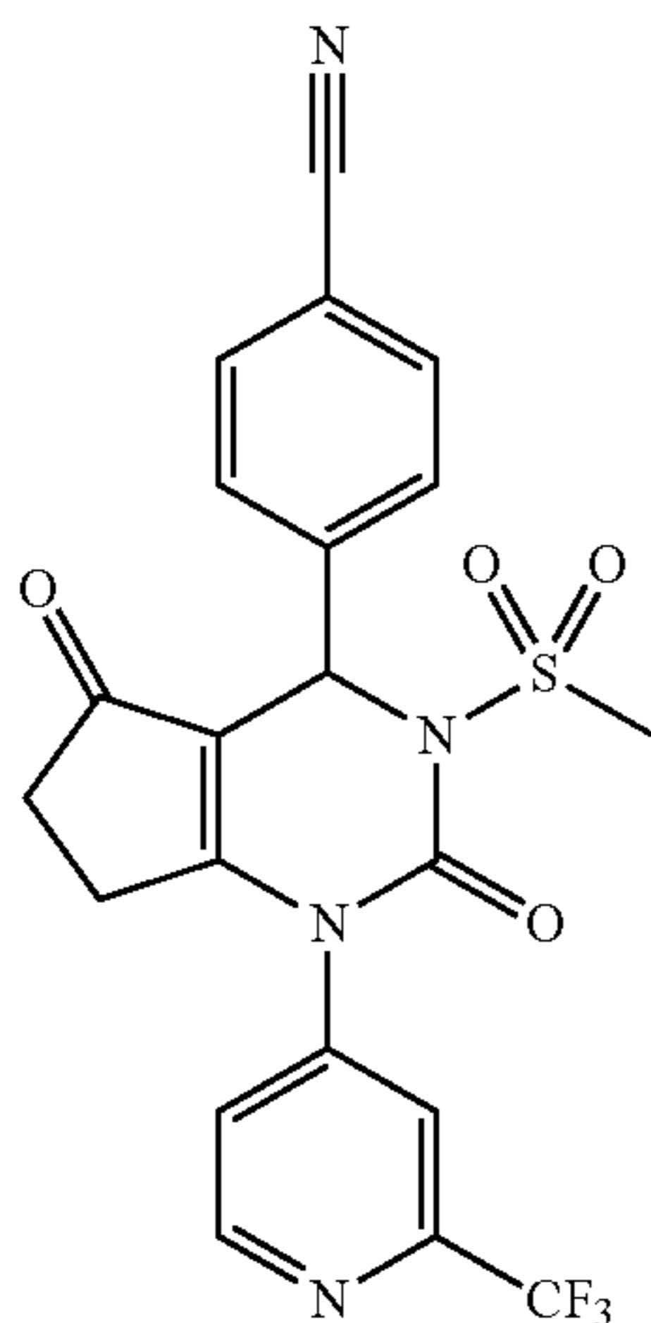
4-(3-(Methylsulfonyl)-2,5-dioxo-1-(2-(trifluoromethyl)pyridin-4-yl)-2,3,4,5,6,7-hexahydro-1H-cyclopenta[d]pyrimidin-4-yl)benzonitrile
