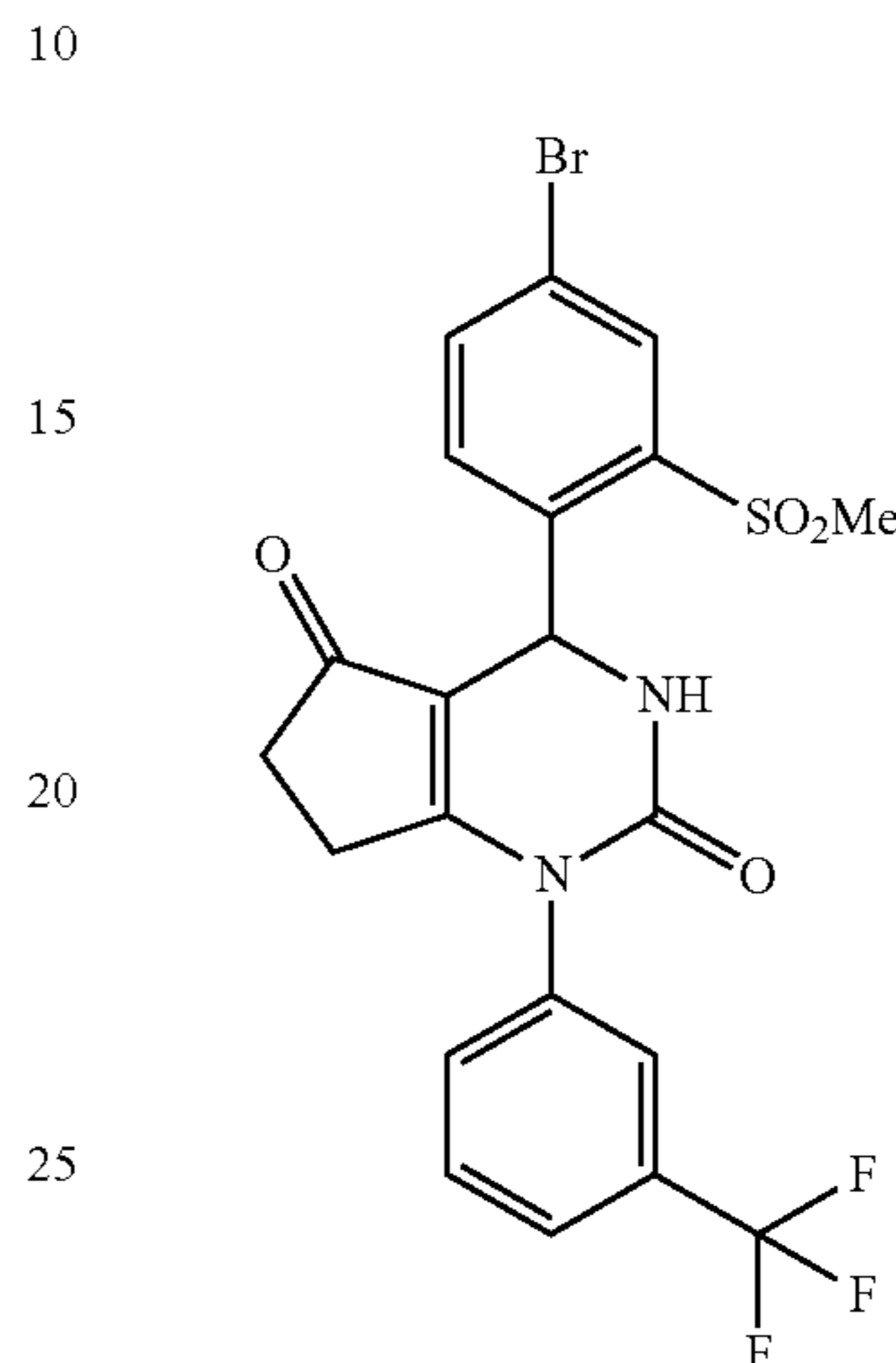
Intermediate 8
