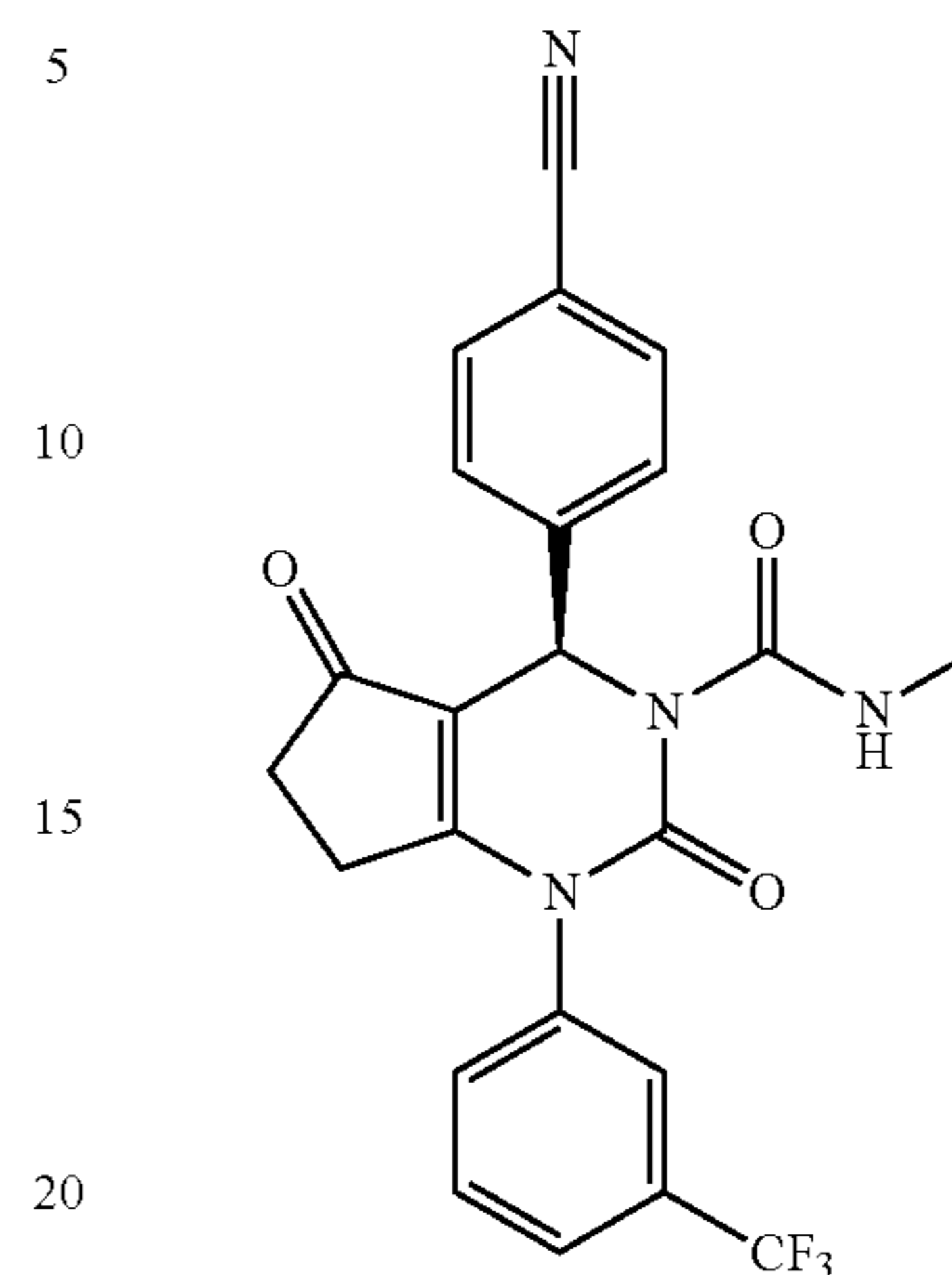
(R)-4-(4-Cyanophenyl)-N-methyl-2,5-dioxo-1-(3-(trifluoromethyl)phenyl)-4,5,6,7-tetrahydro-1H-cyclopenta[d]pyrimidine-3(2H)-carboxamide
