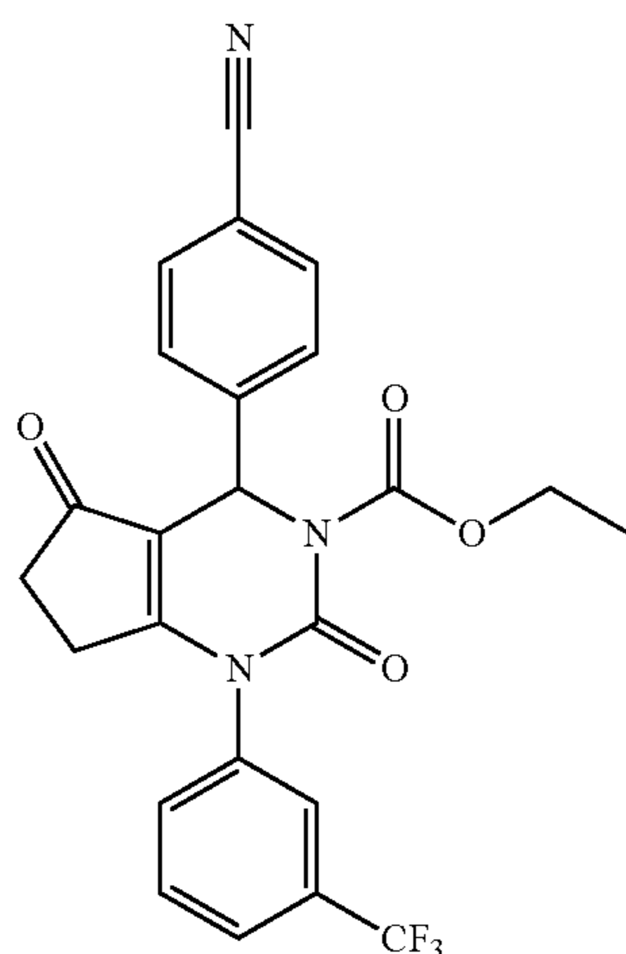
Ethyl 4-(4-Cyanophenyl)-2,5-dioxo-1-(3-(trifluoromethyl)phenyl)-4,5,6,7-tetrahydro-1H-cyclopenta[d]pyrimidine-3(2H)-carboxylate
