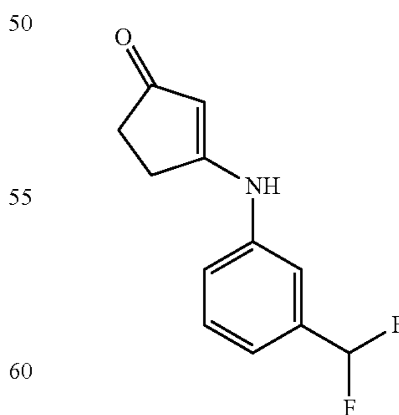
3-(3-(Difluoromethyl)phenylamino)cyclopent-2-enone
