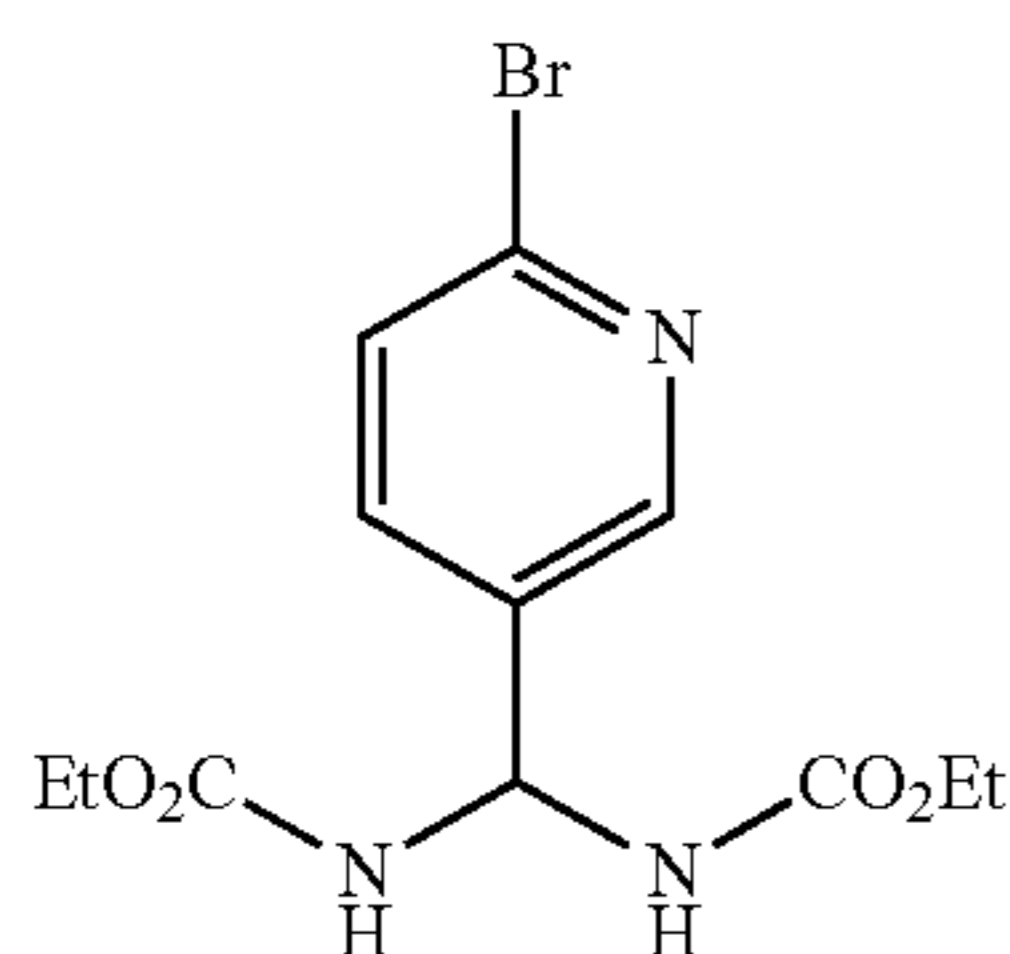
Diethyl(6-Bromopyridin-3-yl)methylenedicarbamate
