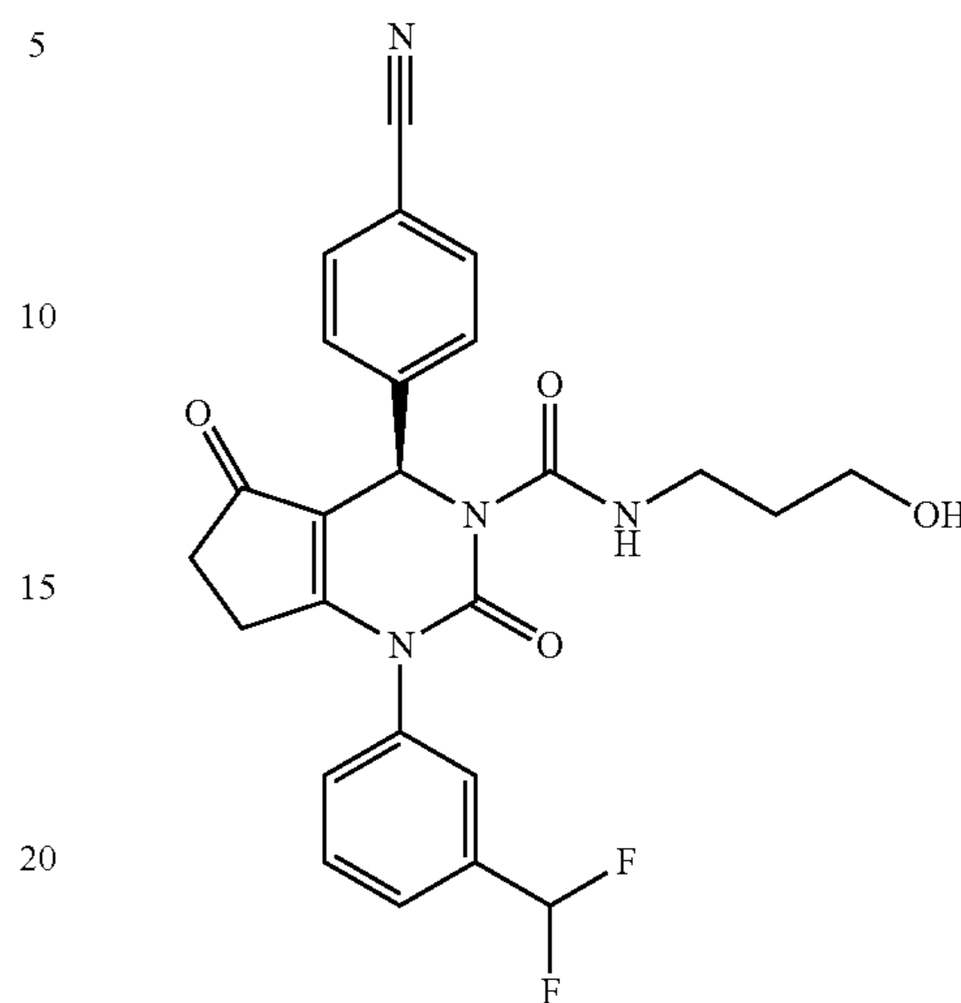
(R)-4-(4-Cyanophenyl)-1-(3-(difluoromethyl)phenyl)-N-(3-hydroxypropyl)-2,5-dioxo-4,5,6,7-tetrahydro-1H-cyclopenta[d]pyrimidine-3(2H)-carboxamide
