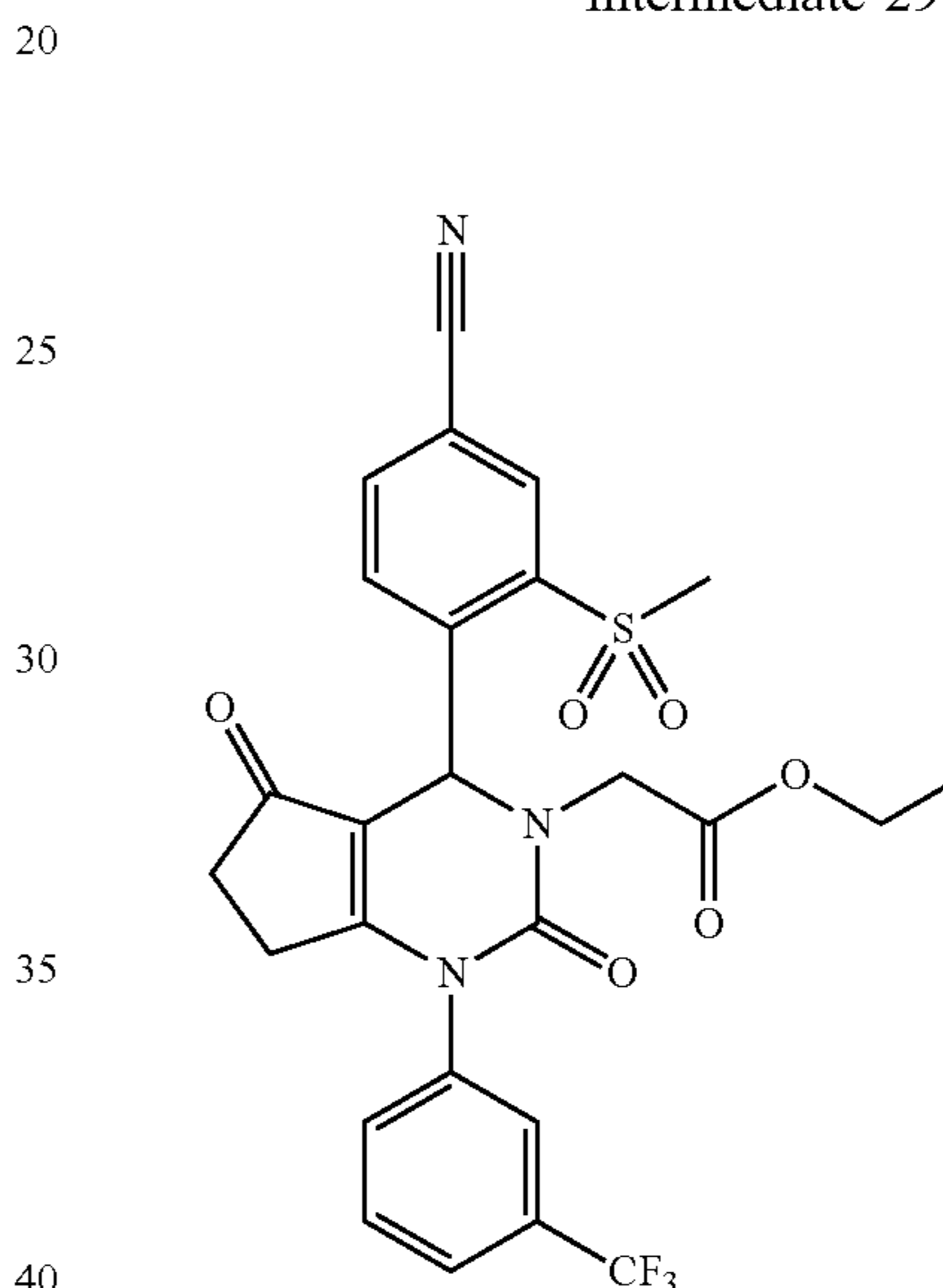
Intermediate 29
