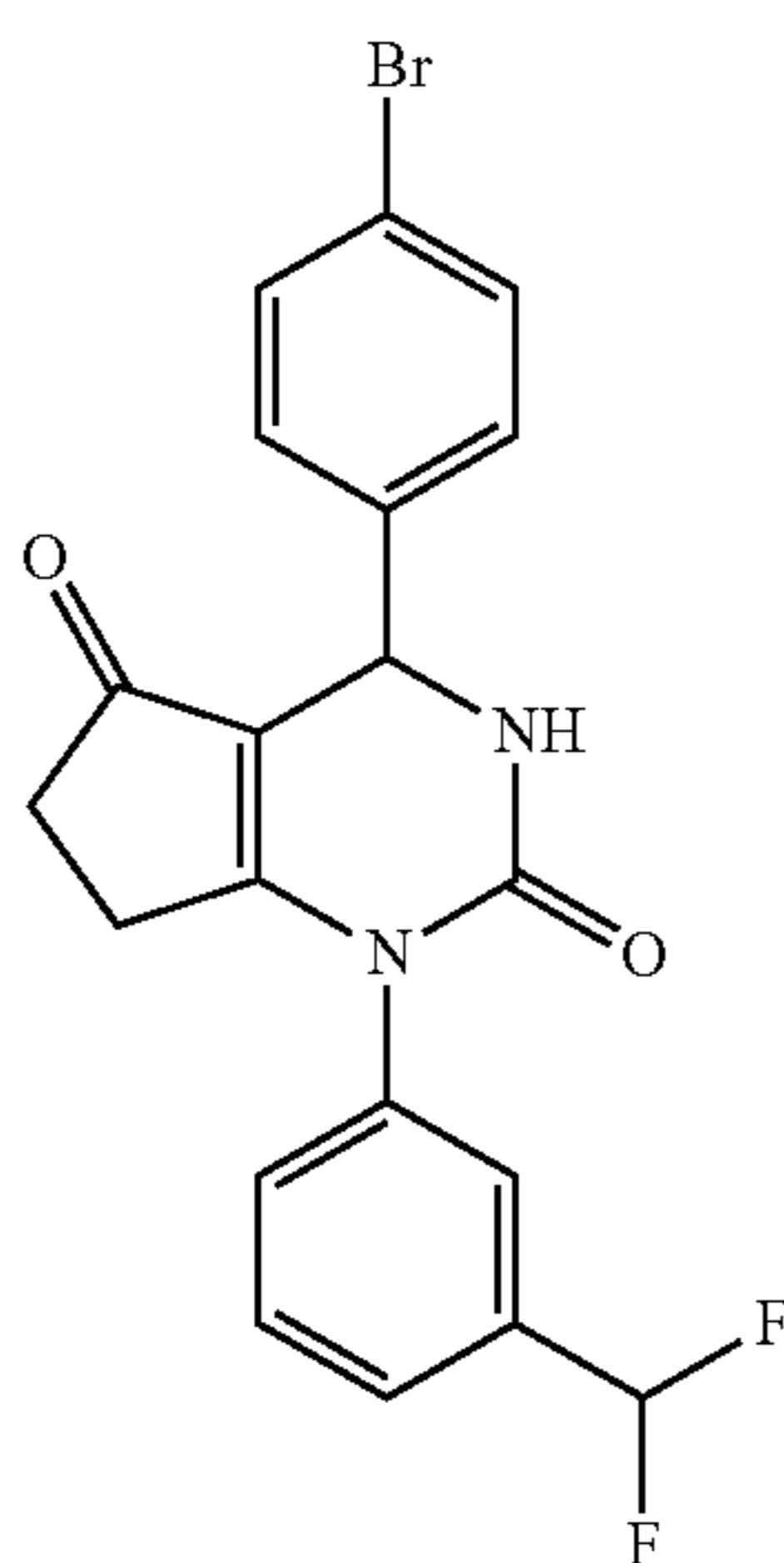
4-(4-Bromophenyl)-1-(3-(difluoromethyl)phenyl)-3,4,6,7-tetrahydro-1H-cyclopenta[d]pyrimidine-2,5-dione
