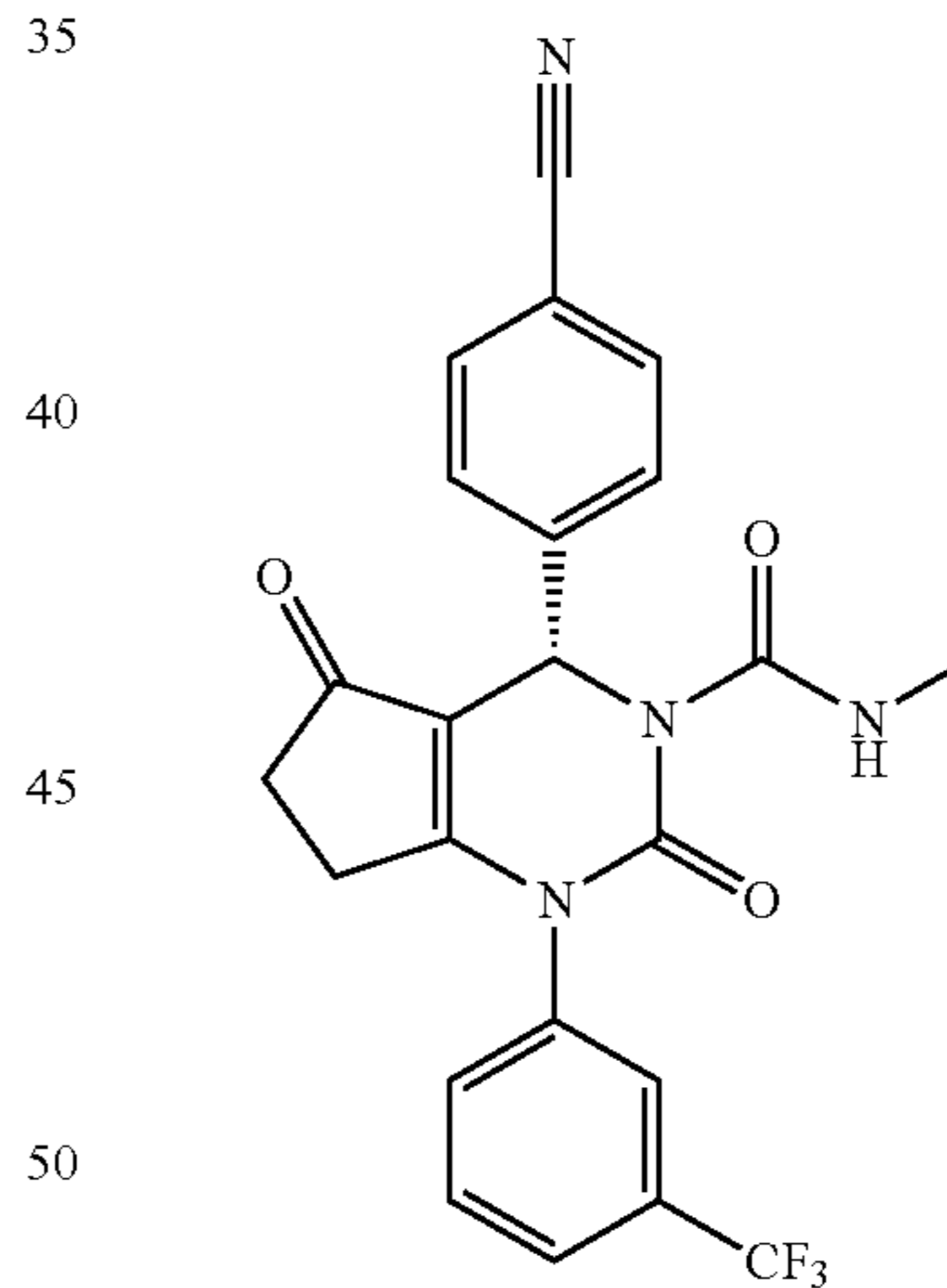
(S)-4-(4-Cyanophenyl)-N-methyl-2,5-dioxo-1-(3-(trifluoromethyl)phenyl)-4,5,6,7-tetrahydro-1H-cyclopenta[d]pyrimidine-3(2H)-carboxamide
