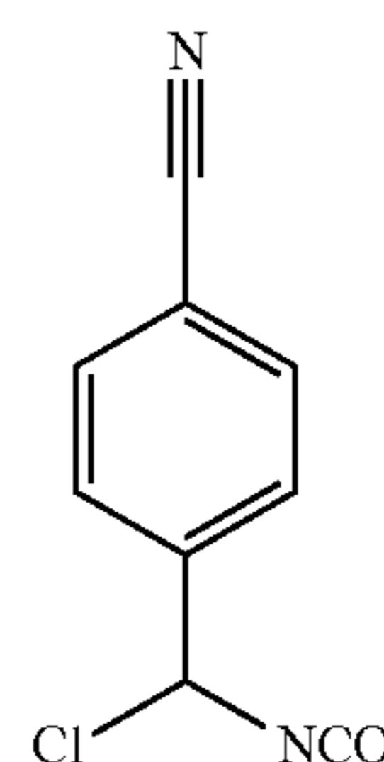
4-(Chloro(isocyanato)methyl)benzotrile
