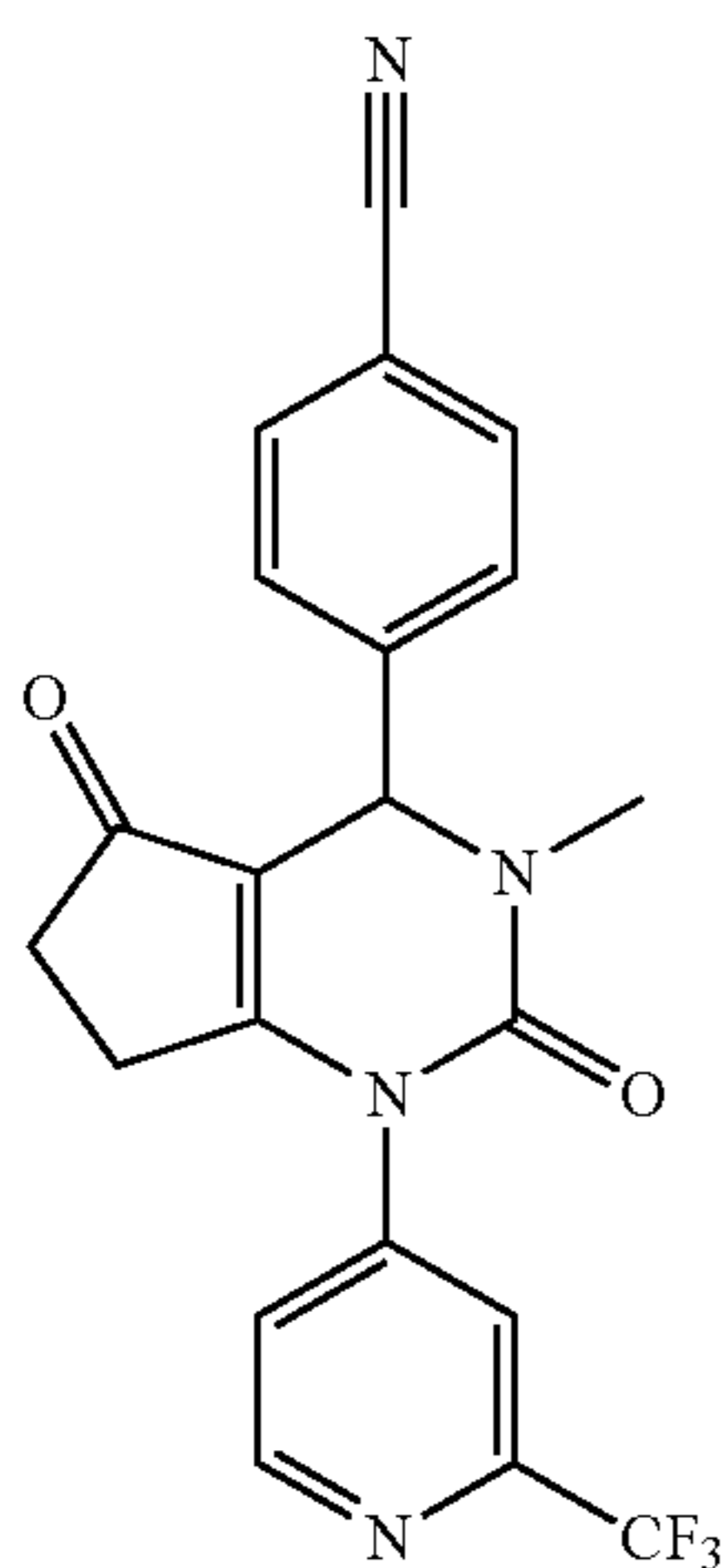
4-(3-Methyl-2,5-dioxo-1-(2-(trifluoromethyl)pyridin-4-yl)-2,3,4,5,6,7-hexahydro-1H-cyclopenta[d]pyrimidin-4-yl)benzonitrile
