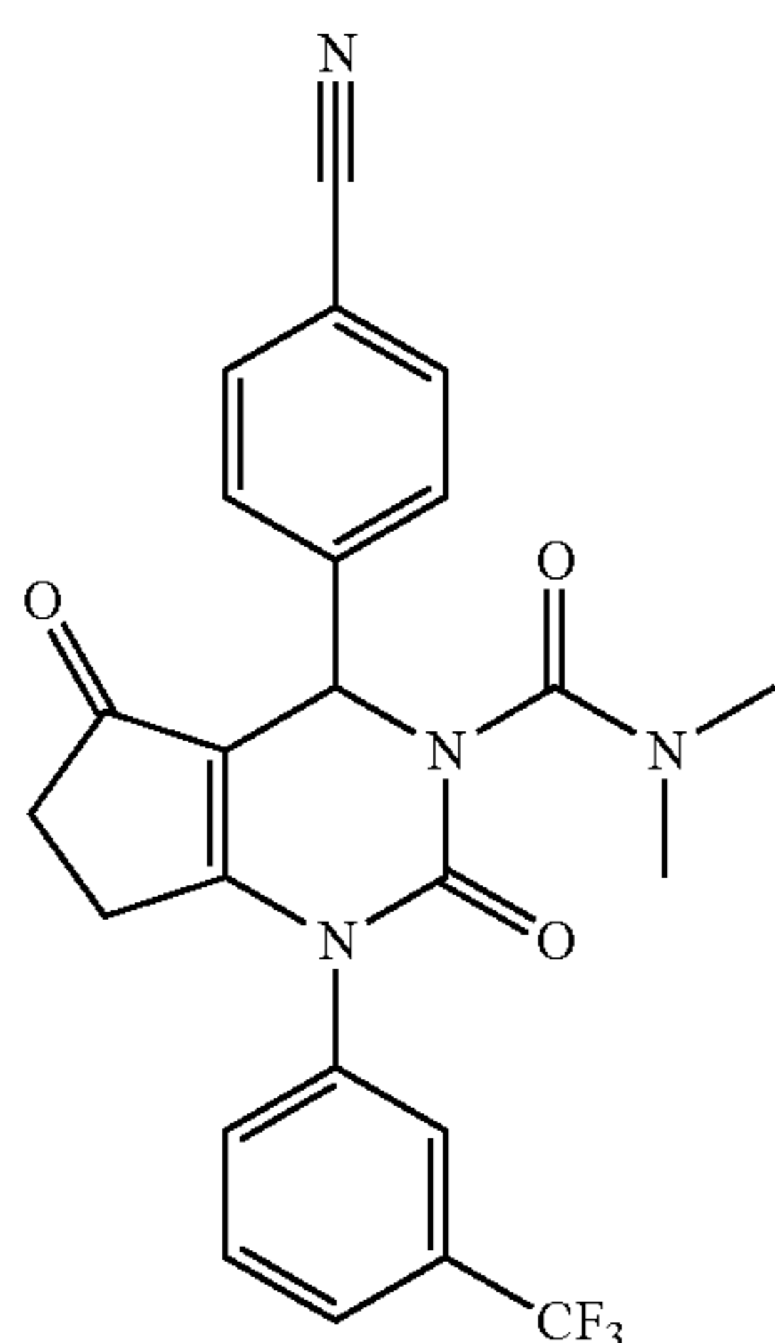
4-(4-Cyanophenyl)-N,N-dimethyl-2,5-dioxo-1-(3-(trifluoromethyl)phenyl)-4,5,6,7-tetrahydro-1H-cyclopenta[d]pyrimidine-3(2H)-carboxamide
