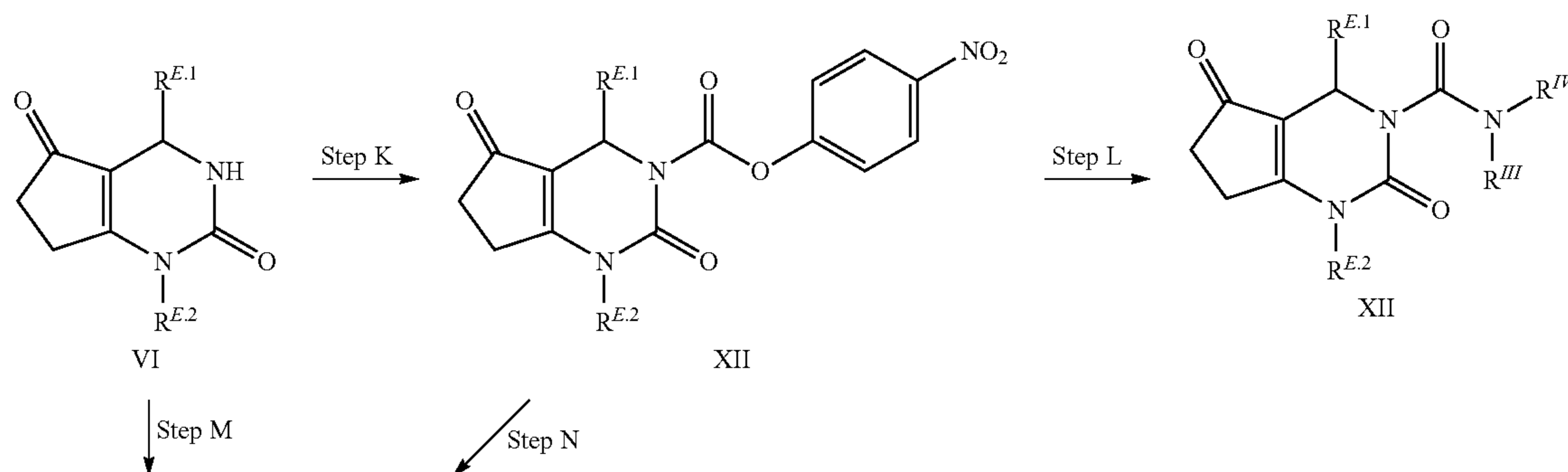
SCHEME 3
