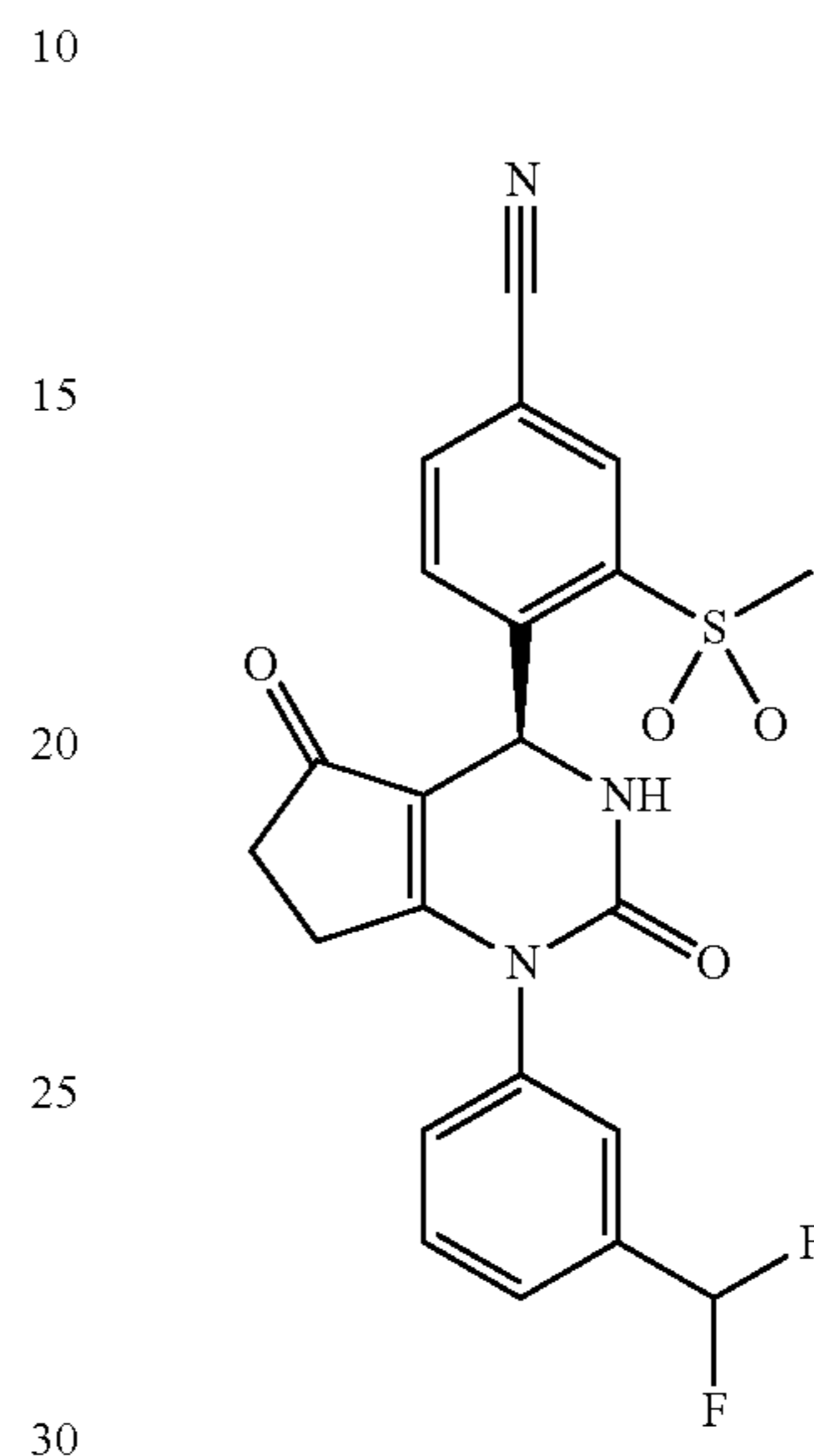
(S)-4-(1-(3-(Difluoromethyl)phenyl)-2,5-dioxo-2,3,4,5,6,7-hexahydro-1H-cyclopenta[d]pyrimidin-4-yl)-3-(methylsulfonyl)benzonitrile
