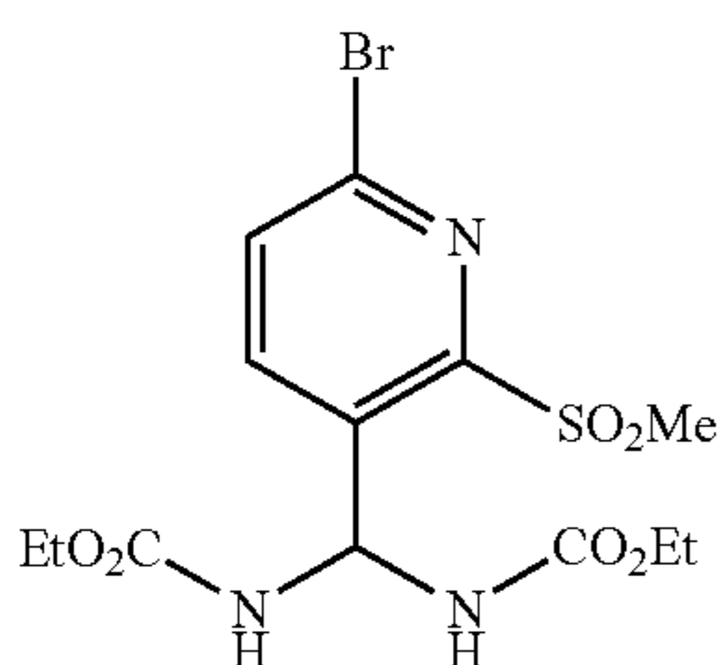
Diethyl(4-Bromo-2-methylsulfonylphenyl)methylenedicarbamate
