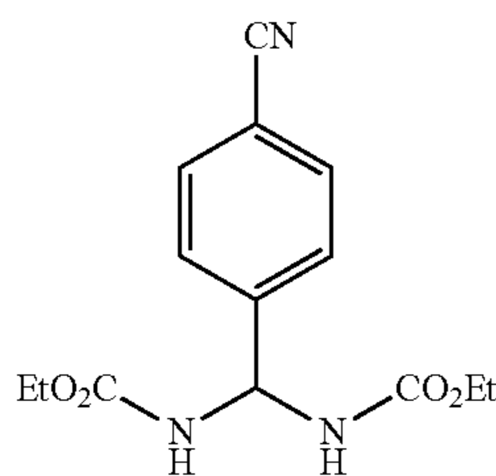
Diethyl(4-Cyanophenyl)methylenedicarbamate
