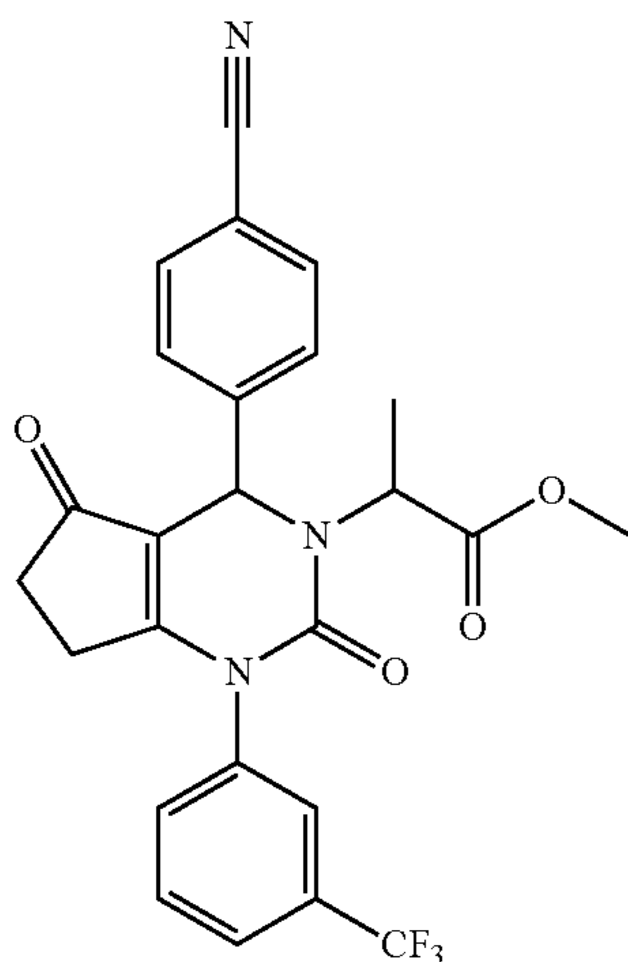
Methyl 2-(4-(4-Cyanophenyl)-2,5-dioxo-1-(3-(trifluoromethyl)phenyl)-6,7-dihydro-1H-cyclopenta[d]pyrimidin-3(2H,4H,5H)-yl)propanoate
