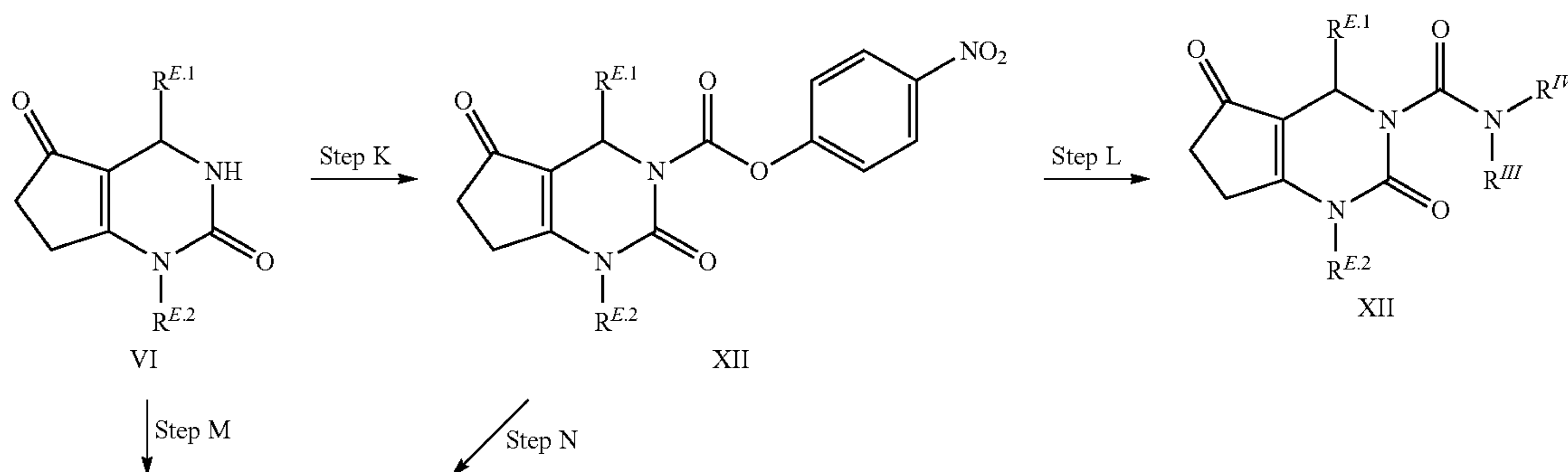
SCHEME 3
