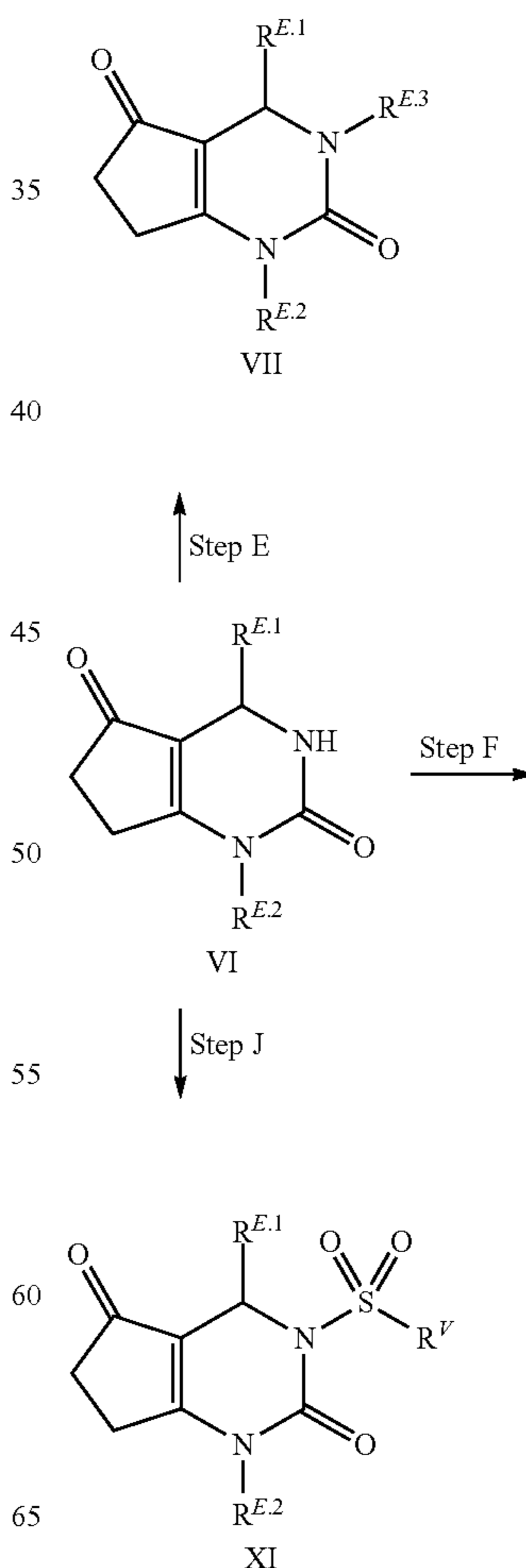
SCHEME 2
