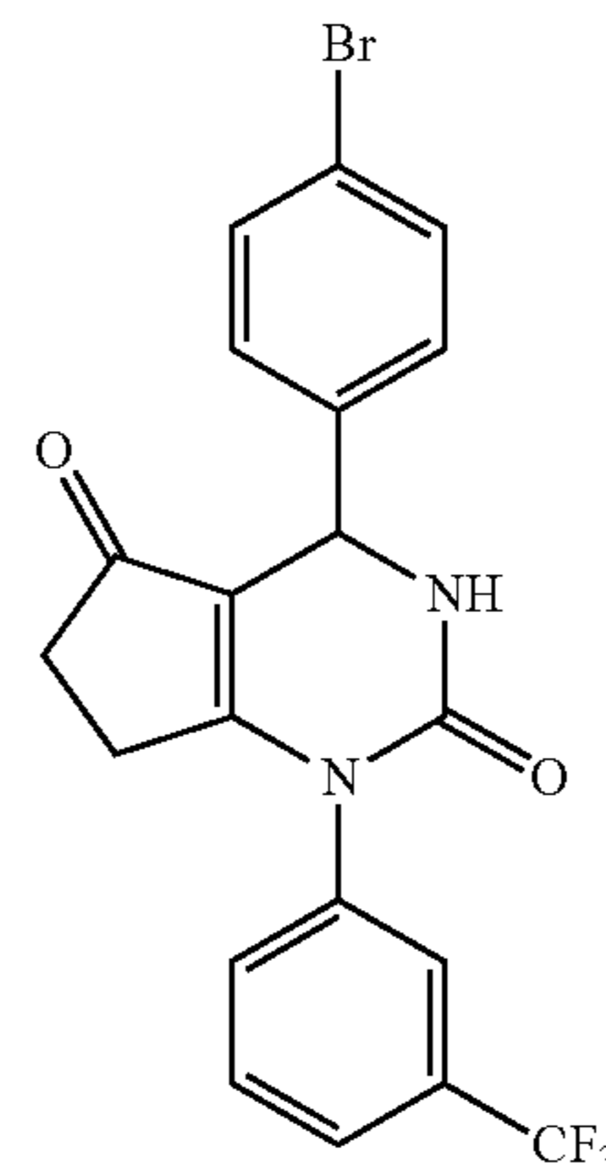
4-(4-Bromophenyl)-1-(3-(trifluoromethyl)phenyl)-3,4,6,7-tetrahydro-1H-cyclopenta[d]pyrimidine-2,5-dione
