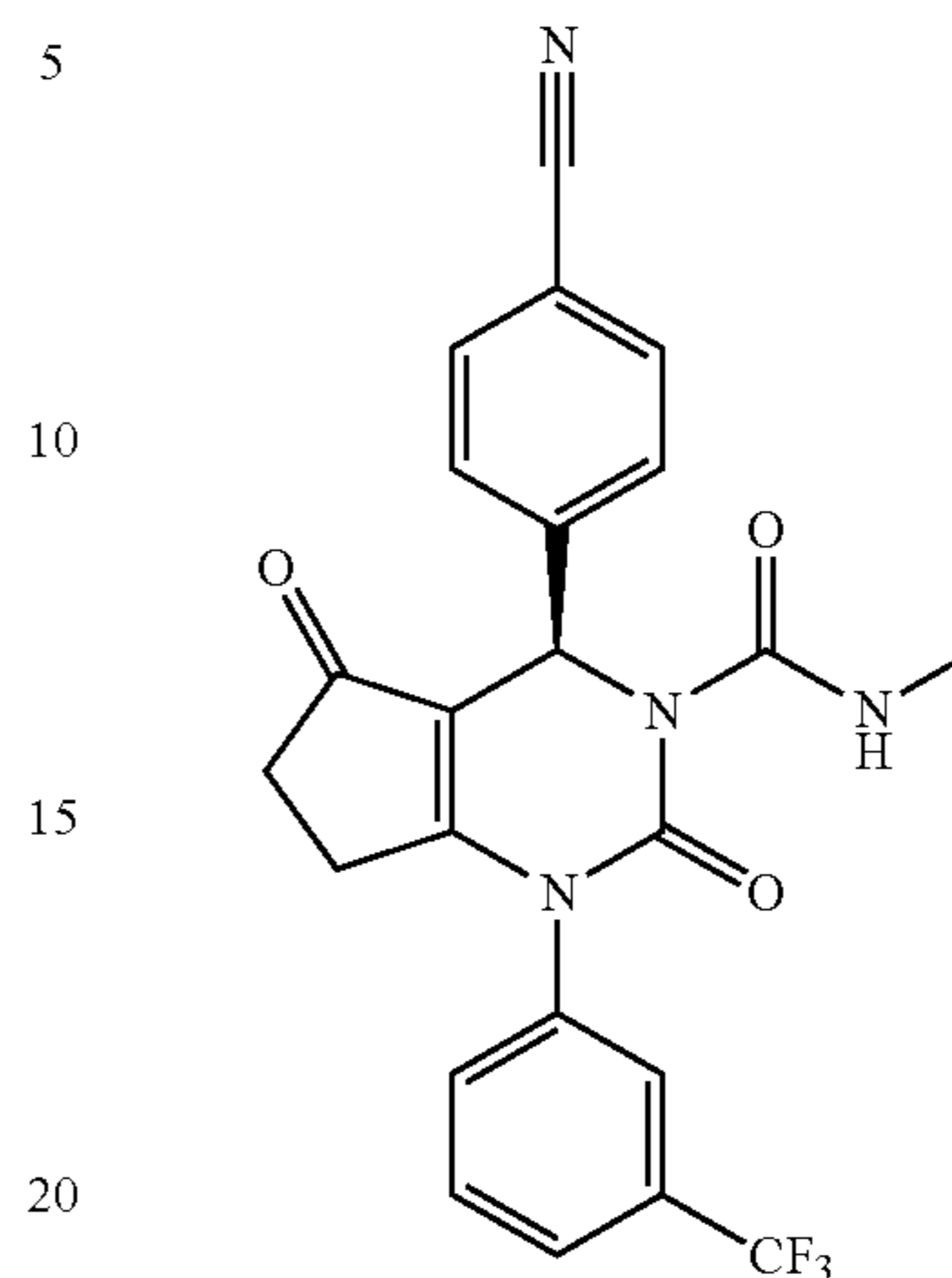
(R)-4-(4-Cyanophenyl)-N-methyl-2,5-dioxo-1-(3-(trifluoromethyl)phenyl)-4,5,6,7-tetrahydro-1H-cyclopenta[d]pyrimidine-3(2H)-carboxamide
