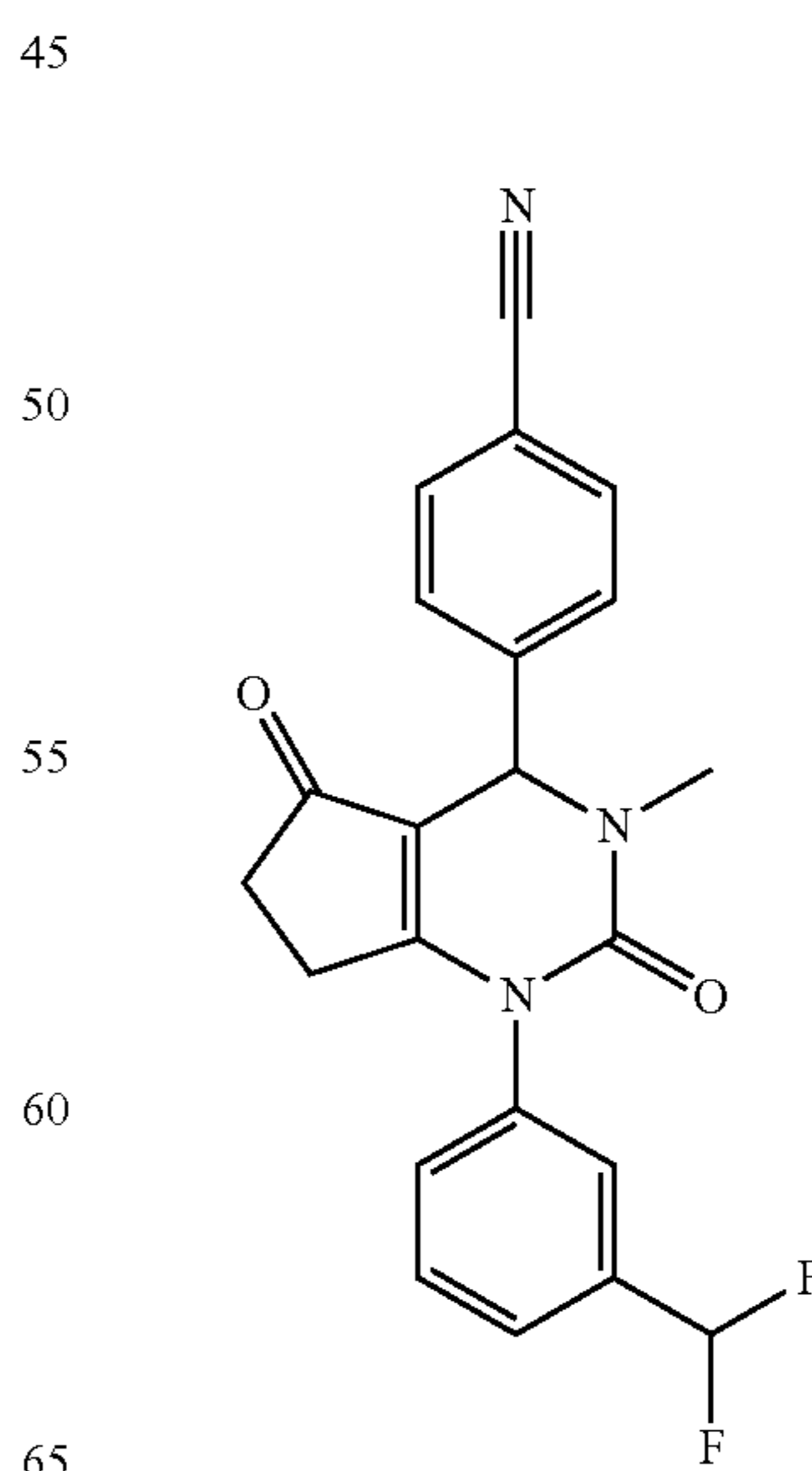
Example 26
