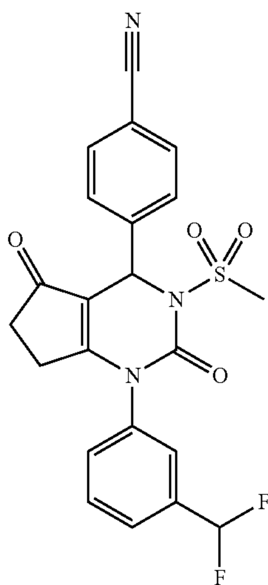
4-(1-(3-(Difluoromethyl)phenyl)-3-(methylsulfonyl)-2,5-dioxo-2,3,4,5,6,7-hexahydro-1H-cyclopenta[d]pyrimidin-4-yl)benzonitrile
