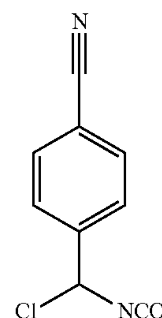
4-(Chloro(isocyanato)methyl)benzotrile
