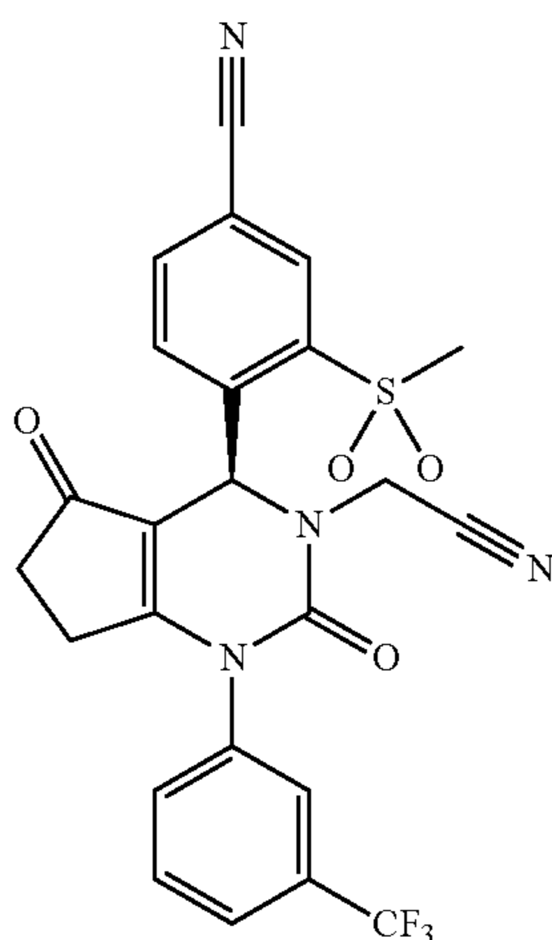
(S)-4-(3-(Cyanomethyl)-2,5-dioxo-1-(3-(trifluoromethyl)phenyl)-2,3,4,5,6,7-hexahydro-1H-cyclopenta[d]pyrimidin-4-yl)-3-(methylsulfonyl)benzonitrile
