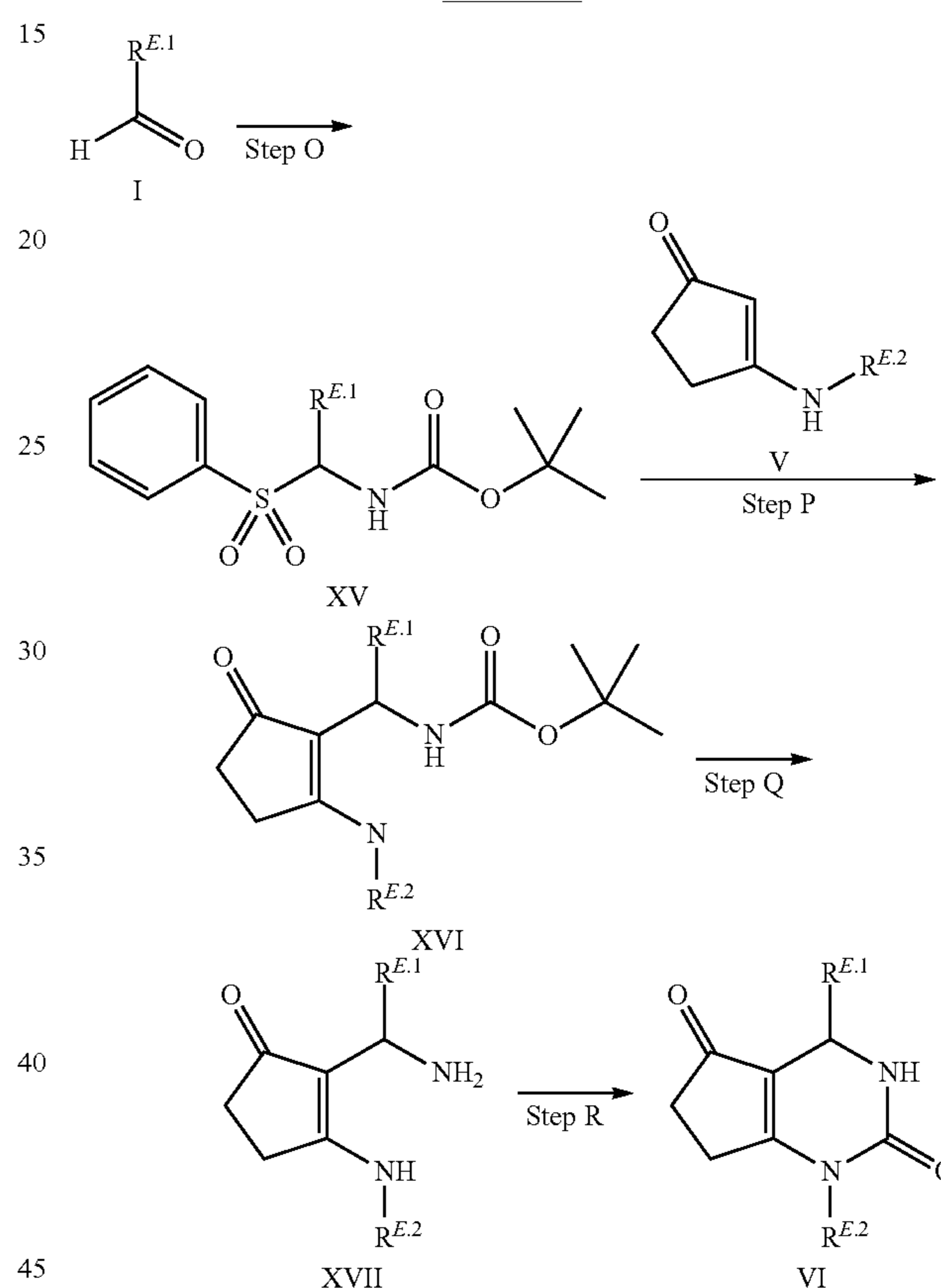
SCHEME 4
