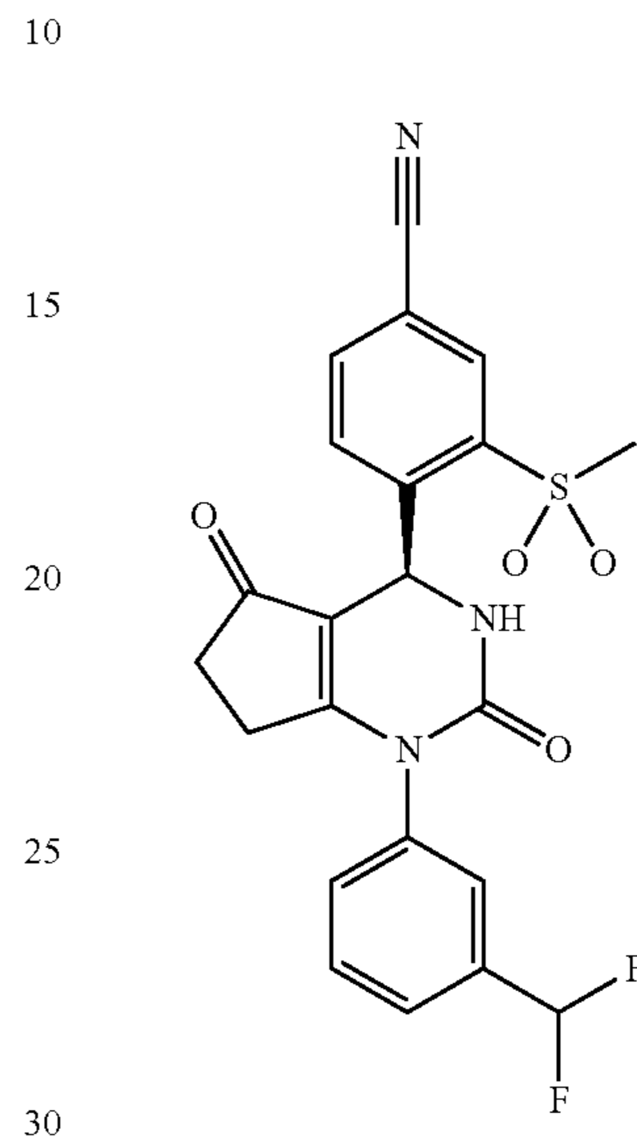
(S)-4-(1-(3-(Difluoromethyl)phenyl)-2,5-dioxo-2,3,4,5,6,7-hexahydro-1H-cyclopenta[d]pyrimidin-4-yl)-3-(methylsulfonyl)benzonitrile
