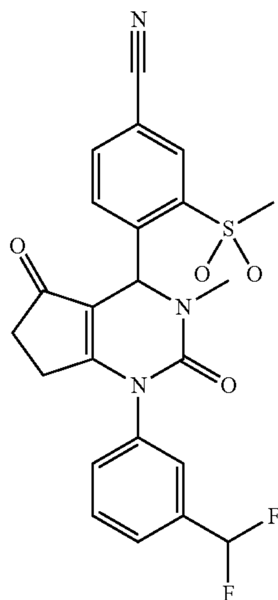
4-(1-(3-(Difluoromethyl)phenyl)-3-methyl-2,5-dioxo-2,3,4,5,6,7-hexahydro-1H-cyclopenta[d]pyrimidin-4-yl)-3-(methylsulfonyl)benzonitrile
