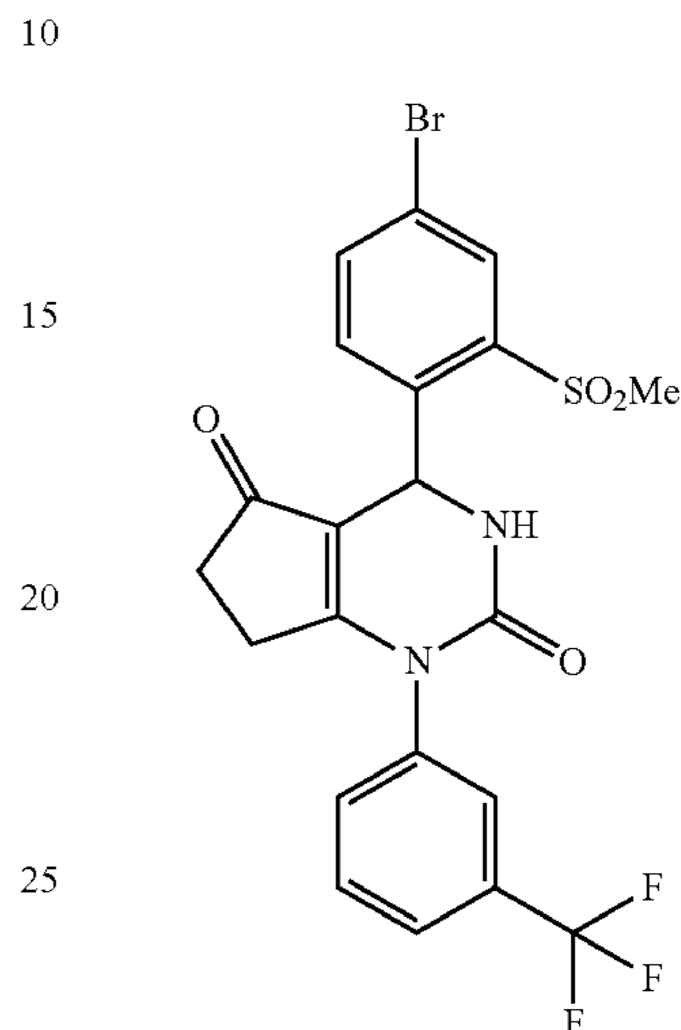
Intermediate 8
