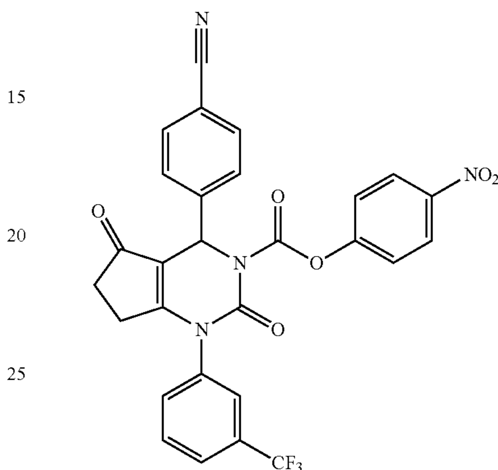
4-Nitrophenyl 4-(4-Cyanophenyl)-2,5-dioxo-1-(3-(trifluoromethyl)phenyl)-4,5,6,7-tetrahydro-1H-cyclopenta[d]pyrimidine-3(2H)-carboxylate
