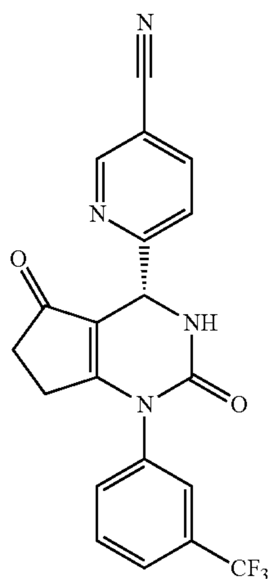
(R)-6-(2,5-Dioxo-1-(3-(trifluoromethyl)phenyl)-2,3,4,5,6,7-hexahydro-1H-cyclopenta[d]pyrimidin-4-yl)nicotinonitrile
