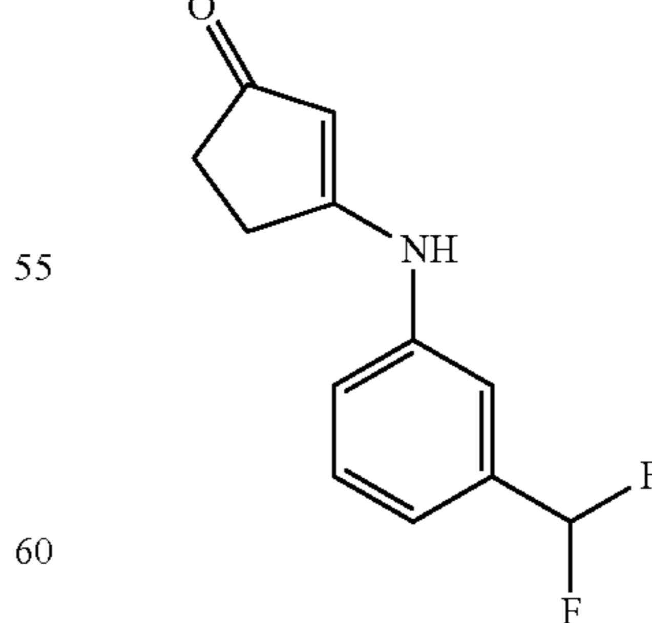
3-(3-(Difluoromethyl)phenylamino)cyclopent-2-enone
