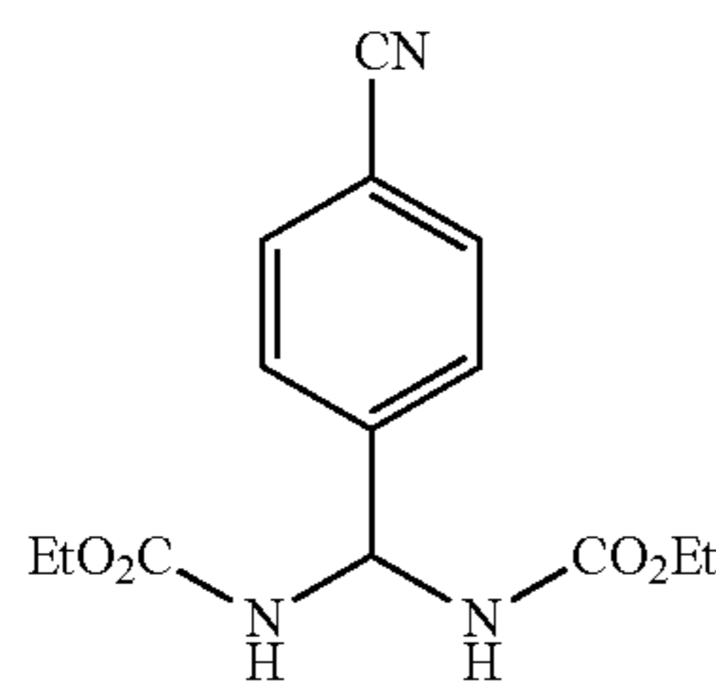
Diethyl(4-Cyanophenyl)methylenedicarbamate
