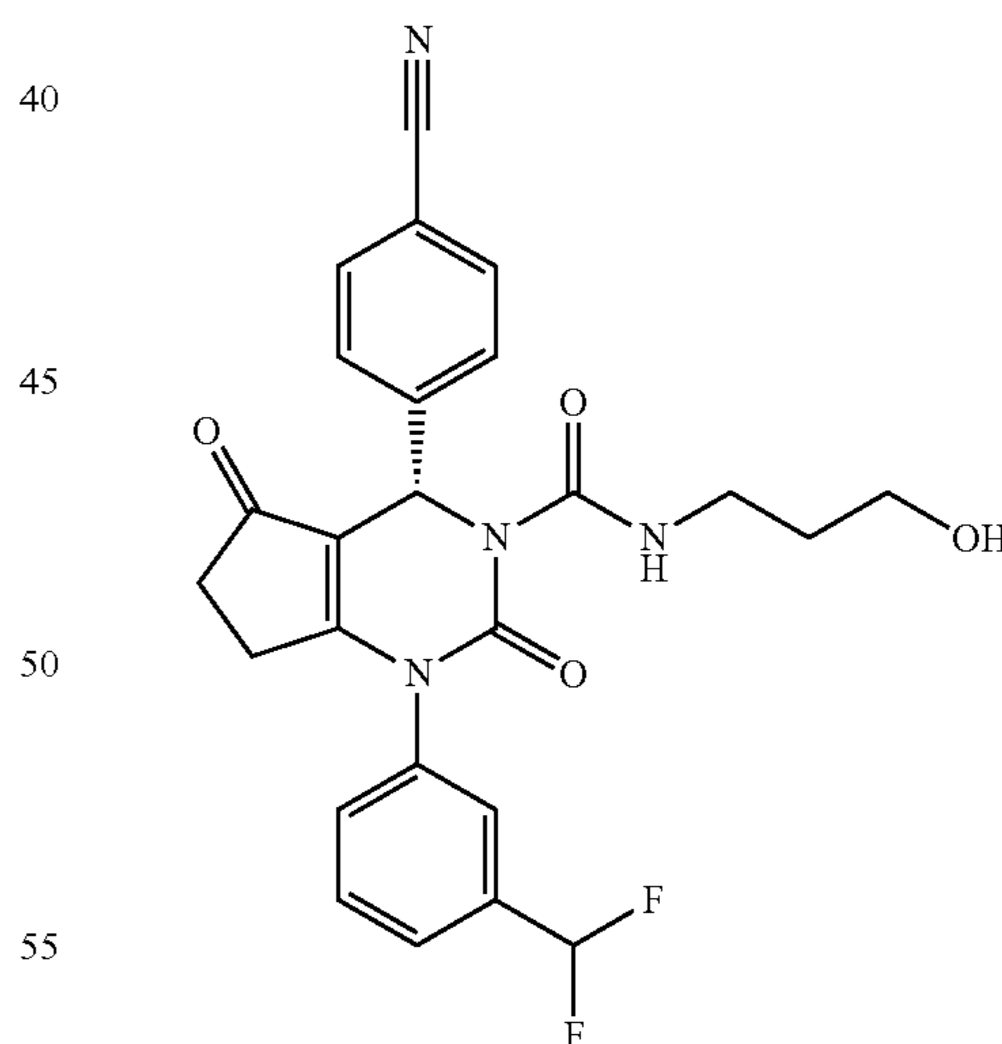
(S)-4-(4-Cyanophenyl)-1-(3-(difluoromethyl)phenyl)-N-(3-hydroxypropyl)-2,5-dioxo-4,5,6,7-tetrahydro-1H-cyclopenta[d]pyrimidine-3(2H)-carboxamide
