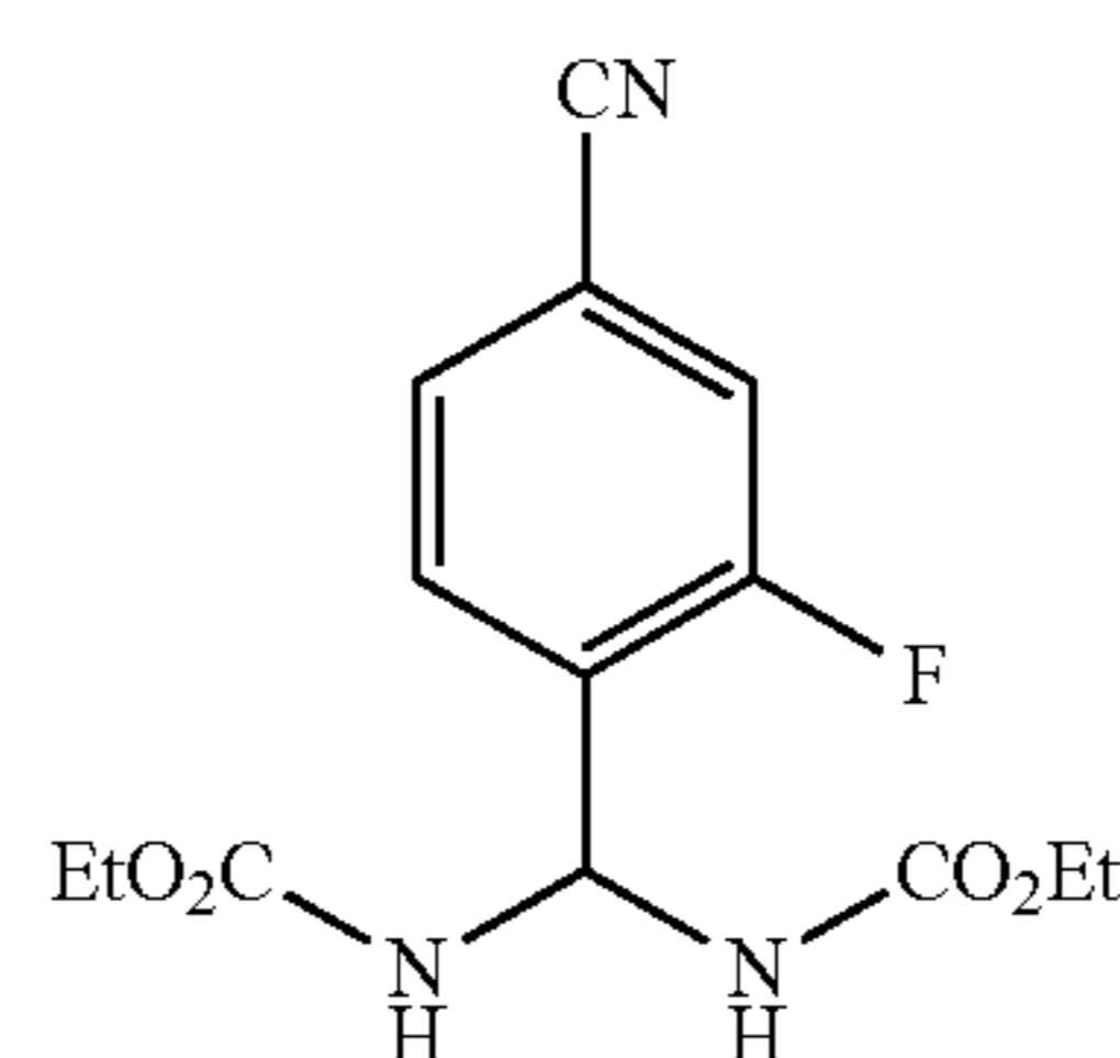
Diethyl(4-Cyano-2-fluorophenyl)methylenedicar- bamate
