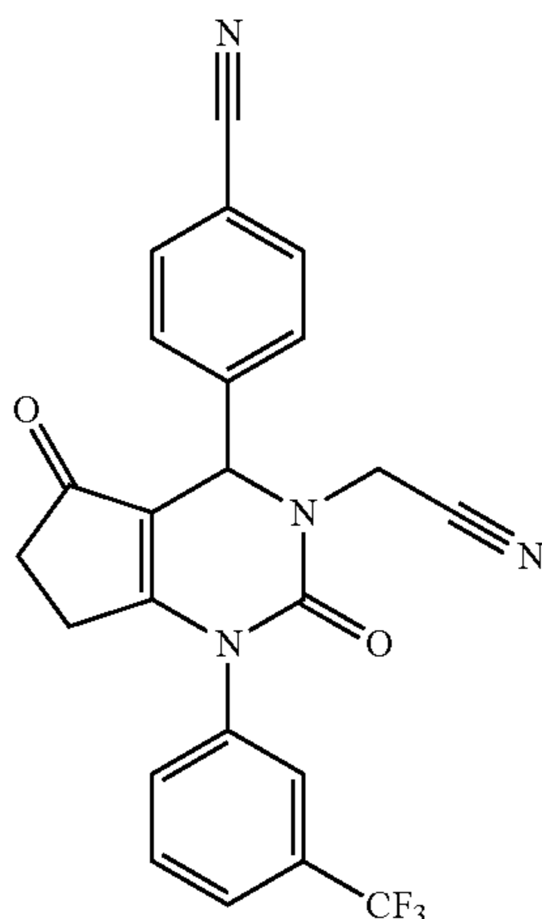
4-(3-(Cyanomethyl)-2,5-dioxo-1-(3-(trifluoromethyl)phenyl)-2,3,4,5,6,7-hexahydro-1H-cyclopenta[d]pyrimidin-4-yl)benzonitrile
